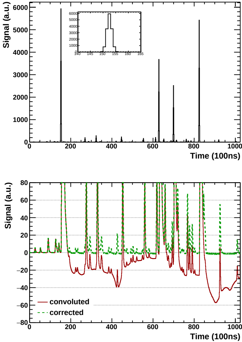
Figure 3.22.: Toy simulation of a single pad read-out. Top: input signal. Bottom: Convoluted (red solid line) and corrected (dashed green line) signals.
