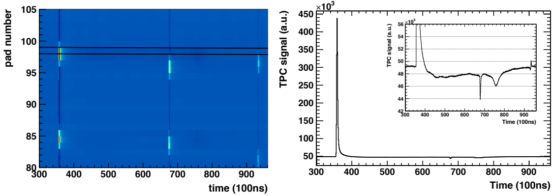
Figure 3.3.: Typical laser signal integrated over 1000 laser events. Non-zero-suppressed TPC signals for 25 pads are shown in the left plot, where the two solid horizontal black lines indicate the pad whose signal is shown in the right. The ion-tail (zoom into signal (y) axis) structure of the main pulse is shown as the inset of the right plot.
