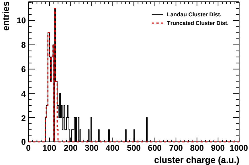
Figure 4.6.: Toy simulation of a given track's charge distribution, which has a Landau shape (black solid line) and the charge distribution after the truncated mean procedure (red dotted line).
