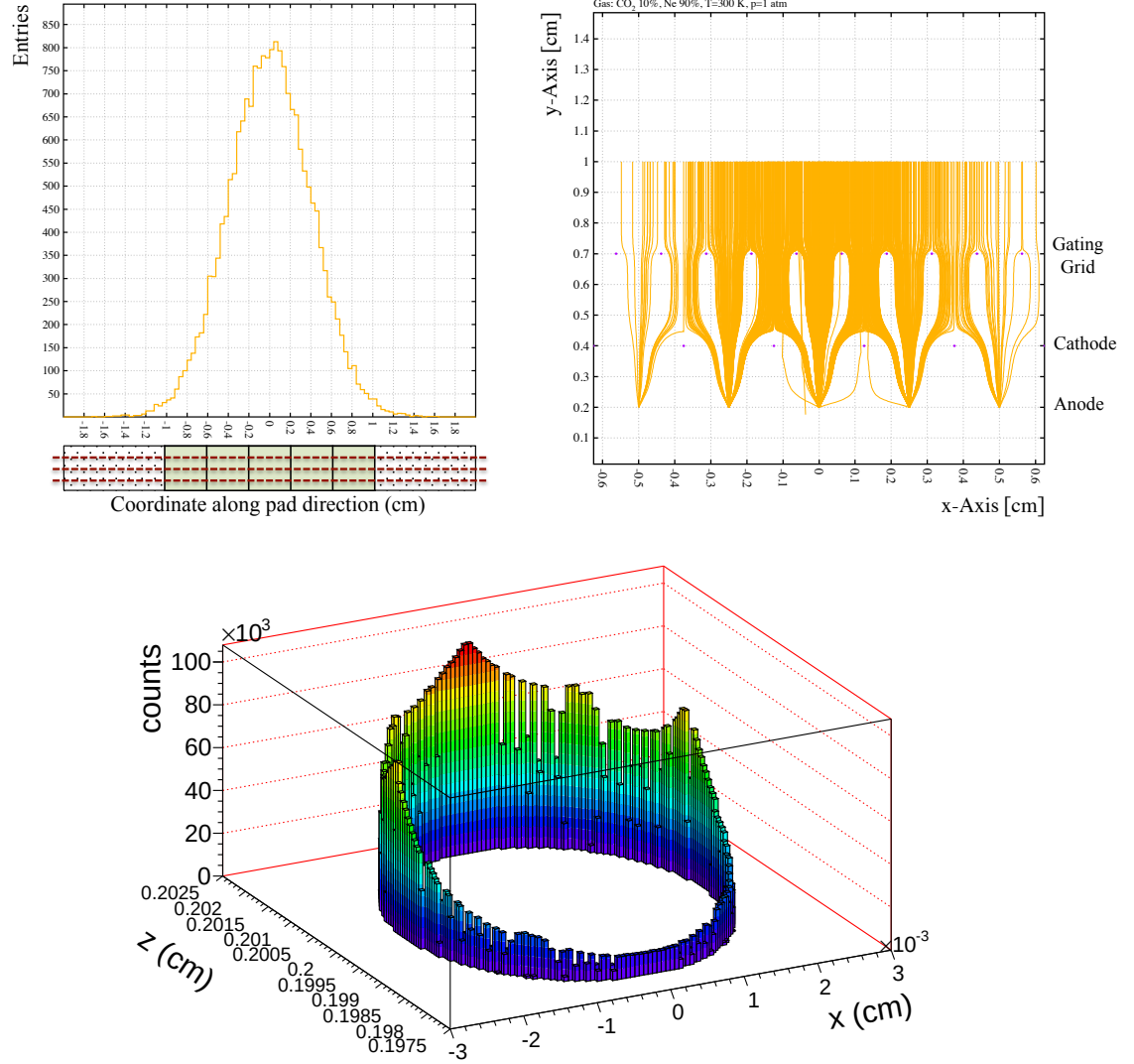
Figure 3.13.: (Upper panel:Left) Distribution of ions along the anode wires with the shape of the TPC PRF. The parameters of the PRF are taken from the OCDB. (Upper panel: Right) Drift lines of electrons in the amplification region (without diffusion), where the primary electrons are assumed to be distributed with a Gaussian shape. (Lower panel) Distribution of ions around the anode wire at the start of drift.
