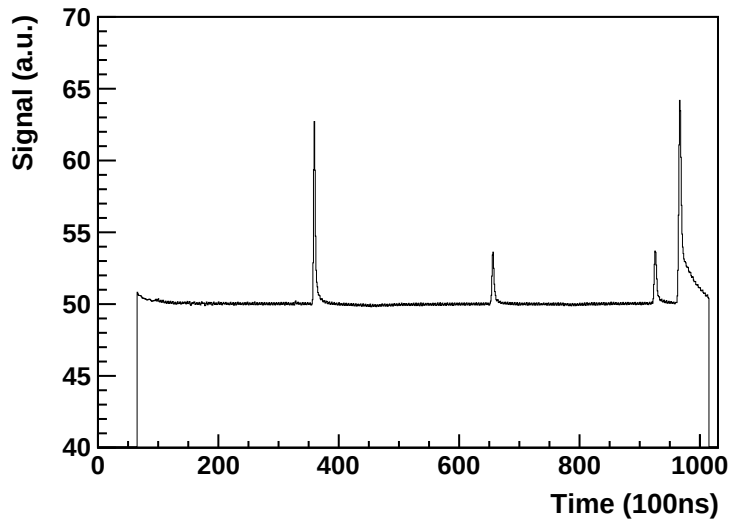
Figure 3.1.: A non-zero-suppressed TPC laser signal from a single pad.
