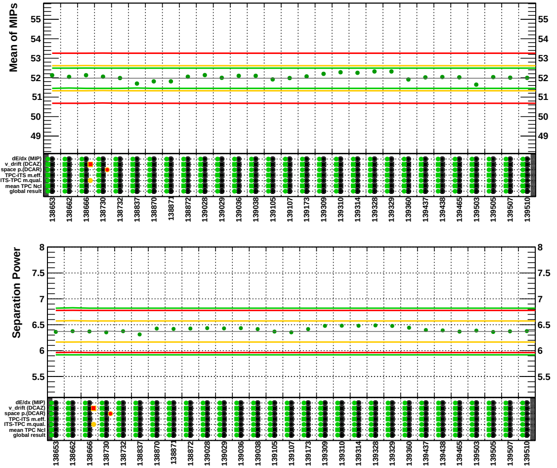
Figure 2.18.: (Top) Mean dE/dx signal for minimum-ionizing pions and (Bottom) separation power between electrons and minimum-ionizing pions measured in the TPC for the first runs of the 2010 Pb–Pb data taking.
