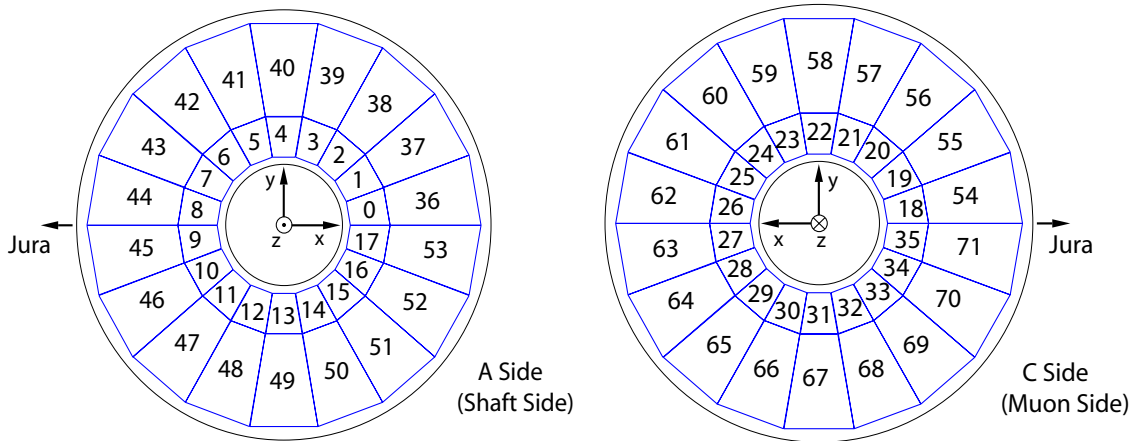
Figure 2.3.: Numbering of the 72 ROCs in the offline code [53].
