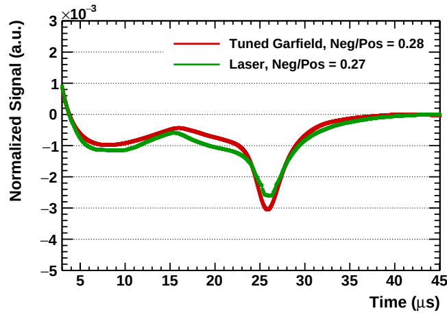
Figure 3.15.: (Color Online) Comparison of the normalized pad signal to the Garfield simulations in Ne-CO 2 (90-10) gas mixture for the most central pad of a cluster. Simulation result is scaled to match the measured ion drift velocity, and also smeared taking the fluctuations of the wire positions into account.
