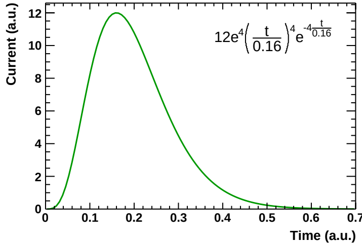
Figure 2.7.: Shaping function used in the FEE.
