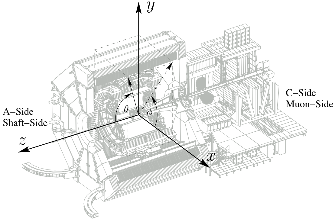
Figure B.1.: Sketch of the ALICE global coordinate system [94, 95].
