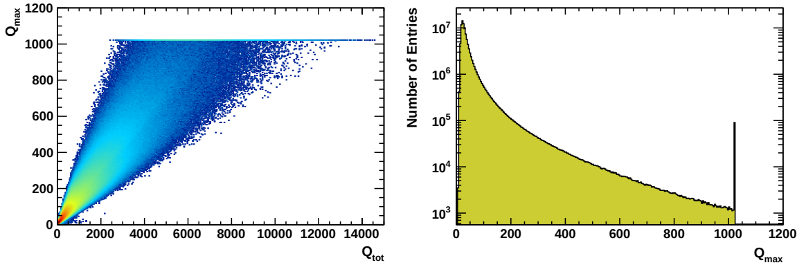
Figure 3.23.: (Left) Total vs maximum charge of TPC clusters. (Right) Distribution of the maximum charge of TPC clusters.
