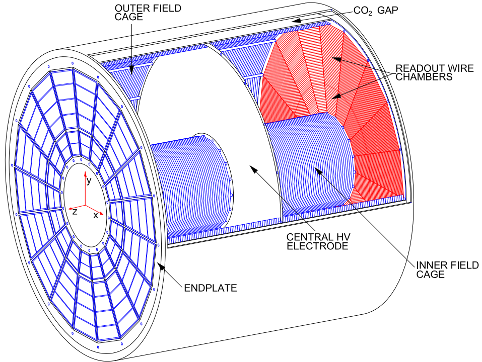
Figure 2.2.: Layout of the TPC [50].
