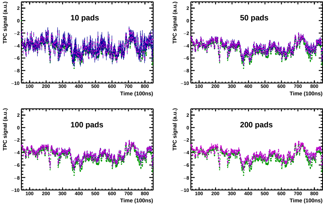
Figure 3.32.: (Color Online) Reference baseline (green points) of a given pad signal with common-mode effect in comparison to the estimated baselines (magenta points) where a different number of pads is used for the estimation.
