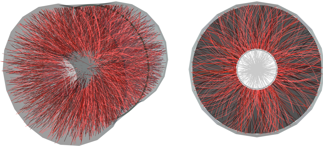
Figure 2.13.: Reconstructed TPC and ITS tracks in a Pb–Pb event at \sqrt{s_{\text{NN}}} = 2.76 TeV. TPC and ITS tracks are shown in red and light grey, respectively.
