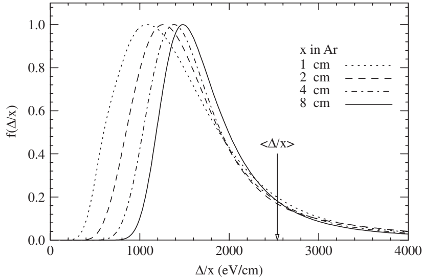
Figure 2.15.: Calculated straggling functions f(\Delta/x) (note that \Delta/x is equivalent to dE/dx ) for \beta\gamma=3.6 particles (MIPs), traversing layers of Argon in different widths [64].
