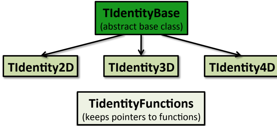
Figure H.1.: Schematic diagram of the Identity Method code.
