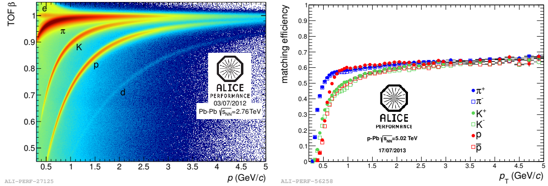
Figure G.2.: (Left) Track velocity \beta vs p from TOF in Pb–Pb collisions. The bands for e , \pi , K , p and d are clearly visible. Particles outside of these bands are tracks wrongly associated with a TOF signal. (Right) The efficiency of matching TPC tracks to TOF for pions, kaons and protons in p–Pb collisions.
