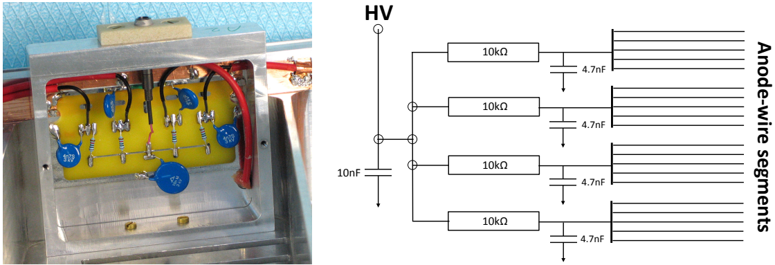
Figure 3.19.: Picture (Left) and diagram (Right) of an electric circuit of an IROC [61, 70].
