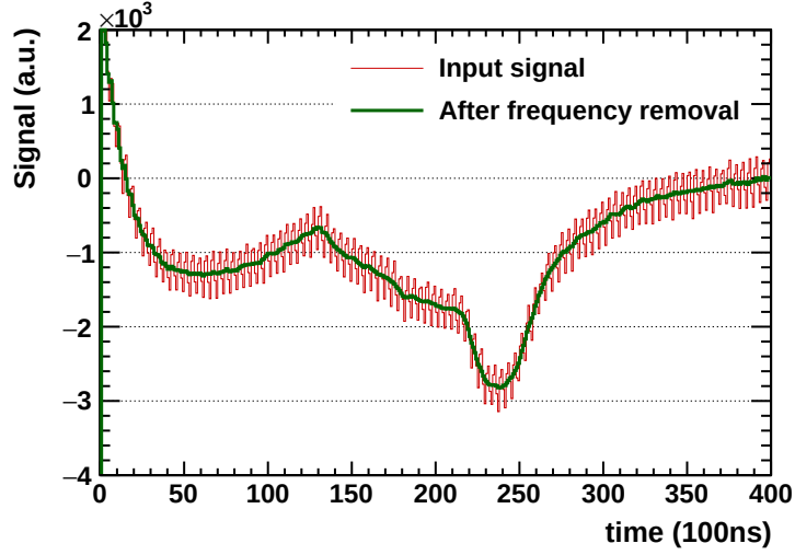
Figure 3.5.: (Color Online) The ion-tail signal before (red solid line) and after (green solid line) the removal of the high frequencies.
