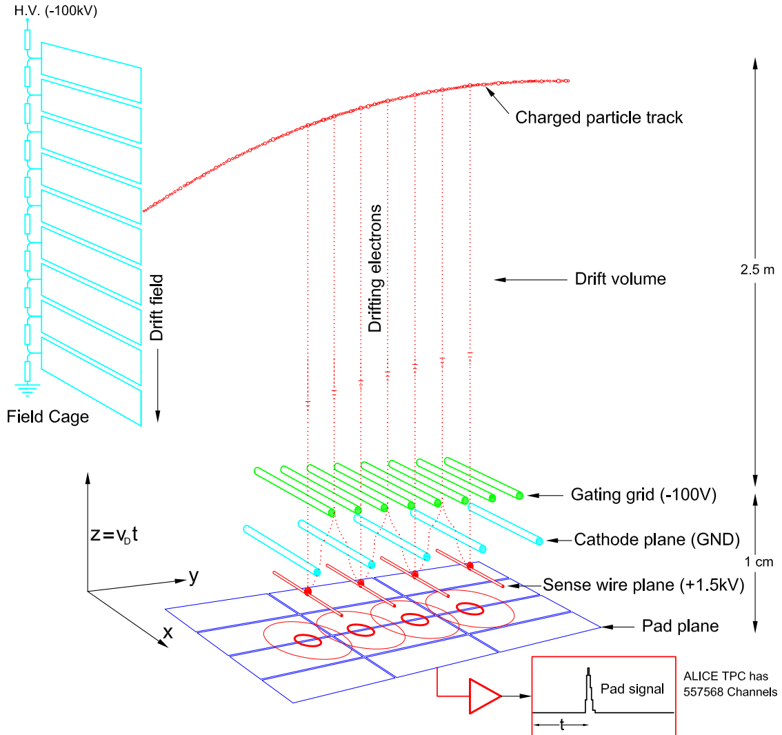
Figure 2.10.: Schematic illustration of the working principle of TPC [61].
