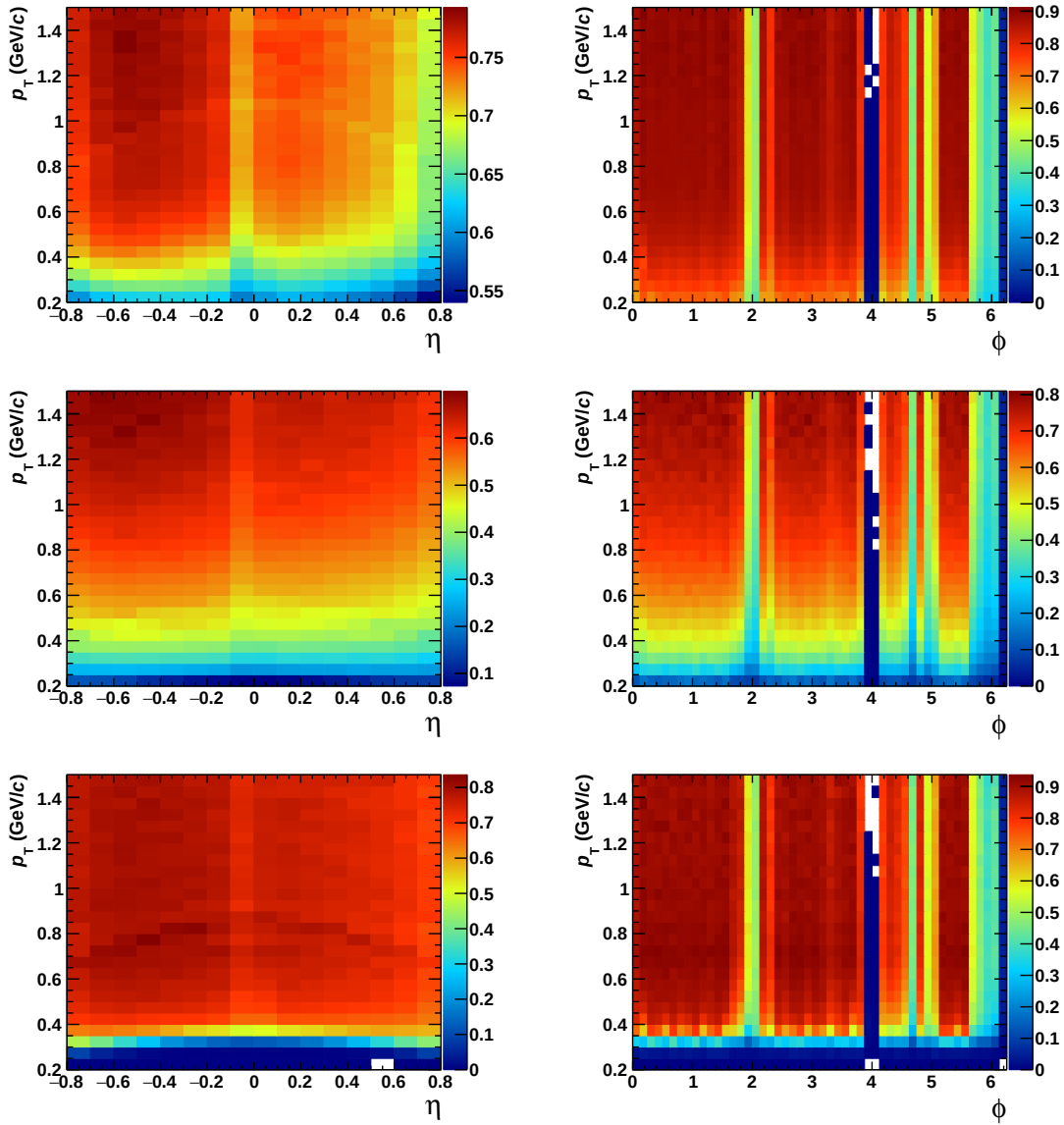
Figure I.1.: Single particle detection efficiencies for pions (first row), kaons (second row) and protons (third row). Efficiencies are shown as a function of transverse momentum vs pseudorapidity (first column) and transverse momentum vs azimuthal angle (second column).
