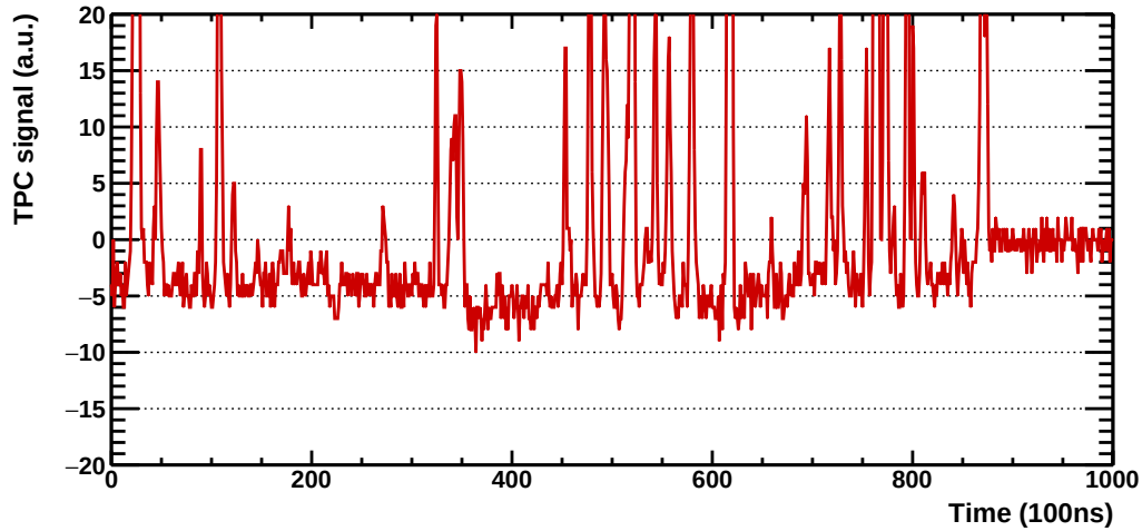
Figure 3.26.: Simulation of a pad signal for a central event where only the common-mode effect is implemented.
