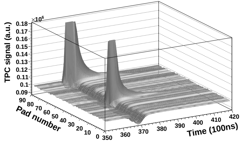
Figure 3.16.: Integrated laser track signal on a given pad-row which illustrates the common-mode effect.
