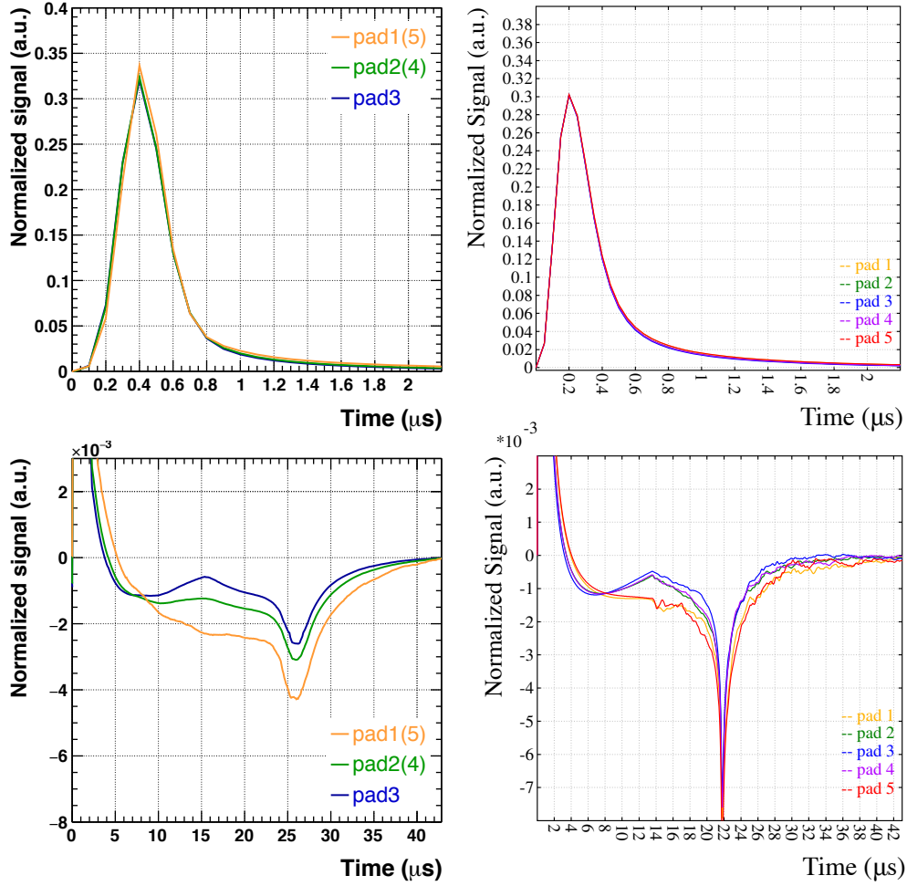
Figure 3.14.: Comparison of the measured and simulated signal shapes in five pads of a cluster where pad number 3 is the center of the cluster. Upper panel: Pulse shape. Lower panel: Ion-tail. Left: data. Right: Garfield simulation.
