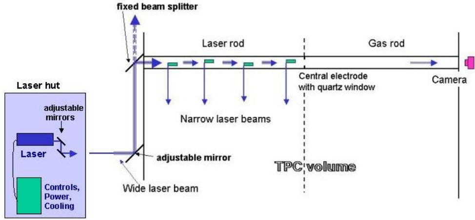
Figure E.2.: Principle of generating narrow laser rays in the TPC volume [60].
