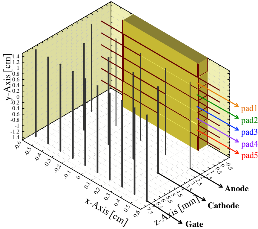
Figure 3.12.: Three dimensional setup of the TPC pad read-out used in the Garfield simulations.
