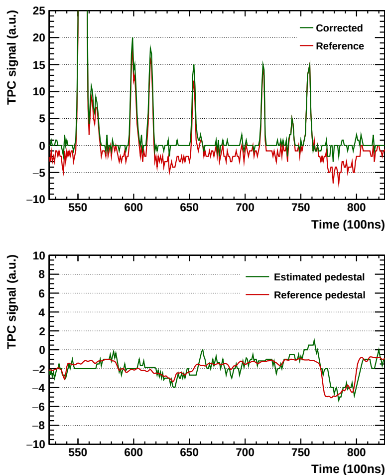
Figure 3.30.: (Upper plot) Pad signal before (red line) and after (green line) the online correction. (Lower plot) Comparison of the corresponding baseline (signals removed) of the pad signal with common-mode effect (red line) to the estimated baseline (green line).
