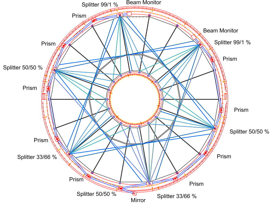
Figure E.3.: Ideal laser tracks in (r, \varphi) in the TPC drift volume, projected to the end-cap. The pattern repeats eight times through the full length of the TPC. [50].
