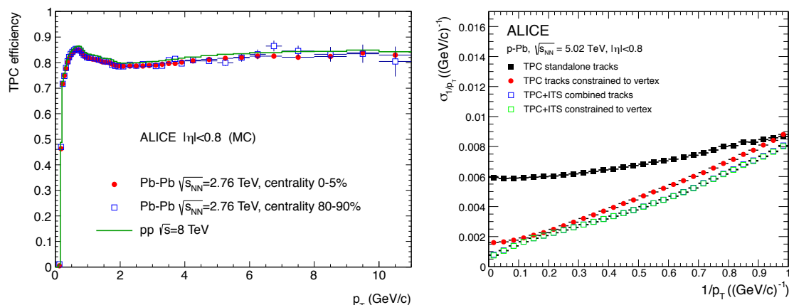
Figure 2.17.: (Left) TPC track finding efficiency for primary particles in pp and Pb–Pb collisions (simulation). (Right) The p_T resolution measured in p–Pb collisions for standalone TPC and ITS–TPC matched tracks with and without constraint to the vertex [66].
