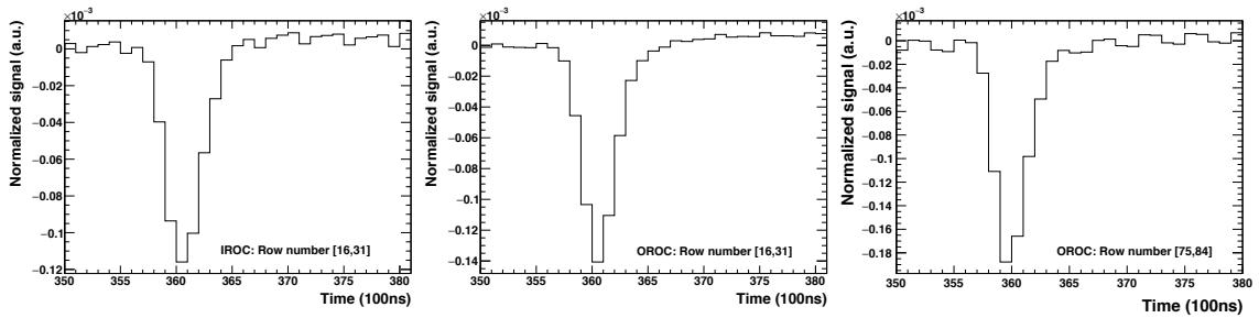
Figure 3.17.: Normalised common-mode response functions for three different pad-size regions: IROC (left), inner OROC (middle) and outer OROC (right).
