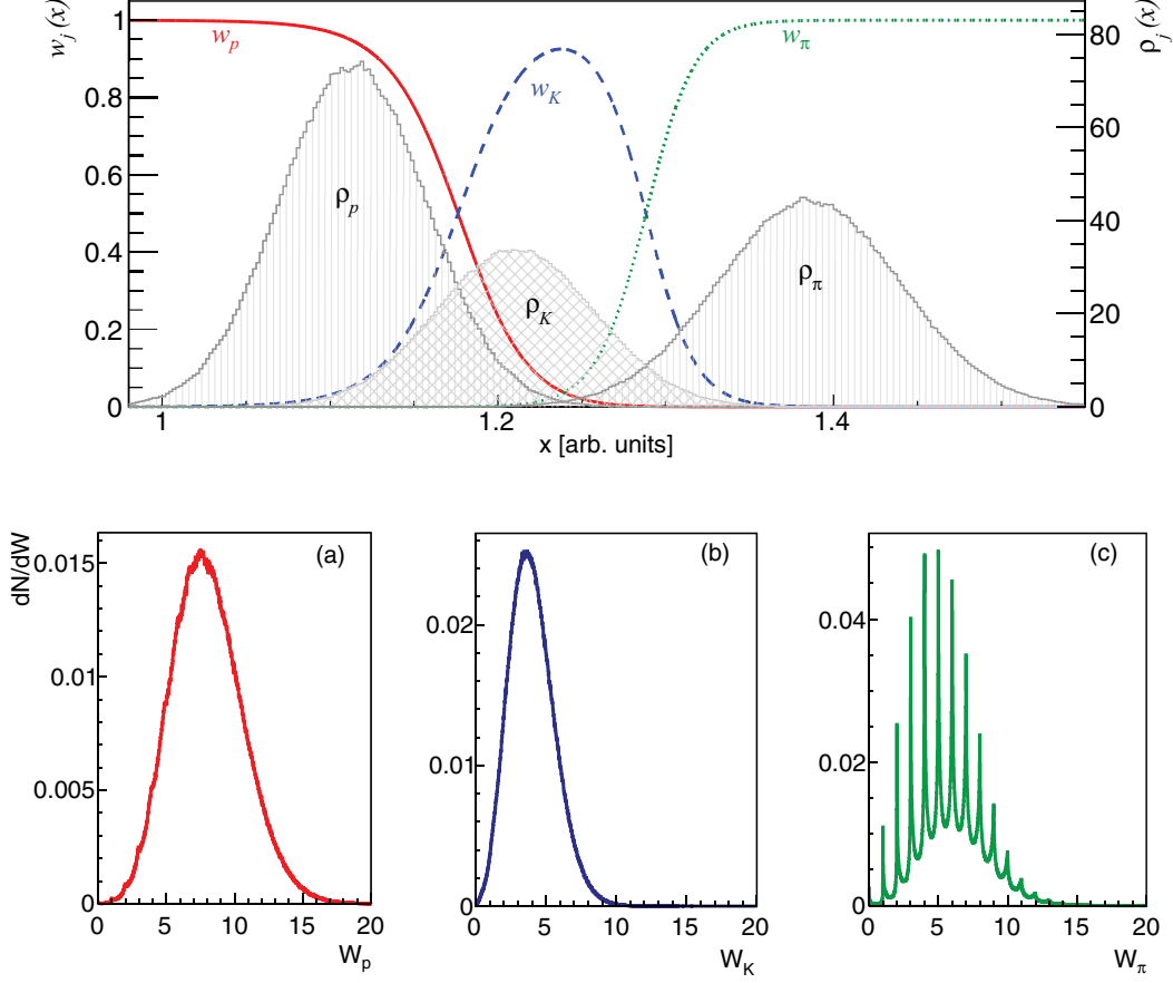
Figure 1.8.: A toy simulation of particle energy loss for pions, kaons and protons where unique particle identification is impossible. Upper panel: The inclusive distribution \rho_j(x) of the particle identification variable x for protons, kaons, and pions, used as an input to the simulation, are depicted with shaded histograms. The distributions of identities \omega_j(x) for protons, kaons, and pions are presented with red solid, blue dashed, and green dotted lines respectively. Lower panel: The distribution of event variables W_j with j standing for (a) protons, (b) kaons, and (c) pions.[34].
