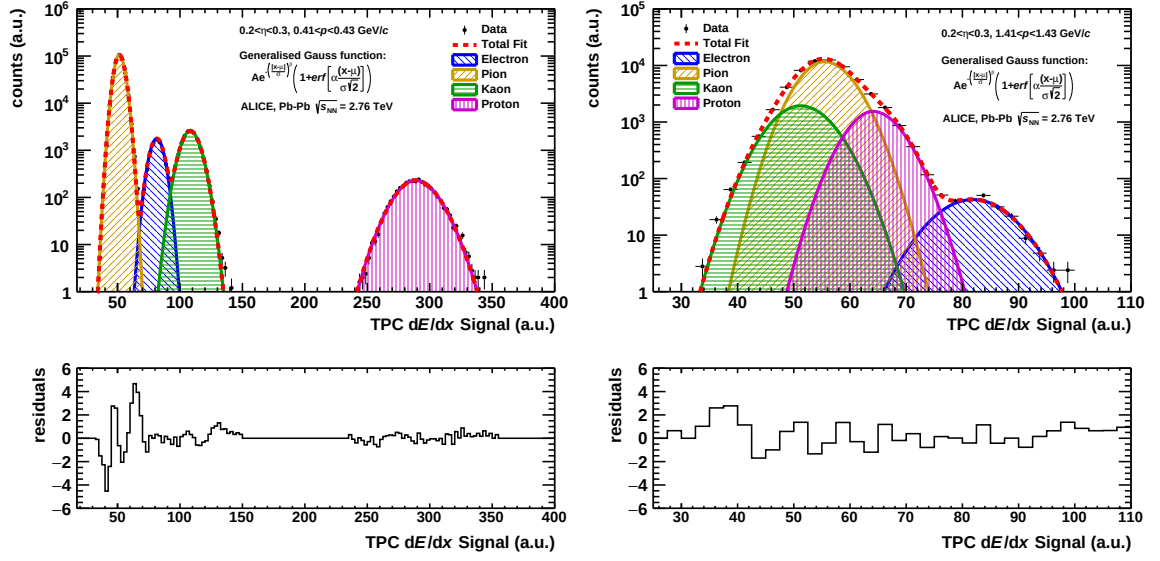
Figure 4.20.: (Upper panel) dE/dx distributions of pions, kaons, electrons and protons fitted with the generalized Gauss function in two different momentum intervals. (Lower panel) The corresponding residual plots.
