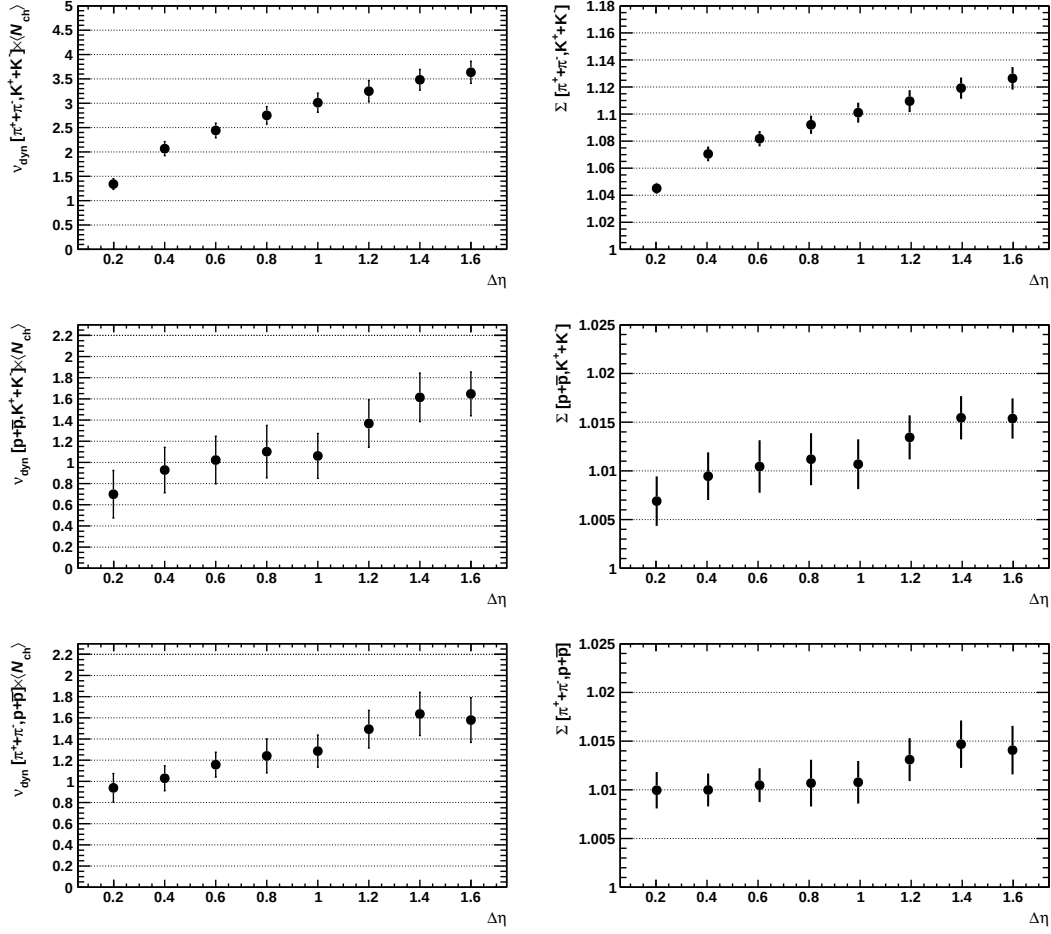
Figure 6.12.: \Delta\eta dependence of \Sigma results in comparison with the \nu_{\text{dyn}} results scaled by \langle N_{\text{ch}} \rangle .
