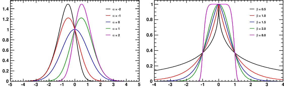
Figure 4.5.: Generalised Gauss function for different skewness ( \alpha ) parameters at fixed \beta = 2 (left) and for different kurtosis ( \beta ) parameters at fixed \alpha = 0 (right).
