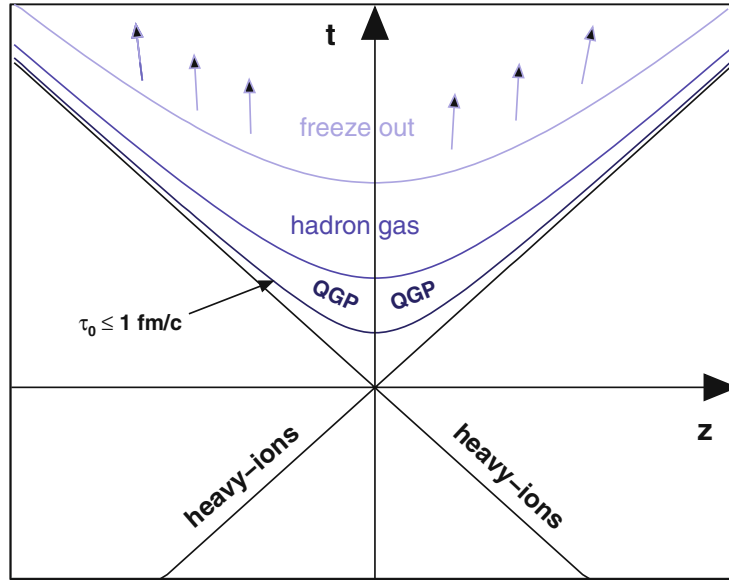
Figure 1.3.: Space-time diagram of a nucleus-nucleus collision, showing the various stages of the evolution of expanding matter [12].
