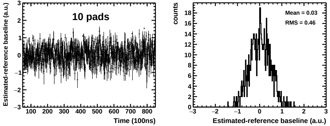
Figure 3.33.: (Left) Baseline of a pad signal with common-mode effect subtracted from the estimated baseline averaging over 10 pads. (Right) Projection of the left plot to the signal ( y ) axis.
