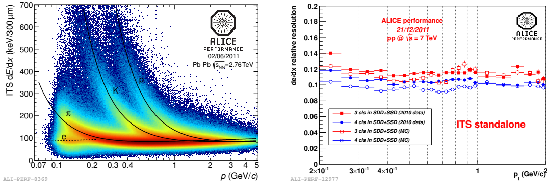
Figure G.1.: (Left) dE/dx of charged particles vs their momentum, measured by the ITS alone. The lines are a parametrization of the detector response based on the Bethe-Bloch formula. (Right) ITS standalone dE/dx resolution as function of p_T for pp at 7 TeV. Monte-Carlo and data are superimposed with different request on SDD+SSD clusters.
