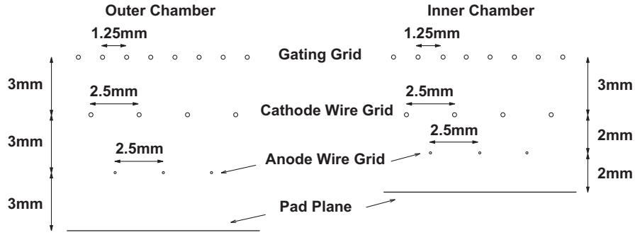
Figure 2.5.: Wire geometries of the outer and inner readout chambers [50].
