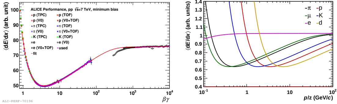
Figure 4.3.: (Left) Bethe-Bloch fit to the TPC dE/dx signal from various clean samples covering the different regions of the Bethe-Bloch curve. (Right) Typical Bethe-Bloch curves of the ionization signal as a function of particle momentum for different particle species. A parameterization like the one suggested in [63] is used to calculate the curves.
