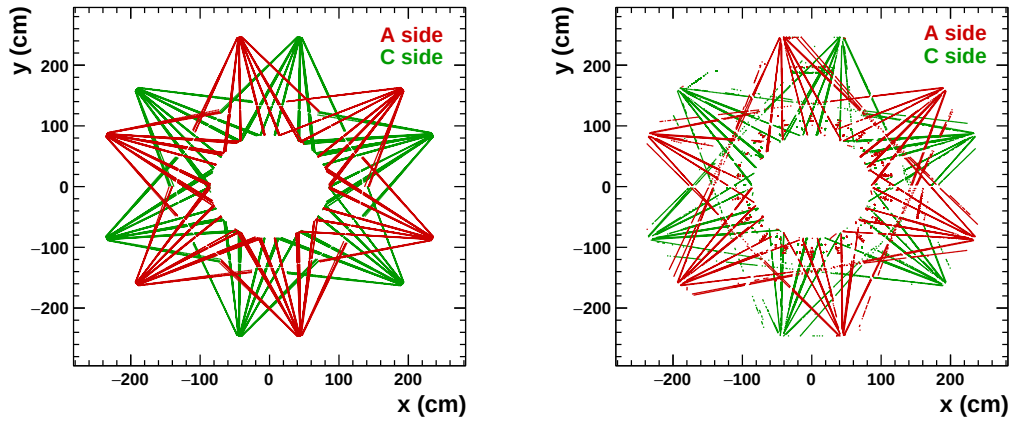
Figure 3.2.: (Left) Ideal laser track positions stored in the Offline Calibration Database (OCDB). (Right) Reconstructed clusters of the laser tracks read out in a stand-alone laser calibration run. The pattern repeats eight times through the full length of the TPC.
