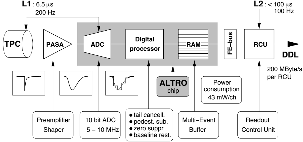
Figure 2.6.: Block diagram of the TPC front-end electronics [55].
