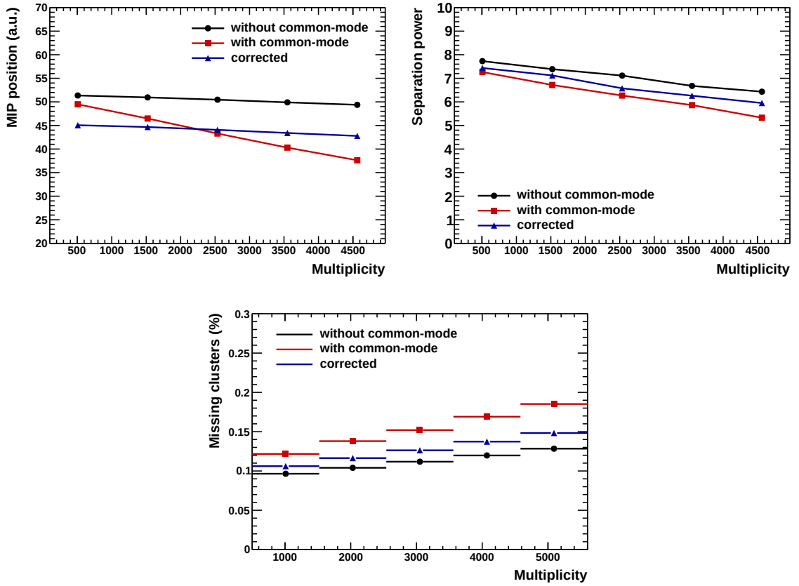
Figure 3.31.: Achieved performance in mean dE/dx position (top left), separation power (top right) and relative number of missing clusters (bottom) after the online correction applied to a HIJING simulation including the common-mode effect. Results are shown as a function of multiplicity.
