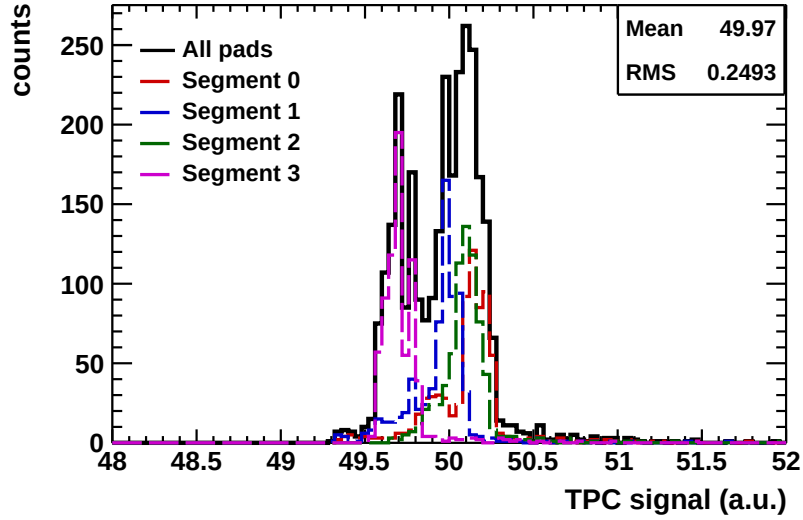
Figure 3.21.: Integrated charge of the four anode wire segments on a given IROC.
