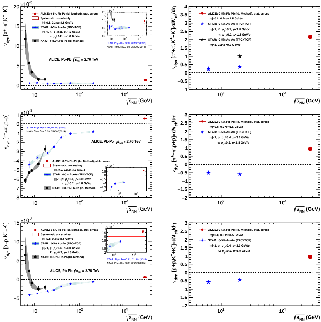
Figure 6.8.: Energy dependence of \nu_{\text{dyn}} with (right) and without (left) scaled by dN_{\text{ch}}/d\eta . ALICE results are shown as red solid circles. Results from the Identity Method for central Pb–Pb collisions from NA49 [28] are shown as black solid squares. Stars represent results from STAR [25] in central Au–Au collisions. STAR dN_{\text{ch}}/d\eta values are taken from [90] and data points on the top right plot with black and blue stars are taken from [89] and [25], respectively.
