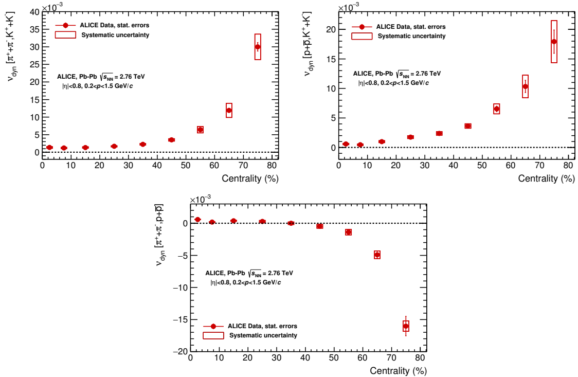
Figure 6.1.: Centrality dependence of the ALICE \nu_{\text{dyn}} results and the statistical and systematic uncertainties.
