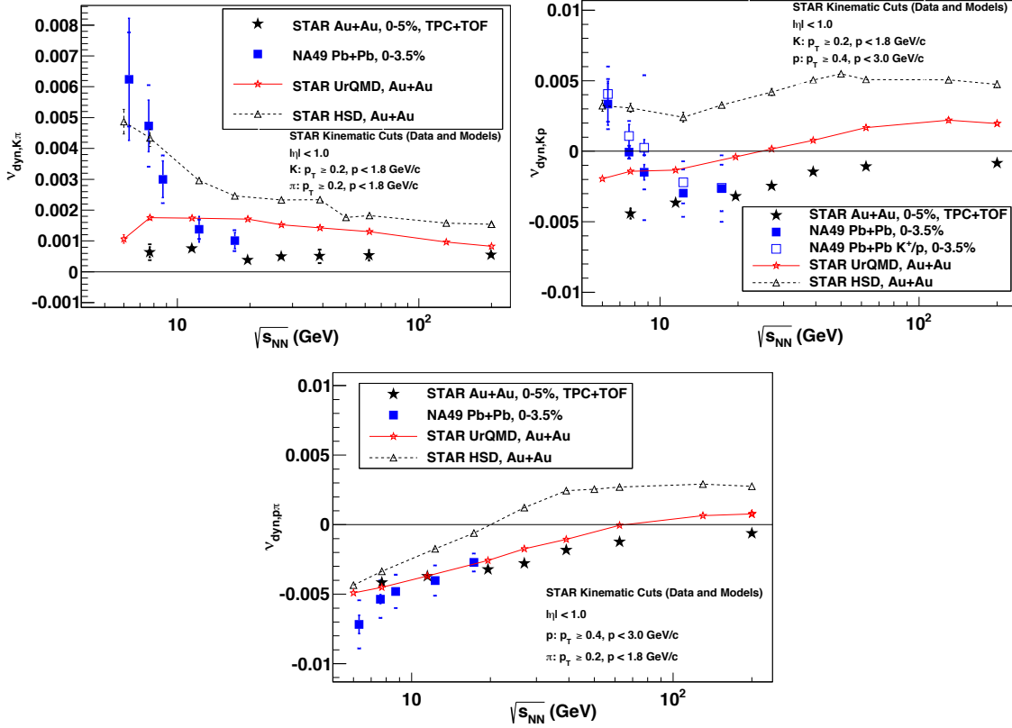
Figure 1.7.: \nu_{\text{dyn}} results of NA49 [28] and STAR [25] collaborations.
