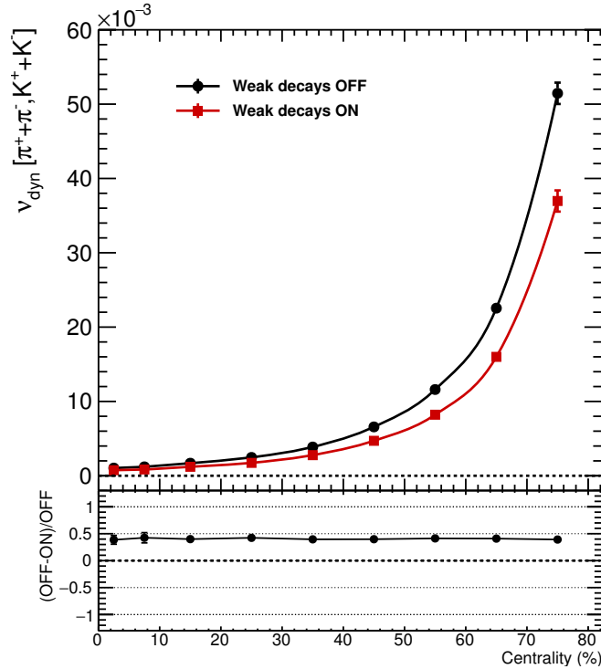
Figure 6.9.: Illustration of the effect of weak decays on \nu_{\text{dyn}}[\pi, K] using HIJING [82] model calculations.
