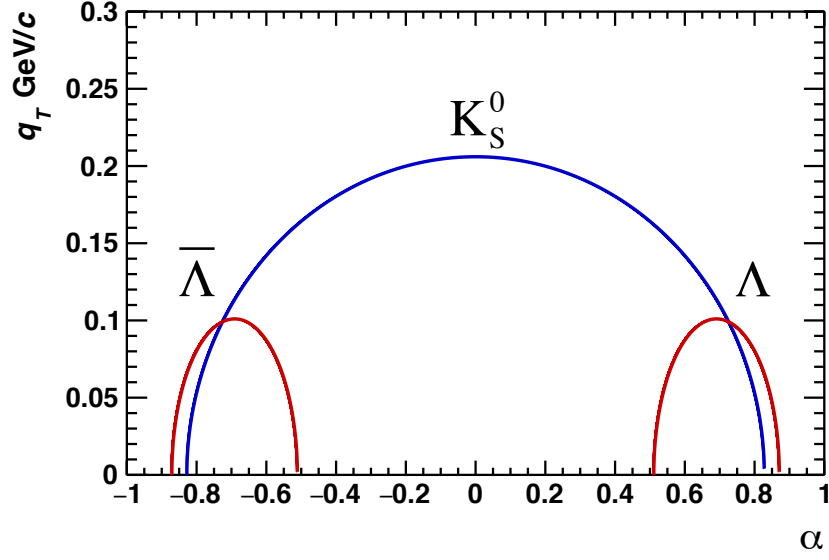
Figure F.2.: The Armenteros-Podolanski plot showing the K_S^0 , \Lambda and \bar{\Lambda} half ellipses.
