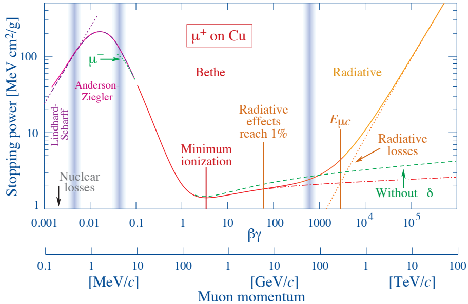
Figure 2.14.: Stopping power ( \langle -dE/dx \rangle ) for positive muons in copper as a function of \beta\gamma over nine orders of magnitude in momentum (12 orders of magnitude in kinetic energy) [4].
