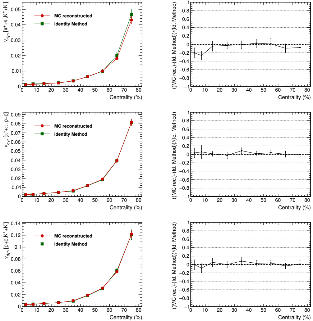
Figure 5.6.: \nu_{dyn} results reconstructed with the Identity Method and calculated from MC samples (left column) and the corresponding comparison plots (right column).
