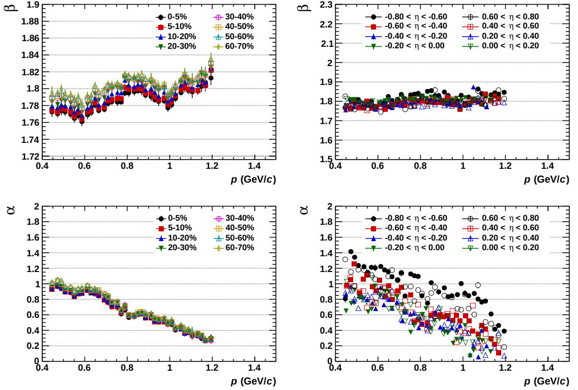
Figure 4.11.: Distribution of the fit parameters \beta (upper panel) and \alpha (lower panel) for clean pions. Centrality and pseudorapidity dependence of both parameters are shown in the left and right columns, respectively.
