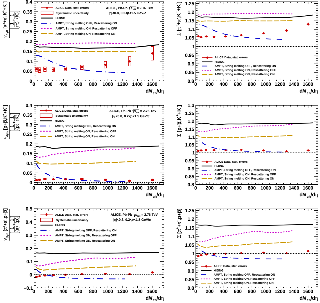
Figure 6.5.: Comparison of \Sigma results to the \nu_{\text{dyn}} results scaled by \frac{1}{1/\langle N_a \rangle + 1/\langle N_b \rangle} .
