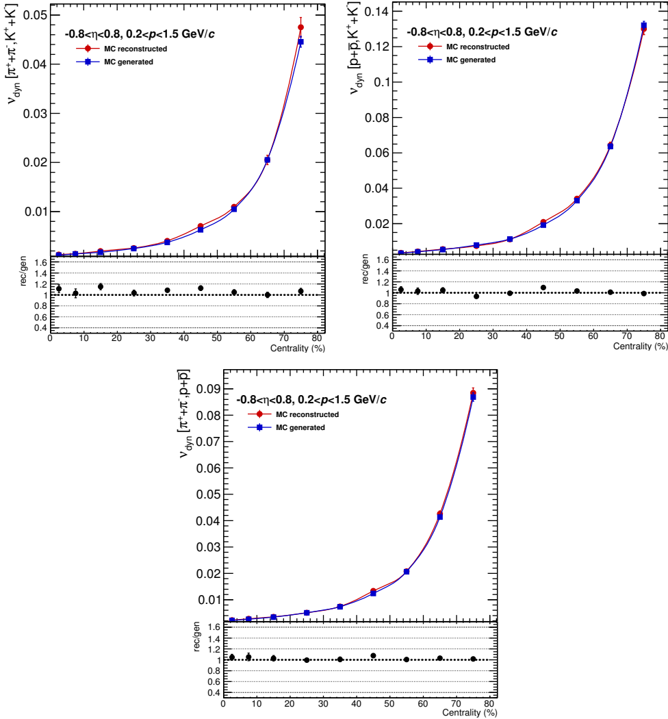
Figure 5.9.: Effect of detection efficiency losses on the \nu_{\text{dyn}} results.
