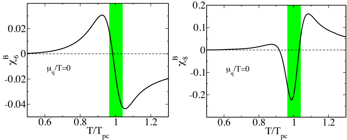
Figure 1.6.: The sixth and eighth order cumulants of the net baryon number fluctuations at \mu_q/T = 0 in the Polyakov Quark Meson (PQM) model [18]. The temperature is given in units of the pseudo-critical temperature T_{pc} corresponding to a maximum of the chiral susceptibility. The shaded area indicates the chiral cross-over region [19].
