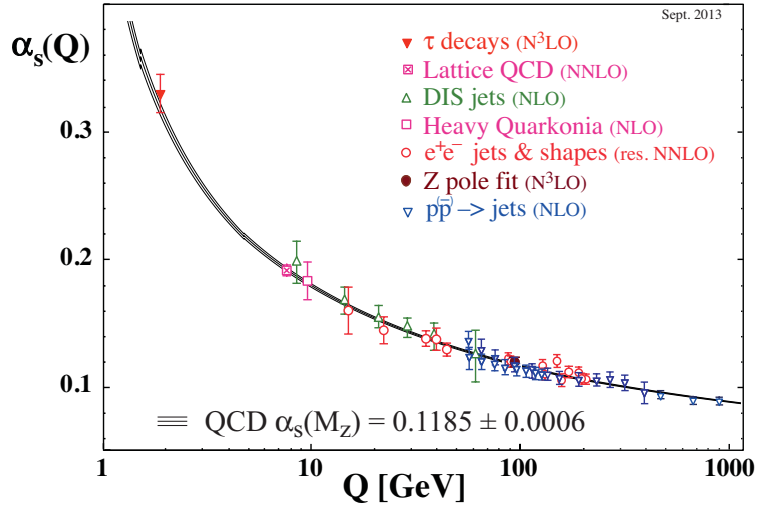
Figure 1.1.: Summary of measurements of the running coupling constant \alpha_s as a function of the energy scale Q . The respective degree of QCD perturbation theory used in the extraction of \alpha_s is indicated in brackets (NLO: next-to-leading order; NNLO: next-to-next-to leading order and so on and so forth. M_Z is the mass of the Z boson) [4].
