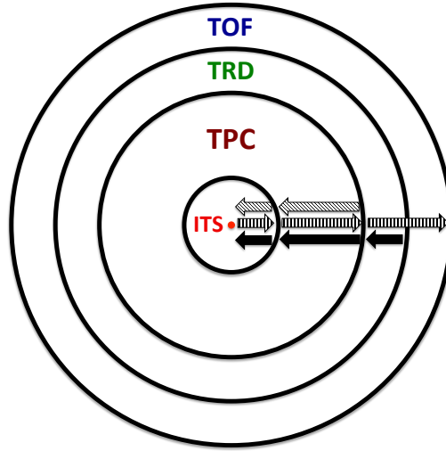
Figure A.2.: Schematic view of the three passes of the combined track finding [92].
