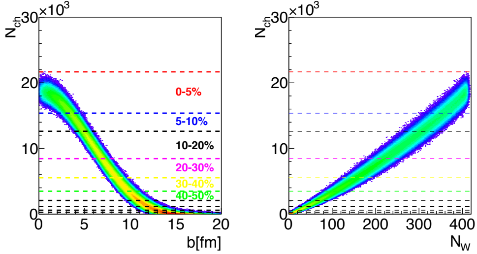
Figure 6.3.: Left Panel: Produced number of charged particles versus the impact parameter. Right Panel: Produced number of charged particles versus the number of wounded nucleons, i.e. number of participants. For a given value of the impact parameter the number of wounded nucleons and binary collisions are calculated with a Glauber Monte Carlo simulation. The corresponding centrality classes are indicated by the dashed horizontal lines [20].
