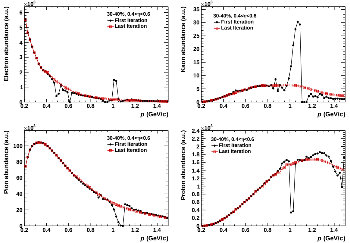
Figure 4.18.: Comparison of the abundances of each particle species in the first (black markers) and last (red markers) iteration.
