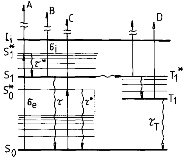
Figure D.1.: Schematic energy level diagram of complex molecule, indicating possible channels for 2-photon ionisation [96].
