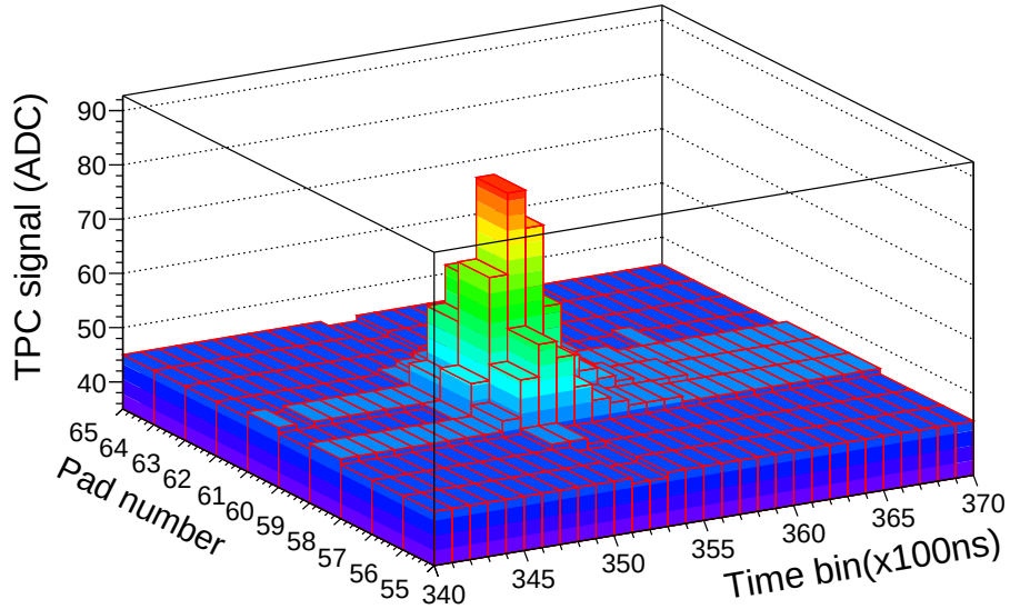
Figure 2.12.: A laser cluster before pedestal subtraction and zero-suppression.
