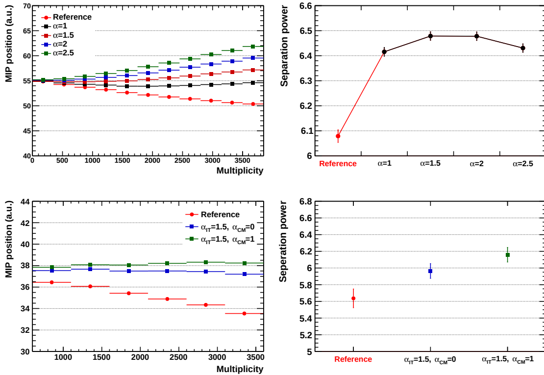
Figure 3.24.: Improvement achieved in the separation power and mean dE/dx positions. Upper Panel: for a given run from the 2010 Pb–Pb data taking period after the offline ion-tail correction with different fudge factors. Lower Panel: for a given run from the 2013 p–Pb data taking period after the offline ion-tail and common-mode corrections.
