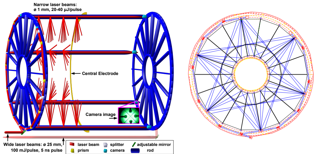
Figure 2.9.: (Left) Schematic 3D view of the TPC and the laser system. (Right) Ideal laser tracks projected to the endcap. The pattern repeats eight times through the full length of the TPC [50].
