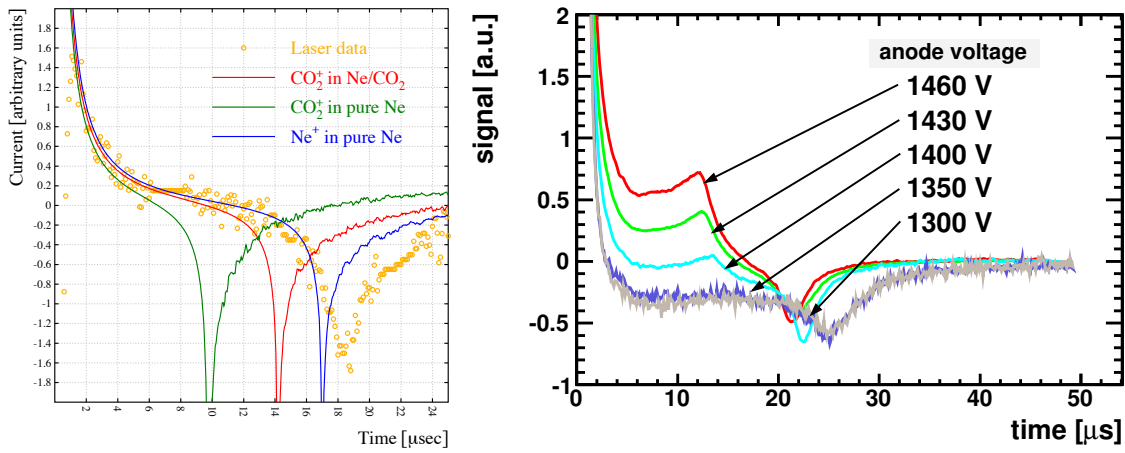
Figure 3.7.: (Left) The laser signal shape measured in the NA49 Vertex TPC at the SPS is shown with orange markers while the solid lines show the Garfield simulations for different assumptions on the drifting ion type and gas mixtures [57]. (Right) Ion-tail signals measured in a ALICE-TPC IROC with Ne-CO 2 -N 2 (90-10-5) gas mixture for different anode voltages [68].
