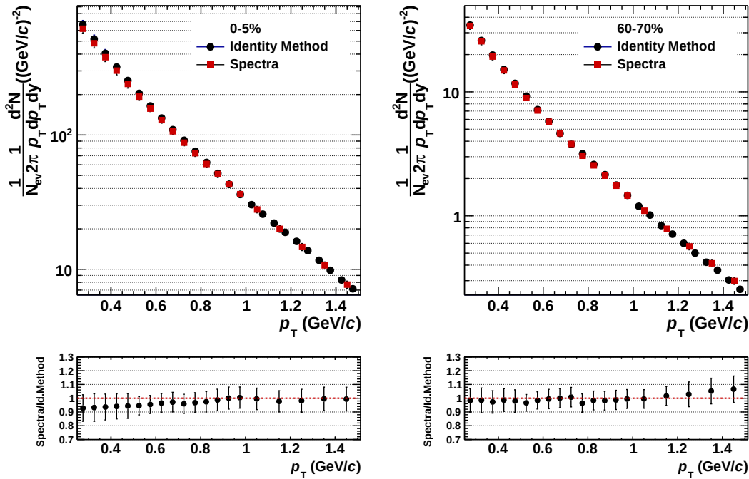
Figure 5.5.: Comparison of the published pion spectra results to the mean pion multiplicities obtained by the Identity Method.
