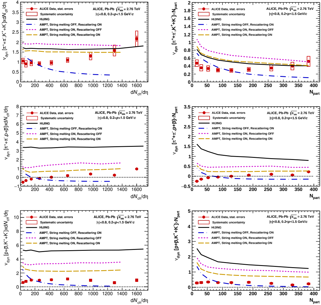
Figure 6.6.: ALICE results for \nu_{\text{dyn}} scaled by dN_{\text{ch}}/d\eta (left column) and N_{\text{part}} (right column) in comparison with the HIJING [82] and AMPT [84] model calculations..
