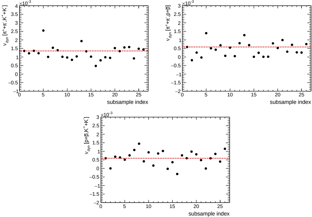
Figure 5.7.: Reconstructed values of \nu_{\text{dyn}}[\pi, K] , \nu_{\text{dyn}}[\pi, p] and \nu_{\text{dyn}}[K, p] for most central events. Dashed red lines indicate the corresponding averaged values of \nu_{\text{dyn}} over subsamples and the black markers for subsamples.
