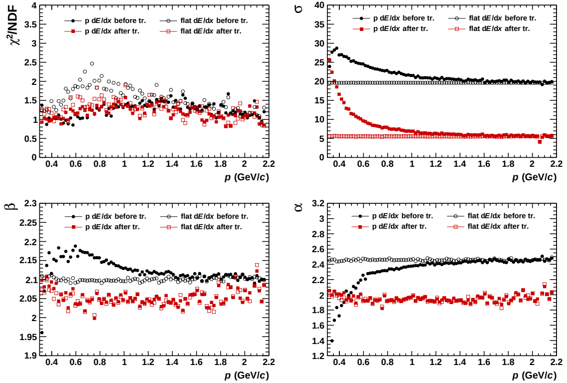
Figure 4.8.: Distribution of the fit parameters \alpha , \beta and \sigma as well as the fit quality measure \chi^2/NDF along the full momentum range used in Figure 4.7 for before (black markers) and after (red markers) the truncated mean procedure. Closed symbols show the results for the rising dE/dx slope and the open symbols for the fixed dE/dx .
