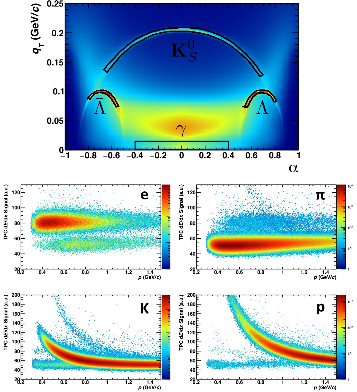
Figure 4.9.: (Upper panel) Armenteros-Podolanski plot obtained from the V0 decay particles. Black lines indicates the graphical cuts used to select K_S^0 , \bar{\Lambda} and \Lambda . The dE/dx distributions of clean electron samples (Middle panel left) from the \gamma conversions, pion samples (Middle panel right) from the decay of K_S^0 \rightarrow \pi^+ \pi^- , proton samples (Lower panel right) from the decays of \bar{\Lambda} \rightarrow \bar{p} \pi^+ and \Lambda \rightarrow p \pi^+ and kaon samples (Lower panel left) obtained using TOF and TRD information.
