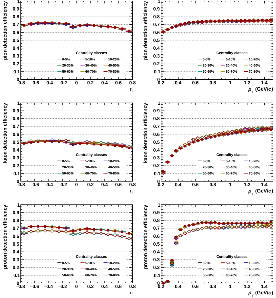
Figure 1.2.: (Color Online) Single particle detection efficiencies for pions (first row), kaons (second row) and protons (third row). Efficiencies are shown as integrated over momentum (first column) and pseudorapidity (second column). Different colors show different centrality classes. Negative and positive particles are shown with open and closed circles, respectively. (Negative particles are corrected for the absorption due to interaction with the material in the detector[80].)
