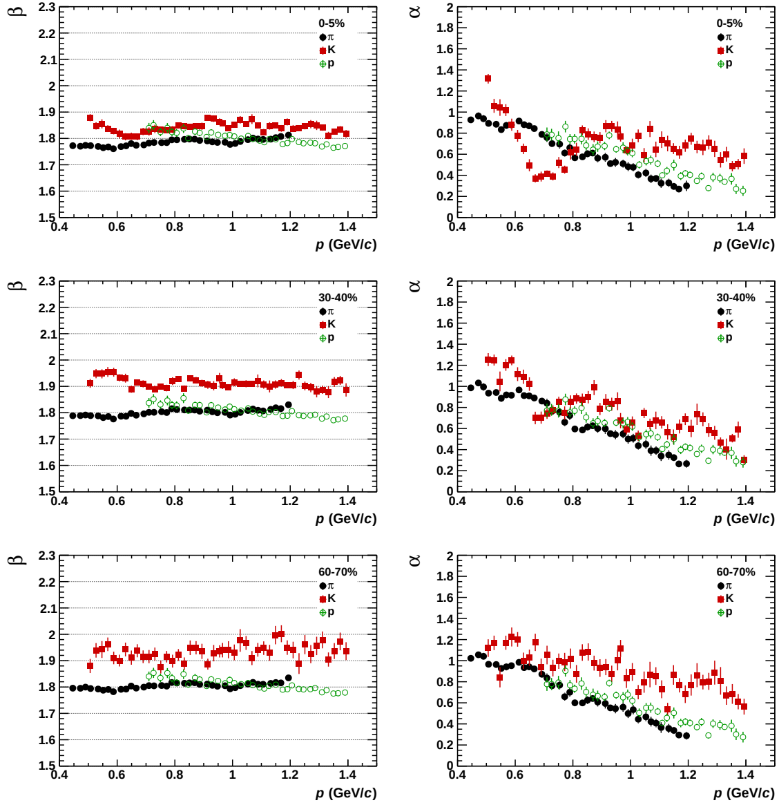
Figure 4.10.: Distribution of the fit parameters \beta (left column) and \alpha (right column) for clean pions (black markers), kaons (red markers) and protons (green markers) in three different centrality bins: 0-5% (upper panel), 30-40% (middle panel) and 60-70% (lower panel).
