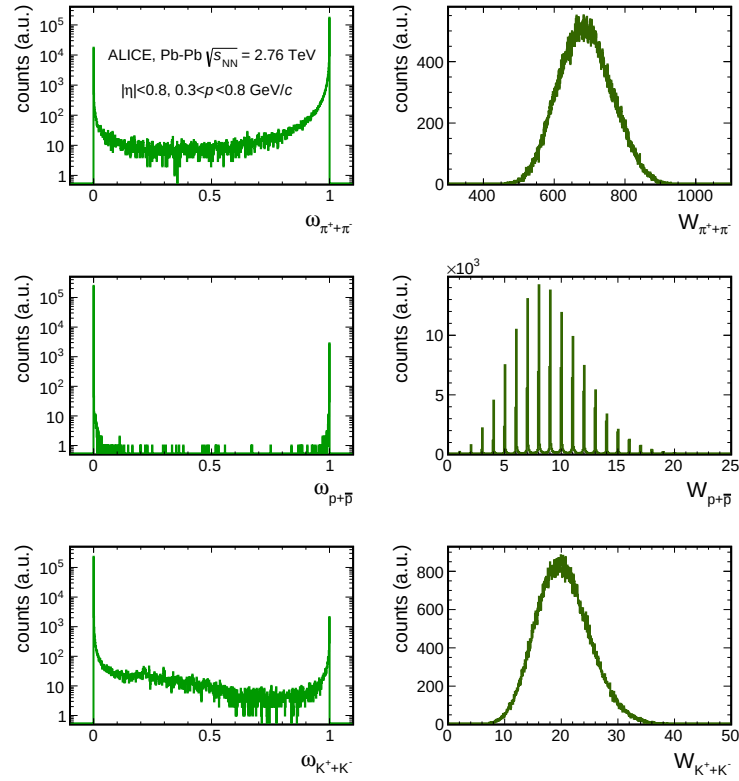
Figure 5.4.: \omega and W distributions for pions, kaons and protons within the momentum range of 0.3 < p < 0.8 GeV/c.
