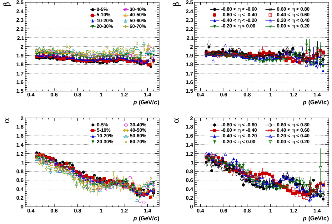
Figure 4.14.: Distribution of the fit parameters \beta (upper panel) and \alpha (lower panel) for MC pions. Centrality and pseudorapidity dependence of both parameters are shown in the left and right columns, respectively.
