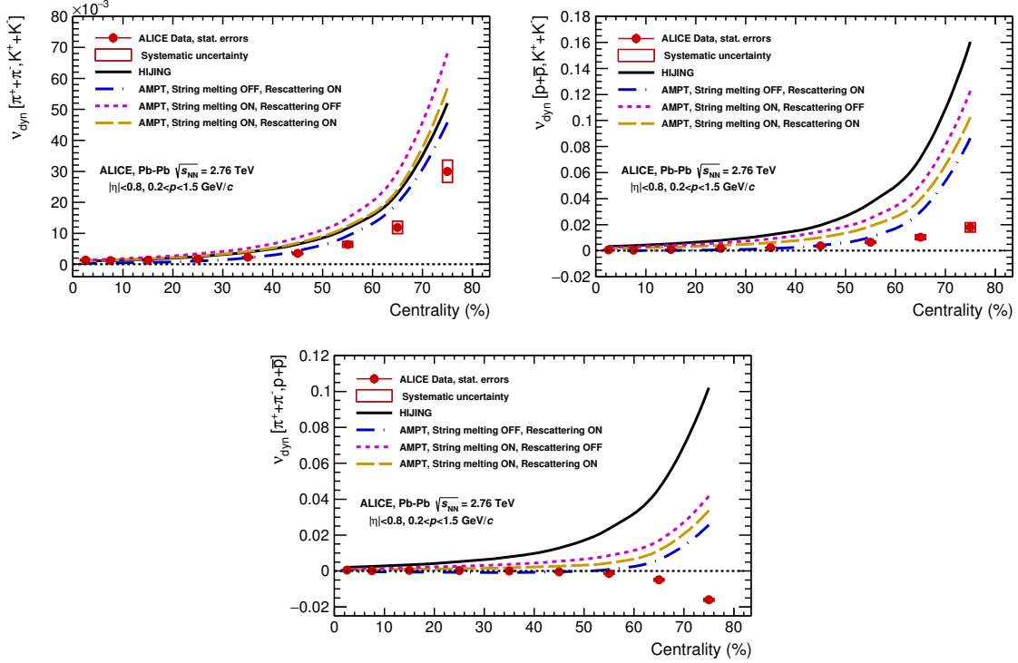
Figure 6.2.: Comparison of non-scaled ALICE \nu_{\text{dyn}} results to HIJING [82] and AMPT [84] model calculations.
