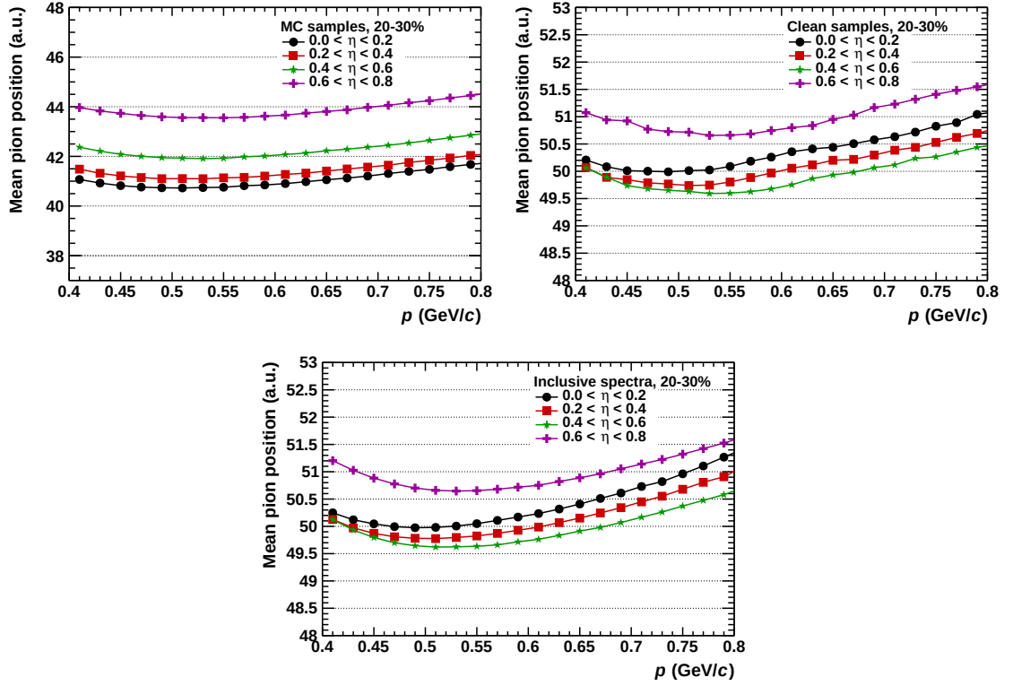
Figure 4.16.: Pseudorapidity dependence of the mean dE/dx positions of the MC simulation (top left), clean sample (top right) and inclusive pion spectra (bottom) in the centrality bin of 20-30%.
