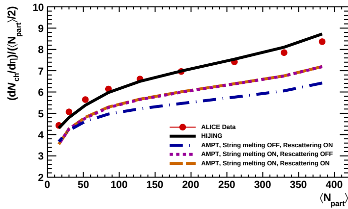
Figure 6.11.: Dependence of (dN_{\text{ch}}/d\eta)/(\langle N_{\text{part}} \rangle/2) on the number of participants ( N_{\text{part}} ) in comparison with the AMPT [84] and HIJING [82] model calculations.
