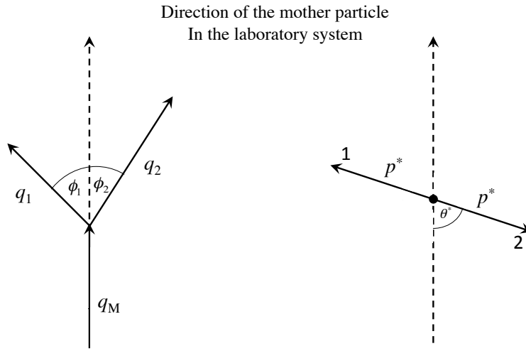
Figure F.1.: The decay of a neutral V^0 into two charged tracks in the laboratory system (left) and the center of mass system (right). Particle 1 and 2 are assumed to be the positively and negatively charged, respectively. In the center of mass system the momentum of mother particle p_M^* , is zero.
