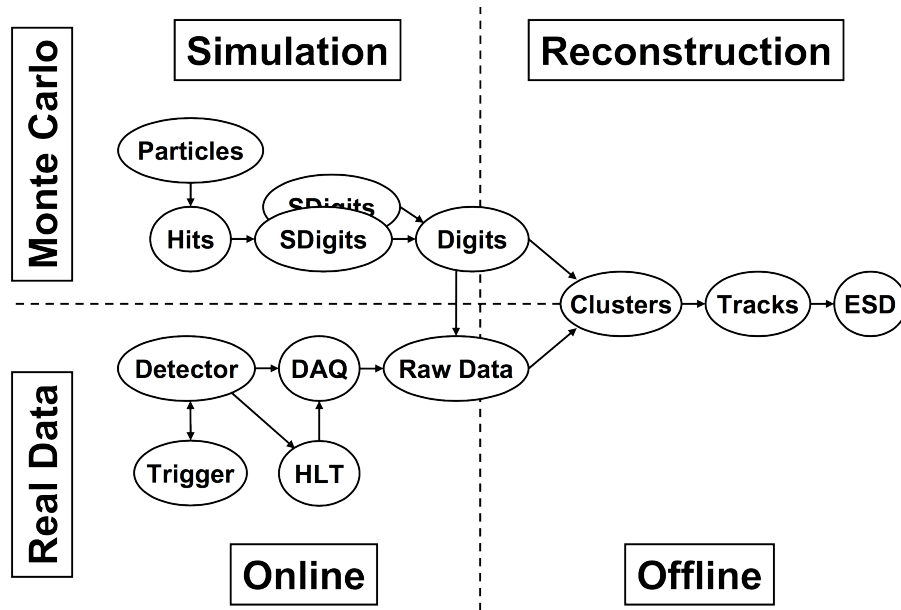
Figure A.1.: Simulation and reconstruction process in ALICE [92].
