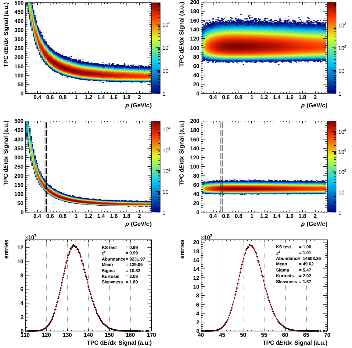
Figure 4.7.: Toy simulation of particle tracks illustrating the effect of truncated mean procedure on the TPC dE/dx . The mean dE/dx values are taken from Monte-Carlo (MC) protons in the left column and are fixed at 100 in the right column. The dE/dx distributions before and after the truncated mean procedure are shown in the upper and middle panels, respectively. The lower panel illustrates the Generalized Gauss function fits of the dE/dx distributions in the momentum intervals indicated in the middle panel by dashed lines.
