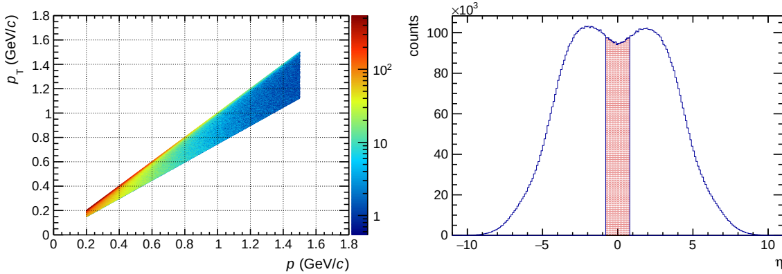
Figure 5.1.: Acceptance in momentum ( 0.2 < p < 1.5 GeV/c) and pseudorapidity ( |\eta| < 0.8 ) spaces (HIJING model calculations).
