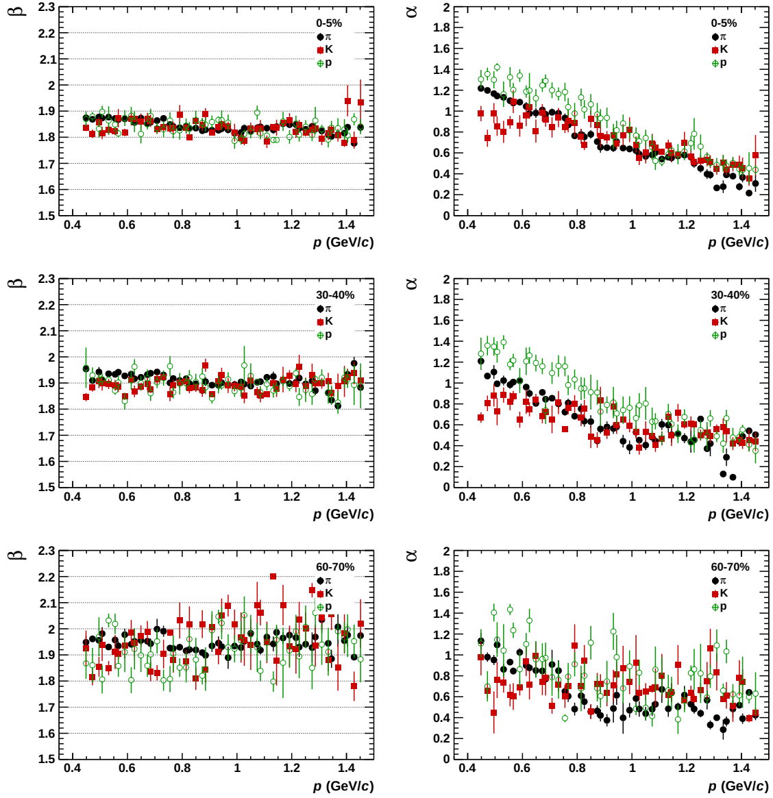
Figure 4.13.: Distribution of the fit parameters \beta (left column) and \alpha (right column) for MC pions (black markers), kaons (red markers) and protons (green markers) in three different centrality bins: 0-5% (upper panel), 30-40% (middle panel) and 60-70% (lower panel).
