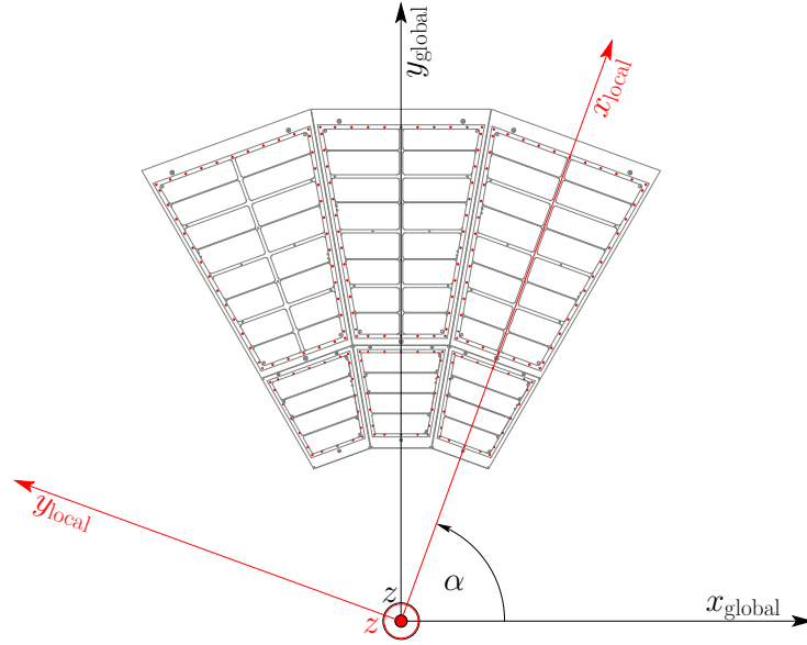
Figure B.2.: Sketch of the ALICE local coordinate system [94, 95].
