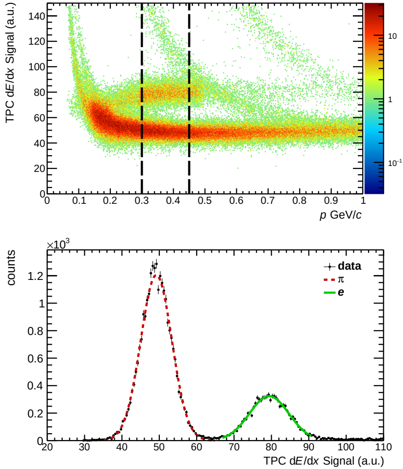
Figure 2.16.: (Top) dE/dx spectrum of simulated central Pb–Pb events obtained via HIJING simulation with GEANT3 implementation of the TPC detector setup, where electrons are enhanced by embedding \gamma conversions in order to obtain sufficient statistics for the fit. Dashed lines depict the momentum range where the separation power calculation is performed. (Bottom) The projection of the marked area of the left plot on the dE/dx axis. Red dashed line for the \pi fit, green solid line for the e fit. Resulting separation power is 6.4 \pm 0.04 .
