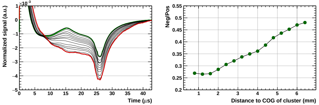
Figure 3.11.: Normalized pad signals with zoom into the y-axis measured at different distances to the center of gravity of the cluster. (Left) Ion-tail shape where solid green and red lines indicate the most central and peripheral pad signals, respectively. (Right) Ratio of the undershoot to the pulse as a function of distance to the center of gravity of the cluster.
