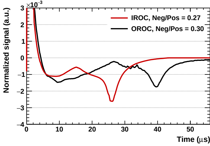
Figure 3.9.: (Color Online) Normalized pad signals with zoom into the y-axis for IROC and OROC geometries (See Section 2.2).
