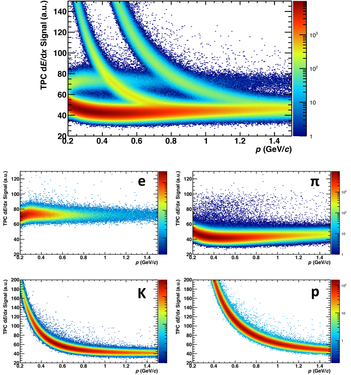
Figure 4.12.: dE/dx distributions of inclusive MC particles (Upper panel), electrons (Middle panel left), pions (Middle panel right), kaons (Lower panel left) and protons (Lower panel right).
