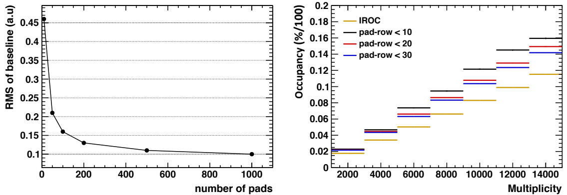
Figure 3.34.: (Left) Effective common-mode noise contribution as a function of the number of pads used for the average calculation. (Right) Signal occupancy in IROCs as a function of multiplicity (total number of primary and secondary tracks).
