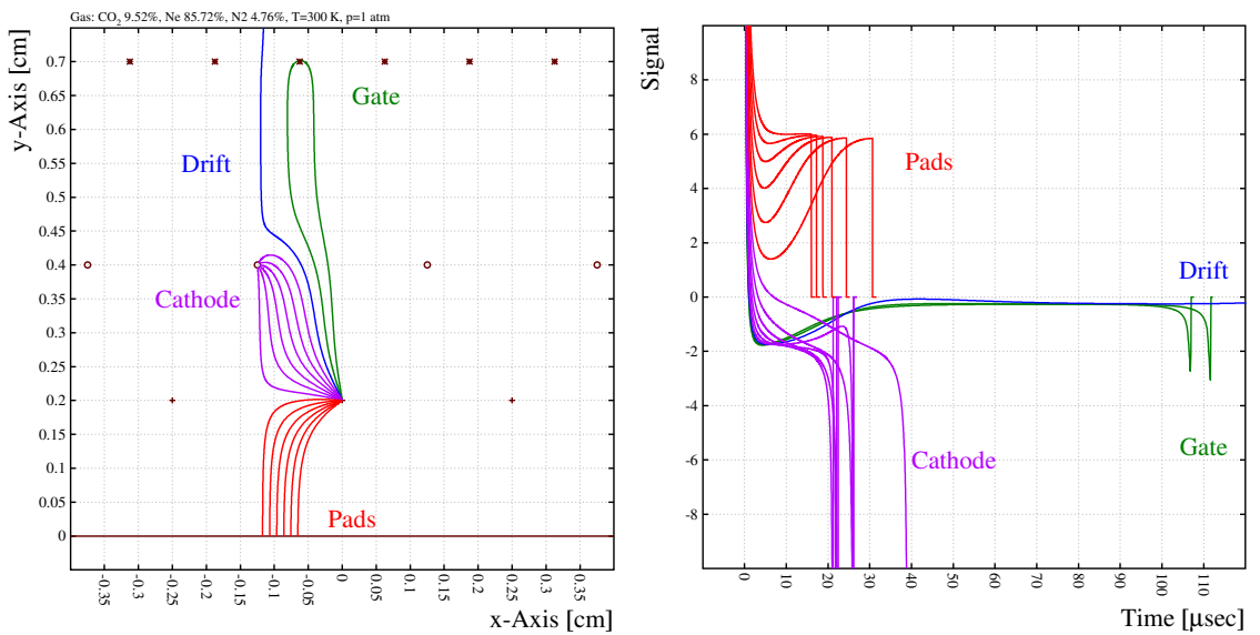
Figure 3.6.: (Left) The drift lines of ions. (Right) Corresponding ion signals induced on the pads [68, 69].
