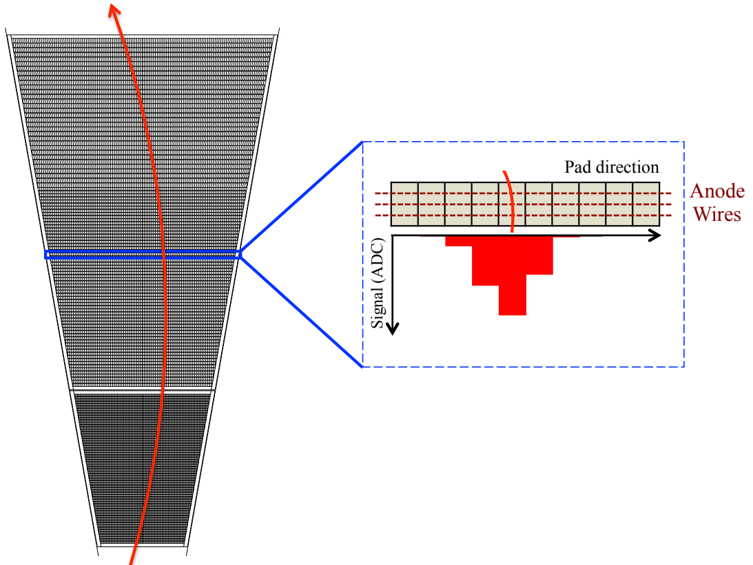
Figure 2.11.: Illustration of a track passing through 159 padrows of a given sector and the corresponding pulse height distribution of a cluster on one padrow. The shape of the signal shown in red is taken from a laser track cluster.
