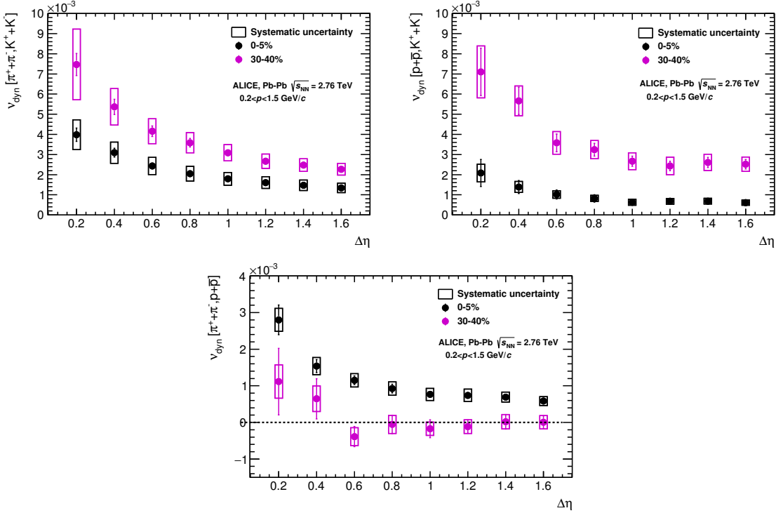
Figure 6.10.: Pseudorapidity dependence of ALICE \nu_{\text{dyn}} results for two centrality classes.
