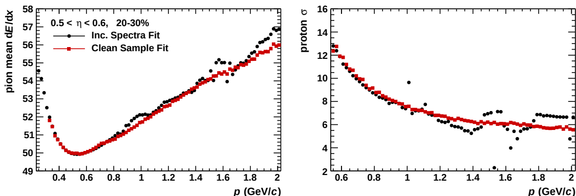
Figure 4.17.: Comparison of the first iteration fit results (black markers) and the clean sample fits (red markers). Left: mean dE/dx position for pions. Right: width ( \sigma ) of the generalized Gauss function fit for protons.
