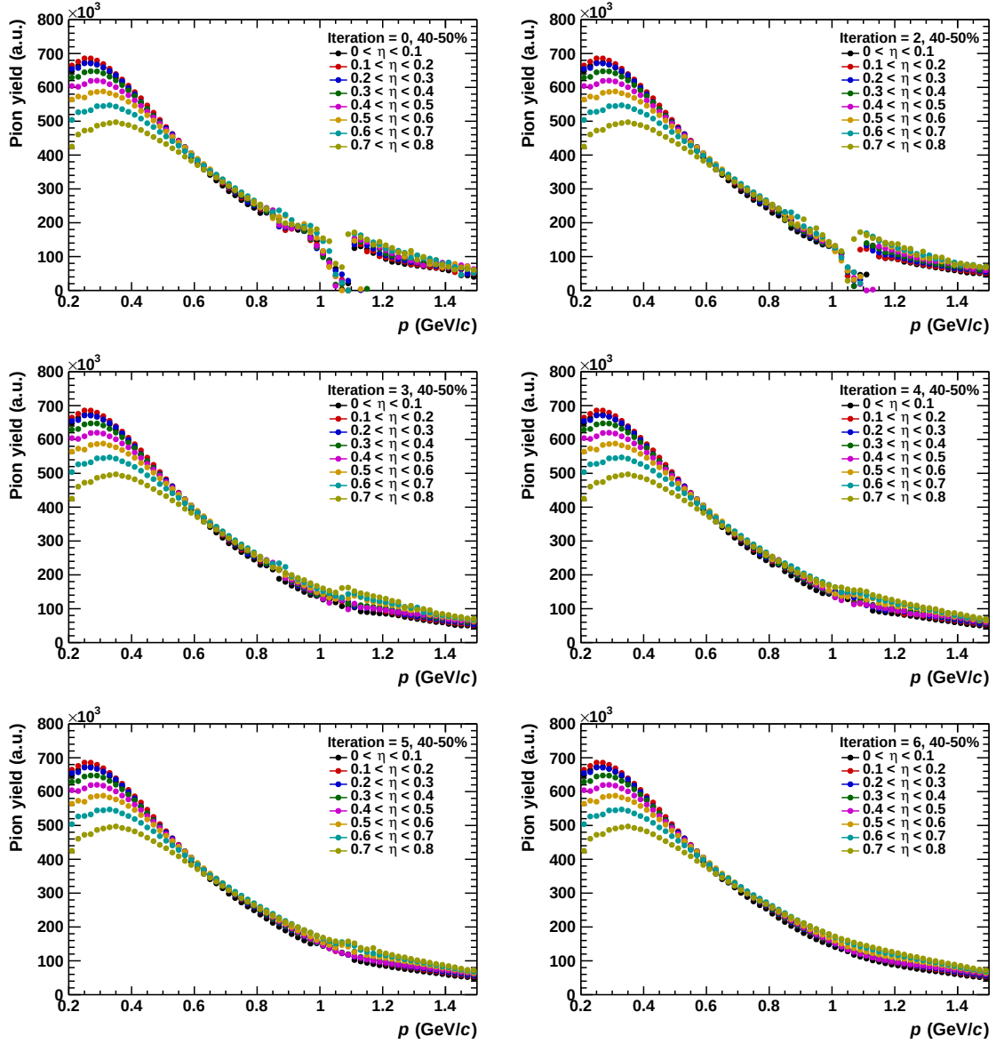
Figure 4.19.: Integral of the fit functions of inclusive pion spectra for several fit iterations.
