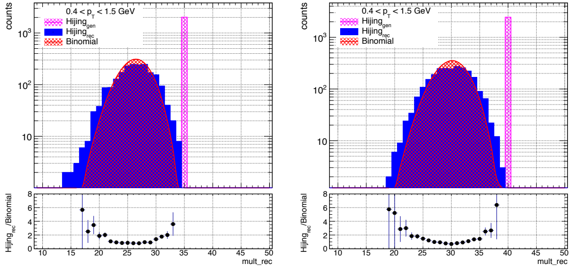
Figure 5.8.: Protons generated by the HIJING model for two different multiplicities, 35 and 40 on the top left and top right, respectively. The distribution of reconstructed protons is overlaid with a Binomial distribution. The corresponding ratios are presented in bottom panels [81].
