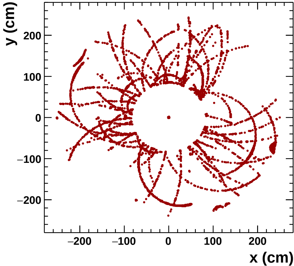
Figure 3.25.: TPC event display of a simulated Monte-Carlo event with 100 tracks.
