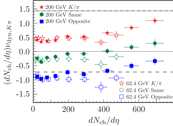
Figure 6.7.: (color online). STAR collaboration results of the dN_{\text{ch}}/d\eta scaled \nu_{\text{dyn}}[\pi, K] for summed charges (stars), same sign (circles), and opposite sign (squares) as a function of dN_{\text{ch}}/d\eta . The errors shown are statistical. The dash-dotted, dotted, and dashed lines represent HIJING calculations for summed charges, same sign, and opposite sign, respectively [89].
