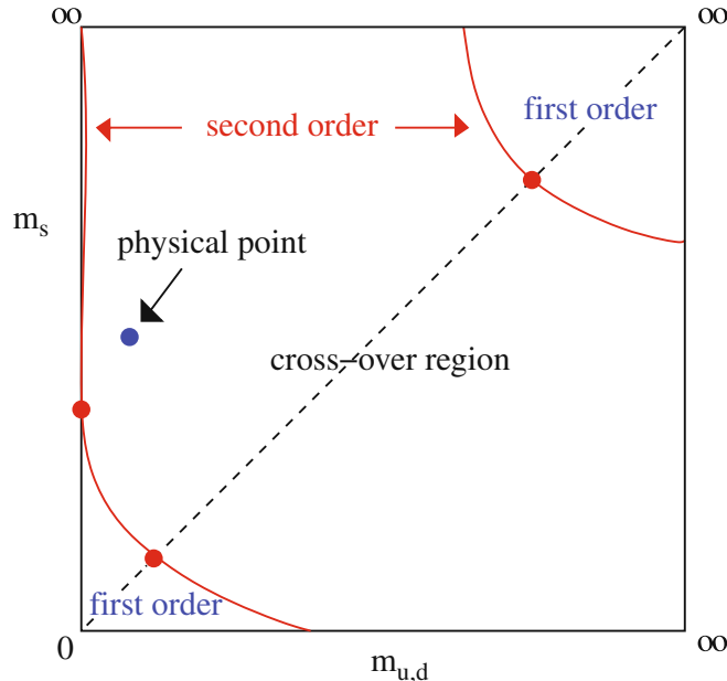
Figure 1.4.: The QCD phase diagram of 3-flavour QCD [17].
