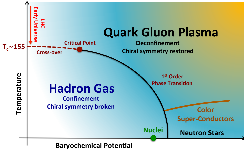
Figure 1.2.: The schematic phase diagram of the QCD.
