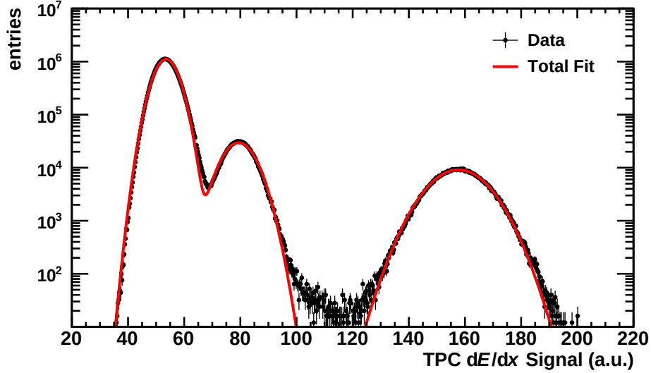
Figure 4.4.: Multi-Gaussian fit of the inclusive dE/dx distribution of TPC in the phase-space region of 0.35 < p < 0.37 GeV/ c and 0 < \eta < 0.2 for the most central events. The overlap region is not covered properly because of the symmetric shape of the Gauss function.
