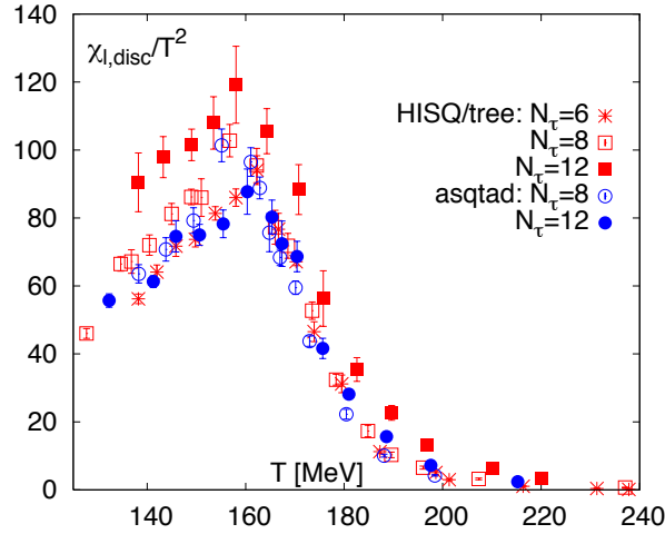
Figure 1.5.: Recent calculations of the chiral susceptibility for m_l = m_s/20 and different N_\tau , where N_\tau is temporal extent and m_l, m_s are the light and strange quark masses, respectively [9].
