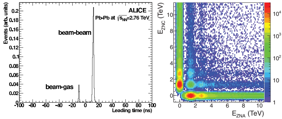
Figure 5.2.: (Left) Time distribution of signals in the V0A detector. The peaks corresponding to beam-beam, beam-gas and satellite collision events are clearly visible [79]. (Right) Correlation between signals in the two neutron zero-degree calorimeters, ZNA and ZNC. Single electromagnetic dissociation events produce a signal in only one of the calorimeters [79].
