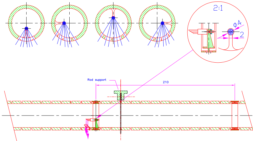
Figure E.4.: Laser rod with micro-mirror bundle and its support, as well as the azimuthal reflection angles of each mirror bundle [60].
