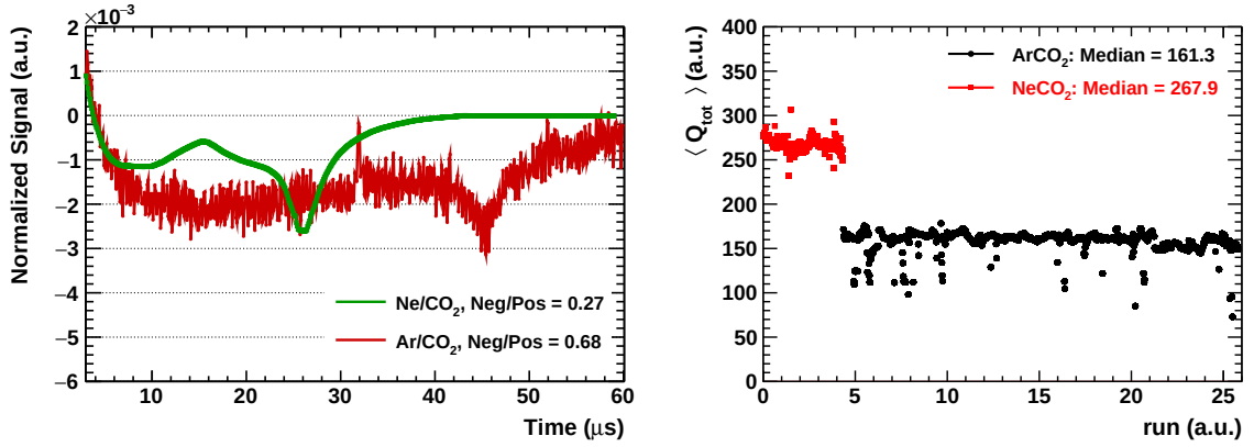
Figure 3.8.: (Color Online) Left: Normalized pad signals with zoom into the y-axis for Ar-CO 2 (88-12) and Ne-CO 2 (90-10) gas mixtures. Right: Mean total charge of clusters for Ar-CO 2 and Ne-CO 2 gas mixtures as a function of run [71]. Ar-CO 2 values are scaled with the relative ratio of primary ionization values ( N_{T,ArCO_2}/N_{T,NeCO_2}=97/40 , where N_T is the total number of electron-ion pairs per cm) taken from [4].
