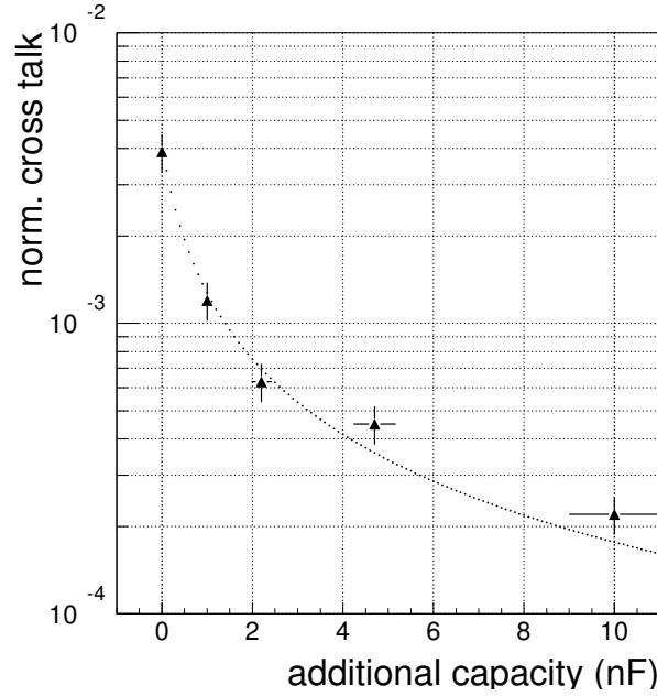
Figure 3.18.: Normalized common-mode signal as function of an additional capacity directly connected to the anode wires (Measured in NA49 experiment [74]). The expected behavior due to a parallel capacity is shown by the dotted line.
