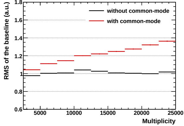
Figure 3.28.: Additional noise resulting from the common-mode effect as a function of multiplicity (total number of primary and secondary tracks).
