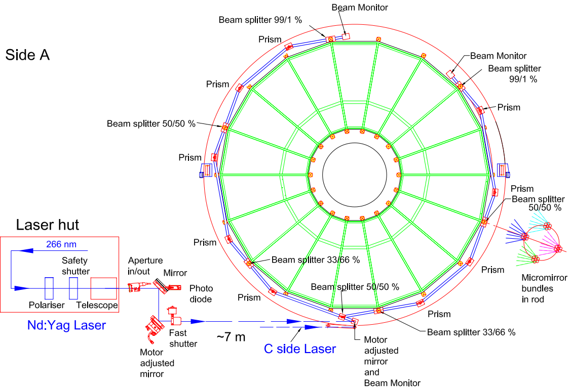
Figure E.1.: Overview of the optical elements to guide the laser beam from the laser hut to the entrance windows in the TPC field cage. The A side system is shown. The C side system is obtained by mirror symmetry in a vertical plane along the TPC axis [50].
