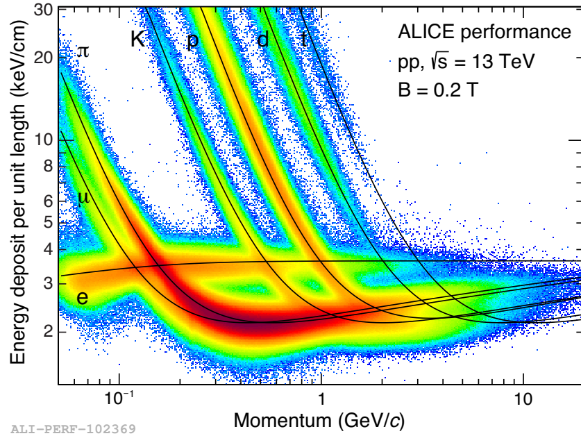
Figure 4.2.: Specific energy loss in the TPC at magnetic field of 0.2 T and \sqrt{s} = 13 TeV as a function of momentum with superimposed Bethe-Bloch lines for various particle species [4].
