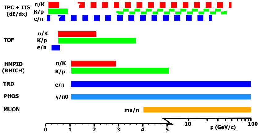
Figure 4.1.: Particle identification capabilities of the subdetectors of ALICE as a function of momentum. Solid bars and dashed regions mark regions of a separation better than 3\sigma and 2\sigma , respectively [78].
