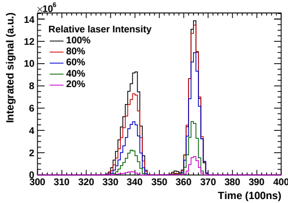
Figure 3.4.: Integrated TPC signals of the second laser layers on the A and C side of the TPC for different laser intensities. For each intensity a stand-alone laser calibration run is taken with a total number of 2000 events.
