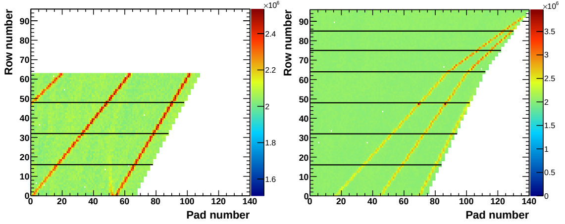
Figure 3.20.: Anode wire segmentation of the IROC (left) and OROC (right) geometries.
