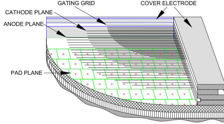
Figure 2.4.: Cross section through a readout chamber showing the pad plane, the wire planes and the cover electrode [50].
