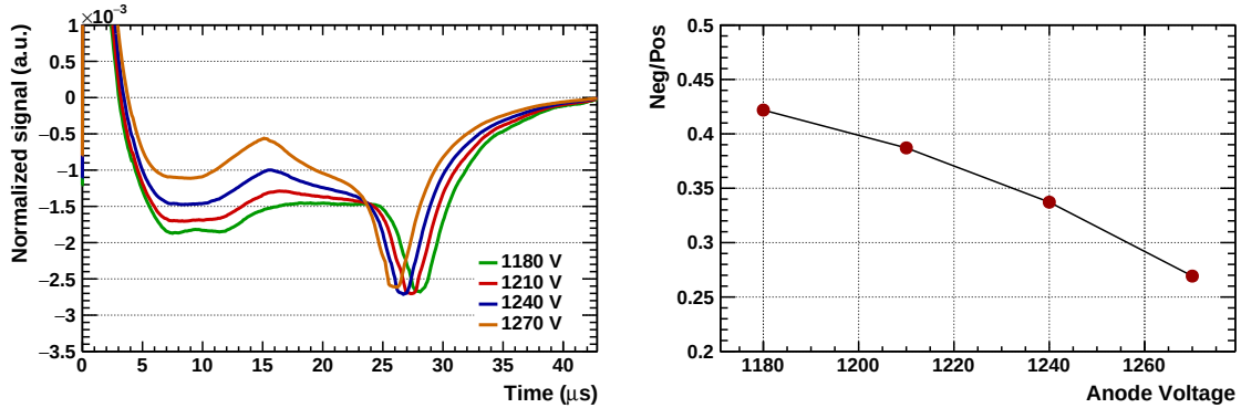
Figure 3.10.: (Color Online) Normalized pad signals with zoom into the y-axis for different anode voltage settings. (Left) Ion-tail shape. (Right) Ratio of the undershoot to the pulse as a function of anode voltage.
