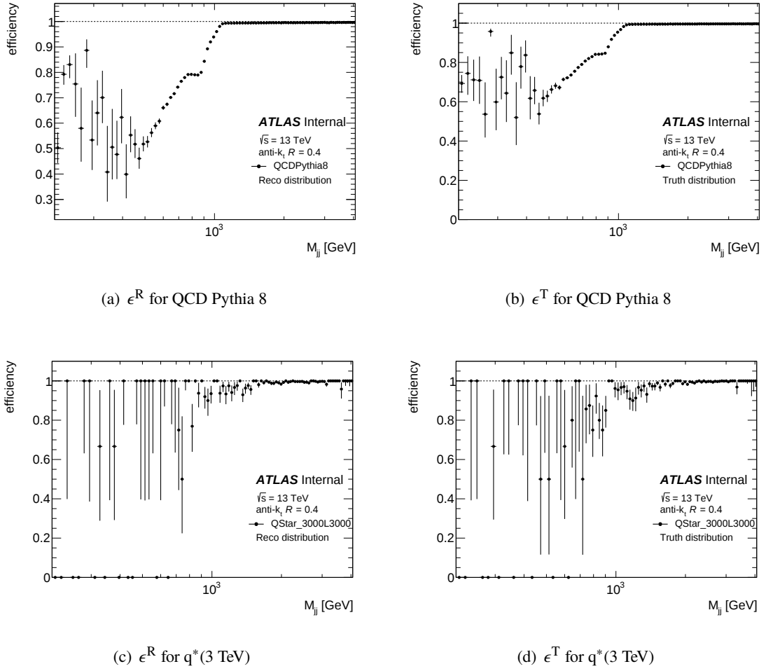
Figure 4.9: Matching efficiencies at truth and reconstructed level for two MC samples: one from QCD and one from q^*(3 TeV).
