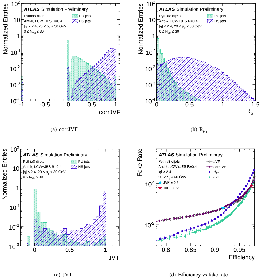
Figure 2.23: Distributions of corrJVF(a), R_{pT} (b) and JVT (c) for pileup and hard-scatter jets. d) Efficiency versus fake rate for the different variables. Figures from [63].
