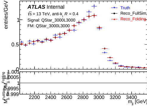
(a) q^*(3 \text{ TeV}) folded with \tilde{A}(q^*(3 \text{ TeV}))
