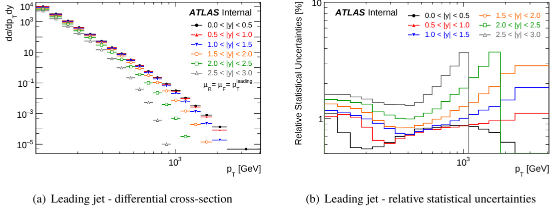
Figure 5.31: Differential cross-sections and relative statistical uncertainties for leading jet observable for the different rapidity bins, using a cut-off regularization \Lambda = 0.001 GeV and p_T leading scales. The number of simulated events is 10^{12} .
