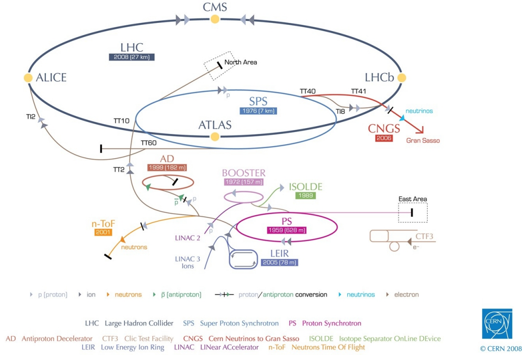
Figure 2.1: The LHC is the largest ring of the CERN chain of particle accelerator complex. The smaller machines are used in a chain to help boost the particles to their final energies. Figure from CERN website.
