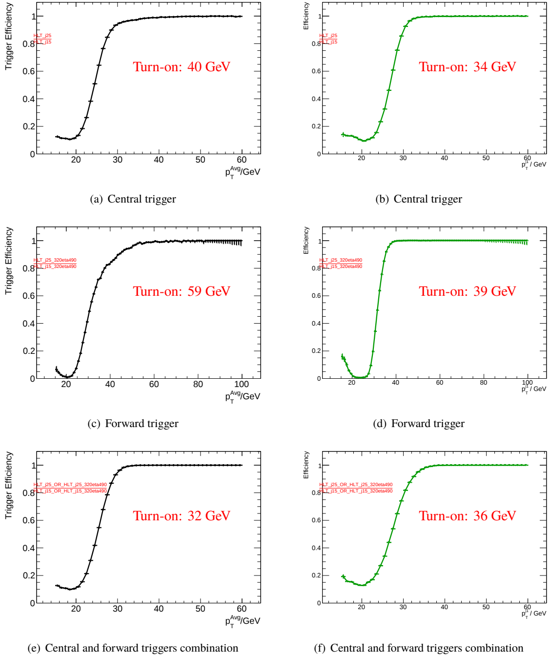
Figure 3.24: Efficiencies for trigger HLT_j25 using HLT_j15 as a reference as a function of p_T^{\text{avg}} in left plots and p_T^{\text{leading jet}} in right plots. From top to bottom, the plots are for central, forward and combined triggers. The HLT_j25 trigger is used for p_T^{\text{avg}} \geq 40 GeV and the turn-on p_T is required to be at least 5 GeV lower.
