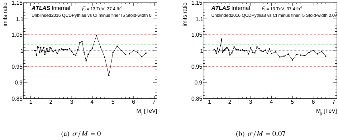
Figure 4.22: Ratios of limits for signals folded with \tilde{A} matrices from CI samples divided by the ones obtained with \tilde{A} matrices from QCD Pythia8 samples. Results are shown for two different resonance widths. The green dotted lines correspond to a 2% deviation from 1, and the red ones to 5%.
