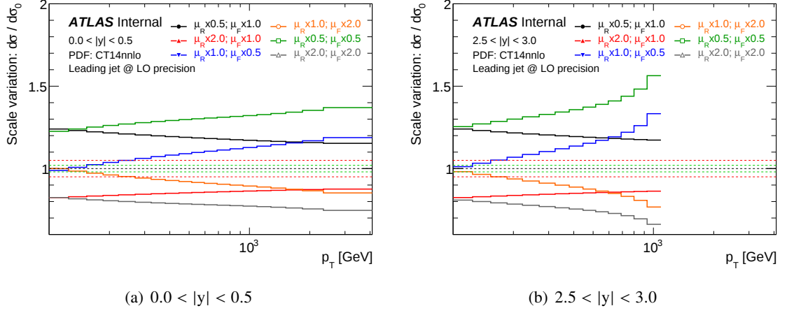
Figure 5.41: Ratio of the LO partonic cross-sections from the scales variation to the prediction using the nominal scale in the most central and the most forward rapidity bins as a function of p_T . The PDF set used is CT14nnlo.
