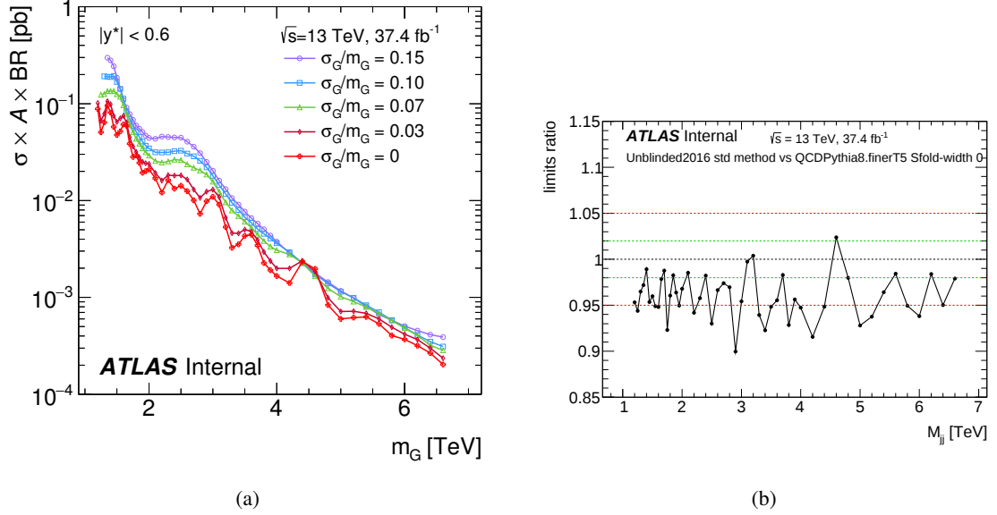
Figure 4.21: (a) Limits of various widths Gaussian signals at truth level folded with \tilde{A} matrix from QCD Pythia8 samples, using 5 times finer binning for the truth axis compared to the reconstructed one. (b) Ratio of the limit for a signal with a width equal to the resolution at reconstructed level, divided by the limit with a narrow signal at truth level folded using a matrix with fine bins on the truth axis. The green dotted lines correspond to a 2% deviation from 1, and the red ones to 5%.
