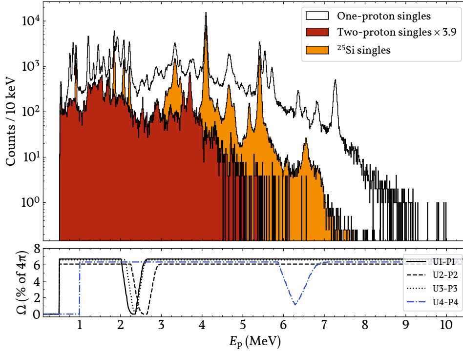
Figure 8.10: Proton singles spectra from the beta decay of ^{26}\text{P} . As in figure 8.9, both one-proton and two-proton singles spectra are shown and the detection efficiency of the two-proton singles spectrum is corrected by the solid angle coverage. A singles spectrum from a dedicated measurement on ^{25}\text{Si} is also shown; it is clearly seen how many of the peaks of the ^{26}\text{P} singles spectrum are due to contamination from ^{25}\text{Si} .
