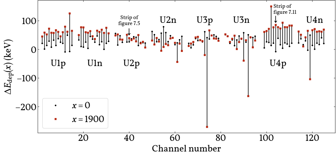
Figure 7.17: Difference between proton and alpha calibrations of various DSSSD detector strips. The difference \Delta E_{\text{dep}} , equation (7.2), is calculated at small and large channel numbers x = 0, 1900 , corresponding roughly to 0 and 6 MeV. These two values are, for each strip, connected with a thin black line to guide the eye. There is quite a variation in the differences between the two types of calibrations, and there are some outliers which might require further investigation. The detectors U5 and U6 (figure 6.5) are not included in this plot.
