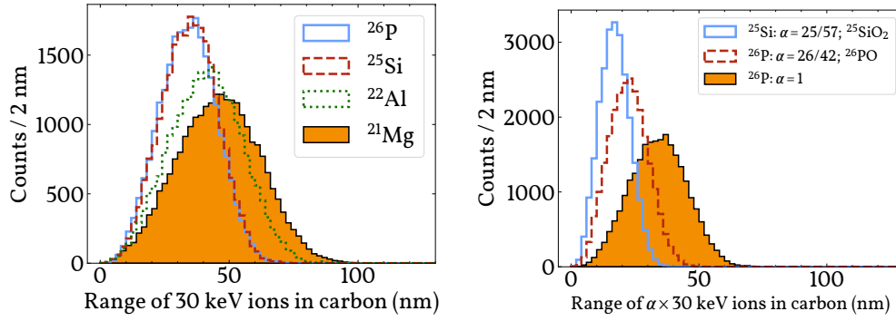
Figure 5.10: Ranges of low-energy ions with initial kinetic energies E_{\text{kin}} = \alpha \times 30 \text{ keV} in carbon with \alpha \leq 1 . Left: The distributions from figure 2.1 are redrawn for comparison with the right part of this figure ( \alpha = 1 for all of the shown distributions). Right: The range of a 30 keV beam of ^{26}\text{P} is illustrated compared to the ranges of an 18.6 keV beam of ^{26}\text{P} and a 13.1 keV beam of ^{25}\text{Si} . These latter two beam energies were effectively the beam energies of the two nuclides, as the ions ^{26}\text{PO}^+ and ^{25}\text{SiO}_2^+ were mass-selected just after the gas cell and then sent to our setup. When the ionised molecules impinge on our carbon foil, the molecular binding energy of, at most, a couple of eV [WA82, pages F180-200] is broken, and the atoms advance into the foil with reduced kinetic energies given by their mass fractions. As in figure 2.1, TRIM has been used to generate the distributions.
