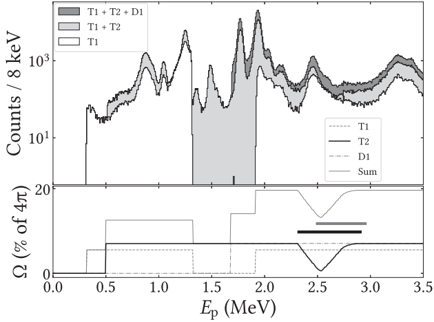
Fig. 6. Top: Beta-delayed proton energy spectrum of ^{21}\text{Mg} at low to intermediate proton kinetic energies E_p as observed by two detector telescopes and one thick DSSD. The data are from the same experiment as referenced in Fig. 2 where protons emitted from excited states in ^{21}\text{Na} are primarily observed. In the figure legends, T1 is short for 42 \mu\text{m} telescope, T2 is short for 67 \mu\text{m} telescope, and D1 is short for 1000 \mu\text{m} DSSD. Bottom: The corresponding energy-dependent solid angle coverage \Omega of the detector telescopes and the thick DSSD. The extents of the spurious zone (black) and the dead zone (grey) are indicated for the 67 \mu\text{m} telescope with the thick lines lying between 2.3 and 3.0 MeV. Taken as a whole, the top and bottom panels illustrate the results of properly accounting for all challenges, as described in this paper, associated with extending the energy spectra of detector telescopes below their punch through thresholds. The variations in solid angle coverage with energy can, if they are not taken into consideration, give a misrepresentation of the underlying nuclear structure. See text for a more detailed discussion.
