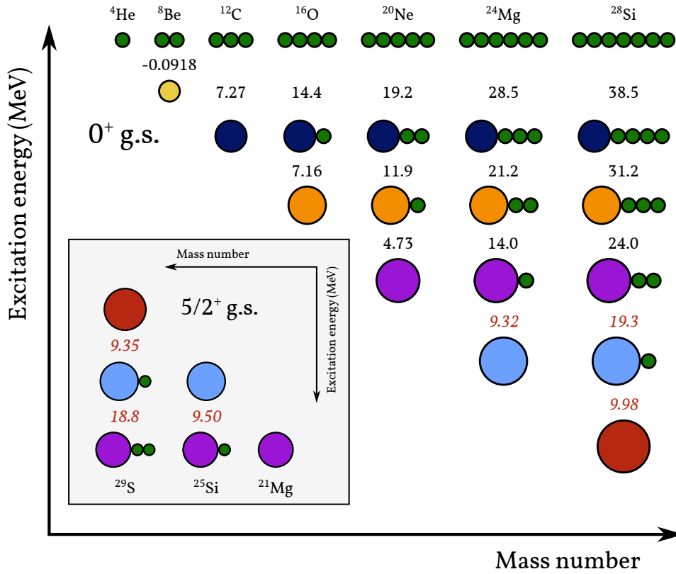
Figure 9.2: Ikeda diagram of the classical {}^4\text{He} - {}^8\text{Be} - {}^{12}\text{C} -...-chain and of a potential parallel in the sd-shell nuclei {}^{21}\text{Mg} , {}^{25}\text{Si} and {}^{29}\text{S} . See text.
