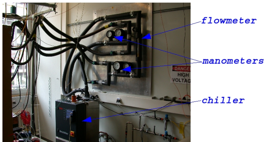
Figure 4.2: Overview of the cooling system of the burn-in test stand.
