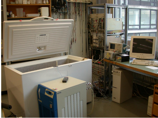
Figure 3.13: Photograph of the laser test stand setup.
