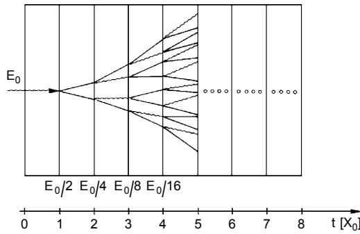
(a) Simplified Model
