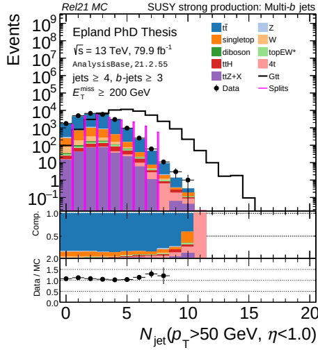
(a) N_{\text{jet}}(p_T > 50 \text{ GeV}, \eta < 1.0)
