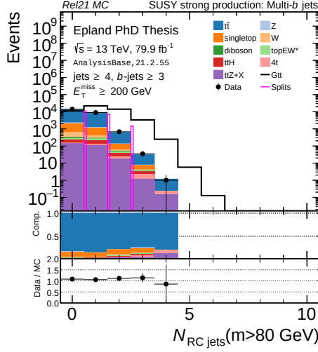
(a) N_{\text{RC,jet}}(m > 80 \text{ GeV})
