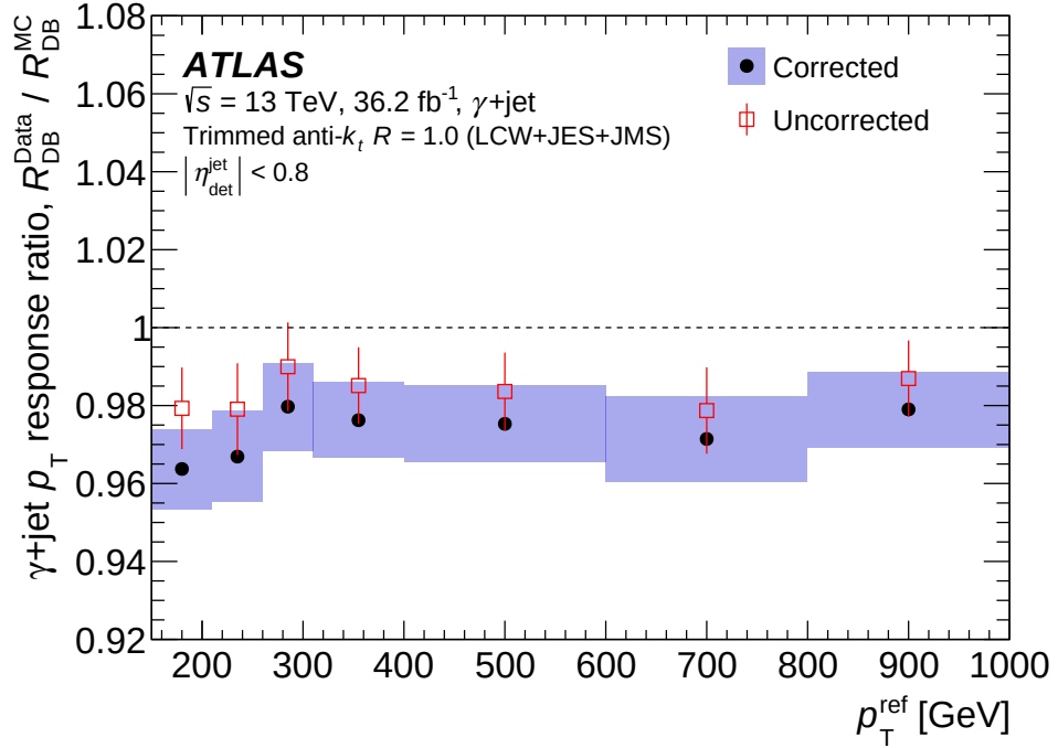
FIGURE E.4: \gamma +jet response with and without photon purity correction [225].
