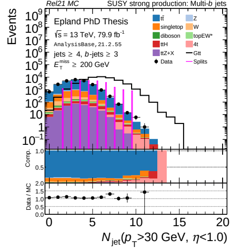
(b) N_{\text{jet}}(p_T > 30 \text{ GeV}, \eta < 1.0)
