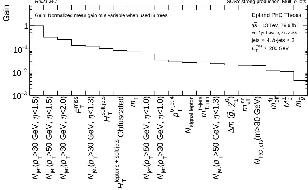
FIGURE 5.2: Input variables used by the BDT in order of relative gain across all mass points.
