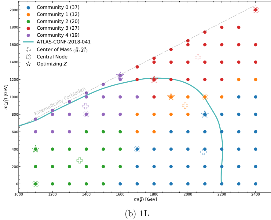
FIGURE 5.4: Positions of representative parameter points (stars) in the 0L and 1L channel with the center-of-mass and central node also shown for reference.
