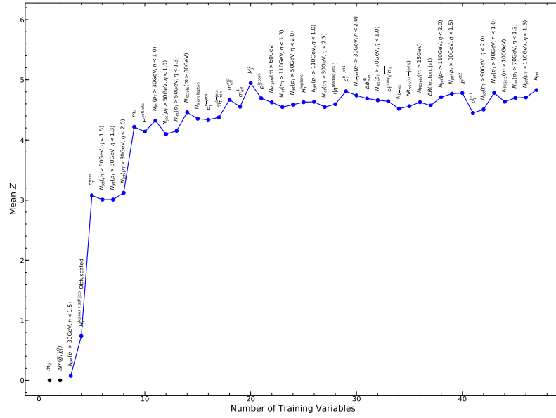
FIGURE A.8: BDT performance measured via mean Z_B on selected mass points during the iterative input variable selection process.
