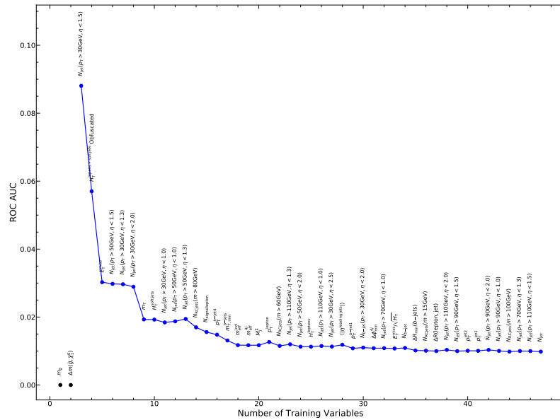
FIGURE A.9: BDT performance measured via ROC AUC during the iterative input variable selection process.
