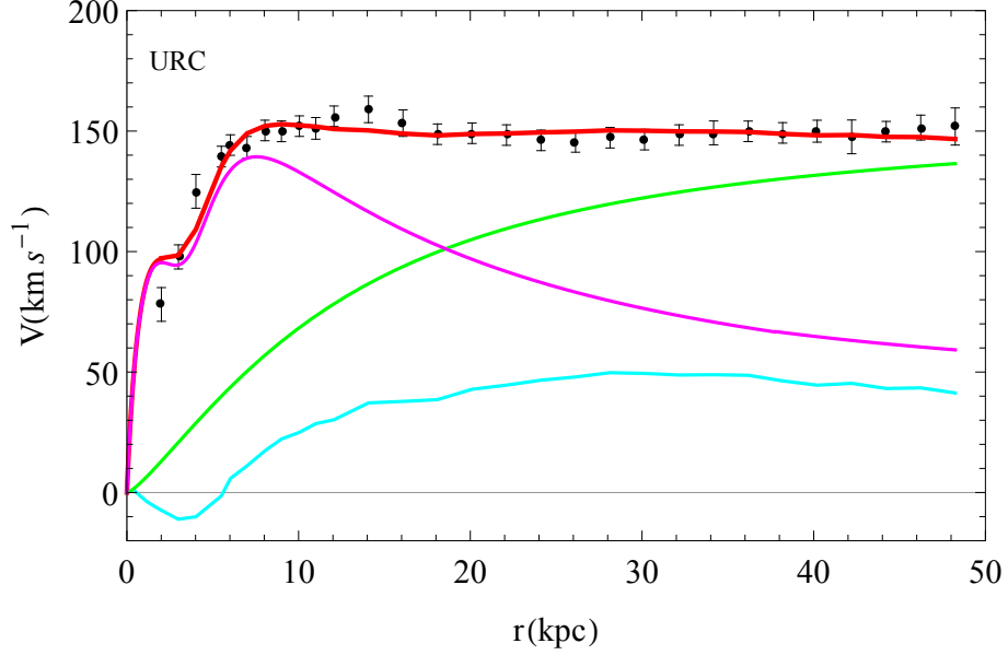
FIGURE 2.9: Rotation curve of the NGC 3198 galaxy [61]. The data points and model (red) with stellar disk (magenta), halo (green), and hydrogen line disk (azure) components are shown. The velocity of an object in orbit a distance r from the center of a galaxy should go as v(r) \propto \sqrt{M_{\text{enc}}(r)/r} , dropping as 1/\sqrt{r} outside the of the visible galactic core. However, as seen here v(r) is approximately constant out to very large distances. This can be explained through the introduction of the DM halo.
