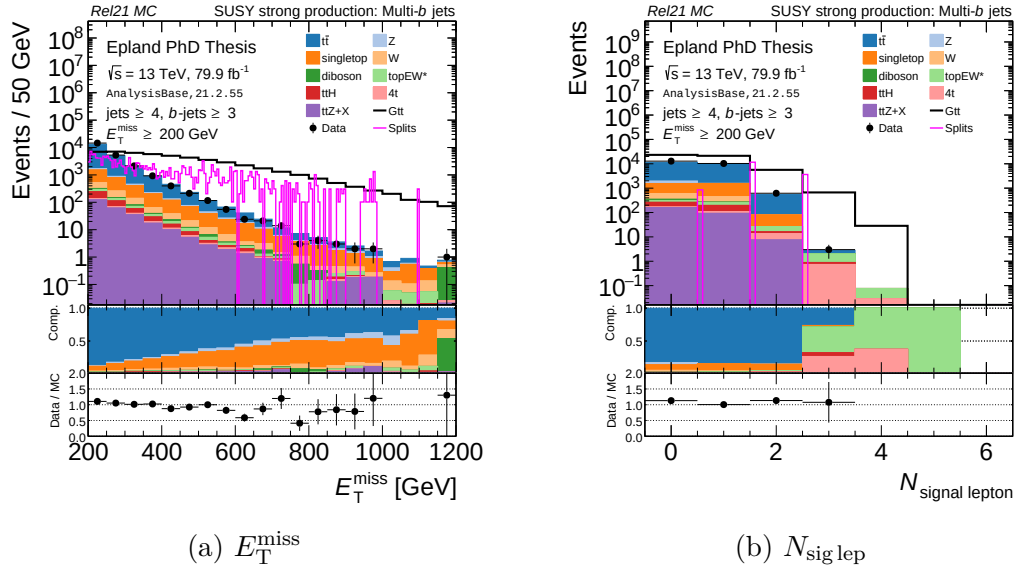
FIGURE A.55: E_T^{\text{miss}} and N_{\text{sig lep}} in data & MC with BDT split values.
