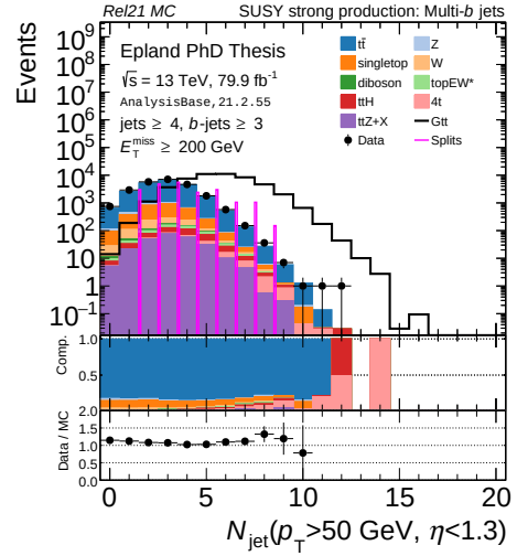
(b) N_{\text{jet}}(p_T > 50 \text{ GeV}, \eta < 1.3)
