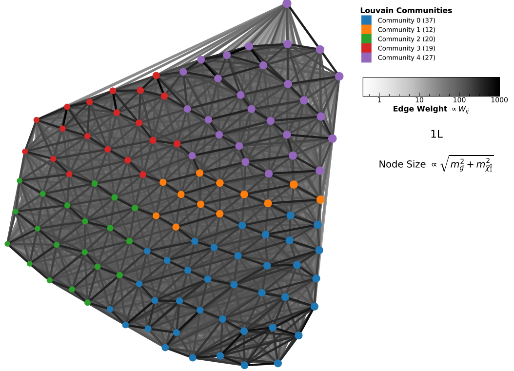
FIGURE A.13: Graph of mass parameter points and Louvain communities in the 1L channel. The position of nodes is set via a spring relaxation algorithm and their size corresponds to their masses. The edge shading is proportional to W_{ij} and is darker for stronger edges.
