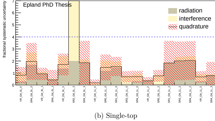
FIGURE A.28: Initial event-driven theory systematic uncertainties for t\bar{t} and single-top. The t\bar{t} uncertainties include parton shower, radiation, and generator systematic components, while single-top includes radiation and interference. The quadrature sum, with error, is also displayed. SR bins with a quadrature sum plus error greater than the blue dashed thresholds are removed from the fit before unblinding. Such SR bins in the t\bar{t} uncertainty, including all of Gtt_0L_4, have already been removed from the single-top results shown here. Gtt_1L_1, Gtt_0L_2, and Gtt_1L_4 were removed for other reasons detailed in Section 5.8.
