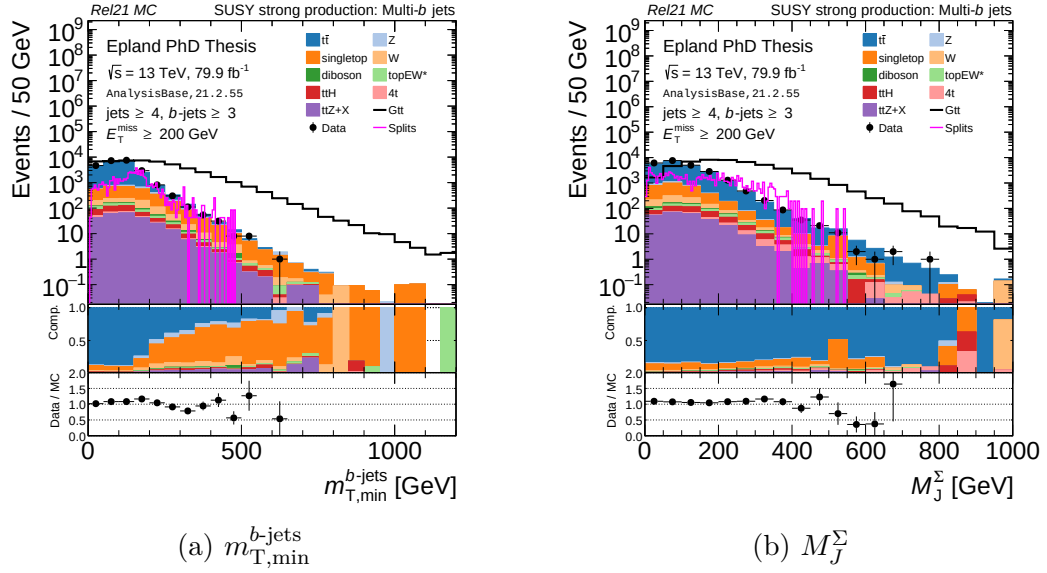
FIGURE A.59: m_{T,\min}^{b\text{-jets}} and M_J^\Sigma in data & MC with BDT split values.
