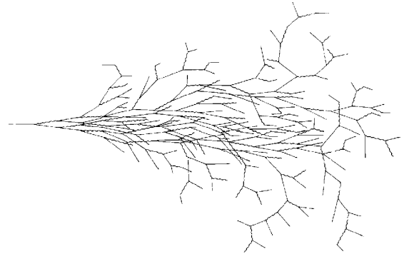
(b) Realistic Model
