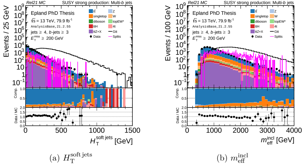
FIGURE A.58: H_T^{\text{soft jets}} and m_{\text{eff}}^{\text{incl}} in data & MC with BDT split values.
