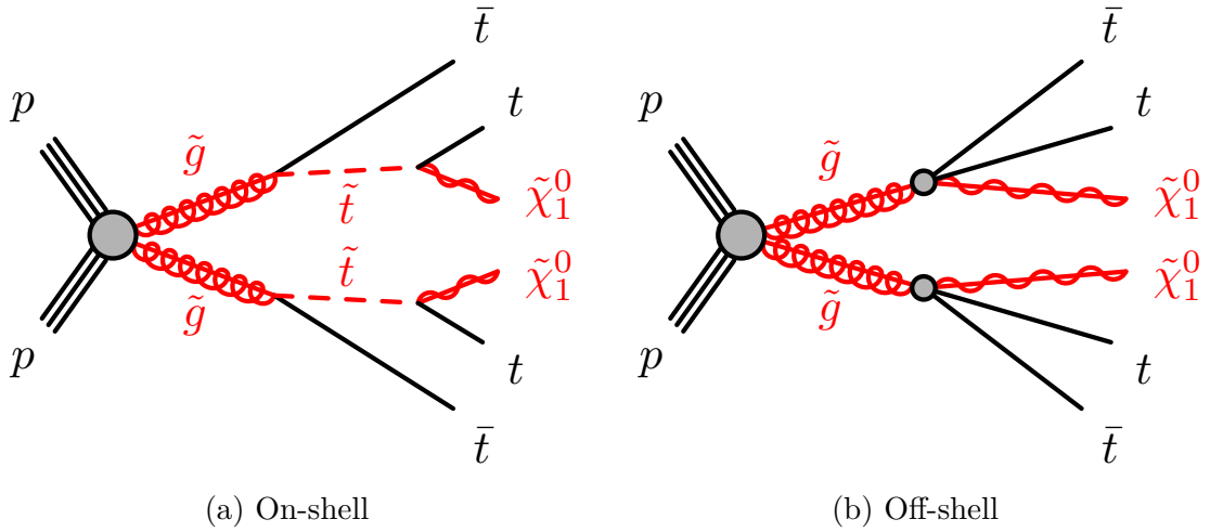
FIGURE 2.15: Feynman diagrams of \tilde{g} \rightarrow t\bar{t} \rightarrow t\bar{t}\tilde{\chi}_1^0 decay in a simplified SUSY model for on and off-shell \tilde{t}_1 . The final state consists of four tops plus E_T^{\text{miss}} in the form of two \tilde{\chi}_1^0 LSPs.
