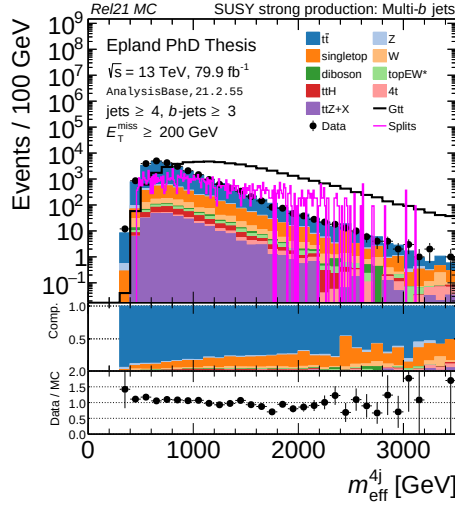
(a) m_{\text{eff}}^{4j}
