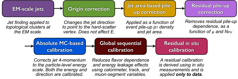
FIGURE 4.6: The calibration sequence for small- R jets [143].
