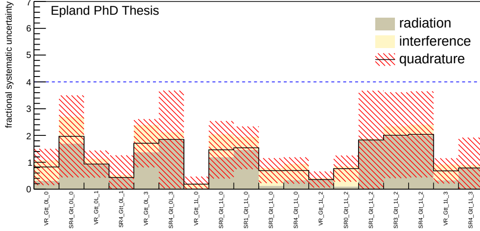
(b) Single-top
