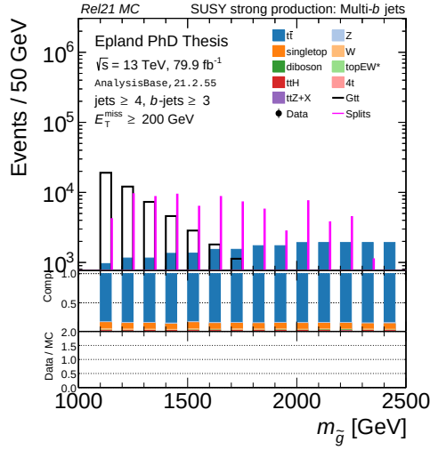
(a) m_{\tilde{g}}
