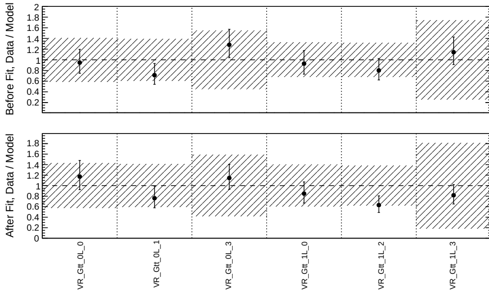
(a) Selected Regions
