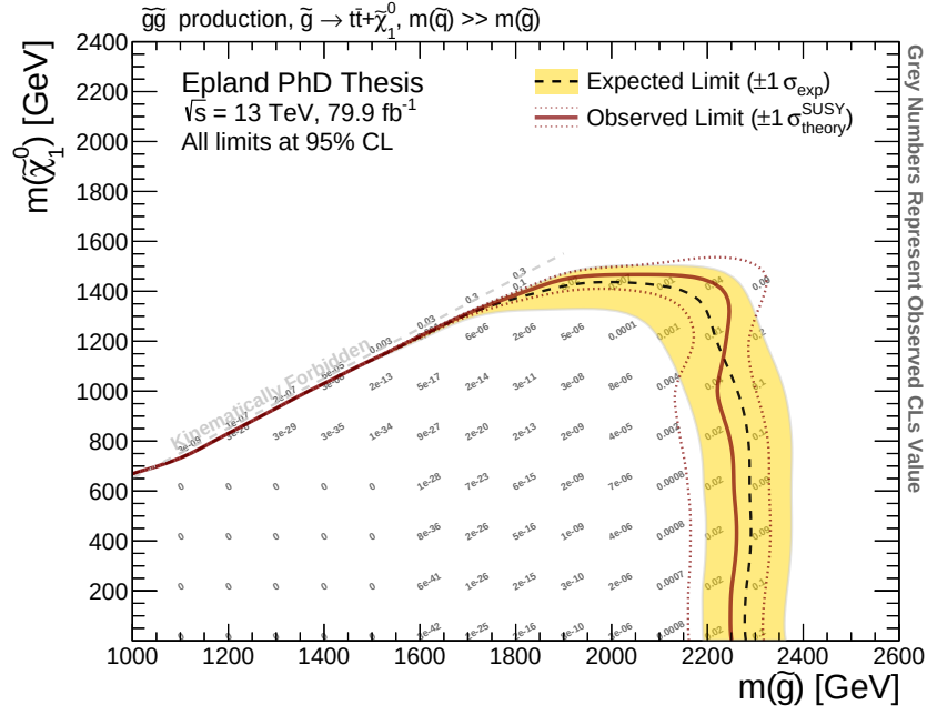
(a) CL_s Limits
