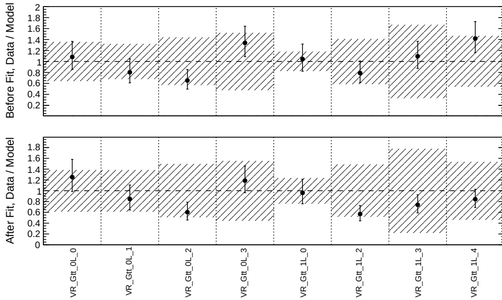
(b) All Regions (Blinded)
