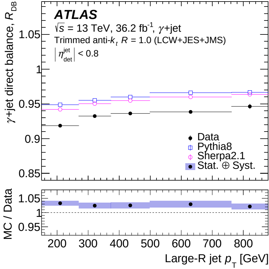
FIGURE E.5: Mean \gamma +jet transverse momentum balance in data and MC, and their ratio [218]. The error bars on the upper inset only show the statistical uncertainty, while those on the lower inset include the systematic uncertainties.
