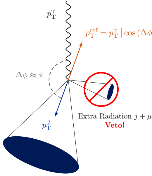
FIGURE E.1: Schematic representation of a well balanced \gamma +jet event.
