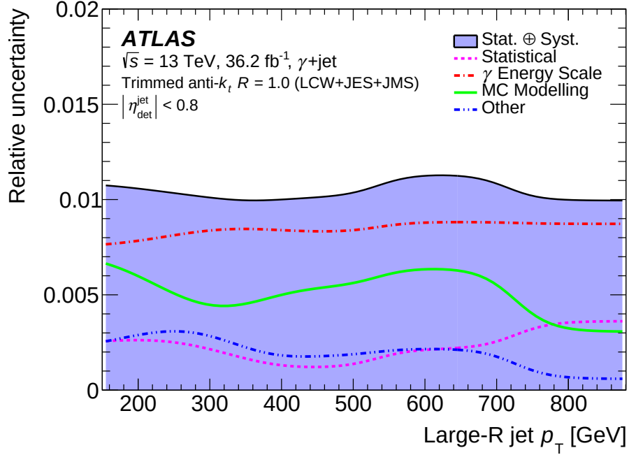
FIGURE E.6: Systematic and statistical uncertainties on the \gamma +jet transverse momentum balance [218]. Smoothed with a Gaussian kernel of width 70 GeV.
