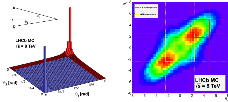
Figure 3.3: Simulated b\bar{b} production angles at LHCb. Left: forward-backward productions fractions as functions of b angles to the beam axis. LHCb acceptance is marked in red. Right: Distribution of pseudorapidities for b\bar{b} pairs with LHCb acceptance marked in red.
