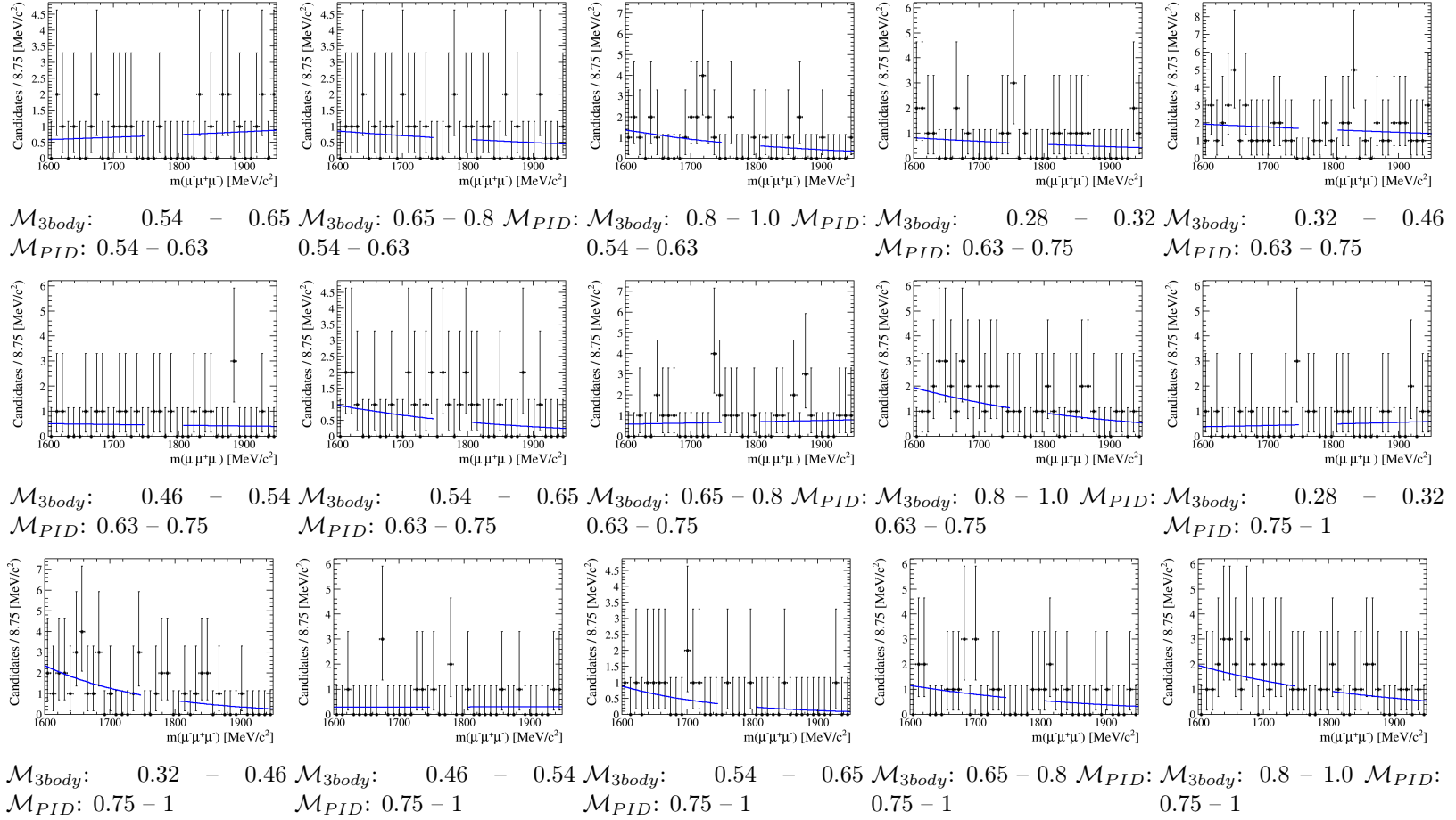
Figure 4.12: Distributions of tri-muon invariant mass (data points) in bins of (\mathcal{M}_{3body}, \mathcal{M}_{PID}) variables for the \tau^- \rightarrow \mu^-\mu^+\mu^- data in 2011 after D_s^- \rightarrow \eta(\mu^-\mu^+\gamma)\mu^-\nu_\mu veto. The blue-solid line shows the results of the fit to an exponential p.d.f. performed in the sidebands of the tri-muon invariant mass.
