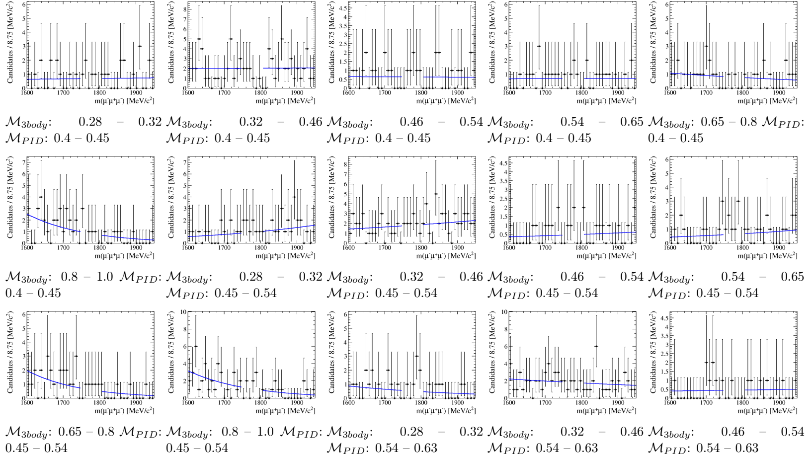
Figure 4.11: Distributions of tri-muon invariant mass (data points) in bins of (\mathcal{M}_{3body}, \mathcal{M}_{PID}) variables for the \tau^- \rightarrow \mu^- \mu^+ \mu^- data in 2011 after D_s^- \rightarrow \eta(\mu^- \mu^+ \gamma) \mu^- \nu_\mu veto. The blue-solid line shows the results of the fit to an exponential p.d.f. performed in the sidebands of the tri-muon invariant mass. Continued in Fig. 4.12.
