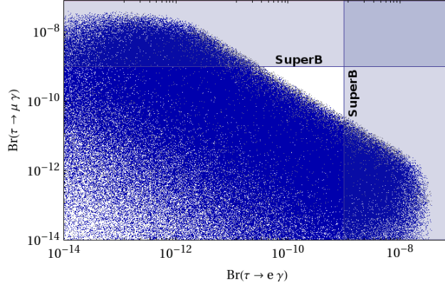
Figure 2.4: Correlation between branching fractions of \tau \rightarrow \mu \gamma and \tau \rightarrow e \gamma decays in the 4 th generation model [51]. Here the sensitivity of the proposed SuperB experiment [52] was marked as blue bands.
