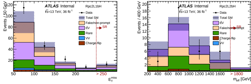
(c) Rpc2L1bH before the E_T^{\text{miss}} requirement re- (d) Rpc2L2bH before the m_{\text{eff}} requirement
