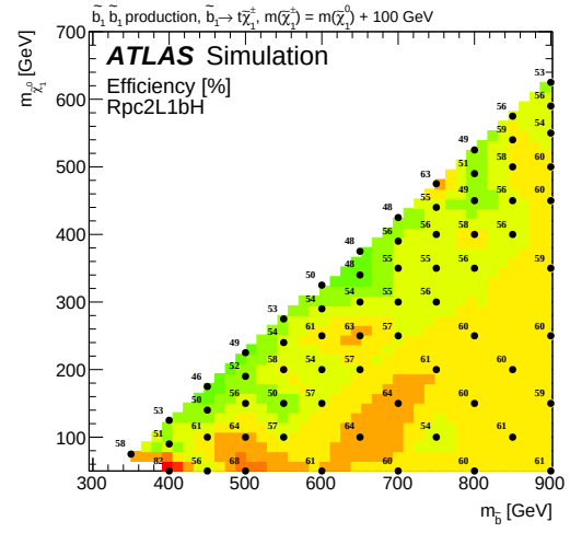
(b) Rpc2L1bH efficiency
