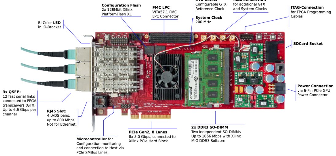
Figure 4.2: Photo of the C-RORC board with the major components and features annotated [4].
