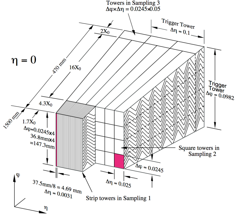
Figure 3.9: Sketch of the accordion structure of the LAr EM calorimeter where the different layers are clearly visible. The granularity in \eta and \phi of the cells of each of the three layers is shown.
