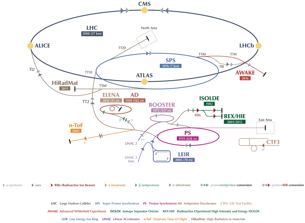
Figure 3.1: The CERN accelerator complex composed of a chain of particle accelerators with the LHC as the last ring (dark blue line) [2].
