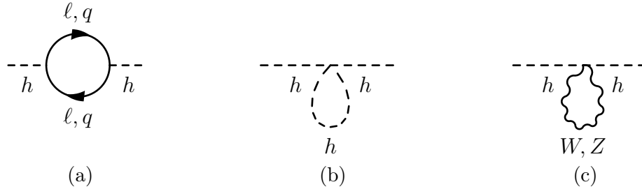
Figure 2.2: The one-loop contribution of (a) quarks and leptons, (b) Higgs bosons, and (c) W, Z bosons to the mass of the Higgs bosons.
