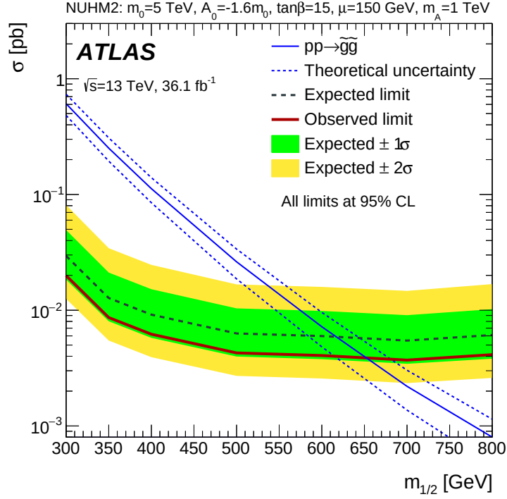
Figure 9.8: Observed and expected exclusion limits as a function of m_{1/2} in the NUHM2 model [7, 8]. The signal region Rpc2L2bH is used to obtain the limits. The contours of the green (yellow) band around the expected limit are the \pm 1\sigma ( \pm 2\sigma ) results, including all uncertainties. The limits are computed at 95% CL.
