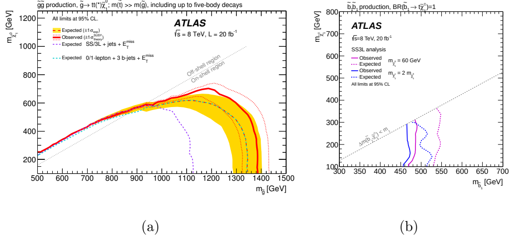
Figure 5.2: Exclusion limits on the gluino-stop offshell [5] (left) and direct sbottom [6] (right) scenarios set by ATLAS with the 2012 dataset prior to the author’s work.
