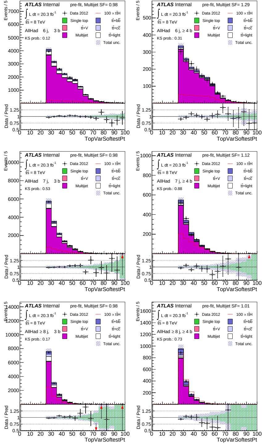
Figure B.27: p_T^{\text{softest jet}} pre-fit.
