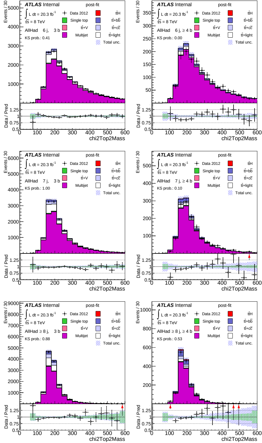
Figure B.24: m_{\text{top},2} post-fit.
