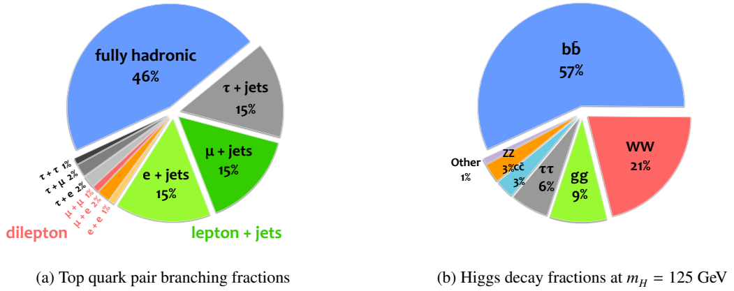
Figure 5.1: (a) Pie chart representing the branching ratios (BR) of a top-antitop quark pair. The light blue represents the fully hadronic BR of 46% (56% when including hadronic decaying \tau ), the dileptonic BR (without \tau lepton) is shown in 3 shades of red, with a total of 4% (6.4% when including leptonic decaying \tau ), and in 2 shades of green the lepton ( e or \mu ) + jets BR of 30% (36% when including leptonic decaying \tau ). (b) Pie chart representing the branching ratios of the Higgs boson, assuming a mass of 125 GeV.
