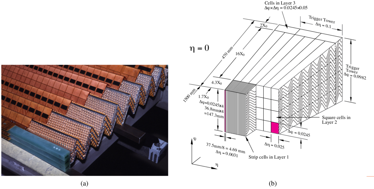
Figure 3.10: A photo (a) and a diagram (b) of the ATLAS liquid argon calorimeter, showing the accordion structure and the different granularity in the different layers [58].
