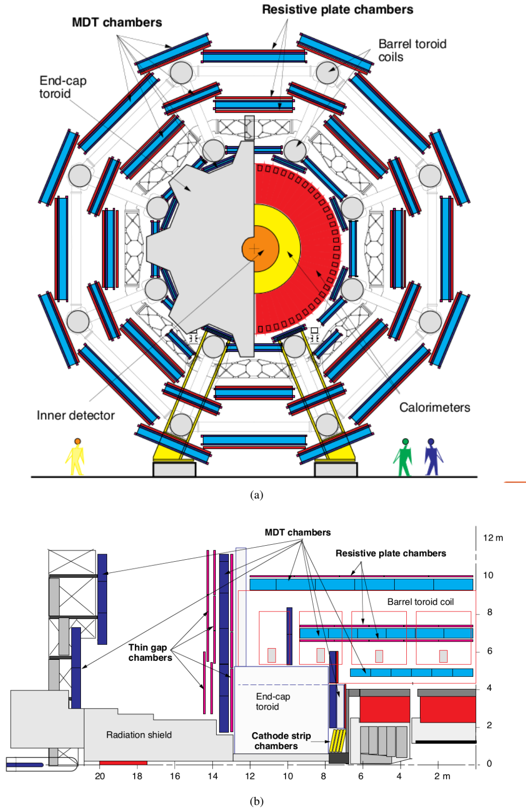
Figure 3.12: Layout of the muon spectrometer (a) in the x - y plane and (b) in the y - z plane [65]: The lower illustration shows a quarter of the y - z plane only, with the interaction point located in the lower right corner.
