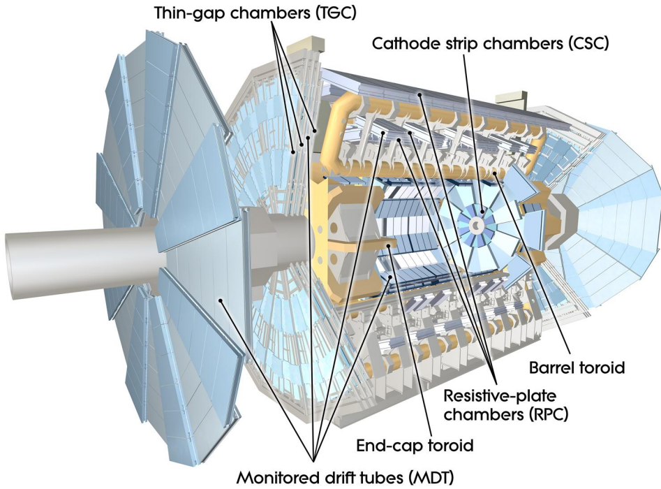
Figure 3.11: A schematic of the ATLAS muon spectrometer [58].
