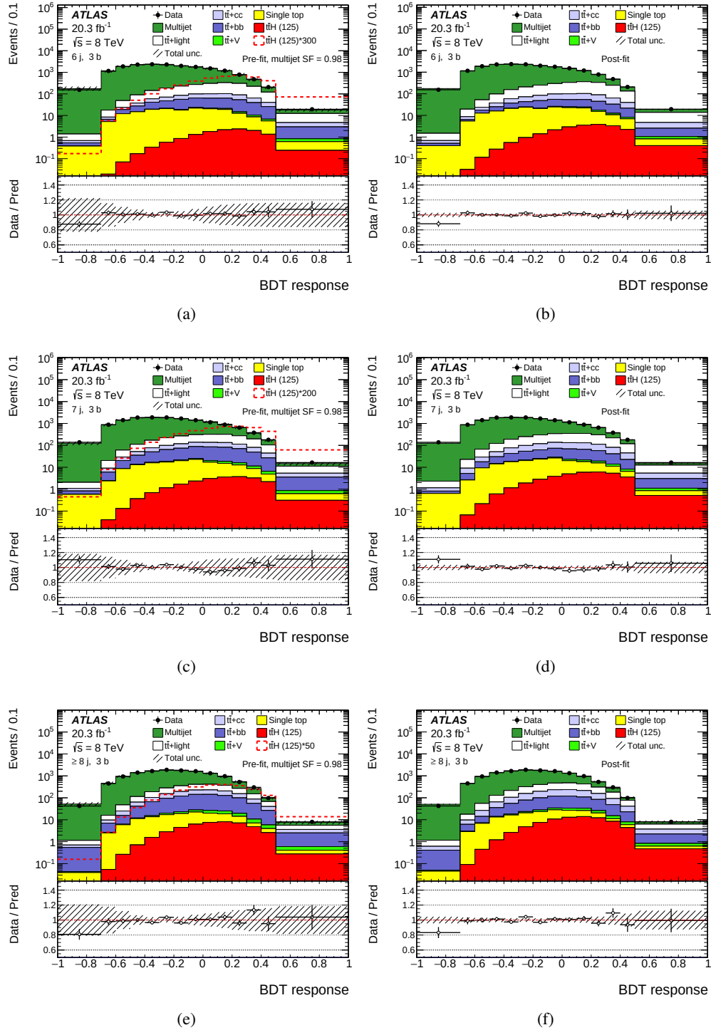
Figure 5.20: Comparison between data and prediction for the BDT discriminant in the, from top to bottom, (6–8j, 3b) regions before (left) and after (right) the fit. The fit is performed under the signal-plus-background hypothesis. Pre-fit plots show an overlay of the multijet distribution normalised to data for illustration purposes only. The bottom panels display the ratios of data to the total prediction. The hashed areas represent the total uncertainty in the background predictions, containing the statistical and systematic contribution. The binning is the same as that used in the fit [104].
