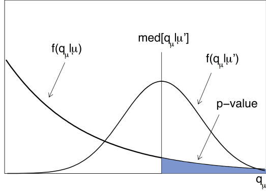
Figure 4.6: Illustration of the p -value corresponding to the median of t_\mu (called q_\mu in the figure) assuming a strength parameter \mu' [98].
