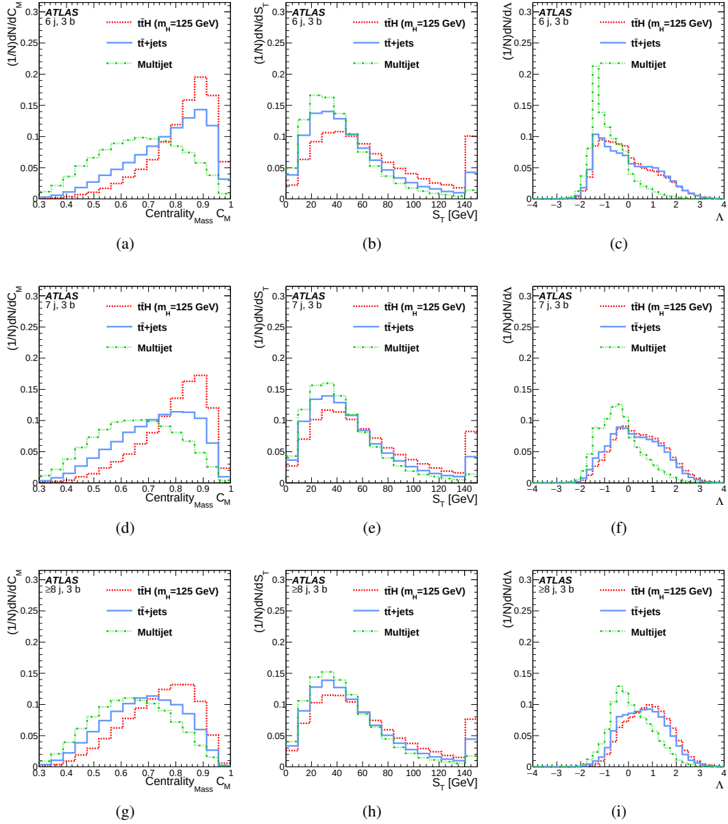
Figure 5.10: Distribution of the most discriminant variables entering the BDT in the 3 b -tag regions (( 6j,3b ) in (a)-(c), ( 7j,3b ) in (d)-(f) to ( \geq 8j,3b ) in (g)-(i)). The plots illustrate the separation power: the red histogram indicates the signal, the blue one the t\bar{t} +jets background, and the green one the multijet background. The definitions of the variables are listed in Table 5.4.
