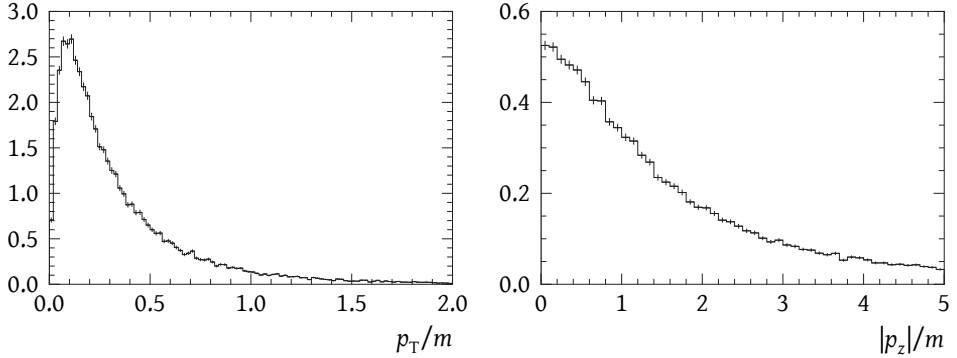
Figure 1.6: Basic kinematic distributions for the production of a standard model-like Brout-Englert-Higgs boson with a mass m of 125 \text{ GeV}/c^2 through the gluon fusion process in 8 TeV pp collisions, generated using PYTHIA8 as described above
