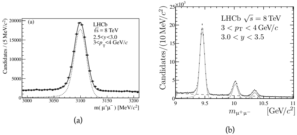
Figure 2.10: Reconstructed \mu^+\mu^- invariant mass spectrum in the region of the (a) J/\psi and (b) Y resonances, figures from [117] and [118], respectively
