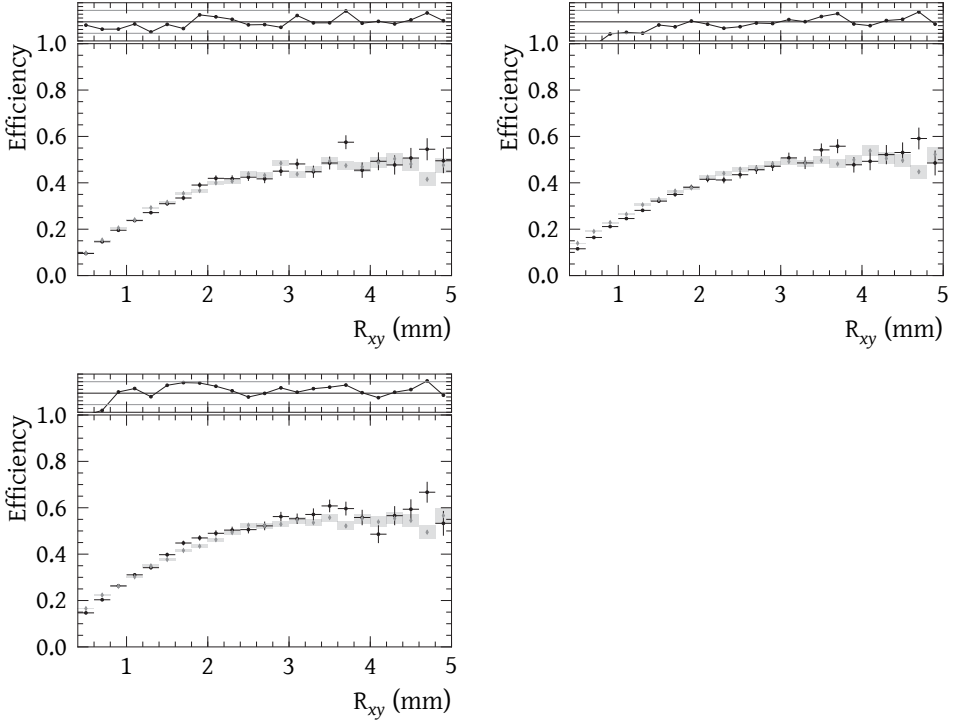
Figure 4.1: Vertex reconstruction efficiency for B^0 \rightarrow J/\psi K^{*0} decays using the 2011 HLT (top left), the 2012 HLT (top right) and the Stripping21 (bottom left) configuration of the displaced vertex finding for data (black circles) and simulation (gray diamonds). The inset shows the efficiency difference, divided by its uncertainty.
