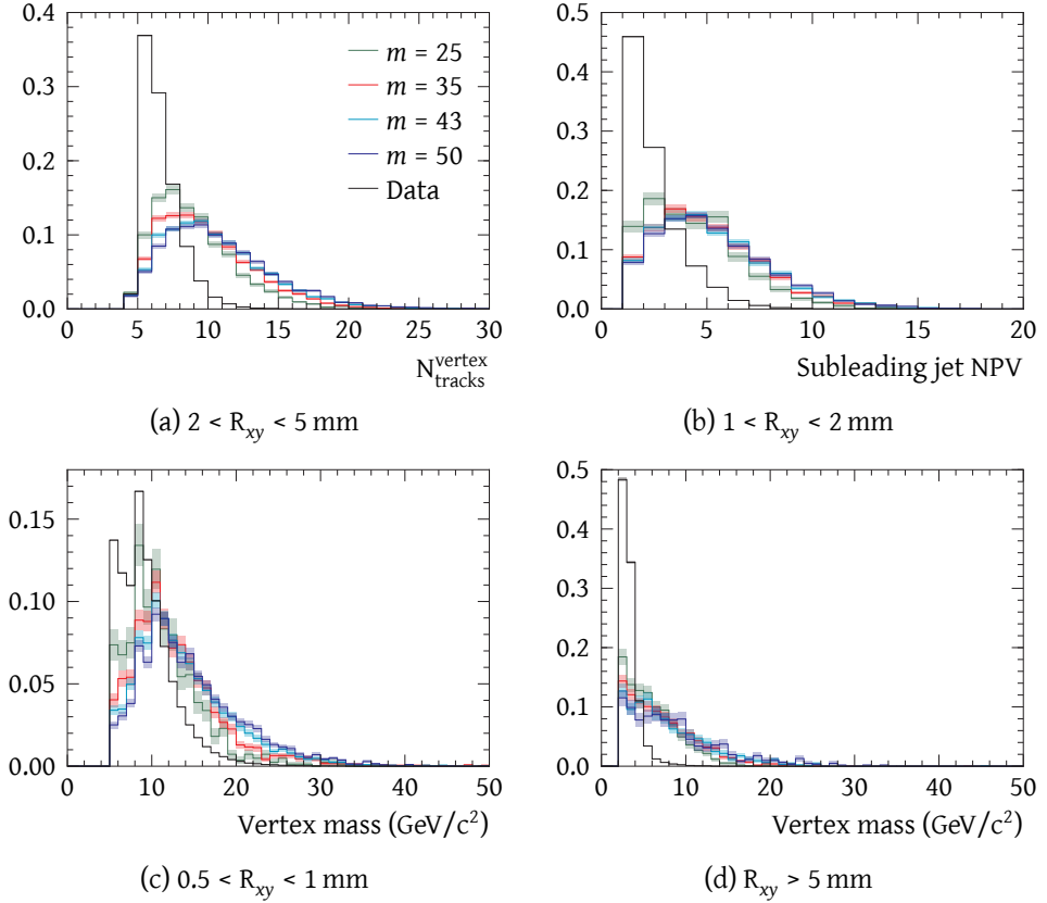
Figure 3.10: Distribution (normalised to unity) of vertex related quantities in different bins of R_{xy} for 2012 data (black) and different \pi_v signal samples with a lifetime of 10 ps (green, red, cyan and blue for a \pi_v mass of 25 \text{GeV}/c^2 , 35 \text{GeV}/c^2 , 43 \text{GeV}/c^2 and 50 \text{GeV}/c^2 , respectively) after preselection (all stripping candidates passing L0, HLT1 and HLT2)
