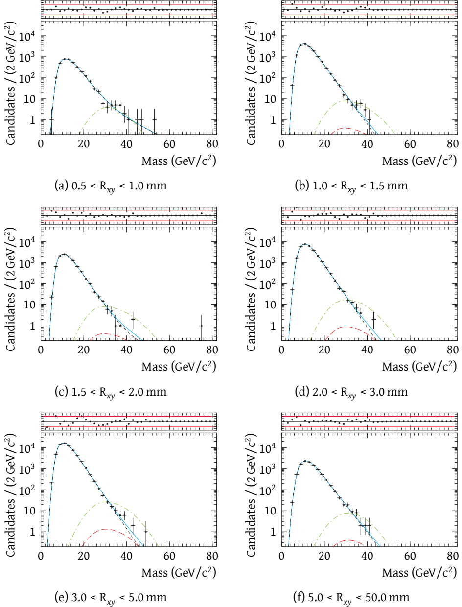
Figure 5.4: Fit to the invariant mass distribution in six bins of R_{xy} for 2012 data (black points) and a signal with \pi_v mass of 35 \text{ GeV}/c^2 and lifetime of 10 ps. The solid blue line indicates the total fit model, whereas the short-dashed black and long-dashed red line show the background and signal components. The long-short dashed green line shows the signal yield expected for a cross-section of 19.24 pb [149].
