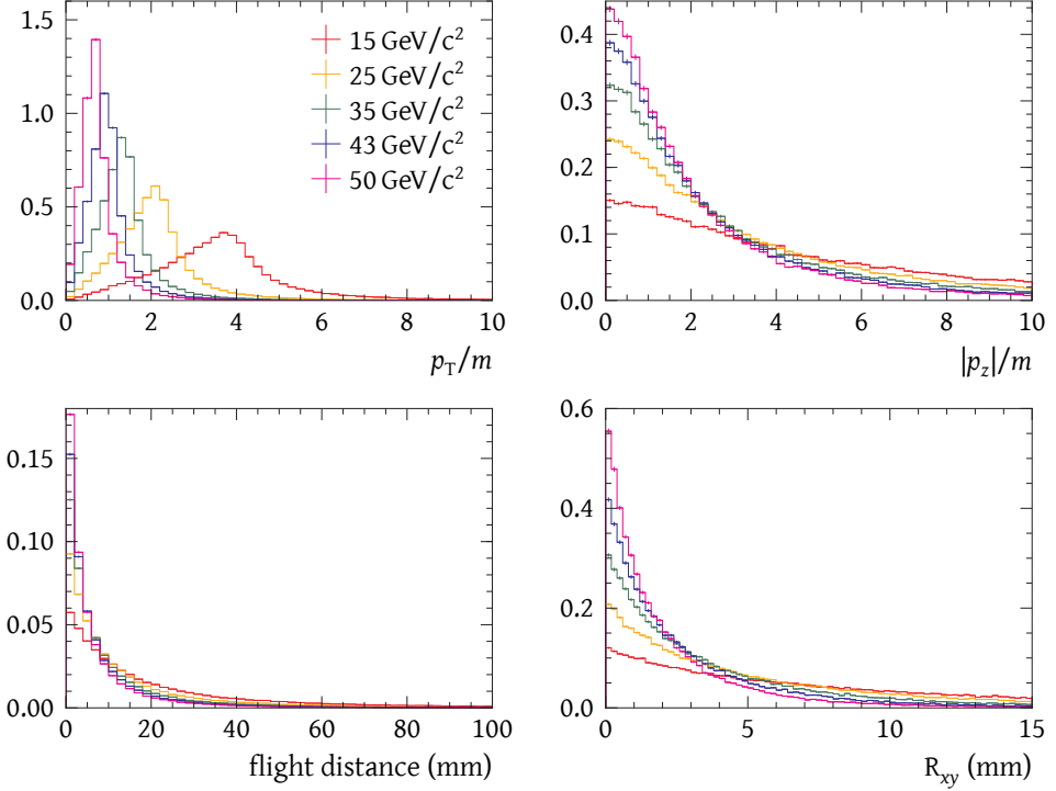
Figure 1.7: Kinematic and lifetime-related distributions for \pi_v particles with a lifetime of 10 ps produced in the decay of a standard model-like Brout-Englert-Higgs boson, for various \pi_v masses
