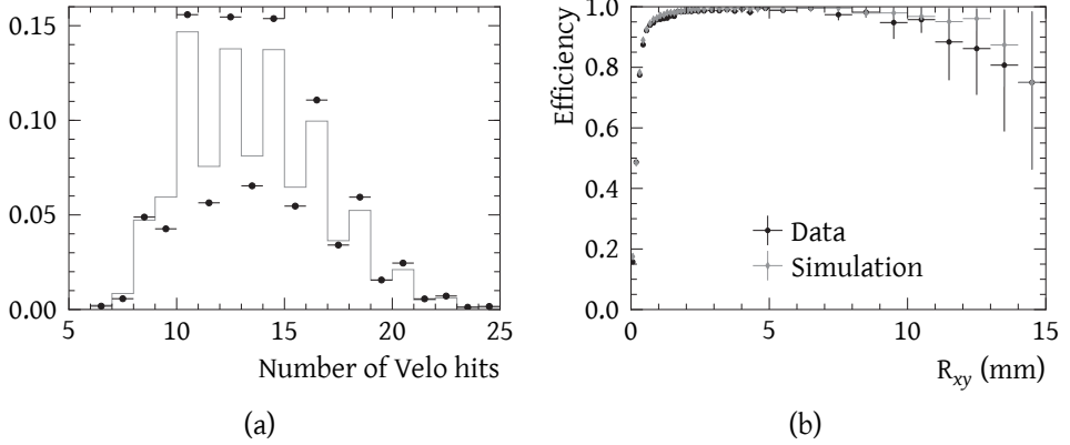
Figure 4.11: Comparison between data and simulation of (a) the number of hits per VELO track, where the markers show the distribution in data, and (b) the topological trigger efficiency versus transverse displacement, both for the dimuon-triggered B^0 \rightarrow J/\psi K^{*0} sample from section 4.1
