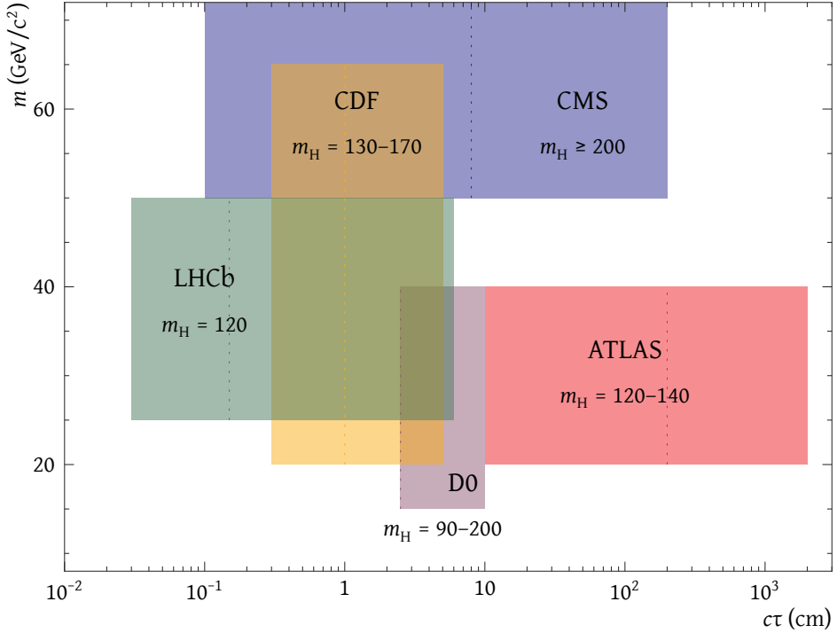
Figure 1.8: Illustration of the parameter space regions probe by different experiments, assuming pair-production of \pi_\nu particles in the decay of a Brout-Englert-Higgs boson, whose assumed mass range (in \text{GeV}/c^2 ) is indicated in each region. The vertical dotted lines indicate the proper lifetime where each search is the most sensitive. For a full comparison, also the sensitivity of each search and the experimental signature, one or two vertices, should be taken into account.
