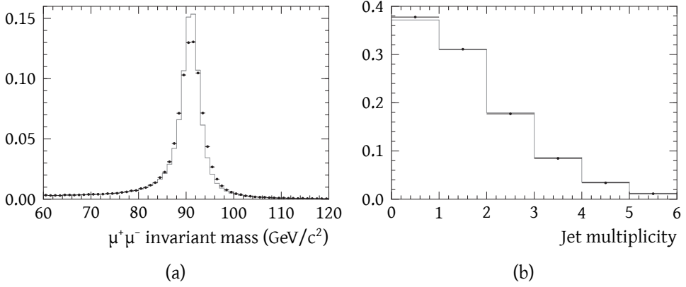
Figure 4.3: Distribution (normalised to unity) of (a) the Z \rightarrow \mu^+\mu^- candidate invariant mass and (b) the number of jets associated to the corresponding primary interaction, for 2012 data (black) and simulation (gray)
