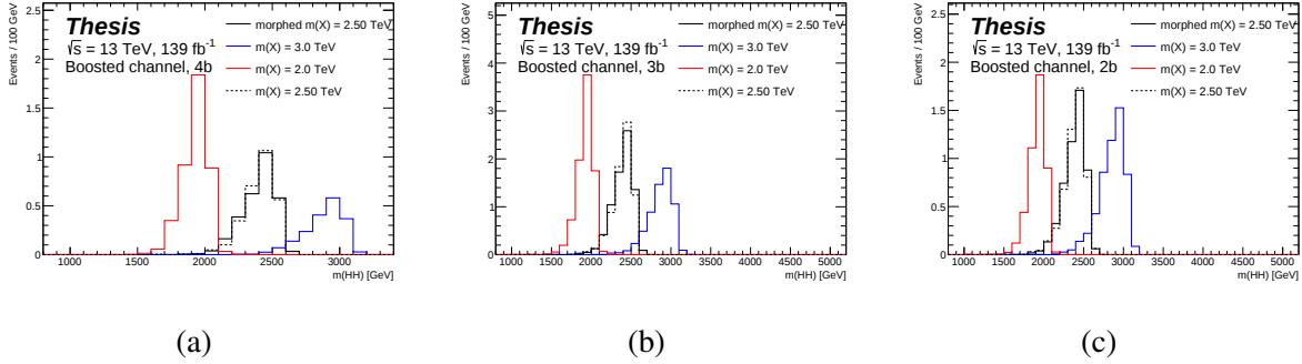
Figure 2.26: Result of using moment morphing to interpolate the 2500 GeV spin-0 signal mass in the (a) 4b , (b) 3b , and (c) 2b -split channels. The 2000 GeV and 3000 GeV mass histograms are used to parametrize the signal. The 2500 GeV spin-0 signal generated from MC is shown for comparison.
