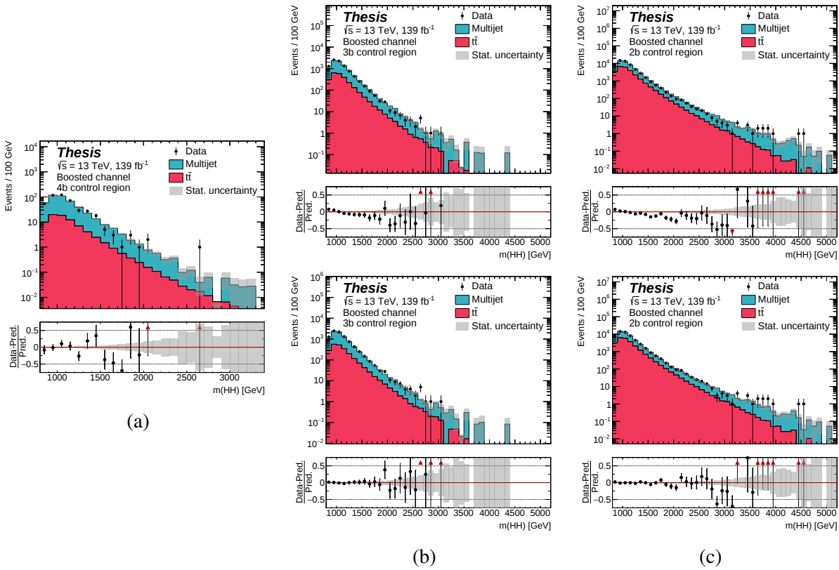
Figure 2.14: HH invariant mass in the (a) 4b , (b) 3b and (c) 2b -split control regions. For the 3b and 2b -split channels, the top plot shows un-reweighted distribution while the bottom plot shows the reweighted distribution. Multijet and t\bar{t} backgrounds are normalized using the \mu_{QCD} and \alpha_{t\bar{t}} values defined in Sec. 2.4.2. The gray band shows only statistical uncertainties.
