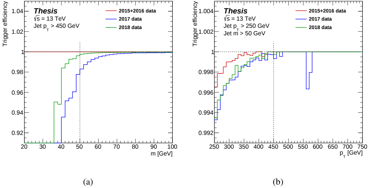
Figure 2.5: Efficiency of the lowest unprescaled Large- R jet trigger as a function of (a) jet mass and (b) jet p_T . Efficiency in each variable is measured in a sample with a fully-efficient cut applied to the other variable. The cuts applied in the analysis, mass > 50 GeV and p_T > 450 GeV, respectively, are indicated by vertical lines.
