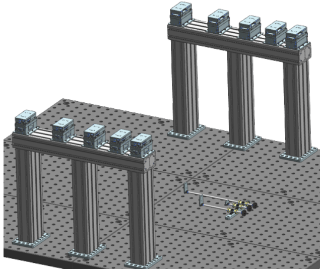
Figure 5.45. | Conceptual design of the DD alignment tooling. The X/Y/Z stages are placed apart by the nominal distance of the DDs. The tilt stages for the first three DDs are shown, the other two DDs will be controlled in the same way from the back side.
