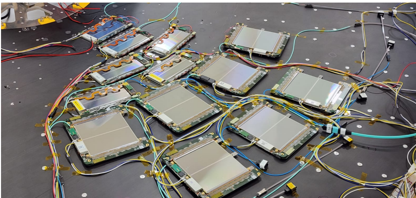
Figure 5.47. | Picture of a partly installed TEDD1 odd top Dee from the pre-integration test at DESY.
