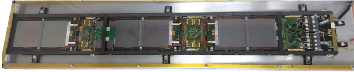
Figure 3.6. | The picture of an assembled TOB rod [20].
