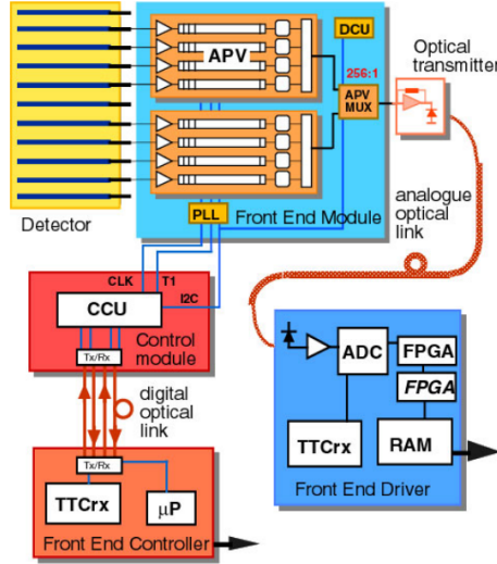
Figure 3.4. | The readout scheme of the SST. From Ref. [20].
