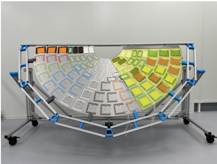
Figure 5.26. | The dee mockup on the dee integration table (the table in the picture is a temporary solution which will be replaced by the final design shown in Figure 5.2).
