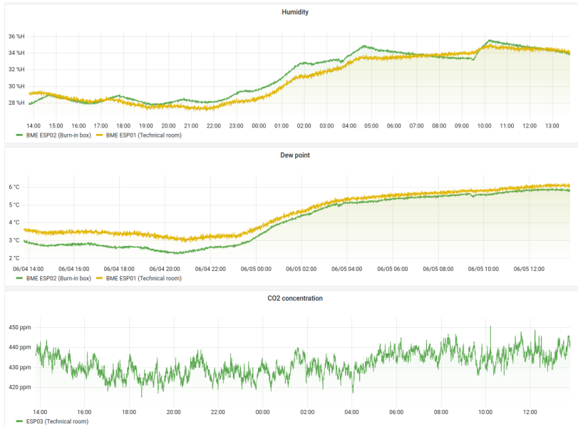
Figure 5.7. | The dashboard created with sensor readout: the humidity levels (top plot) and the dewpoint (middle plot) in the burn-in box and in the technical room, and CO 2 levels in the technical room (bottom plot).
