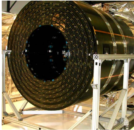
Figure 3.7. | The picture of the naked TOB wheel [20].
