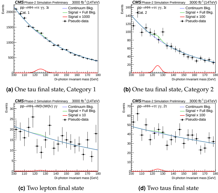
Figure 6.7. m_{\gamma\gamma} distributions in the \tau\tau\gamma\gamma, 1\tau and its two categories (top row) and WW\gamma\gamma, 2L (bottom left), \tau\tau\gamma\gamma, 2\tau (bottom right).
