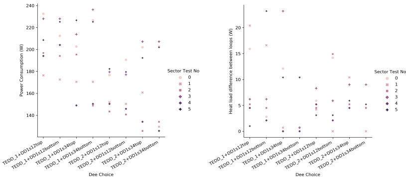
Figure 5.40. | Left: expected power consumption of all sector tests, for different types of dees. Right: differences in the heat load between the two cooling loops for all sector tests. Due to symmetry considerations, other dees inherit the same sector test division as those shown.
