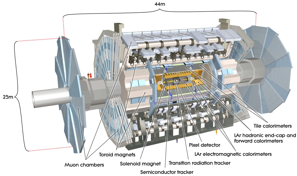
Figure 7: Cut-away view of the ATLAS detector, showing the overall design. From the inner-most to outer-most portions of the detector with respect to the collision point are the inner detector, calorimeters, and muon spectrometer. The overall weight of the apparatus is approximately 7,000 tonnes.
