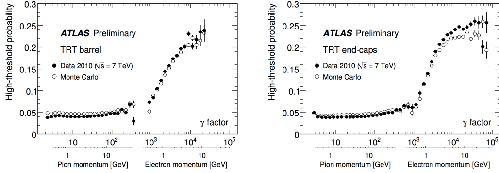
Figure 10: Threshold absorption probabilities for the TRT detector for charged pions and electrons of comparable momentum. This property of the TRT improves electron identification selectivity within the fiducial volume.
