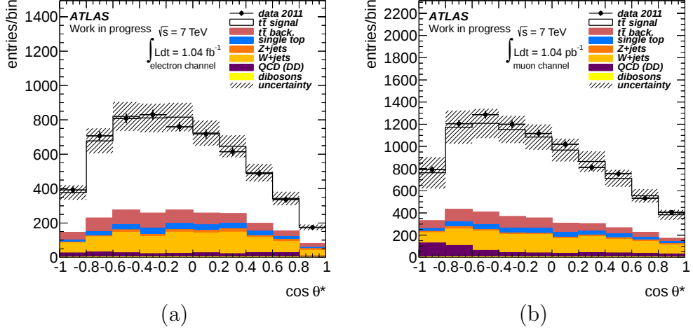
Figure 5.7: \cos \theta^* distributions for the \chi^2 method in the (a) e +jets and (b) \mu +jets channels.
