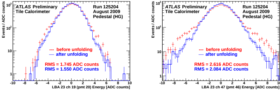
Figure 4.9: LBA23 channels 19 (left) and 47 (right) before and after applying the \chi^2 unfolding.
