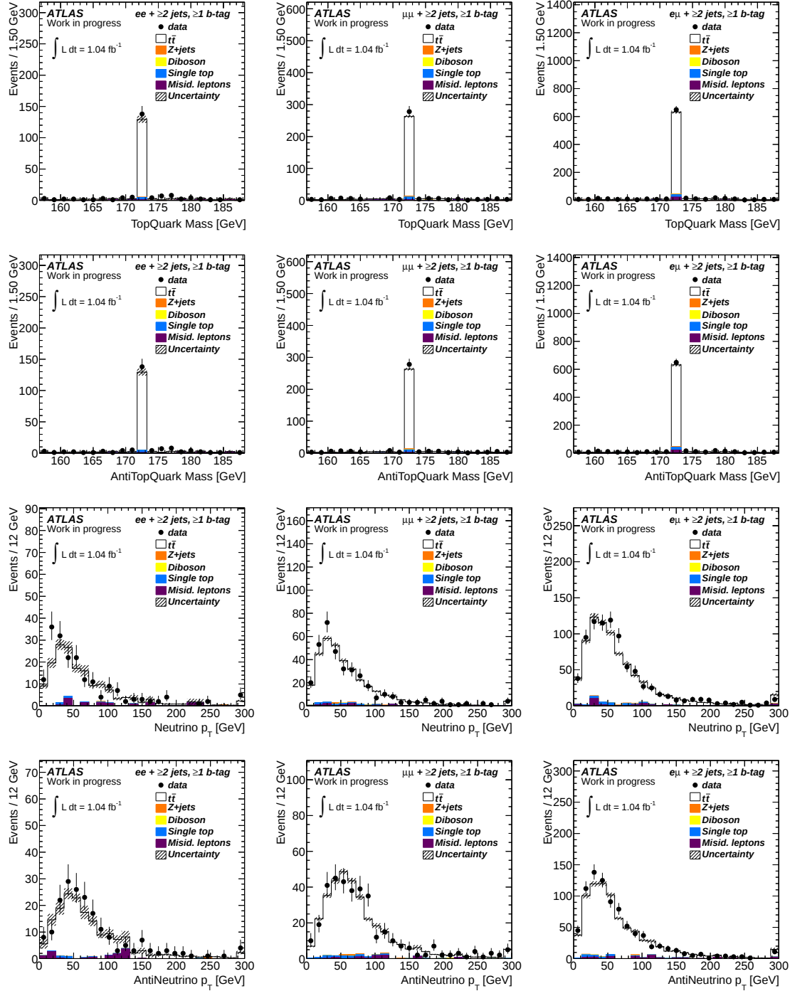
Figure 5.11: Top and anti-top quarks mass distributions, and neutrino and anti-neutrino p_T distributions the e^-e^+ (left), \mu^-\mu^+ (center) and e^\mp\mu^\pm (right) channels.
