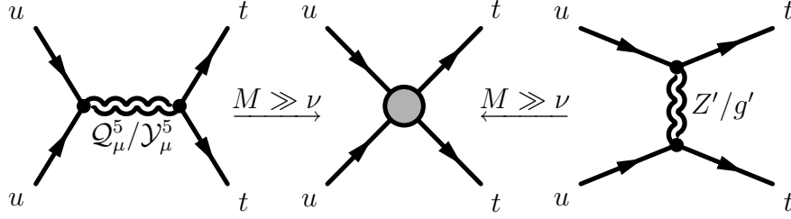
Figure 2.12: Production of same-sign top-quark pairs via the production of a heavy vector boson (such as color-triplet \mathcal{Q}_\mu^5 or color-sextet \mathcal{Y}_\mu^5 ) in the s-channel (left) or exchange of a heavy vector boson (such as Z' or g' ) in the t-channel (right). For large resonance masses, both cases can be described by a four-fermion interaction (middle).
