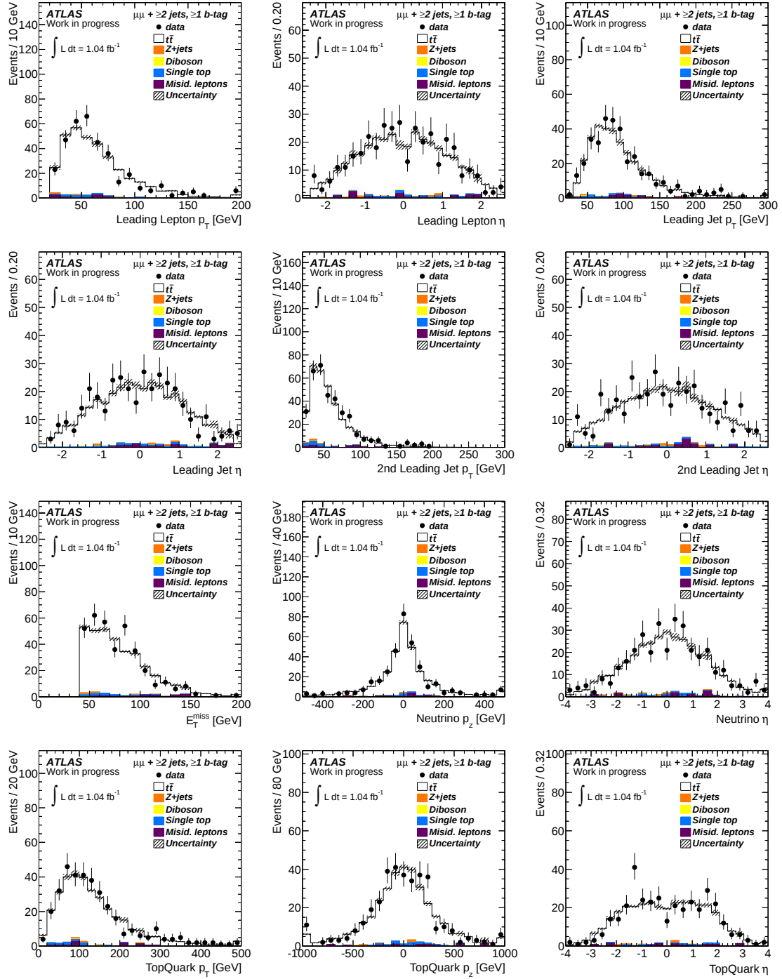
Figure 5.17: Comparison between data and signal+background model in the \mu^- \mu^+ channel after event selection and full t\bar{t} reconstruction. The figures show the distributions of lepton and jet p_T and \eta as well as the missing transverse energy E_T^{\text{miss}} .
