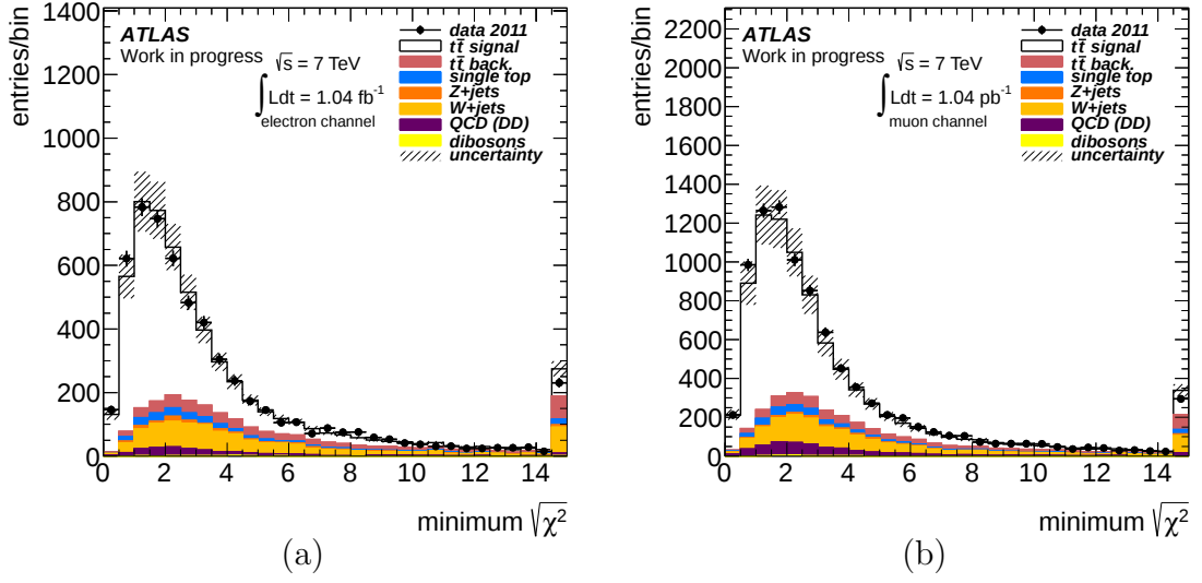
Figure 5.5: \sqrt{\chi^2} distributions for the (a) e +jets and (b) \mu +jets channels.
