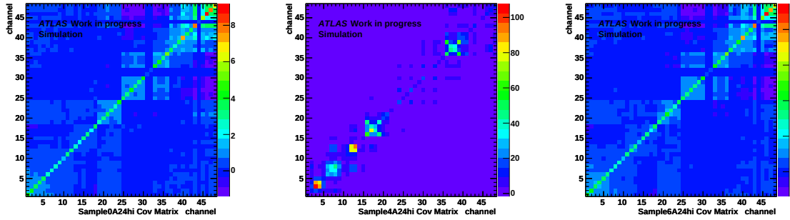
Figure 4.14: Output covariance matrices for Samples 0 (left), 4 (center) and 6 (right) obtained with the simulation of the t\bar{t} sample.
