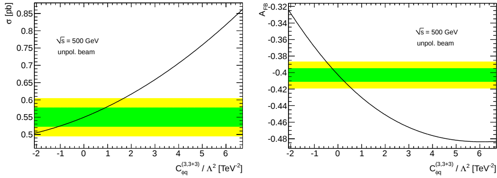
Figure 6.3: Dependence of the unpolarized cross section and FB asymmetry on C_{\phi q}^{(3,3+3)} .
