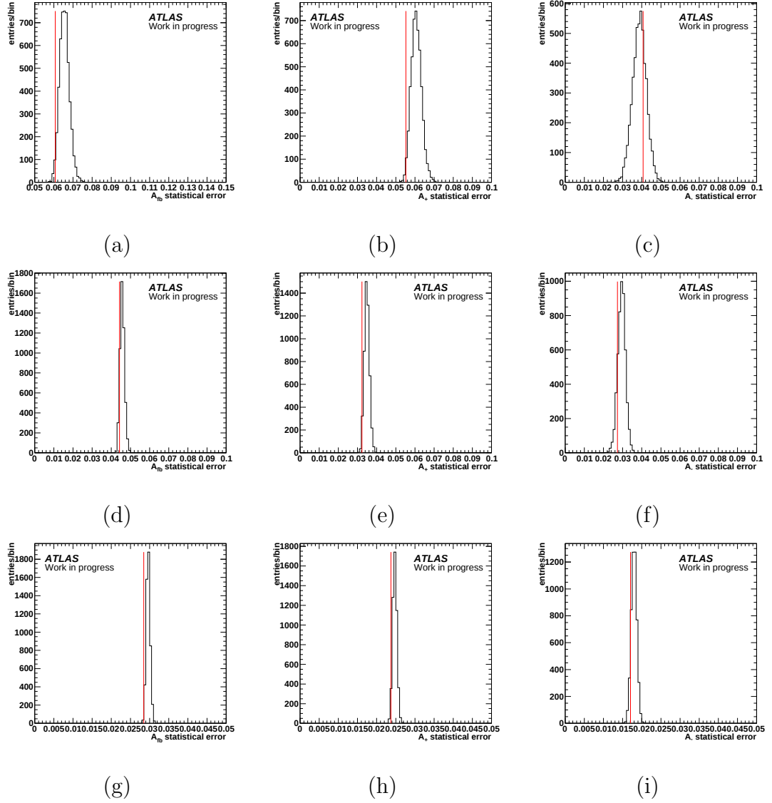
Figure 5.27: Distributions of the expected angular asymmetries statistical errors, obtained for the e^-e^+ channel (upper row), the \mu^-\mu^+ (middle row) and the e^\pm\mu^\pm results (lower row) for the correction function analysis (dilepton topology). 5000 pseudo experiments based on the data distribution of \cos\theta^* were used. The measured error for each observable is represented by the mean value of the distribution.
