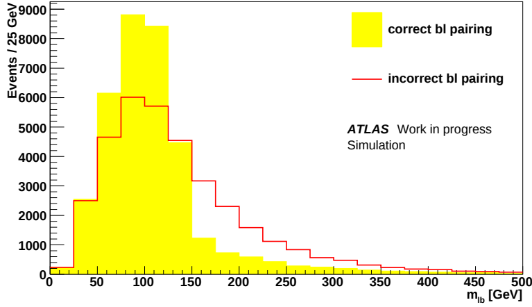
Figure 5.9: The b\ell invariant mass distribution at the reconstruction level is shown for the correct (shaded region) and incorrect (full line) pairing. The distributions are shown at the reconstruction level.
