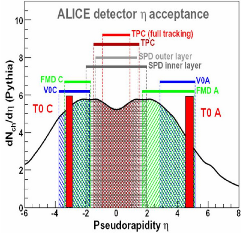
Figure 2.3: Pseudorapidity coverages of different sub-detectors of ALICE [71].
