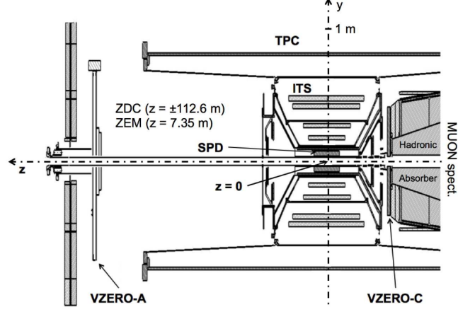
Figure 3.3: Position of the two VZERO arrays, within the general layout of the ALICE experiment [81].
