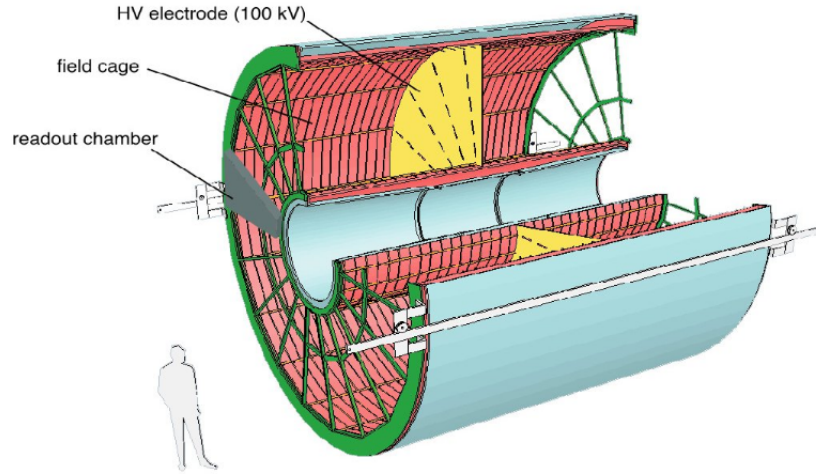
Figure 2.5: The ALICE Time Projection Chamber (TPC) [85].
