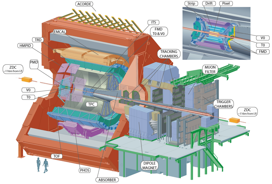
Figure 2.2: Schematic layout of ALICE detector setup [70].
