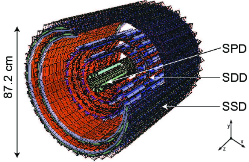
Figure 2.4: Layout of ALICE Inner Tracking System [84].
