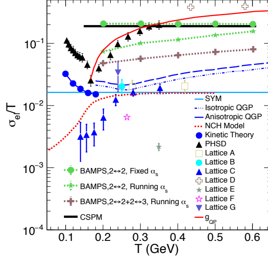
Figure 4.14: (Colour online) \sigma_{el}/T versus T plot [195]. The black solid line is the result obtained in CSM and black triangles are PHSD results [176]. The green and brown dotted lines correspond to various BAMPs results [197]. The NCH model [189] results are shown by the red dotted line. The blue circles are kinetic theory calculations [198]. The horizontal line is the result obtained for conformal supersymmetric (SYM) Yang-Mills Plasma [199]. Lattice data: lattice A- G [180–186, 200] are also shown by various symbols in the figure. The results for isotropic and anisotropic QGP [201] are shown by the blue dash-dotted and dashed lines, respectively. The red solid line depicts the results of quasi-particle (QP) model [188].
