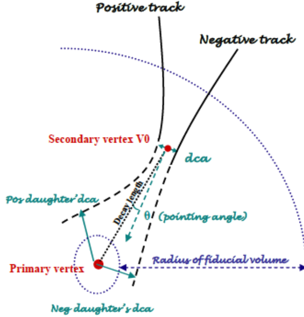
Figure 3.6: Topology of a decaying V^0 particle [111].
