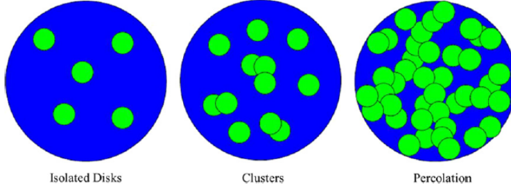
Figure 4.2: Left panel: Disconnected discs, Middle: Cluster formation, Right panel: Overlapping discs forming a cluster of communication [53].
