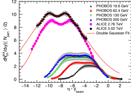
Figure 5.3: The number of participant pair normalized pseudorapidity distribution of charged particles ( dN_{\text{ch}}^{\text{AA}}/d\eta ) in heavy-ion collisions versus \eta - y_{\text{beam}} for various energies [238]. The symbols are experimental data [57, 251–253] and the lines are the double Gaussian fits.
