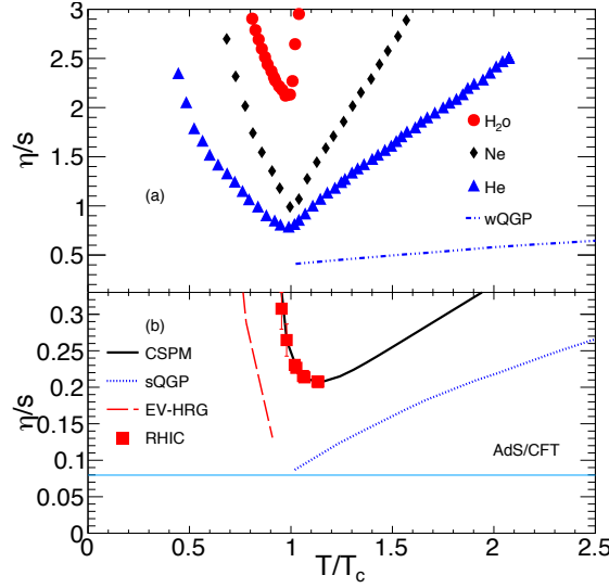
Figure 4.9: (Color online) \eta/s as a function of T/T_c . The red square shows the results from various RHIC energies from the CSPM [144]. The black solid line shows the extrapolation to higher temperatures from CSPM. The solid horizontal line around 1/4\pi represents the AdS/CFT limit [169]. Blue dash-dotted and blue dotted line show the results from wQGP and sQGP, respectively [168]. The red dashed line shows the calculations of EV-HRG [161].
