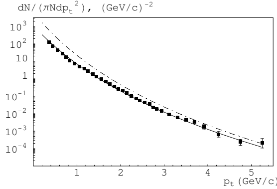
Figure 1.13: Results of color string percolation model predicting transverse momentum. The solid line corresponds to the expected p_T distribution with CSPM for most central (0 - 5%) Au+Au collisions. The filled boxes are the PHENIX experimental data at RHIC. The dotted-dashed line is the expected distribution if color suppression is not accounted for [51].
