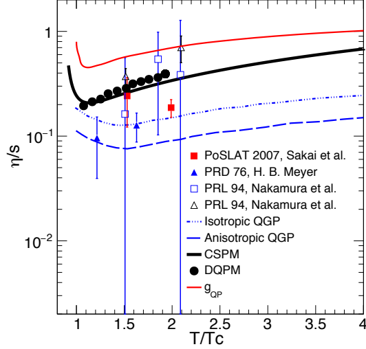
Figure 4.15: (Colour online) The ratio \eta/s as a function of T/T_c [195]. The black solid line is the CSPM result and broken lines are results from Ref. [201]. The symbols are lattice QCD results: full triangles [202], open squares and open triangles [203], full squares [204]. The black circles are the results obtained in DQPM [205]. The red solid line is QP model results [188].
