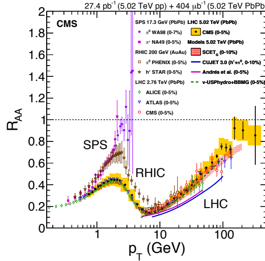
Figure 1.9: R_{AA}(p_T) for neutral pions ( \pi^0 ), charged hadrons ( h^\pm ), and charged particles in central heavy-ion collisions at SPS, RHIC and the LHC [31].
