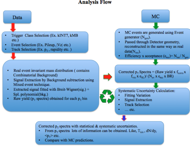
Figure 3.1: Analysis flow chart.
