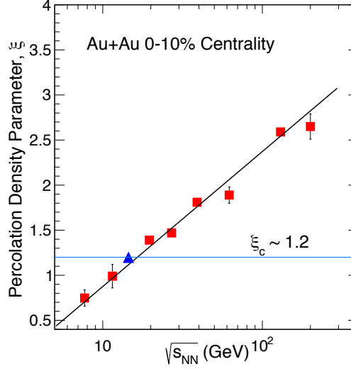
Figure 4.5: (Color online) Percolation density parameter, \xi as a function of \sqrt{s_{NN}} . The red squares show the values for RHIC energies from \sqrt{s_{NN}} = 7.7 - 200 GeV [144]. The blue triangle is the prediction for 14.5 GeV. The horizontal line at \xi \sim 1.2 is the critical value of \xi [141, 142].
