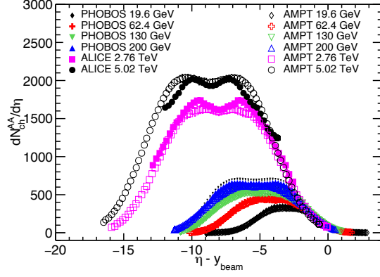
Figure 5.5: The comparison of AMPT model predictions with experimental data on dN_{\text{ch}}^{\text{AA}}/d\eta versus \eta - y_{\text{beam}} for various energies [238].
