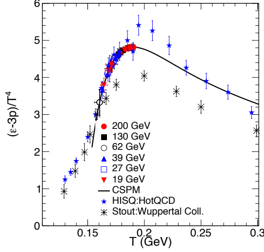
Figure 4.26: (Color online) Variation of trace anomaly \Delta = (\varepsilon - 3P)/T^4 with respect to temperature [207]. Blue star markers represent results from HotQCD collaboration [171]. Black asterisk markers refer to Wuppertal collaboration [172]. Different markers are the results obtained from CSPM for RHIC energies for different centrality bins and the black line represents the extrapolated CSPM results.
