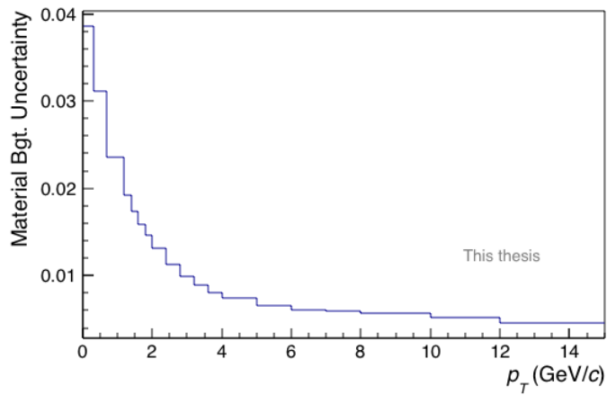
Figure 3.16: Estimated material budget uncertainty for K^{*\pm} as a function of p_T [112].
