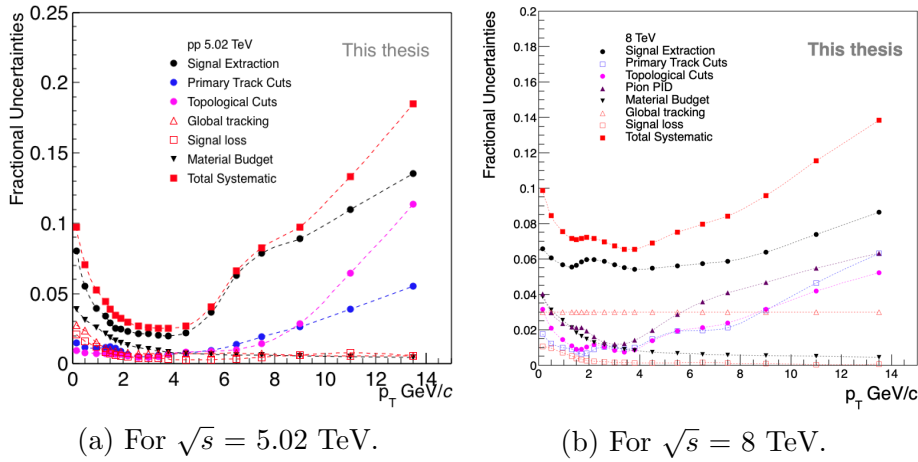
Figure 3.17: Summary of fractional systematic uncertainty at \sqrt{s} = 5.02 and 8 TeV [107, 108].
