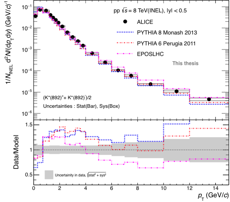
Figure 3.24: Comparison of the measured K^{*\pm} inelastic spectrum shown by black markers in pp collisions at \sqrt{s} = 8 TeV to the distributions predicted by PYTHIA8-Monash 2013 (blue lines), PYTHIA6-Perugia 2011 (red lines), and EPOS LHC (magenta lines). (Bottom panel). The ratio of the rebinning predictions to the measured distribution for K^{*\pm} mesons. The shaded band shows the fractional uncertainty of the measured data points [108].
