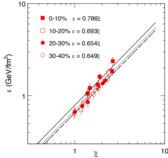
Figure 4.23: (Color online) Initial energy density, \varepsilon as a function of the percolation density parameter ( \xi ) for different centrality classes at RHIC energies from 19.6 to 200 GeV [207]. The different lines are the linear fits to data for different centralities.
