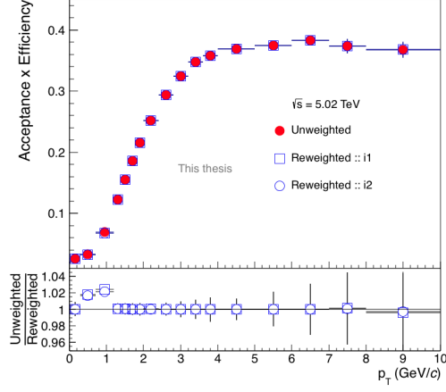
(a) Efficiency comparison at \sqrt{s} = 5.02 TeV.
