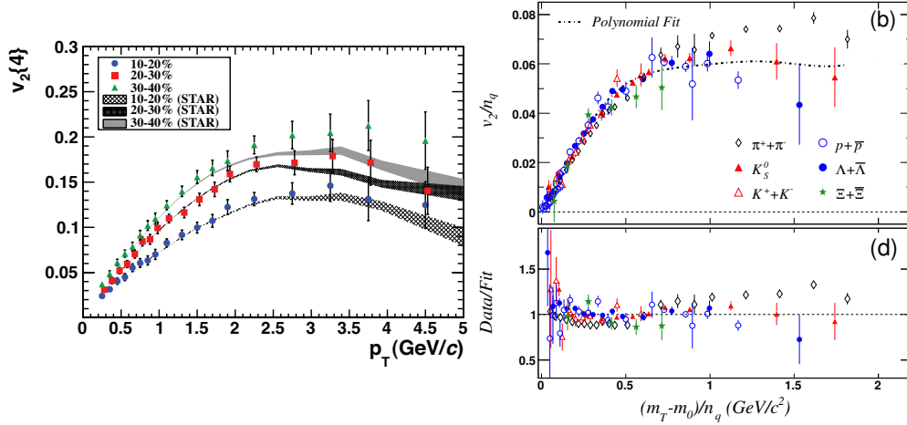
Figure 1.10: Left: The differential elliptic flow of charged particles. The Pb + Pb collisions at \sqrt{s_{NN}} = 2.76 TeV shown in coloured symbols are compared to Au+Au collisions at \sqrt{s_{NN}} = 200 GeV, which are in shaded regions [31]. Right: v_2/n_q versus (m_T - m_0)/n_q of identified hadrons in Au+Au collisions at \sqrt{s_{NN}} = 62.4 GeV [34].
