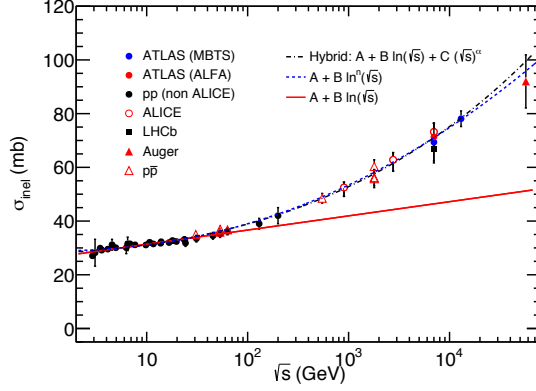
Figure 5.2: The inelastic cross-section as a function of \sqrt{s} [238]. The symbols are experimental data [57, 243–245] and the fitted lines are phenomenologically motivated functions.
