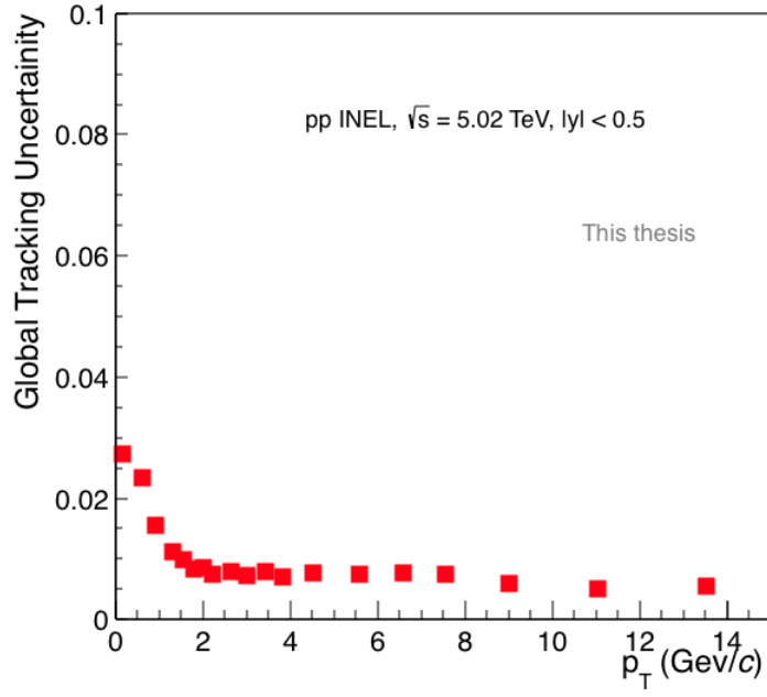
Figure 3.15: Global tracking uncertainty for \sqrt{s} = 5.02 TeV as a function of p_T [107].
