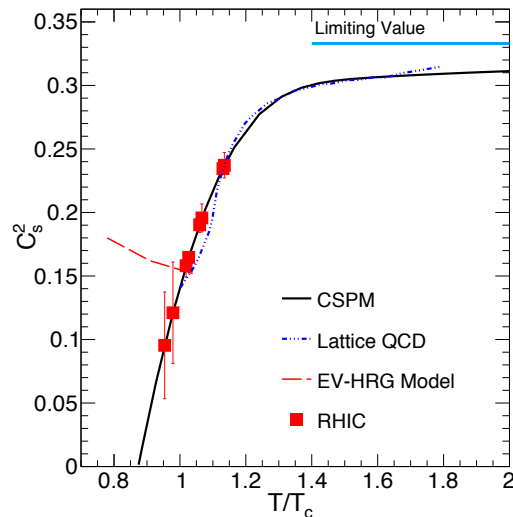
Figure 4.11: (Color online) The squared speed of sound ( C_s^2 ) as a function of T/T_c [144]. The red squares are the CSPM results at RHIC energies. The black line is the extrapolated CSPM result. Blue dash-dotted line represents lQCD results [145]. The red dashed line shows the result from EV-HRG [161].
