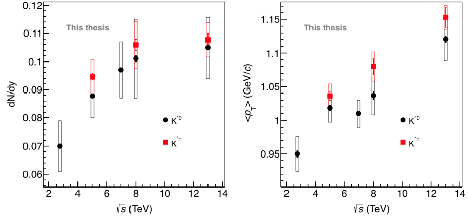
Figure 3.19: (left panel) K^{*\pm} (red symbol) and K^{*0} (black symbol) yield is shown. (right panel) Mean transverse momentum as a function of pp collision energy is shown. K^{*0} results are taken from Ref. [113]. Statistical and systematic uncertainties are shown by error bars and empty boxes, respectively.
