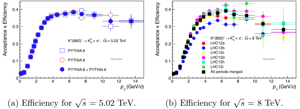
Figure 3.11: The efficiency in pp collisions at \sqrt{s} = 5.02 and 8 TeV as a function of p_T [107, 108]. Details of the plots are described in the text.
