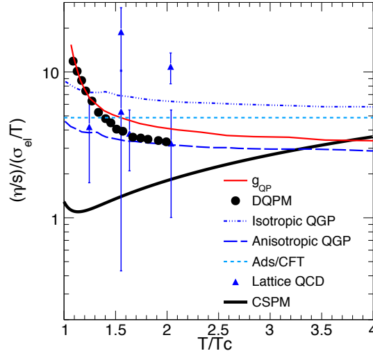
Figure 4.16: (Colour online) The ratio \eta/s and \sigma_{el}/T as a function of T/T_c [195]. The black solid line is the CSPM result and broken lines are results from Ref. [201]. The symbols are lattice QCD results [188]. The DQPM and QP results are shown by the black circles and red solid line, respectively [188].
