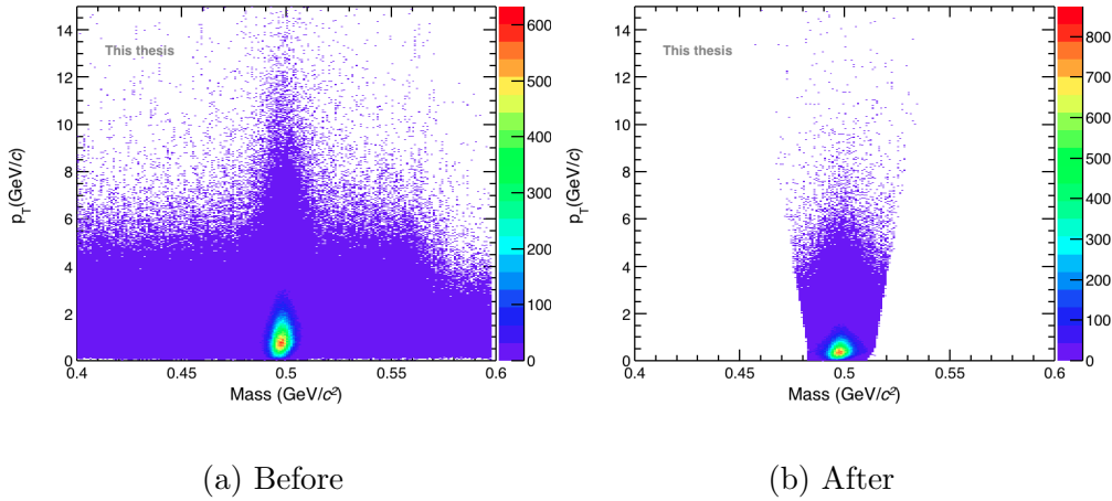
Figure 3.8: Plots showing the effect of p_T -dependent mass tolerance cut on K_S^0 selection [107].
