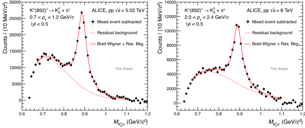
(a) For the bin 0.7 < p_T < 1.2 \text{ GeV}/c at \sqrt{s} = 5.02 \text{ TeV} . (b) For the bin 2.0 < p_T < 2.4 \text{ GeV}/c at \sqrt{s} = 8 \text{ TeV} .
