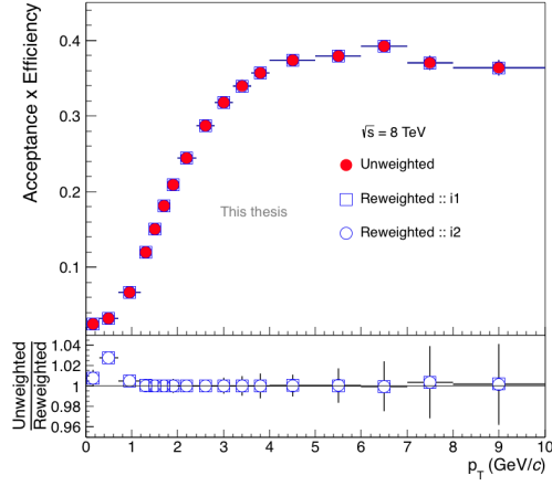
(b) Efficiency comparison at \sqrt{s} = 8 TeV.
