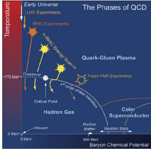
Figure 1.4: Sketch of QCD phase diagram with boundaries that define various states of QCD matter [14].
