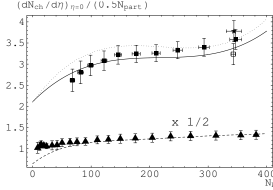
Figure 1.12: Results of color string percolation model predicting multiplicity. The number of participants are from the SPS WA98 data (filled triangles), the RHIC PHENIX (filled square), PHOBOS (open square) data at \sqrt{s_{NN}} = 130 GeV, and with RHIC PHENIX data at \sqrt{s_{NN}} = 200 GeV (filled stars). The dashed, solid, and dotted lines are predictions for the relevant energies [51].
