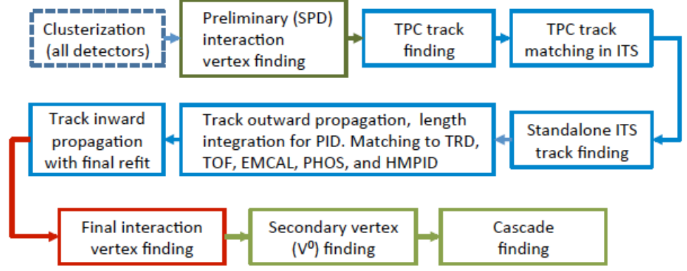
Figure 3.4: Event reconstruction flow [109].
