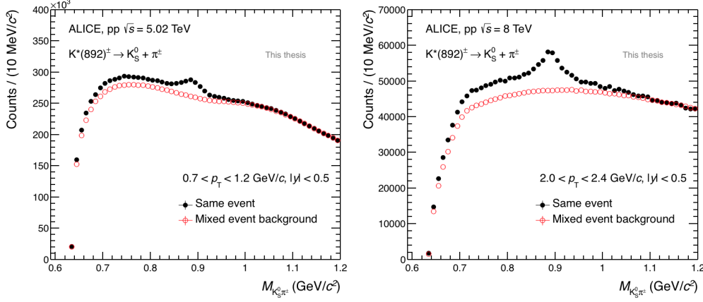
(a) For the bin 0.7 < p_T < 1.2 GeV/c at \sqrt{s} = 5.02 TeV. (b) For the bin 2.0 < p_T < 2.4 GeV/c at \sqrt{s} = 8 TeV.
