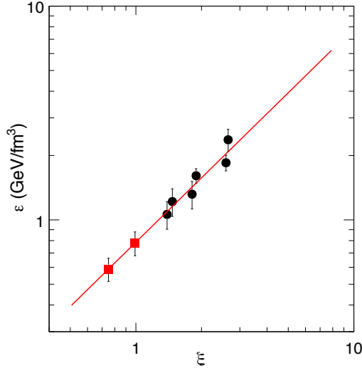
Figure 4.7: (Color online) Initial energy Density \varepsilon as a function of the percolation density parameter, \xi [144]. The black circles show the values for RHIC energies from \sqrt{s_{NN}} = 19.6 - 200 GeV. The red squares are the interpolated \xi values for 7.7 and 11.5 GeV.
