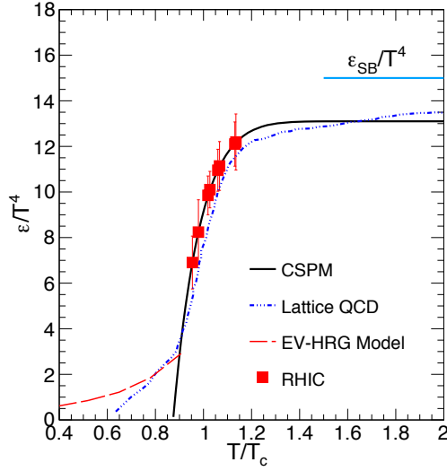
Figure 4.8: (Color online) Scaled energy density ( \varepsilon/T^4 ) as a function of T/T_c [144]. The black solid line is CSPM results and the blue dash-dotted line corresponds to the lattice QCD results [145]. The red dashed line shows the result from EV-HRG model [161].
