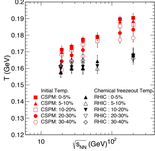
Figure 4.24: (Color online) Initial temperature, T estimated by using CSPM at RHIC energies (red symbols) and extracted chemical freeze-out temperatures for Grand Canonical Ensemble using the experimental data at RHIC energies [158] (black symbols) for different centrality classes [207].
