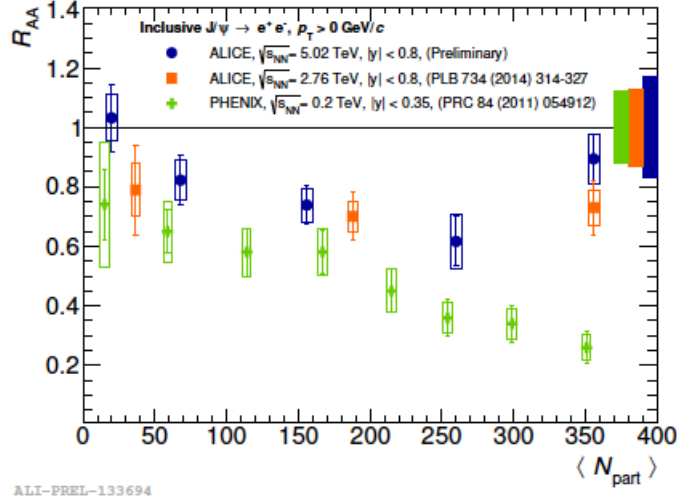
Figure 1.7: The R_{AA} of J/\psi as function of centrality in Pb–Pb collisions at \sqrt{s_{NN}} = 2.76 TeV and 5.02 TeV at ALICE and the measurement is compared with the PHENIX result of Au+Au collisions at \sqrt{s_{NN}} = 0.2 TeV.
