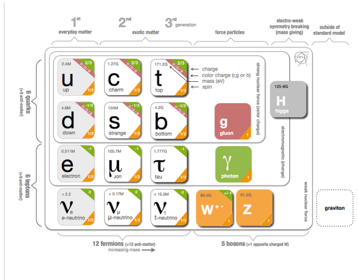
Figure 1.1: The Standard model of particle physics (Image Credit: CERN).
