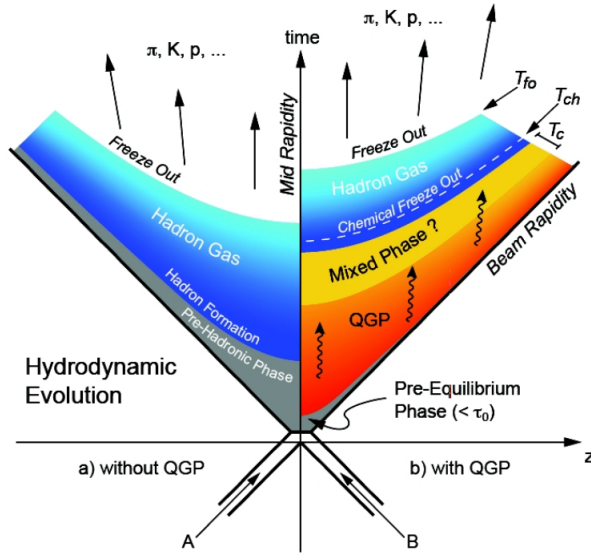
Figure 1.6: A schematic diagram of the longitudinal space-time evolution of relativistic nucleus-nucleus collision [15].
