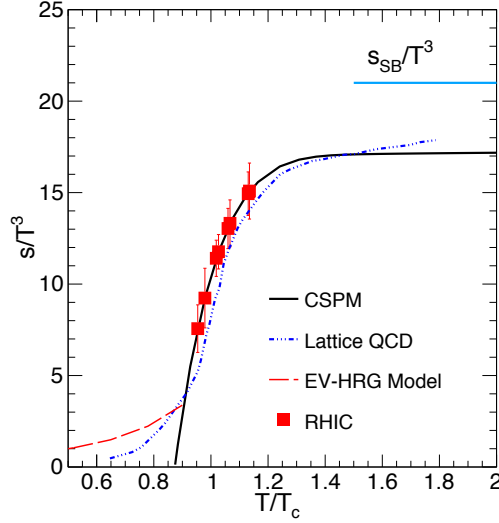
Figure 4.12: (Color online) Entropy density ( s/T^3 ) as a function of T/T_c [144]. The red squares are the results from CSPM for RHIC energies. Blue dash-dotted line represents the lQCD results [145]. The red dashed line shows the result calculated using EV-HRG model [161].
