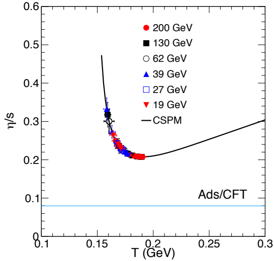
Figure 4.25: (Color online) \eta/s as a function of temperature. The markers show the results from various RHIC energies for different centrality bins from the CSPM [207]. The black solid line shows the extrapolation to higher temperatures from CSPM. The solid horizontal line around 1/4\pi represents the AdS/CFT limit [169].
