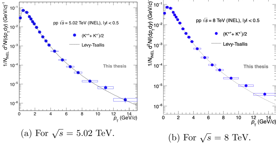
Figure 3.18: Inelastic K^{*\pm} spectrum with Lévy-Tsallis fit (black dotted curve), statistical (bars) and systematics (boxes) uncertainties at \sqrt{s} = 5.02 and 8 TeV [107, 108].
