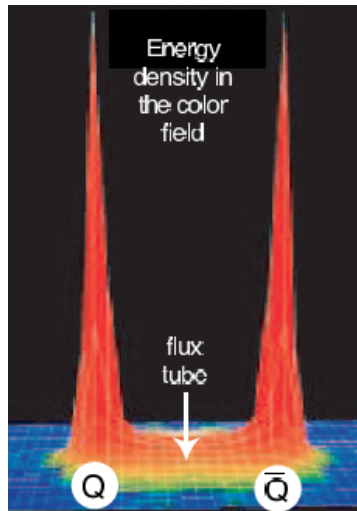
Figure 4.3: Color flux tube between projectile and target [140].
