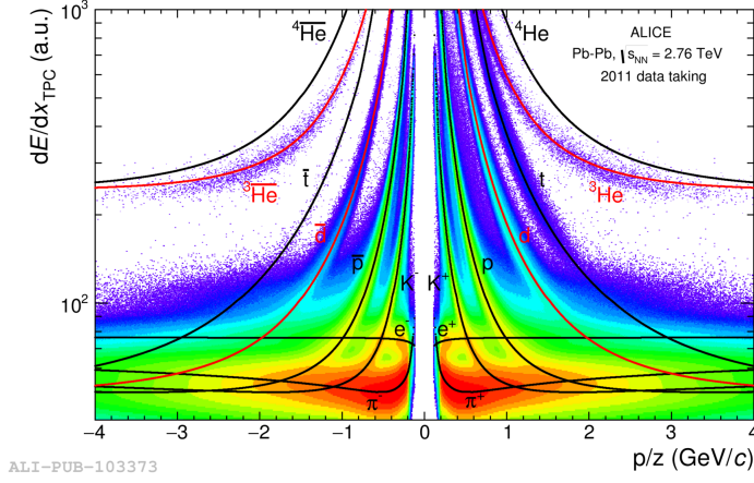
Figure 2.6: Specific energy loss ( dE/dx ) of the tracks as a function of rigidity ( p/z ) for different particles and anti-particles in Pb-Pb collisions at \sqrt{s_{NN}} = 2.76 TeV. The solid line represents the theoretical Bethe-Bloch dE/dx expectations.
