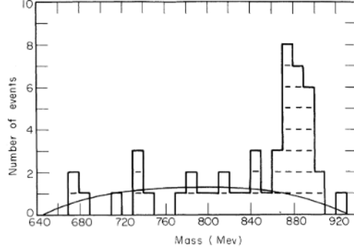
Figure 3.2: The invariant mass spectrum of K^{*-} \rightarrow K_S^0 + \pi^- from K^- + p collision. The solid line represents the phase-space curve normalized to background events [104].
