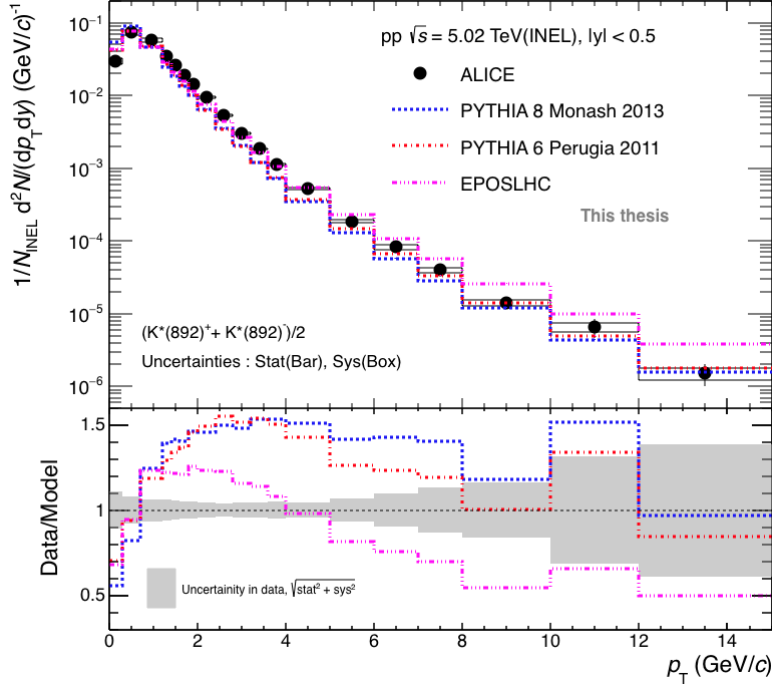
Figure 3.23: Comparison of the measured K^{*\pm} inelastic spectrum shown by black markers in pp collisions at \sqrt{s} = 5.02 TeV to the distributions predicted by PYTHIA8-Monash 2013 (blue lines), PYTHIA6-Perugia 2011 (red lines), and EPOS LHC (magenta lines). (Bottom panel) The ratio of the rebinned predictions to the measured distribution for K^{*\pm} mesons. The shaded band shows the fractional uncertainty of the measured data points [107].
