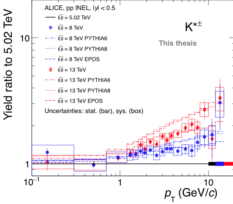
Figure 3.22: Ratios of transverse momentum spectra of K^{*\pm} at \sqrt{s} = 8 and 13 TeV to 5.02 TeV. Statistical and systematic uncertainties are shown by error bars and empty boxes, respectively. The normalization uncertainties are shown as colored boxes around 1. Blue and red histograms represent the prediction of the same ratios from PYTHIA6 - Perugia 2011, PYTHIA8 - Monash 2013 and EPOS LHC [113].
