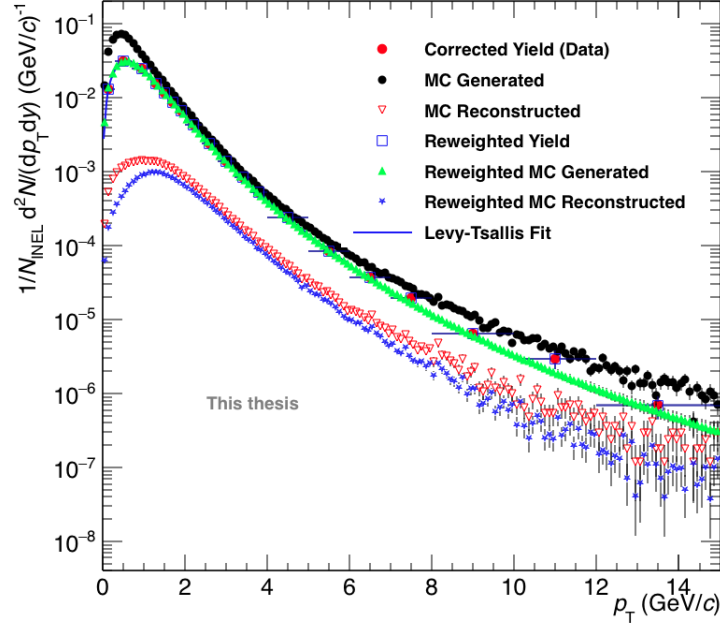
Figure 3.12: Corrected K^{*\pm} spectrum (red circles) with Lévy-Tsallis fit (blue curve). The unweighted generated (black circles) distribution is compared to the reweighted distribution (Green solid triangle). The unweighted reconstructed (inverted triangle) distribution and the reweighted distribution (blue star) are also shown [107].
