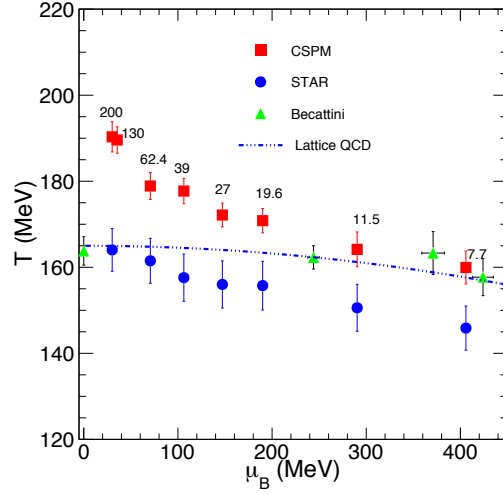
Figure 4.6: (Color online) The temperature and baryon chemical potential ( \mu_B ) estimated in different calculations at various center-of-mass energies [144]. The red squares are the initial temperatures at RHIC energies estimated in CSPM. The blue dash-dotted line is the prediction from lQCD [153]. The green triangles are for hadronization temperature and baryon chemical potential as obtained in the statistical model [154]. The blue circles are (T, \mu_B) at freeze-out estimated by STAR experiment [155].
