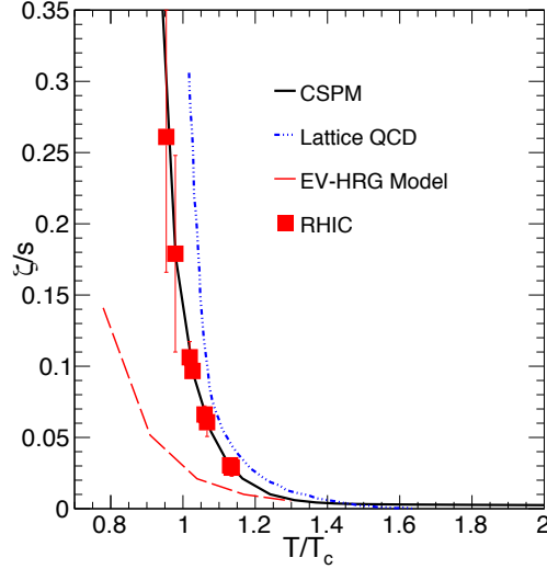
Figure 4.13: (Color online) The ratio of bulk viscosity and entropy density ( \zeta/s ) as a function of T/T_c is shown by red squares from CSPM [144] and the black solid line shows the extrapolated CSPM results. The blue dash-dotted line corresponds to results from lQCD [175]. The red dashed line is the result of EV-HRG model [161].
