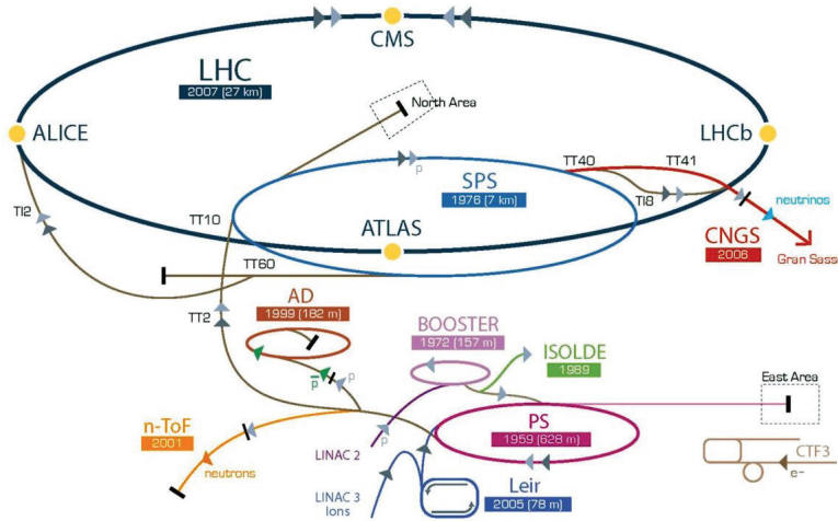
Figure 2.1: CERN accelerator complex showing the PS (Proton Synchrotron), SPS (Super Proton Synchrotron) rings and the four main LHC experiments (ALICE, ATLAS, CMS and LHCb) around the LHC ring [63].
