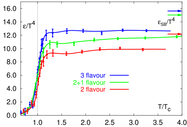
Figure 1.3: lQCD predictions of \varepsilon/T^4 as a function of temperature normalized by the critical temperature ( T_C ). The horizontal arrows show the Stefan-Boltzmann limit [10].
