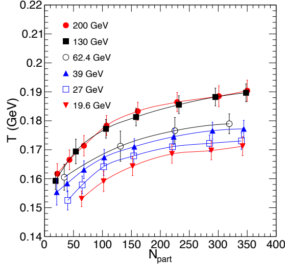
Figure 4.20: (Color online) The initial temperatures at RHIC energies estimated in CSPM as a function of number of participants ( N_{\text{part}} ) for Au+Au collisions [207].
