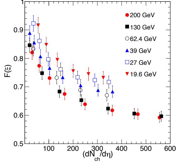
Figure 4.18: (Color online) Color Suppression factor F(\xi) , as a function of charged particle pseudorapidity density, dN_{\text{ch}}/d\eta [207]. Different symbols represent different centre-of-mass energies.
