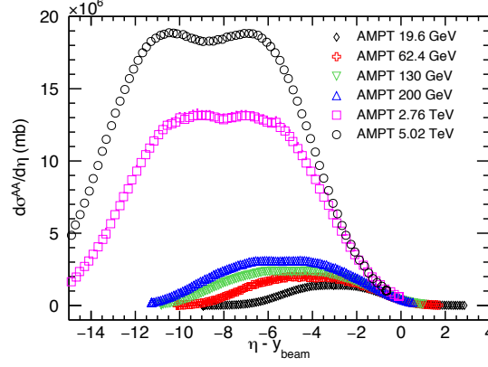
Figure 5.6: d\sigma^{\text{AA}}/d\eta versus \eta - y_{\text{beam}} using AMPT results [238].
