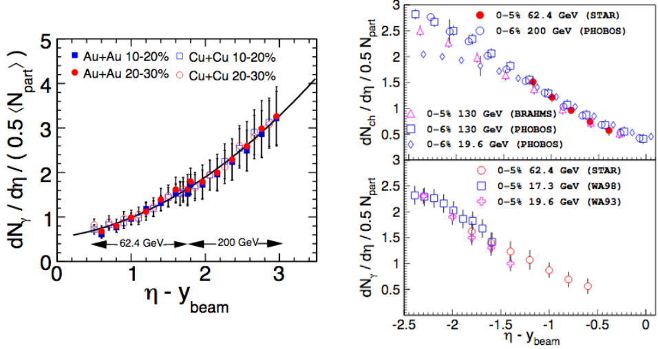
Figure 1.14: Left: Photon pseudorapidity distributions normalized by the average number of participating nucleon pairs for different collision centralities are plotted as a function of pseudorapidity shifted by the y_{beam} for Au+Au and Cu+Cu collisions at \sqrt{s_{NN}} = 62.4 and 200 GeV [58]. Right: Variations of dN_{ch}/d\eta (top panel) and for dN_\gamma/d\eta (bottom panel) normalized to N_{part} with \eta - y_{beam} for different energies central collisions [59].
