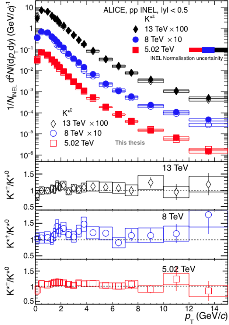
Figure 3.21: Inelastic K^{*\pm} spectrum in solid symbols and K^{*0} spectrum in open symbols for pp collisions at \sqrt{s} = 5.02, 8 and 13 TeV. Statistical and systematic uncertainties are shown by error bars and empty boxes, respectively. The normalization uncertainties are shown as colored boxes and they are not included in the point-to-point uncertainty. In the bottom panels the ratios of the measured p_T -spectra for K^{*\pm} to K^{*0} at \sqrt{s} = 5.02 (red open square), 8 (blue open circle) and 13 (black open diamond) TeV are shown [113].
