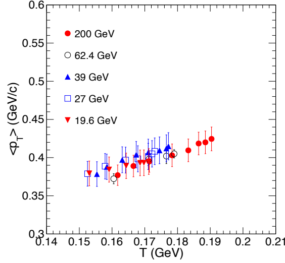
Figure 4.22: (Color online) Average momentum \langle p_T \rangle of pions as a function of initial temperature, T . \langle p_T \rangle are obtained from experimental data [157] and initial temperatures are estimated by using CSPM [207]. Different symbols are for different centre-of-mass energies.
