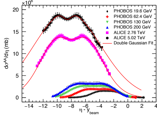
Figure 5.4: The differential cross-section per unit pseudorapidity ( d\sigma^{\text{AA}}/d\eta ) as a function of \eta - y_{\text{beam}} for various collision energies [238]. The symbols are experimental points and the lines are double Gaussian fits.
