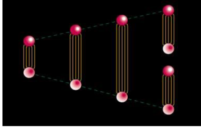
Figure 4.4: Production of new hadrons from color strings [140].
