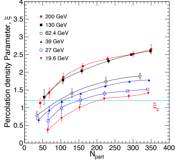
Figure 4.17: (Color online) Percolation density parameter \xi , as a function of number of participants ( N_{\text{part}} ) for Au+Au collisions at RHIC energies from 19.6 - 200 GeV [207]. The symbols correspond to different centre-of-mass energies and the horizontal line is the critical percolation density.
