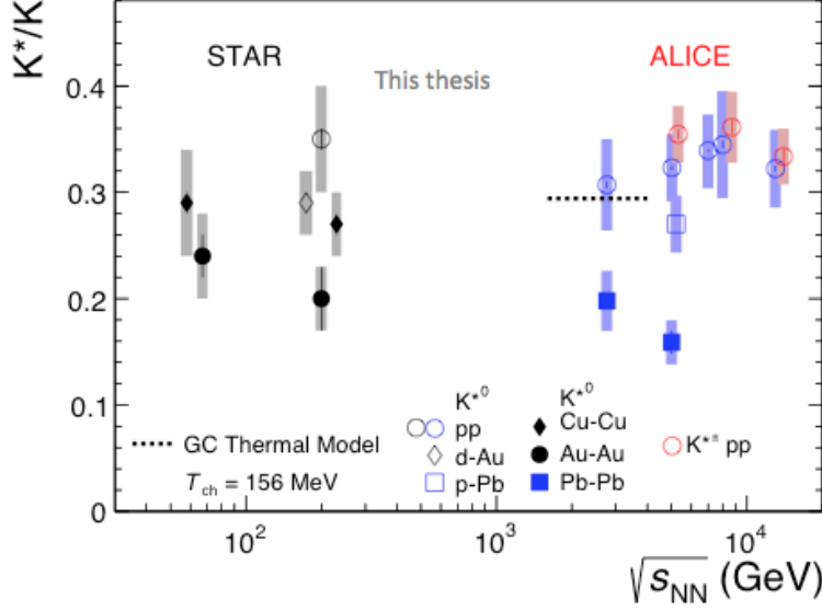
Figure 3.20: Ratios of K^{*\pm}/K and K^{*0}/K in pp, central d–Au and central A+A collisions as a function of \sqrt{s_{NN}} [113]. Error bars represent the statistical uncertainties and boxes represent the systematic uncertainties.
