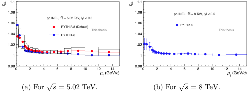
Figure 3.14: Signal-loss correction in pp collisions at \sqrt{s} = 5.02 and 8 TeV [107, 108].
