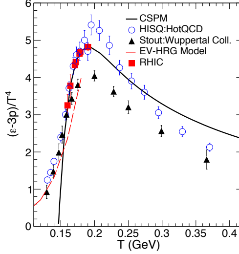
Figure 4.10: (Color online) Variation of trace anomaly \Delta = (\varepsilon - 3P)/T^4 with respect to temperature [144]. Blue circles represent results from HotQCD collaboration [171]. Black triangle refer to Wuppertal collaboration [172]. The red dashed line shows the result from EV-HRG model [161]. The red squares are the results obtained from CSPM for RHIC energies and black line is the extrapolated CSPM results.
