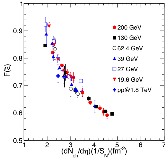
Figure 4.19: (Color online) Color Suppression factor F(\xi) , as a function of pseudorapidity density divided by the nuclear overlap function, (dN_{\text{ch}}/d\eta)/S_N [207]. Different symbols represent different centre-of-mass energies along with high-multiplicity non-jet p\bar{p} collisions at \sqrt{s}=1.8 TeV at Tevatron [146].
