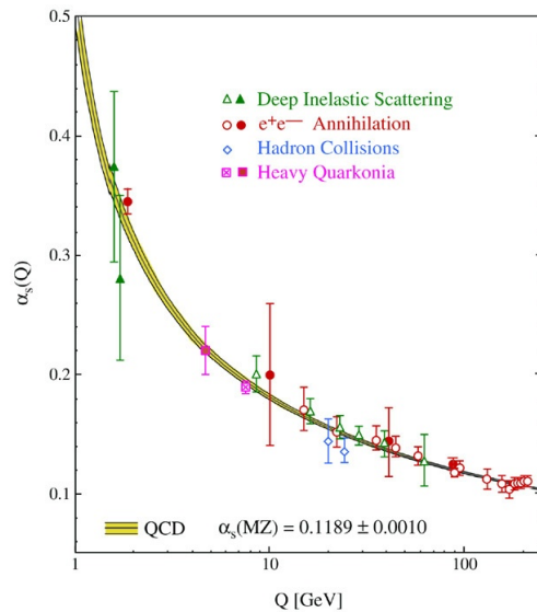
Figure 1.2: QCD running coupling constant ( \alpha_S ) as a function of momentum transfer ( Q ) [7].
