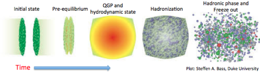
Figure 1.5: A schematic picture of the time evolution of heavy-ion collision. (Image credit: Prof. Steffen A. Bass)
