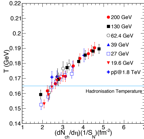
Figure 4.21: (Color online) Temperature as a function of (dN_{\text{ch}}/d\eta)/S_N from pp and Au + Au collisions [207]. The horizontal line corresponds to T \sim 165 MeV, which is the universal hadronisation temperature [152].
