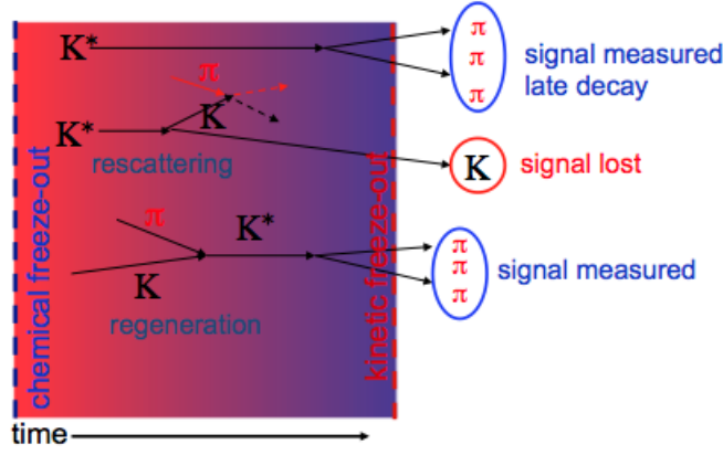
Figure 1.11: Schematic diagram showing chemical and kinetic freeze-out with possible pion and kaon interactions in the hadronic medium.
