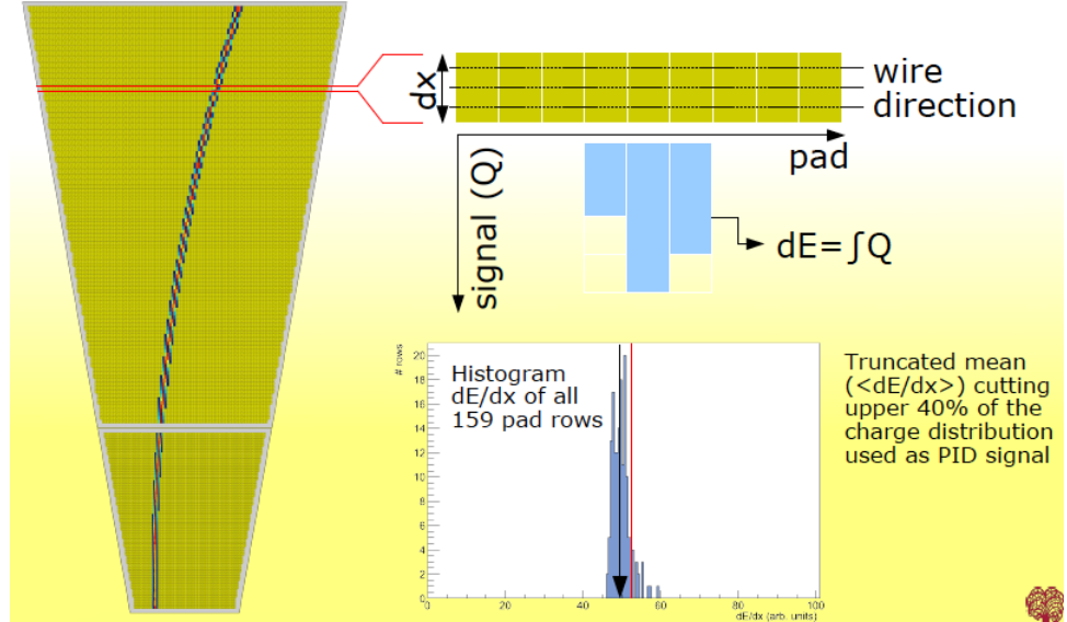
Figure 2.7: Schematic diagram of \langle dE/dx \rangle measurements in TPC [88].
