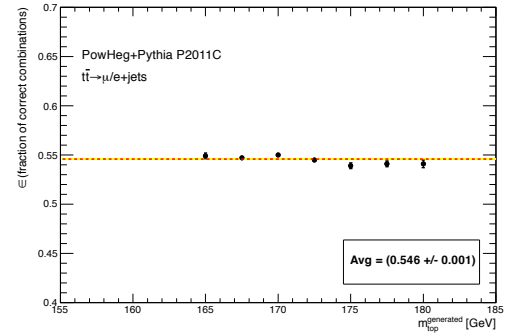
(f) \epsilon (correct combinations fraction) dependence.
