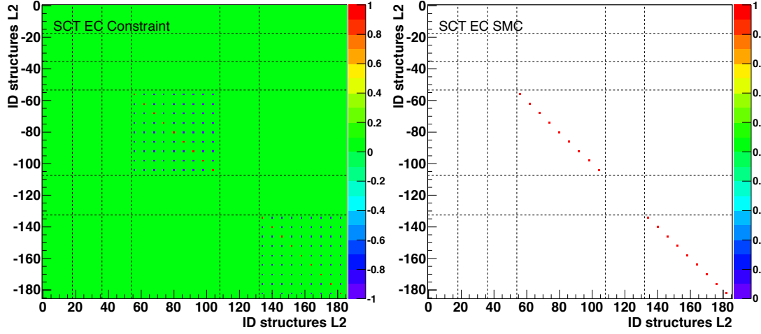
Figure 4.13: The impact of the alignment parameter constraint to the alignment correction enter into the formalism as an extra contribution to the usual big matrix. Left: Survey matrix for the SCT end-cap with a correlated T_Z disc position constraint. Right: SMC matrix for the T_Z DoF of the SCT end-cap discs.
