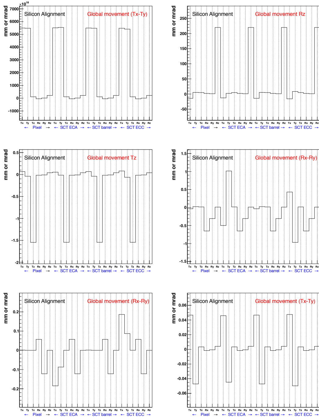
Figure 4.6: First six (1/\text{eigenvalues}) \times \text{eigenvectors} for the silicon tracking detector aligned at L1. The 24 DoFs associated to the four structures at L1 can be seen in the x axis.
