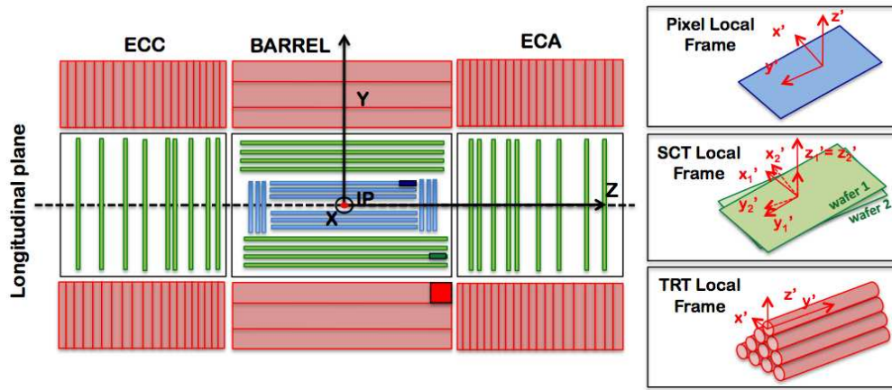
Figure 3.1: Left: Schematic longitudinal view of the ID detector geometry: Pixels (blue), SCT (green) and TRT (red). In this view the Global frame is represented by the black arrows. The dark boxes correspond to the position of the arbitrary selected detector modules. Right: Local frame for each detector module: Pixel (up), SCT (middle) and TRT (bottom).
