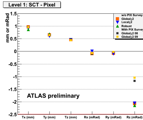
Figure 4.19: Difference between the Pixel and SCT barrel position for each alignment parameter. The results for the Global \chi^2 , Local \chi^2 and Robust methods are shown. Also the Global \chi^2 results obtained with different cosmic data sets are displayed. Notice that the difference in the R_Z corrections are due to the use of the Pixel detector survey.
