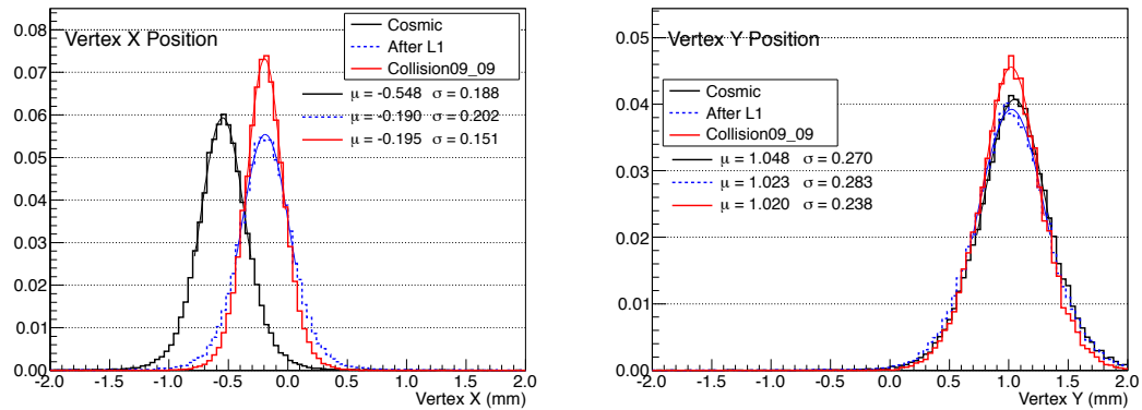
Figure 4.29: X (left) and Y (right) beam spot coordinate position before (black line) and after (red line) alignment. The L1 (blue line) alignment has been also drawn to see its corresponding impact.
