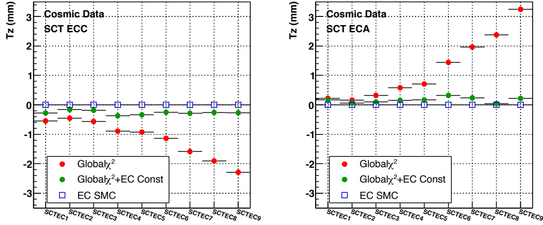
Figure 4.14: T_z end-cap corrections obtained at L2 with cosmic data for the ECA (right) and ECC (left). Three scenarios are shown: normal alignment algorithm mode where the discs in the SCT end-caps are free (red points), alignment algorithm with a end-cap constraint of 10\ \mu\text{m} (green points) and silicon alignment corrections obtained using a SMC of 1 nm for all SCT discs (blue open squares).
