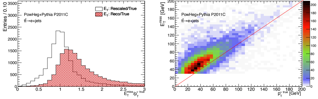
Figure K.2: Evaluation of the raw E_T^{\text{miss}} for those events with initially complex solution for p_z^\nu . Left: comparison of the raw reconstructed E_T^{\text{miss}}/p_T^{\nu \text{ true}} (red histogram) with the rescaled one (white histogram). Right: scatter plot of the raw reconstructed E_T^{\text{miss}} vs. p_T^{\nu \text{ true}} . Both plots show how the raw reconstructed E_T^{\text{miss}} is over estimated ( E_T^{\text{miss}}/p_T^{\nu \text{ true}} above 1 in the left plot, and above the diagonal in the right plot).
