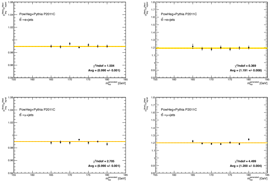
Figure J.2: Left: ratio between the mean of the combinatorial background and the mean of the correct combinations ( \mu_{\text{bkg}}^{\text{fitted}}/\mu_{\text{signal}}^{\text{fitted}} ). Right: ratio between the sigma of the combinatorial background and the sigma of the correct combinations ( \sigma_{\text{bkg}}^{\text{fitted}}/\sigma_{\text{signal}}^{\text{fitted}} ). The results are shown for the e + \text{jets} (upper row) and \mu + \text{jets} (bottom row) channels.
