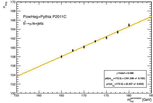
(c) \mu_{bkg} (background mean) fit parameter dependence.
