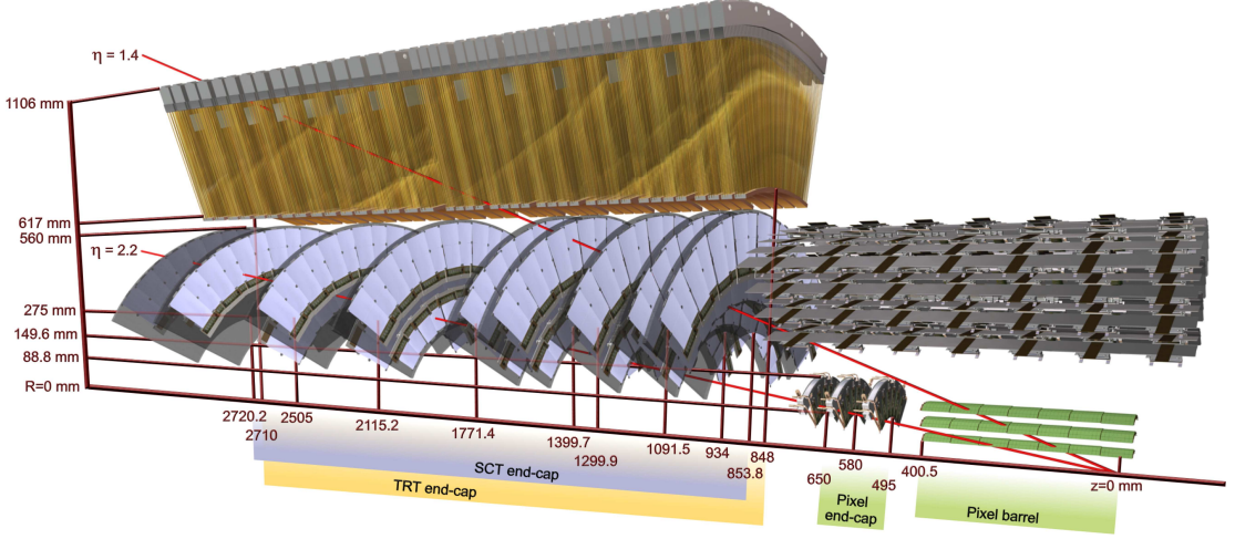
Figure 4.10: An illustration of the structural elements and sensors of the ID end-cap: the beryllium beam-pipe, the three Pixel discs, the nine SCT discs and the forty planes of the TRT wheels. The Pixel and SCT barrel layers are also partially displayed.
