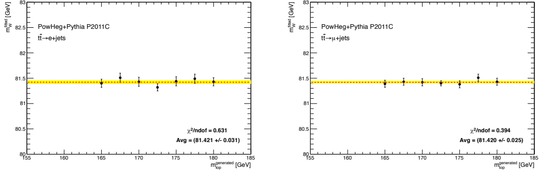
Figure 5.11: Invariant mass of the W jet pair candidate ( m_W^{\text{fitted}} ) versus m_{\text{top}}^{\text{generated}} for the e +jets (left) and \mu +jets (right) channels.
