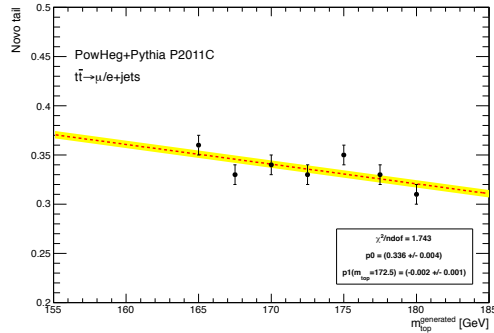
(e) \Lambda_{bkg} (background tail) fit parameter dependence.
