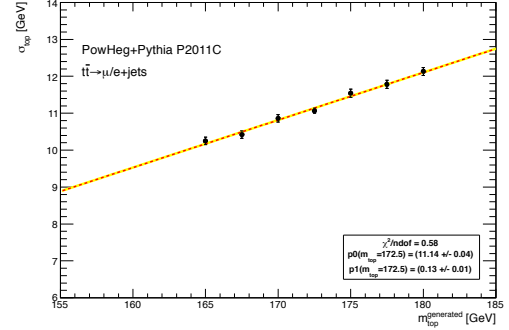
(b) \sigma (resolution) fit parameter dependence.
