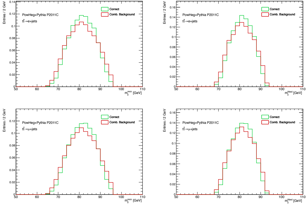
Figure I.2: MC study of the invariant mass of the jets associated to the hadronically decaying W in the t\bar{t} \rightarrow e + \text{jets} channel (upper row) and t\bar{t} \rightarrow \mu + \text{jets} channel (bottom row). Left: with the reconstructed jets before the in-situ calibration. Right: with the jets after the in-situ calibration.
