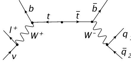
Figure 5.3: Feynman diagram at tree level of the t\bar{t} \rightarrow \ell + \text{jets} decay mode.
