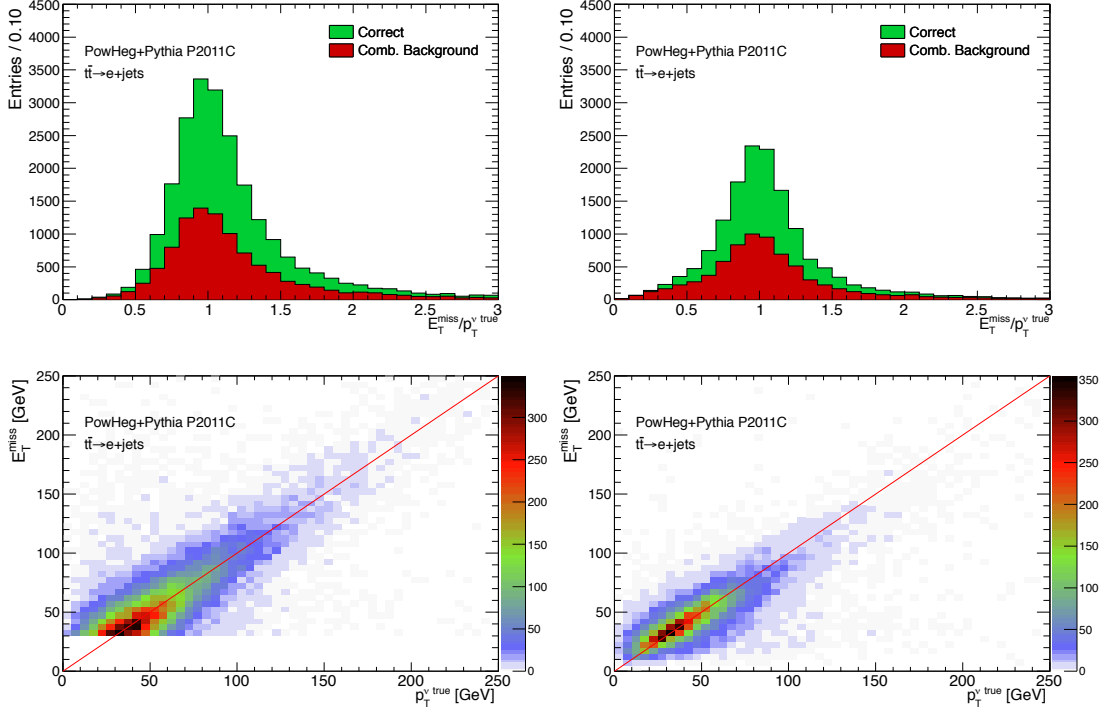
Figure 5.13: E_T^{\text{miss}} related distributions in the MC \bar{t}t \rightarrow e + \text{jets} events. Upper row: reconstructed E_T^{\text{miss}}/p_T^{\nu, \text{true}} for those cases where a valid p_z^{\nu} is found (left) and for those cases where E_T^{\text{miss}} was rescaled to obtain at least one p_z^{\nu} solution (right). Bottom row: correlation plot between E_T^{\text{miss}} and p_T^{\nu, \text{true}} for the same cases as above.
