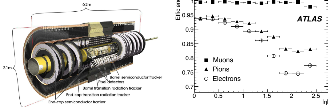
Figure 2.3: Left: Picture of the Inner Detector layout. Right: Track reconstruction efficiencies as a function of |\eta| for muons, pions and electrons with p_T = 5 \text{ GeV} . The inefficiencies for pions and electrons reflect the shape of the amount of material in the inner detector as a function of |\eta| [54].
