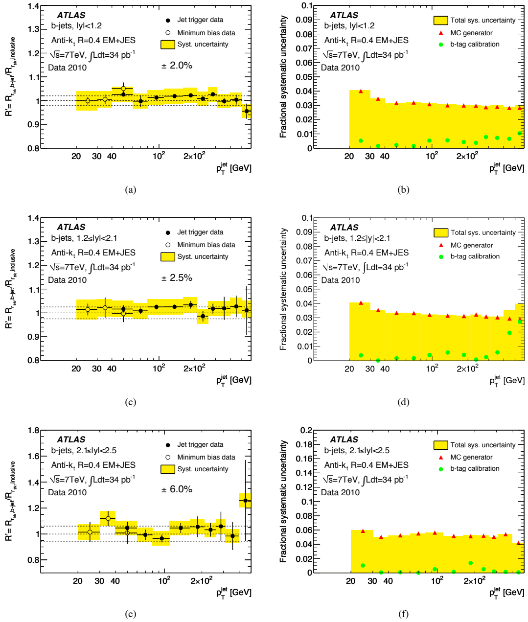
Figure P.2: The ratio R' (left) and the fractional systematic uncertainty (right) as a function of p_T^{jet} for |y| < 1.2 (upper), 1.2 \leq |y| < 2.1 (middle) and 2.1 \leq |y| < 2.5 (bottom). The dashed lines indicate the estimated uncertainty from the data and MC agreement. Only statistical uncertainties are shown on the data points.
