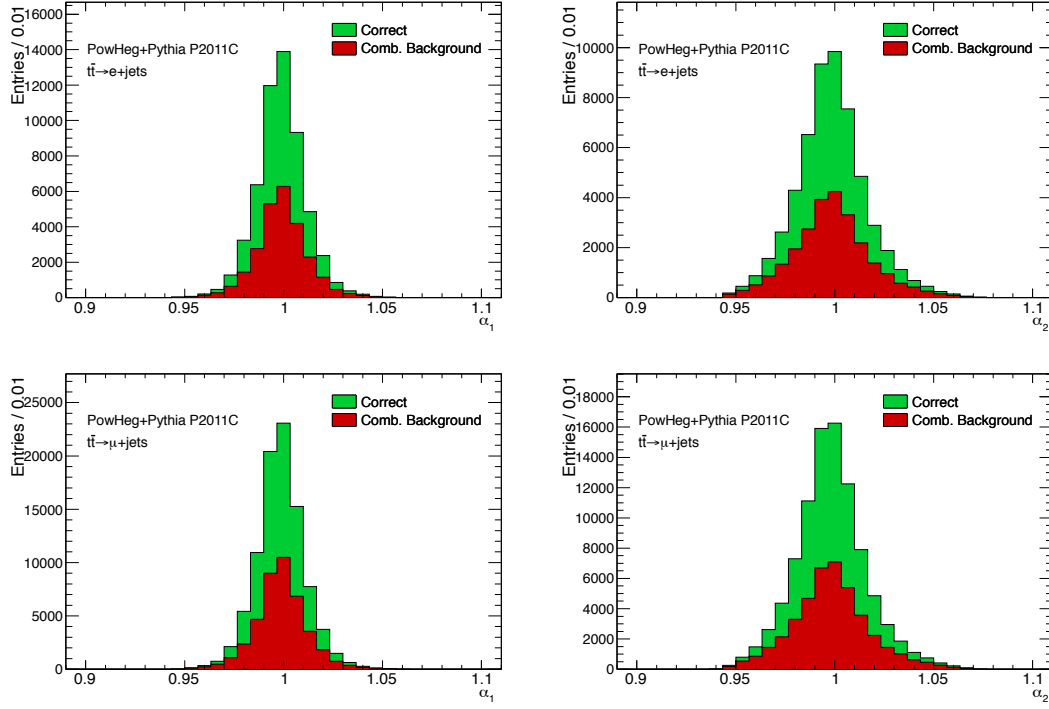
Figure 5.8: MC correction factors \alpha_1 (left) and \alpha_2 (right) obtained from the in-situ calibration fit of the hadronically decaying W for the e + \text{jets} channel (upper row) and \mu + \text{jets} channel (bottom row).
