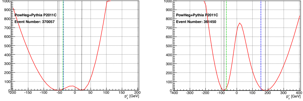
Figure K.1: Quadratic difference between the computed M_W and M_W^{PDG} ( (M_W(p_z^\nu) - M_W^{PDG})^2 ) as a function of the p_z^\nu . Left: Event with good p_z^\nu selection since the final solution (green line) agrees with the truth value (blue line). Right: Event with wrong p_z^\nu selection.
