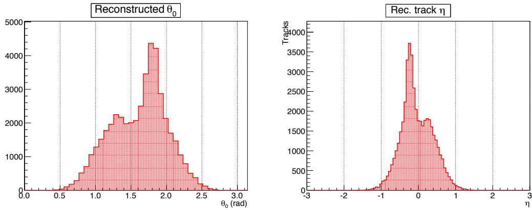
Figure E.4: Left: reconstructed \theta distribution. Right: reconstructed \eta distribution.
