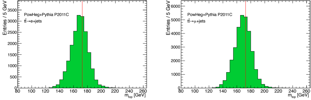
Figure 5.20: Distribution of the fitted m_{\text{top}} as it comes from the Global \chi^2 fit using \bar{t}t \rightarrow e + \text{jets} (left) and \bar{t}t \rightarrow \mu + \text{jets} (right) MC samples and only for the correct combinations. The red line highlights the nominal m_{\text{top}} value (172.5 GeV).
