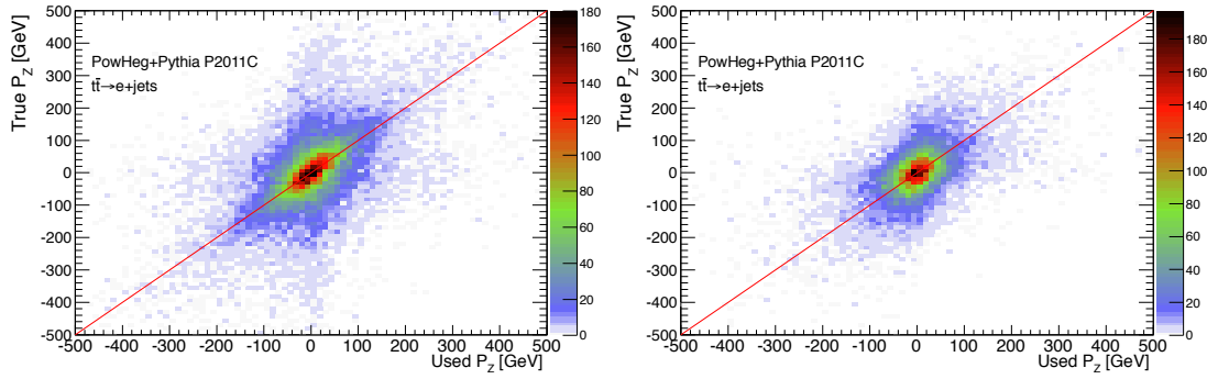
Figure 5.14: MC study of the p_z^\nu in the e+\text{jets} channel. Correlation found between the computed p_z^\nu and the true value. Left: For those cases with 2 p_z^\nu solutions. Right: For those cases where E_T^{\text{miss}} was rescaled to find at least one p_z^\nu solution.
