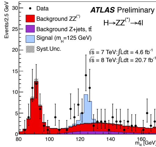
Figure 4.46: The distributions of the four-lepton invariant mass ( m_{4\ell} ) for the selected candidates compared to the background expectation for the combined \sqrt{s} = 8 \text{ TeV} and \sqrt{s} = 7 \text{ TeV} data sets in the mass range of 80-170 GeV. The signal expectation for the m_H=125 \text{ GeV} hypothesis is also shown.
