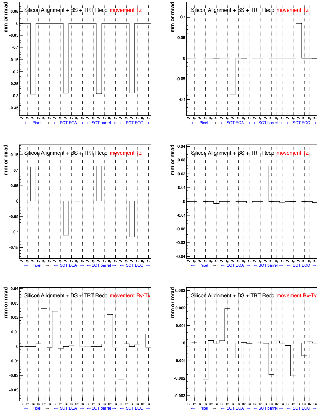
Figure 4.8: First six (1/eigenvalues) \times eigenvectors for the silicon detector aligned at L1 using the BS constraint and the TRT in the reconstruction. The 24 DoFs associated to the structures at L1 can be seen in the x axis.
