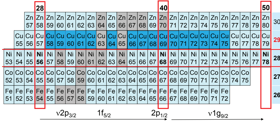
Figure 2.1: The region of the nuclear chart around the semi-magic nickel isotope chain. The number of protons is indicated on the right, the magic numbers are indicated with red lines. Below, the shell model orbits which are filled by neutrons are given. The isotopes with a gray color are stable, the copper nuclei in blue are measured, analyzed and discussed in this work.
