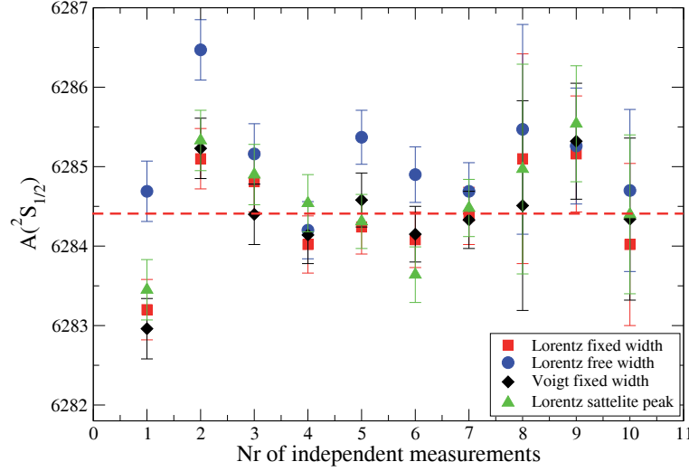
Figure 5.3: A test of different fitting routines on the A(^2S_{1/2}) factor of ^{65}\text{Cu} . The dashed line corresponds to the literature value of 6284.405(5) MHz [86]. All fitting routines yield equivalent results, except when the width of every peak is left as a free parameter. Hence, the most simple fitting routine, a Lorentzian lineshape with one width for all peaks, is chosen to fit the rest of the hyperfine structure spectra.
