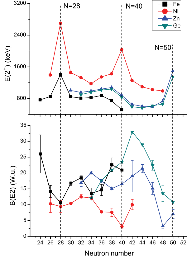
Figure 2.3: Systematics of 2^+ excitation energies and B(E2, 2^+ \rightarrow 0^+) values for the even-even nuclei around nickel. Data taken from [13–21].
