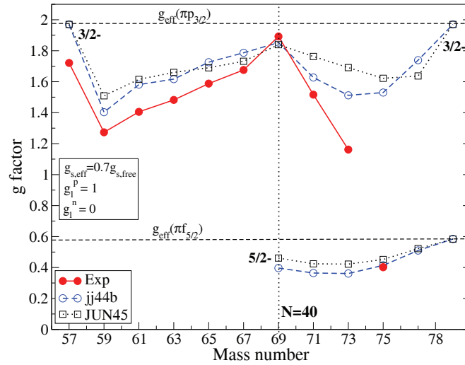
Figure 8: (color online) Experimental g -factors (filled dots) compared with calculations (open symbols) using the jj44b and JUN45 interactions [17]. An effective spin g -factor of 0.7g_{s,\text{free}} was adopted.
