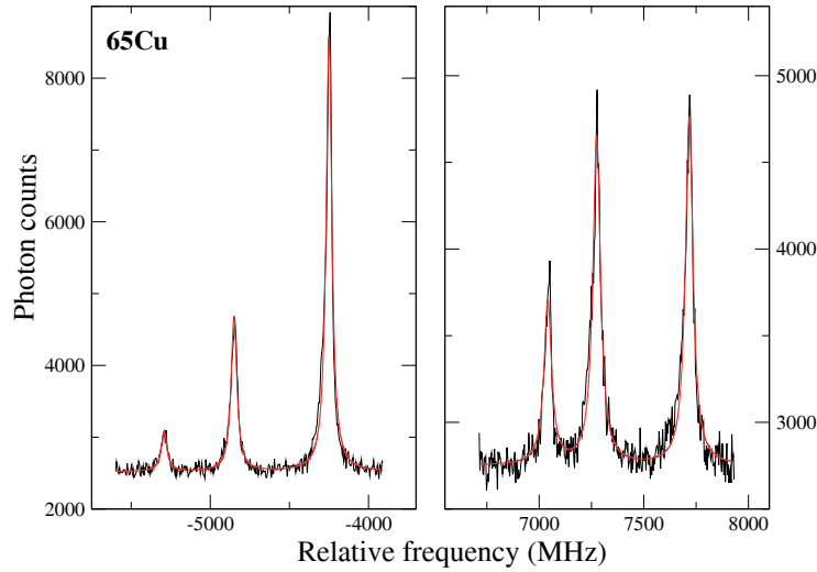
Figure 5.2: Example of a 65 Cu hyperfine spectrum converted to frequency.
