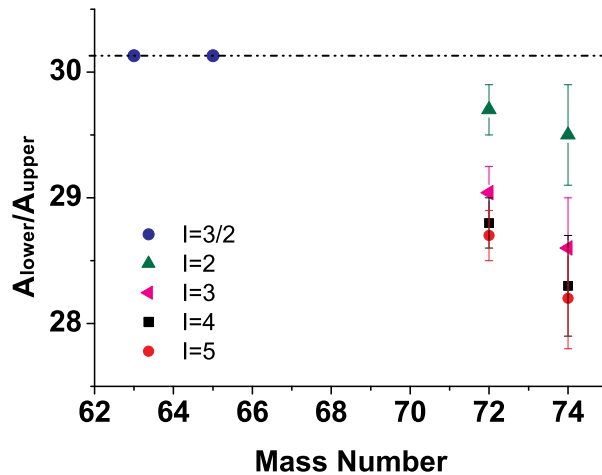
Figure 3: (Color on-line) Plot of the hfs A coefficient ratio of the ^2S_{1/2} and ^2P_{3/2} states. The values for the stable isotopes ^{63,65}\text{Cu} are compared to the values obtained for ^{72,74}\text{Cu} using nuclear spin options I = 2, 3, 4 and 5 to fit observed spectra.
