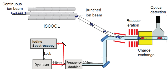
Figure 1: (Color online) Experimental setup of the COLLAPS collinear laser spectroscopy beamline.
