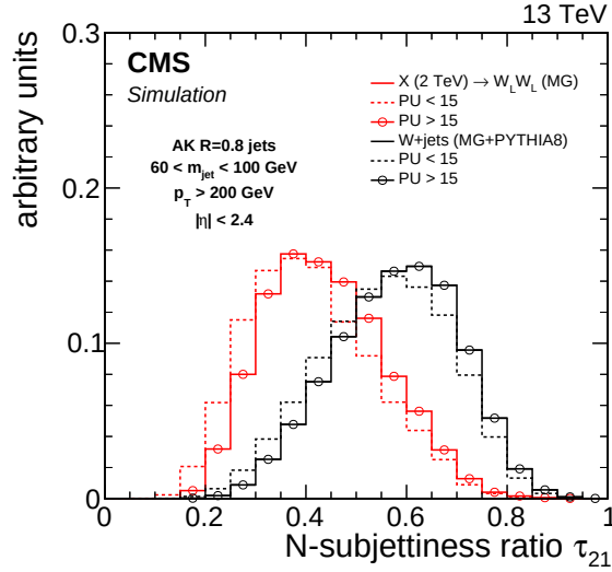
Figure 7.2: Distribution in N-subjettiness ratio \tau_{21} for simulated events of highly-boosted and longitudinally-polarized W bosons and inclusive QCD jets expected in the W +jets process. The distributions are shown after a selection on the mass of the pruned jet requiring 60 < m_{\text{jet}} < 100 GeV. The histograms are the expected distributions after full CMS simulation with pileup corresponding to an average number above and below 15 interactions.
