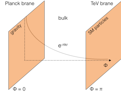
Figure 2.10: Setup of the five dimensions in the RS1 model. The Planck and TeV branes are the 4-dimensional boundaries of the extra dimension \phi compactified in an interval [0, \pi] .
