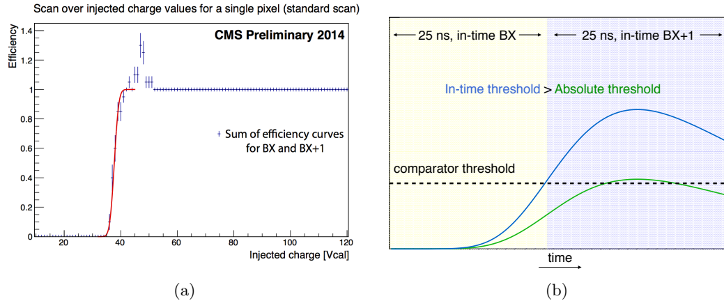
Figure 15.14: (a) Single pixel efficiency curve determined performing a scan over injected signal amplitudes ( Vcal ). The curve is the result of the sum of efficiency curves for the in-time bunch crossing (BX) and the following one (BX+1). Points exceeding the 100% efficiency are due to statistical fluctuations of the two curves in the turn-on region. The effect on the fit is negligible. (b) Diagram illustrating the difference between in-time and absolute thresholds due to the finite rise-time of the signals.
