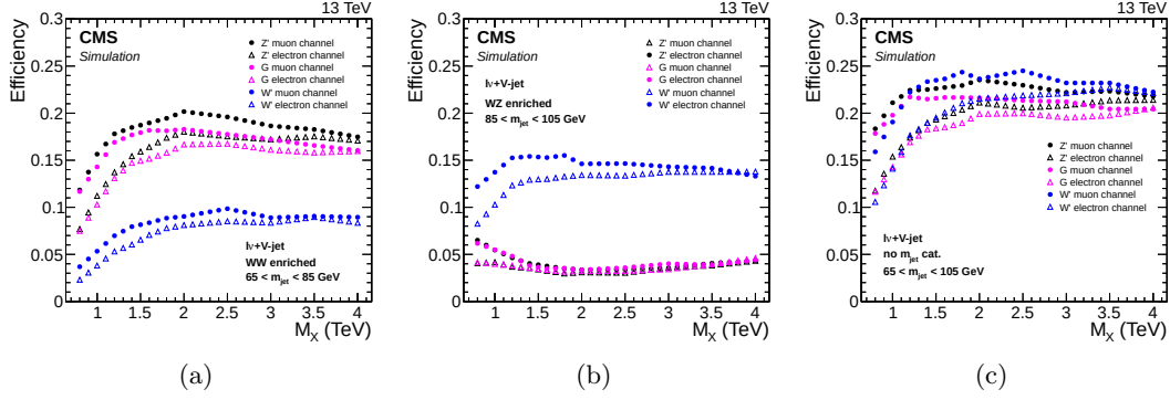
Figure 8.16: Signal efficiency in the \ell\nu q\bar{q} analysis channel as a function of the generated resonance mass for all signal benchmarks and for different m_{\text{jet}} selection: (a) WW-enriched category; (b) WZ-enriched category; (c) 65 < m_{\text{jet}} < 105 GeV.
