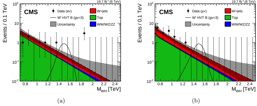
Figure 9.1: Final distributions in m_{WH} for data and expected backgrounds for electron (a) and muon (b) categories. The 68% error bars for Poisson event counts are obtained from the Neyman construction [164]. The hatched region indicates the statistical uncertainty of the fit combined with the systematical uncertainty in the shape. This figure also shows a hypothetical W' signal with mass of 1.5 TeV, normalized to the cross section predicted by the HVT model B with parameter g_V = 3 as described in Section 2.3.3.
