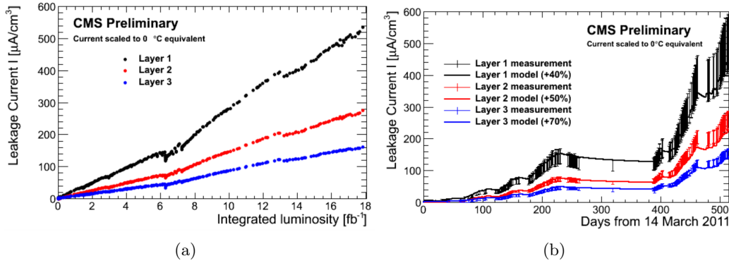
Figure 15.1: Leakage current scaled to 0^\circ\text{C} operational temperature for the barrel layers as a function of the integrated luminosity (a) and time (b) in 2011-2012 [188].
