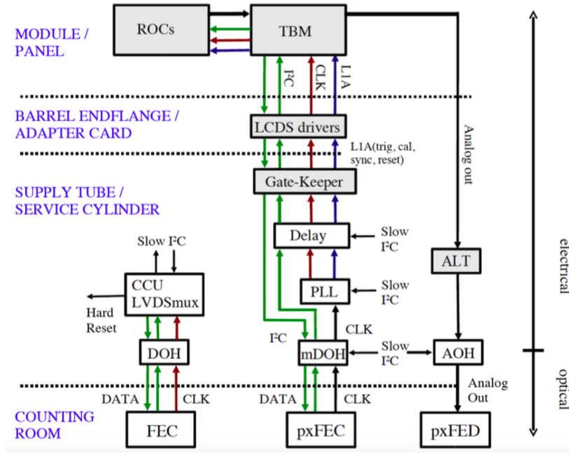
Figure 14.6: Overview of the BPix readout and control system [180].
