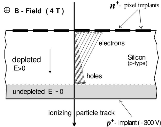
Figure 14.4: Illustration of a charged particle crossing a sensor of the CMS pixel detector. The charge carriers produced by the passage of the ionizing particle are collected at the high dose n^+ implants.
