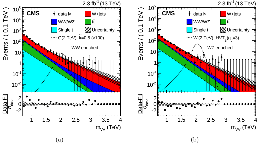
Figure 10.1: Final m_{WV} distributions for data and expected backgrounds obtained combining muon and electron channels in the WW-enriched (a) and WZ-enriched (b) signal regions. In each plot the solid curve represents the background estimation provided by the \alpha ratio method. The hatched band includes both statistical and systematic uncertainties. The data are shown as black points. At the bottom of each plot are the bin-by-bin fit residuals, (N_{\text{data}} - N_{\text{fit}})/\sigma_{\text{data}} , shown together with the uncertainty band of the fit normalized by the statistical uncertainty of data, \sigma_{\text{data}} . The distributions for a bulk graviton and for a W' signal are also shown with black dashed lines.
