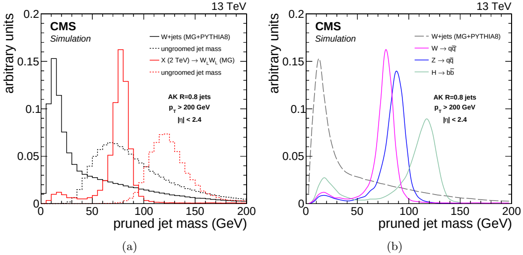
Figure 7.1: (a) Mass distributions for the pruned jet in simulated events of highly-boosted and longitudinally-polarized W bosons and inclusive QCD jets expected in the W+jets process. The ungroomed jet mass is shown as a dotted line to illustrate the effect of pruning. MG denotes the MADGRAPH generator. (b) Comparison of the distributions in m_{\text{jet}} for simulated events of highly boosted V and Higgs bosons.
