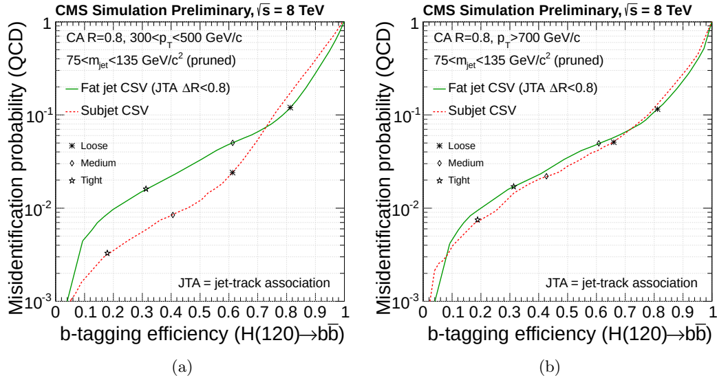
Figure 7.4: Misidentification probability as a function of b -tagging efficiency for boosted H \rightarrow b\bar{b} jets and inclusive QCD jets for the CSV algorithm applied to CA8 jets and pruned subjects for jets with (a) 300 < p_T < 500 \text{ GeV} and (b) p_T > 700 \text{ GeV} . Loose, medium, and tight operating points of the CSV discriminator are indicated [127].
