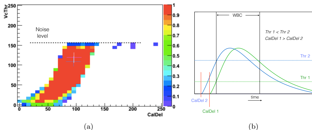
Figure 15.11: (a) Efficiency for detecting a hit as a function of the comparator threshold ( VcThr ) and delay ( CalDel ) settings for one ROC. Large values of VcThr , corresponding to a low threshold, generate much noise that saturates the digital circuit and no hits are detected. The optimal point is indicated in black while the blue point indicates the old settings. For small values of VcThr the signal reaches the threshold later and hence a smaller delay is needed for the signal. This behavior is illustrated in (b).
