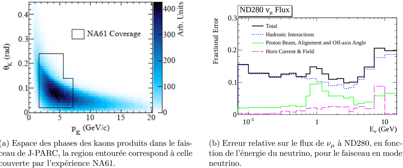
FIGURE 2.8 – Figures provenant de [70].
