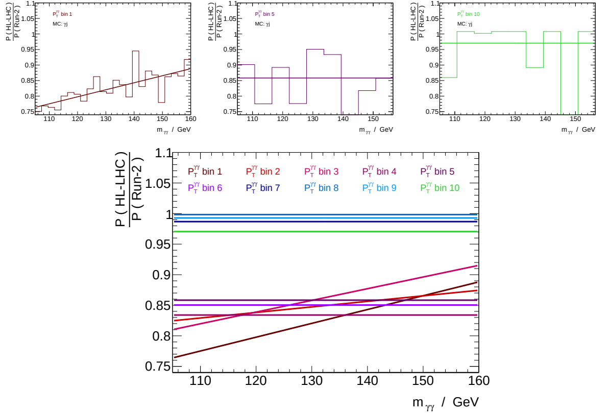
Figure 8.6: Parameterisation of \omega_{\gamma j}^{\text{bkg}} \equiv \frac{P(\text{HL-LHC})}{P(\text{Run-2})} from reweighted simulation in (top) three individual bins of p_T^H \equiv p_T^{\gamma\gamma} and (bottom) in all bins.
