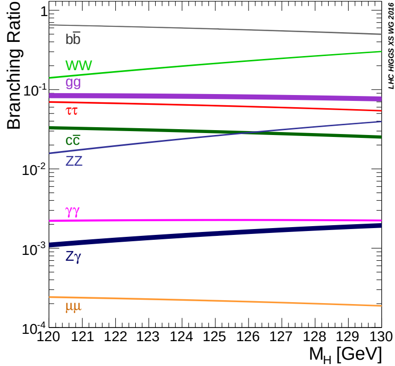
Figure 2.9: Branching ratios of the Higgs provided by Ref. [28]. The Higgs mass is 125.09 \pm 0.24 GeV measured by ATLAS and CMS in Run 1 [26].
