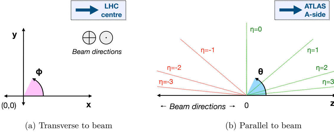
Figure 4.2: ATLAS coordinate system. The x, y -plane is transverse to the beamline which runs parallel to the z axis. Beams collide at the interaction point at (x, y, z) = (0, 0, 0) . Solid angles are defined by the coordinates, (\eta, \phi) .
