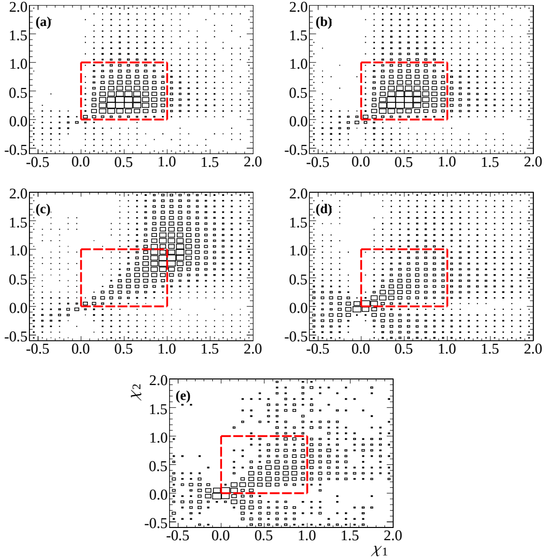
Figure 5.19: Correlations between the visible momentum fractions \chi_1 and \chi_2 for the leptonic final state shown for (a) H \rightarrow \tau\tau with m_H=120 GeV, (b) Z \rightarrow \tau\tau , (c) Z \rightarrow \ell\ell , (d) t\bar{t} and (e) W + \text{jets} events. The dashed box indicates the physical range 0 < \chi_{1,2} < 1 in the collinear approximation.
