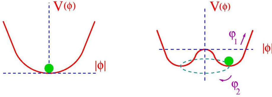
Figure 2.1: Illustration of the Higgs potential for \mu^2 > 0 (left) and \mu^2 < 0 (right). In the latter case, spontaneous symmetry breaking occurs when the system moves to one of the ground states [7].
