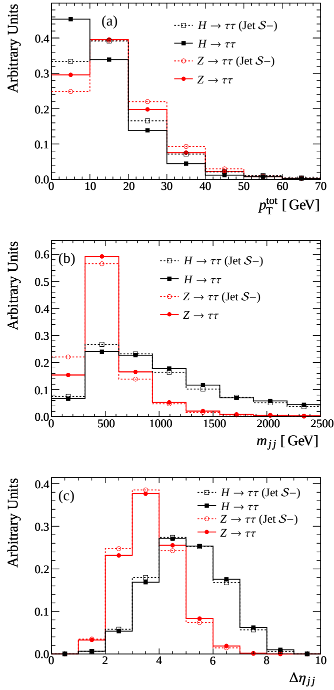
Figure 8.3: Distributions of (a) p_T^{\text{tot}} , (b) m_{jj} and (c) \Delta\eta_{jj} for the signal (squares) and the Z \rightarrow \tau\tau background (circles) without (full lines) and with a systematic shift of the jet energy scale towards lower values (Jet S^- , dashed lines).
