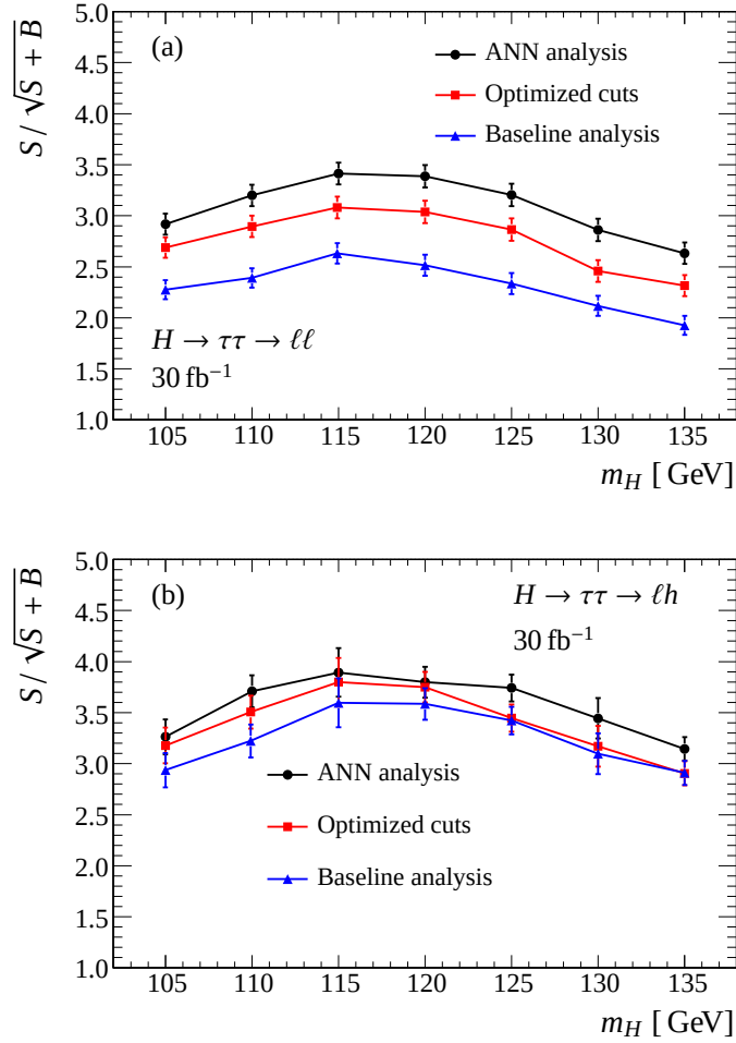
Figure 8.2: Expected signal significance S / \sqrt{S+B} of the optimized cut-based and the ANN analysis for (a) the leptonic and (b) the semileptonic channel and an integrated luminosity of 30 \text{ fb}^{-1} as a function of the Higgs mass. For comparison, the results obtained by the baseline analysis are shown. The error bars indicate the uncertainty due to the limited Monte Carlo statistics.
