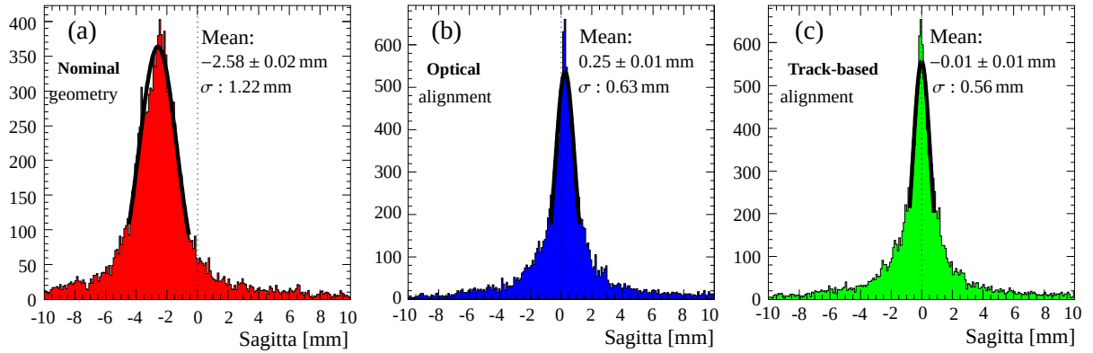
Figure 4.9: Distributions of the measured sagitta of straight cosmic muon tracks in the ATLAS muon spectrometer without magnetic field (a) without applying corrections to the actual muon chamber positions after installation, (b) after taking into account the information of the optical alignment system and (c) after applying misalignment corrections determined with the alignment algorithm using straight cosmic muon tracks [41].
