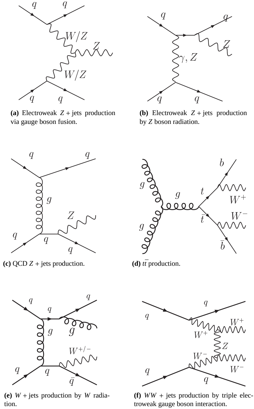
Figure 5.2: Tree-level Feynman diagrams of the dominant background processes.
