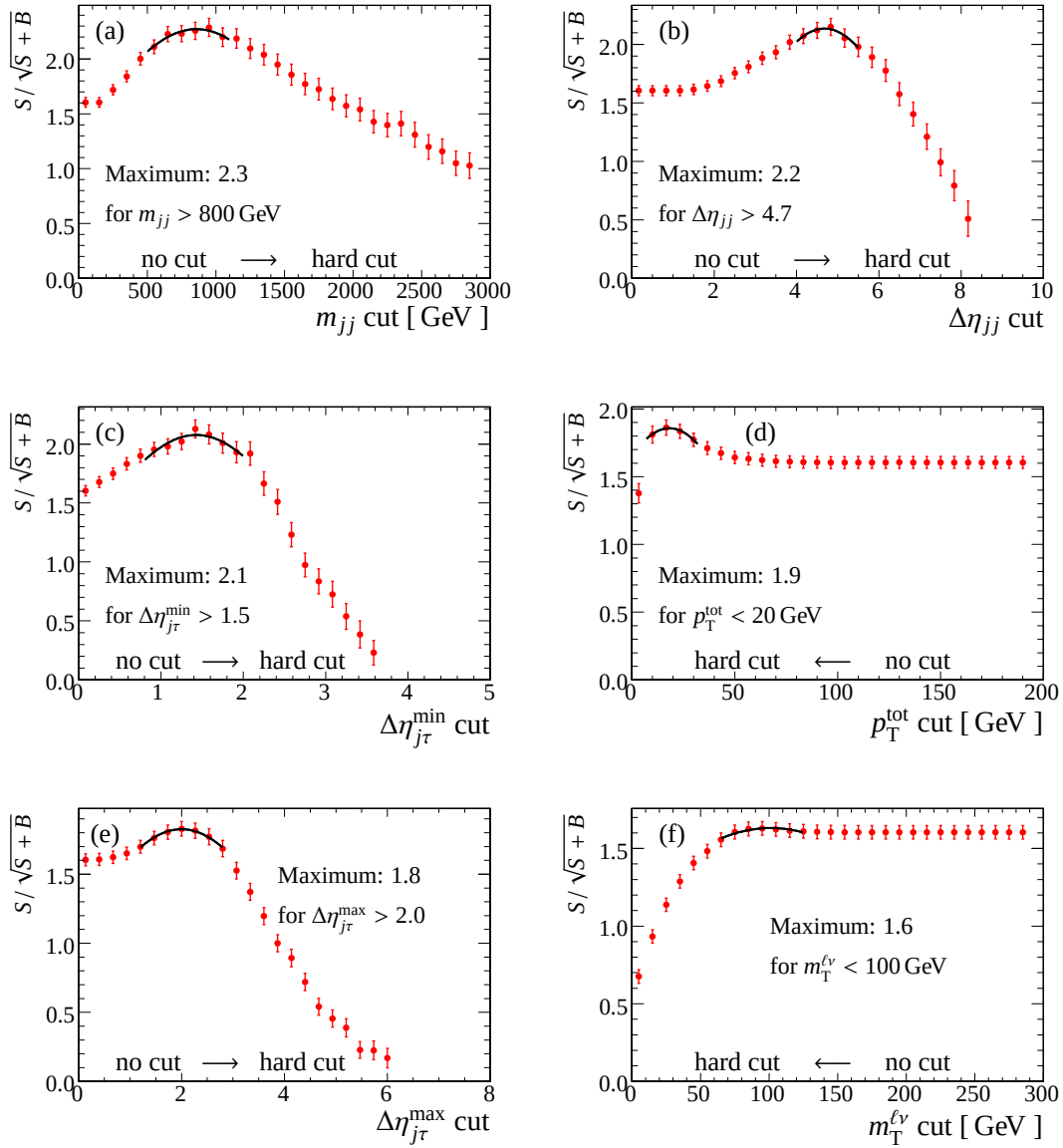
Figure 6.2: The ratio S / \sqrt{S+B} as a function of the cut value for selected discriminating variables (see text). Applying cuts on these variables improves S / \sqrt{S+B} . The Gaussian fits around the maxima of the functions are indicated.
