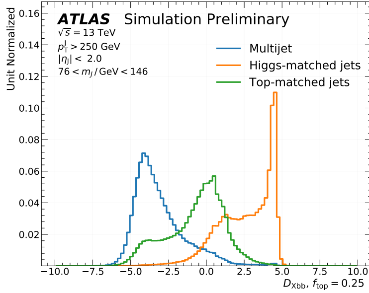
Figure 8.1: The distributions of D_{Xbb} with f_{top} = 0.25 for the Higgs, multijet, and top jets. The multijet and Higgs jets are well separated by D_{Xbb} , while the Higgs and top jets D_{Xbb} distributions overlap more. The graphic is taken from [193].
