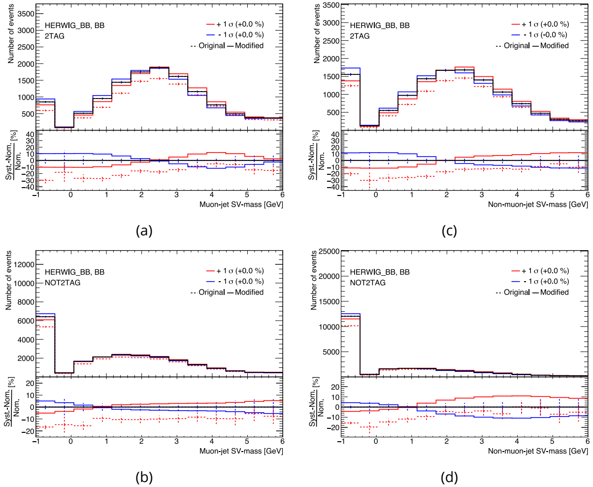
Figure 8.14: The parton shower and hadronisation uncertainty on the BB template before (dotted cross) and after smoothing (solid line) in the fitted SV mass distributions at the 50% WP in the bin with large-R jet p_T : 600 < p_T < 750 GeV. The +1\sigma ( -1\sigma ) up (down) variation is shown by the red (blue) solid line, with the normalisation removed.
