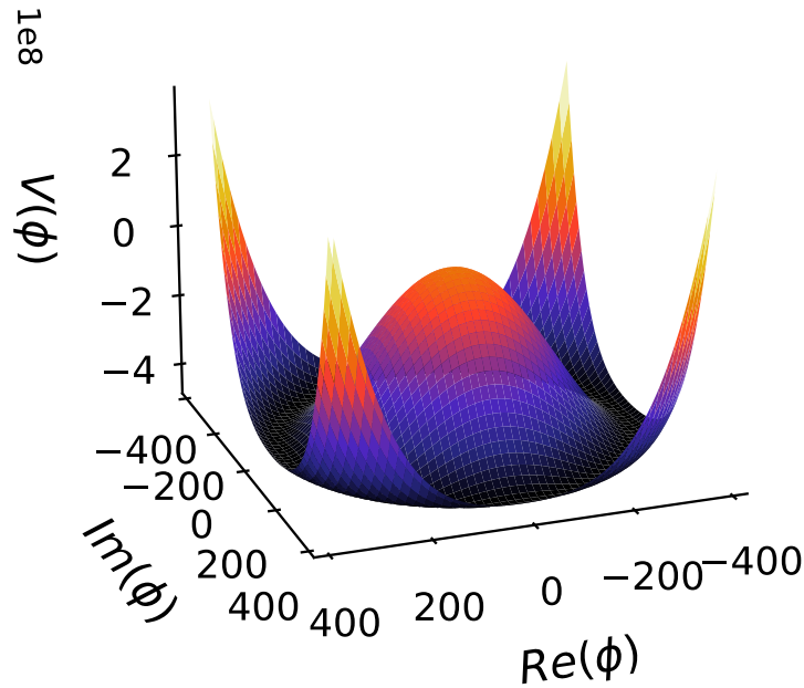
Figure 1.2: The Higgs potential, V(\phi) = \mu^2 \phi + \lambda(\phi^\dagger \phi)^2 , where \mu^2 < 0 .
