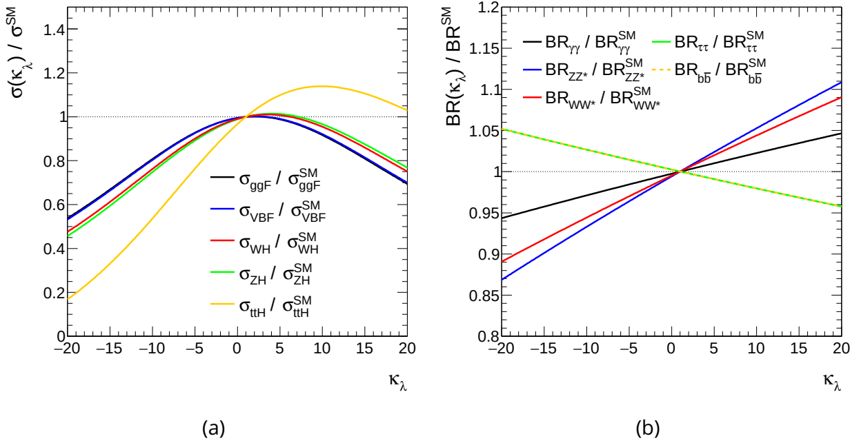
Figure 2.8: The modification of the SM production signal strength, \mu^i , is shown in (a), while the branching fraction correction, \mu^f , is shown in (b). The figure is taken from [42], which calculates \mu^i and \mu^f according to Equation 2.10 and 2.11 using the values for C_1^j , K_{EW}^j and k_j^2 as obtained by [43, 44].
