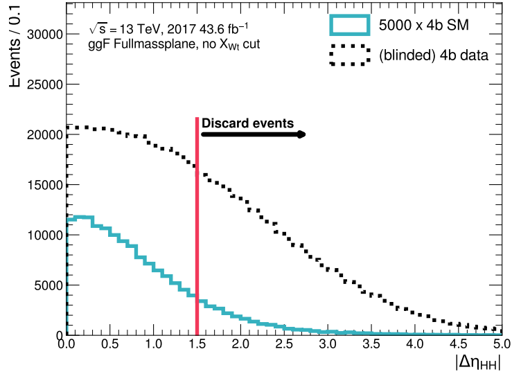
Figure 6.6: The distribution of the blinded 4b data (dotted line) and the ggF SM 4b signal (solid line) is shown. It can be seen that placing a cut \Delta\eta < 1.5 reduces the background, while the majority of the signal is still kept. The data shown was collected during the year 2017 of data taking. The SM HH signal is normalised to the SM cross-section obtained from theory, and scaled to the integrated luminosity collected during 2017. In addition, the SM HH signal is scaled by a factor of 5000 for easier visualisation.
