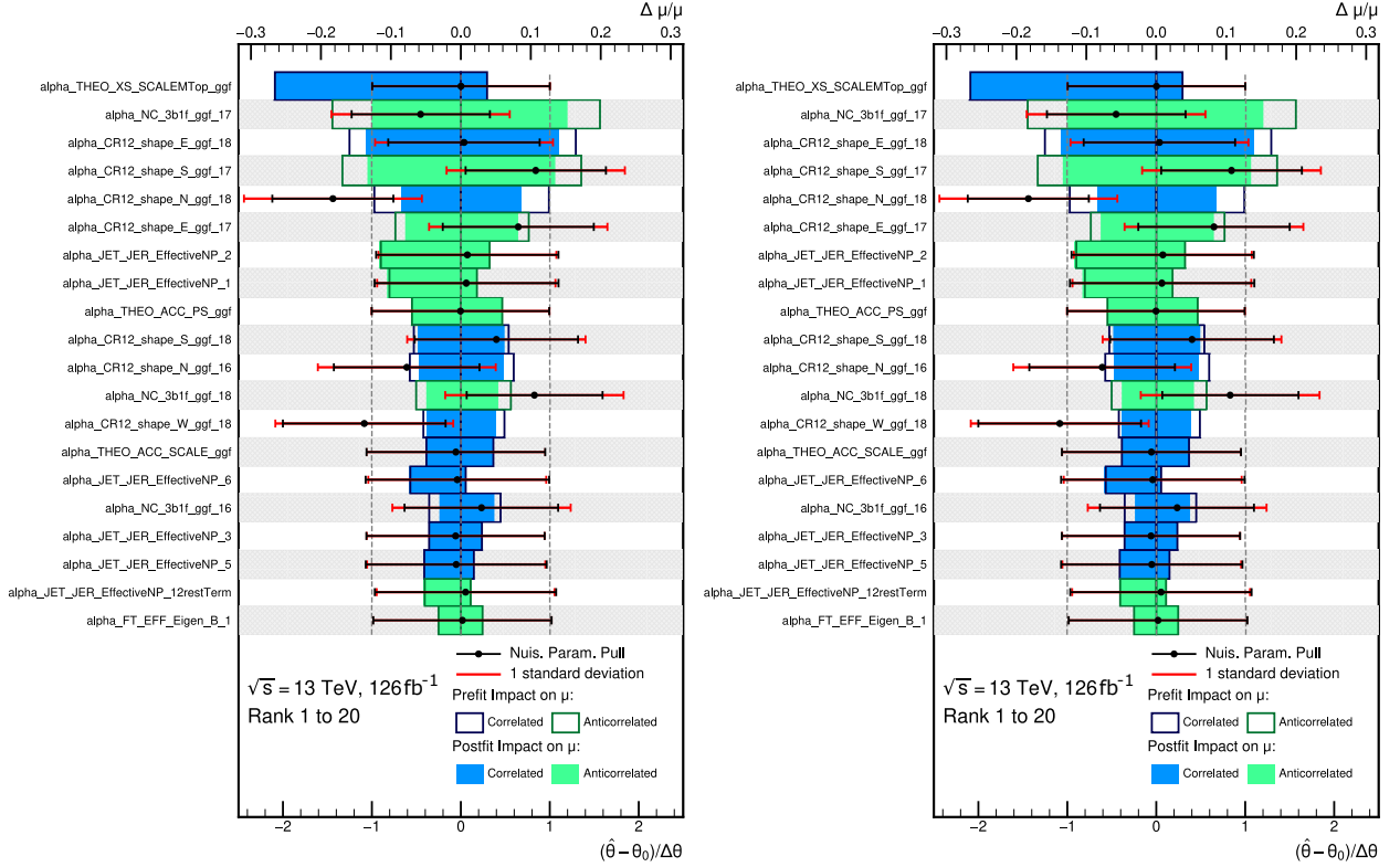
Figure 6.20: The pulls on the nuisance parameters (NPs) and impacts as extracted from the fit with \mu_{ggF+VBF} , as the POI. To pre-fit impact (green or blue rectangle) of a nuisance parameter ( \theta ) is defined as the change in the POI when the systematic under question is fixed to \theta \pm \sigma_\theta in the likelihood fit. Similarly, the post-fit impact (blue or green shaded area) is computed, only that \theta is fixed to \hat{\theta} \pm \hat{\sigma} , where the hat indicates the values that maximise the likelihood in the unconstrained fit. The procedure is repeated for each nuisance parameter in the fit. The plot shown is called a ranking plot as it shows the nuisance parameters ranked by the size of their relative post-fit impact on the POI. The upper x-axis indicated the size of the relative impact \frac{\Delta\mu}{\mu} , where \mu = \mu_{ggF+VBF} and \Delta\mu is the change in \mu_{ggF+VBF} when the NP examined is fixed in the fit. The lower x-axis shows the size of the pull on an NP (\frac{\hat{\theta} - \theta_0}{\Delta\theta}) , \hat{\theta} is the best-fit value taken by the NP, \theta_0 is the pre-fit value and \Delta\theta is the uncertainty on \theta_0 . The red line indicates the unconstrained ( 1\sigma ) NP. Only the 40 highest-ranked nuisance parameters are shown. The NPs representing the non-closure systematic estimated from the alternative background estimation are labelled as alpha_CR12_shape_{quadrant}_{channel}_{year} . The alpha_NC_3B1f_ggF_{year} is the non-closure systematic derived in the 3b1f validation region. The NPs encoding the systematic uncertainties in the jet reconstruction due to energy resolution, scale, and pileup modelling to name a few have the prefix alpha_JET_{NP name} , while the flavour tagging NPs have the prefix alpha_FT_{NP name} and alpha_SF_PRW is the uncertainty in the pileup reweighting. The theoretical uncertainties have the prefix alpha_THEO_{NP name}_{signal} , for example, alpha_THEO_XS_SCALEMTOP_ggf is uncertainty in the ggF production cross-section, due to the scale choice and finite top mass scheme.
