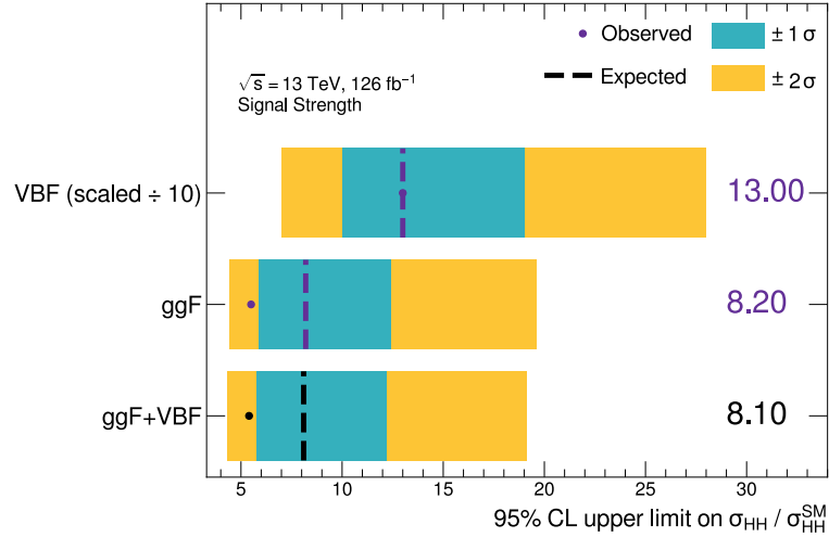
Figure 6.21: The upper limit on the signal strength of the SM VBF, ggF, and combined ggF+VBF HH production is plotted. The limits on the VBF signal are scaled down by a factor of 10 for better visualisation. The observed limits are shown as a circle. The expected limits are shown as dashed lines and the 1\sigma ( 2\sigma ) error bounds are plotted as turquoise (yellow) bands.
