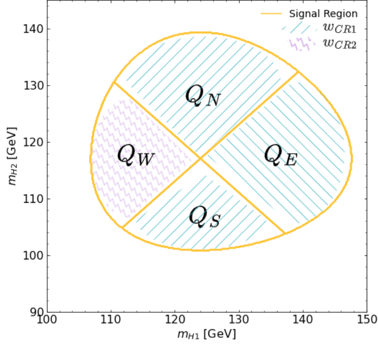
Figure 6.12: The SR split into quadrants is used to define the systematics of the CR12 non-closure from deriving an alternative background using weights derived in CR2. The example shown is how the CR12_shape_W NP is derived, the w_{CR2}(x) are applied only on 2b events in the SR quadrant Q_W (purple zigzag region), while in all other quadrants, the 2b events are reweighted with w_{CR1}(x) (turquoise hatched region).
