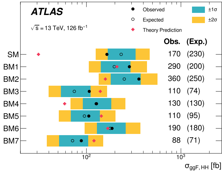
Figure 6.24: The upper limits set at a 95% confidence level on HEFT benchmarks and the SM point, defined in Table 2.1. The hollow black circle represents the expected limit and its corresponding 1\sigma ( 2\sigma ) error bounds as the turquoise (yellow) band. The observed upper limits are marked as a filled-in black circle. The pink crosses mark the theoretically predicted cross-section for each BM. The plot is shown as published in [2].
