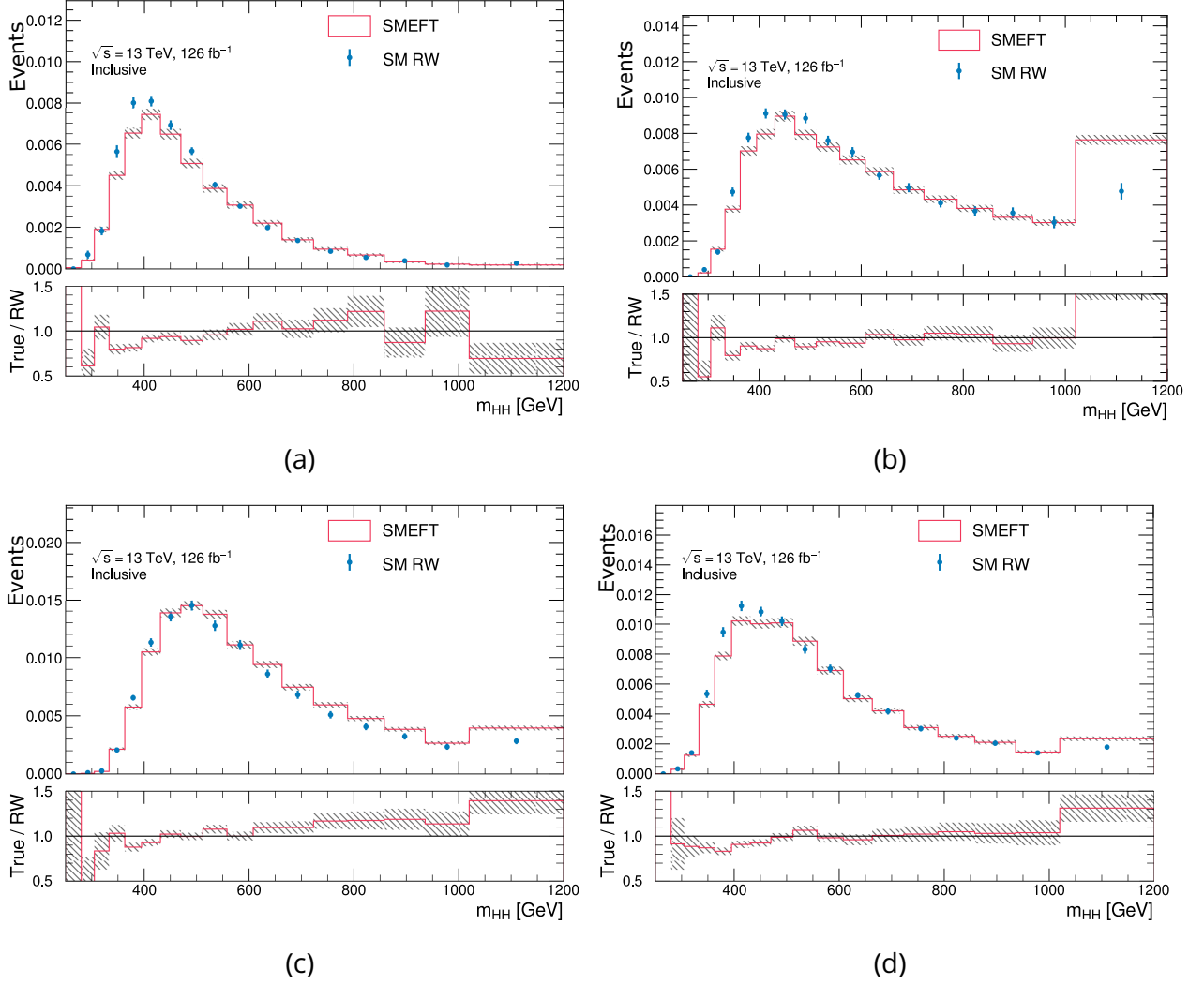
Figure 6.15: The simulated SMEFT signal (red line) is compared to the SM sample reweighted to the examined variation (blue dots) in bins of m_{HH} . The SMEFT variation shown are c_H = 14.93 in (a), c_{tG} = -0.9 in (b), c_H = -2, c_{tH} = 1.5 in (c), and c_H = -2.5, c_{tG} = 0.15 in (d). Only the statistical error is shown. As is the case for the HEFT signals as well the overflow (last bin) and underflow (first bin) exhibit the largest discrepancy.
