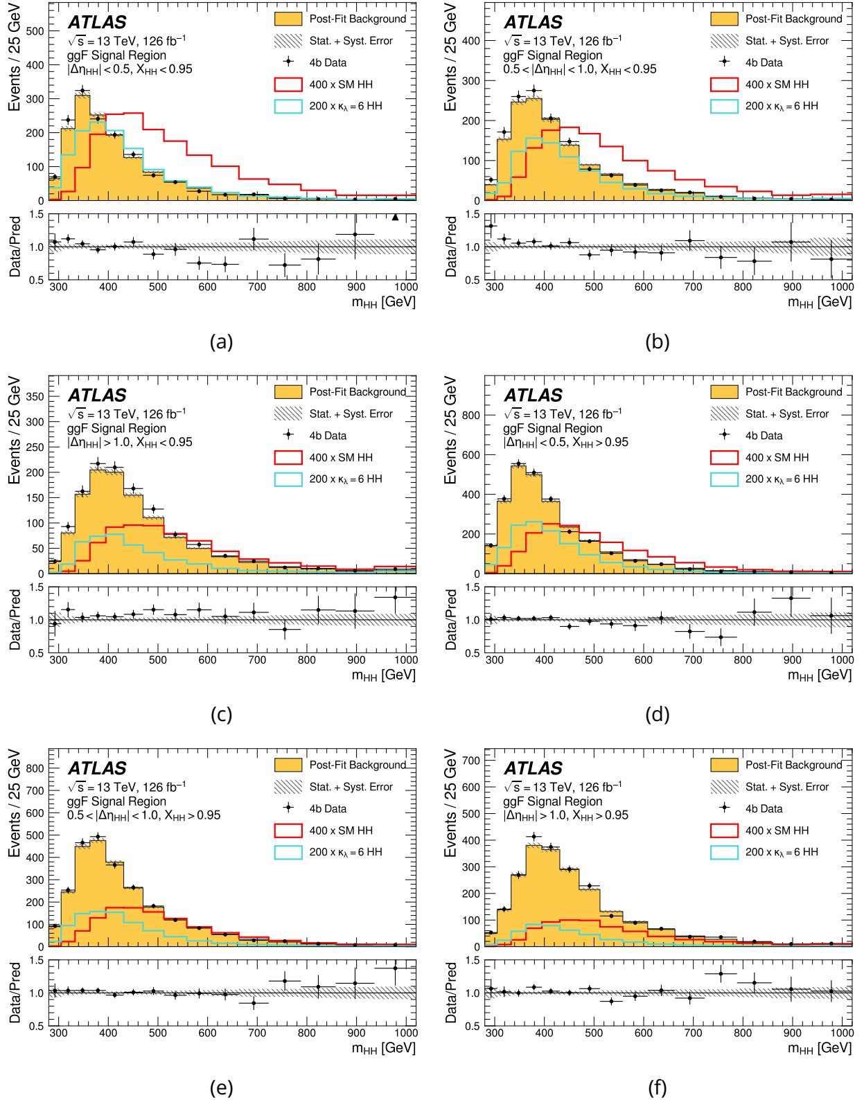
Figure 6.18: The data and post-fit background estimation, with the background-only hypothesis fitted, agree in all considered categories. Each year is considered to be a separate category in the fit, but for visualisation purposes, all the years are combined in the plots per kinematic category in |\eta_{HH}| and |X_{HH}| . The plot is overlaid with the scaled SM and \kappa_\lambda = 6 HH signals for greater clarity. The plots are published in [2].
