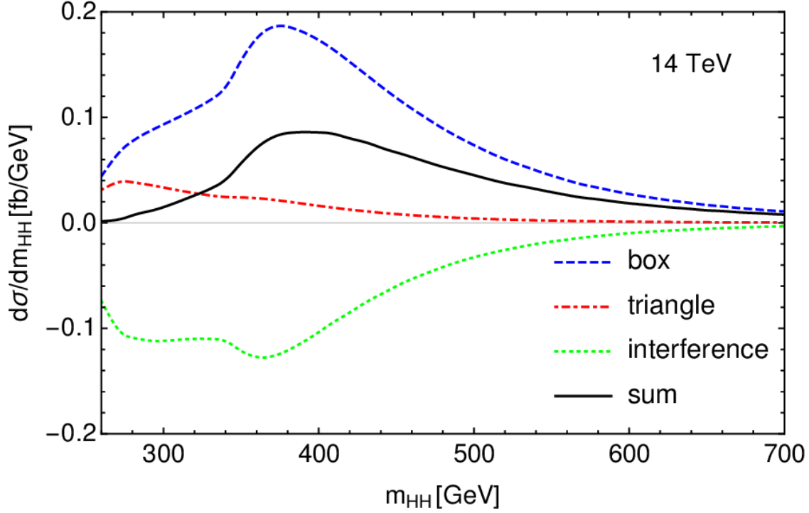
Figure 2.2: The expected m_{HH} spectrum in the ggF SM diHiggs production channel at \sqrt{s} = 14 TeV in a proton-proton collider is shown as the solid black line. The dashed lines show the different contributing terms, in blue is the box diagram, in green is the interference, and in red is the triangle term. The figure is taken from [33].
