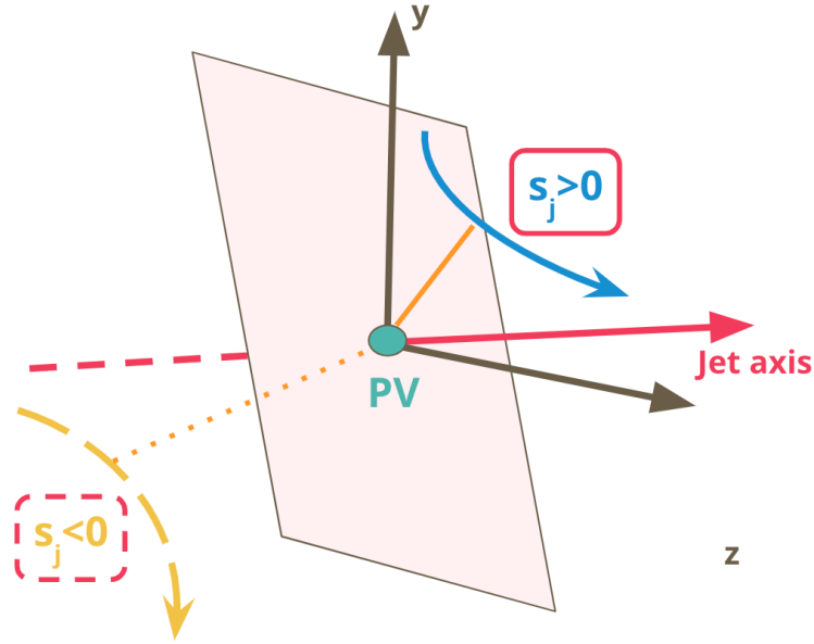
Figure 8.4: The method for determining the sign of the transverse impact parameter, denoted as s_j , for tracks that are ghost-associated with a jet. If the angle between the jet axis and the line connecting the closest approach point to the PV is less than 90^\circ , then s_j is positive. In the sketch, the blue track has s_j > 0 , while the yellow track has s_j < 0 . The shown plane is perpendicular to the jet axis.
