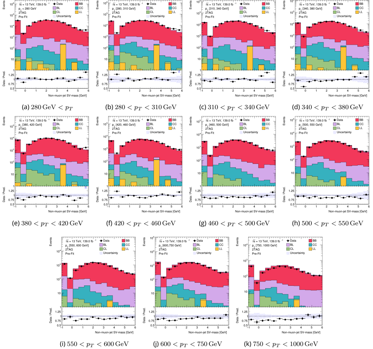
Figure 8.10: The pre-fit SV mass distribution in the non-muon jet pass region in different large-R jet p_T bins for the 50% WP.
