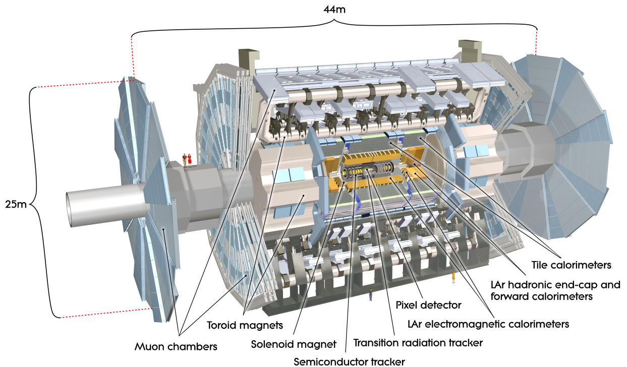
Figure 3.3: The ATLAS detector at the LHC as operated during Run 2 is depicted. The subdetector systems are labeled on the plot that has been taken from [68].
