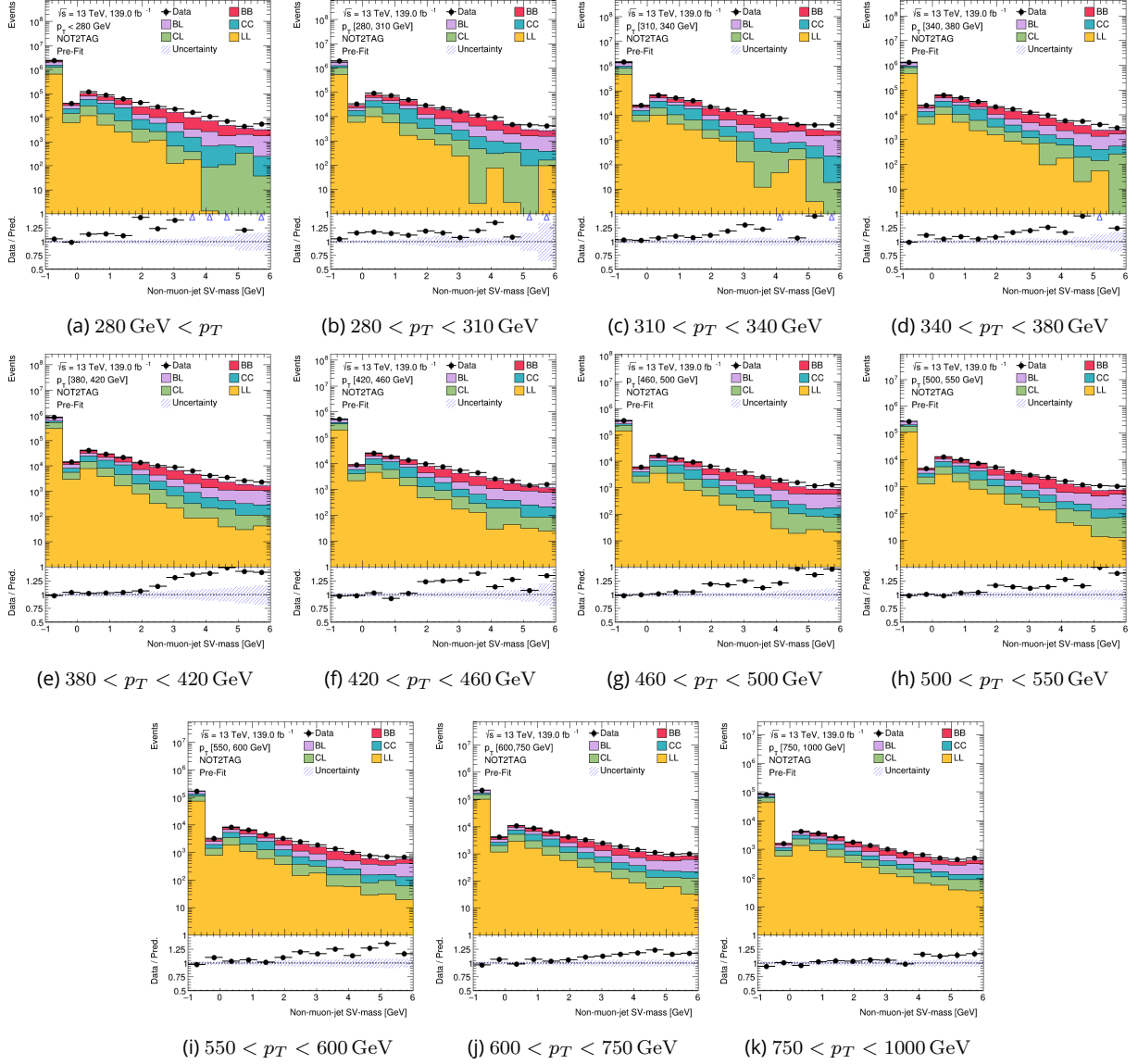
Figure 8.11: The pre-fit SV mass distribution in the non-muon jet fail region in different large-R jet p_T bins for the 50% WP. Mis-modelling in the tail of the SV mass distribution can be observed across the large-R jet p_T bins.
