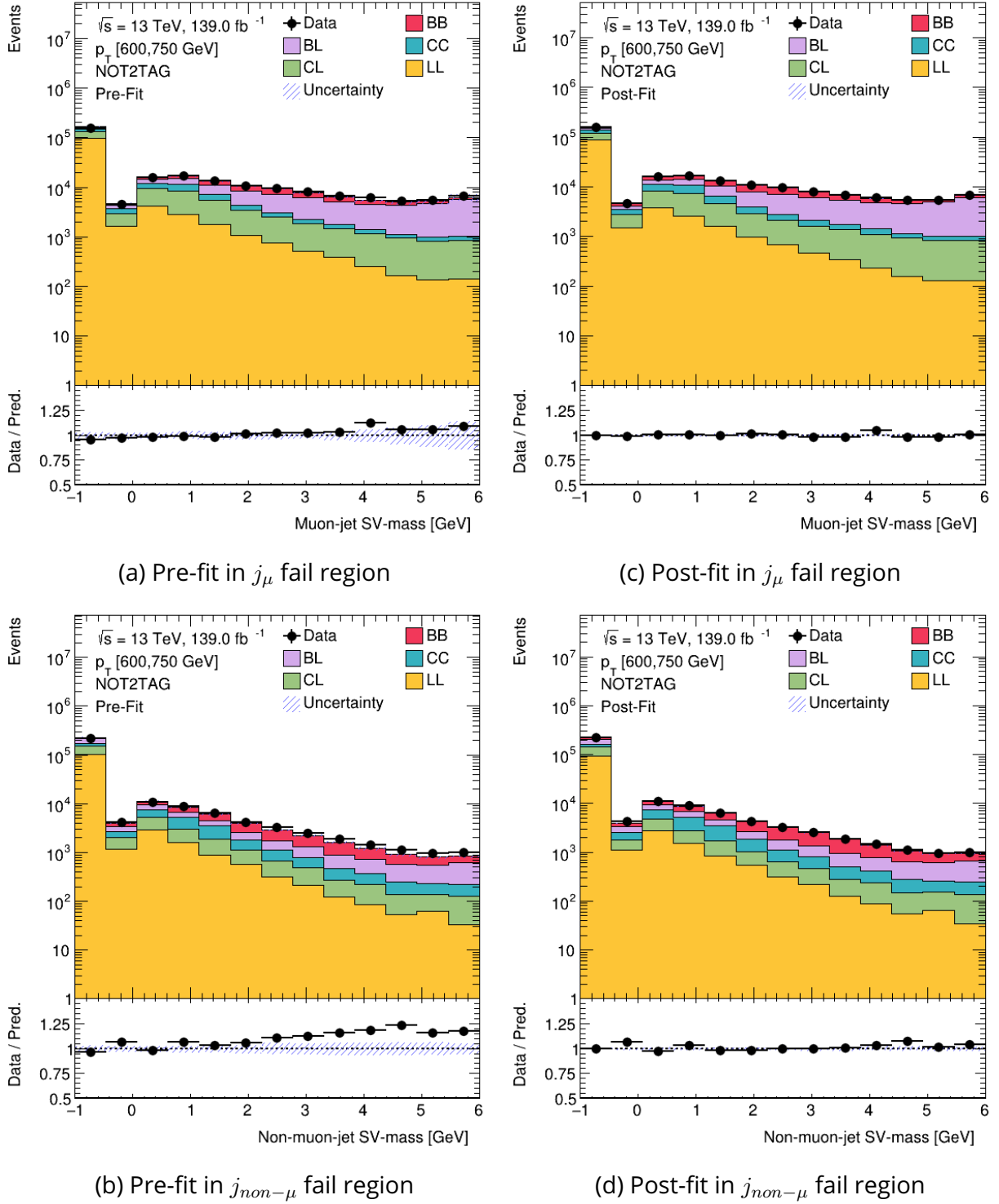
Figure 8.20: Pre- and post-fit SV mass distributions in the fail region at the 50% WP in the bin with large-R jet p_T : 600 < p_T < 750 GeV. The pre-fit distributions are on the left-hand side, the muon jet in (a) and the non-muon jet in (b). The post-fit distributions are on the right-hand side, the muon jet in (c) and the non-muon jet in (d).
