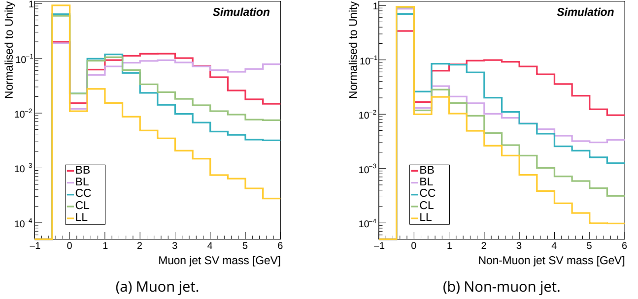
Figure 8.6: The simulated templates of the SV mass distribution for each flavour category in the inclusive large-R jet p_T bin. The enhanced tail at masses above 3.5 GeV in the muon jet, see the plot in (a), is observed only in the BL category. The source of the enhancement is the reconstruction of g \rightarrow b\bar{b} splittings as a single subject.
