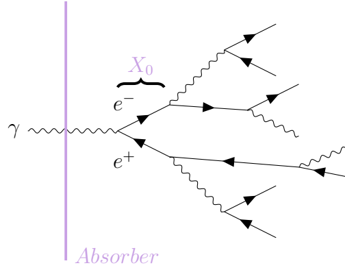
Figure 3.7: A simplified illustration of an electromagnetic shower initiated by a photon entering an absorption material with a radiation length X_0 .
