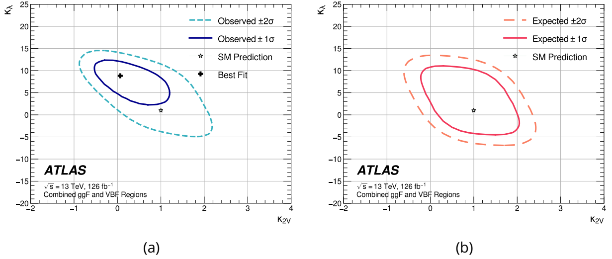
Figure 6.23: The observed in (a) and expected in (b) \pm 1\sigma (solid line) and \pm 2\sigma (dashed line) confidence contours in the \kappa_\lambda - \kappa_{2V} parameter space as derived from the -2\Delta \ln(L) scans are shown. The star indicates the SM point, while the best-fit ( \kappa_\lambda, \kappa_{2V} ) point in the observed data is shown as the cross. All other \kappa are fixed to their SM values. The figure has been published in [2].
