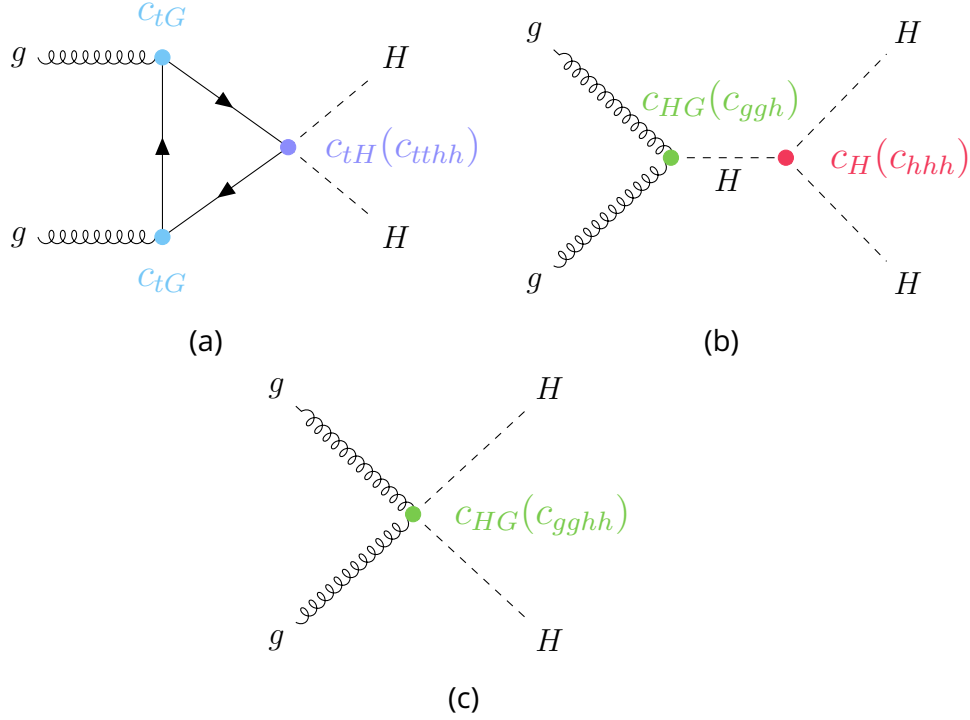
Figure 2.5: The BSM contributing diagrams from SMEFT dimension 6 and HEFT operators that can have a significant impact on the diHiggs production, the later are shown in brackets. The main difference is the Higgs coupling to the gluons, the ggHH and ggH vertex are moderated by the same operator in SMEFT but not in HEFT.
