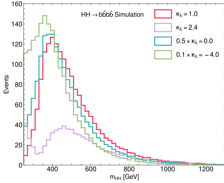
Figure 2.3: The reconstructed m_{HH} distribution for different \kappa_\lambda values is shown. Selection and reconstruction criteria resembling the one used in the HH \rightarrow b\bar{b}b\bar{b} analysis presented in this thesis are applied to the SM sample. The sample is showered with Pythia 8 and no detector simulation is used. To obtain the various \kappa_\lambda variations the SM sample is reweighted according to the strategy described in Chapter 6. The characteristic dip at \kappa_\lambda = 2.4 seen on the plot is wiped out by detector resolution effects. The \kappa_\lambda = 0.0 signal is scaled by 0.5, while the \kappa_\lambda = -4.0 signal is scaled by 0.1.
