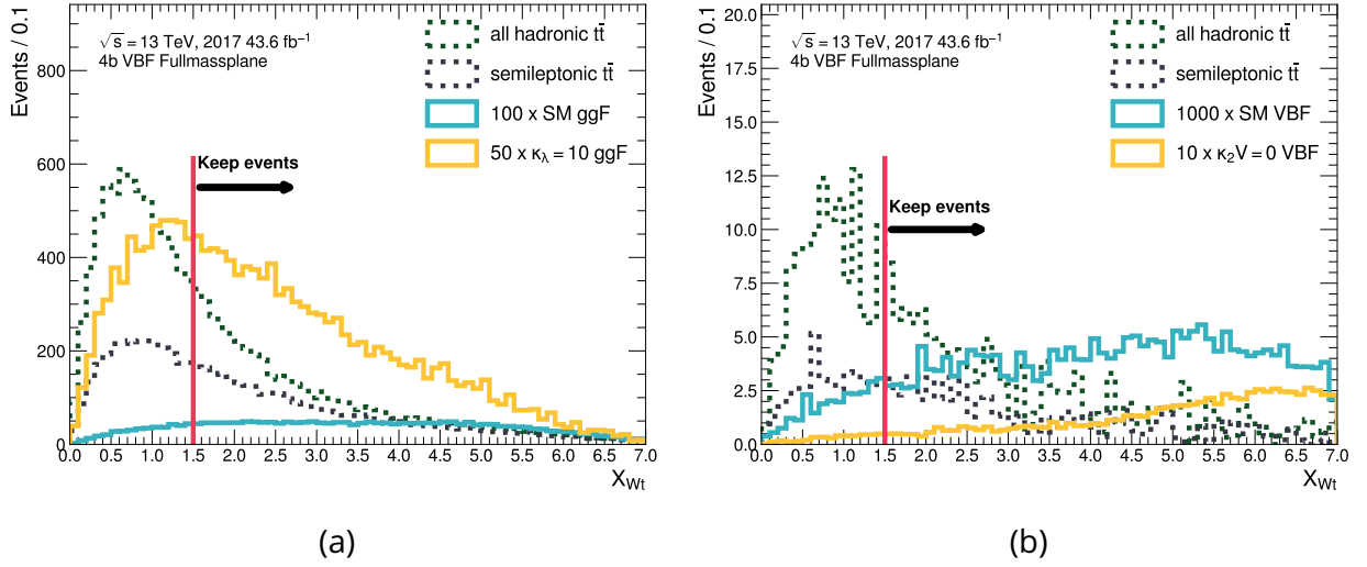
Figure 6.5: The X_{Wt} distribution for the fully hadronically (dotted green line) and semi-leptonically (dotted grey line) decaying t\bar{t} background in the ggF and VBF channels are shown along the SM (solid turquoise line) and a BSM (solid yellow line) non-resonant signal. The normalisation of the t\bar{t} sample is taken from the simulation, while the HH cross-section is the theoretically calculated value. All the histograms shown are scaled to the integrated luminosity collected during 2017. The SM ggF and VBF signals are scaled by a factor of 100, while the BSM ggF \kappa_\lambda = 10 (VBF \kappa_{2V} = 0 ) signal is scaled by a factor of 50 (10) for clarity.
