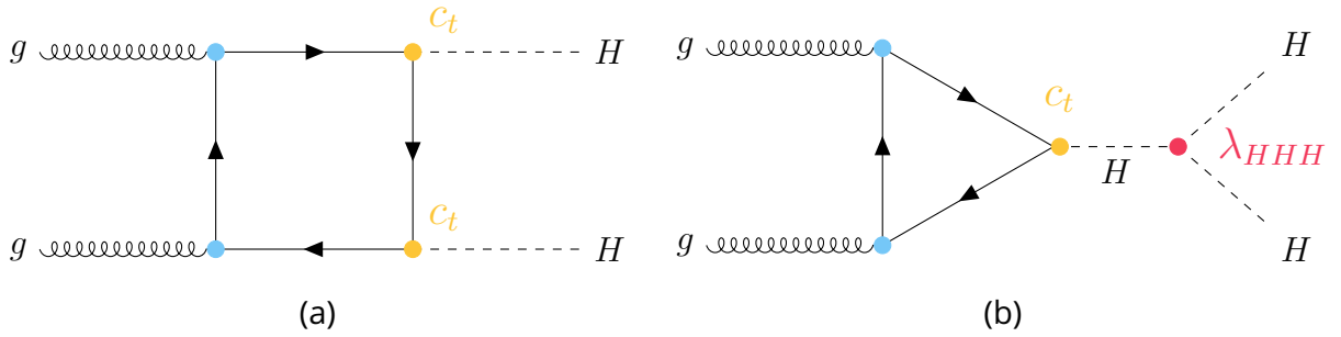
Figure 2.1: The two tree-level Feynman diagrams that contribute to the DiHiggs production via gluon-gluon fusion.
