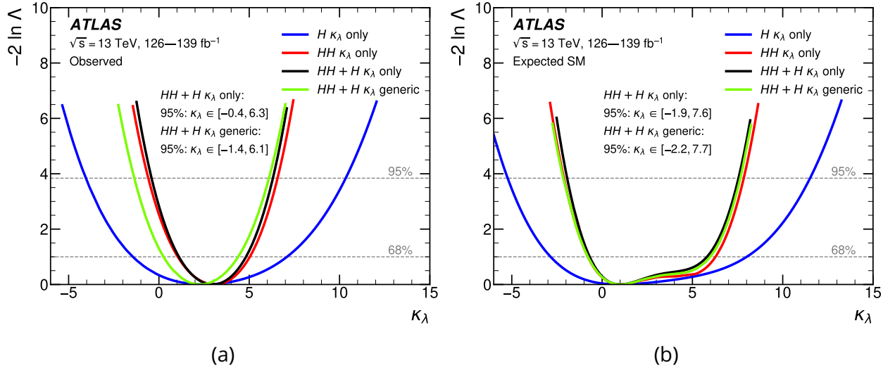
Figure 7.4: The -2 \ln \Delta test statistic with \kappa_\lambda as a POI is shown for the \kappa_\lambda only model (black line) and the \kappa_\lambda generic model (green line). Besides \kappa_\lambda the generic model allows \kappa_t , \kappa_b , \kappa_V and \kappa_\tau to float in the fit as well. The intersection of the test statistic with the 68% (95%) dashed lines sets the 68% (95%) confidence levels on \kappa_\lambda . The expected data assumes the SM HH signal exists. The publication containing the results is [3].
