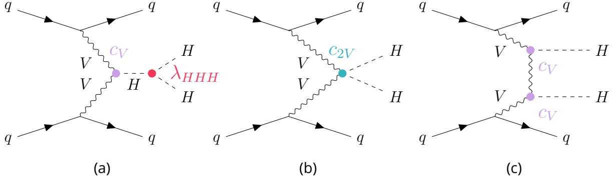
Figure 2.4: The three tree-level Feynman diagrams that contribute to the diHiggs production via Vector Boson Fusion.
