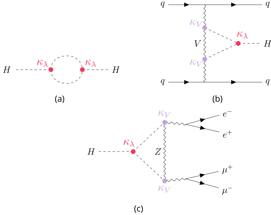
Figure 2.7: The impact of the trilinear Higgs self-coupling on single Higgs measurements via NLO corrections is shown. The quadratic dependence on \kappa_\lambda of the Higgs self-energy is depicted in (a). The diagram in (b) shows the dependence of the VBF production channel on \kappa_\lambda , while in (c) its impact on the Higgs decaying to two Z bosons can be seen.
