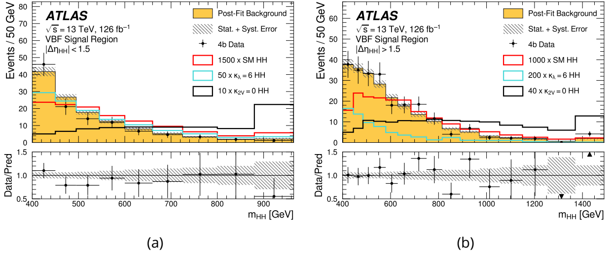
Figure 6.19: Good agreement between data and the post-fit background estimation is observed in both VBF categories, the |\eta_{HH}| < 1.5 category shown in (a) and |\eta_{HH}| > 1.5 category in (b). The post-fit background estimation is shown for the profile likelihood fit assuming the background-only hypothesis. The expected SM, \kappa_\lambda = 6 , and \kappa_{2V} = 0 HH signals are overlaid on the plot and scaled for better visualisation. The two plots have been published in [2].
