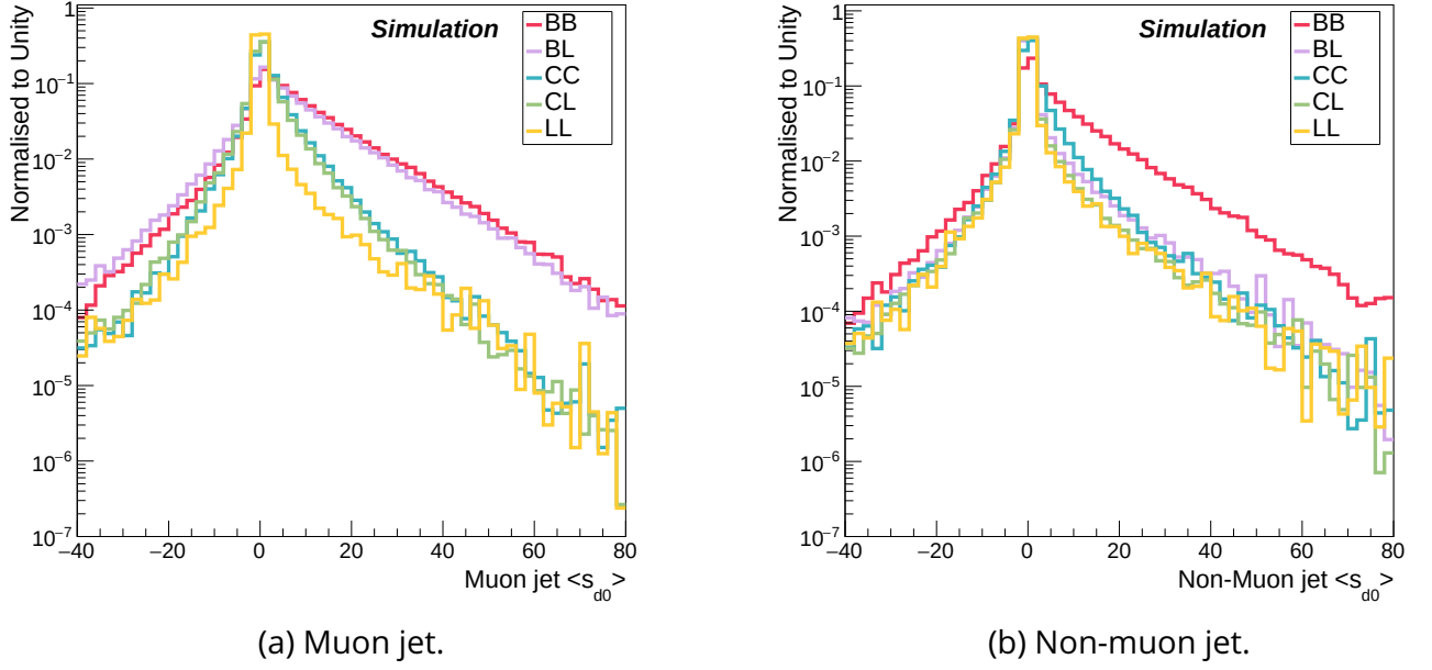
Figure 8.5: The templates of the simulated \langle s_{d0} \rangle distributions for each flavour category in the inclusive large-R jet p_T bin.
