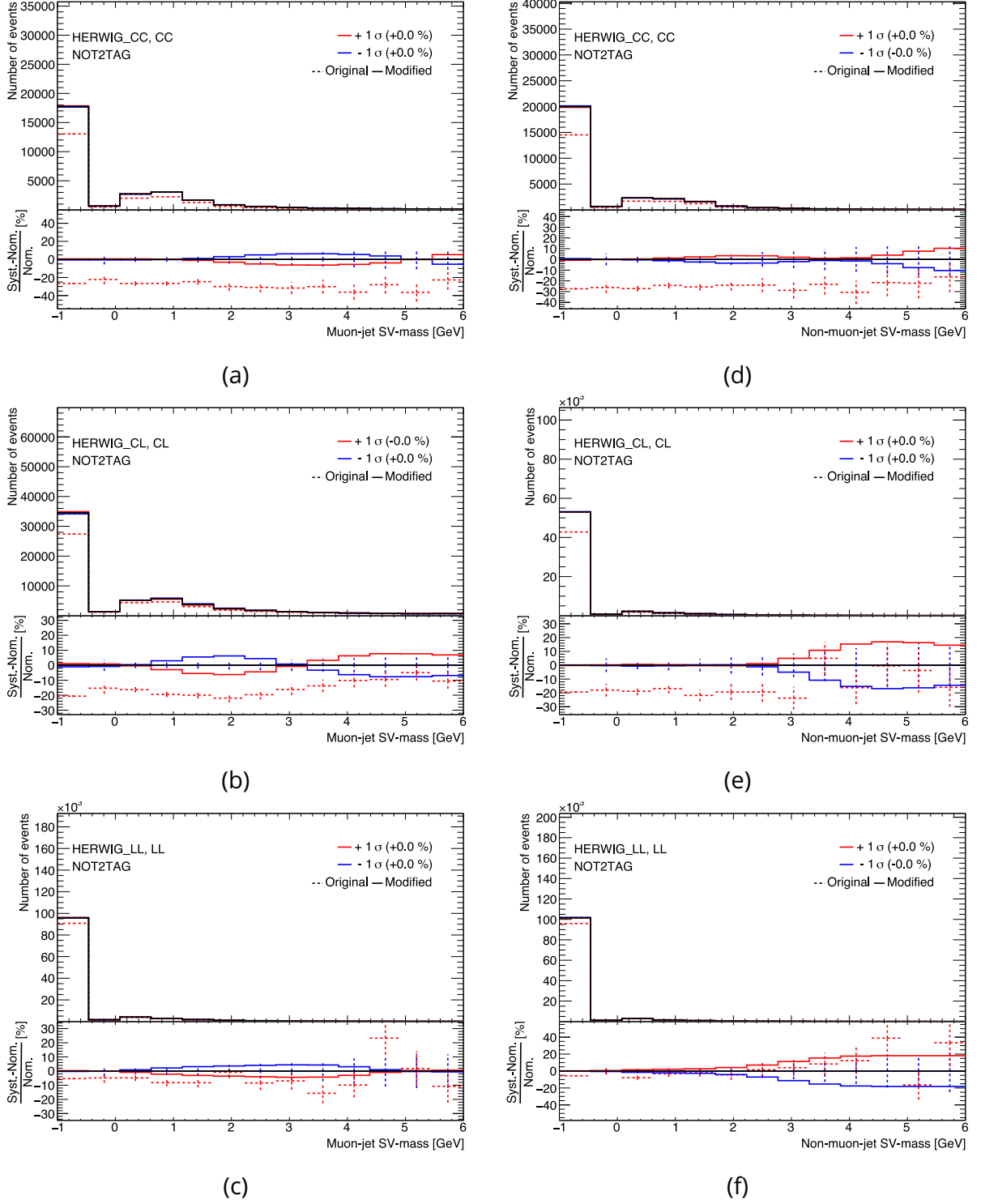
Figure 8.16: The parton shower and hadronisation uncertainty on the CC, CL, and LL templates before (dotted cross) and after smoothing (solid line) in the fitted SV mass distributions at the 50% WP in the bin with large-R jet p_T : 600 < p_T < 750 GeV. The +1\sigma ( -1\sigma ) up (down) variation is shown by the red (blue) solid line, with the normalisation removed. The systematics in the pass regions are dropped by pruning.
