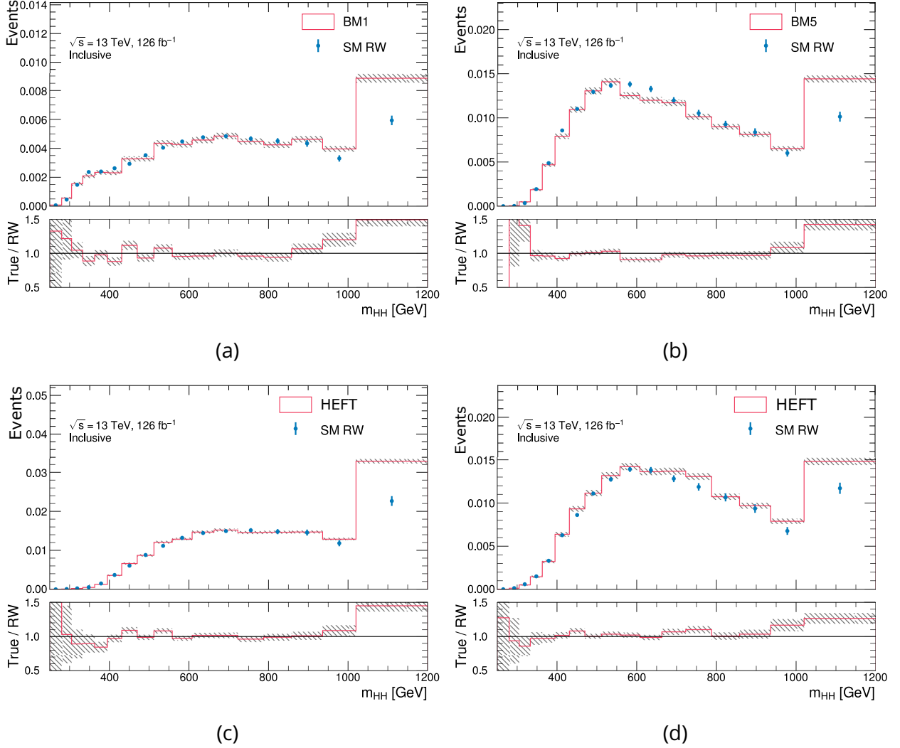
Figure 6.14: The simulated HEFT signal (red line) is compared to the SM sample reweighted to the examined variation (blue dots) in bins of m_{HH} . The HEFT variation shown are BM1 in (a), BM5 in (b), c_{gghh} = 0.5 in (c), and c_{tthh} = 0.5 in (d). Only the statistical error is shown. The overflow (last bin) and underflow (first bin) bins are shown for visualisation purposes (in the actual analysis they are merged into the highest m_{HH} bin) and an explanation for the discrepancy observed is offered in the text of the thesis.
