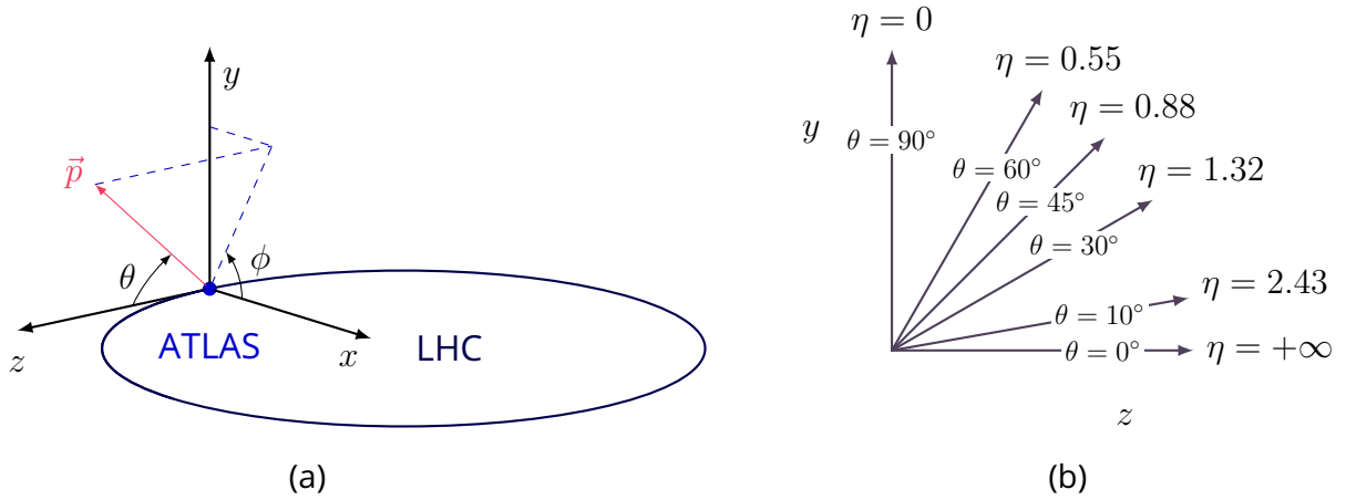
Figure 3.4: An illustration of the coordinate system used by ATLAS to describe the position of particles emerging from a proton-proton collision. The coordinate system as defined with respect to the LHC ring (black circle) for the ATLAS detector (blue dot) is depicted in (a). The momentum of a particle emerging from the proton-proton collision is shown as \vec{p} (dark pink vector). The relationship between \eta and \theta in the y - z plane is shown in (b). The graphics in (a) is adapted from [69] and the graphics in (b) from [70].
