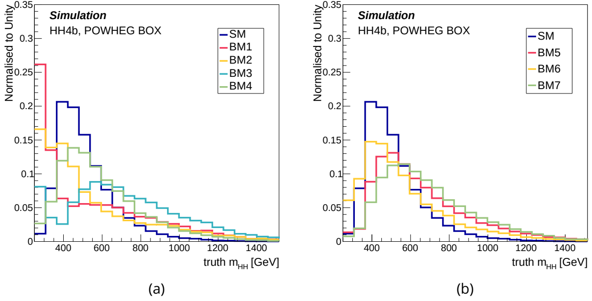
Figure 2.6: The truth m_{HH} distribution for the HEFT BMs considered as compared to the SM HH production are shown. PowhegBox has been used to produce the HH events.
