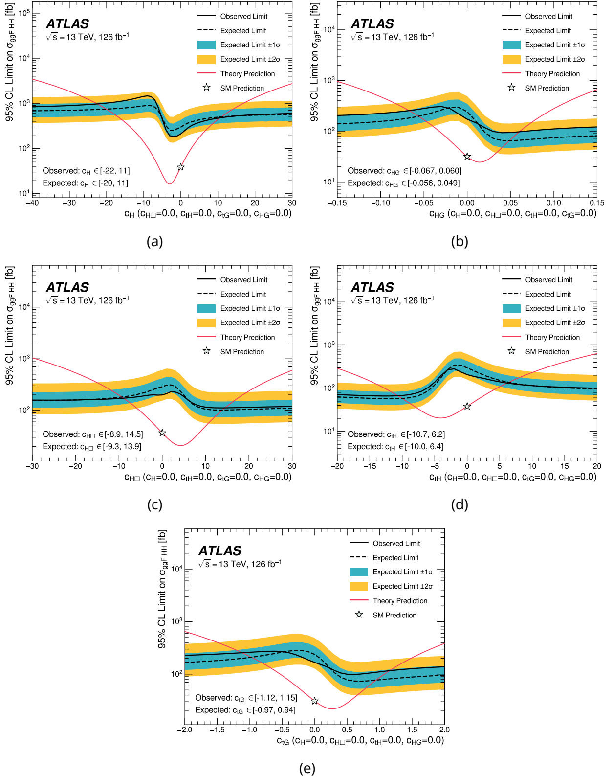
Figure 6.26: The 95% upper exclusion limits on c_H in (a), c_{HG} in (b), c_{H\Box} in (c), c_{tH} in (d), and c_{tG} in (e) are shown. The solid black line represents the observed limits, while the pink line illustrates the theoretical cross-section corresponding to each considered variation. The dashed black line shows the expected limits and the turquoise (yellow) bands are the corresponding 1\sigma ( 2\sigma ) error bounds. The SM point is located at zero. The figures have been published in [2].
