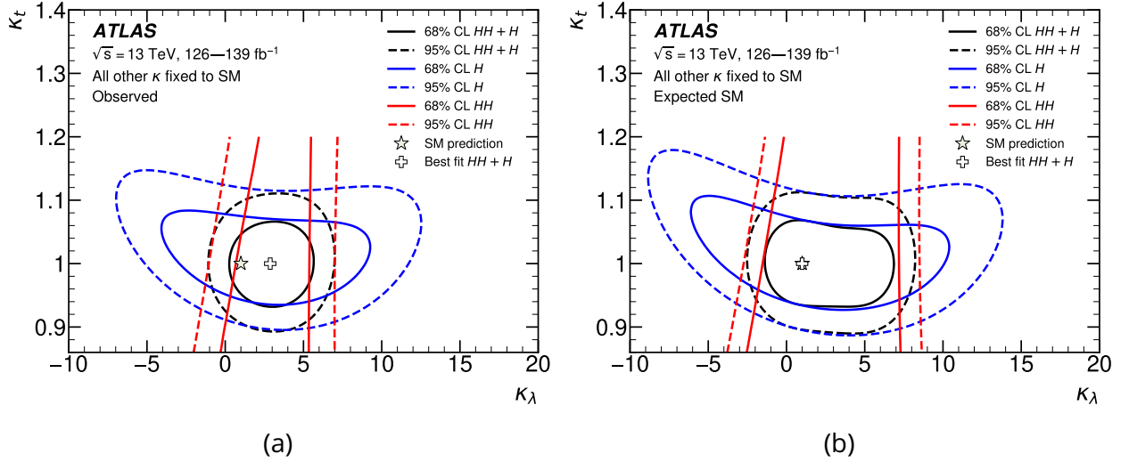
Figure 7.5: The solid (dashed) lines show the 68% (95%) CL contours in the \kappa_\lambda - \kappa_t plane, the other Higgs couplings are fixed to their SM value. The observed constraints are shown in 7.5a, while the expected limits are shown in 7.5b and have been published in [3]. In expected limits fit it is assumed the SM HH signal exists.
