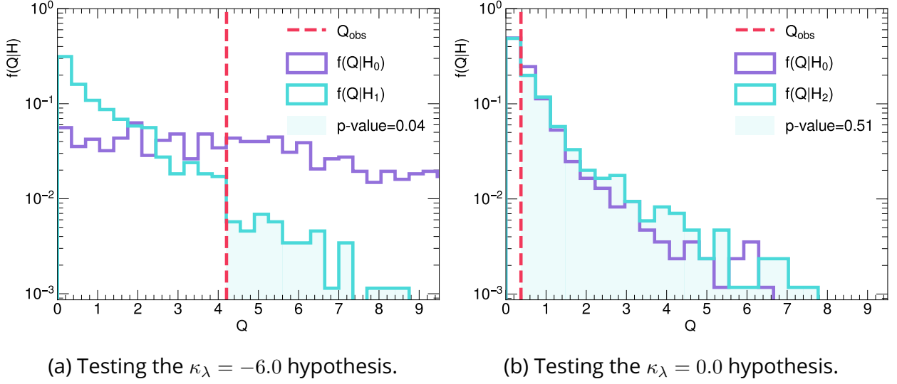
Figure 6.16: The computation of the p-value, assuming the \kappa_\lambda = -6 hypothesis ( H_1 ) in (a) and the \kappa_\lambda = 0 hypothesis ( H_2 ) in (b) given the expected dataset follows the SM hypothesis. The turquoise histogram is the distribution of the test statistic f(Q|H_1) ( f(Q|H_2) ), while the purple histogram is the distribution of the expected observed test statistic f(Q|H_0) . It should be noted that for simplicity the test statistic is denoted by Q in both plots but in fact Q = -2 \ln(\Lambda(\kappa_\lambda = -6)) in (a) and Q = -2 \ln(\Lambda(\kappa_\lambda = 0)) in (b). The expected observed test statistic is defined as the median of the sampled test statistic and marked as the pink dashed line on the plots. The shaded turquoise area is the p-value given the expected data generated assuming the SM case and testing the alternative hypothesis. Each of the plotted distributions is generated by sampling approximately 850 toy datasets ( m_{HH} distributions) from the PDF of the hypothesis considered. The background estimation and the \kappa_\lambda signal model as defined in the ggF channel of the HH \rightarrow b\bar{b}b\bar{b} analysis are used to define the PDF of a hypothesis. Only the statistical uncertainties and dominant uncertainties on the background estimation are accounted for. The same set of toy datasets is used to compute f(Q|H_0) in (a) and (b), while Q in f(Q|H_0) is distinct.
