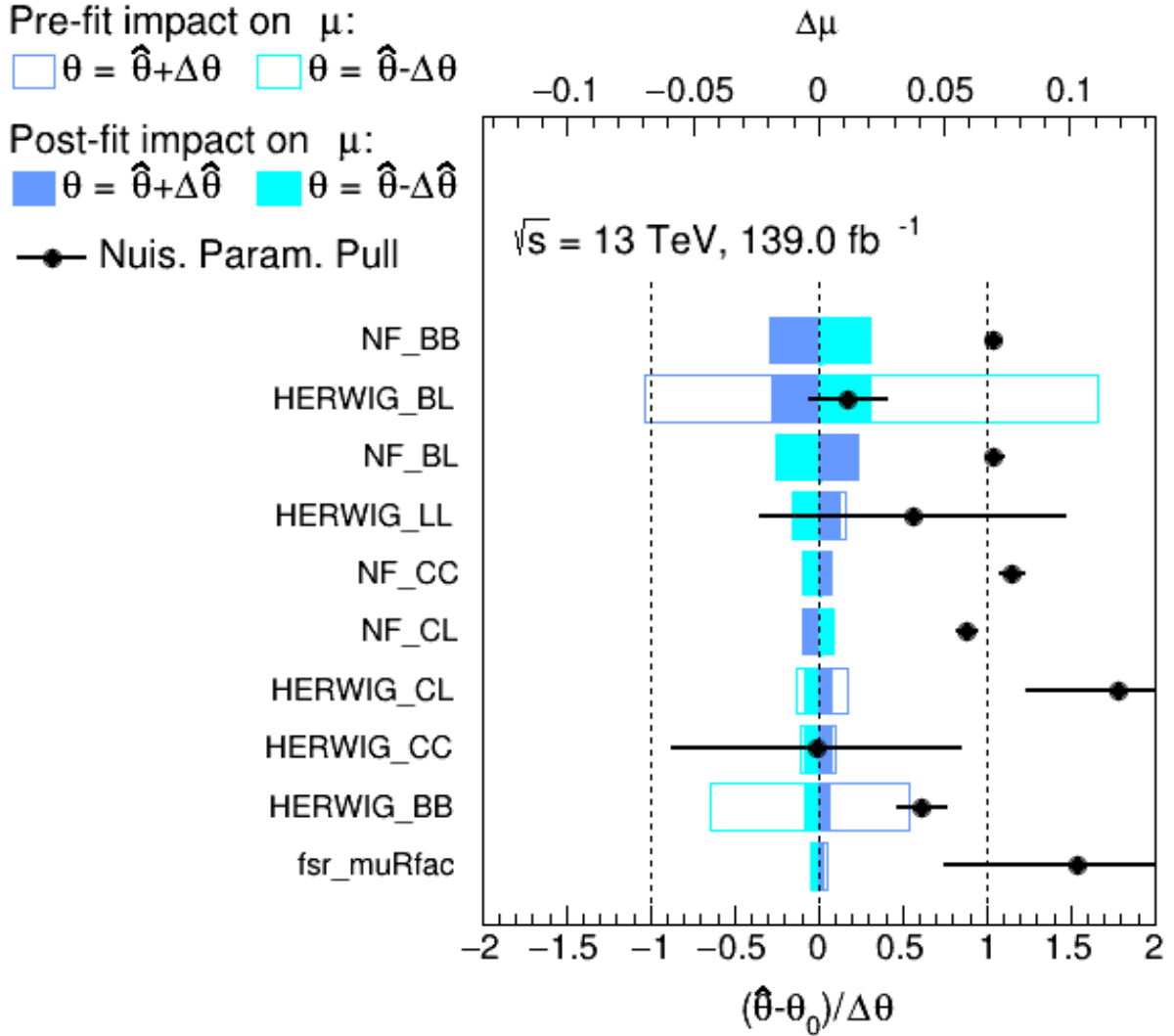
Figure 8.21: The ten highest-ranked nuisance parameters (NPs) found in the large-R jet bin 600 < p_T < 750 \text{ GeV} at 50% WP. The pulls (scale on the bottom x-axis) and the impacts on the SF (scale on the top x-axis) are shown. The normalisation factors ( NF_{flav} ) pre-fit value is one, while the other NPs have a pre-fit value of zero. The constraints observed on the parton shower and hadronisation uncertainty on the BB and BL templates (HERWIG_BB, HERWIG_BL) are expected from the Asimov fit. The source of the constraints is the pass region data, as the pass region consists of BB and to a lesser BL, while the non-B flavours contribute a negligible amount. Therefore, nearly all of the data statistics are used to constrain the BB and BL parton shower systematic uncertainty. As discussed in the text of this thesis some NPs, especially the final state factorisation scale (fsr_muRfac) and parton shower and hadronisation uncertainty on the CL template (HERWIG_CL), are pulled significantly as they correct the mis-modelling in the tails of the fail regions.
