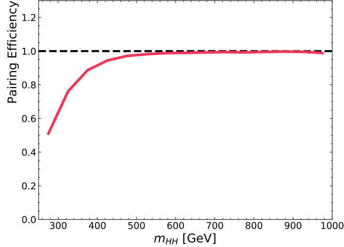
Figure 6.3: The efficiency of \min\Delta R as the mass of the diHiggs system for the ggF SM signal. The efficiency is evaluated on events that have two truth Higgs bosons and at least four central jets, no other event selection is applied.
