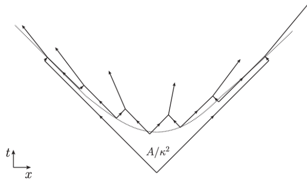
Figure 4.2: Illustration of the idea behind the Lund string taken from [89]. The light-like trajectory is the originally produced q\bar{q} parent. The breaking of the string and consequential hadron production is indicated by the trajectories along the hyperbola.
