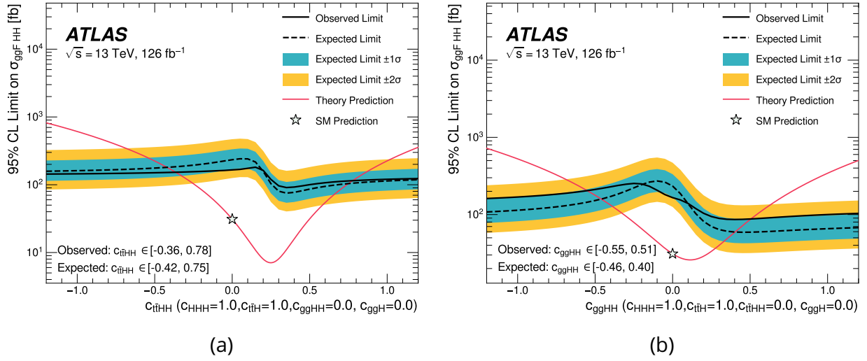
Figure 6.25: The observed 95% confidence level upper exclusion limits on the c_{t\bar{t}HH} in (a) and c_{ggHH} in (b) in the range [-1.2, 1.2] is shown by the black line. The red line indicates the theoretically predicted cross-section, if the observed limit is below the theoretical prediction the point is excluded with a confidence level of more than 95%. The star indicates the SM point, which is zero for both coefficients considered. Expected upper exclusion limits are shown as the dashed line with the 1\sigma ( 2\sigma ) error bound in turquoise (yellow). In each of the scans, only the considered coefficient is varied, while all other HEFT coefficients are fixed at their SM value. From these, the extracted observed (expected) upper exclusion limits are c_{t\bar{t}HH} \in [-0.36, 0.78] ( c_{t\bar{t}HH} \in [-0.42, 0.75] ) and c_{ggHH} \in [-0.55, 0.51] ( c_{ggHH} \in [-0.48, 0.40] ). The figures have been published in the auxiliary material of [2].
