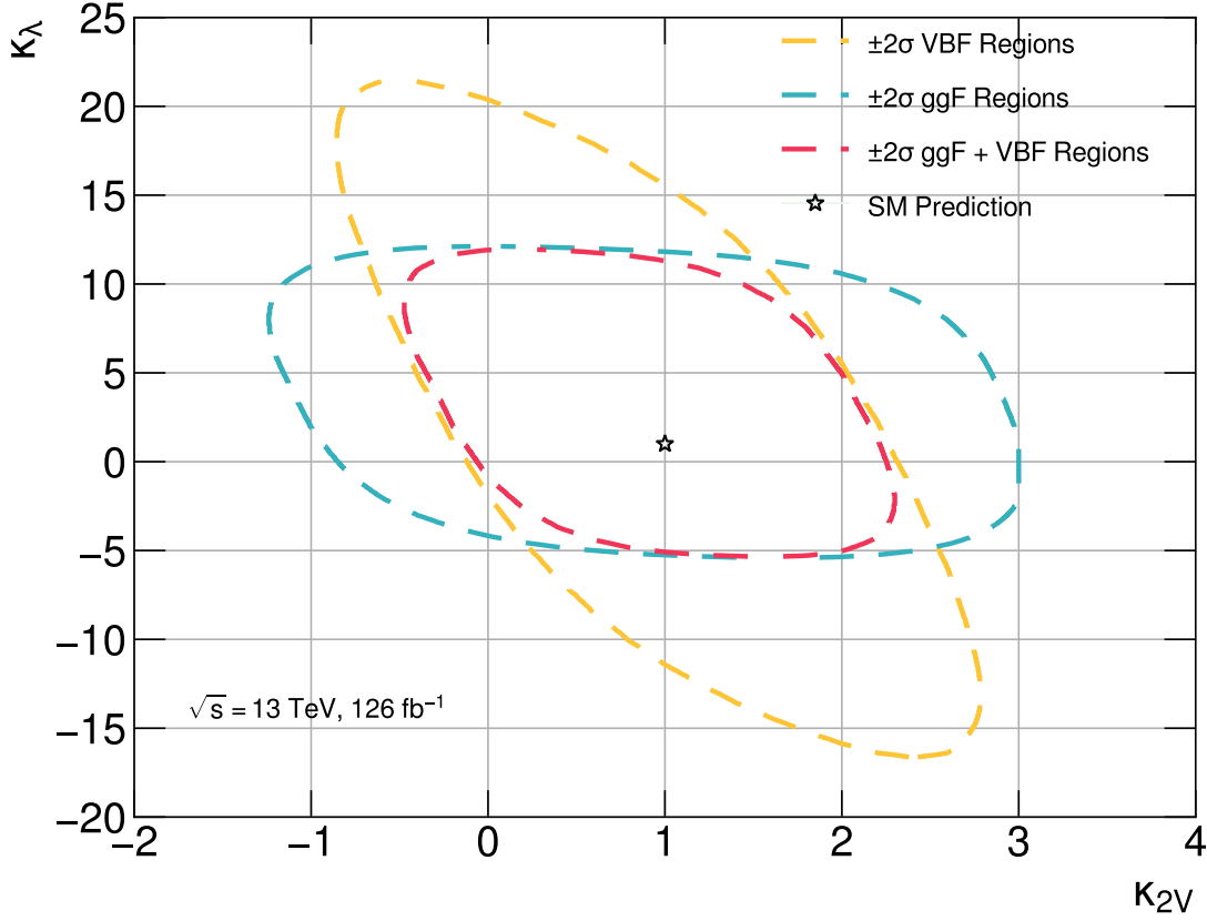
Figure 6.17: The expected 2\sigma confidence regions deduced from the HH \rightarrow b\bar{b}b\bar{b} ggF (turquoise), VBF (yellow), and combined ggF and VBF (dark pink) channels. The contour represents the \kappa = (\kappa_\lambda, \kappa_{2V}) values of constant -2 \ln \Lambda , where -2 \Delta \ln L = 6.18 as the bounded region has a 2\sigma coverage probability to capture the true (\kappa_\lambda, \kappa_{2V}) values. The sensitivity to \kappa_{2V} in the ggF channel comes from the VBF signal that leaks into the region, whose contribution can be significant as \kappa_{2V} varies (the \kappa_{2V} = 0 signal is expected to have a contribution of 23 events to the ggF signal region as evident from Table 6.3). The 2\sigma confidence regions are derived from the expected Asimov dataset and only the statistical and background uncertainties are considered.
