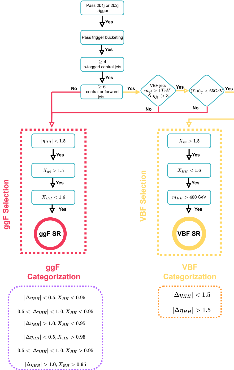
Figure 6.4: The summary of the event selection. The final categorisation in the ggF and VBF channels that increases the sensitivity to the SM signal is shown in the two dotted boxes.
