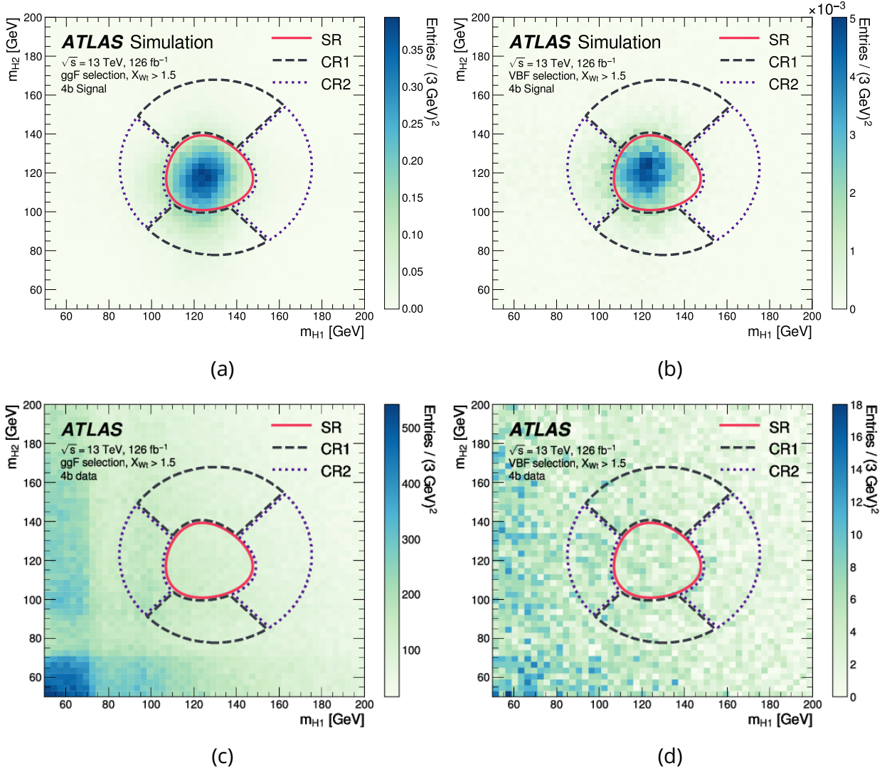
Figure 6.8: The upper subfigures show the non-resonant ggF (left) and VBF (right) SM signal with a clear peak in the SR and only a small leakage into the CR. The lower subfigures show the 4b data in the ggF (left) and VBF (right) channels. The effect of the X_{Wt} cut can be seen on the ggF 4b data, as stripes around m_{H1/H2} \sim 80 GeV. The plots have been published in the non-resonant HH \rightarrow b\bar{b}b\bar{b} paper [2].
