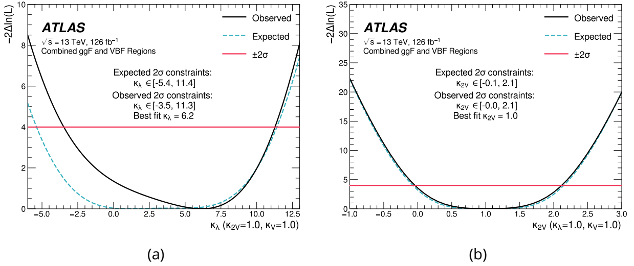
Figure 6.22: The -2\Delta\ln(L) with \kappa_\lambda in (a) and \kappa_{2V} in (b) as a POI are shown. The expected -2\Delta\ln(L) scans derived from an Asimov dataset (dashed line) assume the existence of an SM HH signal. In the fit, the ggF and VBF channels are combined and all \kappa but the POI are fixed to unity. The VBF HH signal is included in the ggF channels and vice versa. The signal strengths are fixed to their theoretical predictions and can be modified only through their systematic uncertainties. The observed (expected) \pm 2\sigma confidence levels are -3.5 < \kappa_\lambda < 11.3 ( -5.4 < \kappa_\lambda < 11.4 ) and -0.0 < \kappa_{2V} < 2.1 ( -0.1 < \kappa_{2V} < 2.1 ) as derived from the -2\Delta\ln(L) scans shown in (a) and (b) respectively. The best-fit value in the \kappa_\lambda -2\Delta\ln(L) scan is shifted away from the SM to \kappa_\lambda = 6.2 , as the data distribution at low m_{HH} has a slightly more prominent peak than the pre-fit background estimation. The results have been published in [2].
