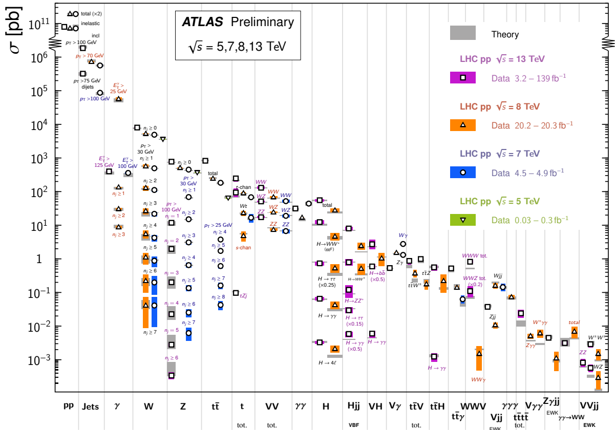
Figure 1.3: The total and fiducial production cross-section measurements of various SM processes at different center-of-mass energies are summarised. The measurements are based on the data collected by the ATLAS experiment and compared to the theoretical predictions of the SM, which are shown in grey. The figure is taken from [21].
