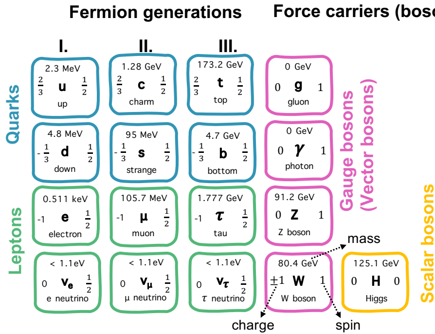
Figure 1.1: The particle content of the Standard Model is shown, each particle has its mass, electric charge, and spin indicated. The fermions are ordered into three generations, the only difference between generations is in the particle's mass which increases per generation.
