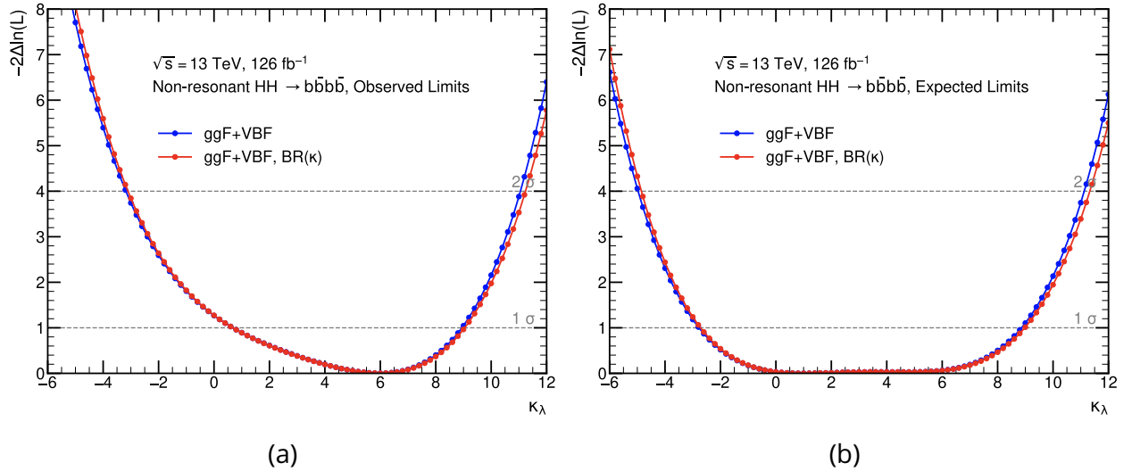
Figure 7.1: The observed (left) and expected (right) -2\ln\Lambda scans show the scenario that accounts for the NLO EW corrections (red line) and the one that ignores the effects (blue line) in HH \rightarrow b\bar{b}b\bar{b} . The POI is \kappa_\lambda , all other \kappa_m are fixed to unity.
