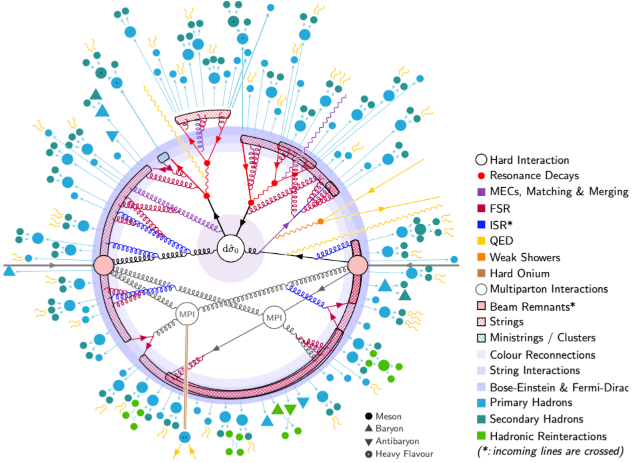
Figure 4.1: A simplified sketch of the structure of a pp \rightarrow t\bar{t} event, as simulated by Pythia. The colliding protons, light pink circles, contribute partons to the hard scatter (HS), the white circle labelled d\sigma_0 , and underlying events (UE), white circles labelled MPI. Before the HS or UE, the partons entering the interactions can emit initial state radiation, represented by dark blue lines. Similarly, the partons that emerge from the HS or UE can radiate, the final state radiation is indicated by purple lines. The t\bar{t} final state and its subsequent decays are represented by the red circles. The purple and hatched areas represent hadronisation, the formation of colour singlets. Primary hadrons are shown as blue-coloured shapes, while green-coloured shapes are the hadrons from subsequent decays, usually what is observed by the detector. The simplifications made are; there are fewer final-state hadrons, the recoil is depicted incorrectly, light-flavour hadrons are shown as stable and the incoming momentum is not accurately depicted [89]. The illustration is taken from [89].
