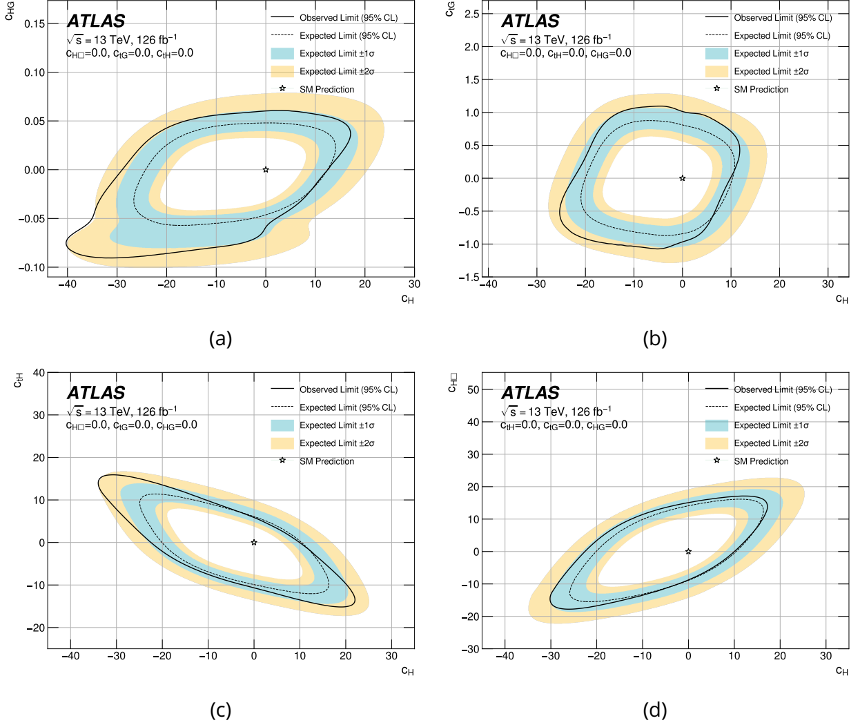
Figure 6.27: The observed (expected) contours that bound the allowed two-dimensional parameter space c_H - c_{HG} in (a), c_H - c_{tG} in (b), c_H - c_{tH} in (c), and c_H - c_{H\Box} in (d) at 95% confidence level are shown as a black solid (dashed) line. The 1\sigma ( 2\sigma ) error bounds on the expected contours are illustrated as turquoise (yellow) bands. The SM point is within the allowed parameter space in all cases considered. The two-dimensional contours have in published in [2].
