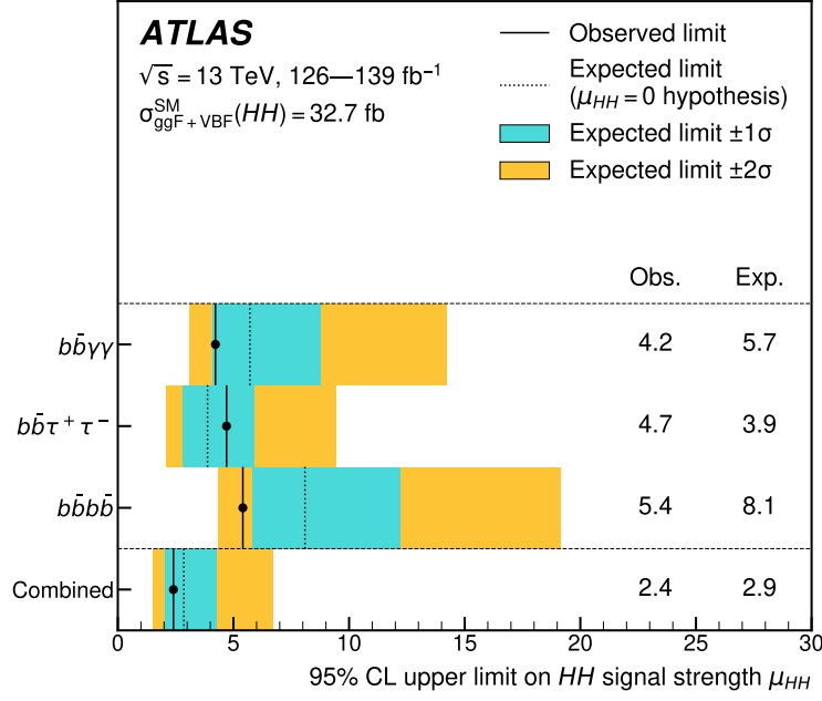
Figure 7.3: The diHiggs only combination includes the three diHiggs channels leading in sensitivity, b\bar{b}\gamma\gamma , b\bar{b}\tau^+\tau^- , and b\bar{b}b\bar{b} . The HH combination provides the latest 95% CL upper limits on the SM signal strength published by the ATLAS Collaboration, shown in the plot in addition to the upper limits in each channel. The extracted expected limits and corresponding error bands assume no HH production and take the NP values from the profiled fit to data. The results are published in [3].
