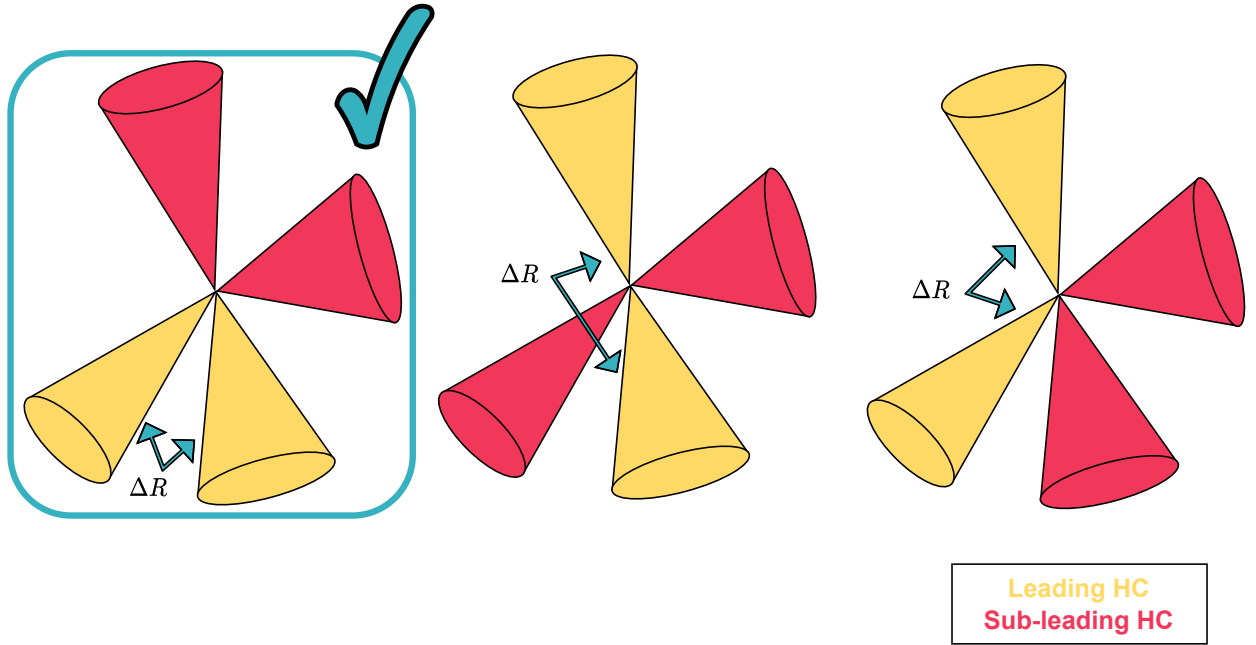
Figure 6.2: The sketched \min\Delta R pairing strategy. The correct pairing is circled and indicated by a tick. The leading HC jets are shown in yellow and the sub-leading HC jets are shown in pink. Only the \Delta R between the jets in the leading HC is considered in the pairing strategy.
