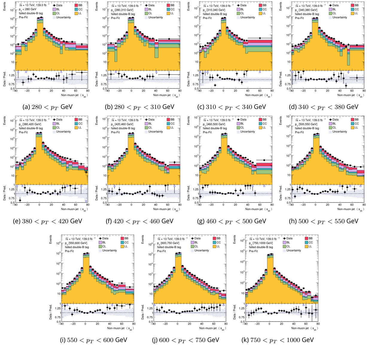
Figure C.3: The \langle s_{d0} \rangle distribution in the fail region of the non-muon-jet in different large-R jet p_T bins for the 50% WP.
