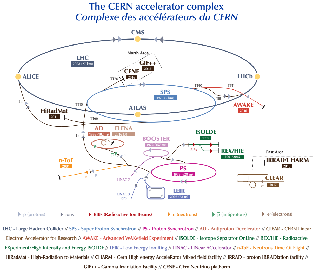
Figure 3.1: The LHC complex during Run2 is shown. The acceleration chain of the LHC consists of the Linac2, Proton Synchrotron Booster (PSB), Proton Synchrotron (PS), and Super Proton Synchrotron (SPS). The accelerated proton beams at an energy of 450 GeV are injected into the LHC from the SPS (line T18). The proton-proton beams are crossed to collide at four interaction points marked on the plot as yellow circles. At each interaction point, one of the four LHC experiments is placed, ATLAS, CMS, LHCb, or ALICE. The Figure is taken from [59].
