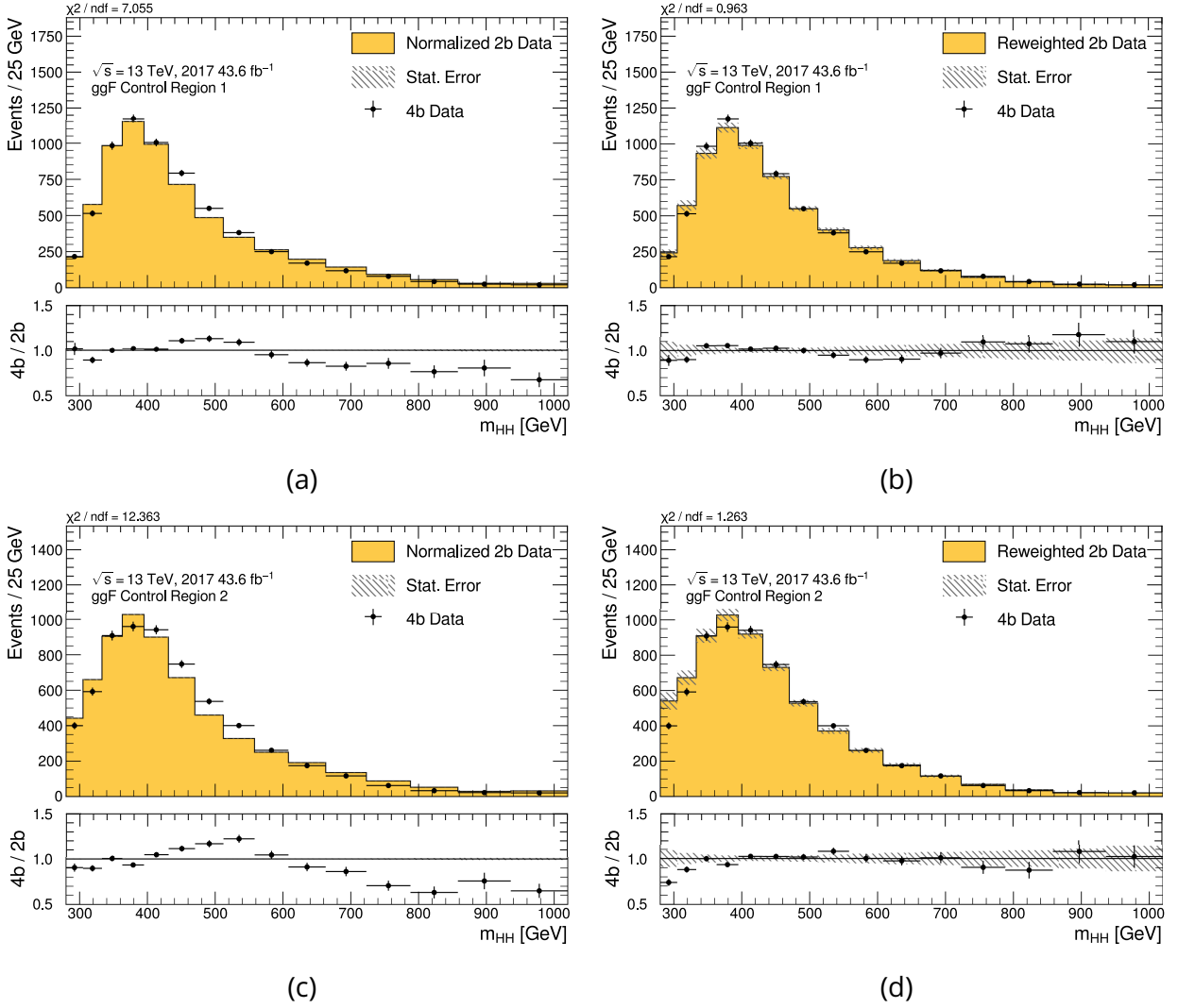
Figure 6.11: The 2b data normalised (left) and reweighted (right) plot compared to the 4b data. Clearly the reweighting outperforms the normalisation, despite m_{HH} not being used in the training. The upper two plots show CR1, while the lower two plots show CR2. The 2b distributions in (b) and (d) have weights derived from CR1 and CR2 respectively. The Poisson error from 2b data and the bootstrapping uncertainty are included in the statistical error on reweighted 2b data.
