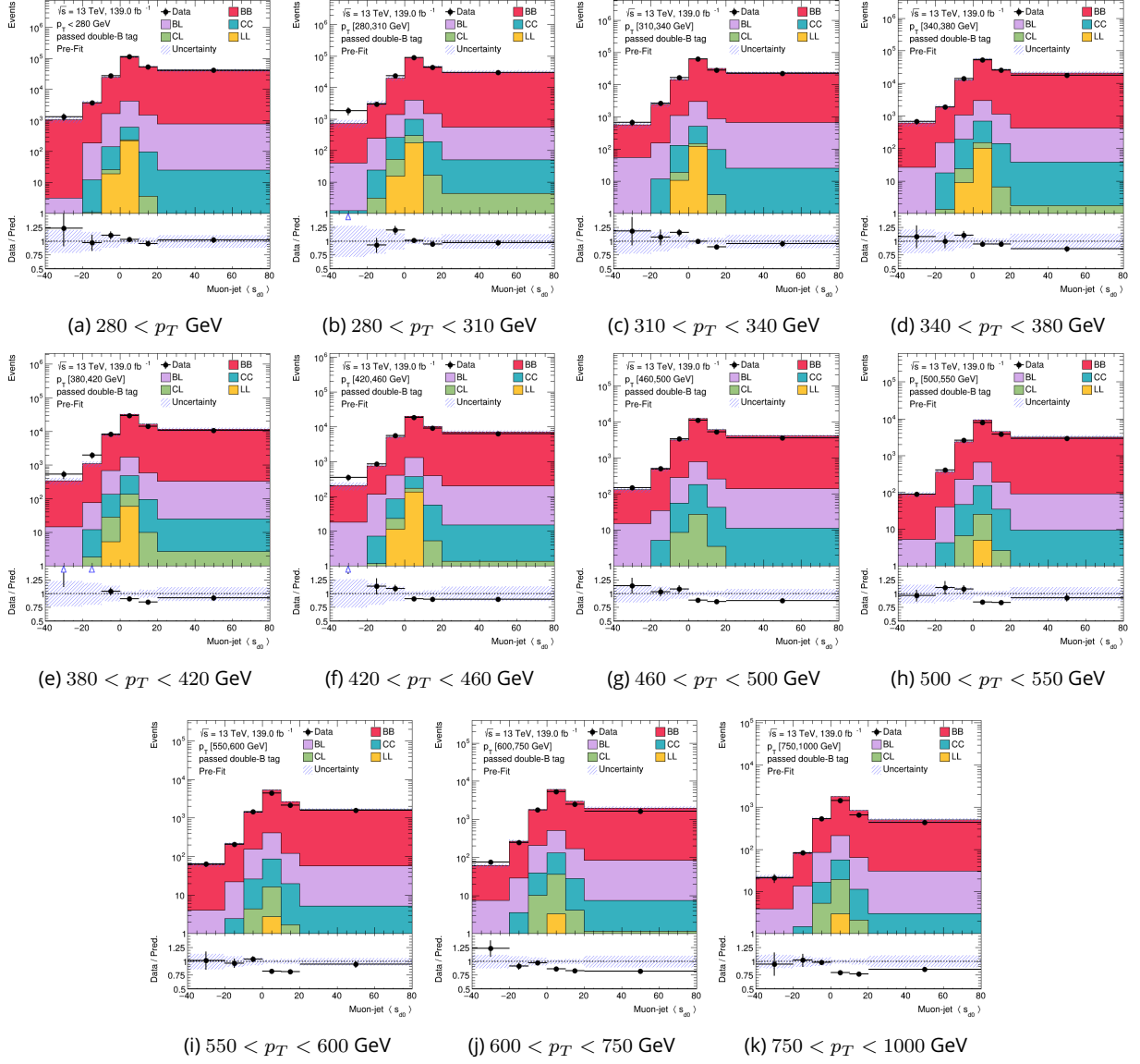
Figure C.1: The \langle s_{d0} \rangle distribution in the pass region of the muon jet in in different large-R jet p_T bins for the 50% WP.
