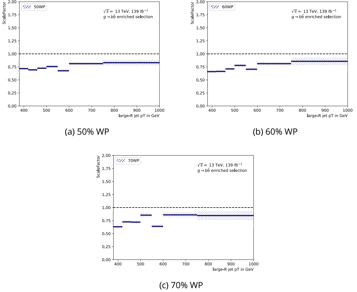
Figure 8.17: The Scale Factors derived in bins of large-R jet p_T for the 50%, 60%, and 70% WPs. The flavour fractions are corrected by fitting SV mass flavour templates in the fails and pass regions of the muon and non-muon jets. The hatched region represents the total uncertainty on the derived SFs.
