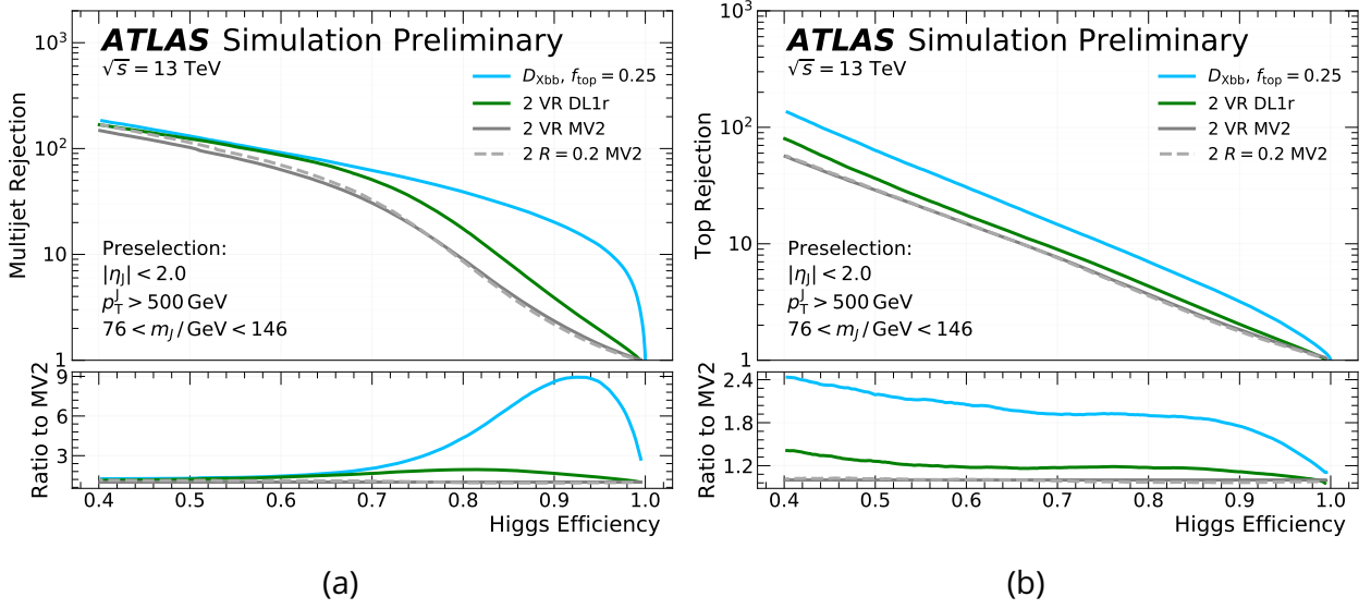
Figure 8.2: The multijet rejection in (a) and top rejection in (b) are shown as functions of the Higgs identification efficiency. All jets are required to have a p_T > 500 GeV to capture the performance in the boosted regime better. The figure is taken from [193].
