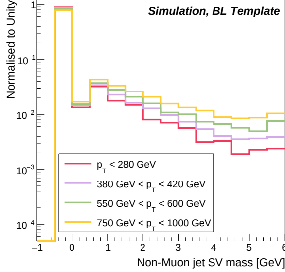
Figure 8.13: The large-R jet p_T dependence of the BL template shape. Only a few p_T bins are plotted for clarity.
