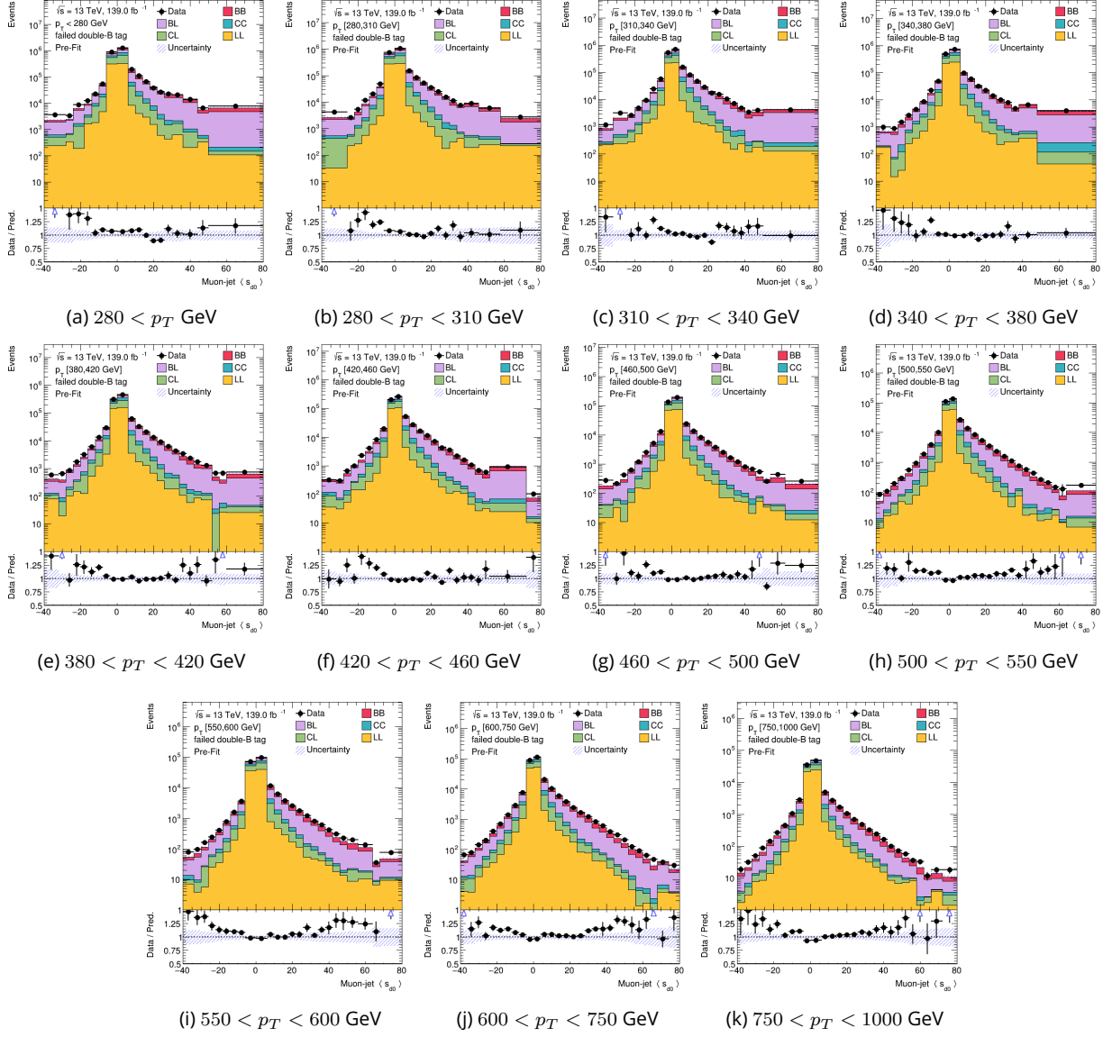
Figure C.2: The \langle s_{d0} \rangle distribution in the fail region of the muon jet in in different large-R jet p_T bins for the 50% WP.
