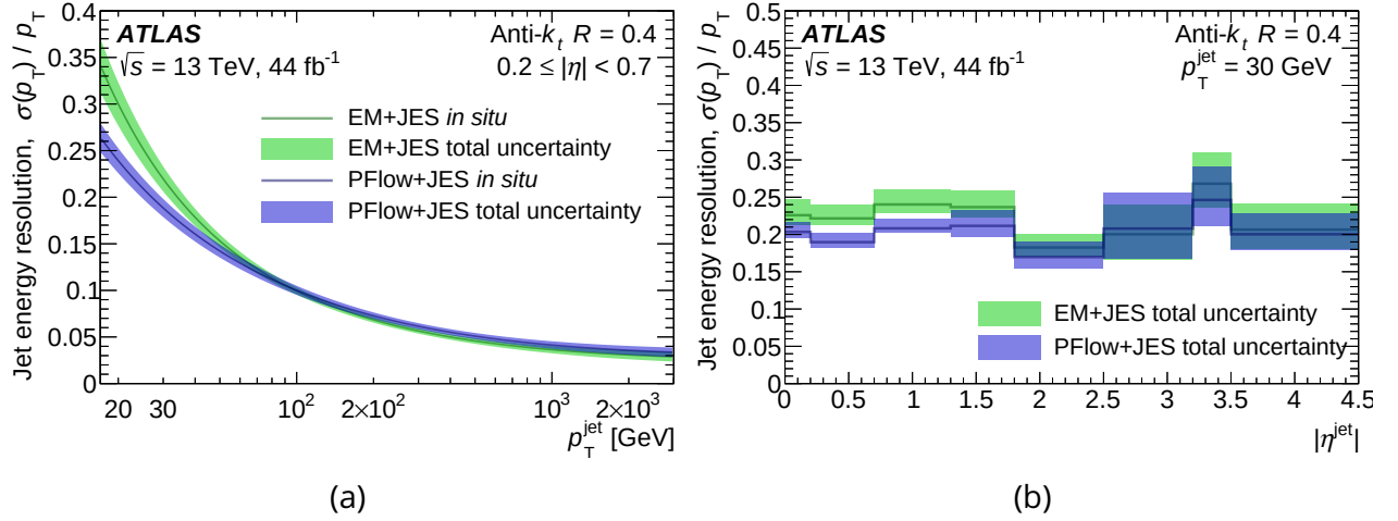
Figure 5.2: The relative jet energy resolution is compared between PFlow (blue line) and EMTopo (green line) jets. All jets have been clustered with the anti- k_T algorithm setting R = 0.4 and are fully calibrated. The energy resolution is plotted as a function of p_T in (a) and \eta in (b). The figure is taken from [80].
