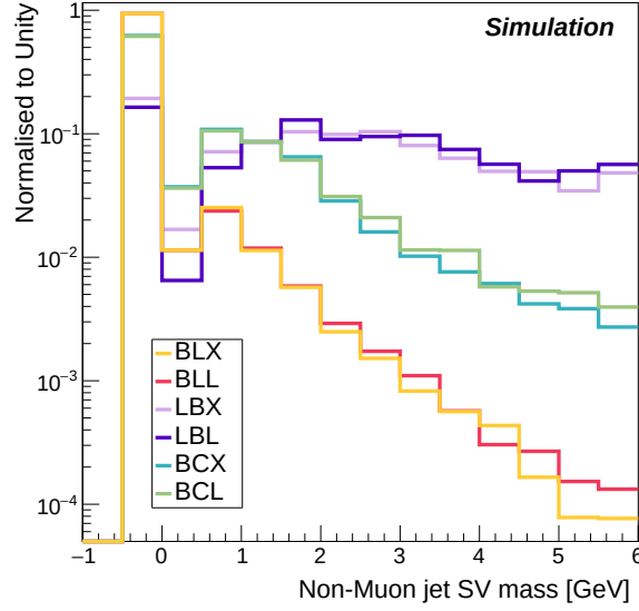
Figure 8.7: A selection of templates that are merged into the non-muon jet BL template. The second letter on each label indicates the truth flavour of the non-muon jet. Only a few large-R jet flavour compositions that are merged into the BL category are plotted for clarity.
