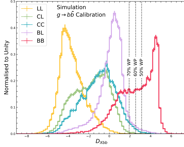
Figure 8.3: The D_{Xbb} distributions in dijet MC of the five flavour categories. The three dotted vertical lines indicate the cuts applied when the 70%, 60% and 50% WP are chosen for double-b tagging. The events on the right of the vertical line are said to be double-b tagged at the 70%, 60% or 50% WP (depending on the cut considered).
