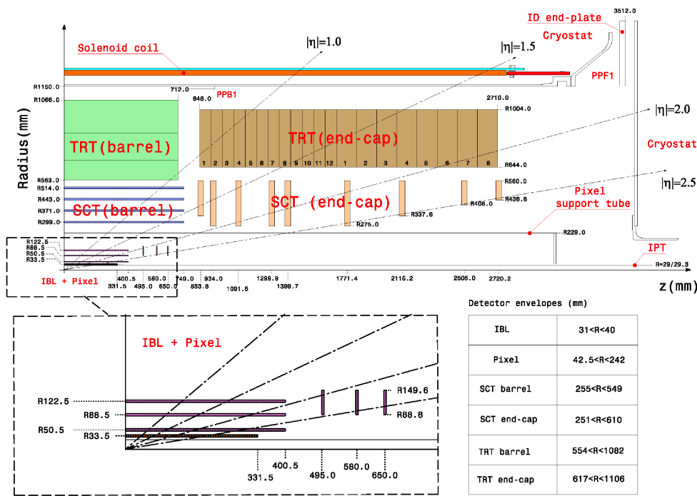
Figure 3.6: The precise layout of the Inner Detector also shows the inner positioning tube (IPT), mechanical support structures, and solenoid coils. The graphic is taken from [74].
