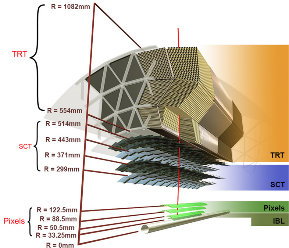
Figure 3.5: The cutout of the Inner Detector, each subdetector and its distance from the beam axis is indicated. The figure is taken from [73].
