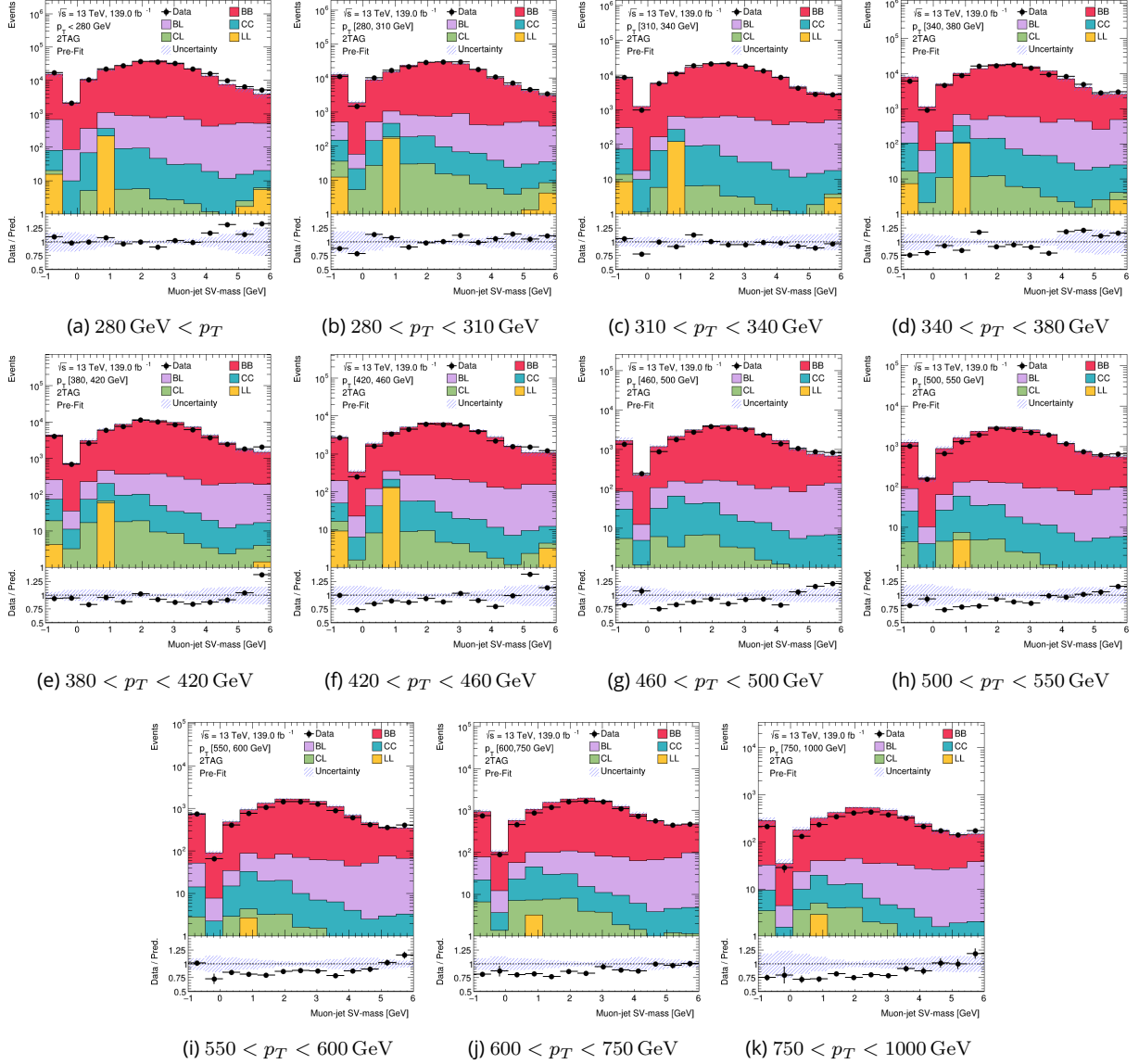
Figure 8.8: The pre-fit SV mass distribution in the pass region of the muon jet in different large-R jet p_T bins for the 50% WP.
