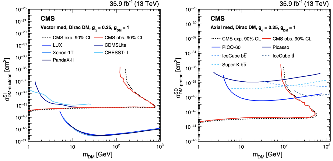
Figure 1.13: DM-nucleon interaction limits set by CMS with mon-X searches [71].
