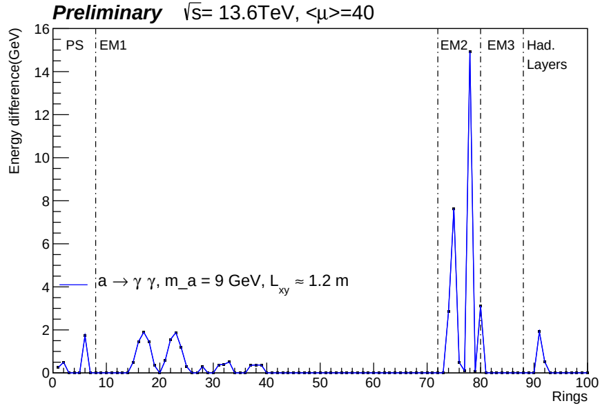
Figure 5.25: Absolute energy differences in Ring profiles. The x-axis represents the rings index according to table 5.1 as explained in section 5.4.2
