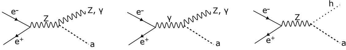
Figure 4.1: Tree level diagrams contribution to the production of ALPs + X at e^+e^- colliders.
