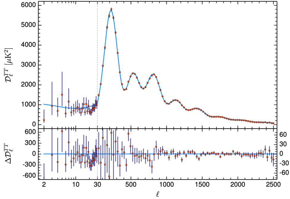
Figure 1.4: The temperature power spectrum of the CMB, with data points fitted by the \Lambda CDM model. From Planck 2018 results [3].
