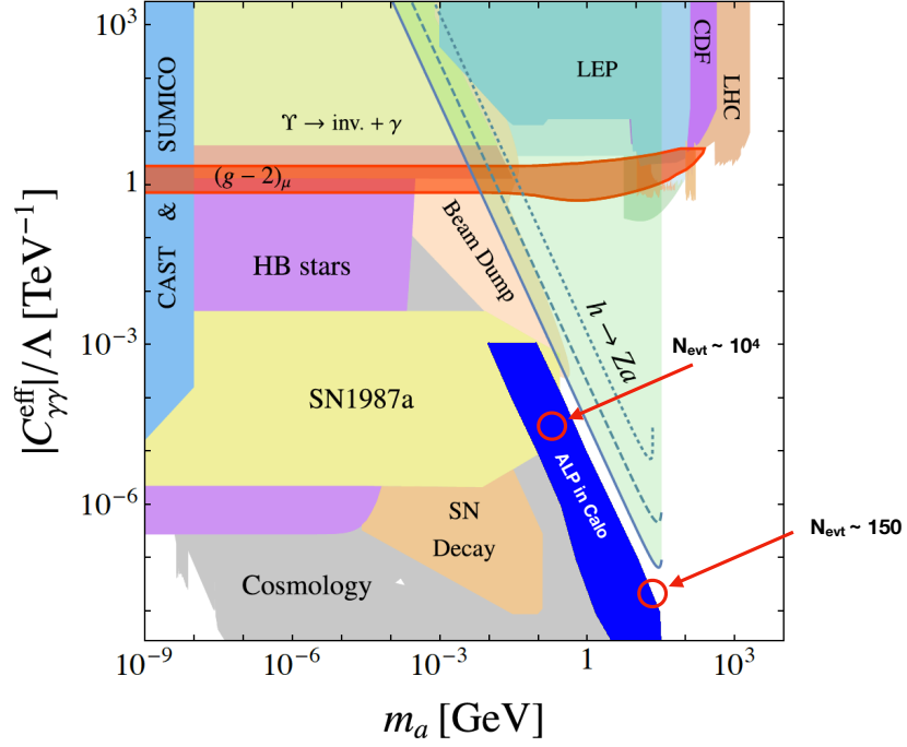
Figure 4.17: Resulting parameter space potentially leading to a discovery of LL-ALPs, decaying in calorimeters, in run 3 with a realistic f_a cut. The arrows show several events for run3 at the limit (minimum) and center (maximum) of the region of interest for in-calorimeter decays. Adapted from [79].
