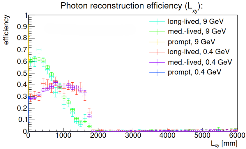
Figure 4.5: Photon reconstruction efficiency of ALP decay products for 2 mass points (0.4, 9) GeV and 3 life-times (prompt, medium, long) - samples described in 4.5. Note that the two masses are above and below the merged threshold (2 GeV) of prompt ALPs. The L_{xy} axis is the distance traveled by the ALP in the x-y plane. The reconstruction efficiency is computed by truth-matching the reconstructed loose photons to the truth-simulated particles.
