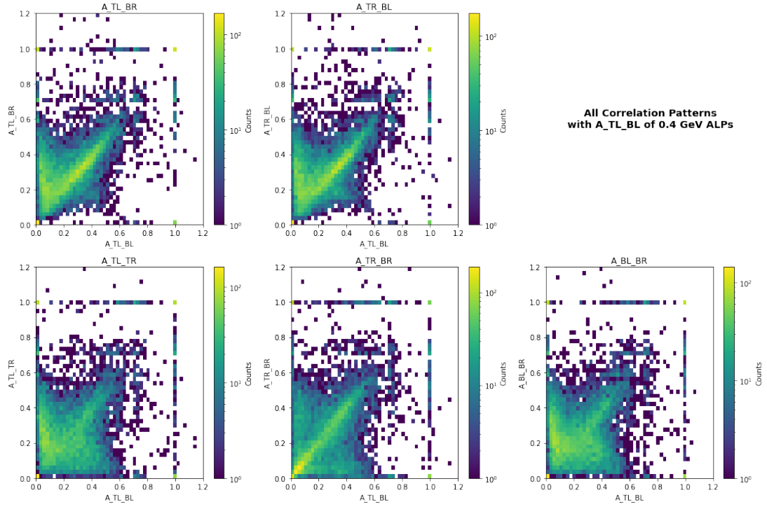
Figure 5.30: 2D histograms of correlations of the asymmetry axis TL-BL with the 5 other axes. Computed for 0.4 GeV ALPs with the medium lifetime (see 4.5). The different shapes of correlation reflect the two-body structure of the energy deposit.
