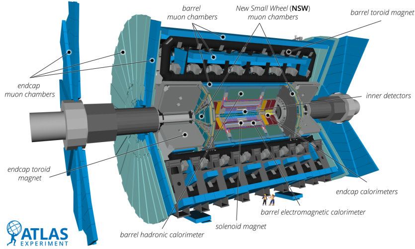
Figure 2.3: Schematics representation of ATLAS, each main sub-system is labeled [102]. The diameter of the detector is about 25 meters.
