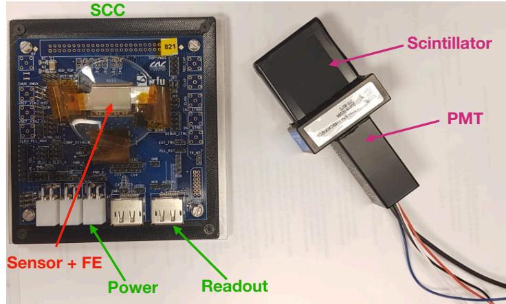
Figure 3.7: A picture of an SCC hosting a hybrid module wire-bonded to the chip next to a standard small crystal scintillator and photomultiplier tube assembly.
