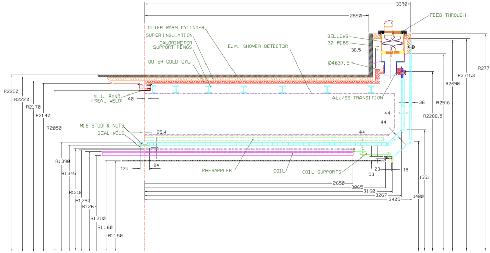
Figure 4.11: Side view of the LAr calorimeter. Relevant distances in the R axis are illustrated as depicted in the LAr calorimeter technical design report [112].
