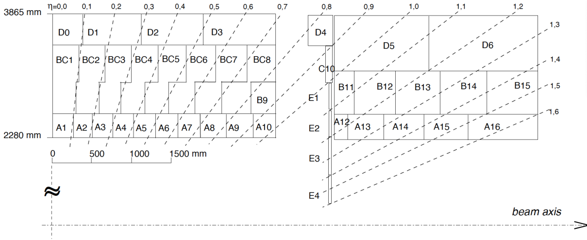
Figure 4.13: ATLAS TileCal segmentation in \eta . The left side is the barrel, and the extended barrel is on the right side. From the ATLAS experiment paper [100].
