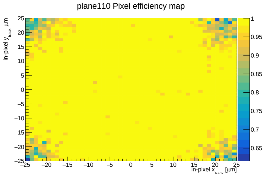
Figure 3.19: A 2D histogram of in-pixels average efficiency. The x and y coordinates are local.
