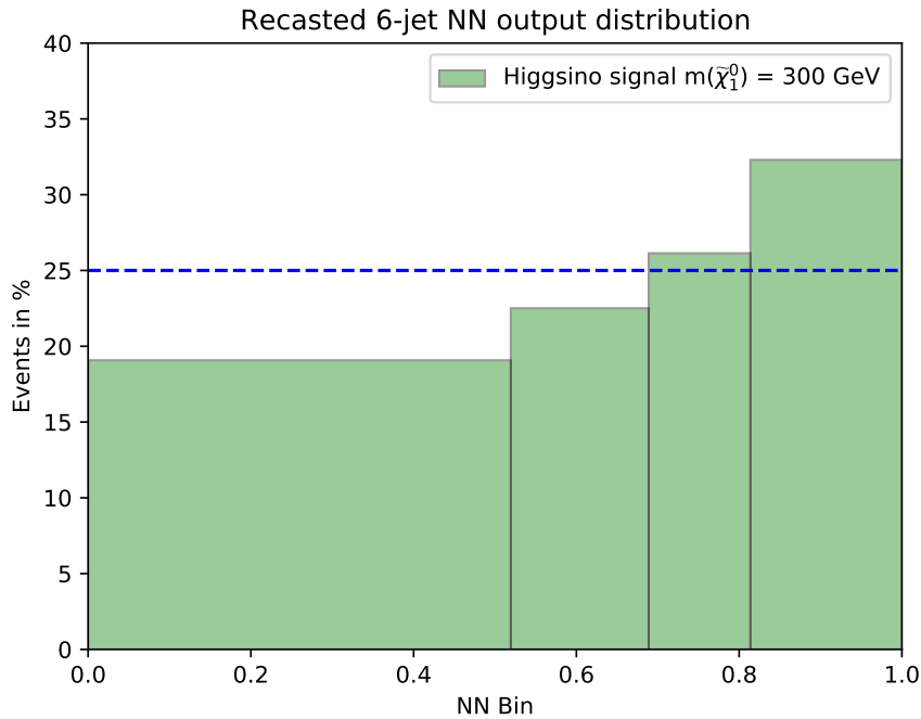
Figure 6.6: A reproduction of figure 6.4. The horizontal blue line represents the target of 25%. Each bin should contain an equal percentage of the higgsino signal population. The bins are : [0.0, 0.52, 0.69, 0.81, 1.0]
