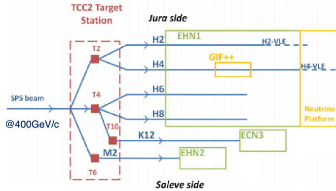
Figure 3.9: Target station TCC2 in the North Area.
