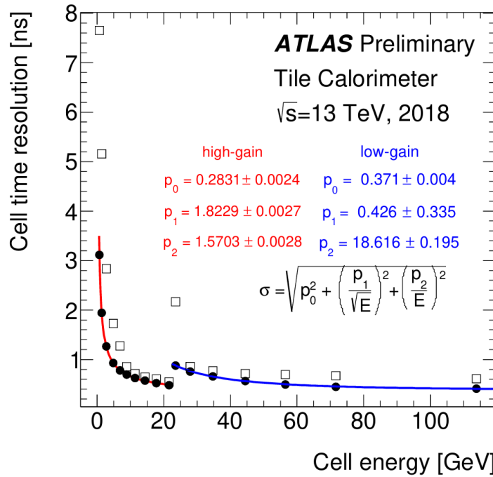
Figure 2.9: Timing resolution of a single cell of the Tile calorimeter [118] with respect to the deposited energy.
