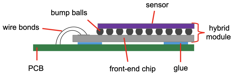
Figure 3.2: Crossectional view of an assembled module consisting of a hybrid module glued and wire bonded to the PCB.
