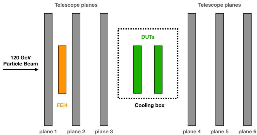
Figure 3.11: Scheme of the test bench. Six planes are used in the telescope to build tracks, an FEi4 detector is used for timing, and the DUTs are kept at a controlled temperature inside a cooling box. The total size of the bench is around 1.1 meters along the beam axis.
