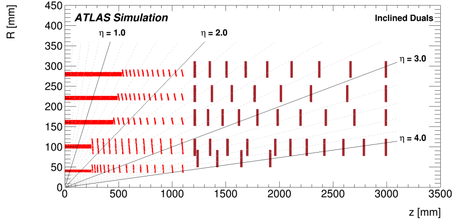
Figure 2.14: Inner part of the ITk detector. It is only composed of pixel modules. Barrel layers L0-L4 are shown in red, and all end-cap rings are darker. The position of inclined pixels is visible.
