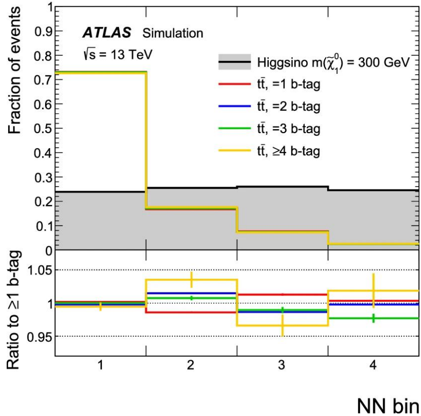
Figure 6.4: From [206]. Distribution of the NN output used for 6 jets events Higgsino signal is set with a neutralino mass of 300 GeV. Background events with diverse b-jet multiplicities peak at low values. Bins are chosen to artificially flatten the distribution.
