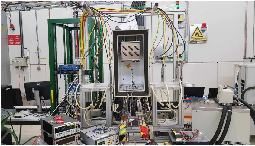
Figure 3.13: Picture of the test bench with an open cooling box. A single DUT is installed. The chiller tank and the tubes conducting the silicon oil are visible on the bottom right. Taken at PS test-beam facilities CERN
