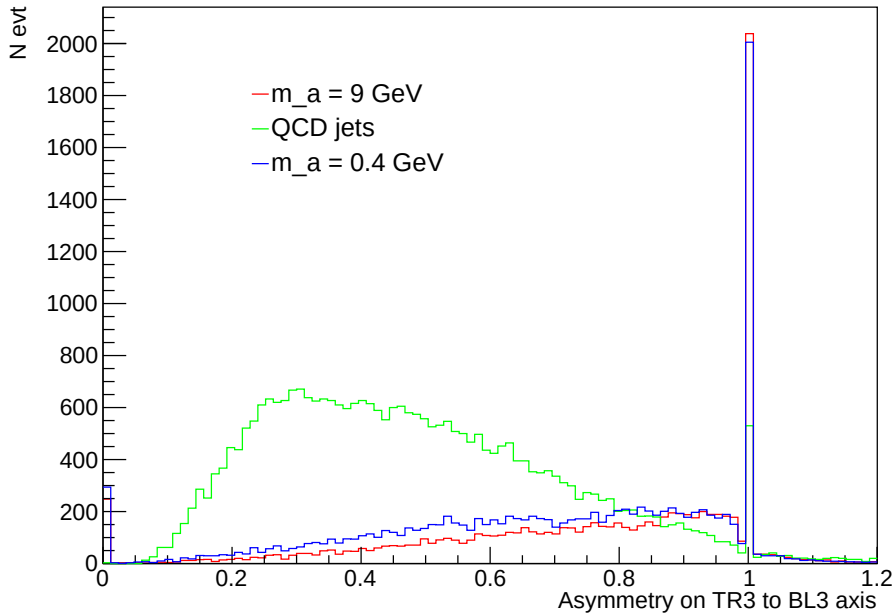
Figure 5.27: Asymmetry distribution between QCD jets and ALPs
