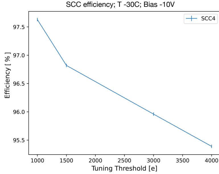
Figure 3.23: Threshold parameter scan of an SCC and impact on detection efficiency.
