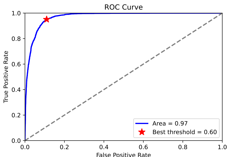
Figure 5.33: The ROC curve of the MLP classifier using asymmetry inputs. The dashed line illustrates the random guess performance. The best threshold is computed by maximizing the difference between signal and background efficiencies.
