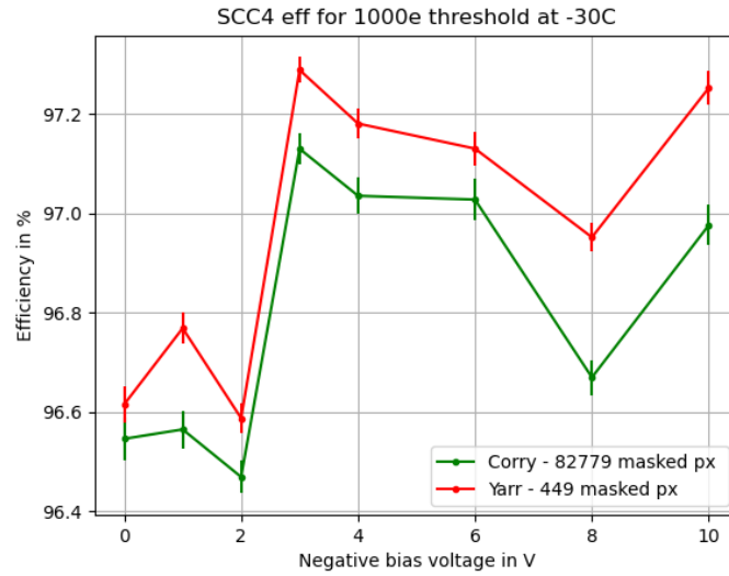
Figure 3.22: Efficiency of a SCC at different voltages using both masking techniques
