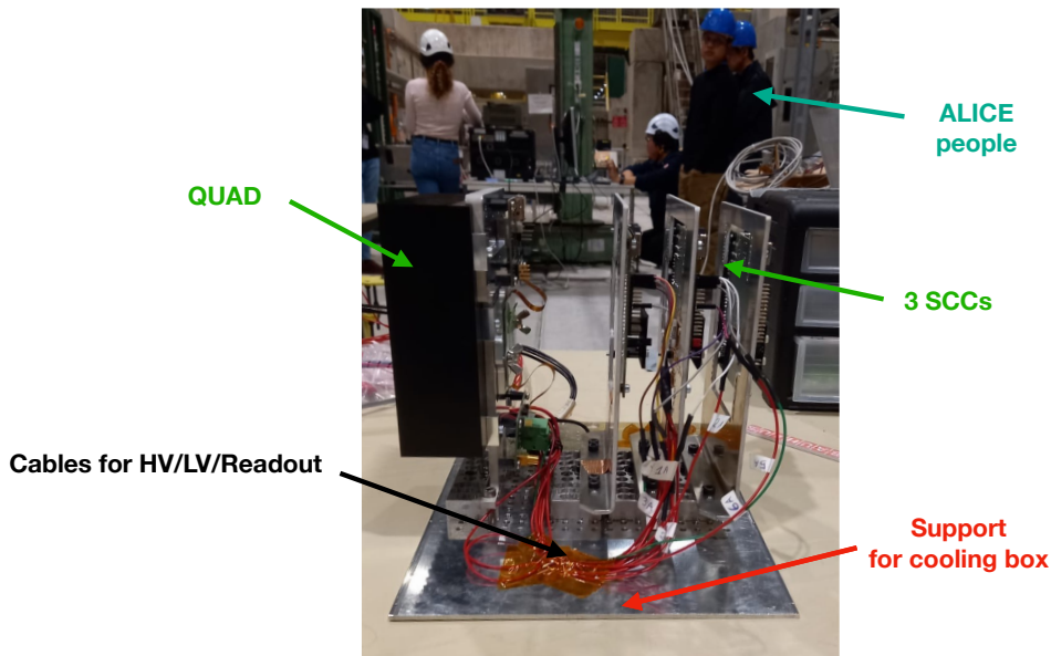
Figure 3.12: Picture of DUTs mounted onto support before insertion inside the cold box. Additional probes would be taped on the support surface for environment monitoring.
