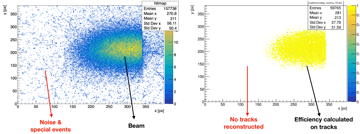
Figure 3.18: Left: Raw hitmap off all pixels on the sensor plane. Right: the associated chip efficiency map. A clear difference between the beam-induced signal and the background is visible on the reconstructed track region on the right figure. These results are obtained on an RD53B SCC.
