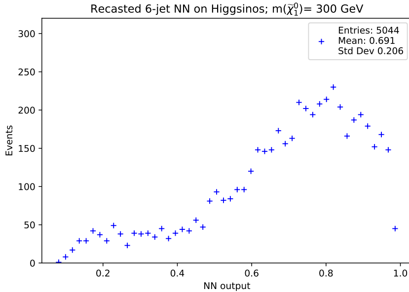
Figure 6.7: NN output for the 6 jet slice. Binned from 0 to 1 with 50 bins. Obtained in Madanalysis5.
