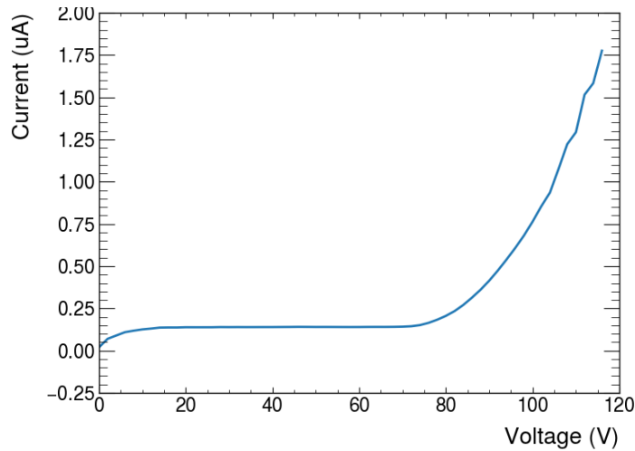
Figure 3.3: An IV curve of a planar module's sensor taken at room temperature. The breakdown point is visible at 80V, which means the depletion zone is already fully depleted prior and further increase in voltage is not necessary for particle detection as it only causes the current to jump.
