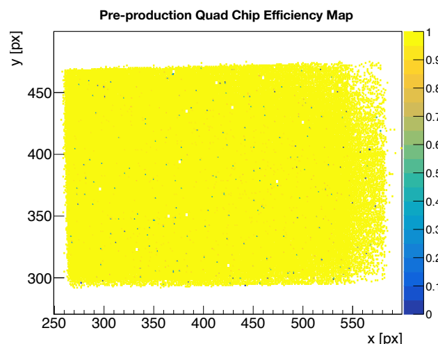
Figure 3.21: The chip efficiency map of the pre-production Quad module.
