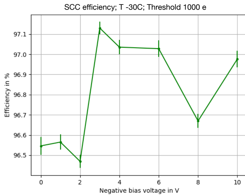
Figure 3.24: Bias voltage parameter scan of an SCC and impact on detection efficiency.
