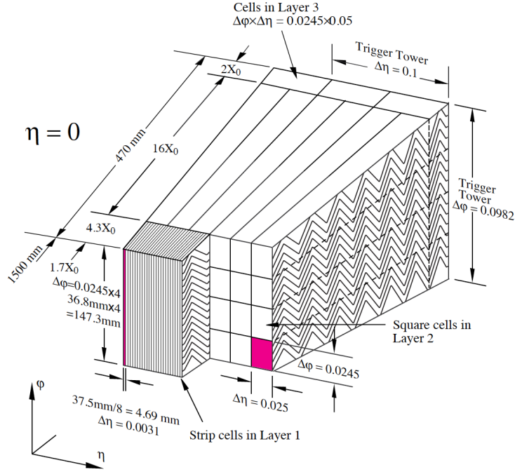
Figure 2.7: A module of the EM calorimeter displaying each layer depth. From the ATLAS experiment paper [100].
