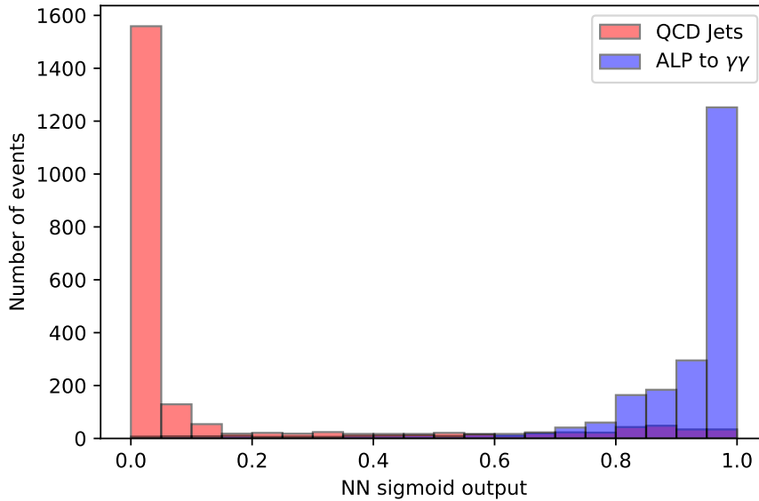
Figure 5.32: MLP classifier output distribution of ALP and QCD jet events. A clear and important separation between the two classes is visible. The raw output is processed in a sigmoid function to represent the prediction.
