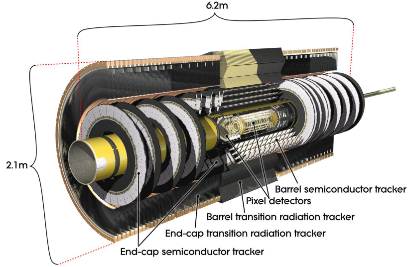
Figure 2.4: Schematics of the inner detector, each sub-system is labeled [103]. The maximum detector dimensions in the transverse plane and beam axis are written.
