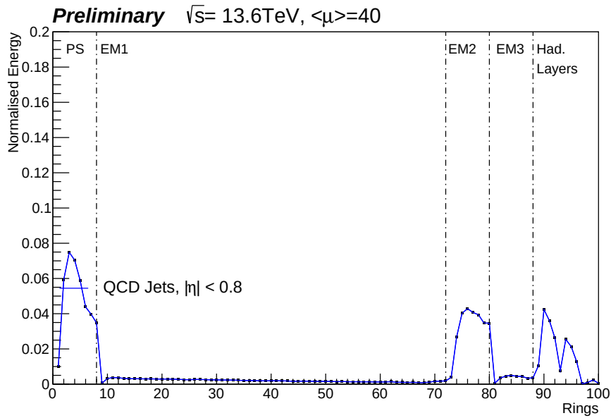
Figure 5.10: Average ring profiles of QCD jets created at the collision point. The x-axis represents the rings index according to table 5.1 as explained in section 5.4.2
