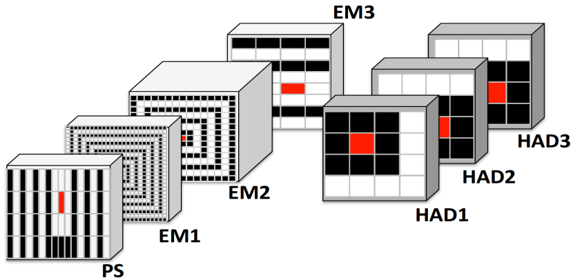
Figure 5.4: Sketch of Calorings longitudinal structure in multiple layers around a given region of interest (ROI) window. The change in granularity impacts heavily the number of rings.
