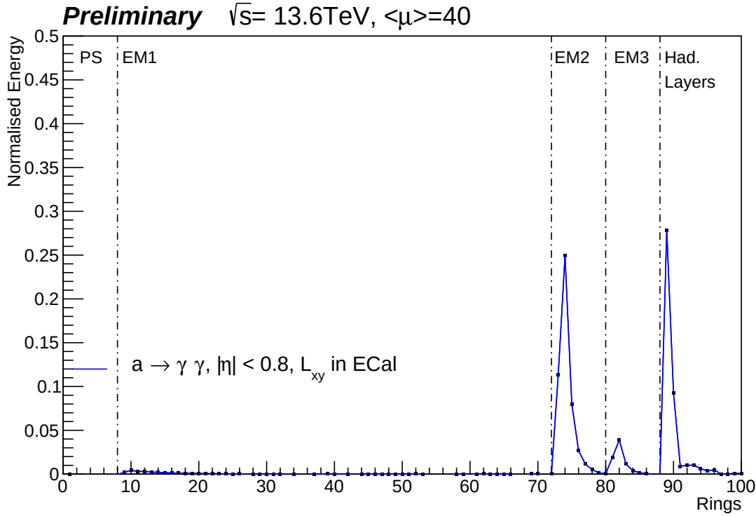
Figure 5.14: Average ring energy profile for 0.4 GeV ALP EM-calorimeter decays into two photons. The x-axis represents the rings index according to table 5.1 as explained in section 5.4.2
