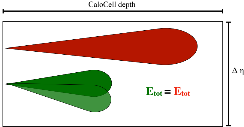
Figure 4.10: Illustration of how same energy single-photon and photon pairs are absorbed with different depths in an EM Calorimeter cell. The depth is in the R axis, perpendicular to \vec{z} .
