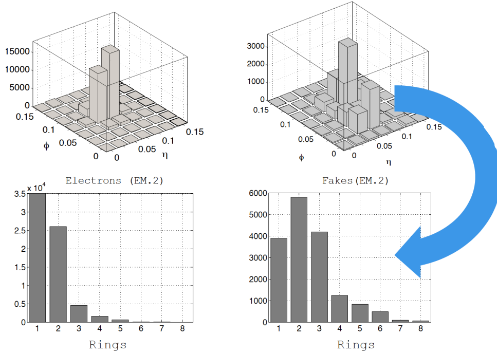
Figure 5.7: Differences in ring profiles for electrons and fakes.
