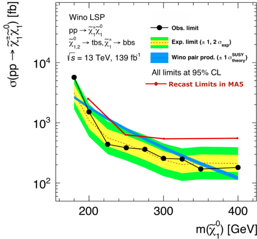
Figure 6.8: Resulting cross-section limits obtained with the recasting script. Overlapped with the ATLAS measurement exclusion plot [206]. Limits computed on simulated events of the RPV wino LSP model.
