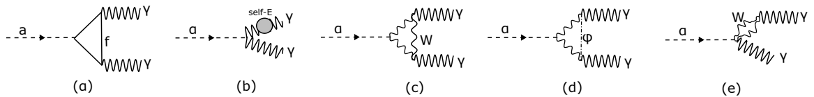
Figure 4.3: Diagrams contributing to the decay a \rightarrow \gamma\gamma . Fermion loops are considered (a), as well as internal charged W bosons (c,e) and associated Goldstone fields (d). (b) introduces the self-energy coupling.
