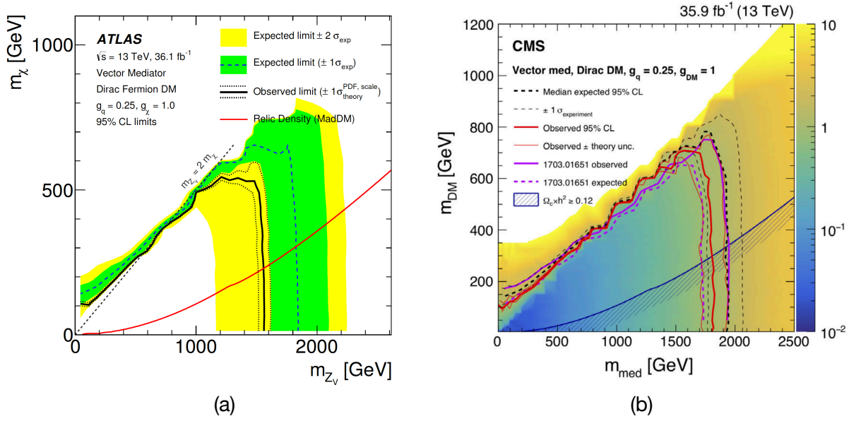
Figure 1.12: Limits on DM models as a function of DM particle mass and mediator mass on mono-jet + E_T^{\text{miss}} searches [68] [71]. (a) is from ATLAS results, and (b) is from CMS.
