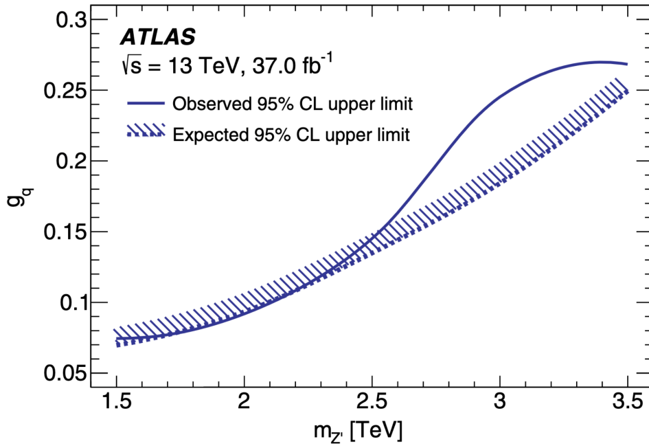
Figure 1.15: Limits on mediator mass and couplings emerging from ATLAS di-jet searches [77]
