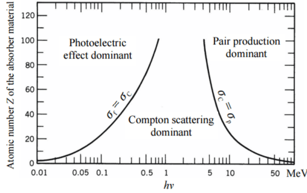
Figure 5.1: Three major types of photon interactions with matter as a function of their energy and the atomic number [179].
