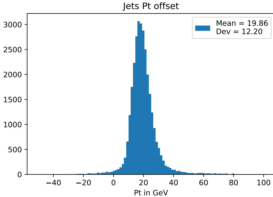
Figure 4.25: Pt absolute difference between the reconstructed topo jet and the associated truth ALP.
