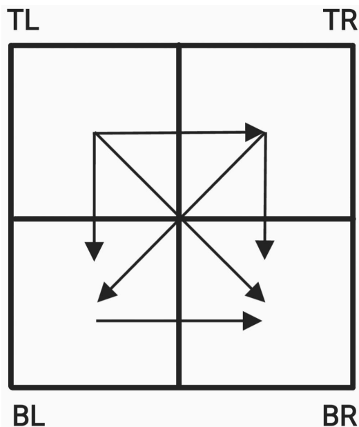
Figure 5.21: Illustration of all axes one can define with the TR, BL, BR, TL ring sets. Each axis can be used to compute ring energy distribution asymmetries.
