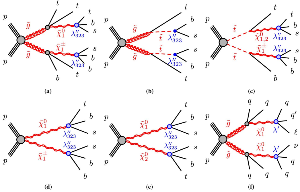
Figure 6.3: From [206]. Several simplified signal models were investigated during the analysis, including gluino, stop quark, and electroweakino decays. Anti-particle notation is omitted.
