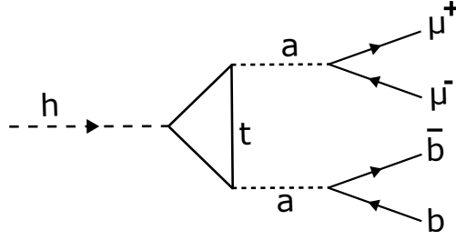
Figure 1.17: Double ALP Higgs boson decay producing a final state with a pair of bottom quarks and a pair of muons.
