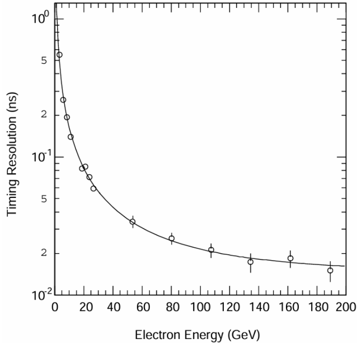
Figure 2.8: Timing resolution of single electronic channels of the LAr calorimeter [113].
