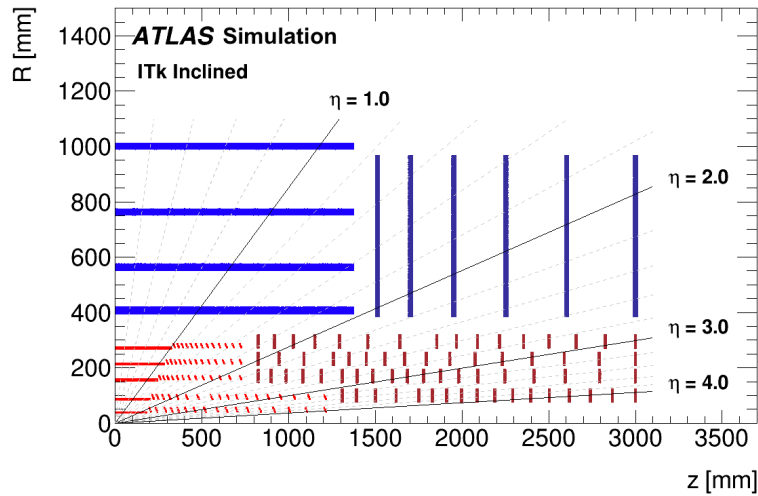
Figure 2.13: ITk layout in one quadrant and only showing the active detector elements. Strip detectors are shown in blue, and pixel detectors are shown in red.
