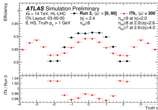
Figure 2.16: Tracking efficiency of the Run 3 and ITk hardware in their respective pile-up ( \mu ) environments and the same collision energy [146]. The required number of hits for different eta ranges is labeled.
