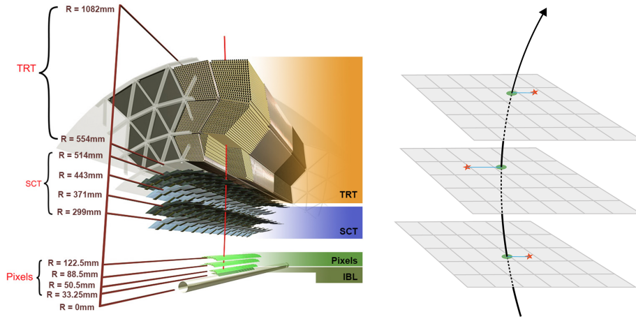
Figure 2.5: Schematic representation of ATLAS tracking system(left) including Pixels, SCT and TRT. A representation on the right indicates track reconstruction of a charged particle crossing the sub-detector planes. Red stars indicate each detector hit, while the fitted track is depicted with a black arrow. Green dots highlight the intersections of the track with each surface, and blue lines illustrate the track-to-hit residuals for each layer. From [109]
