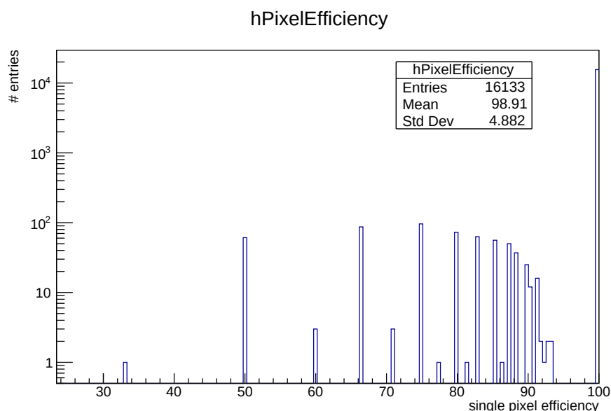
Figure 3.17: Distribution of single pixel efficiencies of an RD53 reference SCC used throughout the TB campaigns. Only showing the efficiency of unmasked pixels.
