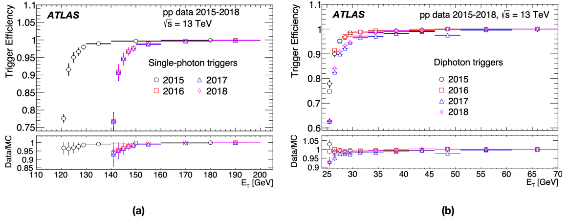
Figure 5.2: Run2 single (a) and di-photon (b) trigger efficiencies versus transverse energy. From the ATLAS performance paper [183]
