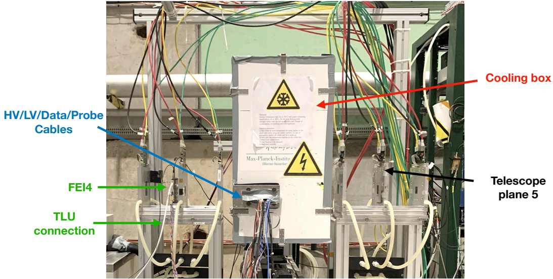
Figure 3.10: Picture of the test bench at CERN north area facilities. An arbitrary telescope plane is highlighted but the 6 planes are visible. The distance between the first and last telescope planes (1 and 6) is about 1.1 meters.
