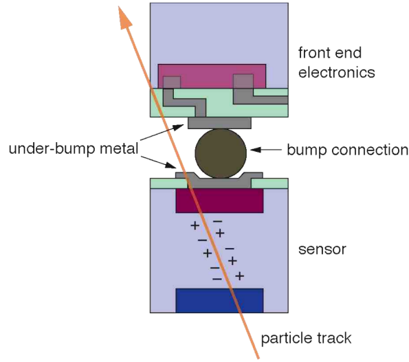
Figure 2.12: Illustration of a single pixel detector sensor. Particles ionize the active material (sensor), and the resulting pair charges drift towards the anode and cathode on the top and bottom. The collection of charges in the cathode is passed through the bump connection and creates a signal in the electronic chip. If the signal is above a given threshold, the acquisition system will record a hit. Taken from [144]
