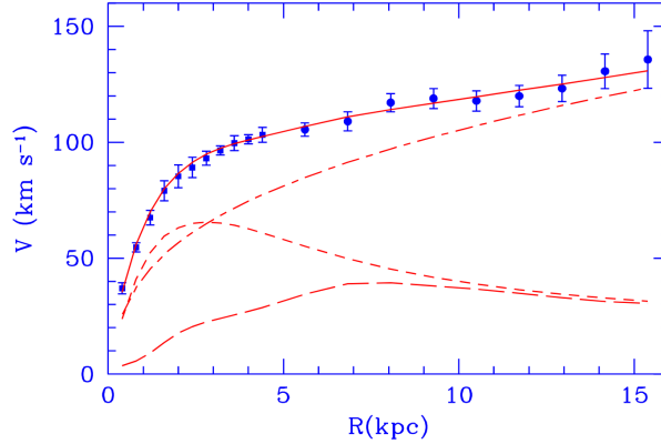
Figure 1.2: Evolution of experimental star rotation velocities as a function of the radial distance to the galactic center. Velocities are measured using the Doppler effect of the starlight in the galaxy. Large dashed lines represent the gas mass contribution. Short dashed lines are the stellar disk contribution. The fitted DM halo contribution is presented in dashed-dotted lines [17]
