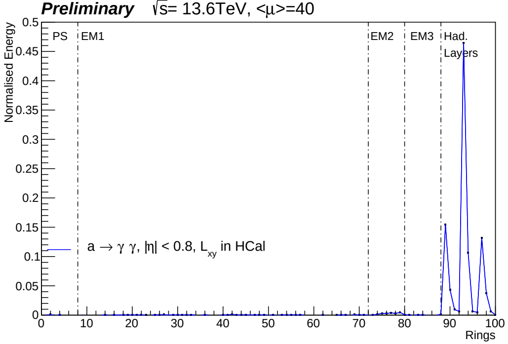
Figure 5.15: Average ring energy profile for 0.4 GeV ALP hadronic-calo decays into two photons. The x-axis represents the rings index according to table 5.1 as explained in section 5.4.2
