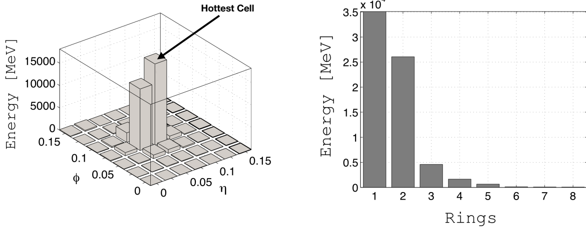
Figure 5.5: An illustration of how the calorimeter cell grid is compacted into a lower dimension ring energy profile. From [187].
