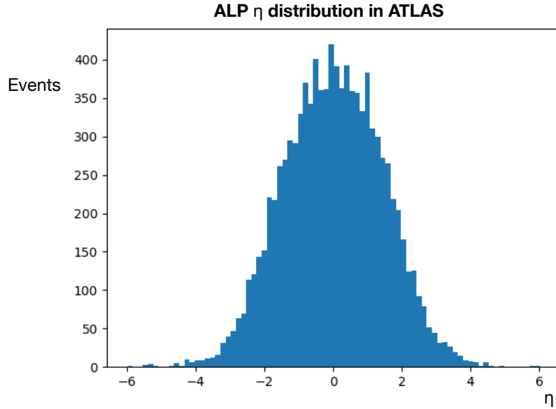
Figure 4.20: ALP \eta distribution in ATLAS, produced from a gluon-fused Higgs boson decay in association with a Z boson. Computed via the fast computation Python tool described in the current chapter.
