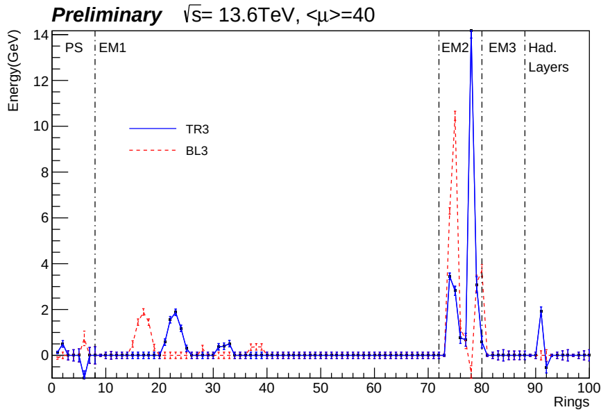
Figure 5.24: Ring profiles for TR3 and BL3 sets for the example ALP event. The x-axis represents the rings index according to table 5.1 as explained in section 5.4.2
