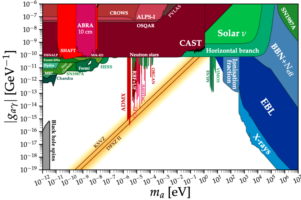
Figure 1.10: ALP parameter space with current experimental constraints [61].
