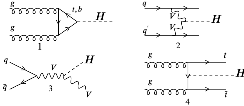
Figure 4.18: Feynman diagrams main processes for Higgs production in pp collisions at the LHC. 1: gluon-gluon fusion mechanisms; 2: Vector boson fusion, V stands for W or Z bosons; 3: Higgs-strahlung of an off-shell vector boson; 4: production in association with top quarks
