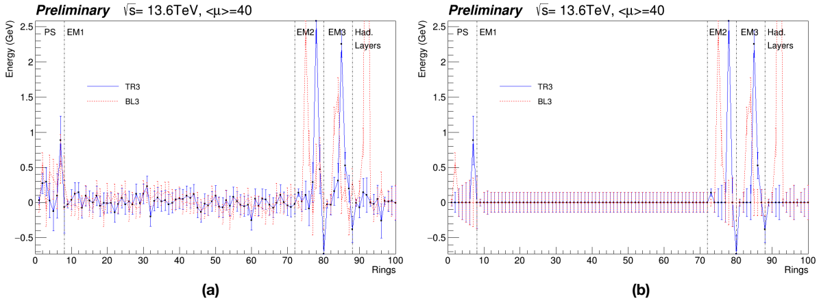
Figure 5.23: TR3 and BL3 ring profiles for a very asymmetric energy deposit. (a) without the noise removal procedure and (b) with removed noise. The x-axis represents the rings index according to table 5.1 as explained in section 5.4.2
