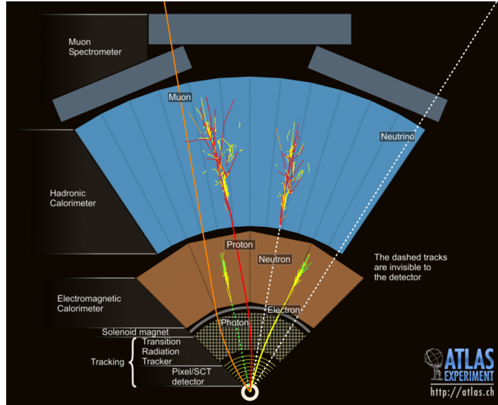
Figure 2.10: Different particles captured by ATLAS sub-systems. From [129]
