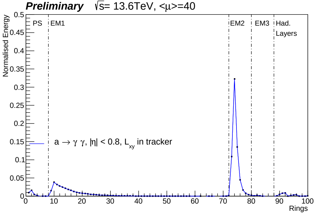
Figure 5.13: Average ring energy profile for 0.4 GeV ALP tracker decays into two photons. The x-axis represents the rings index according to table 5.1 as explained in section 5.4.2
