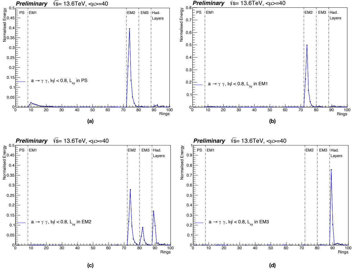
Figure 5.16: Average ring energy profiles for different 0.4 GeV ALP decay lengths associated with 4 layers of the EM calorimeter. Mind the fact that all vertical axes do not reach the same maximum for visualization's sake. (a): ALPs decaying in the Presampler. (b): ALPs decaying in the first sampling. (c): ALPs decaying in the second sampling. (d): ALPs decaying in the third sampling. The x-axis represents the rings index according to table 5.1 as explained in section 5.4.2
