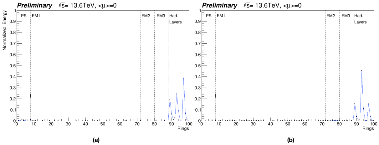
Figure 5.17: Average ring profiles for ALPs decaying at same displacement L_{xy} inside the hadronic calorimeter. (a) ALPs going towards the extended barrel and end caps ( \eta [0.8 - 2]). (b) ALPs are directed to the main barrel. The x-axis represents the rings index according to table 5.1 as explained in section 5.4.2
