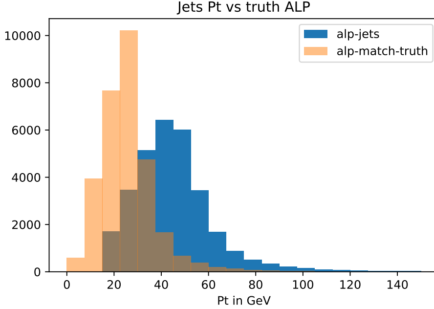
Figure 4.24: Pt distribution of the ALP and the associated reconstructed jets.
