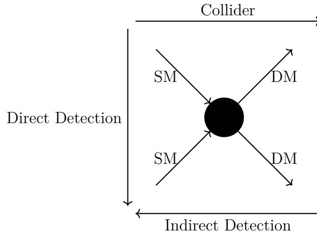
Figure 1.1: Schematic representation of dark matter detection methods at microscopic scales based on an unknown effective interaction of DM with standard model particles.
