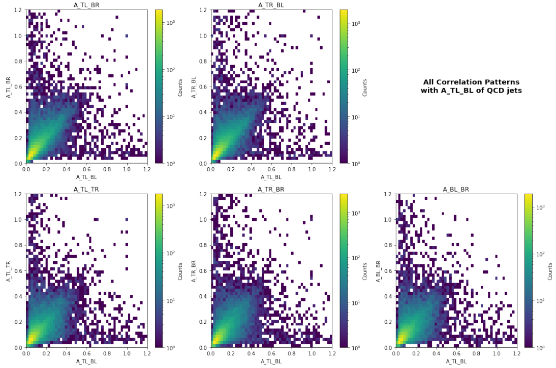
Figure 5.31: 2D histograms of correlations of the asymmetry axis TL-BL with the 5 other axes. Computed for QCD jets. The correlations remain similar no matter the combination of axes. This reflects the homogeneity of the energy deposit.
