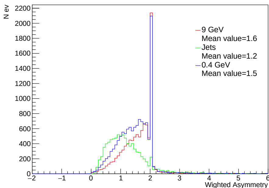
Figure 5.28: Asymmetry distribution between QCD jets and ALPs with metric using ring average normalization.
