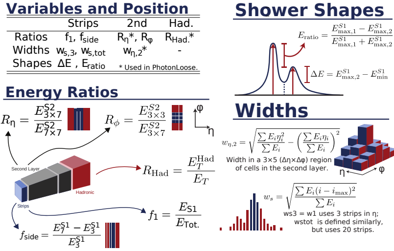
Figure 5.3: Geometrical sketch of the standard shower-shape variables used for electron and photon identification against jets in ATLAS. [184]
