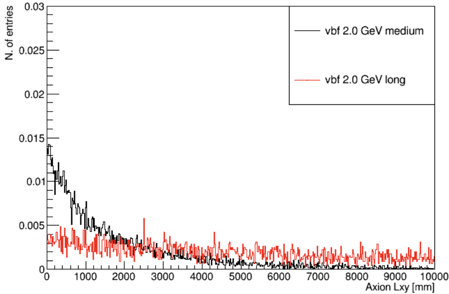
Figure 5.12: Transversal displacement distribution of an ALP ( m_a = 2\text{GeV} ) produced by a VBF-Higgs (boson-fusion) decay for two lifetimes: c\tau_{med} = 131\text{ mm} and c\tau_{long} = 1.3\text{ m}
