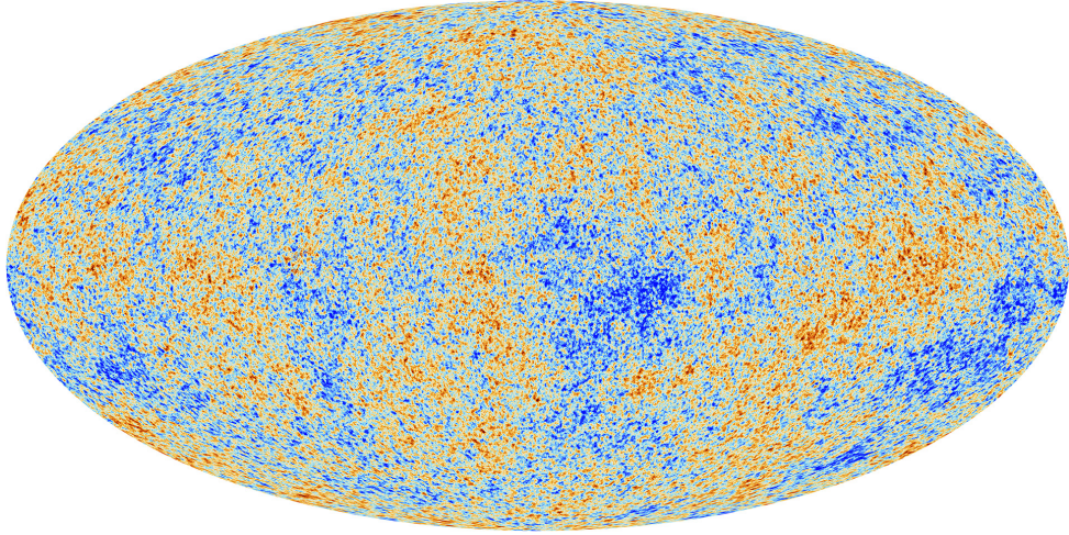
Figure 1.3: An intensity map of the CMB, showing temperature fluctuations. Maximum and minimum fluctuations are: -300\mu K (blue) + 300\mu K (red). Credit ESA and the Planck Collaboration.
