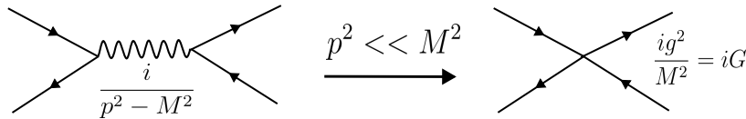
Figure 1.7: Illustration of EFTs replacing a mediator term by a point-like interaction.
