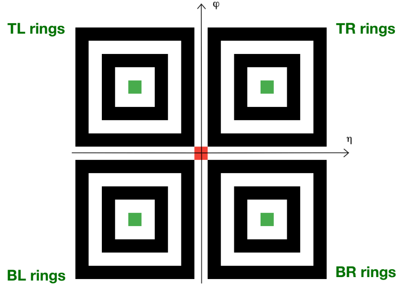
Figure 5.19: Schematics of Quad-Rings placement around the center. The red cell is the hottest in the energy deposit. While the green cells give the 4 new corner-seed positions to compute 4 new ring sets.
