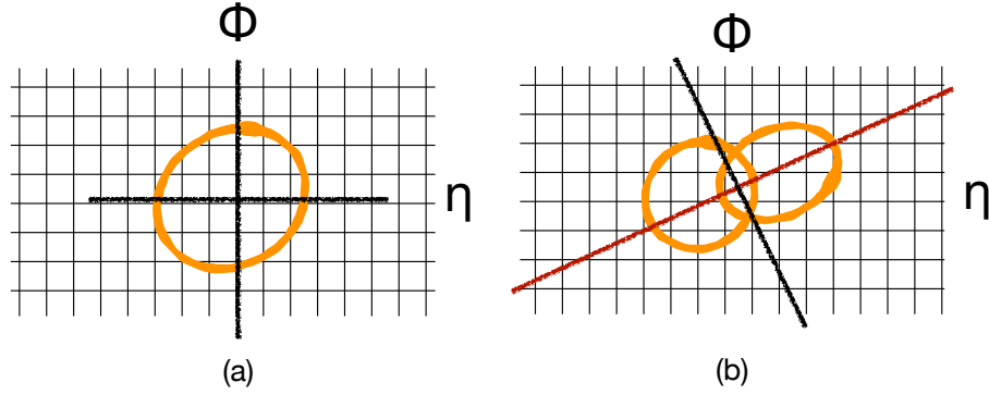
Figure 4.4: Representation of single (a) and double body (b) cluster in a calorimeter transversal cut. A red line is drawn to represent the preferred axis for energy distribution in (b).
