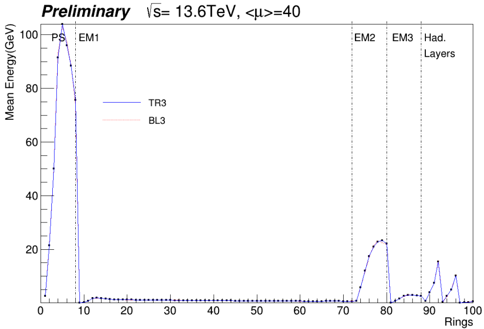
Figure 5.22: Average ring profile for QCD Jets for TR3 and BL3. The x-axis represents the rings index according to table 5.1 as explained in section 5.4.2
