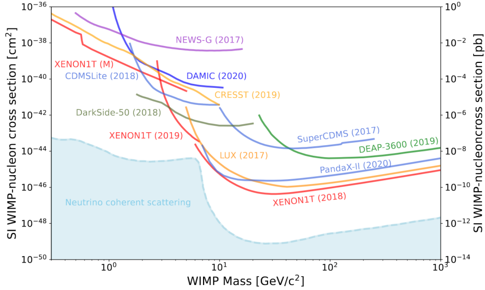
Figure 1.9: Overview of WIMP searches at direct detection experiments. From [41]
