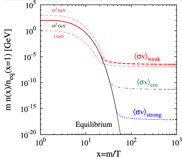
Figure 1.8: Evolution of WIMP abundance for different choices of annihilation cross section \sigma v [35]. The number of WIMPs normalizes the abundance during the equilibrium phase. Three different final abundances depend on \sigma v , with v being the velocity of particles. This is used instead of \sigma as it represents an interaction rate for a volume unit.
