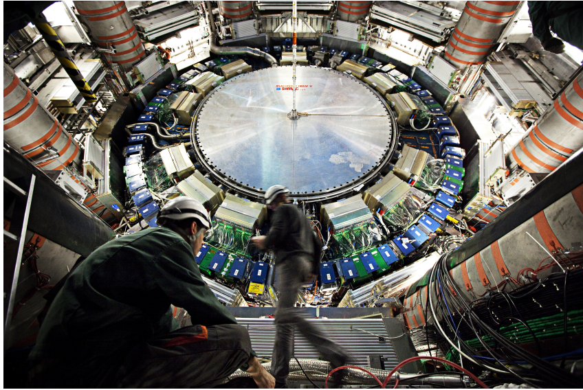
Figure 2.2: A picture of ATLAS taken in front of a calorimeter end-cap. Picture from [101].
