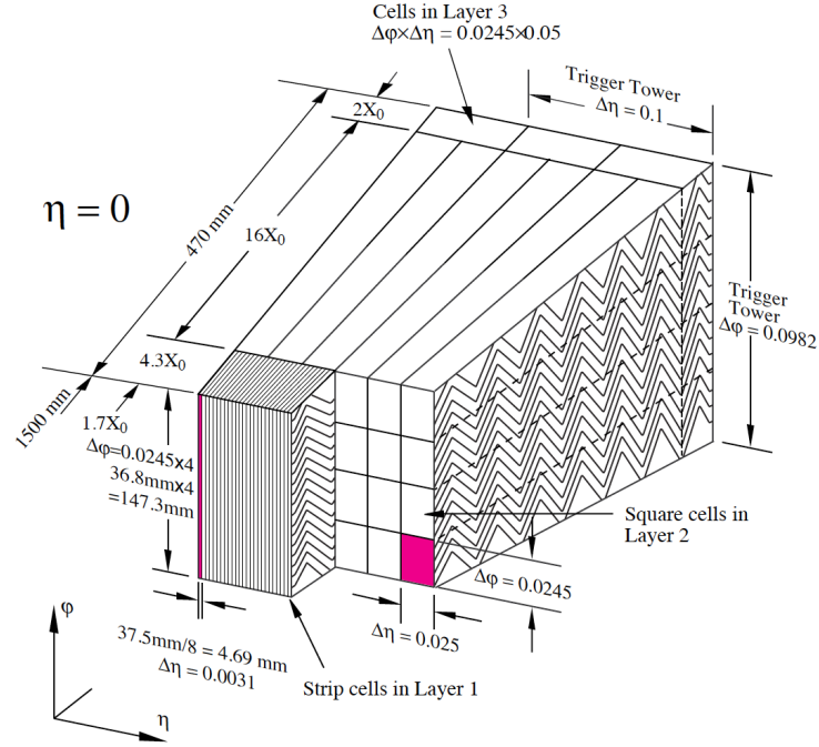
Figure 5.11: A module of the EM calorimeter displaying each layer depth. From the ATLAS experiment paper [100].
