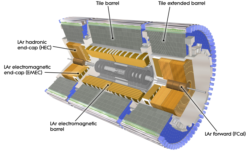
Figure 2.6: Schematics of ATLAS EM and hadronic calorimeter systems in barrel and end-cap regions. From [111]
