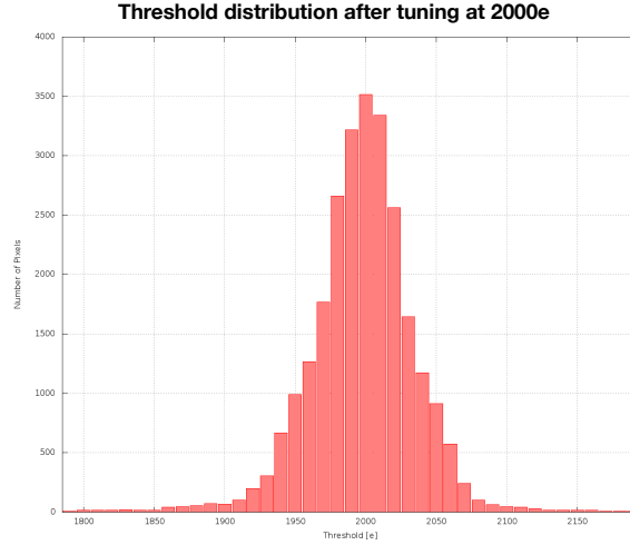
Figure 3.6: A resulting distribution pixel thresholds after tuning. Realized on an RD53A SCC with a target threshold of 2000 electron charges.
