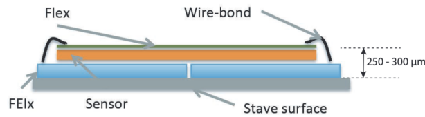
Figure 2.15: Hybrid Quad module layout. The flex is glued to the sensor, which is bump-bonded to four front-end chips. Very small wires connect the front-end readout pads to the flex. FEIx refers to one of the four FE chips of a quad module.
