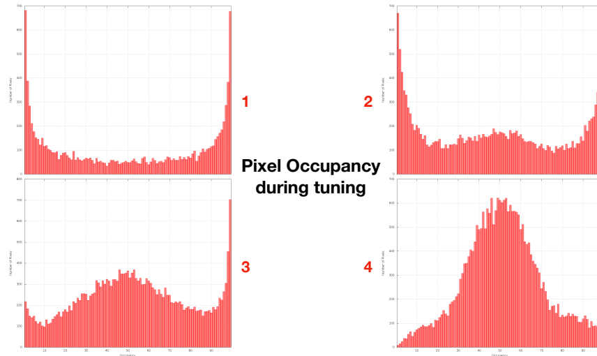
Figure 3.5: The occupancy distribution during 4 steps of pixel threshold tuning. The x-axis is the occupancy in percentage, and the y-axis is the number of pixels. Realized on an RD53A SCC
