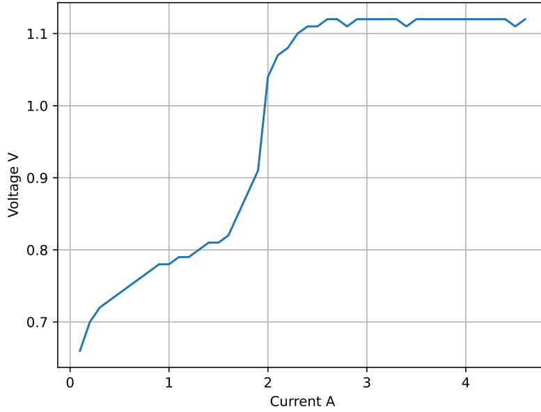
Figure 3.4: A VI curve of a digital module (no sensor installed) taken at room temperature.
