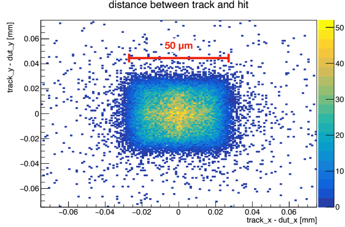
Figure 3.16: Distribution of distance between hit position and track position on the x,y plane. The main bulk is kept inside a 50 * 50 \mu m^2 area. Obtained with a fully depleted RD53B SCC.
