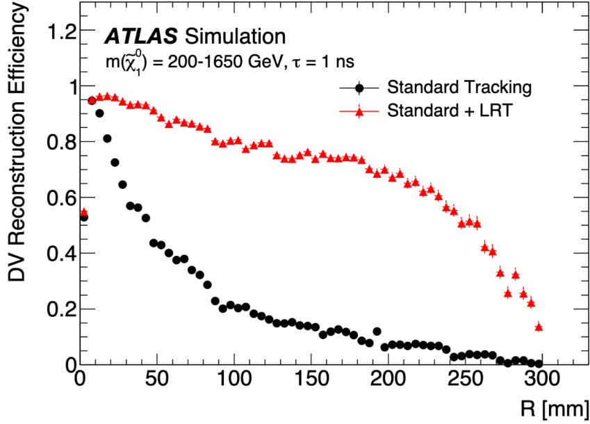
Figure 4.8: DV reconstruction efficiencies for ATLAS standard and modified track reconstruction algorithms. The modified algorithm is large-radius tracking and is tailored for LLP cases [110].
