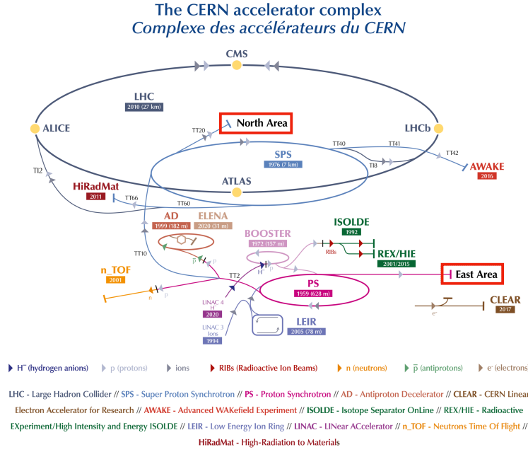
Figure 3.8: The CERN accelerator complex. The north and east test-beam areas are highlighted in red. Modified from [160].
