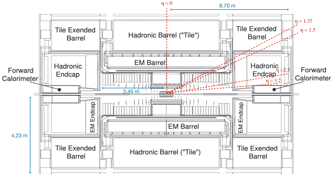
Figure 4.12: Side view of ATLAS calorimeters with relevant dimensions and important eta segmentation.
