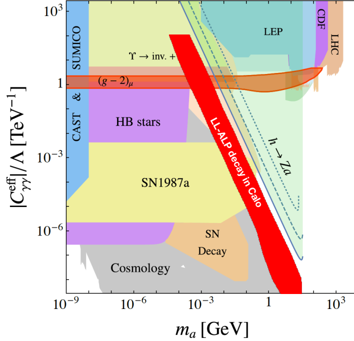
Figure 4.15: Resulting parameter space for ALP decays inside the Calorimeters. The region compatible with h \rightarrow Za ALP decays in the calorimeter is highlighted in red. The limits are computed as described in 4.4.4. The prompt ALP decay region corresponding to the same process is highlighted in light green. Adapted from [79].
