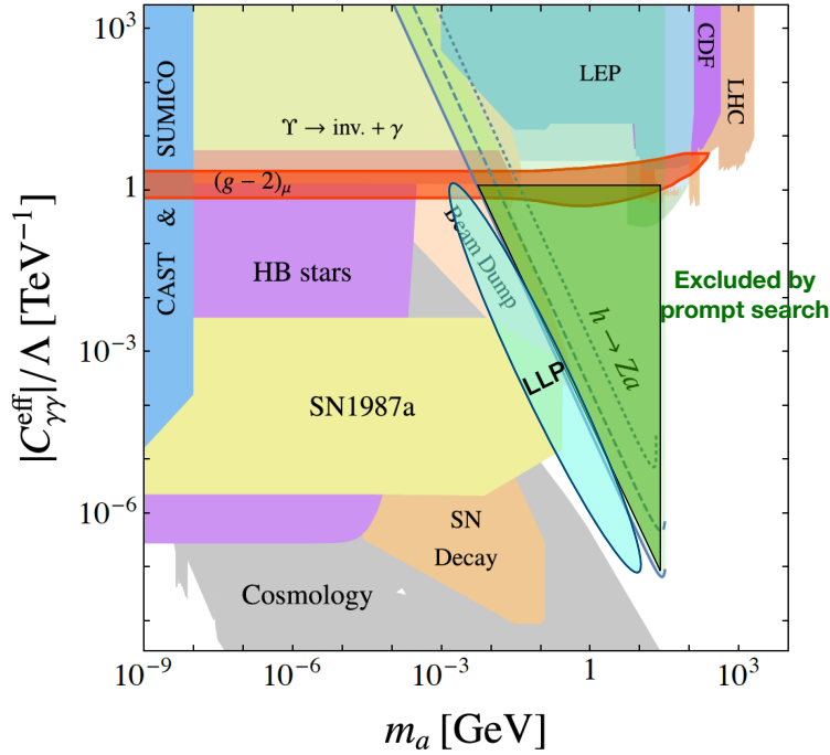
Figure 4.6: The ALP parameter space of photon decays. Presenting the LLP and prompt regions associated with h \rightarrow Za . Adapted from [79].
