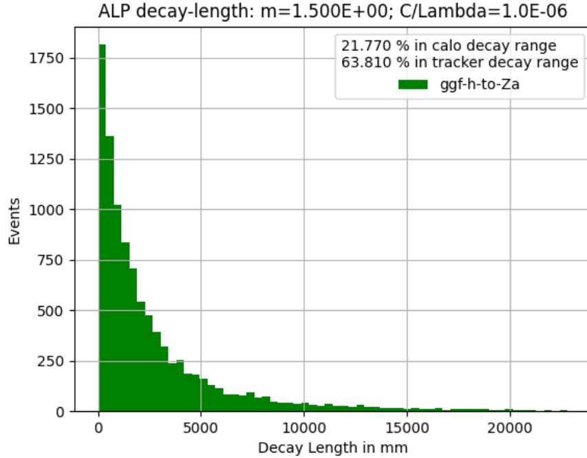
Figure 4.14: ALP computed decay length distribution for m_a = 1.5 GeV and f_a = 10^{-6} .
