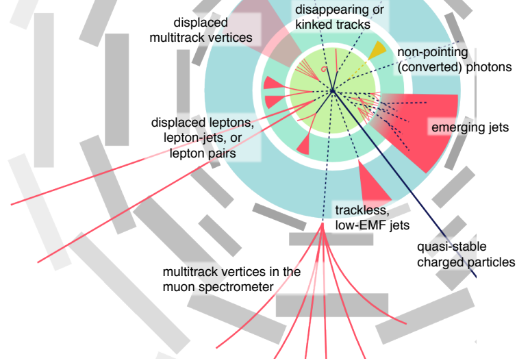
Figure 4.7: Schematic of various LLP signatures at LHC experiments. Represented on an ATLAS-like detector.
