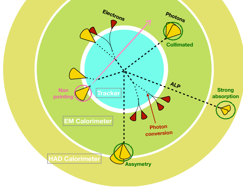
Figure 4.9: Diversity of photon decays from an LL-ALP in an ATLAS-like detector.
