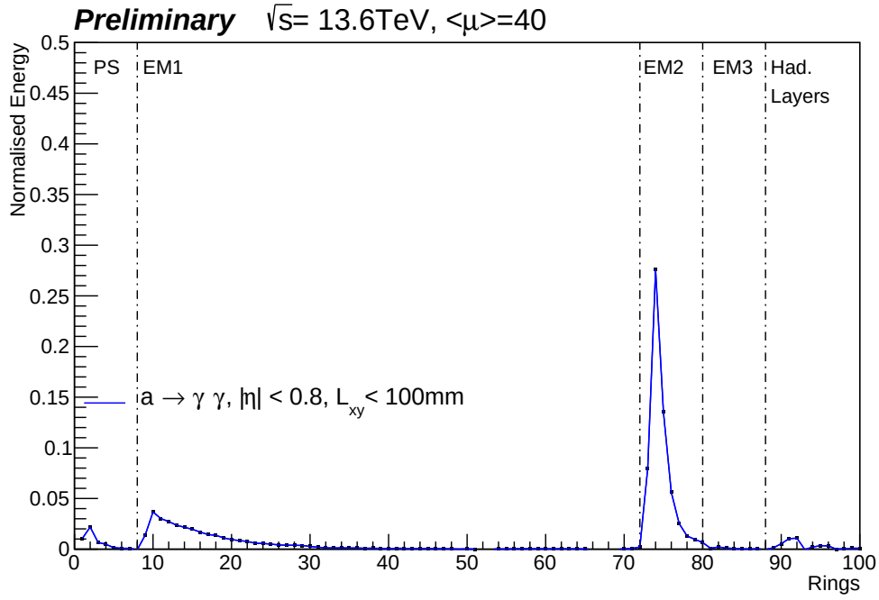
Figure 5.9: Average energy profile of rings, for low ( L_{xy} < 100 mm) displaced 0.4 GeV ALPs. Tails are visible following main peaks, reflecting the spectrum of secondary peak positions. The x-axis represents the rings index according to table 5.1 as explained in section 5.4.2
