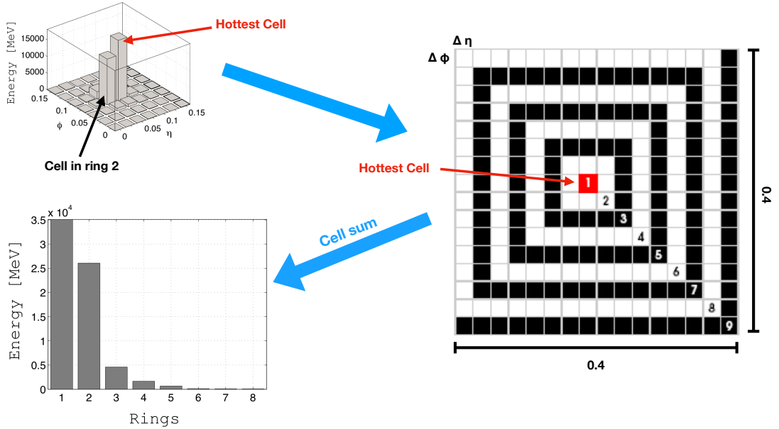
Figure 5.6: Schematics of how the cell grid is turned into rings with the correct number labeling. All cells are then summed into ring energy values.
