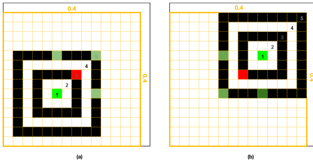
Figure 5.20: Schematics of TR and BL ring sets for a 2-cell displacement between the new seed (green) and the one used for standard rings (red) in the EM2 layer. The red cell indicates the usual center for rings, while the green cells indicate the 4 offset centers. (a) is the TR2 set, and (b) is the BL2 set.
