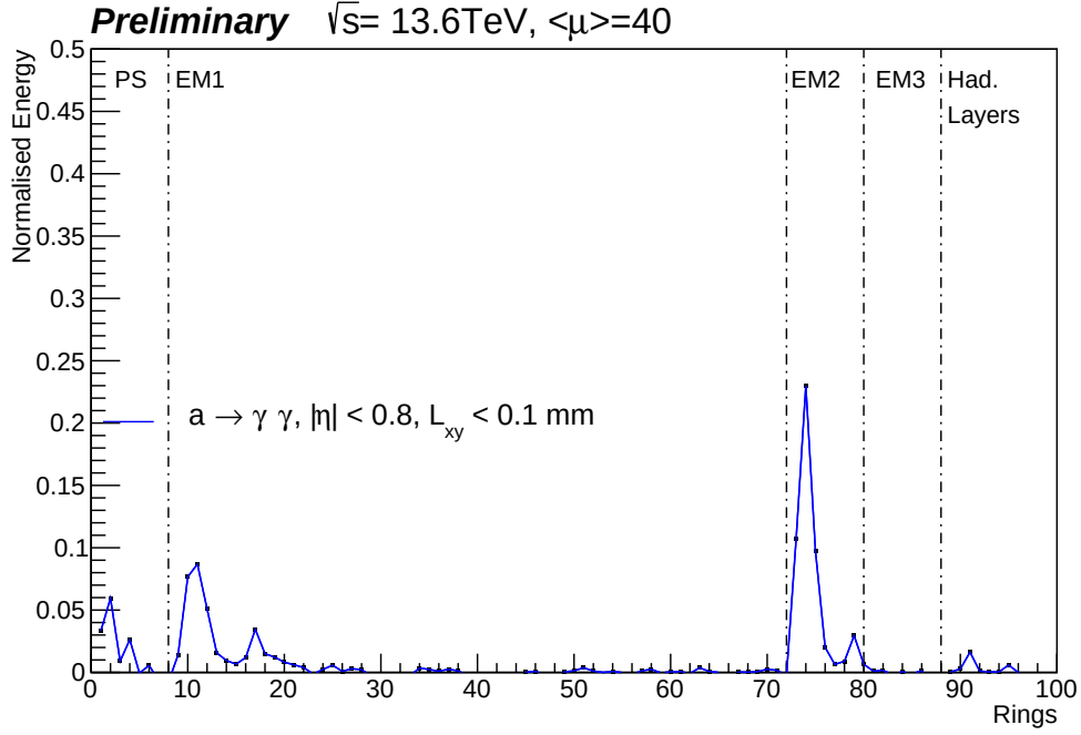
Figure 5.8: Energy profile of rings, for a prompt boosted merged photon decay of a 0.4 GeV ALP. A double peak structure is visible in the main absorber layers. The x-axis represents the rings index according to table 5.1 as explained in section 5.4.2
