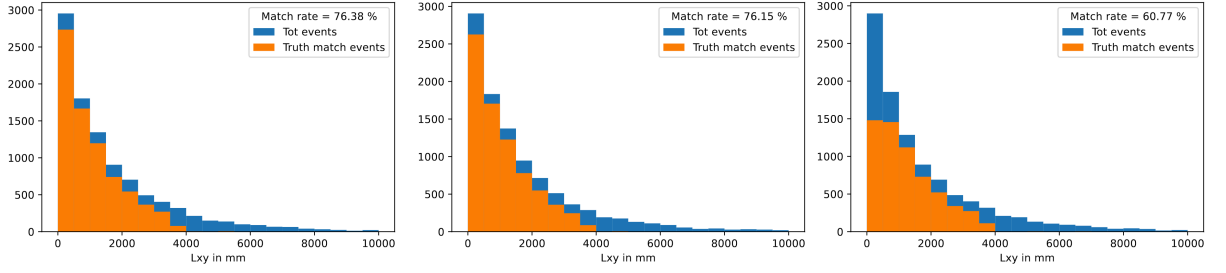
Figure 4.23: Matching rate of ALPs with topo jets for different bins of displacements. L_{xy} refers to the displacement in the (x, y) plane. Left: 0.4 GeV ALPs. Middle: 2 GeV ALPs (threshold between merged and resolved). Right: 9 GeV ALPs.
