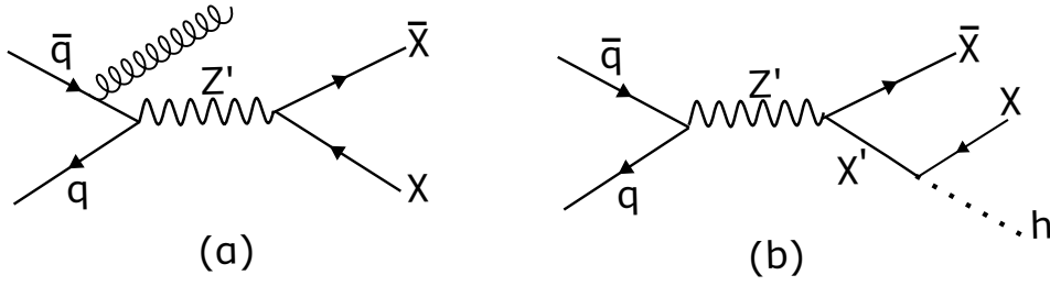
Figure 1.11: Feynman diagrams of DM pair production at the LHC with the emission of an associated SM particle. Z' is a massive vectorial mediator linking the SM to the dark sector. \chi' represents an excited state of the DM particle. (a) represents mono-jet + E_T^{miss} events and (b) illustrates possible mono-Higgs + E_T^{miss} events
