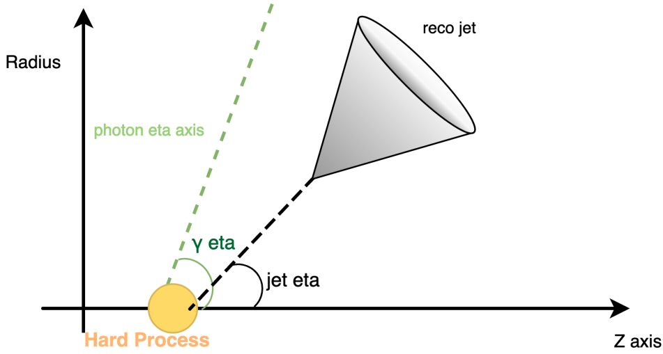
Figure 4.22: The angular separation in \eta between the photon axis and the jet axis for a displaced case. The photon axis is projected to the collision point to illustrate the large difference. This difference is above the threshold for truth matching; however, the photon is inside the jet cone. This demonstrates that only angles cannot be used for truth-matching LLPs.
