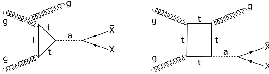
Figure 1.16: Processes contributing to DM plus one jet events through a pseudo-scalar mediator.
