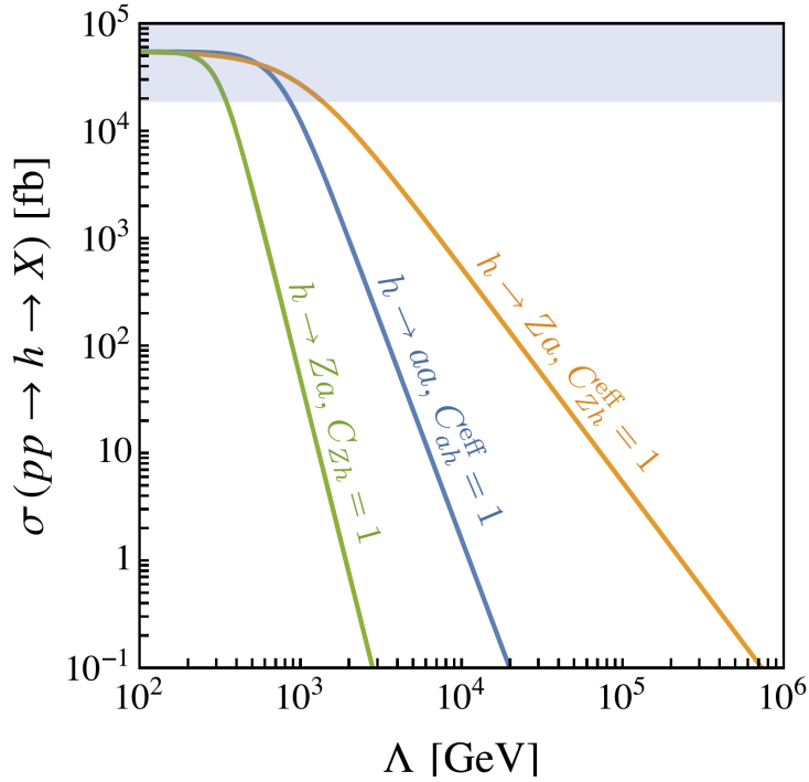
Figure 4.16: Production cross sections of ALPs produced in the decays of Higgs and Z bosons at the LHC for the energy scale \Lambda [79].
