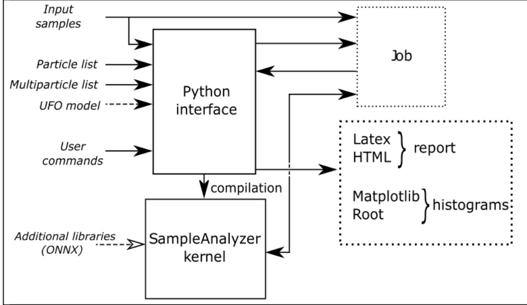
Figure 6.1: The madanalysis5 manual mode flowchart. Additional libraries can be added to the SA kernel manually. However, recent developments have directly included ORT within the framework.
