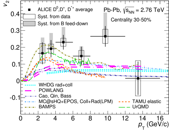
Figure 2.11: Comparison of the prompt D-meson v_2 (average of D^0 , D^+ and D^{*+} ) in Pb–Pb collisions at \sqrt{s_{NN}} = 2.76 TeV in the 30-50% centrality class, compared to various models. A qualitative description of the data is seen from the models MC@sHQ+EPOS , Coll+Rad(LPM) , BAMPS , TAMU elastic and UrQMD [99]. The models WHDG rad+coll , POWLANG and Cao, Qin, Bass , which either do not include collective expansion of the medium, or lack a contribution to the hadronization via recombination with light quarks from the medium, in general predict a smaller anisotropy than observed in data [99]. A more descriptive summary of the models can be found in [99].
