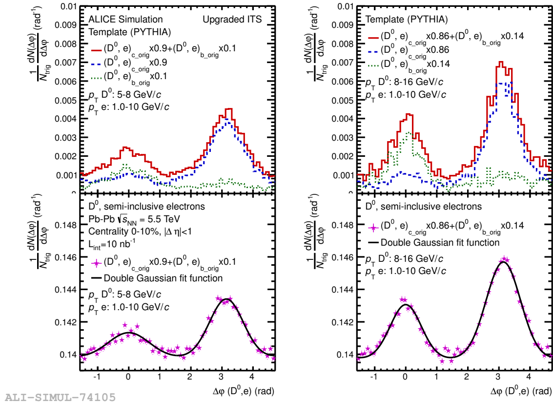
Figure 7.2: D0-e correlations based on simulations with the ITS detector upgrade planned for LHC Run 3. The template (upper row) and output (lower row) distributions, as expected for 8 \times 10^9 Pb–Pb collisions at 0-10% centrality, at \sqrt{s_{NN}} = 5.5 TeV, are presented in the two trigger particle p_T regions of 5 < p_T^{D^0} < 8 GeV/c and 8 < p_T^{D^0} < 16 GeV/c, with the associated particles studied in the interval 1 < p_T^e < 10 GeV/c. The blue dashed line represent the contribution from prompt D 0 mesons, while the dotted green line correspond to the feed-down contribution. The prompt and feed-down contributions were scaled by their relative fractions calculated from FONLL predictions, as indicated by the numbers in the legend. The solid red line represents the combined distribution from both sources. Figure from [152].
