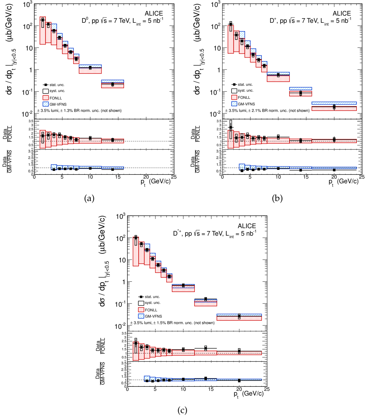
Figure 2.2: p_T differential inclusive cross section for prompt (a) D^0 , (b) D^+ and (c) D^{*+} mesons in pp collisions at \sqrt{s} = 7 TeV, compared with FONLL and GM-VFNS theoretical predictions [72]. The results are compatible within uncertainties to both of the theoretical calculations. Figure from [72].
