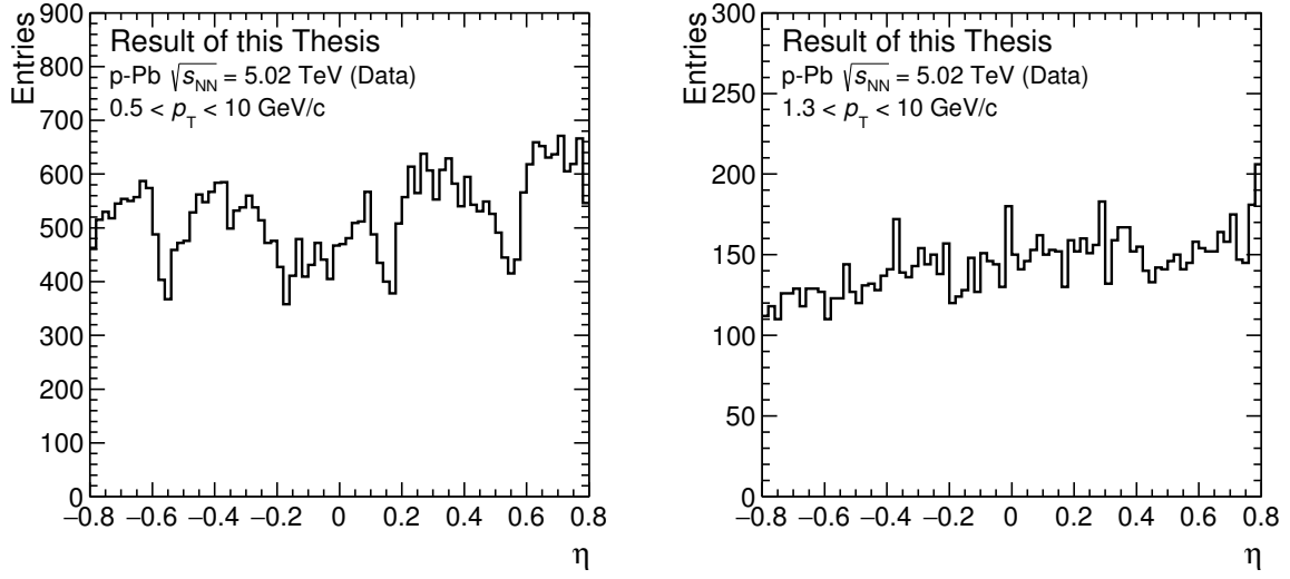
Figure 4.7: Pseudorapidity, \eta , distributions for the selected electron sample in the regions (left) 0.5 < p_T < 10 GeV/ c and (right) 1.3 < p_T < 10 GeV/ c . In the region below p_T = 1.3 GeV/ c , a requirement of TOF matching is imposed, and a clear structure caused by the segmentation of the TOF detector into 5 segments in the beam direction is seen, indicating a loss of selection efficiency towards the edges of the detector segments. Above p_T = 1.3 GeV/ c , TOF matching is no longer required, and a smoother distribution is observed. An increasing trend is observed from negative to positive \eta , due to the asymmetric p-Pb collision environment, where the proton arrives from positive \eta and the lead ion from negative \eta .
