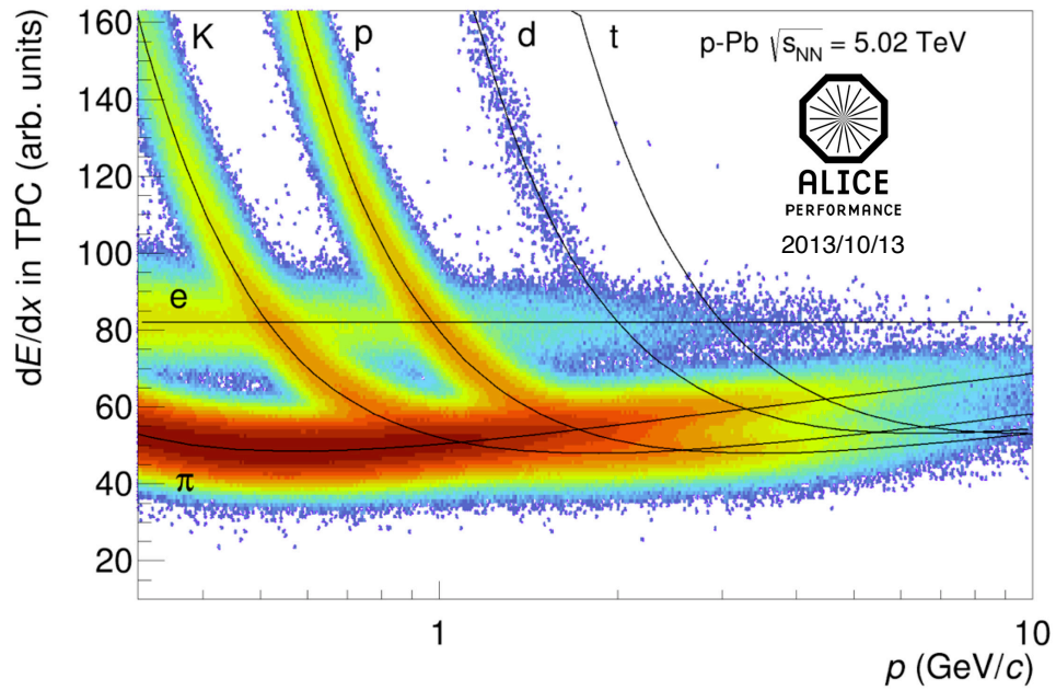
Figure 3.7: dE/dx of charged particles vs their momentum measured by the TPC in pPb collisions. The solid lines are parametrizations of the detector response based on the Bethe-Bloch formula for various particle species.
