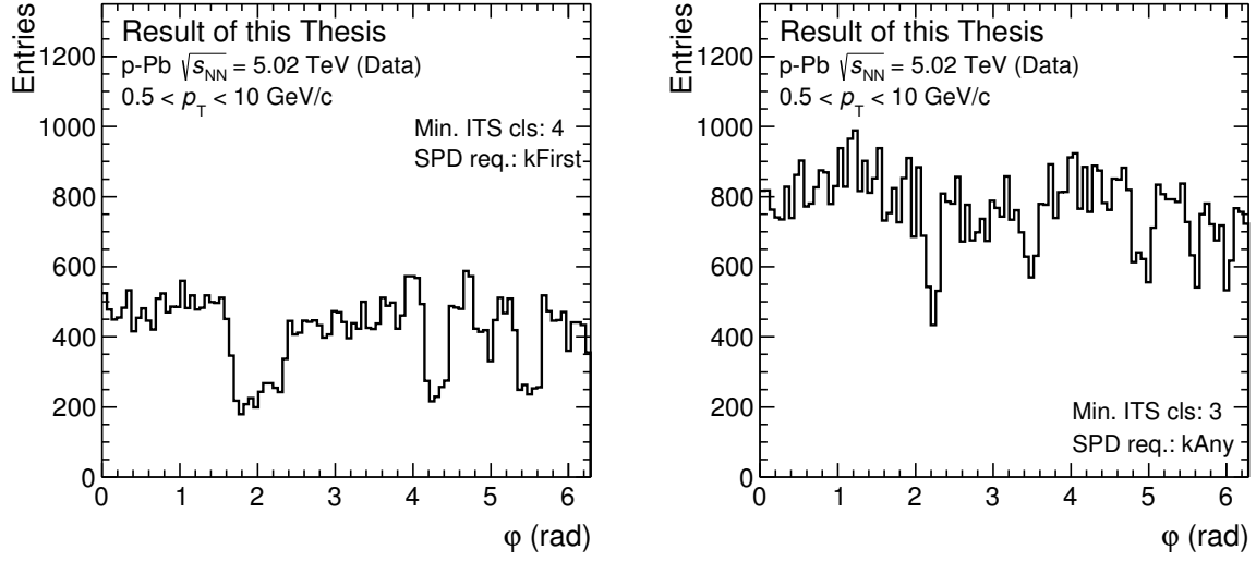
Figure 4.8: Azimuthal, \phi , distributions for the selected electron sample. The left panel displays the ITS cut configuration used in the thesis, where 4 hits are required in the detector, and a hit in the first layer of the SPD is required (kFirst). The panel to the right shows the same distribution with less strict cuts, where only 3 hits are required in the ITS, and a hit must be registered in one of the two layers in the SPD. The well defined structures seen in the distribution produced with strict cuts are washed out to some degree in the case of looser cuts. A higher total number of entries is also observed for the scenario using looser cuts, indicating some loss of efficiency while tightening the ITS requirements.
