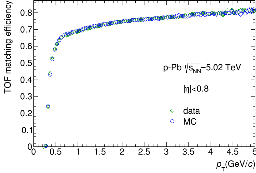
Figure 4.11: Matching efficiency (including the geometric acceptance factor) at TOF for tracks reconstructed in the TPC in p-Pb collisions at \sqrt{s_{NN}} = 5.02 TeV, compared to Monte Carlo simulation. Figure and caption from [126].
