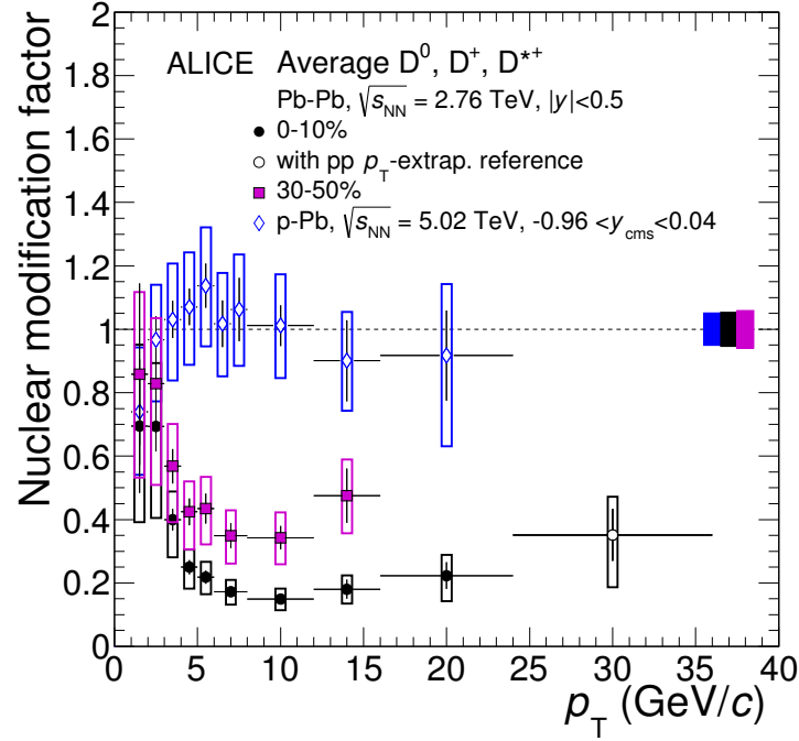
Figure 2.9: Comparison of the prompt D-meson R_{AA} (average of D^0 , D^+ and D^{*+} ) as a function of p_T in Pb–Pb collisions at \sqrt{s_{NN}} = 2.76 TeV in the 0-10% and 30-50% centrality classes, compared to the R_{pA} measured in p–Pb collisions at \sqrt{s_{NN}} = 5.02 TeV [101] [64]. The R_{pA} is compatible with unity within uncertainties, indicating that the suppression seen in R_{AA} is of different origin than Cold Nuclear Matter (CNM) effects.
