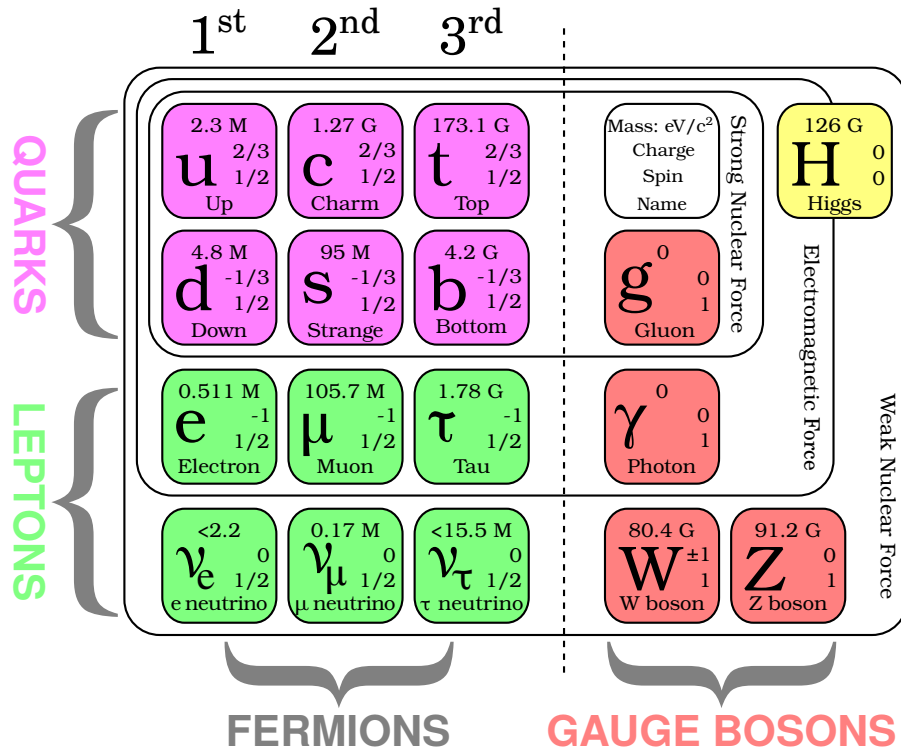
Figure 1.1: A summary of the Standard Model of Particle Physics, displaying the fermions (spin 1/2) to the left, and the bosons to the right. The bosons are divided into the gauge bosons (spin 1) and the Higgs boson (spin 0). The fermions are divided into quarks and leptons, and are sorted by their generations in columns. The quarks are also sorted by their charge in rows. The particles are associated to the forces responsible for their interactions. Figure modified from [2].
