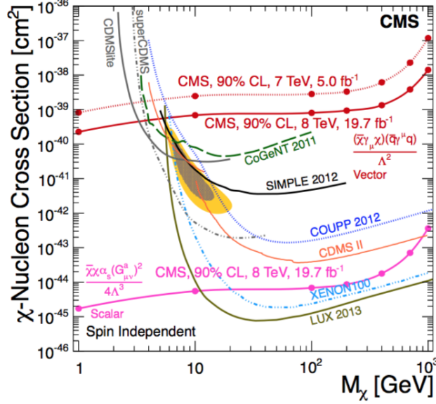
Figure 4.8: Upper limits for vector and scalar operators interpreted in inclusive monojet channel on the \sigma_{\chi-nucleon} , at 90% CL, plotted against DM particle mass and compared with previously published results.
