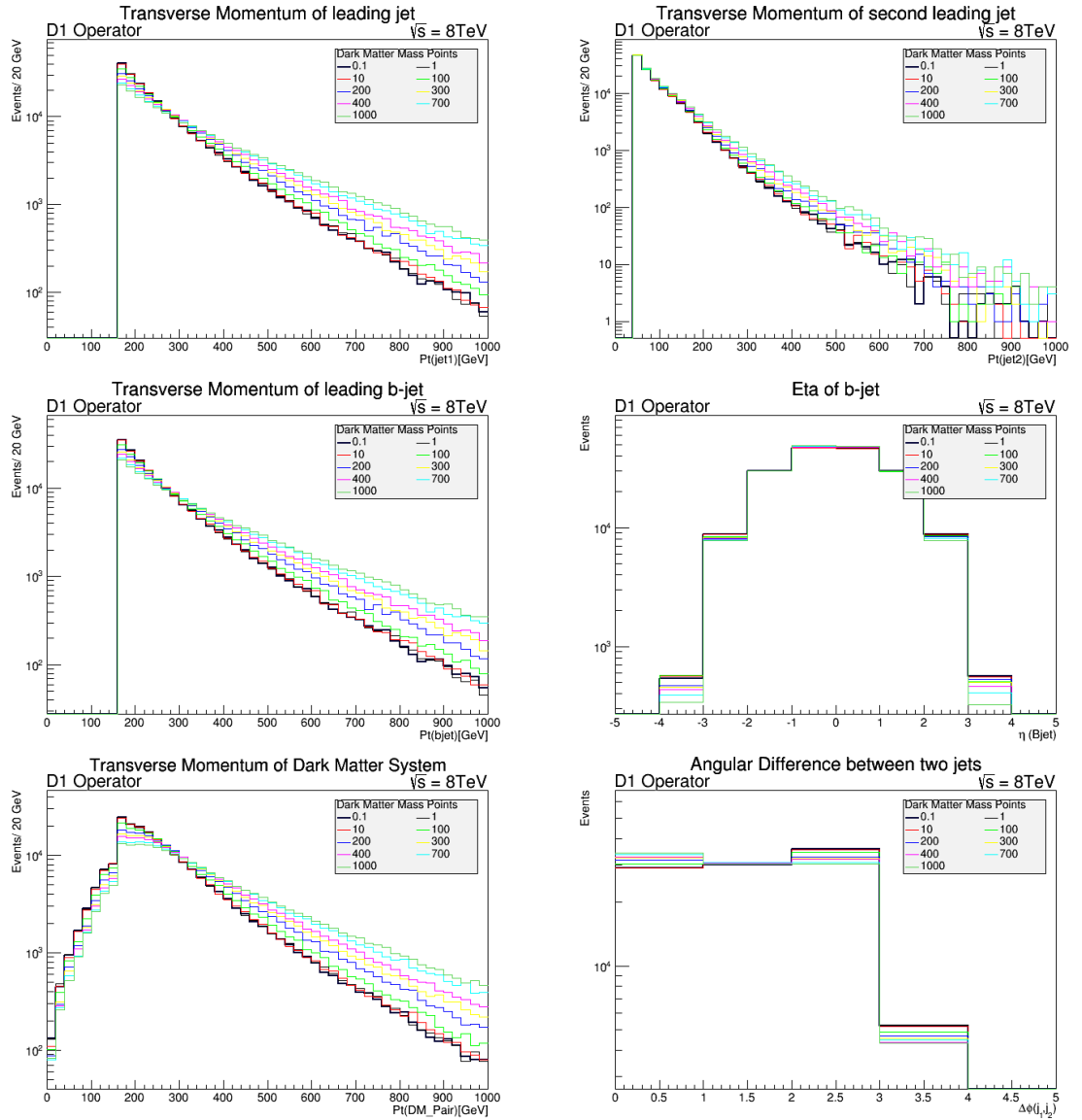
Figure 4.5: The basic kinematics for the generated signal process consisting two leading jets and a DM system.
