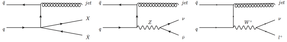
Figure 2.12: The Feynman Diagram of DM pair production in association with gluon (left), and the background Z(\nu\bar{\nu}) + jet (middle) and W(l\nu) + jet (right).
