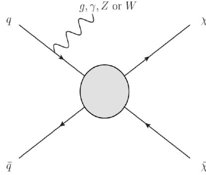
Figure 2.9: In the Mono-X topology, the interaction between DM and SM are described by a physical scale as a result of the mediator being factorized out.
