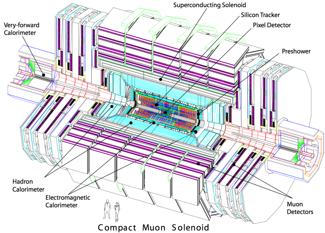
Figure 2.2: A schematic view of the CMS detector (CMS Collaboration, 2008).
