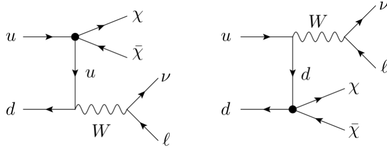
Figure 2.13: The interference of two scenarios where the W boson radiates from the u-quark or the d-quark (Bai & Tait, 2013).
