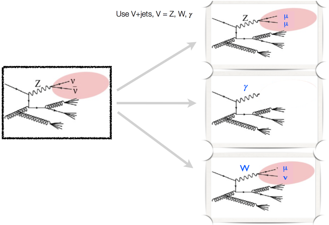
Figure 3.1: Processes with similar topology, V+jets can be used to estimate exclusively on Z(\nu\bar{\nu}) + jets .
