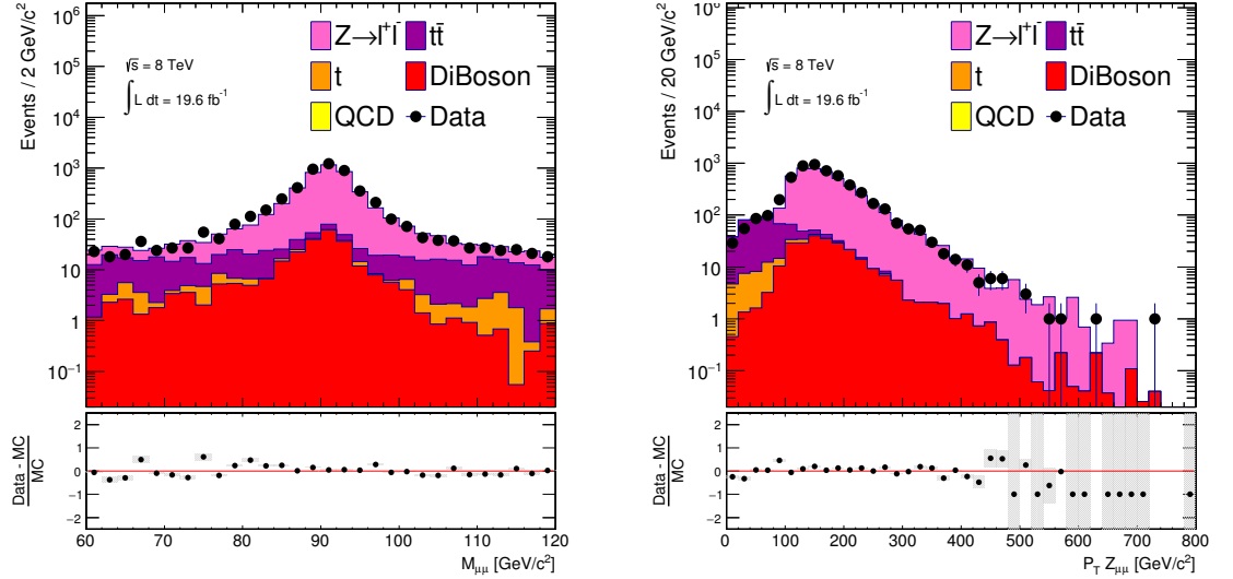
Figure 3.3: Invariant mass and transverse momentum of the di-muon pair in the Z(\mu\bar{\mu}) control sample.
