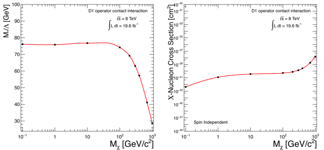
Figure 4.7: (left) The 90% CL lower limit on M_* and (right) the 90 % CL upper limit on \sigma_{\chi-nucleon} as a function of M_\chi assuming a D1 scalar operator in mono-b + E_T^{miss} channel.
