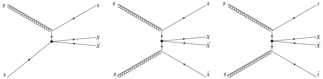
Figure 2.14: The dominant diagrams contributing to associated production of dark matter with bottom and top quarks (Lin et al., 2013).
