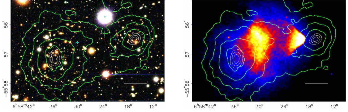
Figure 2.6: Images of the bullet cluster, 1E0657-558: optical image from the Hubble Space Telescope (left) and X-ray image from Chandra telescope (right). The mass density contours from gravitational lensing reconstruction superimposed on two images (Clowe et al., 2006).
