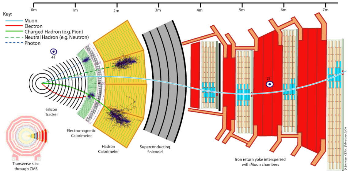
Figure 2.4: The transverse slice of the CMS detector and the interaction of each type of particle with the sub-detectors. Different type of particle interacts with different CMS components, various colored curved lines represent paths that a particular particle might take.
