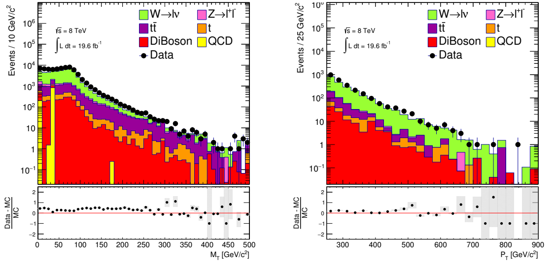
Figure 3.4: Transverse mass and transverse momentum of W^\pm candidates in the single-muon sample.
