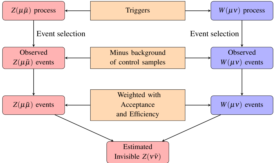
Figure 3.2: The flow chart data-driven background estimation on Z(\nu\bar{\nu}) events by using two different control sample in the context of b-tagged monojet event selection.
