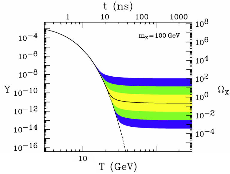
Figure 2.7: The number density Y (left) of a 100 GeV, P-wave annihilating Dark Matter particle evolves as a function of time t (top) and temperature T (bottom). The solid contour is the annihilation cross section yields the correct relic density \Omega_\chi (right), which is \sim 0.23 (Feng, 2010).
