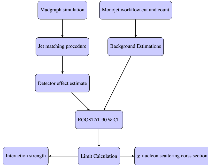
Figure 4.3: The flow chart of the sensitivity study on mono-b + E_T^{miss} channel within the standard monojet framework.
