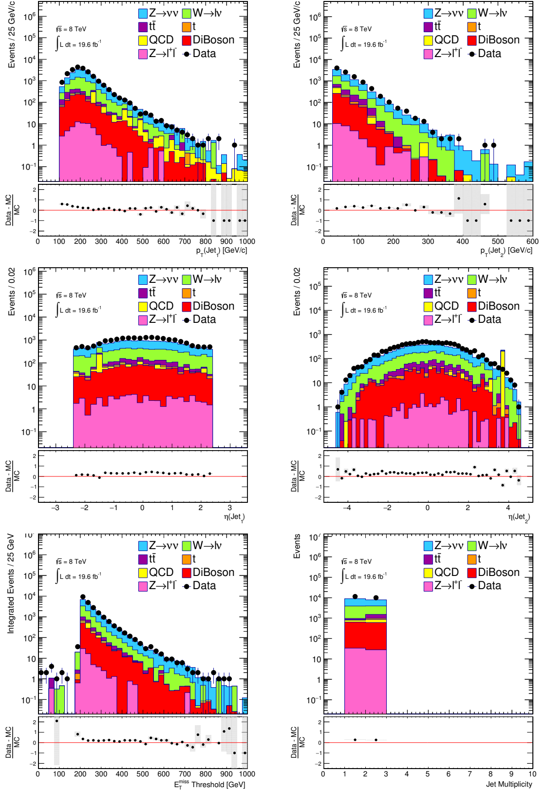
Figure 4.6: The kinematics plots after the mono-b event selection with b-tagging operating at medium working point.
