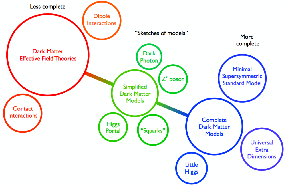
Figure 2.8: Artistic view of the DM theory space.
