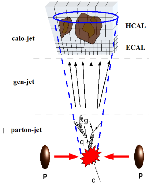
Figure 2.5: Schematics of the jet reconstruction from parton level, hadron level and calorimeter level objects. HCAL refers to hadron calorimeter and ECAL refers to electromagnetic calorimeter.
