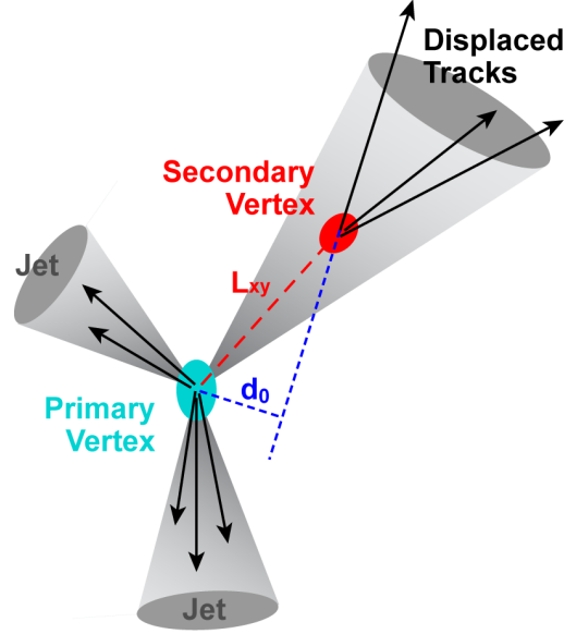
Figure 4.2: Schematic view of identifying a b-jet in the b-tagging algorithm (Abazov et al., 2009)
