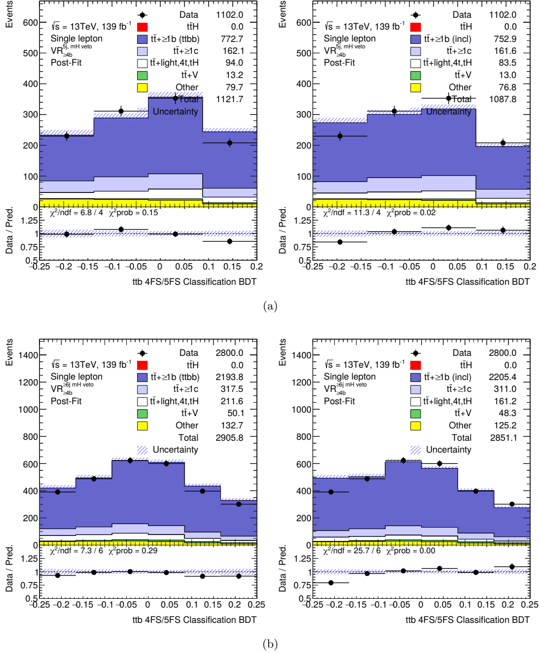
Figure B.1: Distributions of the two validation region used to determine the nominal t\bar{t}+1b sample, (a) the VR_{5j, m_H}^{5j, m_H \text{ veto}} region and (b) the VR_{4b}^{6j, m_H} region. On the left is the t\bar{t}b\bar{b} sample while on the right the t\bar{t} +jets sample, all shown as post-fit plots of a background fit with the corresponding sample used as the t\bar{t}+1b component. Courtesy of Ryunosuke Iguchi.
