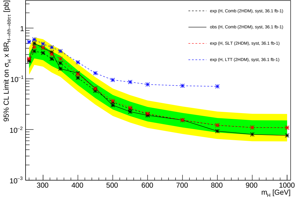
Figure 10.4: Expected (dashed black) and observed (solid black) limits at 95% C.L. on the cross-section times branching ratio of the 2HDM heavy scalar Higgs, H \rightarrow hh \rightarrow b\bar{b}\tau\tau , process when combining the \tau_\ell\tau_{\text{had}} SLT and LTT channels. The expected limits for the SLT (dashed red) and LTT (dashed blue) are also shown separately.
