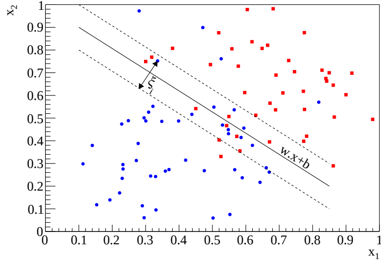
Figure 3.2: Illustration of the soft margin SVM. The slack parameters, \xi_i , allow for misclassification of points weighted by the tunable cost parameter, C . Dotted lines are the margins, with the SVM finding the maximum geometric margin, \gamma .
