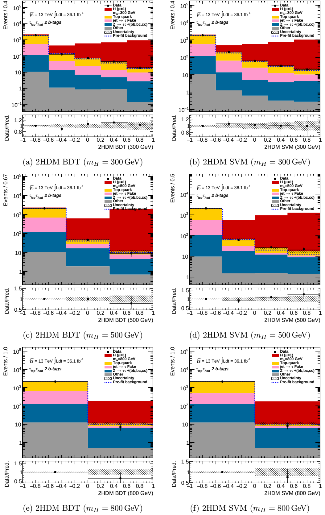
Figure 11.7: MVA output distributions using the optimised binning and after performing the fit, assuming a background only hypothesis, for the BDT (left) and SVM (right) in the \tau_{\ell}\tau_{\text{had}} LTT channel for resonance masses of 300 GeV (top), 500 GeV (middle) and 800 GeV (bottom).
