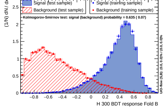
(b) 2HDM ( m_H = 300 GeV) Fold 2
