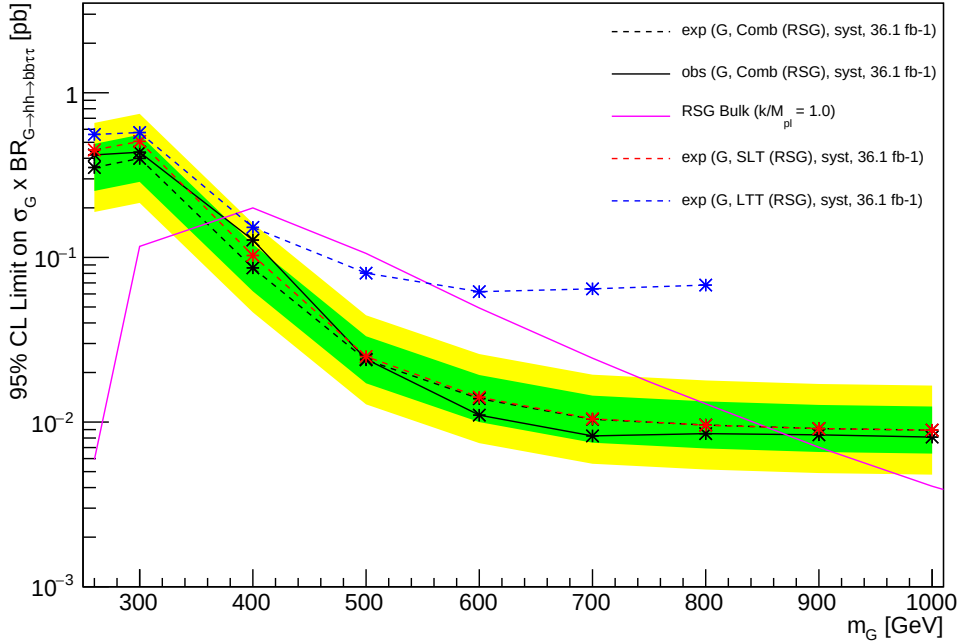
Figure 10.5: Expected (dashed black) and observed (solid black) limits at 95% C.L. on the cross-section times branching ratio of the KK RS graviton, G \rightarrow hh \rightarrow b\bar{b}\tau\tau , process when combining the \tau_\ell\tau_{\text{had}} SLT and LTT channels. The expected limits for the SLT (dashed red) and LTT (dashed blue) are shown separately as well as the expected benchmark cross-section for KK RS graviton production assuming k/M_{Pl} (magenta).
