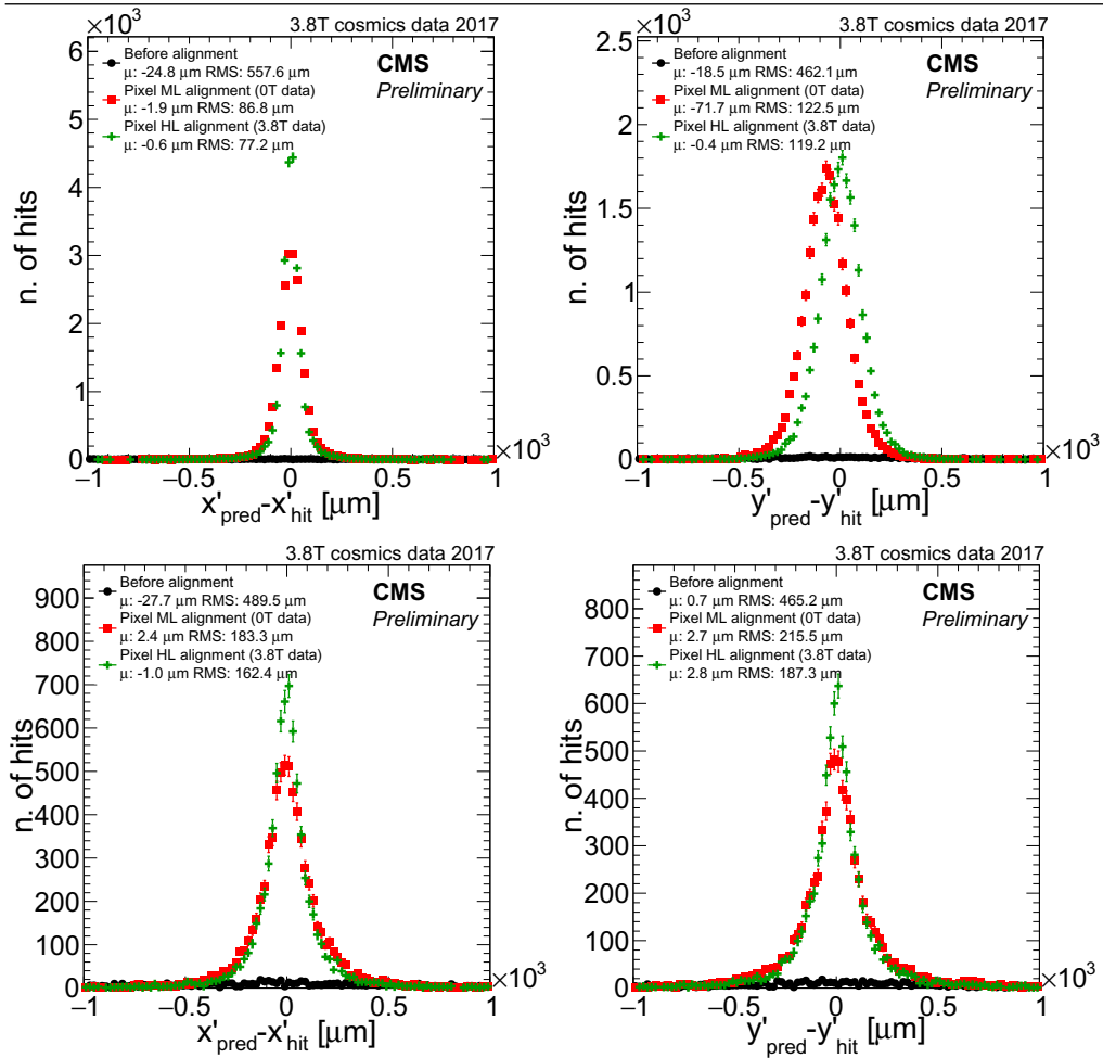
Figure 4.19 Unbiased track-hit residuals in the barrel (top) and forward (bottom) pixel, in the local x (left) and y (right) directions. The distributions are shown for the geometry assumed before performing any alignment (black circles), for the geometry derived with 0T cosmic ray tracks (red squares) and for the alignment derived with 3.8T cosmic ray tracks (green crosses) [125].
