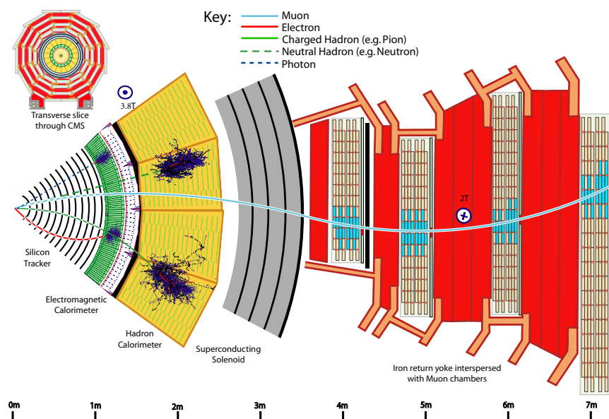
Figure 3.1 A sketch of the specific particle interactions in a transverse slice of the CMS detector, from the beam interaction region to the muon detector [91].
