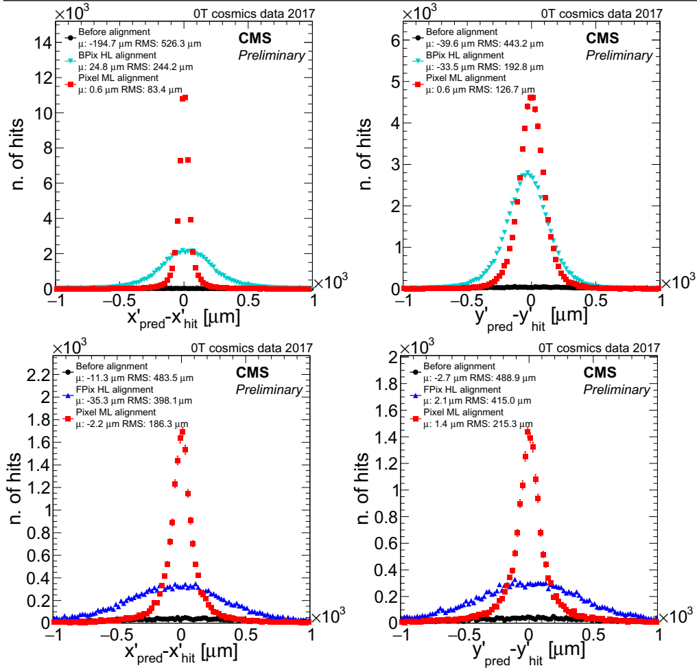
Figure 4.17 Unbiased track-hit residuals in the barrel (top) and forward (bottom) pixel, in the local x (left) and y (right) directions. The distributions are shown for the different alignment iterations performed: the black circles are relative to the geometry assumed before performing any alignment, the triangles are relative to the high level structures alignment of the barrel and forward pixel, and the red squares represent the pixel module level alignment structures alignment. After each alignment iteration, both the bias and the width of the distributions are strongly reduced [125].
