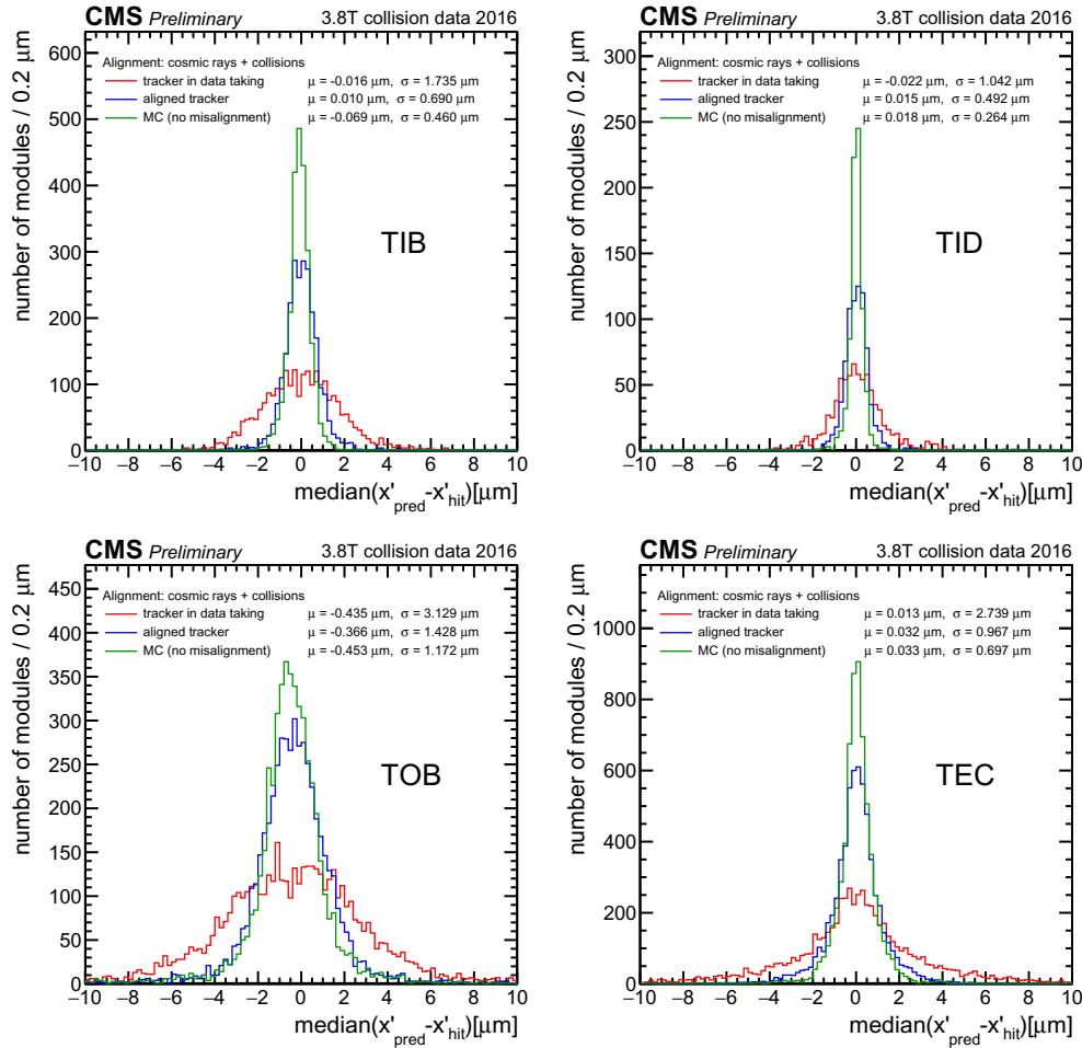
Figure 4.7 The distribution of median residuals along the x' direction for the strip detector subcomponents (TIB, TID, TOB and TEC). Distributions are produced using 1 million collision events collected with the magnetic field at 3.8 T. The red line shows the geometry used in data taking during 2016, while the alignment shown in blue is obtained after the end of the 2016 data taking using 3.8 T cosmic ray and collision data from the whole 2016 pp run. As a reference, the green line shows the distribution obtained from a Monte Carlo simulation, where no misalignment is applied [121].
