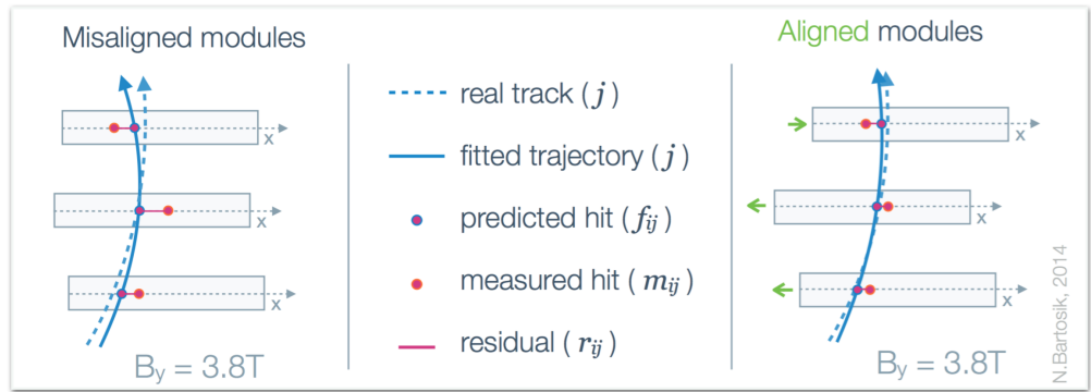
Figure 4.1 Schematic view of the fitted track prediction depending on the alignment of tracker modules. Locally measured hit positions are constant, but their global positions depend on the alignment of the corresponding modules. Misaligned modules pull the measured hit positions away from the real trajectory, leading to an increase of the track-hit residuals and to a distortion of the trajectory [113].
