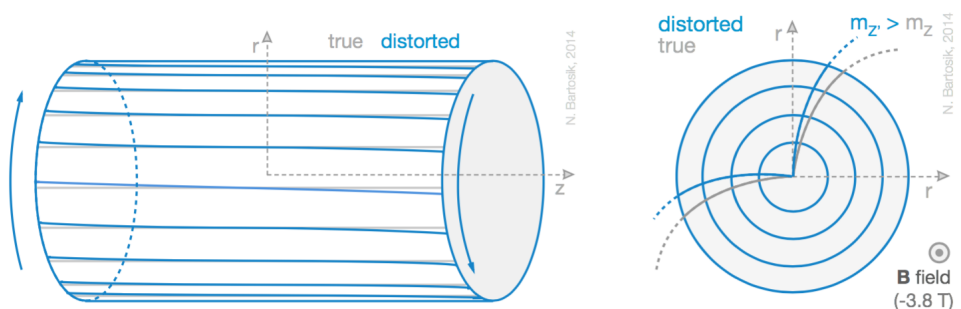
Figure 4.3 Illustration of the twist weak mode, in which \Delta\phi \propto z . The real tracker geometry (grey) is compared with the distorted one (in blue) (left). Tracks can be reconstructed in the distorted geometry without increasing the track-hit residuals by changing the track curvature, and hence the track momentum (right). Track pairs originating from Z boson decays are sensitive to such deformation, as their invariant mass should be compatible with the one of a Z boson [113].
