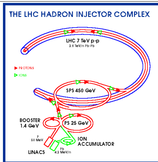
Figure 2.4 The LHC injection chain [51].
