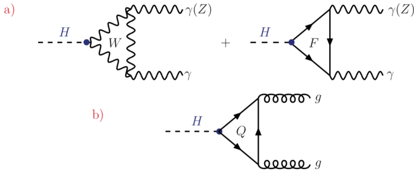
Figure 1.7 Loop-induced Higgs boson decays to \gamma\gamma and Z\gamma (top row) and to gg (bottom row) [29]
