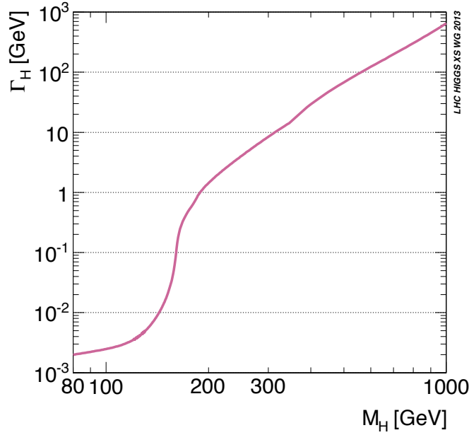
Figure 1.9 Total decay width of the Standard Model Higgs boson, as a function of its mass [40].
