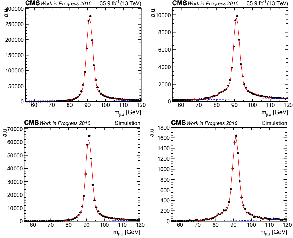
Figure 5.13 Example of fit of the dimuon invariant mass distributions, for muons with 50 < p_T < 60 GeV and |\eta| < 0.9 , for data (top) and Drell-Yan simulation (bottom). The distribution of passing probes (left) and of failing probes (right) are shown. The red line indicates the signal+background fit, while the blue dotted line represents the fitted background.
