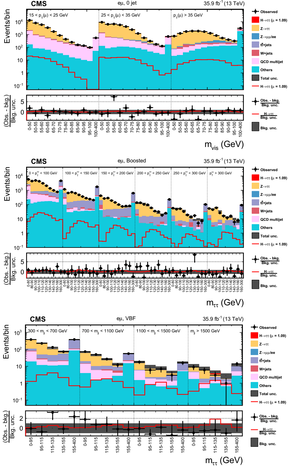
Figure 6.7 Observed and predicted 2D distributions in the e\mu channel, after the final fit, for the 0-jet (top), boosted (middle) and VBF (bottom) categories. The signal distribution is normalised to its best fit signal strength. The uncertainty band includes systematic and statistical uncertainties, after the final fit. The signal is shown both as a stacked filled histogram and an open overlaid histogram. The bottom panel shows the difference between the data and the predicted backgrounds divided by the background uncertainty, and compares it to the fitted H \rightarrow \tau\tau signal [135].
