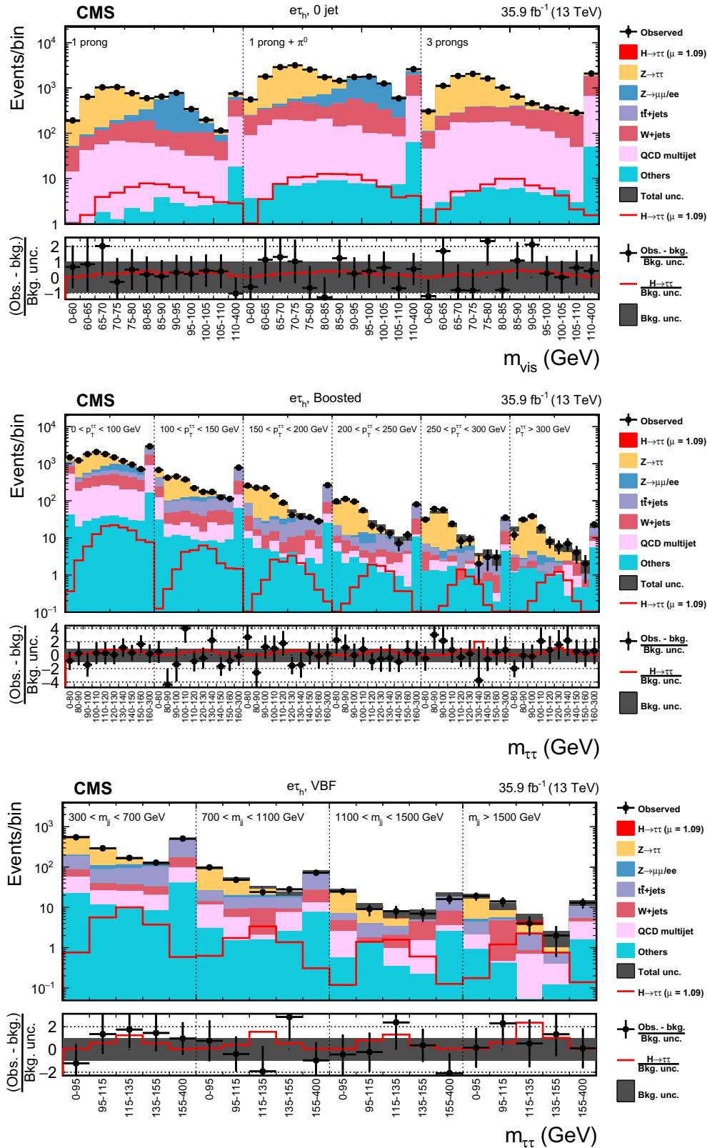
Figure 6.5 Observed and predicted 2D distributions in the e\tau_h channel, after the final fit, for the 0-jet (top), boosted (middle) and VBF (bottom) categories. The signal distribution is normalised to its best fit signal strength. The uncertainty band includes systematic and statistical uncertainties, after the final fit. The signal is shown both as a stacked filled histogram and an open overlaid histogram. The bottom panel shows the difference between the data and the predicted backgrounds divided by the background uncertainty, and compares it to the fitted H \rightarrow \tau\tau signal [135].
