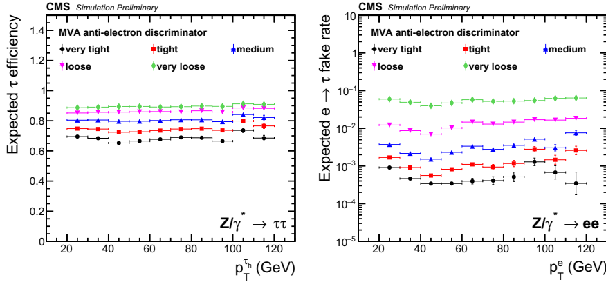
Figure 3.7 Efficiency of the \tau_h identification (left) and e \rightarrow \tau_h fake rate (right) of the anti-electron discriminator from simulated Drell-Yan events, for \tau_h candidates passing the loose MVA-isolation cut [108].
