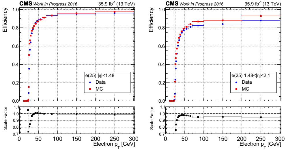
Figure 5.18 Efficiency of the single electron trigger used in the e\tau_h channel, measured with the tag-and-probe method in the full 2016 dataset (blue circles) and in Drell-Yan simulated events (red squares), as a function of the electron p_T in two different \eta regions: |\eta| < 1.48 (left) and 1.48 < |\eta| < 2.1 (right). This trigger has a p_T threshold of 25 GeV, that is indicated by the vertical dashed line. The bottom panel in each plot shows the ratio of the efficiency in data and in simulation. A fine binning in p_T is used especially around the trigger threshold to better model the trigger turn on. The last p_T bin includes electrons with p_T > 200 GeV.
