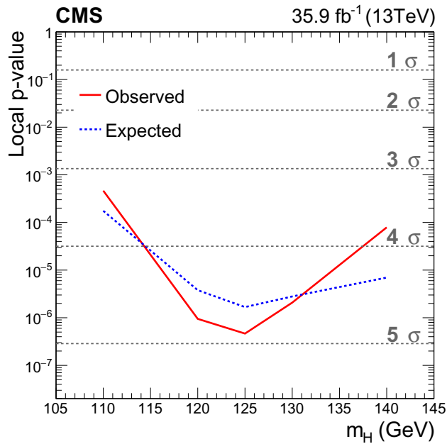
Figure 6.10 Local p -value and significance as a function of the Standard Model Higgs boson mass hypothesis. The observation (red, solid) is compared to the expectation (blue, dashed) for a Higgs boson with a mass m_H = 125.09 GeV: the observed significance is 4.9 \sigma , expected 4.7 \sigma [135].
