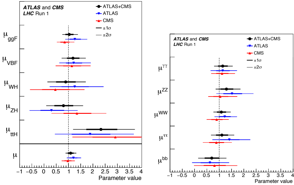
Figure 1.10 Best fit results for the production (left) and decay (right) signal strengths for the combination of ATLAS and CMS Run 1 data, also shown separately for each experiment. The error bars indicate the 1\sigma (thick lines) and 2\sigma (thin lines) intervals [49].
