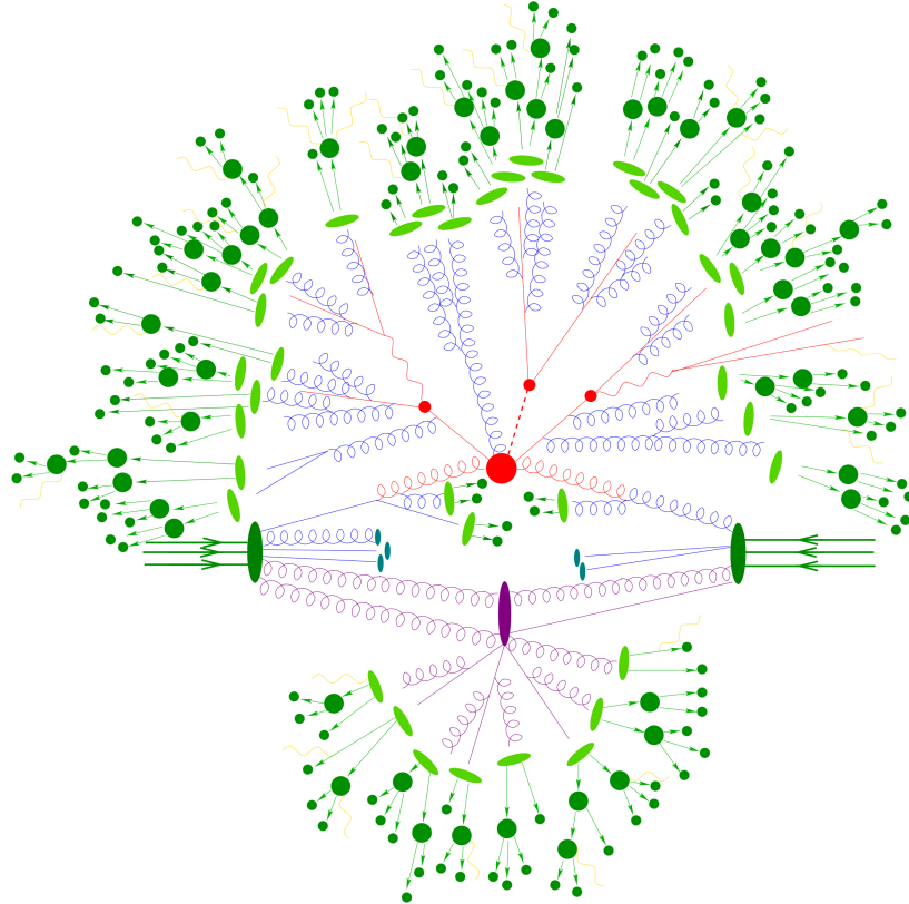
Figure 2.19 Sketch of a t\bar{t}H event produced from a pp collision. The hard scattering process is shown in red. The underlying event comprises additional multiparton interactions, shown in purple, and initial and final state radiation drawn in blue. The hadronisation products are shown in green [77].
