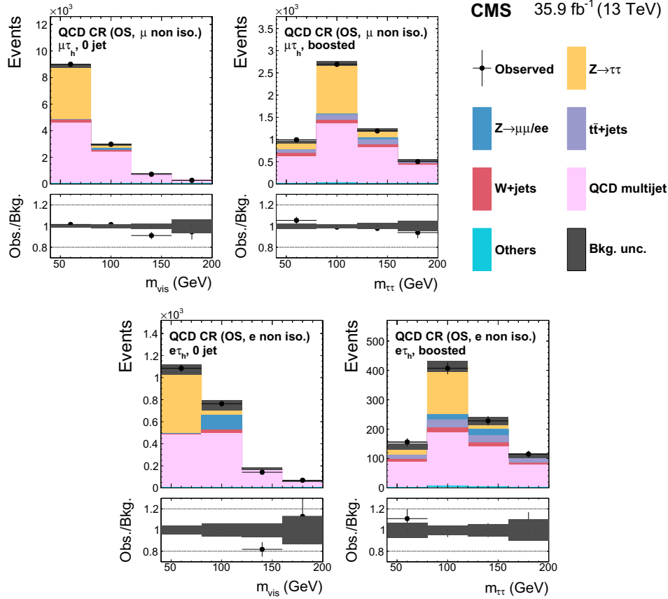
Figure 6.3 Control regions for the QCD background, for the 0-jet and boosted categories of the \mu\tau_h and e\tau_h channels. They are obtained inverting the isolation requirement on the leptons, namely 0.1 < R_{iso}^e < 0.3 for electrons and 0.15 < R_{iso}^\mu < 0.3 for muons [135].
