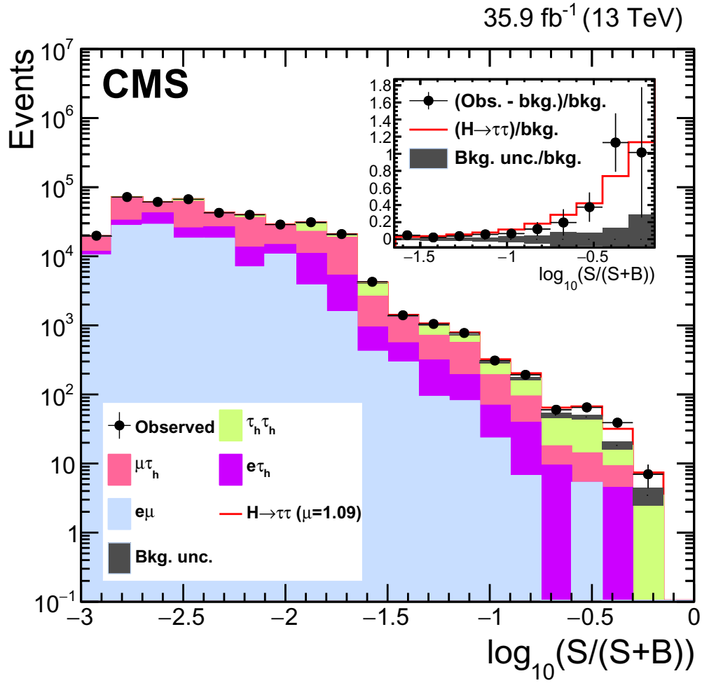
Figure 6.8 Distribution of the decimal logarithm of the S/(S+B) ratio, where S and B are the numbers of expected signal and background events in each bin of the mass distributions, respectively, for the different decay channels. The inset shows the corresponding difference between the observed data and expected background distributions divided by the background expectation, as well as the signal expectation divided by the background expectation [135].
