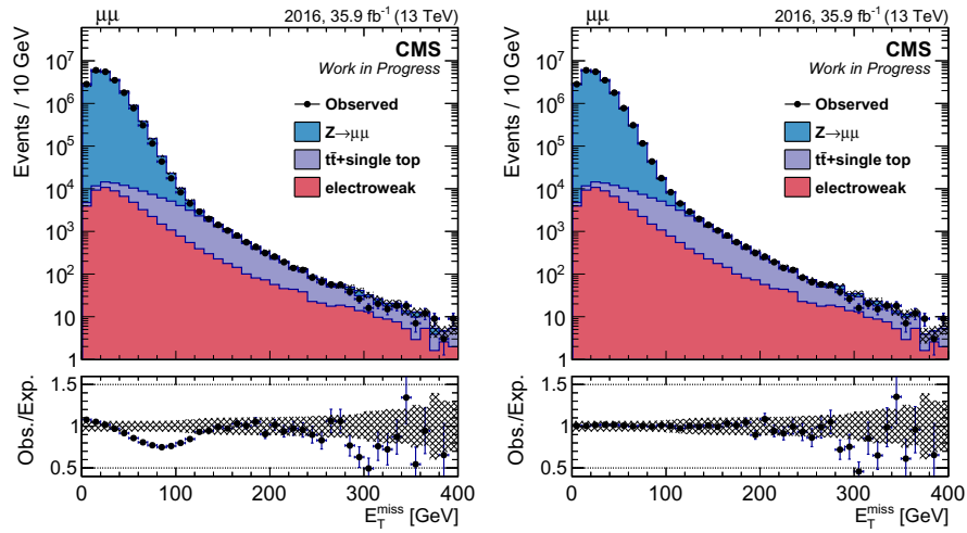
Figure 5.22 Distribution of the E_T^{\text{miss}} variable in Z \rightarrow \mu\mu events, before (left) and after (right) applying recoil corrections. The recoil corrections improve the agreement between data and simulation.
