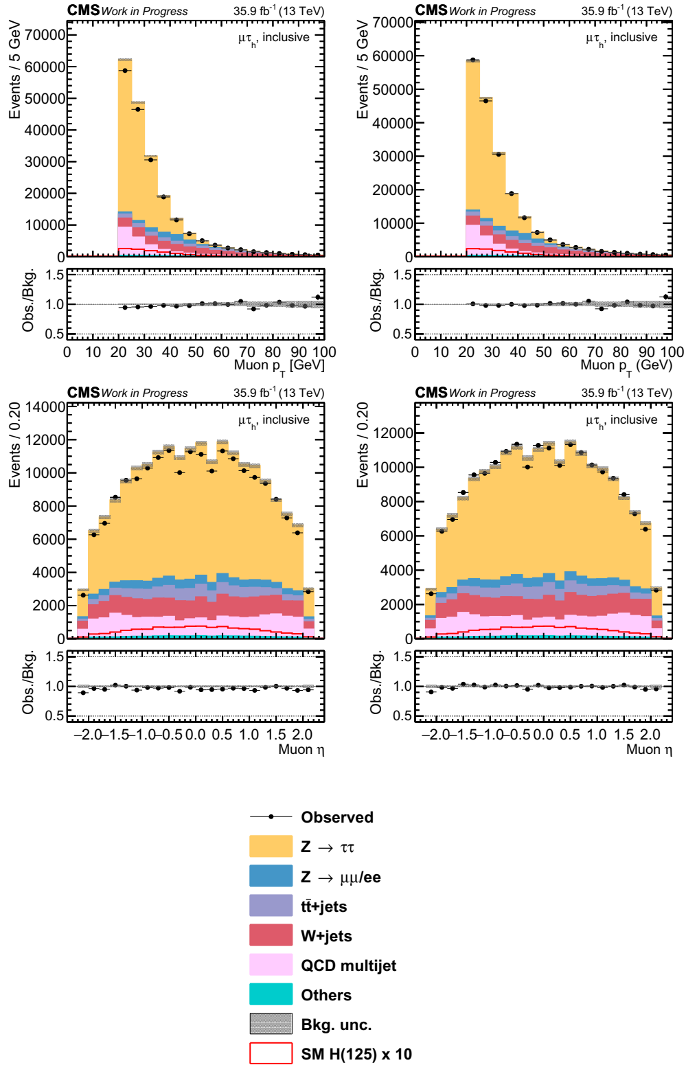
Figure 5.19 Distributions of the muon p_T (top row) and \eta (bottom row), before (left) and after (right) applying the muon identification, isolation and trigger scale factors. Applying the corrections improve the agreement between data and simulation.
