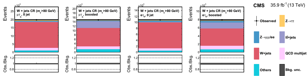
Figure 6.2 Control regions used to derive the normalisation of the W +jets background, for the 0-jet and boosted categories of the \mu\tau_h and e\tau_h channels. During the final fit, the W +jets yield is fitted such to have a perfect agreement between the observed and the expected yields in the high- M_T sideband [135].
