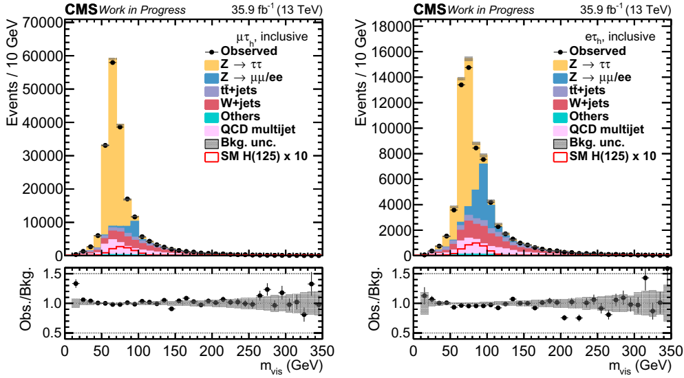
Figure 5.8 Pre-fit distribution of the visible mass for events passing the \mu\tau_h (left) and the e\tau_h (right) channel selection, after applying all simulation corrections. The uncertainty band corresponds to the pure statistical uncertainty.
