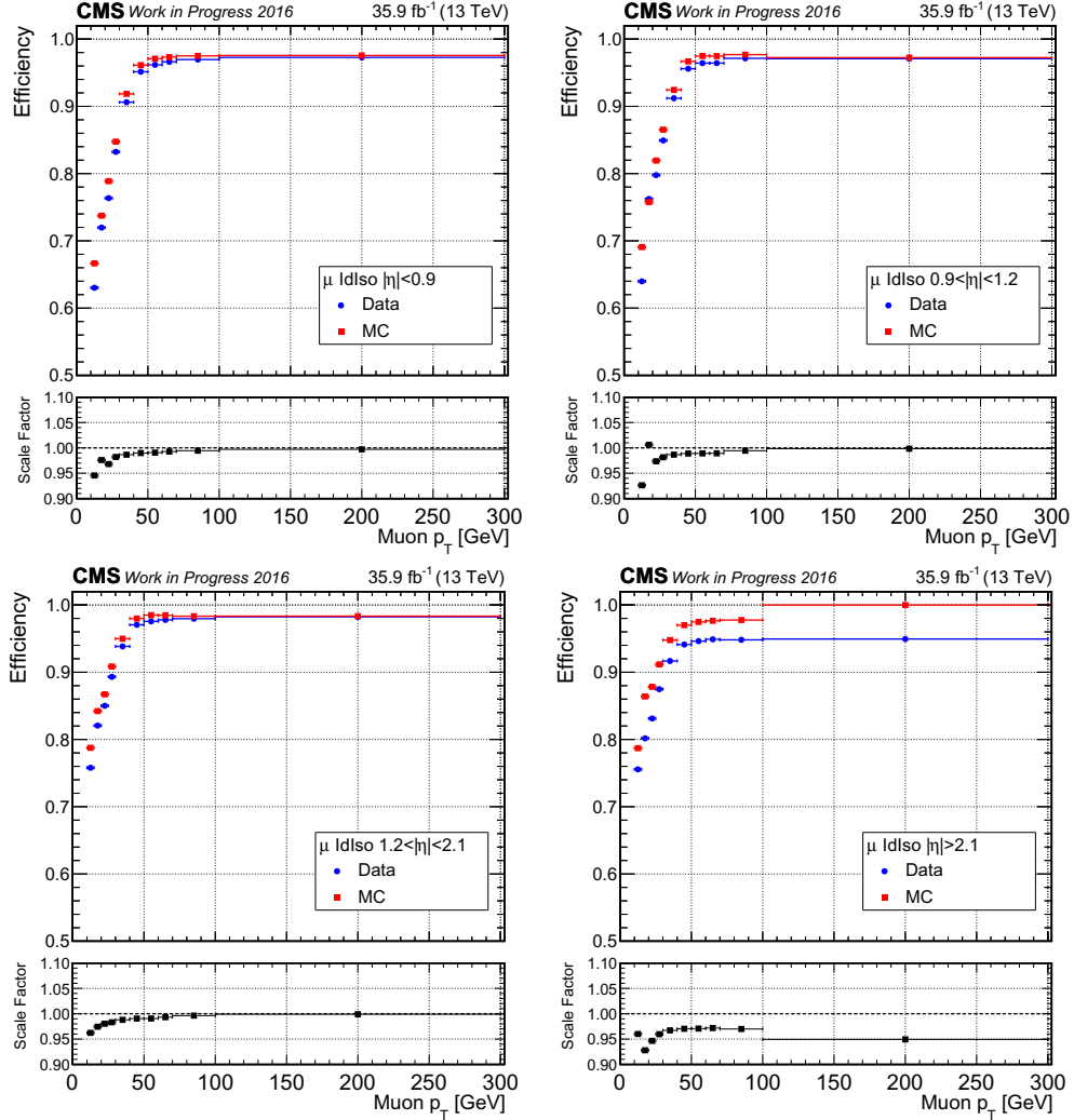
Figure 5.15 Efficiency of the muon identification and isolation criteria used in the \mu\tau_h channel, measured with the tag-and-probe method in the full 2016 dataset (blue circles) and in Drell-Yan simulated events (red squares), as a function of the muon p_T in four different \eta regions: |\eta| < 0.9 (top left), 0.9 < |\eta| < 1.2 (top right), 1.2 < |\eta| < 2.1 (bottom left) and 2.1 < |\eta| < 2.4 (bottom right). The bottom panel in each plot shows the ratio of the efficiency in data and in simulation, which is applied in the analysis as a scale factor to correct simulated events. The last p_T bin includes muons with p_T > 100 GeV.
