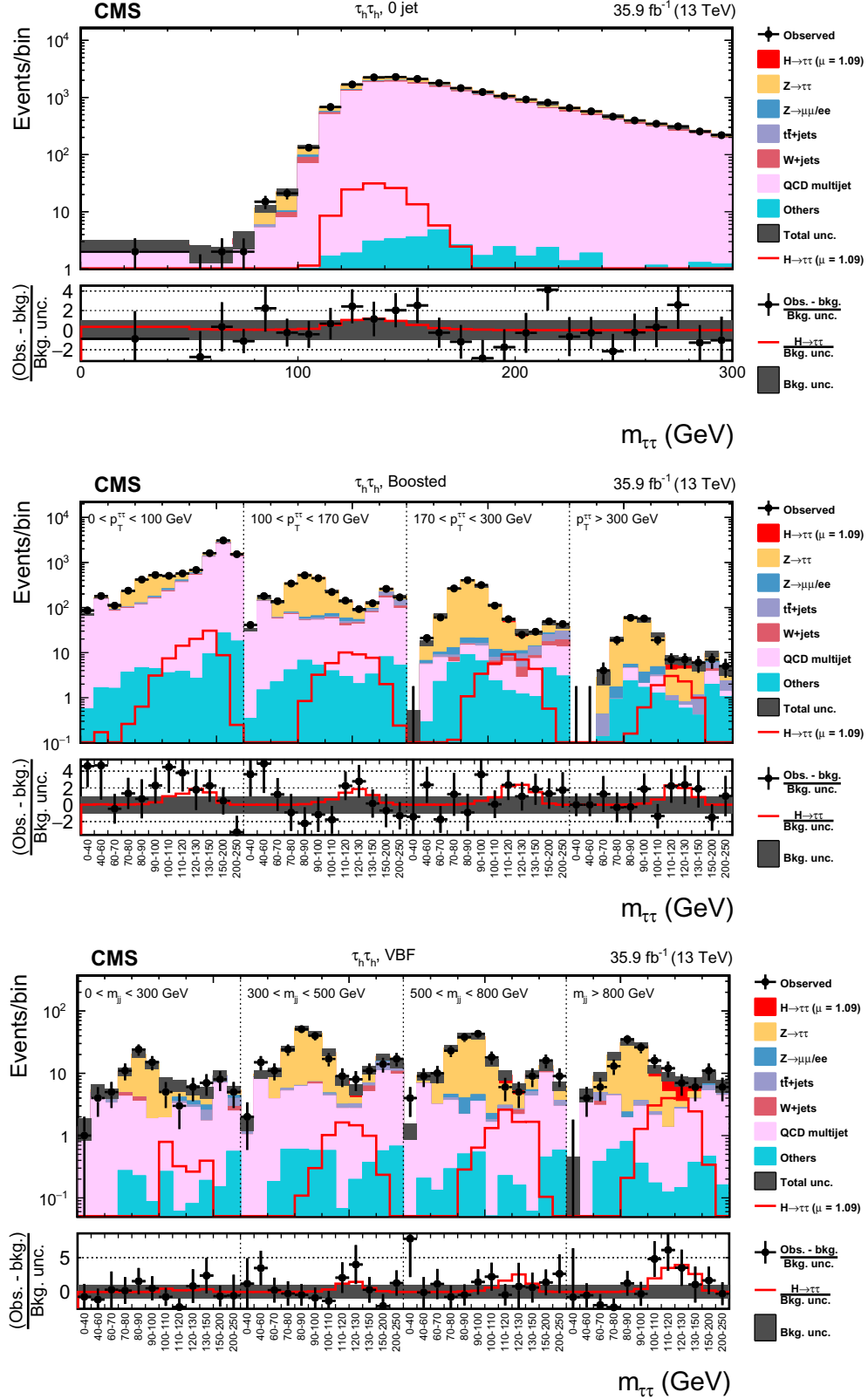
Figure 6.6 Observed and predicted 2D distributions in the \tau_h\tau_h channel, after the final fit, for the 0-jet (top), boosted (middle) and VBF (bottom) categories. The signal distribution is normalised to its best fit signal strength. The uncertainty band includes systematic and statistical uncertainties, after the final fit. The signal is shown both as a stacked filled histogram and an open overlaid histogram. The bottom panel shows the difference between the data and the predicted backgrounds divided by the background uncertainty, and compares it to the fitted H \rightarrow \tau\tau signal [135].
