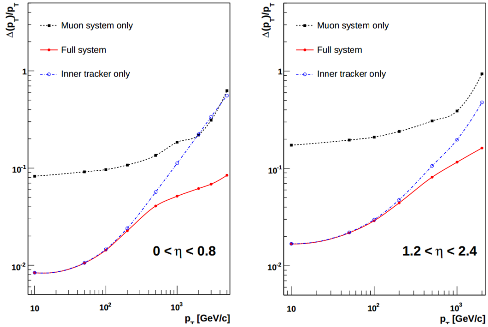
Figure 2.17 Muon transverse momentum resolution, using either the muon system only, the inner tracker only or their combination, in the barrel (left) and endcap (right) regions [56].
