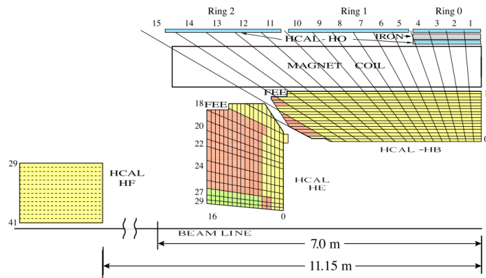
Figure 2.15 Schematic quarter view of the CMS hadronic calorimeter (HCAL) in the barrel (HB and HO), endcap (HE) and forward (HF) regions [73].
