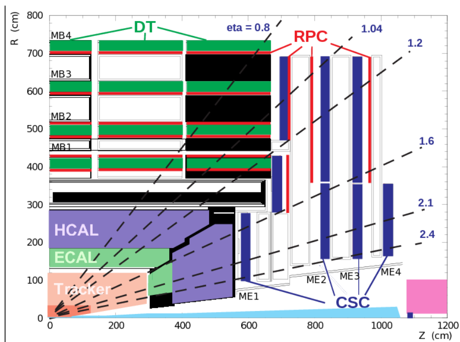
Figure 2.16 Longitudinal layout of one quadrant of the CMS detector. The four DT stations in the barrel (MB1-4, green), the four CSC stations in the endcap (ME1-4, blue), and the RPC stations (red) are shown [74].
