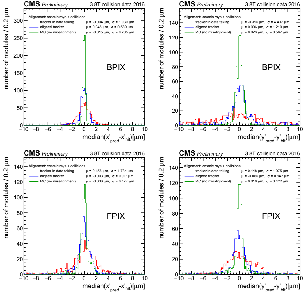
Figure 4.6 The distribution of median residuals along the x' and y' directions for the pixel detector (BPIX and FPIX). Distributions are produced using 1 million collision events collected with the magnetic field at 3.8 T. The red line shows the geometry used in data taking during 2016, while the alignment shown in blue is obtained after the end of the 2016 data taking using 3.8 T cosmic ray and collision data from the whole 2016 pp run. As a reference, the green line shows the distribution obtained from a Monte Carlo simulation, where no misalignment is applied [121].
