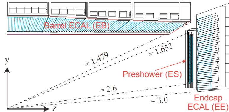
Figure 2.13 Geometric view of one quarter of the ECAL showing the arrangement of crystal modules in the barrel and endcaps region. The preshower detector is placed in front of the endcap [56].
