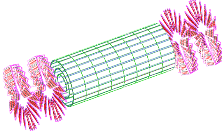
Figure 2.11 View of the CMS pixel tracker, with the three barrel layers (green) and two endcap disks (pink) on each side [68].
