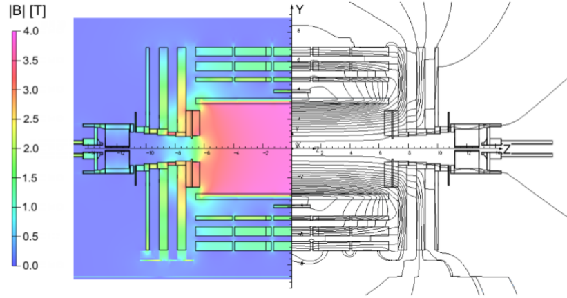
Figure 2.9 The magnetic field strength (left) and lines (right) of the CMS superconducting solenoid. Muon stations are embedded between the yoke layers, where the return field is exploited to bend muons [66].
