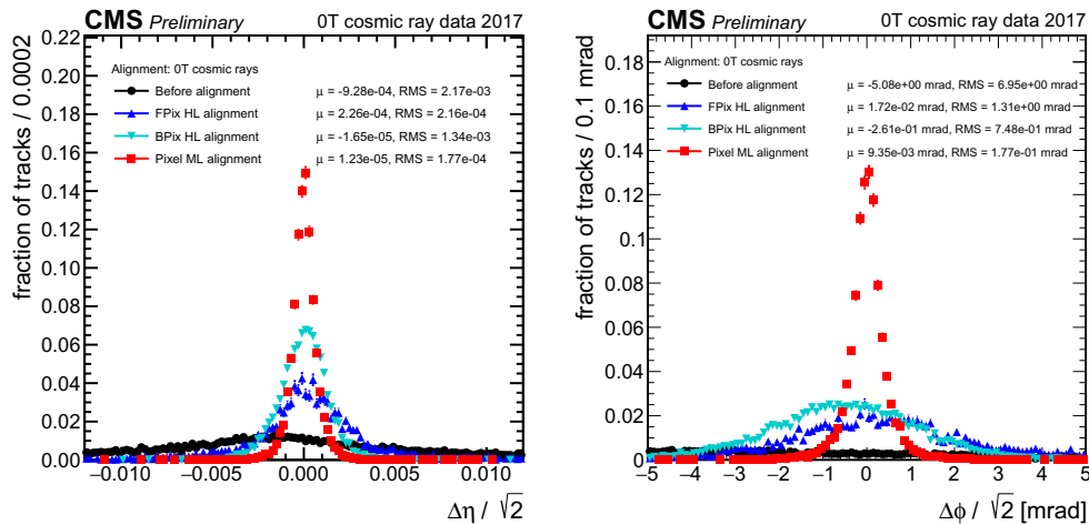
Figure 4.18 Normalised difference between the two halves of a cosmic ray track at 0 T, split at the point of closest approach to the interaction region, in the track \eta (left) and \phi (right). The distributions are shown for the different alignment iterations performed: the black circles are relative to the geometry assumed before performing any alignment, the triangles are relative to the high level structures alignment of the barrel and forward pixel, and the red squares represent the pixel module level alignment structures alignment. After each alignment iteration, both the bias and the width of the distributions are strongly reduced [125].
