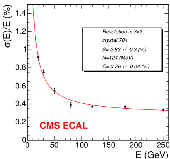
Figure 2.14 Energy resolution of the electromagnetic calorimeter as a function of the electron energy, as measured in a test beam. Measured values of the three parameters in Eqn. 2.4 are listed in the box [72].
