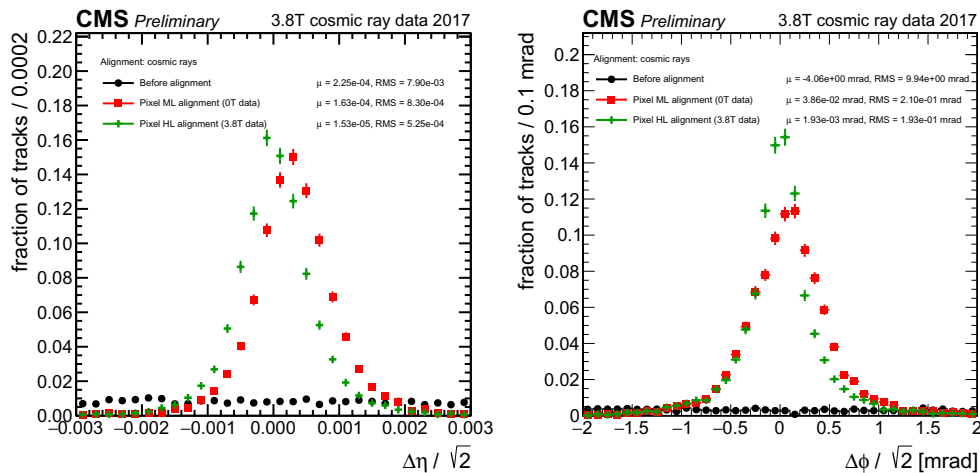
Figure 4.20 Normalised difference between the two halves of a cosmic ray track at 3.8 T, split at the point of closest approach to the interaction region, in the track \eta (left) and \phi (right). After the ramp up of the magnetic field, the positions of the high level structures have been recomputed using 3.8 T cosmic ray tracks. The latter alignment (green crosses) shows improved performance over the geometry derived from 0 T cosmic ray data [125].
