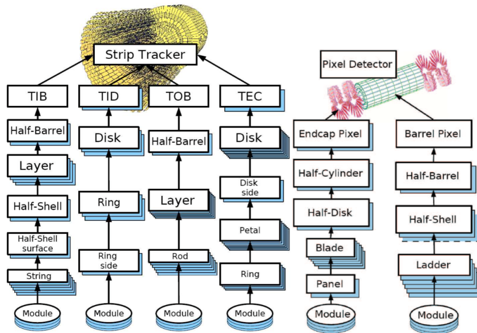
Figure 4.4 Hierarchical structure of the CMS tracker, for the strip (left) [119] and for the pixel detectors [120].
