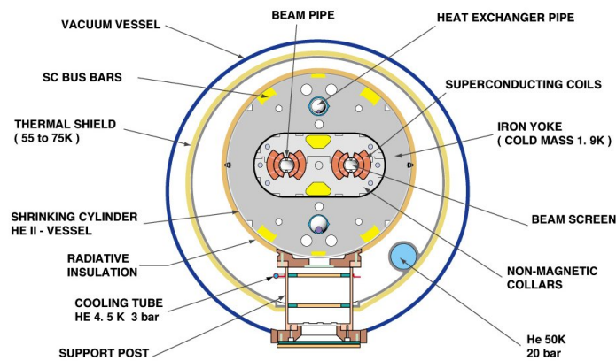
Figure 2.2 Cross section of a LHC dipole magnet showing its structure and features [53].
