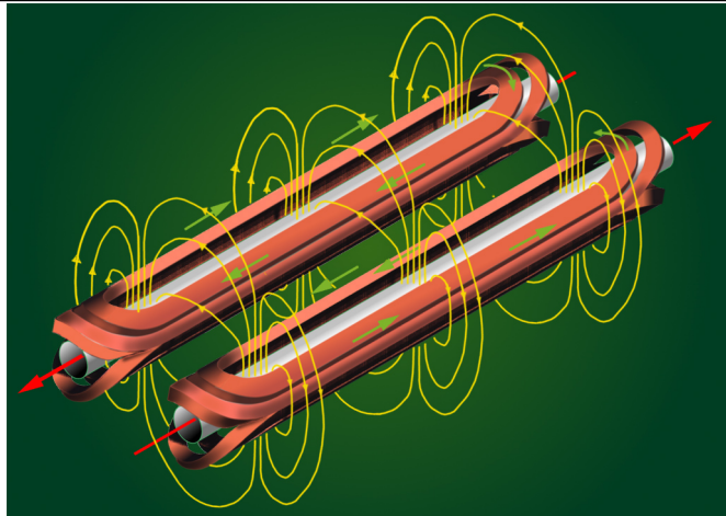
Figure 2.3 Beam pipes and magnetic field lines of the LHC dipole magnets [54].
