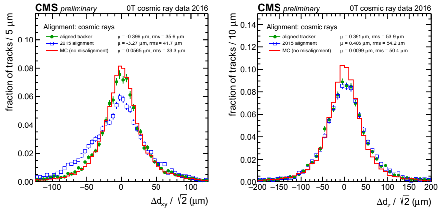
Figure 4.10 The normalised differences between two halves of a cosmic track, split at the point of closest approach to the interaction region, in the track transverse (left) and longitudinal (right) impact parameters, d_{xy} and d_z . The first alignment of the CMS tracker performed in 2016 with cosmic ray data recorded at B = 0 T is compared to the tracker geometry of 2015, which is no longer valid mostly because of temperature and magnetic field changes. The mean and rms values show that the bias is reduced compared to the 2015 geometry, and the precision comes close to the ideal case (from simulation) where no misalignment is included [122].
