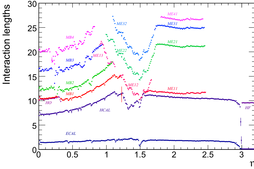
Figure 2.18 Material thickness in interaction lengths after the ECAL, HCAL, and at the depth of each muon station as a function of pseudorapidity [68].
