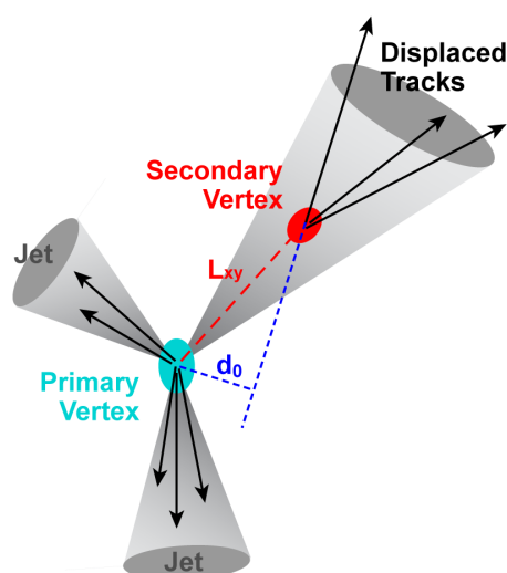
Figure 3.2 A simplified illustration of the structure of a b jet [100]. B hadron decays lead to the presence of displaced tracks with large impact parameters with respect to the primary vertex, and they possibly identify a secondary vertex in the jet due to the sizable lifetime of B hadrons.
