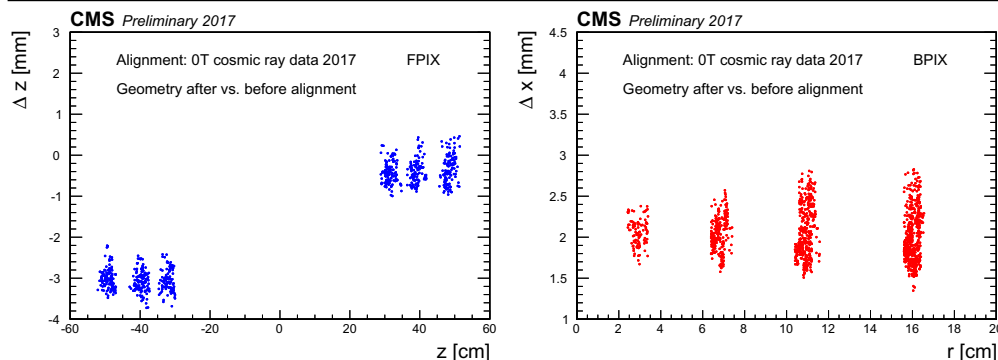
Figure 4.16 Largest corrections after the first pixel high-level structures alignment, for the forward pixel (left) and for the barrel pixel (right). The plots show the modules positions corrections after the alignment, with respect to the geometry before performing any alignment, as a function of the design positions. The alignments were performed with 0 T cosmic ray tracks. In the forward pixel tracker, the largest correction is a shift of \approx -2.8 mm of the z -endcap in the longitudinal direction. For the barrel pixel tracker instead, both half cylinders appear to be systematically misaligned by \approx 2 mm in the horizontal plane along the x direction. Since the detector is also rotated with respect to the geometry assumed before alignment, there is an increasing spread of \Delta x with the radius r [125].
