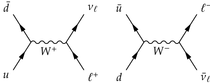
Figure 5.3 Feynman diagrams for the production of W bosons and their leptonic decay, at leading order.
