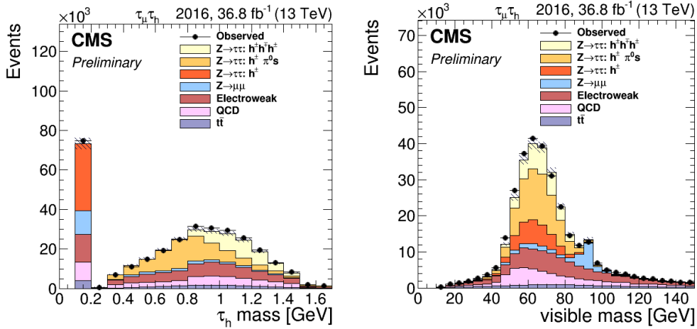
Figure 3.5 Reconstructed visible mass of the \tau_h leptons (left) and of the \mu\tau_h system (right) in Z \rightarrow \tau^+\tau^- events, in 2016 data and in simulation. Simulated events with genuine \tau_h candidates are divided accordingly to their reconstructed decay mode: 3-prong (pale yellow), 1-prong+ \pi^0 (yellow) and 1-prong (orange) [109].
