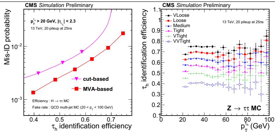
Figure 3.6 Left: misidentification probability \text{jet} \rightarrow \tau_h as a function of the \tau_h identification efficiency estimated from simulation, for different working points of the cut-based and MVA-based isolation discriminators. Right: \tau_h identification efficiency for different working points of the MVA-based isolation, from Z \rightarrow \tau^+\tau^- simulated events. The working points of the MVA-based discriminator are constructed to have a uniform efficiency as a function of p_T [108].
