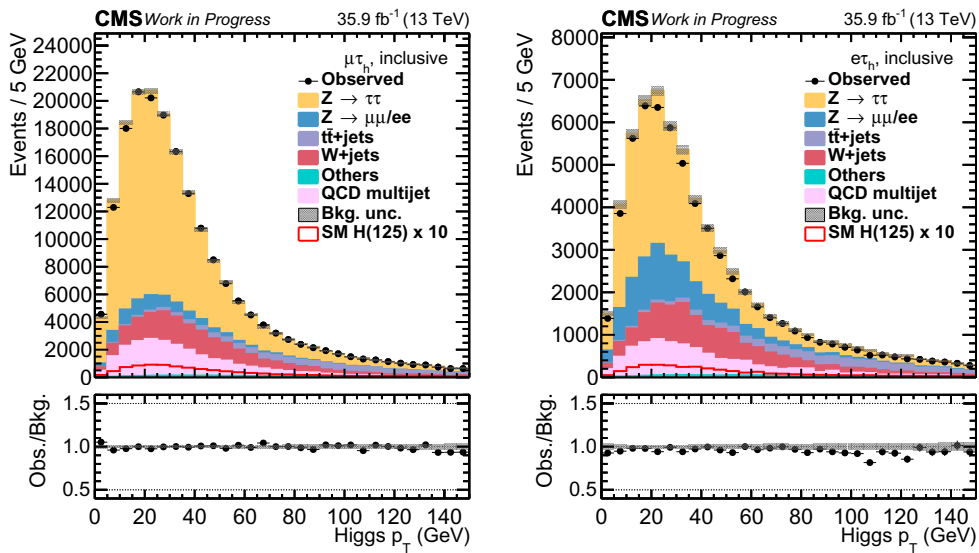
Figure 5.10 Pre-fit distribution of the reconstructed Higgs boson transverse momentum for events passing the \mu\tau_h (left) and the e\tau_h (right) channel selection, after applying all simulation corrections. The uncertainty band corresponds to the pure statistical uncertainty.
