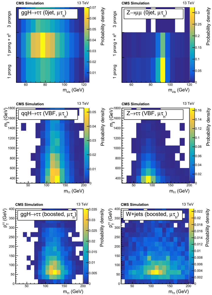
Figure 6.1 Distributions for the signal (left) and for the dominant background processes (right) of the two observables chosen in the 0-jet (top), VBF (centre), and boosted (bottom) categories in the \mu\tau_h channel, demonstrating how the chosen variables help in disentangling the signal from the background. Distributions are obtained from simulated events only, and their binning is not the one used for the final distributions [135].
