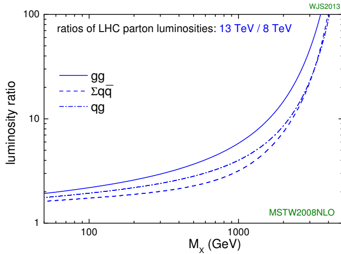
Figure 5.1 Expected ratio of LHC parton luminosities for a centre-of-mass energy of 13 TeV with respect to 8 TeV as a function of the mass of the intermediate resonance M_X [134].
