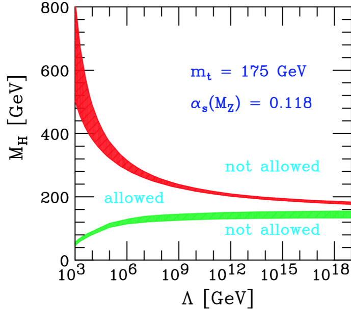
Figure 1.3 Triviality and stability bounds on the Higgs boson mass M_H as a function of the cut-off energy \Lambda_C . The values of the top mass and of the strong coupling constant \alpha_s used are indicated in the plot. The thickness of the bands represents the effect of the uncertainties [34].
