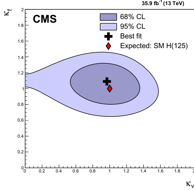
Figure 6.12 Scan of the negative log-likelihood as a function of \kappa_V and \kappa_f , for m_H = 125.09 \text{ GeV} . All nuisance parameters are profiled for each point. For this scan, the H \rightarrow W^+W^- contribution is treated as a signal process [135].
