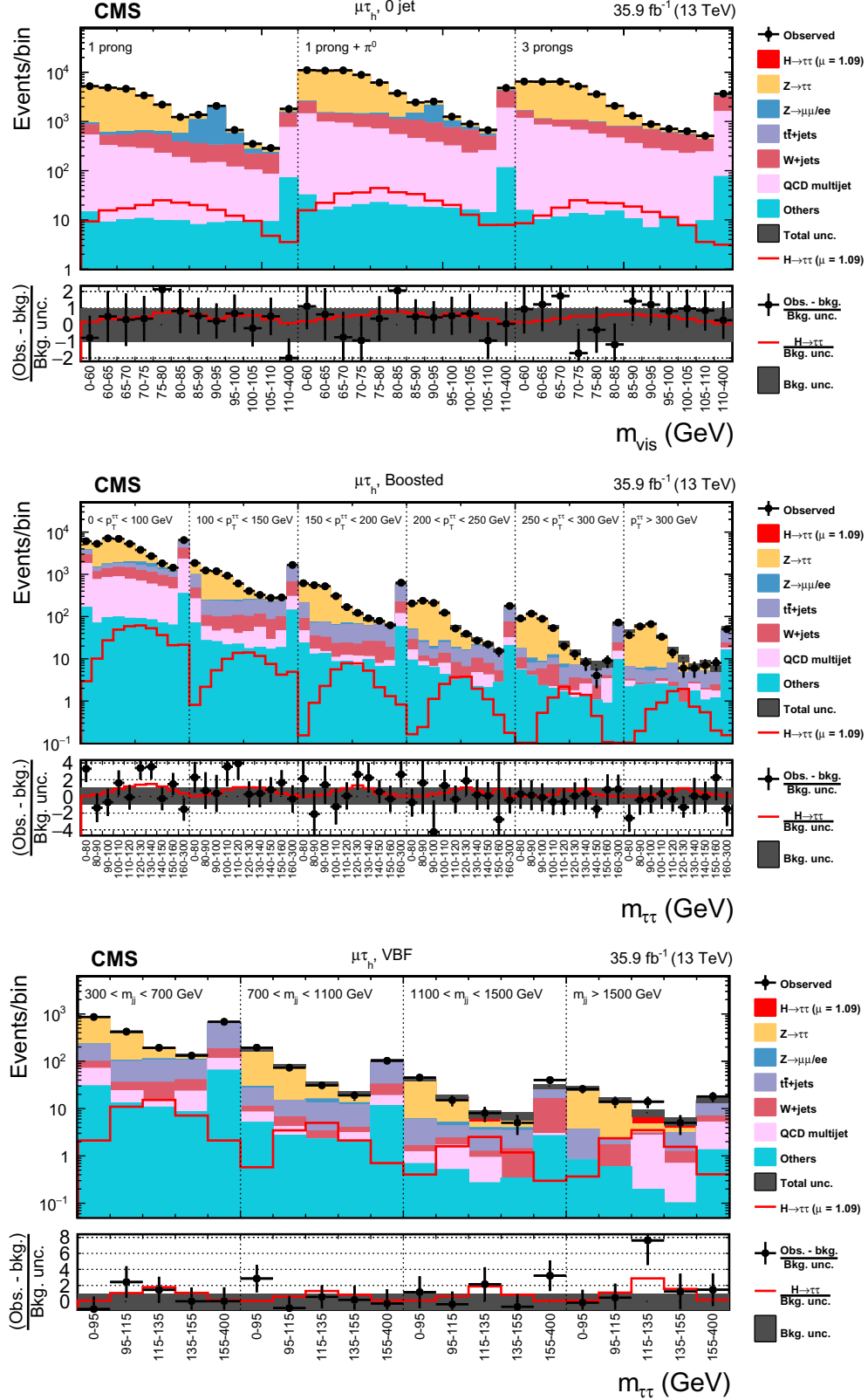
Figure 6.4 Observed and predicted 2D distributions in the \mu\tau_h channel, after the final fit, for the 0-jet (top), boosted (middle) and VBF (bottom) categories. The signal distribution is normalised to its best fit signal strength. The uncertainty band includes systematic and statistical uncertainties, after the final fit. The signal is shown both as a stacked filled histogram and an open overlaid histogram. The bottom panel shows the difference between the data and the predicted backgrounds divided by the background uncertainty, and compares it to the fitted H \rightarrow \tau\tau signal [135].
