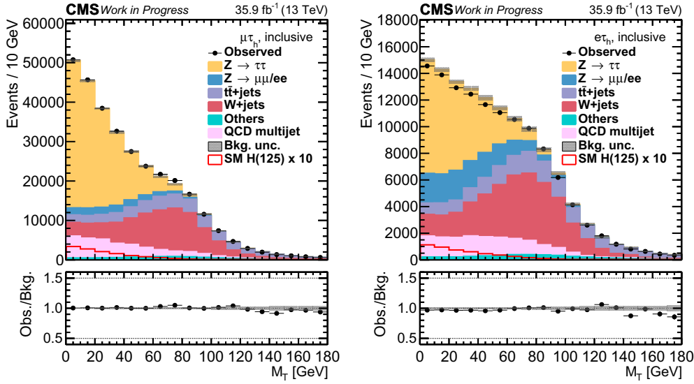
Figure 5.5 Observed and expected distributions of the transverse mass between the muon and the transverse missing energy, calculated according to Eqn. 5.2, in the \mu\tau_h (left) and e\tau_h (right) channels. The uncertainty is statistical only.
