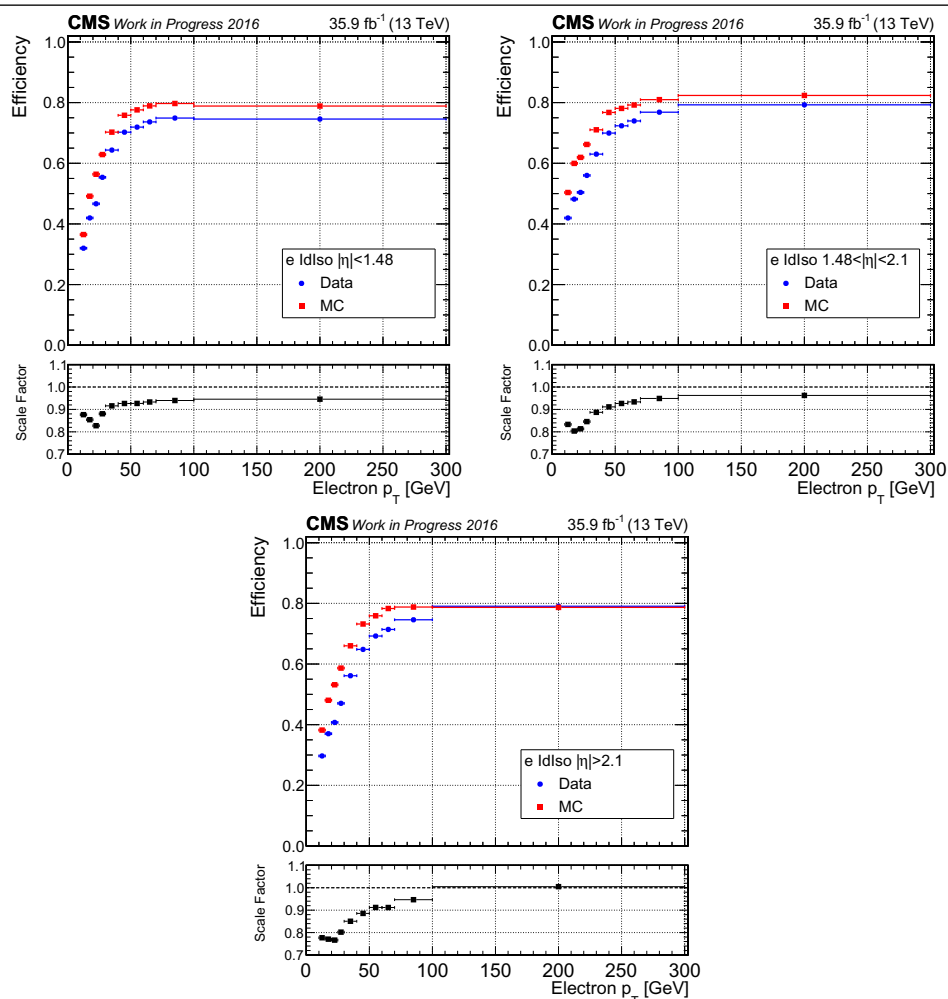
Figure 5.16 Efficiency of the electron identification and isolation criteria used in the e\tau_h channel, measured with the tag-and-probe method in the full 2016 dataset (blue circles) and in Drell-Yan simulated events (red squares), as a function of the electron p_T in three different \eta regions: |\eta| < 1.48 (left), 1.48 < |\eta| < 2.1 (middle), 2.1 < |\eta| < 2.5 (right). The bottom panel in each plot shows the ratio of the efficiency in data and in simulation, which is applied in the analysis as a scale factor to correct simulated events. The last p_T bin includes electrons with p_T > 100 GeV.
