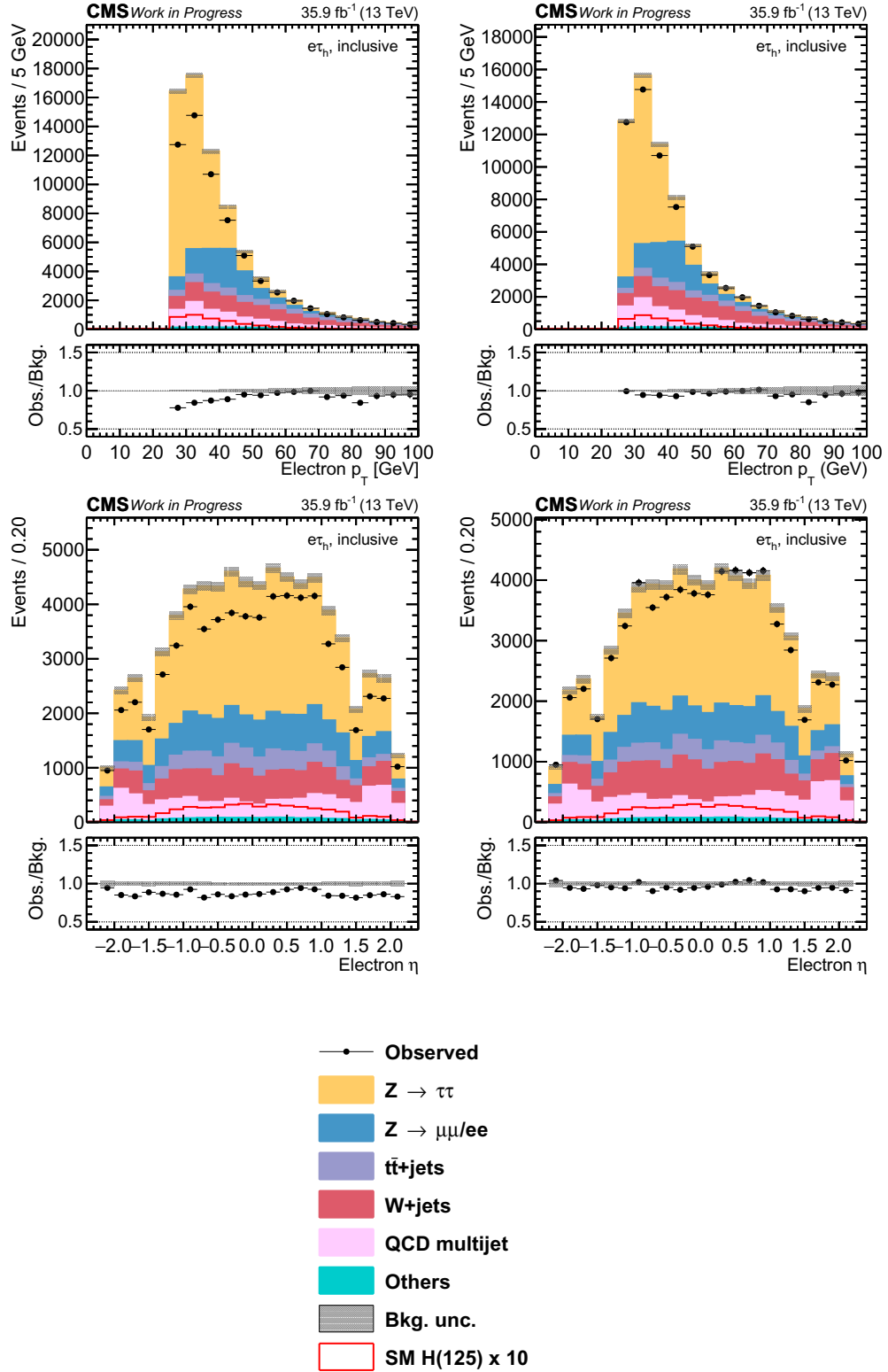
Figure 5.20 Distributions of the electron p_T (top row) and \eta (bottom row), before (left) and after (right) applying the electron identification, isolation and trigger scale factors. Applying the corrections improve the agreement between data and simulation.
