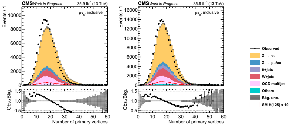
Figure 5.12 Number of primary vertices distributions in data and in simulation, before (left) and after (right) applying the pileup reweighting, for events passing the selection summarised in Table 5.6.
