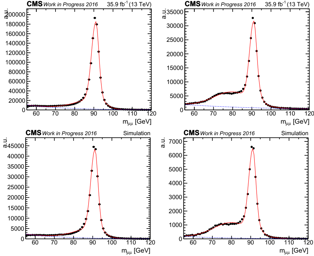
Figure 5.14 Example of fit of the dimuon invariant mass distributions, for muons with 25 < p_T < 30 GeV and |\eta| < 0.9 , for data (top) and Drell-Yan simulation (bottom). The distribution of passing probes (left) and of failing probes (right) are shown. The red line indicates the signal+background fit, while the blue dotted line represents the fitted background. To better fit the distribution of failing probes in this p_T regime, a Gaussian function with its central value shifted to the left of the Z peak is added to the signal template to account for final state radiation events Z \rightarrow \ell\ell + \gamma .
