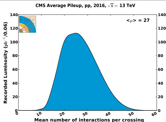
Figure 2.7 Distribution of the mean number of interaction per bunch crossing (average pileup) in the data recorded with the CMS detector in 2016 [64].
