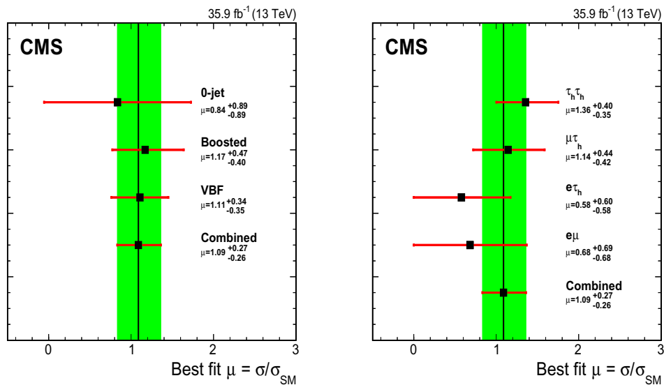
Figure 6.11 Best fit signal strength per category (left) and channel (right), for m_H = 125.09 GeV. The constraints from the global fit are used to extract each of the individual best fit signal strengths. The combined best fit signal strength is \mu = 1.09^{+0.27}_{-0.26} , and it is compatible among categories and channels and with the Standard Model expectation within the uncertainties [135].
