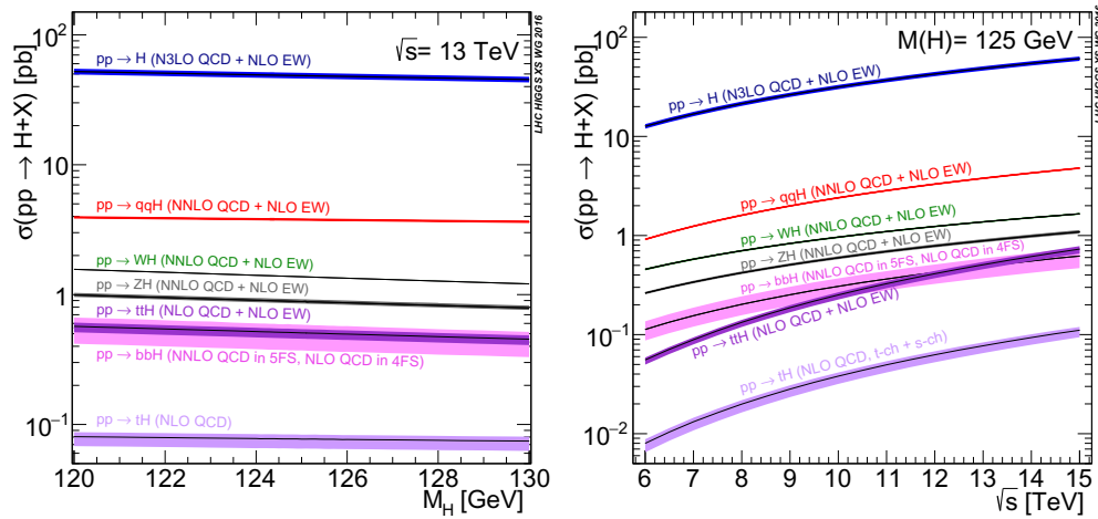
Figure 1.6 Inclusive cross section for the production of a Standard Model Higgs boson from pp collisions, separately for each production mode, as a function of the Higgs boson mass (left) and of the center of mass energy (right). Calculations are performed up to the order indicated in the plot, color bands represent the uncertainty [40].
