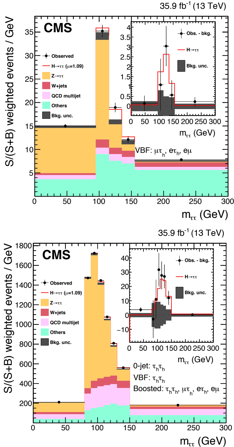
Figure 6.9 Observed and predicted m_{\tau\tau} distributions, combined for the categories with compatible binning, namely the VBF category of the \mu\tau_h , e\tau_h and e\mu channels (top) and the three categories of the \tau_h\tau_h channels and the boosted categories of the \mu\tau_h , e\tau_h and e\mu channels (bottom). The normalisation of the backgrounds and of the signal and the uncertainty are adjusted to the values obtained from the final fit. The mass distributions for a constant range of the second dimension are weighted according to S/(S+B) , where S and B are computed, respectively, as the signal and background contribution in the mass distribution excluding the first and last bins. The inset shows the corresponding difference between the observed data and expected background distributions, together with the signal expectation for the Standard Model Higgs boson [135].
