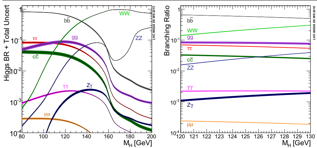
Figure 1.8 Branching ratios of Standard Model Higgs boson decays, as a function of its mass, in the range 80 < m_H < 200 GeV (left), and for 120 < m_H < 130 GeV (right) [40, 42].
