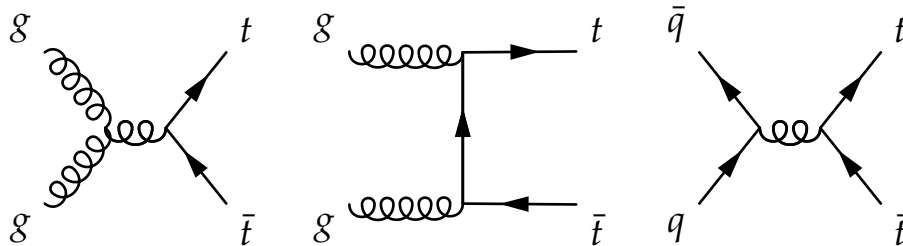
Figure 5.4 Feynman diagrams of t\bar{t} production processes. At the LHC, the dominant production mode is the one initiated by gluon-gluon fusion.
