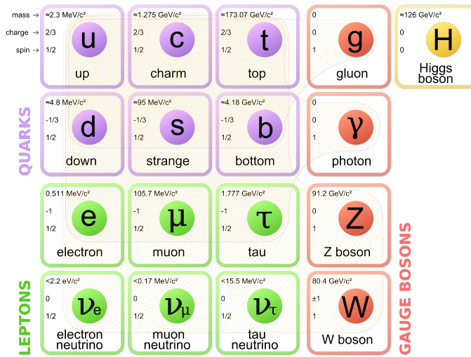
Figure 1.1 Particle content of the Standard Model: quarks, leptons and bosons with their mass, charge and spin values. Picture from Wikipedia.
