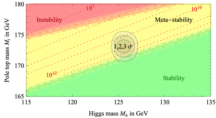
Figure 1.4 Stability of the Higgs potential as a function of the Higgs boson and of the top quark masses [35]. The current measurements of the top quark and of the Higgs boson masses indeed suggest that the electroweak vacuum is metastable. However, for a definite conclusion more accurate measurements especially of the top quark mass are needed.
