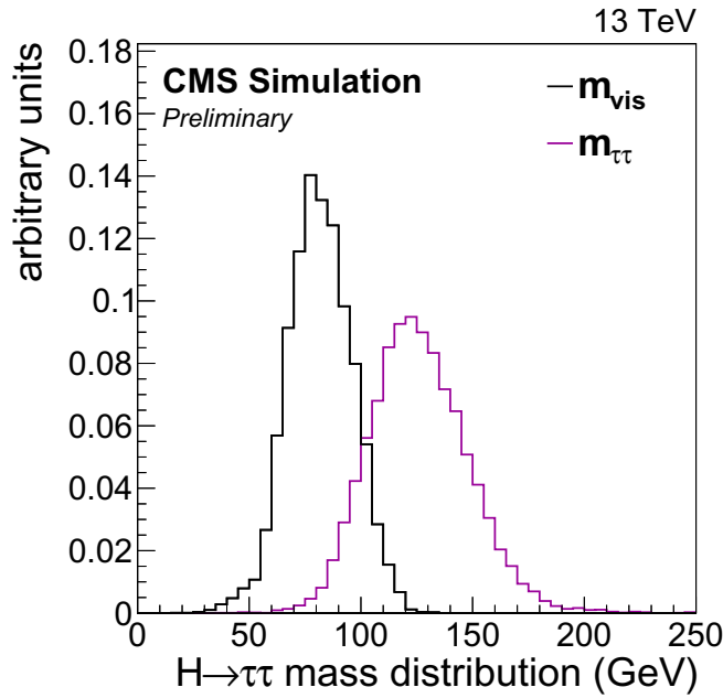
Figure 5.9 Normalised distributions of the visible mass m_{vis} , and of the SVF TT mass, m_{\tau\tau} , for simulated events with a Higgs boson of mass m_H = 125 GeV decaying to a pair of \tau leptons in the \mu\tau_h final state [138].
