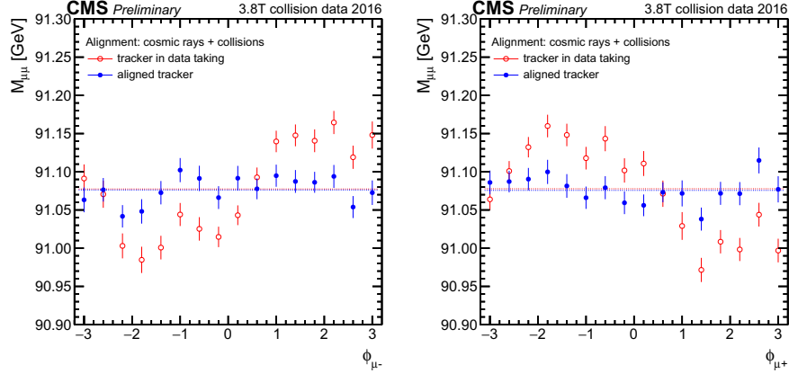
Figure 4.9 Reconstructed Z \rightarrow \mu\mu mass as a function of \phi of the negatively (left) and of the positively (right) charged muons, for the initial alignment used during the 2016 data taking and for the one performed after the 2016 pp run (aligned tracker). A constant function is fitted to illustrate the deviation from the ideal behaviour [121].
