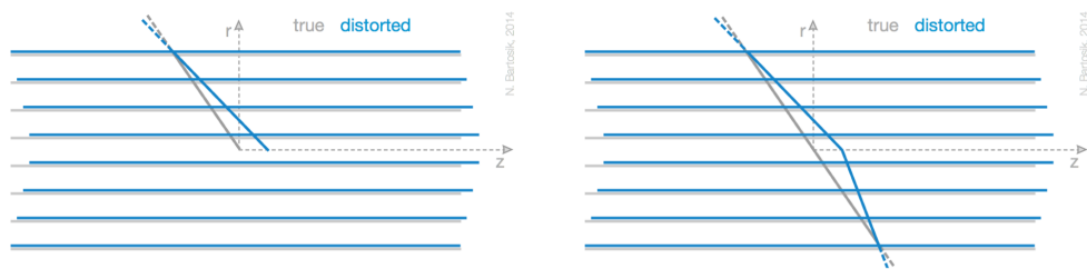
Figure 4.3 Illustration of the twist weak mode, in which \Delta\phi \propto z . The real tracker geometry (grey) is compared with the distorted one (in blue) (left). Tracks can be reconstructed in the distorted geometry without increasing the track-hit residuals by changing the track curvature, and hence the track momentum (right). Track pairs originating from Z boson decays are sensitive to such deformation, as their invariant mass should be compatible with the one of a Z boson [113].
