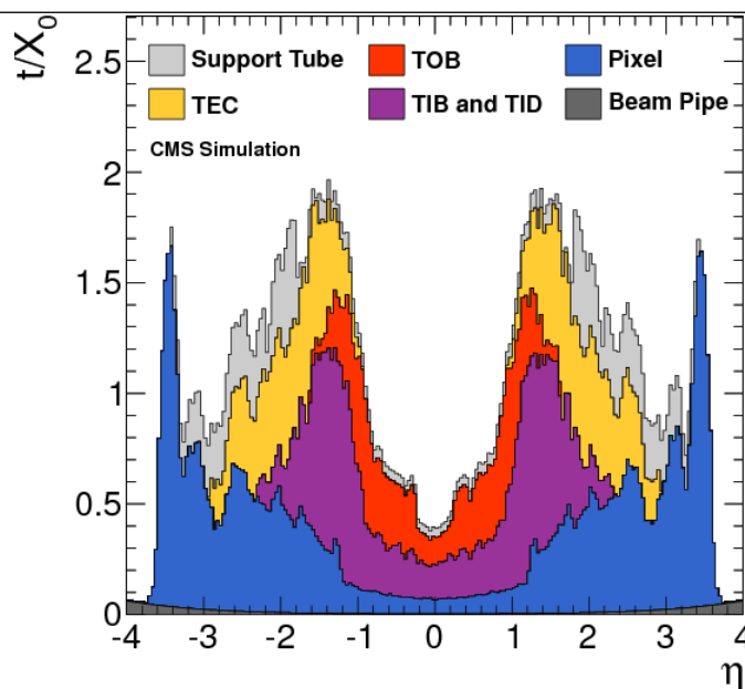
Figure 2.12 Material budget of the CMS tracker in units of radiation length X_0 , as a function of \eta [71].
