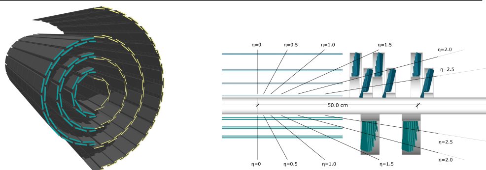
Figure 4.11 The pixel detector geometry before and after the Phase 1 upgrade, in the barrel and in the endcap regions. Left: the original barrel geometry (blue) is placed aside the upgraded four-layer geometry (yellow). Right: the previous tracker design (bottom) compared to the upgraded geometry (top) [124].
