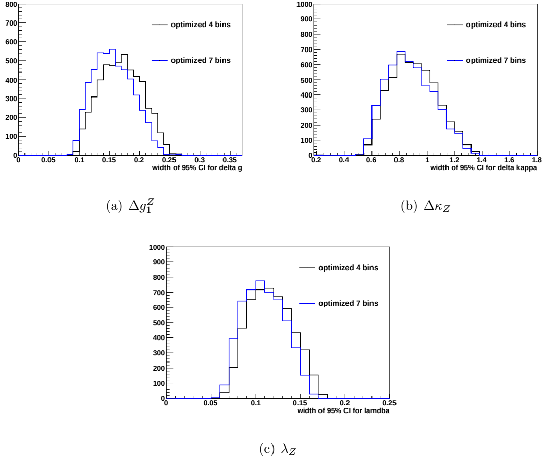
Figure 11.4: Expected aTGC limits from 7 versus 4 bins. The 95% confidence interval widths corresponding to limits extracted by setting delta log-likelihood = 1.92 in 5000 toy experiments for each aTGC parameter. The distribution of widths extracted from the optimized 4 bin (black) and optimized 7 bin (blue) p_T^Z binnings are compared. The cut-off scale is 2 TeV for this comparison.
