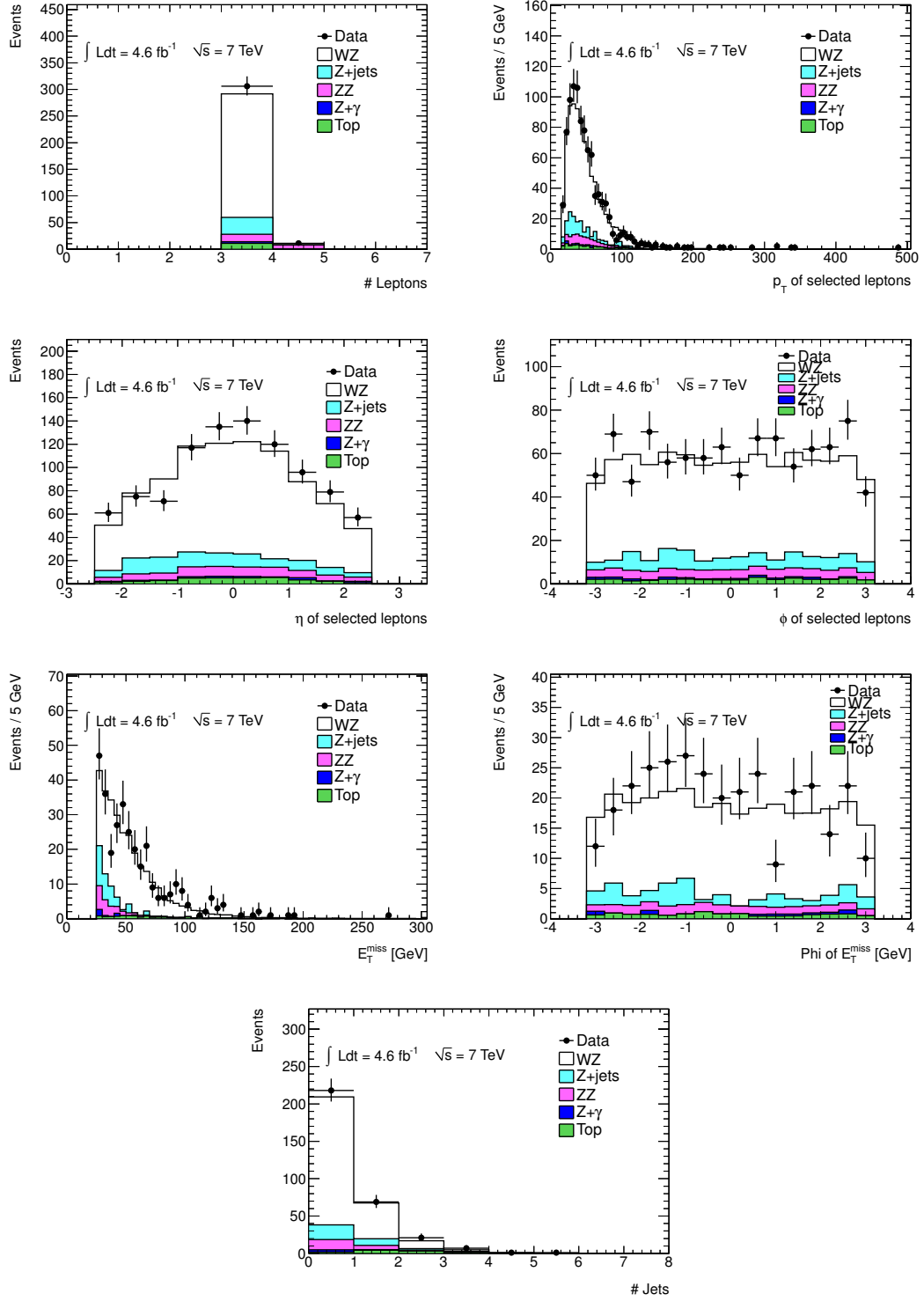
Figure 10.2: Selected kinematic distributions for events in the selected WZ sample. The Z+\text{jets} and t\bar{t} backgrounds are MC normalized by data-driven estimates.
