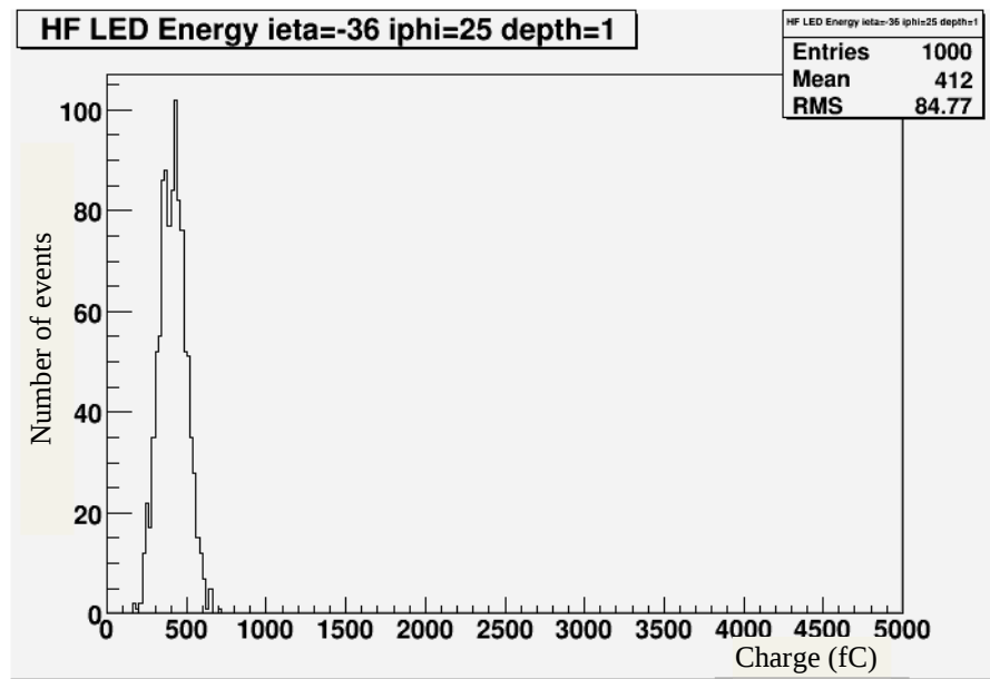
Figure 6.1. LED energy of channel ieta – iphi: 36/25, long fibers for run 101915
