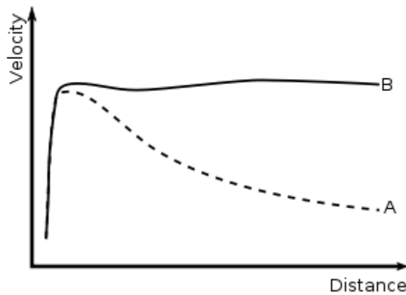
Figure 3.4. Velocity versus distance curve for spiral galaxies, according to Vera Rubin's studies: the predicted curve (A) and the observed one (B)
