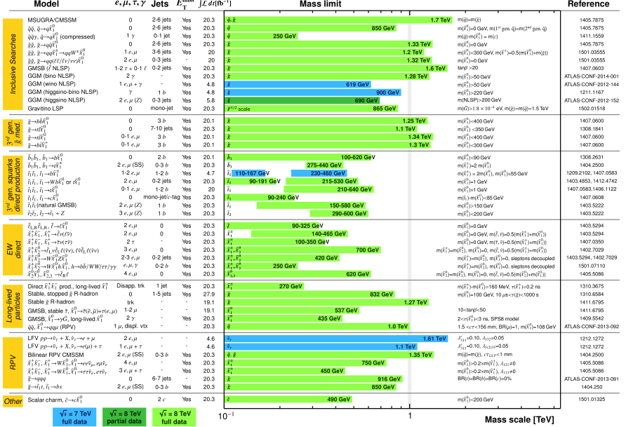
Figure 11.7.: The current lower limits on the production particles in various SUSY scenarios [90] (Status at 2015 February). Limits on long lived particles are set for a number of models including RPV with the results from the DV + \mu search in 2014 [62] (The summary plot has not been updated to include results published after February 2015). Comparable mass-limits are set for prompt RPV.
