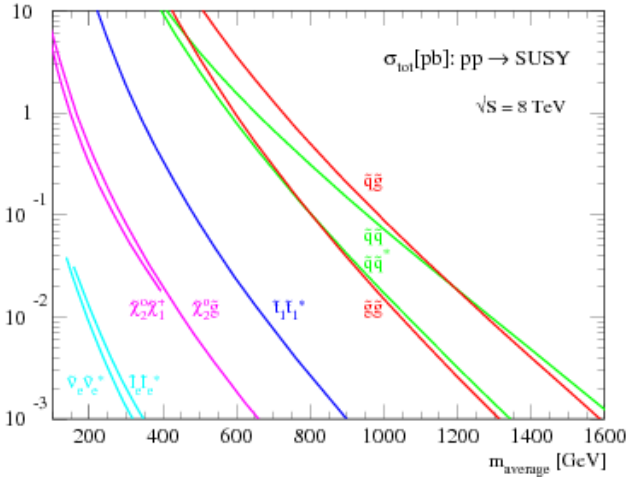
Figure 2.7.: The expected cross-sections for production of SUSY particles at the LHC for an average mass m_{\text{average}} at \sqrt{s} = 8 TeV. [24]
