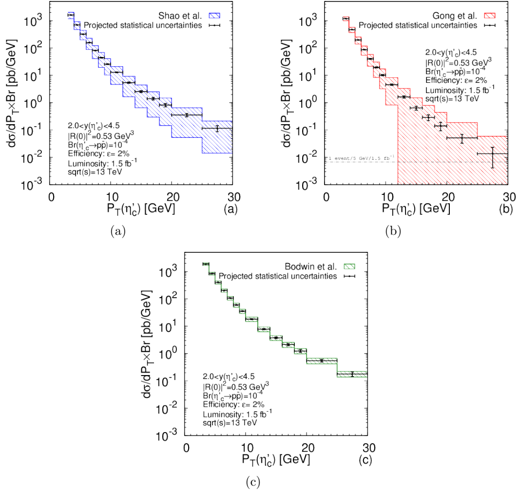
Figure 2.16: The NRQCD predictions of the p_T -differential \eta_c(2S) production cross-section for the LHCb fiducial region at \sqrt{s} = 13 \text{ TeV} from Refs. [119] (a) [117] (b) [133] (c). Figure is taken from Ref [132].
