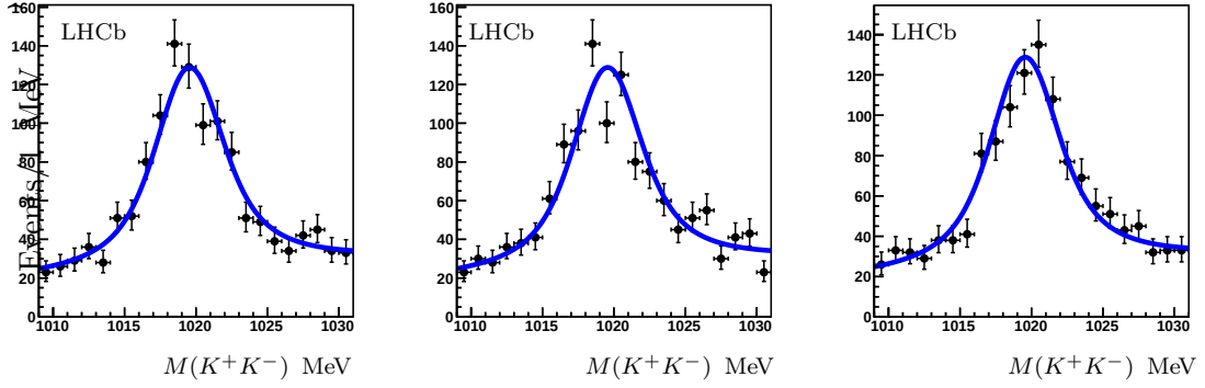
Figure 9.4: Projections of the entire sample of the \phi\phi\phi candidates 3D fit on each \phi candidate.
