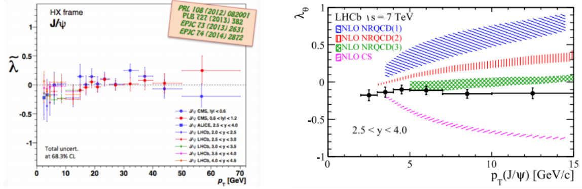
(a) J/\psi polarisation measurements at LHC [102, 103, 115]. (b) LHCb measurement compare to theory [115].
