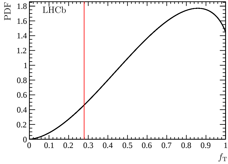
Figure 9.13: The PDF for the fraction of transverse \phi meson polarization f_T for the B_s^0 \rightarrow \phi\phi\phi candidates. The 95% Bayesian lower limit is shown by the red vertical line.
