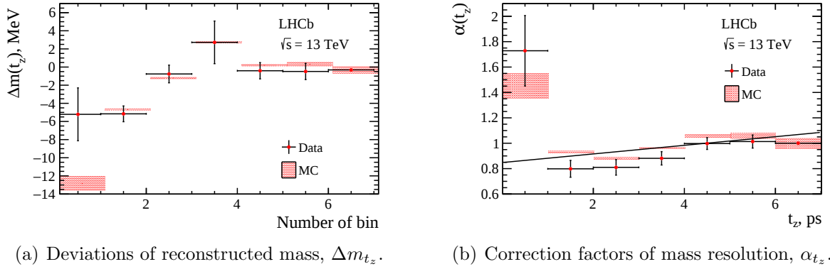
Figure 5.5: Mass deviations (a) and correction factors of mass resolution (b) as a function of t_z bin number from simultaneous fit to the \eta_c and J/\psi invariant masses in the MC samples in bins of t_z (red boxes) and from fit to total p_T -integrated data sample (black points with error bars).
