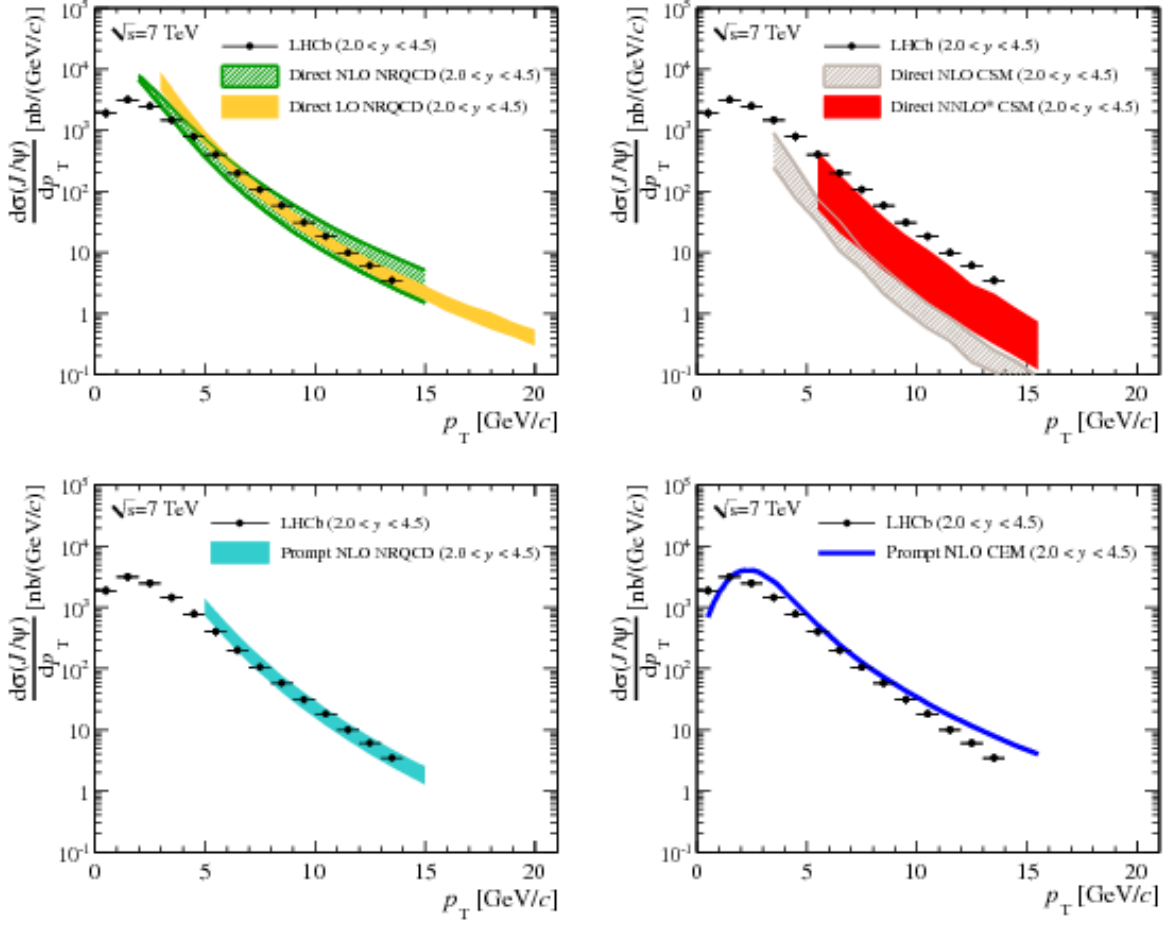
Figure 2.6: The p_T -differential cross-section of prompt J/\psi production at LHCb at \sqrt{s} = 7 TeV compared to theory: direct NLO and LO NRQCD (top left), NLO and NNLO CS model (top right), prompt NLO NRQCD (bottom left), CEM (bottom right) [92].
