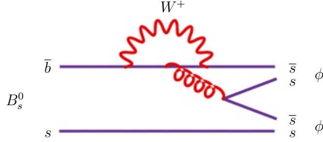
Figure 9.1: Quark diagram describing B_s^0 \rightarrow \phi\phi decay.
