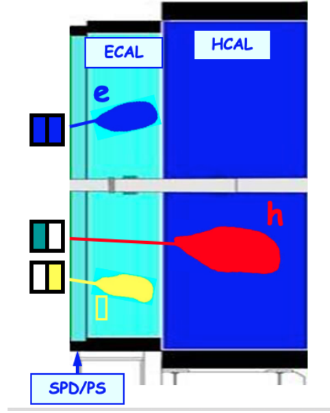
Figure 4.13: Principle of PID with the LHCb calorimeter system comprising PS, SPD, ECAL and HCAL. Hadronic (red) and electromagnetic (yellow and blue) showers are illustrated.
