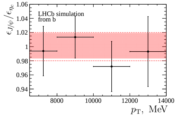
(b) The efficiency ratio for production in b -decays.
