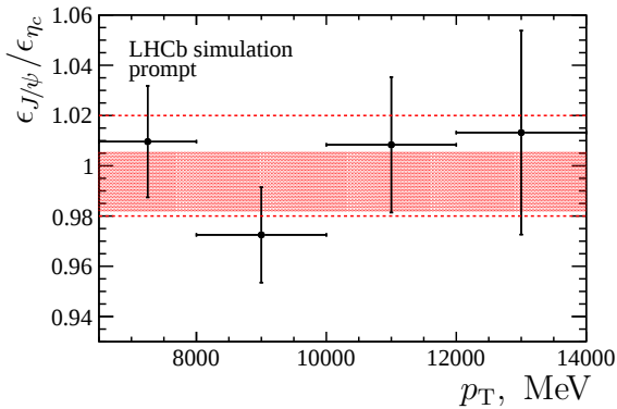
(a) The efficiency ratio for prompt production.
