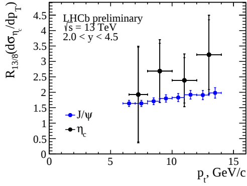
(a) Prompt production.
