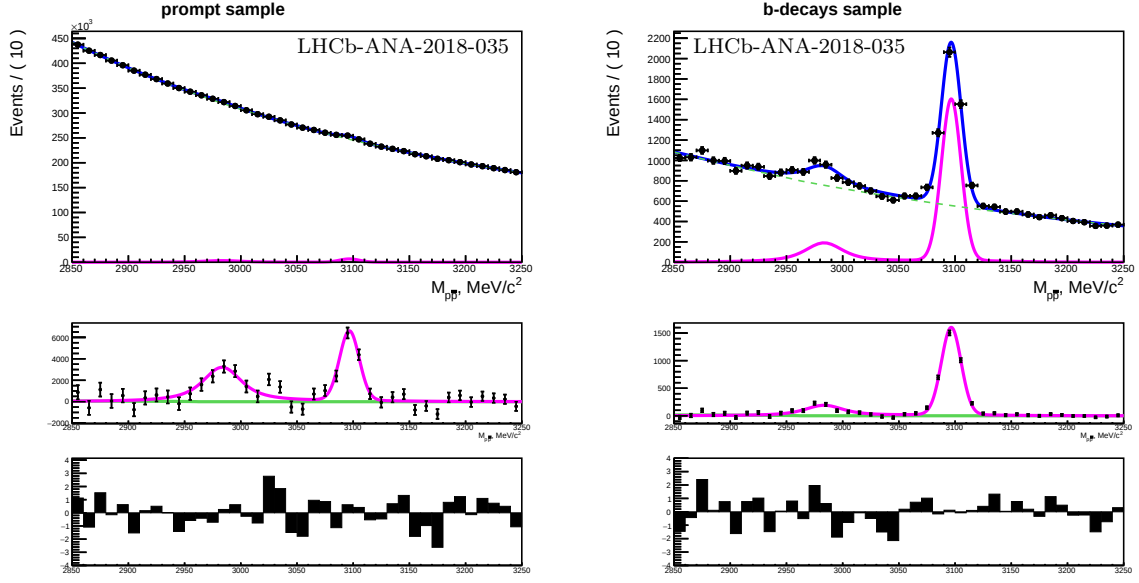
Figure 5.33: The M_{p\bar{p}} distribution for prompt (left) and b -decays (right) for (10.0 \text{ GeV} < p_T < 12.0 \text{ GeV}) . The solid blue lines represent the fit result. Magenta and green lines show the signal and background components, respectively. The corresponding residual and pull distributions are shown below.
