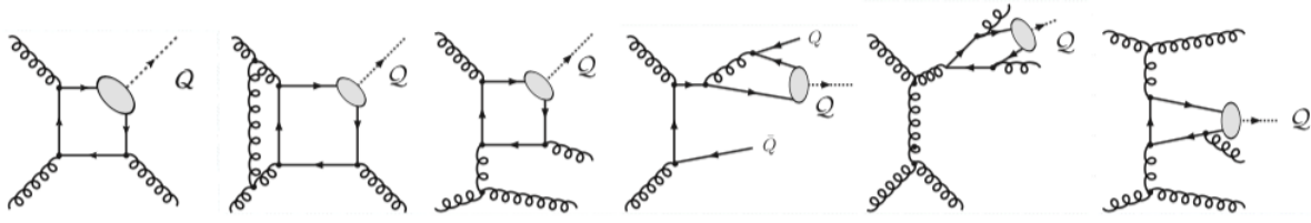
Figure 2.18: Diagrams representing J/\psi hadroproduction within CS mechanism. Figure is taken from Ref. [64].
