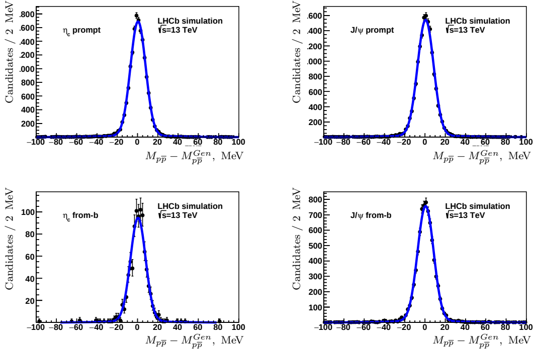
Figure 5.2: Distribution of the M_{p\bar{p}} - M_{p\bar{p}}^{Gen} value in the MC samples: prompt \eta_c (top left), prompt J/\psi (top right), \eta_c from b -decays (bottom left) and J/\psi from b -decays (bottom right). The solid blue lines represent a simultaneous fit by a double Gaussian function to all four MC samples.
