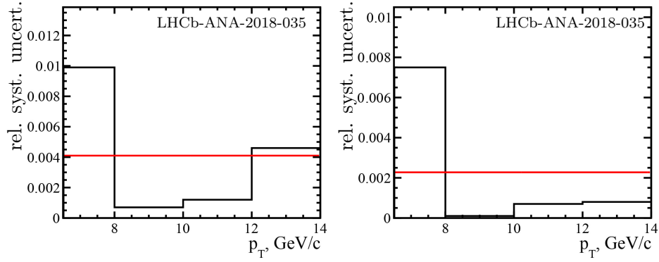
Figure 5.35: The relative systematic uncertainty due to the p_T -dependence of \eta_c and J/\psi resolution ratio in bins of p_T . The solid red line shows a smoothing curve.
