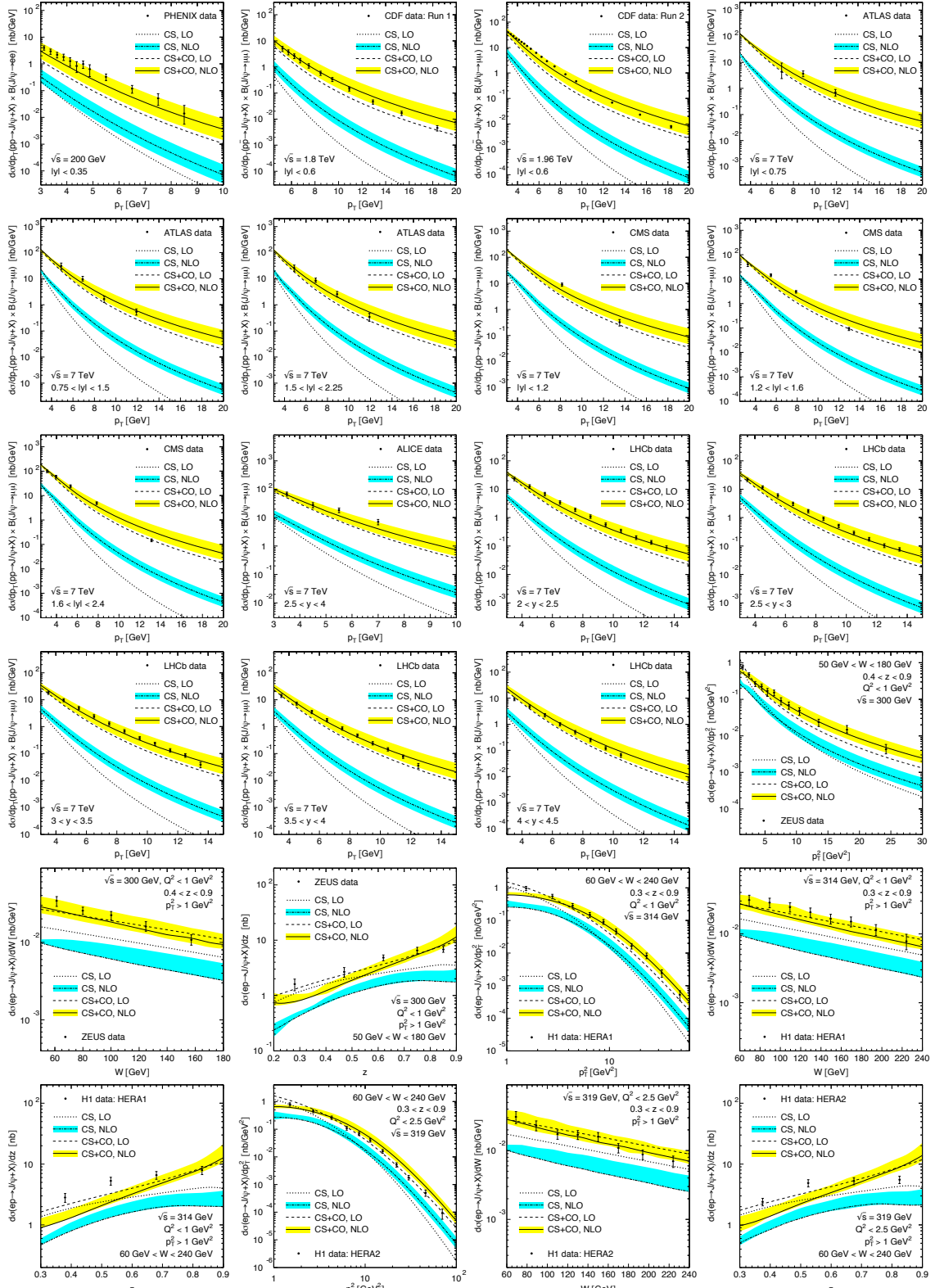
Figure 2.20: The NRQCD NLO fit to hadroproduction at RHIC, Tevatron and LHC and protonproduction measurements at HERA [116].
