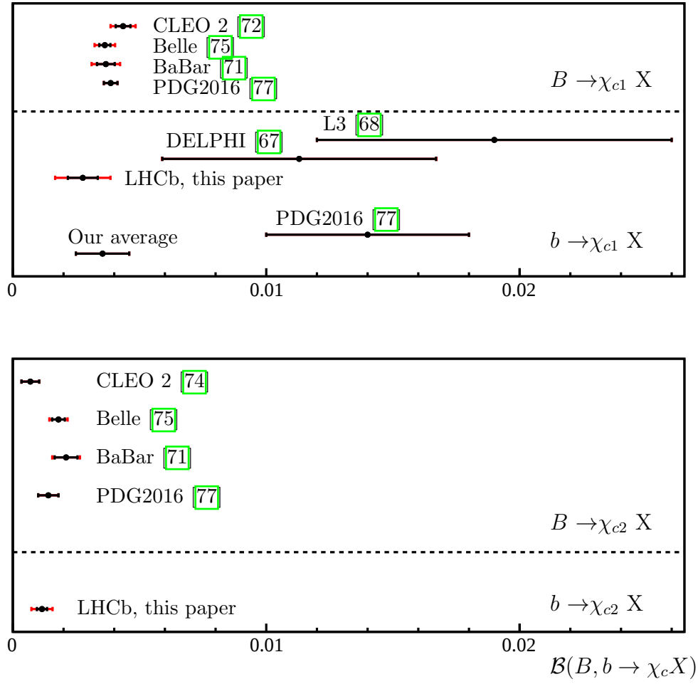
Figure 6.18: Summary of the branching fraction measurements for inclusive decays of light B mesons, \mathcal{B}(B \rightarrow \chi_c X) , and of all b hadrons, \mathcal{B}(b \rightarrow \chi_c X) , shown in each plot above and below the dashed line, respectively. The branching fractions for the decays to \chi_{c1} and \chi_{c2} are shown in the top and bottom plots, respectively. The world averages noted “PDG2016” do not include the LHCb results.
