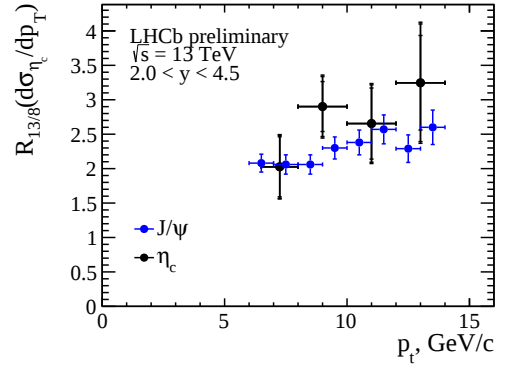
(b) Production in inclusive b -decays.
