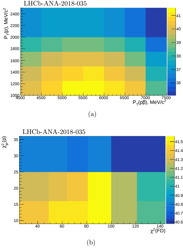
Figure 8.3: Optimisation map as a function of applied requirements on proton transverse momentum p_T ( p ) and charmonium transverse momentum p_T ( p\bar{p} ) (a), \chi^2 of flight distance of charmonium candidates \chi^2(FD) and \chi^2 of track impact parameter (b) with respect to the best primary vertex \chi^2_{IP}(p) . The FoM = N_{sig}/\sqrt{N_{sig} + N_{bkg}} is shown with the color code. The plots are 2D projections of the 4D optimisation.
