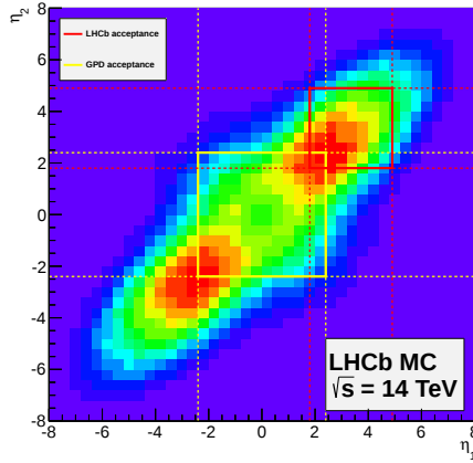
Figure 4.2: The b\bar{b} production as a function of quarks pseudorapidity. The red rectangle shows the LHCb acceptance. The yellow rectangle shows the ATLAS and CMS acceptance [213].
