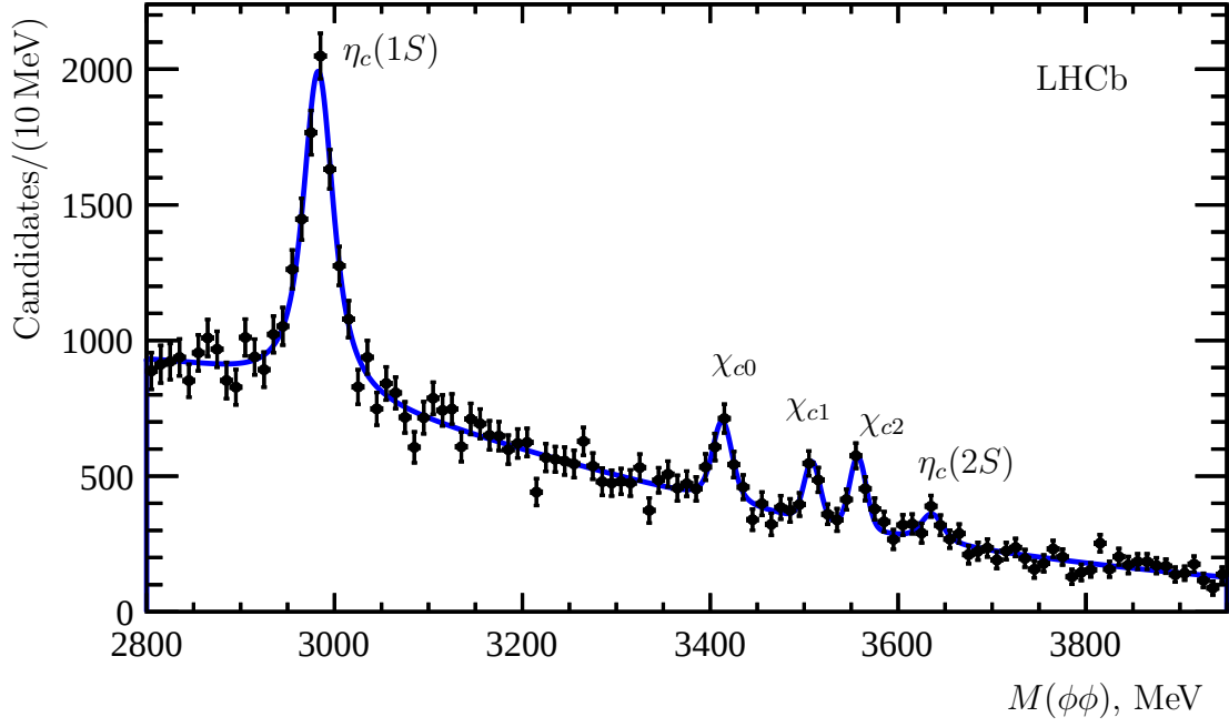
Figure 6.7: Distribution of the invariant mass of \phi\phi combinations. The number of candidates in each bin is obtained from the corresponding 2D fit. The peaks corresponding to the c\bar{c} resonances are marked on the plot.
