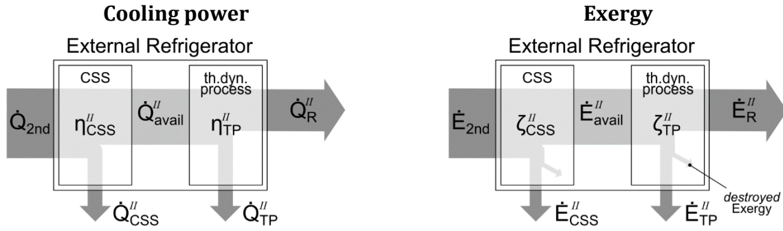
Figure 5.13. Flow of the cooling power and exergy provided by the cryocooler's 2nd stage.
