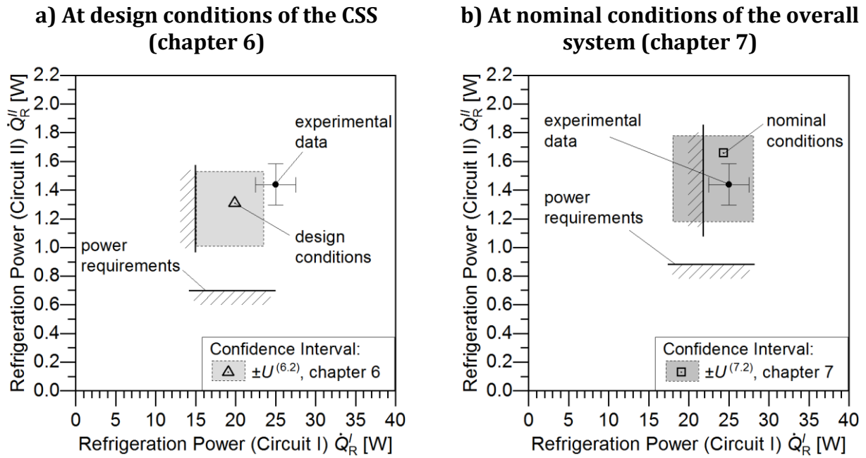
Figure 8.20. Confidence intervals \pm\%U for the refrigeration power in chapters 6 and 7. The estimates are applicable to the CSS design (a) and to the assessment of the overall cryogenic system (b). The power requirements vary between chapters and the experimental data corresponds to the measurements reported by Haug et al. [55].
