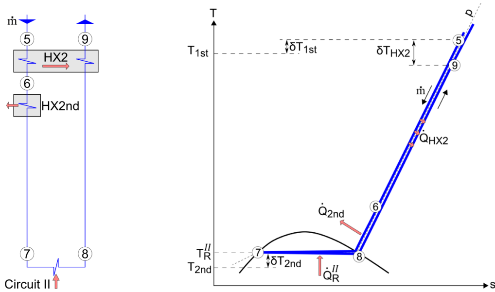
Figure 5.14. Segment of the flow chart (left) and T-s diagram (right) of configuration CFG0. This basic configuration does not comprise any additional component.
