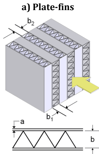
Figure 3.18. Use of fins in heat exchangers. [25], [49]
