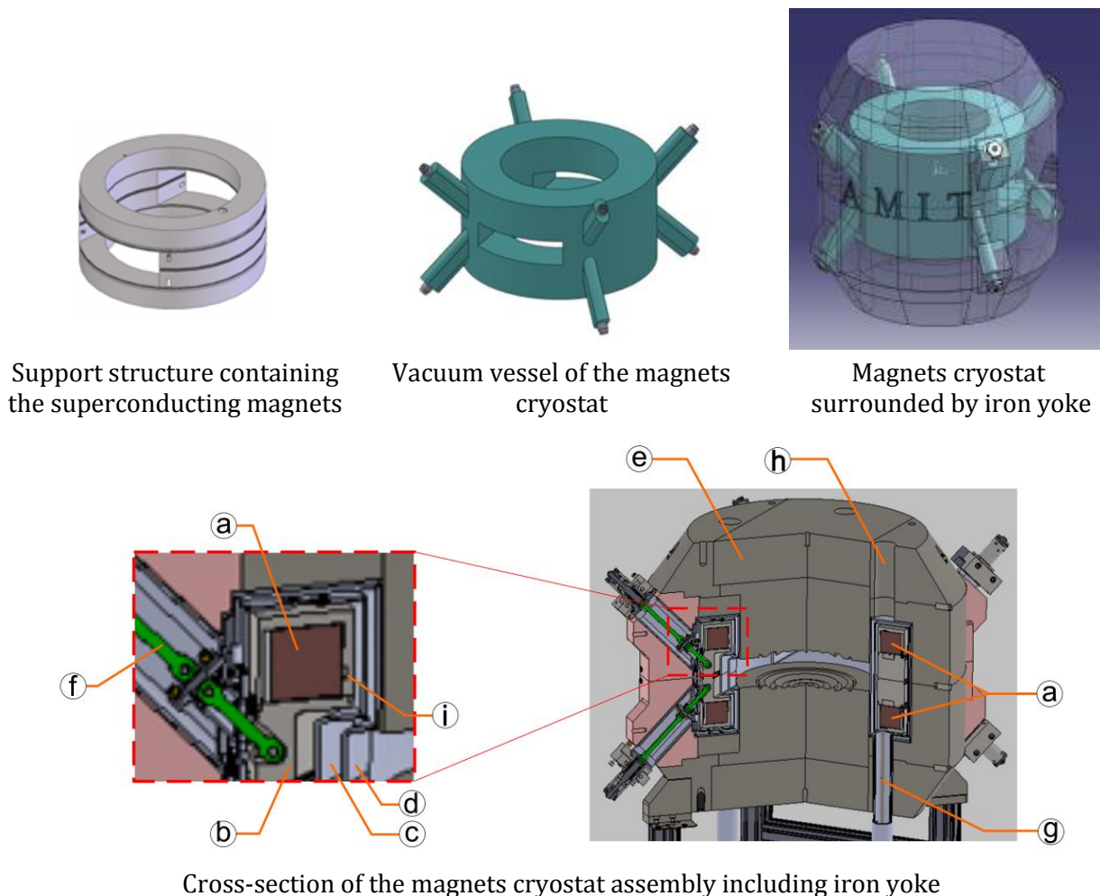
Figure 4.5. Overview of the components comprising the magnets cryostat assembly of the compact superconducting cyclotron. [53], [51]
