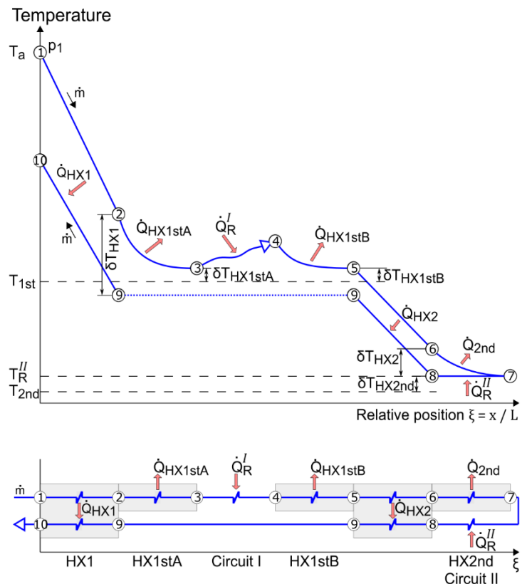
Figure 5.1. Flow diagram and qualitative temperature distribution of the remote refrigeration system in its basic configuration.
