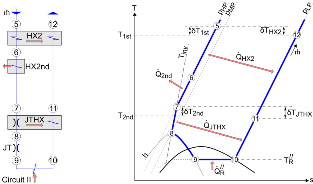
Figure 5.27. Segment of the flow chart (left) and T-s diagram (right) of configuration CFG3. It presents a Joule-Thomson recuperator JTHX before the JT expansion step.
