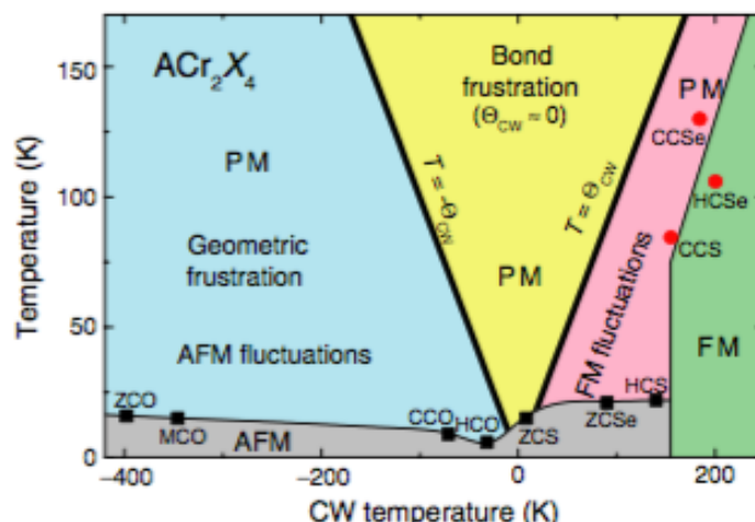
Figure 1.13 – Schematic magnetic phase diagram of ACr_2X_4 compounds, where characteristic temperatures are plotted versus the CW temperature: FM (red circles) and AFM (black squares) ordering temperatures. Hypothetical magnetic ordering temperatures ( T = \pm\theta_{CW} ) are indicated by thick solid lines. Thin solid lines separate magnetically ordered from PM phases and are drawn to guide the eye. (From ref. 126)
