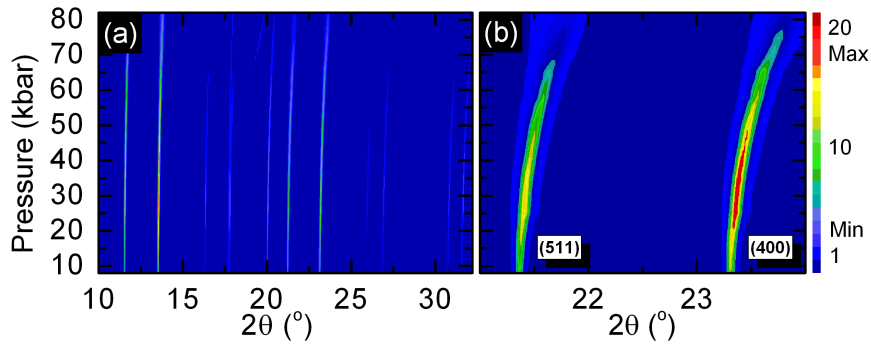
Figure 3.16 – (a): Contour plot of the x-ray diffraction data as a function of pressure. (b): Detailed 2\theta from 21 to 24° of the X-ray diffraction data.
