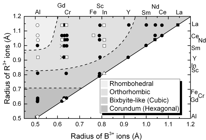
Figure 1.19 – Classification of the \text{R}^{3+}\text{B}^{3+}\text{O}_3 type compounds according to the constituent ionic radii. ○ - Rhombohedral perovskite, \alpha > 90^\circ ; □, orthorhombic perovskite \text{CaTiO}_3 type; △, \text{Ti}_2\text{O}_3 structure type; ◇, corundum structure type; ■, \text{La}_2\text{O}_3 structure type; ●, compounds assumed to have the structure by the areas bounded by dashes. (Adapted from ref. 198)
