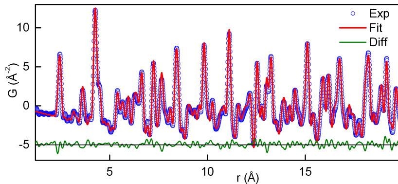
Figure 3.4 – PDF of the spinel \text{CdCr}_2\text{S}_4 structure at 80 K.
