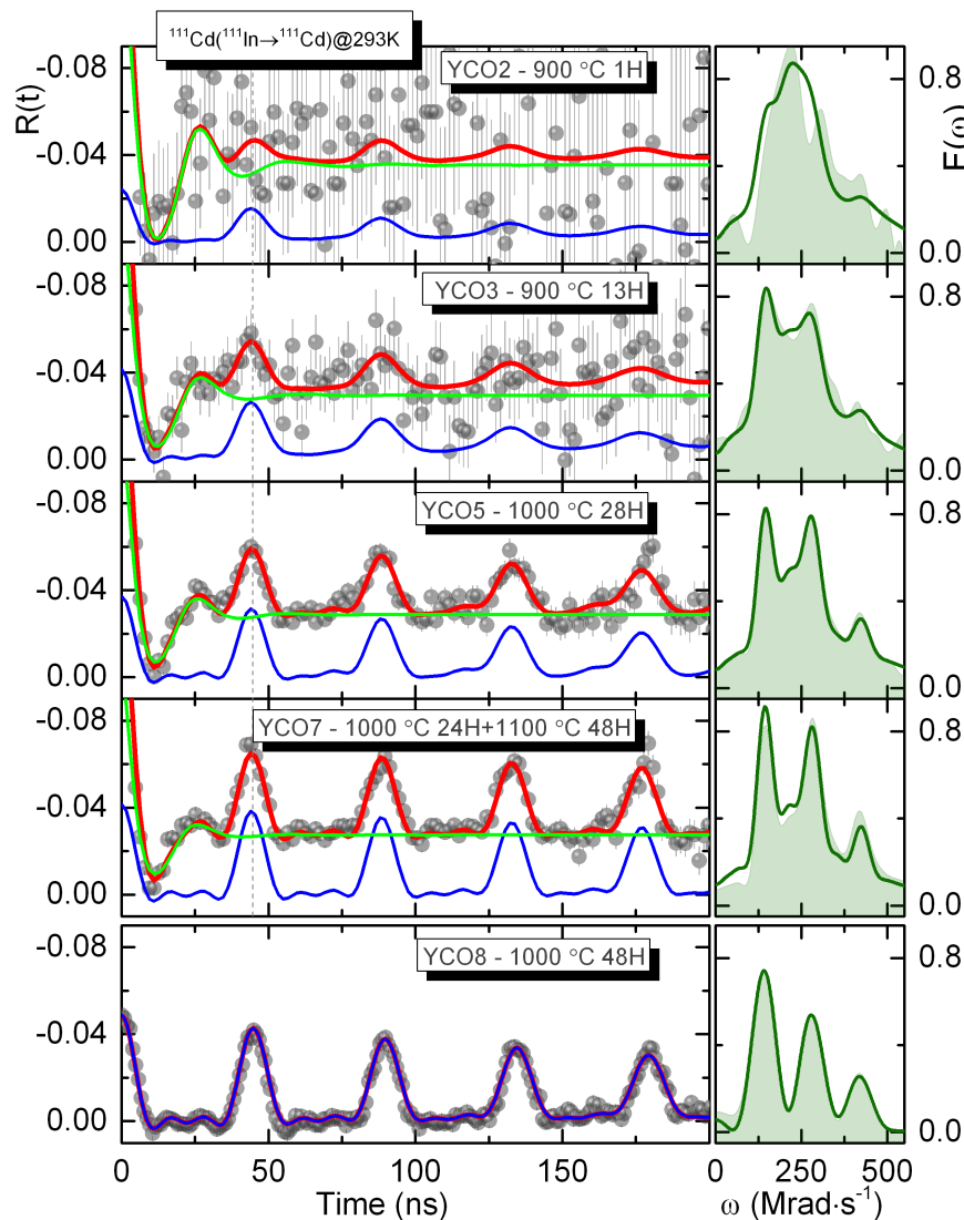
Figure 5.12 – Representative R(t) functions, corresponding fits (partial fits, corresponding to each individual EFG, are represented in blue and green) and respective Fourier transform taken at different annealing temperatures and dwell times for the ^{111}\text{In} probe on \text{YCrO}_3 . The bottom R(t) spectrum correspond to sample YCO-8 which experienced a slower cooling after the annealing.
