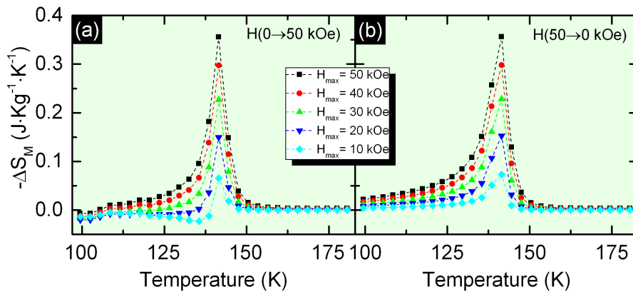
Figure 5.4 – Magnetic entropy changes with respect to temperature at different field changes for \text{YCrO}_3 sample.
