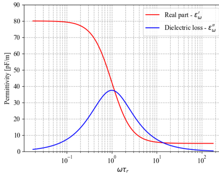
Figure 2.3: Real and imaginary parts of the permittivity of H 2 O as a function of the normalized frequency, assuming Debye relaxation as described by eq. (2.8)-(2.10).
