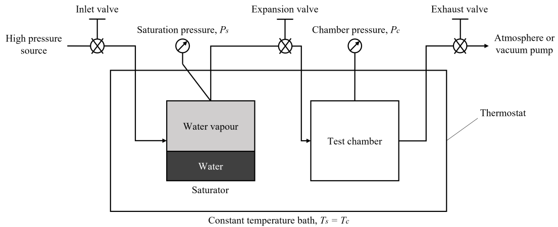
Figure 4.19: Schematic diagram of two-pressure humidity generator.
