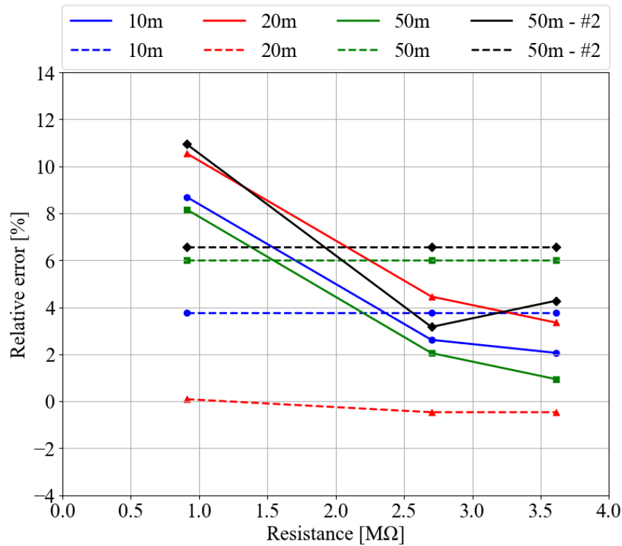
Figure 5.12: Relative error at different frequencies, lengths of NEK RG 58 C/U coaxial cable, and types of coaxial cables (Bedeia 0801 CA labeled as #2). Leakage resistor values are also varied. The solid lines show the relative error of measurements obtained at 1 kHz, while the dashed lines present the measurement relative error at 6.2 kHz.
