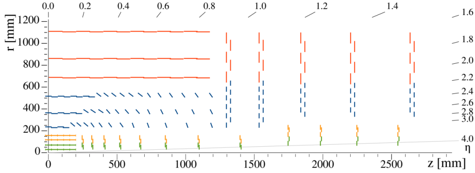
Figure 1.9: One-quarter view of the tracker layout in r - z projection. The Inner Tracker contains pixel modules made of two readout chips (green lines) and pixel modules with four readout chips (yellow lines), while the Outer Tracker exhibits the pixel-strip (PS) and 2-strip (2S) modules denoted by blue and red lines, respectively.
