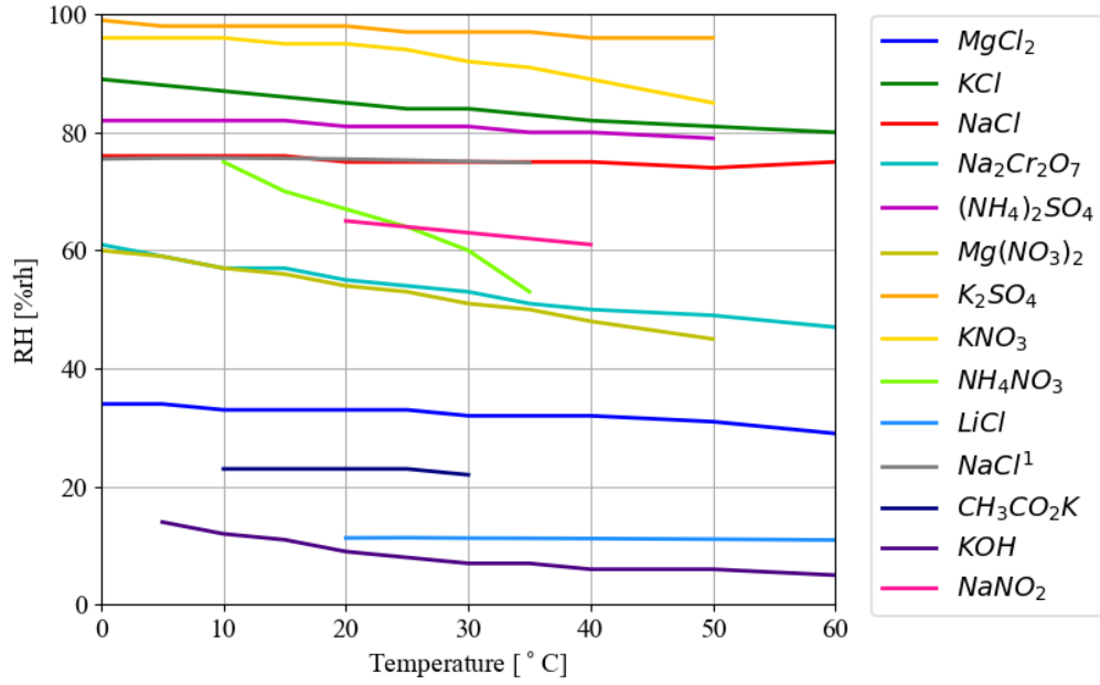
Figure 4.18: Relative humidity over different saturated salt solutions. \text{LiCl} and \text{NaCl}^1 are saturated aqueous solutions of inorganic salts.
