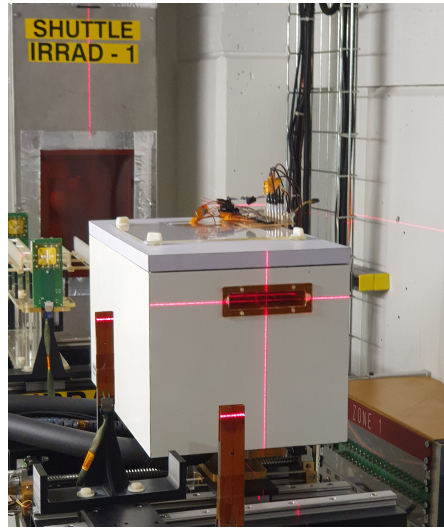
Figure 4.10: A photograph of the cold box with the samples inside positioned on one of the tables in the radiation area. The lasers show the center of the incoming proton beam.
