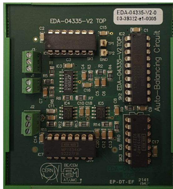
Figure 5.6: Single channel PCB prototype for capacitive humidity sensor readout.
