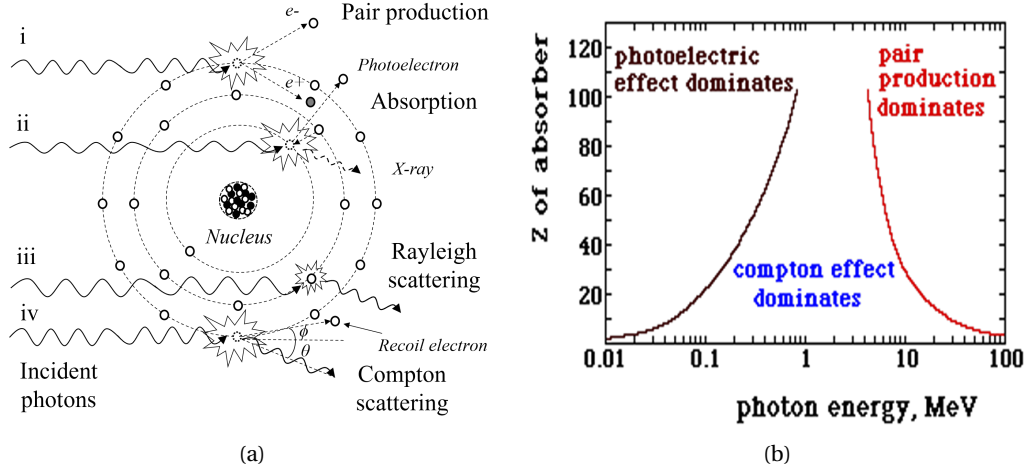
Figure 3.2: (a) Illustrative summary of photons interactions: (i) Pair production - the electron and positron are emitted in the direction of the photon motion; (ii) Photoelectric absorption results in total removal of the incident photon with energy greater than the binding energy of the electron in its shell, with subsequent x-ray emission; (iii) Rayleigh scattering is interaction with an electron (or whole atom) in which no energy is exchanged and incident photon energy equals scattered photon energy with a small angular change in direction; (iv) Compton scattering interactions occur with essentially unbound electrons, with a transfer of energy shared between recoil electron and scattered photon. (b) The curves demarcate the regions where three major types of photon interaction with matter effect are dominant.
