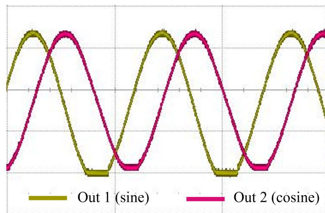
Figure 5.14: Output signals of the quadrature oscillator based on the TLV2474 chip and three RC networks. The phase difference between the output signals is 89.92^\circ .
