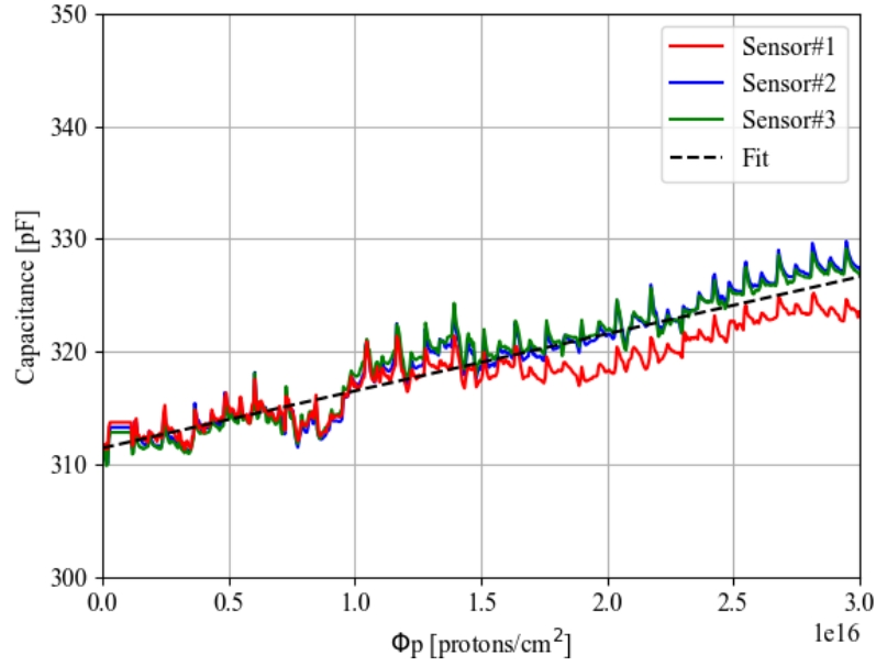
Figure 4.12: Measurements were continuously taken during the irradiation of the samples. During the 33-day irradiation period, the ambient condition was dry air, and the temperature was -20^{\circ}\text{C} . The dependence of the sensor capacitance on the fluence can be described by a linear fit.
