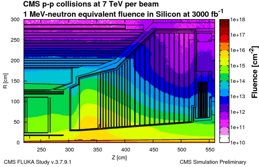
Figure 1.15: Integrated particle fluence in 1 MeV neutron equivalent per \text{cm}^2 , accumulated in HGCal after an integrated luminosity of 3000 \text{ fb}^{-1} .
