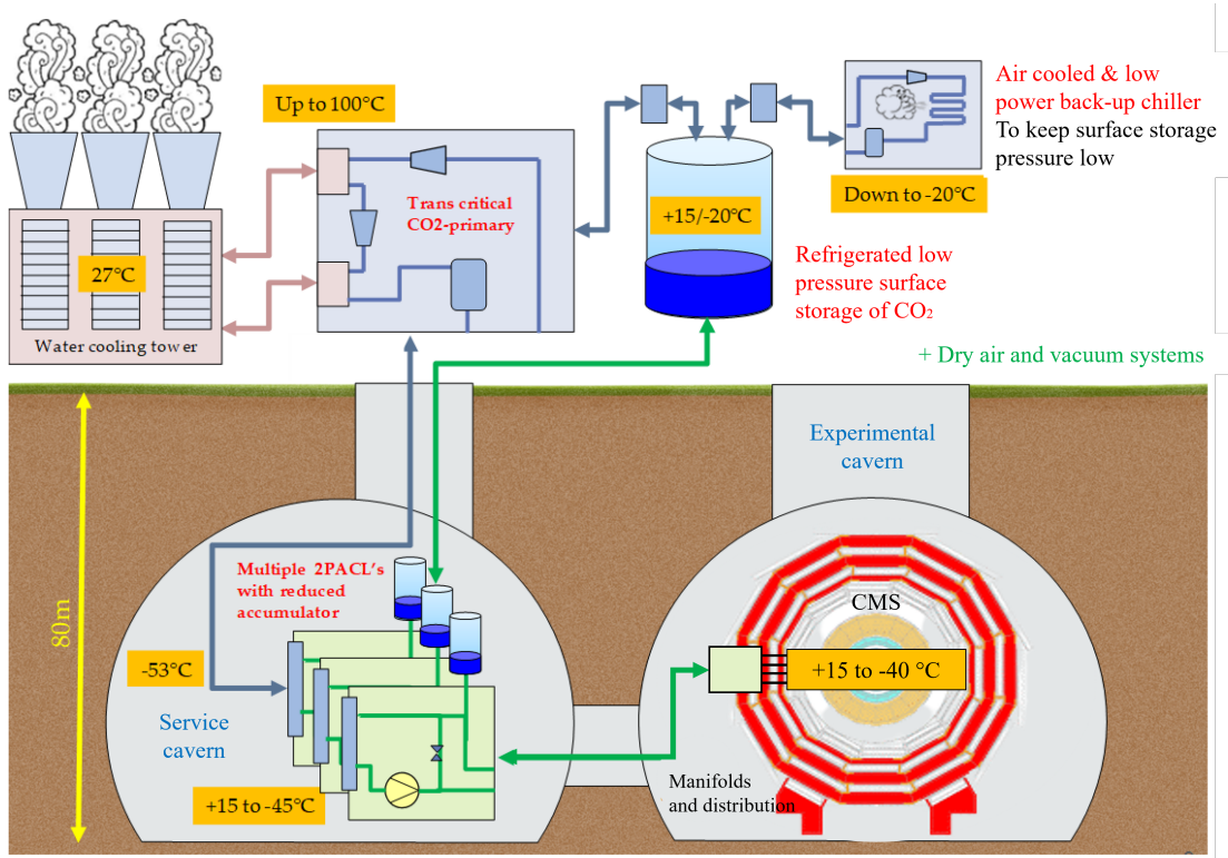
Figure 6.1: R744 and 2PACL system overview [206].
