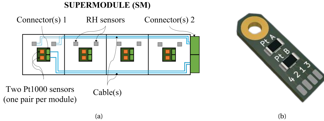
Figure 6.9: (a) A schematic representation of the ECAL supermodule. The supermodule is comprised of four individual modules, each of which accommodates a pair of Pt1000 temperature sensors and a pair of humidity sensors. (b) A 3D design on the PCB featuring two Pt1000 temperature sensors mounted on the same board.
