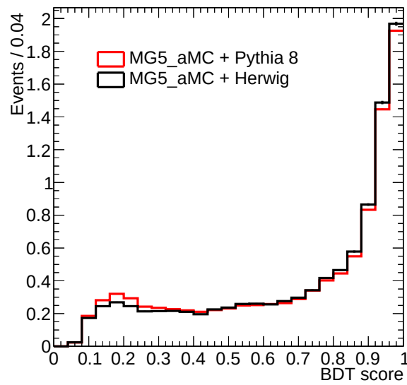
Figure 5.6: Comparison of the impact of the parton showering model in PYTHIA and HERWIG on the MG5_AMC signal simulation of the BDT score distribution.
