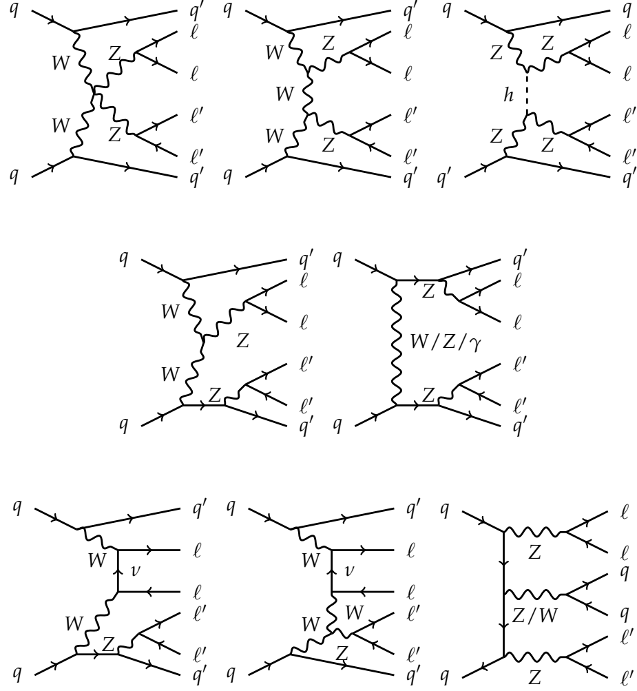
Figure 1.3: Feynman diagrams for the electroweak production of the \ell\ell'\ell'jj final state. The top row illustrates diagrams of the VBS signal. The scattering of massive gauge bosons as depicted in the first two diagrams of the top row is unitarized by the interference with diagrams that feature the Higgs boson (top right). The center row features diagrams that are required to ensure gauge invariance. The bottom row illustrates non-resonant production and triboson processes.
