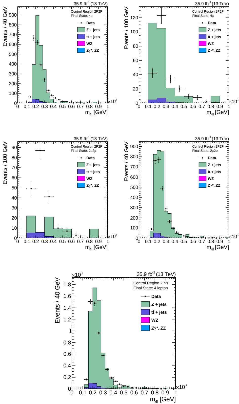
Figure 6.10: Invariant mass distribution of the events selected in the 2P2F control sample, for the 4e (top left), 4μ (top right), 2e2μ (center left), 2μ2e (center right), and 4ℓ (bottom) final states. The full 2016 dataset with an integrated luminosity of 35.9 \text{ fb}^{-1} is used.
