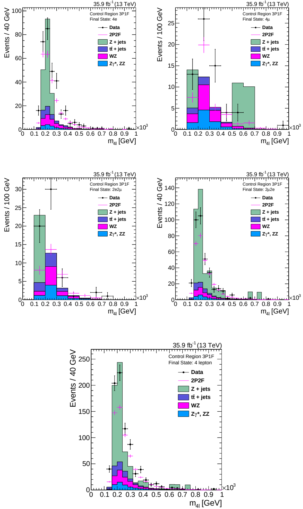
Figure 6.11: Invariant mass distribution of the events in the 3P1F control region, for the 4e (top left), 4\mu (top right), 2e2\mu (center left), 2\mu2e (center right), and 4\ell (bottom) final states. The full 2016 dataset with an integrated luminosity of 35.9 \text{ fb}^{-1} is used.
