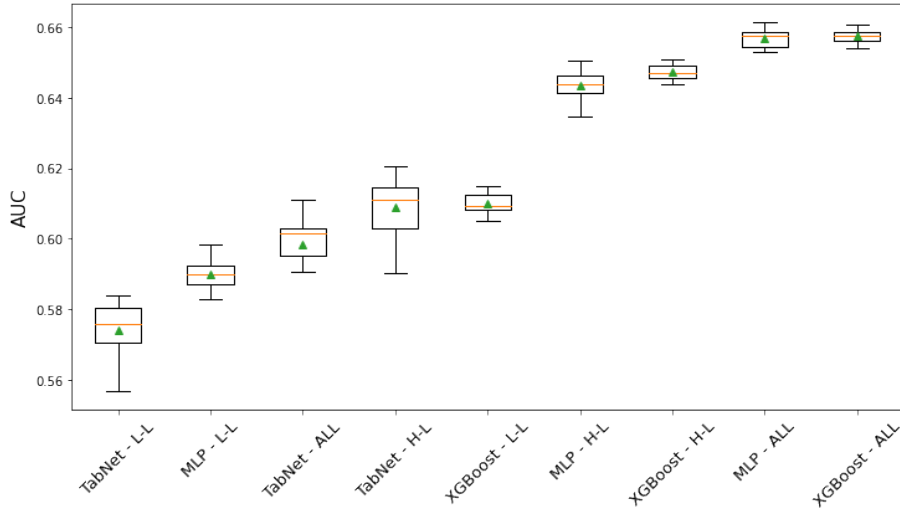
Figure 5.4: AUC dependance on algorithm and feature selection - training with weights - Exp.1
