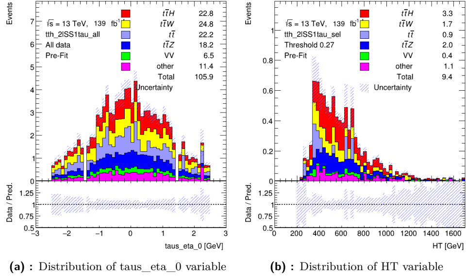
Figure 5.22: Distribution of all simulated events in the simulated dataset - most important variables 2/2
