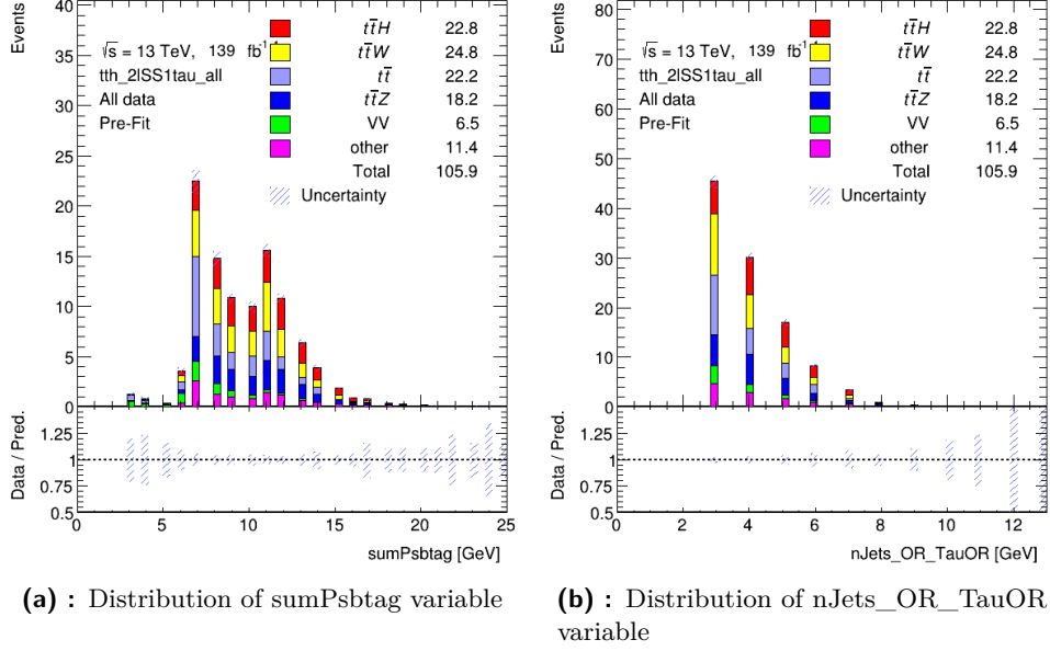
Figure 5.21: Distribution of all simulated events in the simulated dataset - most important variables 1/2
