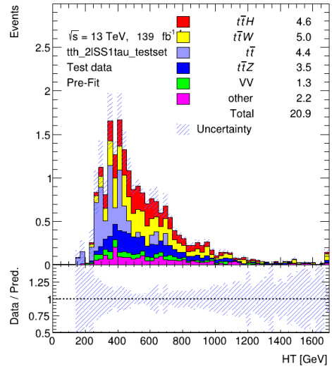
(b) : Distribution of HT variable
