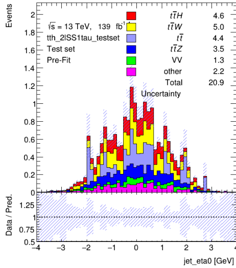
(a) : Distribution of jet_eta0 variable
