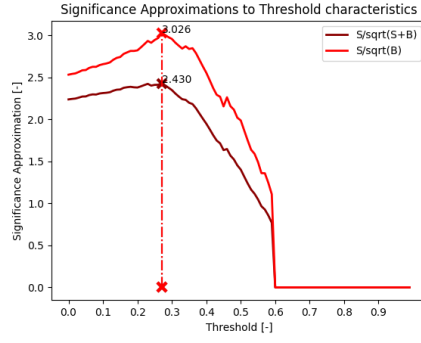
(a) : Significance on thresholds
