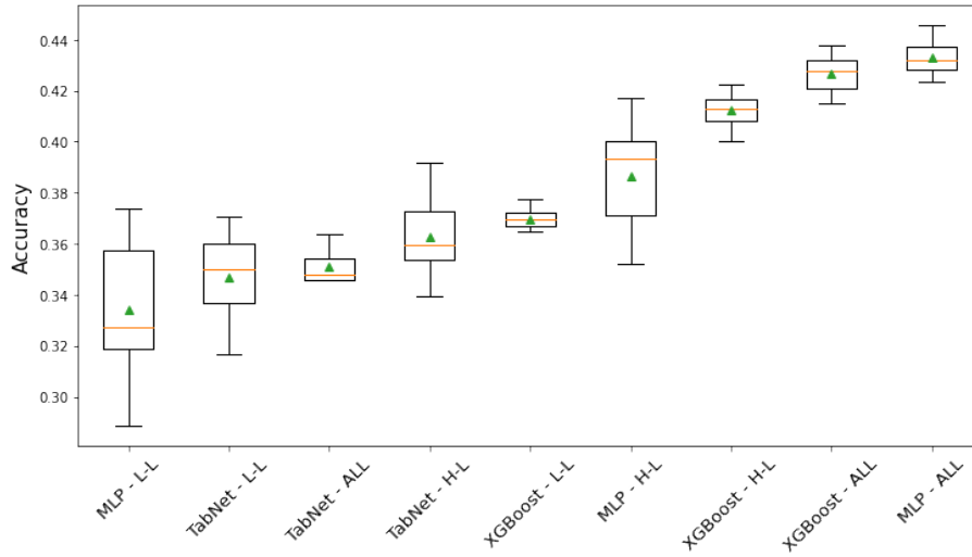
Figure 5.5: Accuracy dependance on algorithm and feature selection - training with weights - Exp.1
