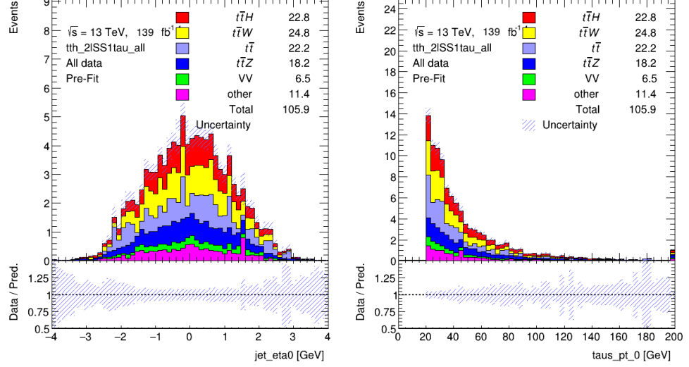
(a) : Distribution of jet_eta0 in all (train- ing+testing) data
