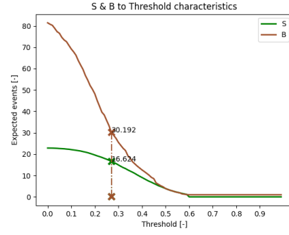
(b) : Signal/Background on different decision thresholds
