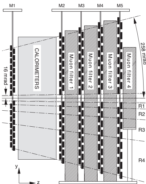
Figure 4.13: Side view of the muon system [50].
