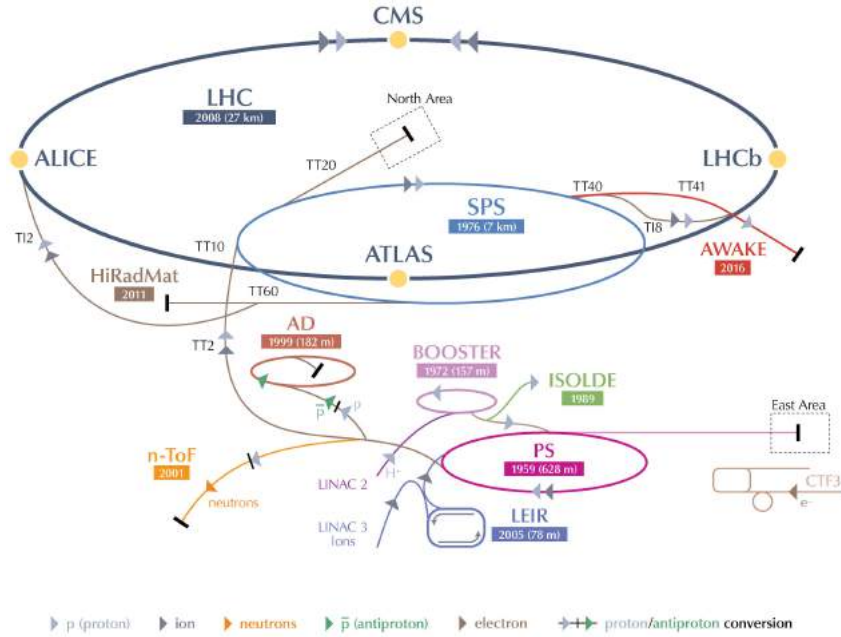
Figure 4.2: The full complex of accelerators that dumps protons into the LHC [40].
