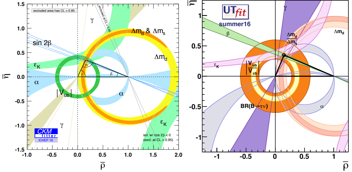
Figure 3.2: Global fit results for the Unitary Triangle, performed by the CKMfit [30] and UTfit [32] groups respectively.
