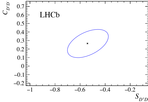
Figure 6.20: Two dimensional likelihood profile scan for S_{D^+D^-} and C_{D^+D^-} . The contour line shows the 1\sigma confidence level.
