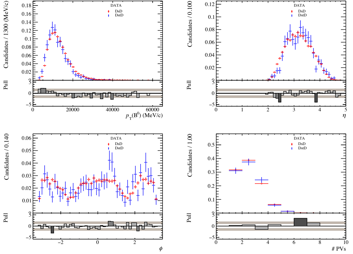
Figure 5.13: Comparison between B^0 \rightarrow D_s^+ D^- Run 1 data sample (red) and B^0 \rightarrow D^{*\pm} D^\mp (blue) for B^0 transverse momentum (top left), pseudorapidity (top right), azimuthal angle (bottom left) and number of primary vertex (bottom right).
