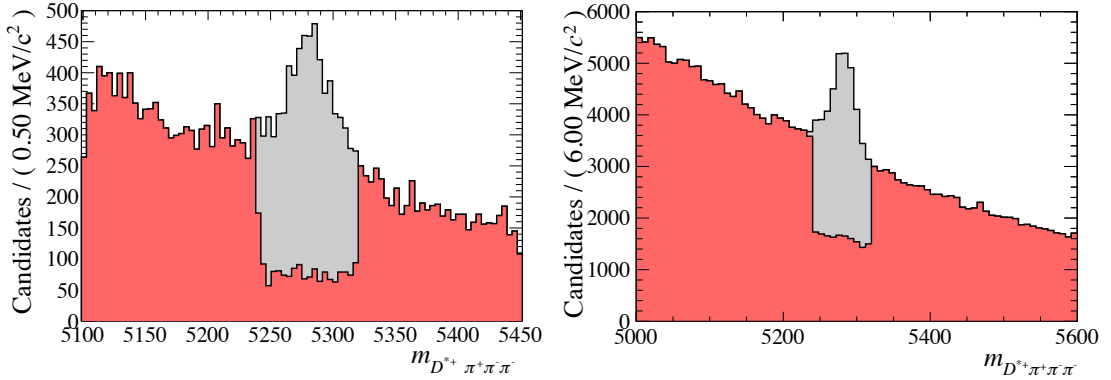
Figure 7.8: Plots of the invariant mass of the D^* \pi\pi\pi combination. The distributions are given without (grey) and with (red) the B^0 \rightarrow D^* \pi\pi\pi veto described in the text, for D^0 decaying into K^-\pi^-\pi^+\pi^+ (left) and to K^-\pi^+ (right) on Run 1 data sample.
