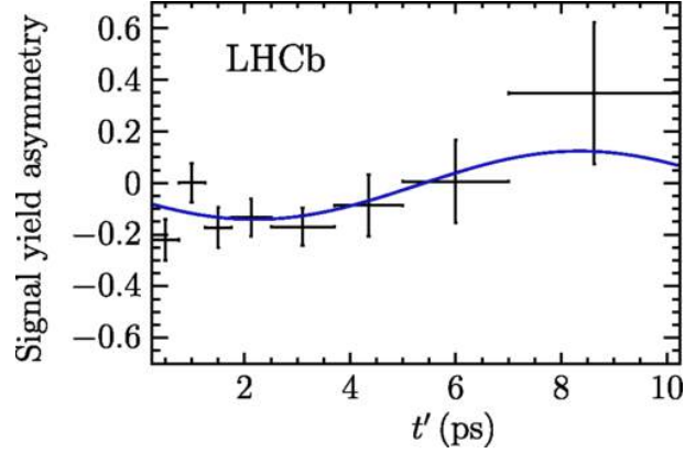
Figure 6.19: Time-dependent signal yield asymmetry (N_{\bar{B}^0} - N_{B^0})/(N_{\bar{B}^0} + N_{B^0}) . Here N_{B^0}(N_{\bar{B}^0}) is the number of B^0 \rightarrow D^+ D^- decays with a B^0 ( \bar{B}^0 ) flavour tag. The data points are obtained with the sPlot technique, assigning signal weights to the events based on a fit to the reconstructed mass distribution. The solid curve is the projection of the signal PDF.
