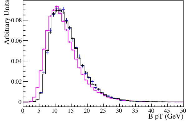
Figure 5.16: Comparison between B_d transverse momentum distributions for B^0 \rightarrow D^{*+} D_s^- (k3\pi/k\pi/kk) (black), B^0 \rightarrow D^{*+} D^+ (k3\pi) (blue) and B^0 \rightarrow D^{*+} D^+ (k\pi) (magenta) in Run 1 MC.
