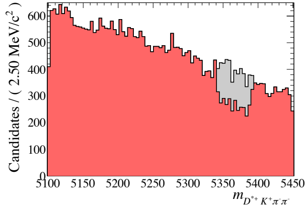
Figure 7.6: Plots of the invariant mass of the D^* K\pi\pi combination. The distributions are given without (grey) and with (red) the B_s^0 \rightarrow D^* K\pi\pi veto described in the text, for D^0 decaying into K^-\pi^-\pi^+\pi^+ in Run 1 data sample.
