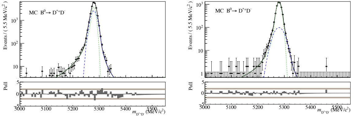
Figure 7.16: Mass distribution of the B^0 \rightarrow D^{*+} D^- ( D^0 \rightarrow K^-\pi^-\pi^+\pi^+ ) signal MC sample overlaid with the projection of the fitted PDF, for Run 1 (left) and Run 2 (right). The y-axis has a logarithmic scale.
