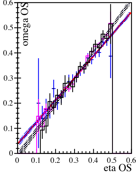
Figure 5.18: Mistag probability \omega as a function of the predicted mistag probability \eta using OS tagger for the B^0 \rightarrow D^{*+}D_s^-(k3\pi/k\pi/kk) Run1 Monte Carlo sample (black), B^0 \rightarrow D^{*\pm}D^\mp(k3\pi) (blue) and B^0 \rightarrow D^{*\pm}D^\mp(k\pi) MC sample (magenta).
