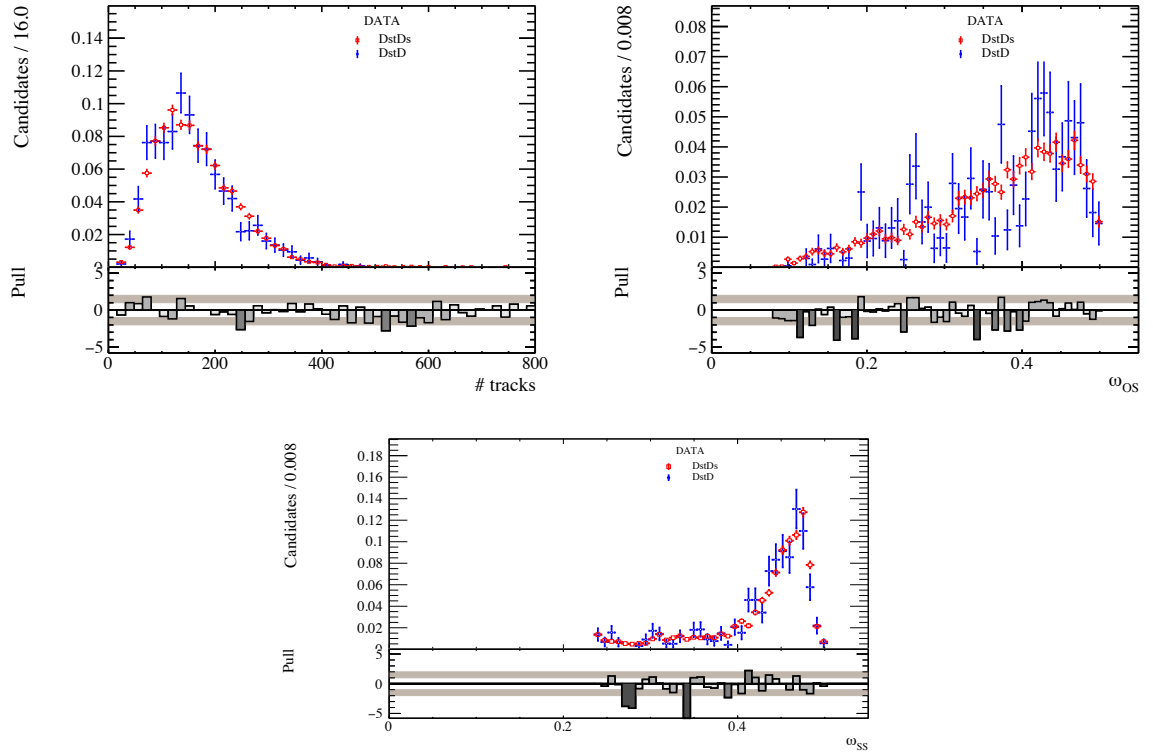
Figure 5.20: Comparison between B^0 \rightarrow D^{*+} D_s^- Run 1 data sample (red) and B^0 \rightarrow D^{*\pm} D^\mp (blue) for number of tracks (top left), mistag probability for the Opposite Side tagger combination (top right) and mistag probability for the Same side tagger combination (bottom).
