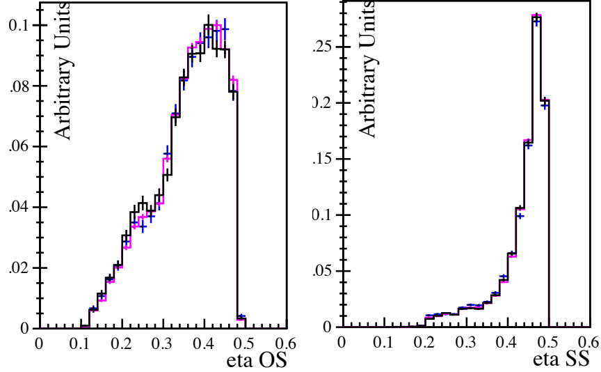
Figure 5.17: Comparison between mistag distributions for B^0 \rightarrow D^{*+} D_s^- (k3\pi/k\pi/kk) (black), B^0 \rightarrow D^{*+} D^+ (k3\pi) (blue) and B^0 \rightarrow D^{*+} D^+ (k\pi) Run 1 signal MC (magenta) using Opposite Side and Same Side tagger combinations respectively.
