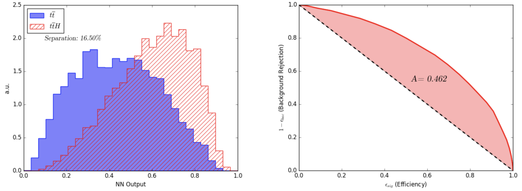
(a) Normalised NN response for the test dataset including signal (red) and background (blue) events. The general shape of the distribution is in good agreement with the separation power. (b) ROC curve corresponding to the separation power of the NN on the test dataset.
