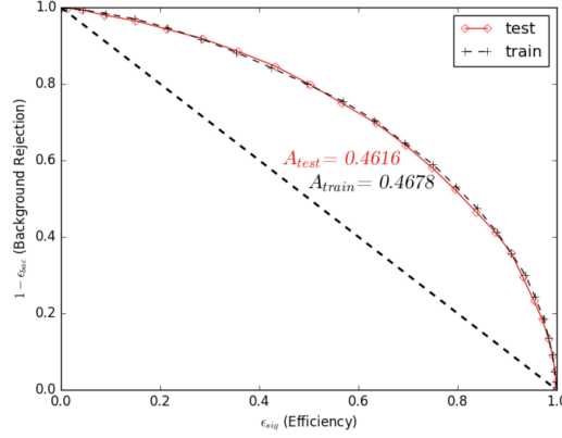
Figure 5.18.: Comparison of ROC curves for an overtraining test. The solid red (dashed black) curve corresponds to the separation power of the NN applied on the test (training) sample. Both curves are in good agreement suggesting the overtraining is insignificant.
