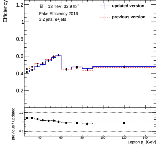
(a) Fake efficiency for the e + \text{jets} channel.
