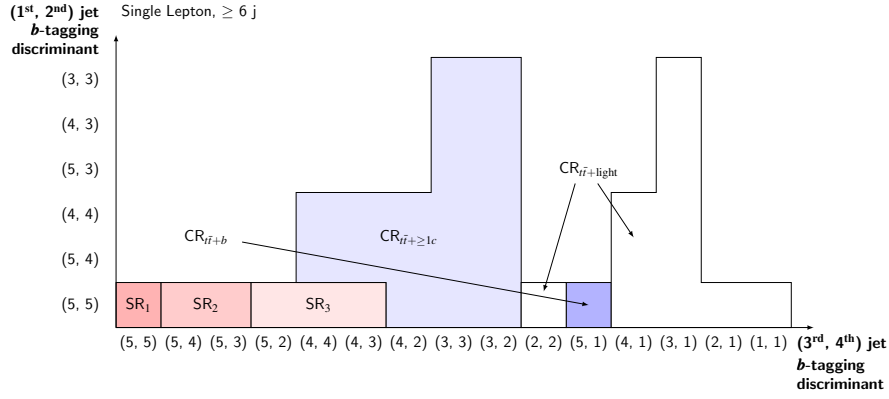
Figure 5.11.: Definition of the SRs and CRs in the single-lepton channel. The categorisation is made in dependence of the b -tagging discriminant. The vertical axis displays the values of the b -tagging discriminant assigned to the first two jets, while the horizontal axis displays these values for the third and fourth jets.
