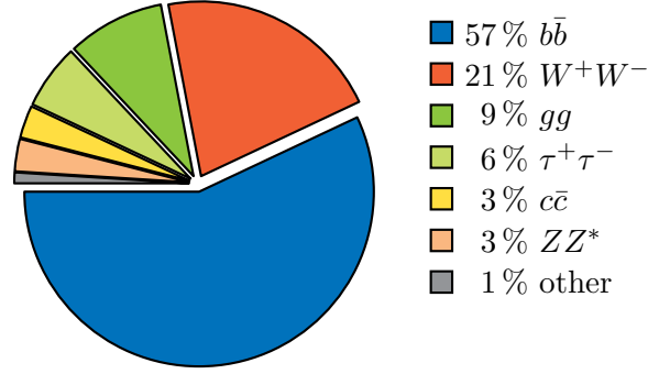
Figure 2.6.: The decay channels of a Higgs boson.
