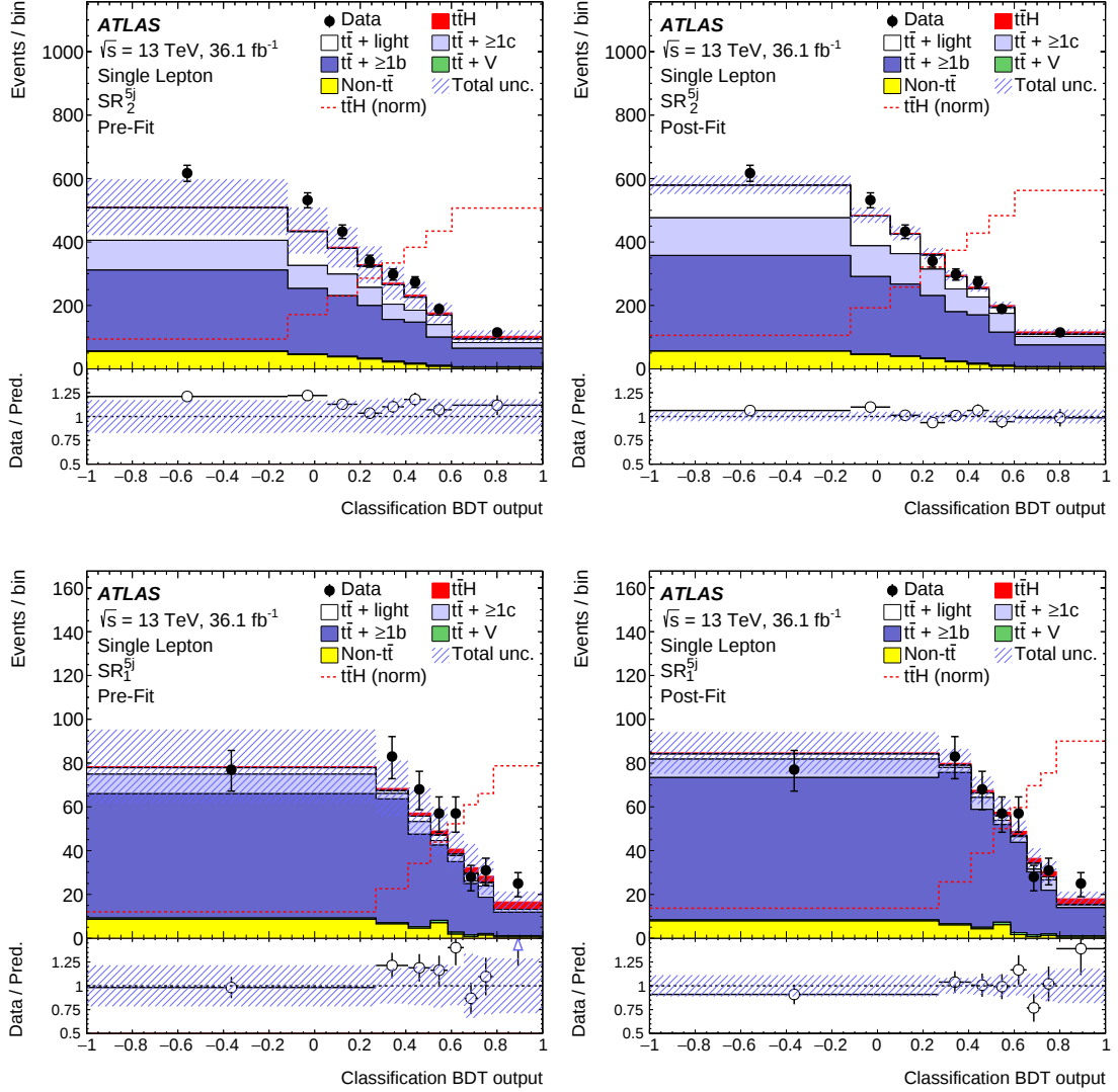
Figure 5.29.: Comparison between data and prediction for the BDT discriminant in the single-lepton channel five-jet SRs before and after the fit.
