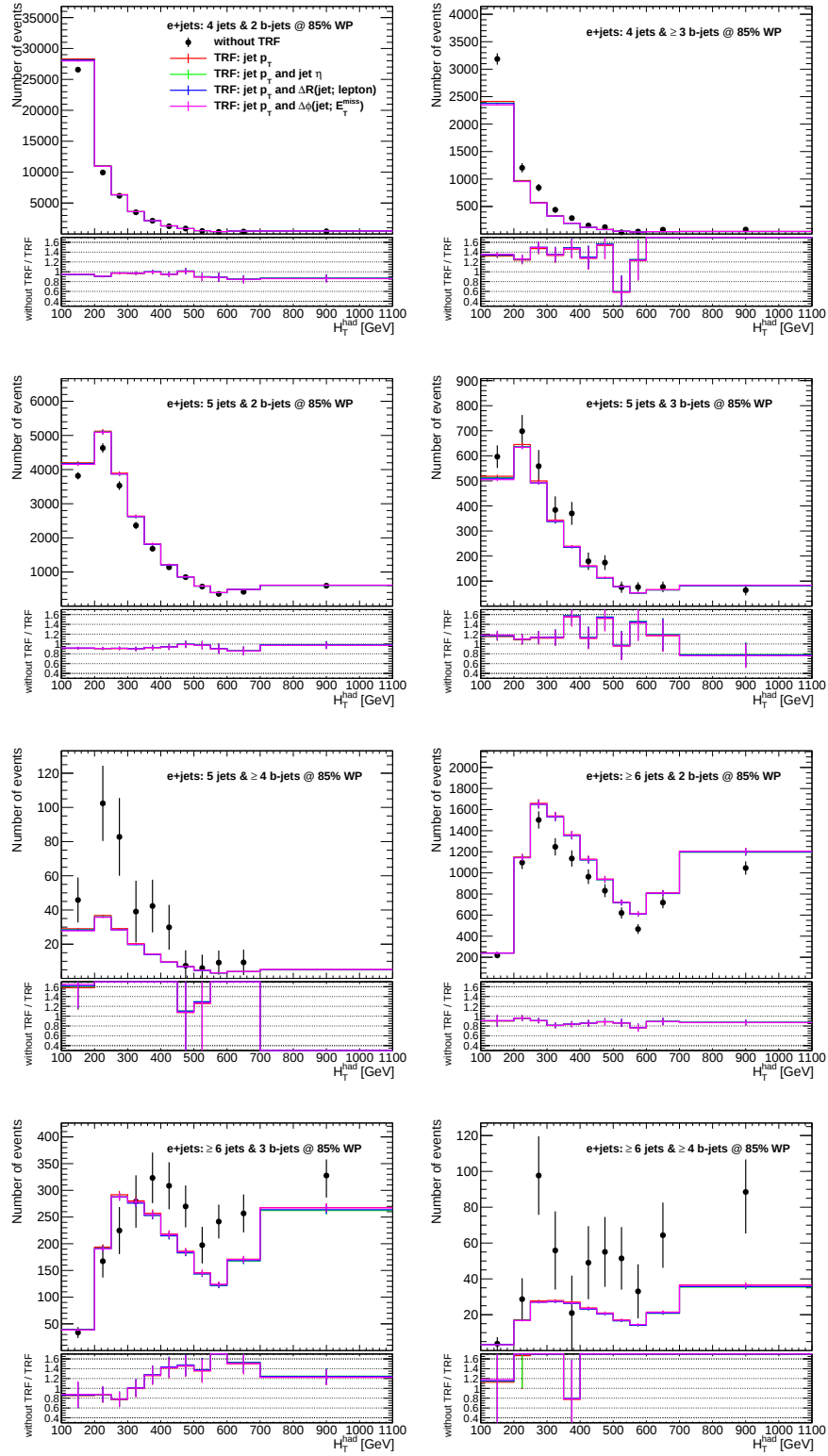
Figure 5.9.: Comparison of the event yields of the fake estimation with and without the TRF method. Selection: electron + jets with a b -tagging WP of 85 %.
