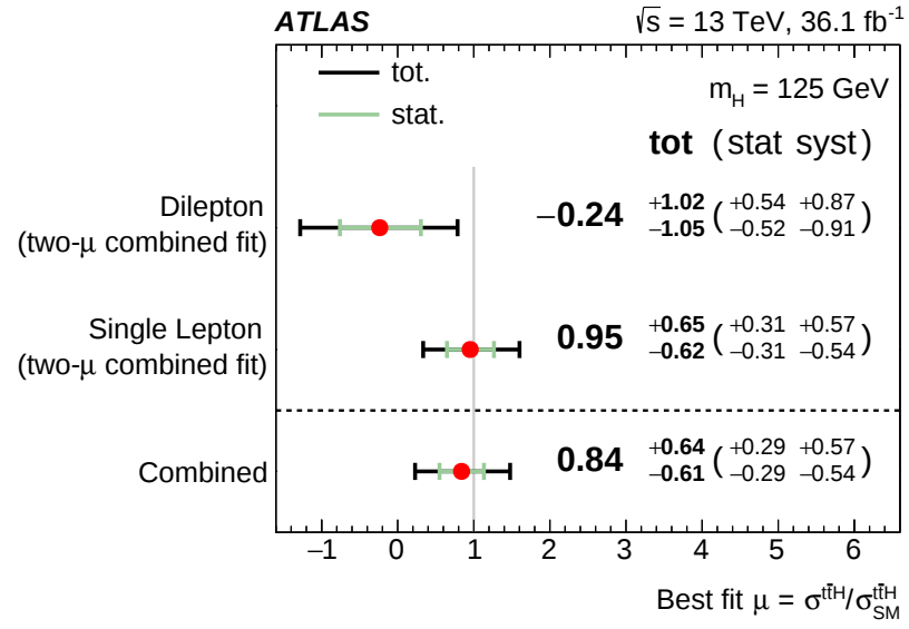
Figure 5.33.: Signal strength measurements in the single-lepton and dilepton channel (top) and for the combination (bottom) obtained from a simultaneous profile likelihood fit to data. The results for the individual channels are calculated without correlation between the signal strengths, while including correlations between nuisance parameters across channels.
