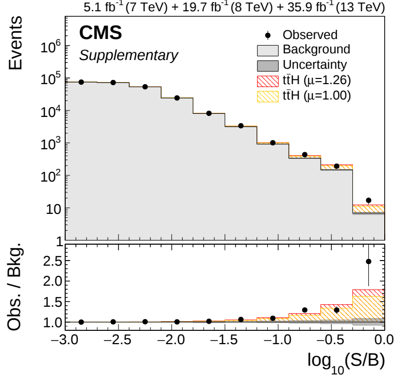
Figure 6.11.: Signal and background yields as a function of \log_{10}(S/B) , compared to data for all analysis categories from CMS. The signal is shown normalised to the best-fit value and to the SM prediction, including the background prediction from the fit. In addition, the ratios of the expected signal and observed results relative to the expected background are shown for \mu = 1.26 ( \mu = 1 ) and represented in red (orange).
