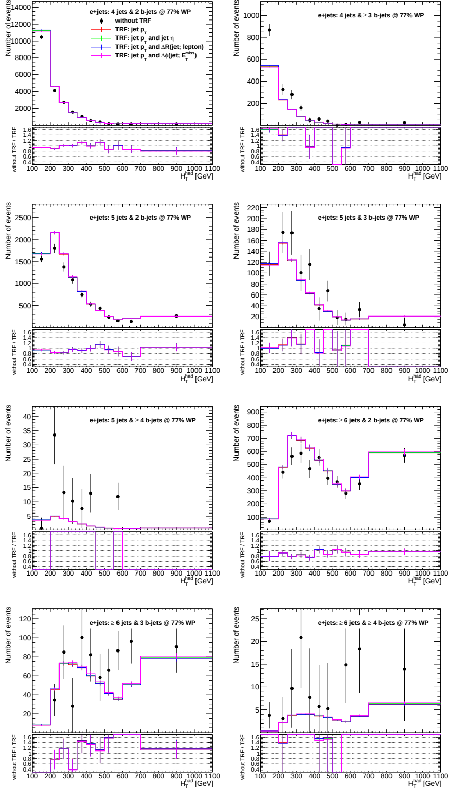
Figure B.6.: Comparison of the event yields of the fake estimation with and without the TRF method. Selection: electron + jets with a b -tagging WP of 77 %.
