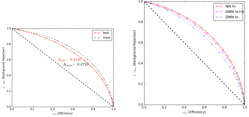
(a) ROC curves for a DNN in the best configuration using jet b -tag weights in addition to low-level variables. (b) Comparison of variable set performance. The addition of TRF b -tagging weight information (DNN lo+b) recovers some of the performance lost when changing from high-level variables (hi) to low-level variables (lo).
