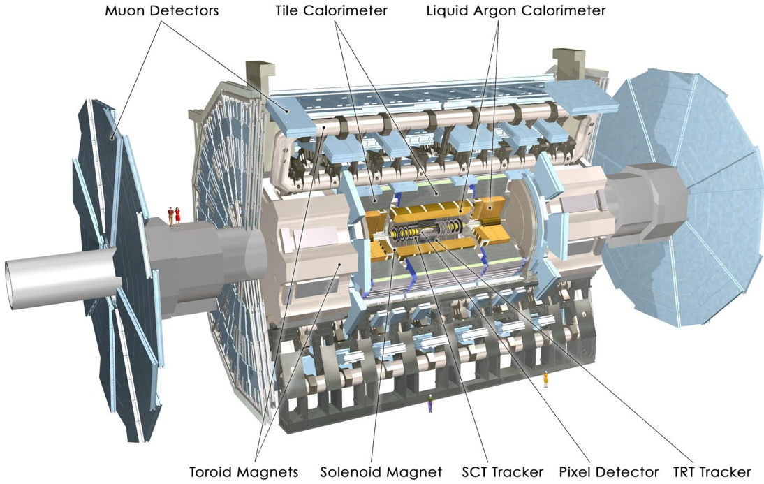
Figure 3.2.: Cutaway rendering of the ATLAS detector. © CERN
