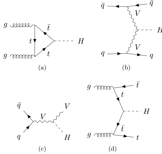
Figure 2.5.: Feynman diagrams of the main Higgs boson production mechanisms at the LHC. (a) gluon-gluon fusion, (b) vector boson fusion ( V = Z, W ), (c) associated production with a vector boson, (d) associated production with a top-quark pair.
