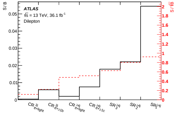
(b) Dilepton channel.
