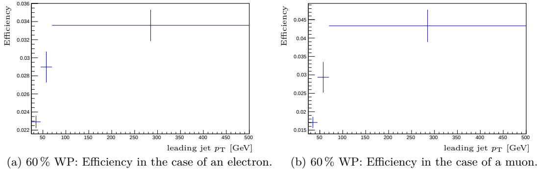
Figure B.1.: TRF b -tagging efficiency calculated in a four jet inclusive region with at least one b -jet using different b -tagging WPs in dependence of the leading jet p_T ; electrons (left) and muons (right) are considered separately. Continued on the next page.
