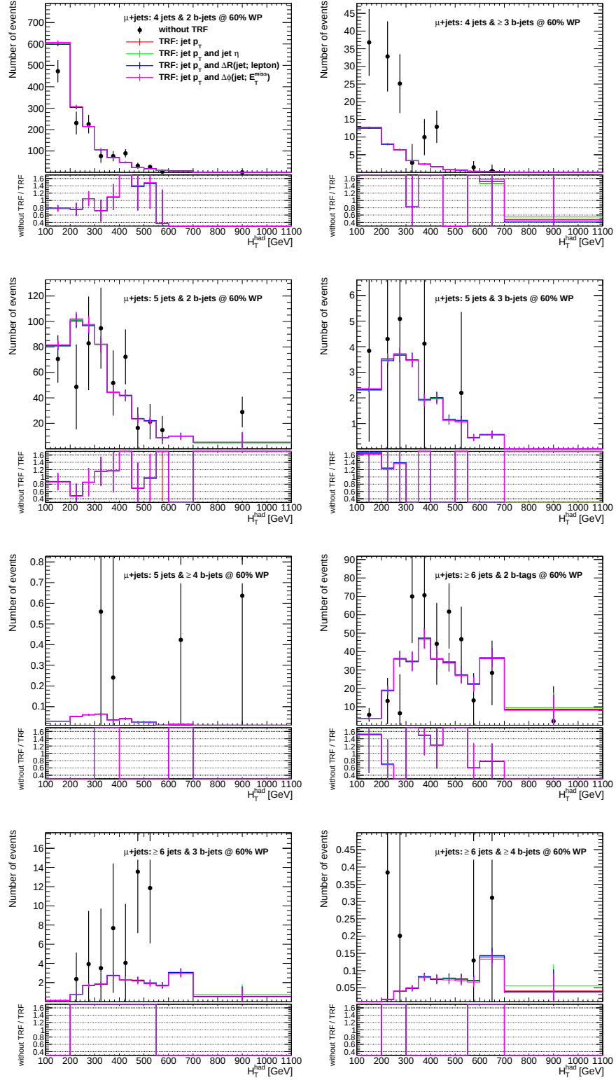
Figure B.3.: Comparison of the event yields of the fake estimation with and without the TRF method. Selection: muon + jets with a b -tagging WP of 60 %.
