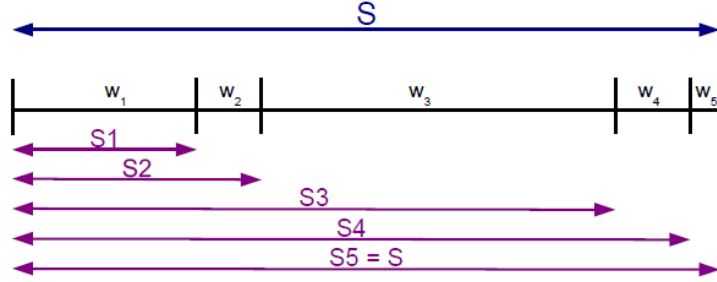
Figure 4.1.: Illustration of the choice of permutation in a case with five possible permutations (e.g. one b -tag among five jets). The total sum S is divided in partial sums S_i , with S_5 = S . A random number is then generated between 0 and S . Depending on the interval S_i - S(i-1) (with S_0 = 0 ) that includes this number, a corresponding TRF weight w_i is selected, e.g. for a random number between S_2 and S_3 the permutation three with TRF weight w_3 is chosen.
