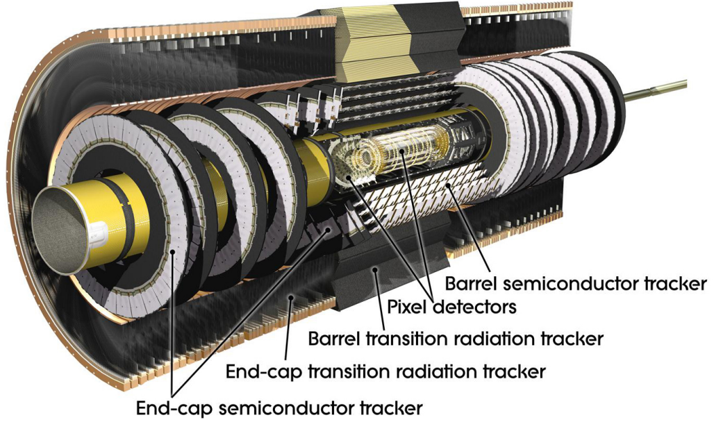
Figure 3.4.: Overview of the inner detector (without the IBL). © CERN
