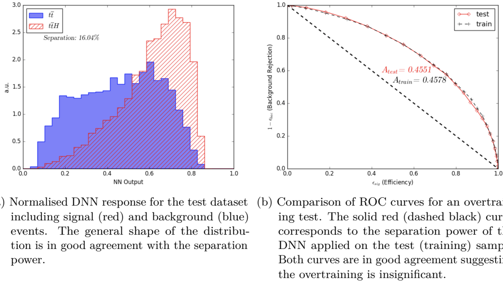
Figure 5.20.: Separation power of the deep neural network using high-level variables.
