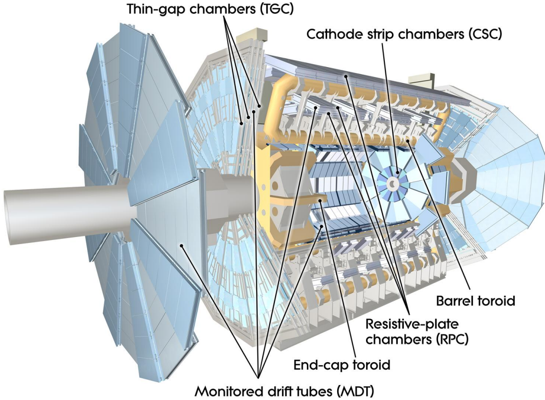
Figure 3.6.: Overview of the muon spectrometer. © CERN
