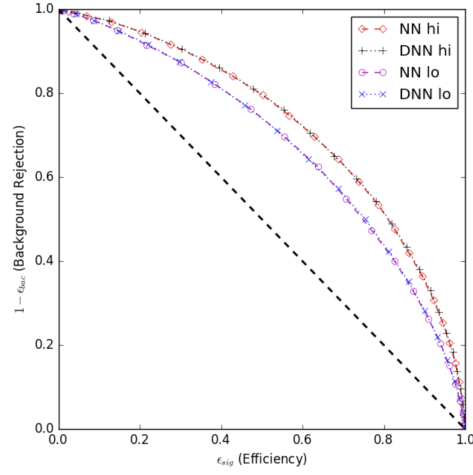
Figure 5.23.: Comparison of ROC curves for a single (shallow) and three layered (deep) NN using low- (lo) and high-level (hi) variables.
