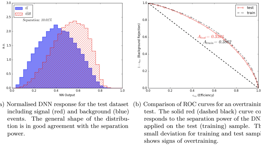
Figure 5.22.: Separation power of a deep neural network using low-level variables.
