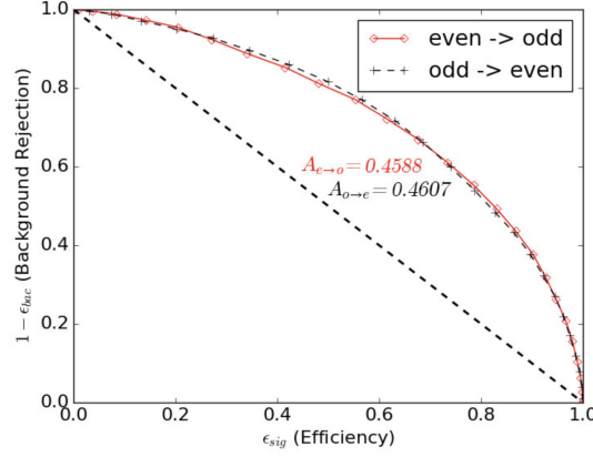
Figure 5.19.: Comparison of ROC curves for a two-fold validation test. The solid red (dashed black) line corresponds to the ROC curve obtained by training in the even (odd) and testing in the odd (even) dataset. Both curves are in good agreement suggesting the training procedure is independent of the training set.
