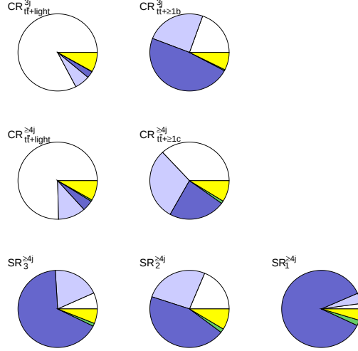
(b) Dilepton channel.
