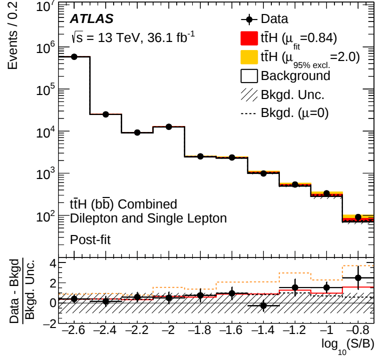
Figure 5.36.: Signal and background yields as a function of \log_{10}(S/B) , compared to data for all bins used in the combined fit of the single-lepton and dilepton channels. The signal is shown normalised to the best-fit value and to the excluded value at 95 % confidence level, including the background prediction from the fit. In addition, the pulls of the data relative to the background prediction are compared to the pulls of the signal-plus-background prediction from the fit for \mu = 0.84 ( \mu = 2 ) and represented as a solid red line (dashed orange line). For the background-only hypothesis the pulls are drawn as a dashed black line. Underflow is included in the first bin.
