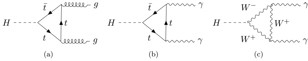
Figure 2.7.: Feynman diagrams of decay channels of the Higgs boson involving virtual loop contributions.
