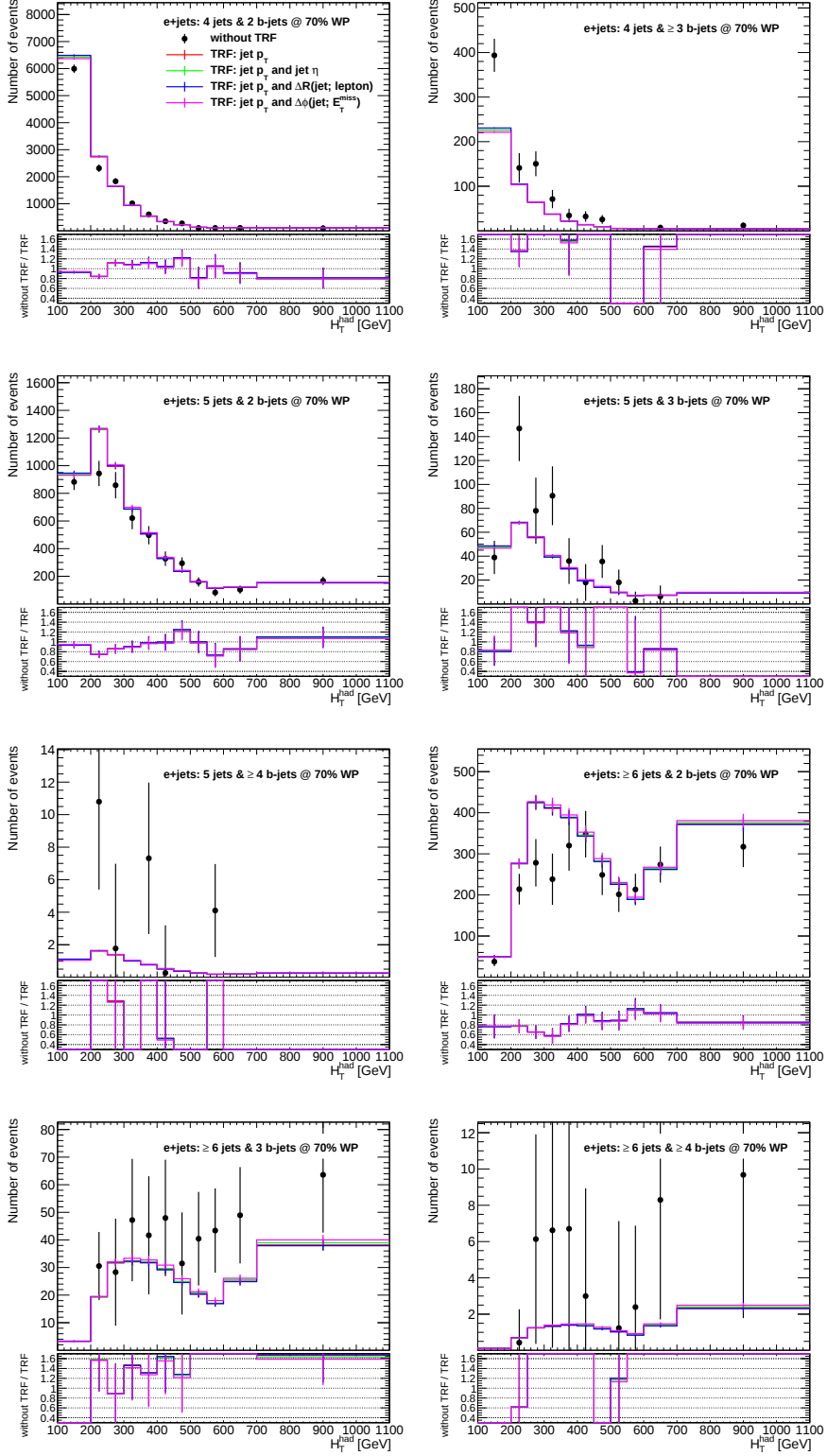
Figure B.4.: Comparison of the event yields of the fake estimation with and without the TRF method. Selection: electron + jets with a b -tagging WP of 70 %.
