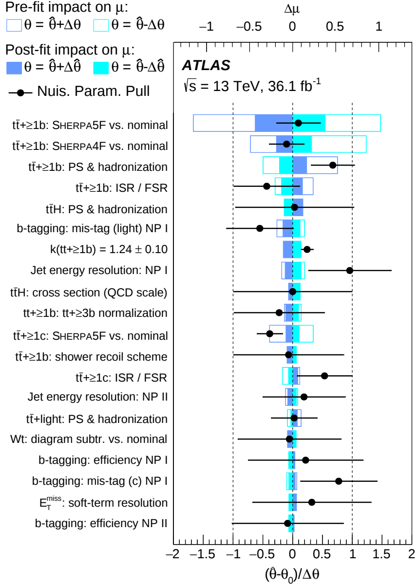
Figure 5.34.: Ranking of the 20 nuisance parameters with the largest contribution to the total uncertainty (ranked by decreasing contribution). Comparing the best-fit value of \mu to the fit result obtained with post-fit nuisance parameter values, \hat{\theta} , shifted by their pre-fit (post-fit) uncertainties \pm\Delta\theta ( \pm\Delta\hat{\theta} ), gives the impact of each nuisance parameter, \Delta\mu . The black points indicate the pulls of the nuisance parameters relative to their nominal values, \theta_0 . k(t\bar{t} + \geq 1b) denotes to the floating normalisation of the t\bar{t} + \geq 1b background.
