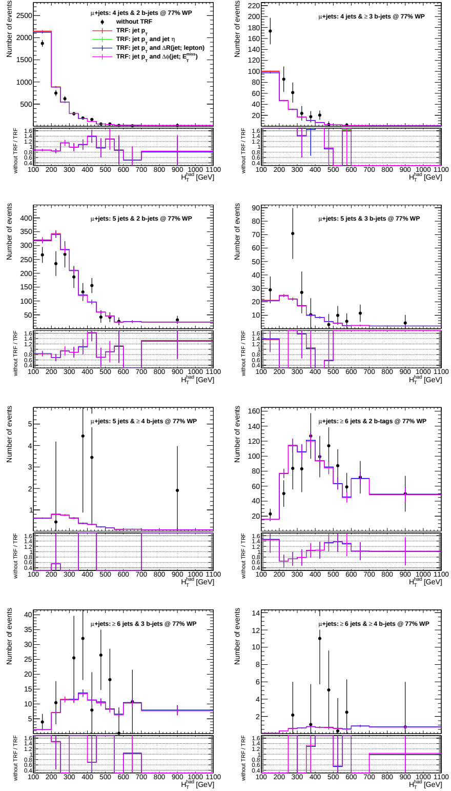
Figure B.7.: Comparison of the event yields of the fake estimation with and without the TRF method. Selection: muon + jets with a b -tagging WP of 77 %.
