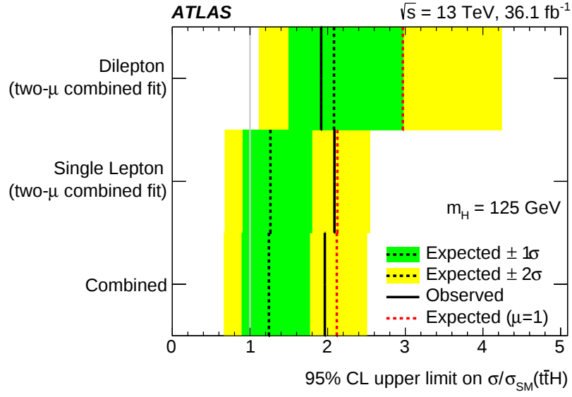
Figure 5.35.: Upper limits on \sigma(t\bar{t}H) at the 95% confidence level relative to the SM prediction in the single-lepton and dilepton channel and for the combination. Observed limits (solid black lines) as well as expected limits for the background-only hypothesis (dotted black lines) and for the SM hypothesis (dotted red lines) are shown.
