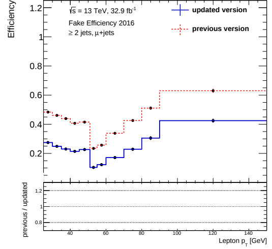
(b) Fake efficiency for the \mu + \text{jets} channel.
