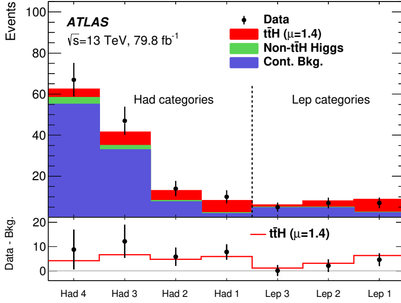
Figure 6.6.: Number of events in the different analysis regions of the H \rightarrow \gamma\gamma analysis, in a diphoton mass windows that contains 90 % of the t\bar{t}H signal.
