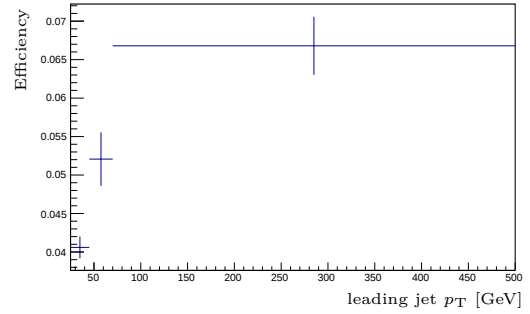
(f) 77 % WP: Efficiency in the case of a muon.
