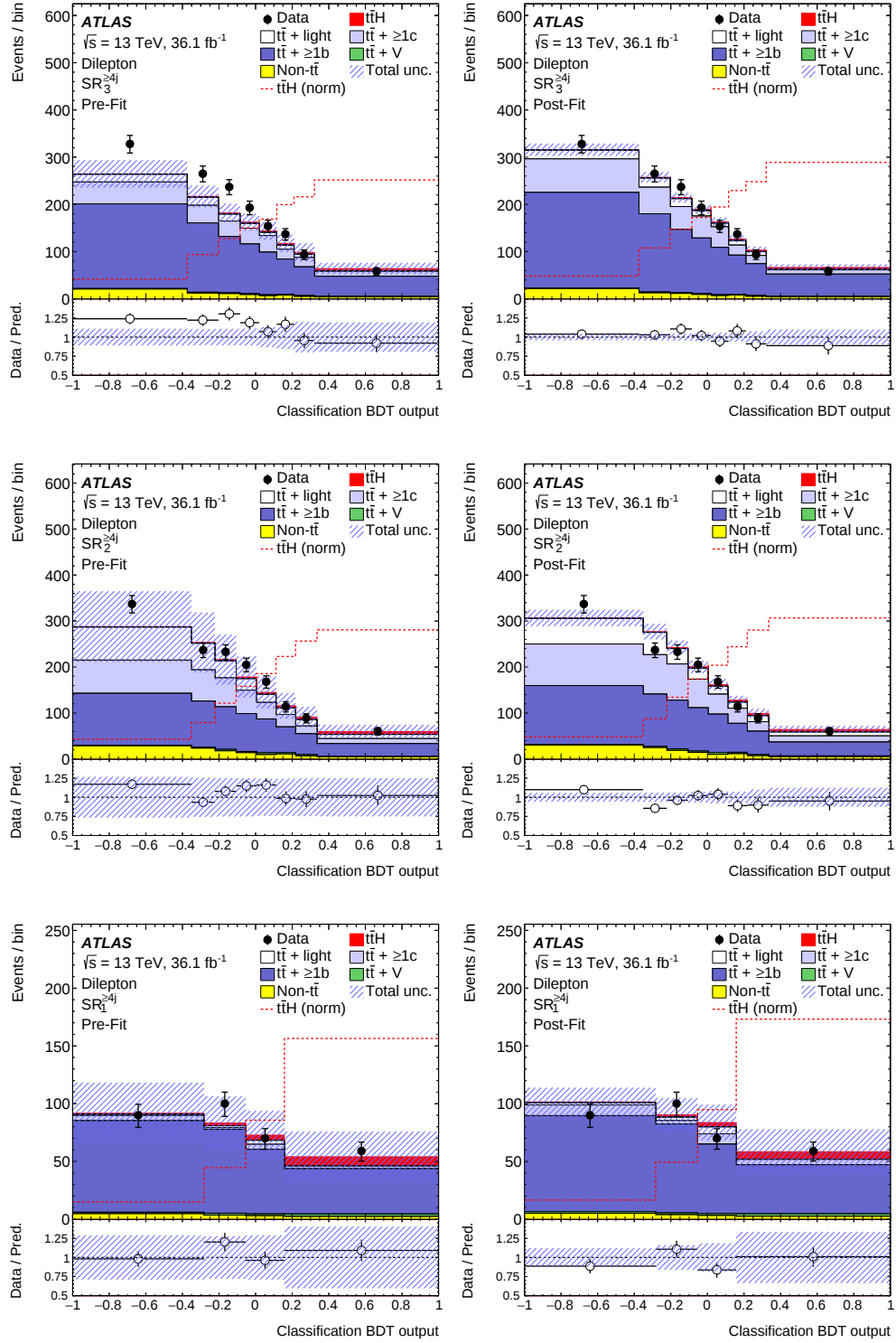
Figure 5.31.: Comparison between data and prediction for the BDT discriminant in the dilepton channel SRs before and after the fit.
