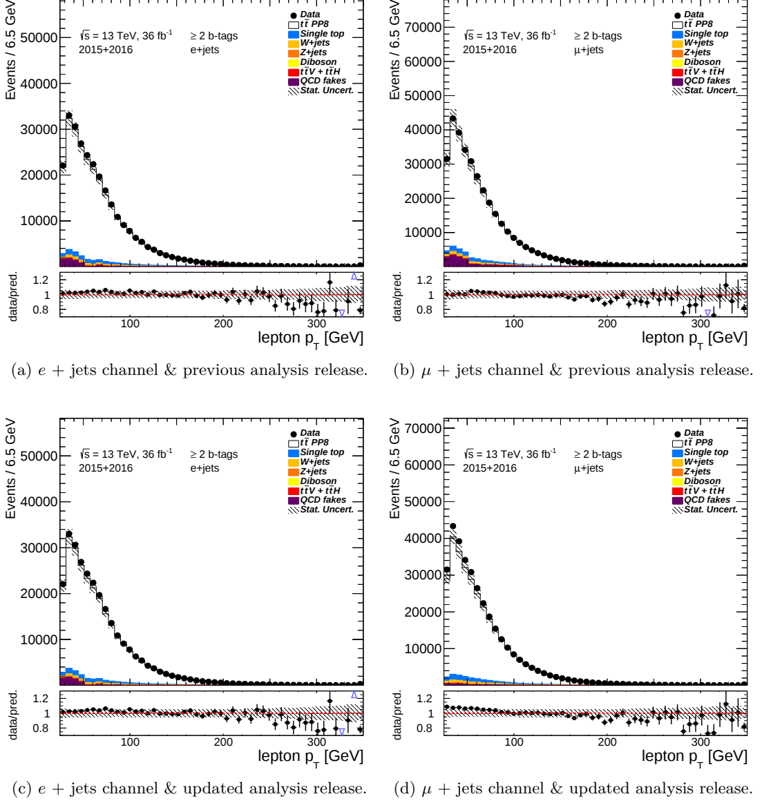
Figure 5.7.: Comparison between data and prediction for both analysis software versions for a selection of at least four jets with at least two b -jets as a function of lepton p_T . Figures (a) and (b) use the previous release, whereas Figures (c) and (d) use the updated release.
