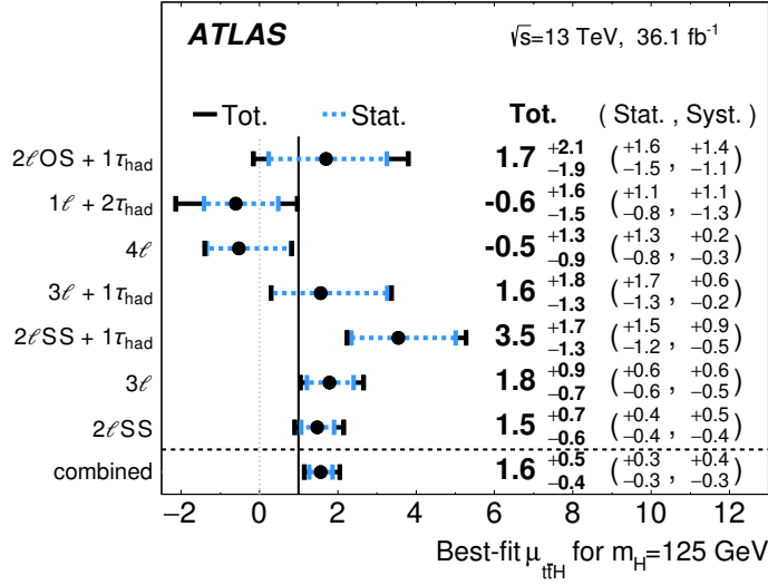
Figure 6.3.: The observed best-fit values of the t\bar{t}H signal strength \mu and their uncertainties of the H \rightarrow multilepton analysis for each channel (top) and combined (bottom).
