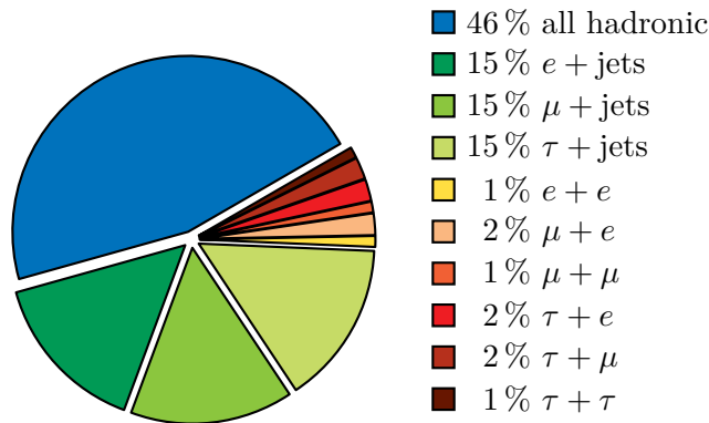
Figure 2.3.: The decay channels of a top-quark pair.
