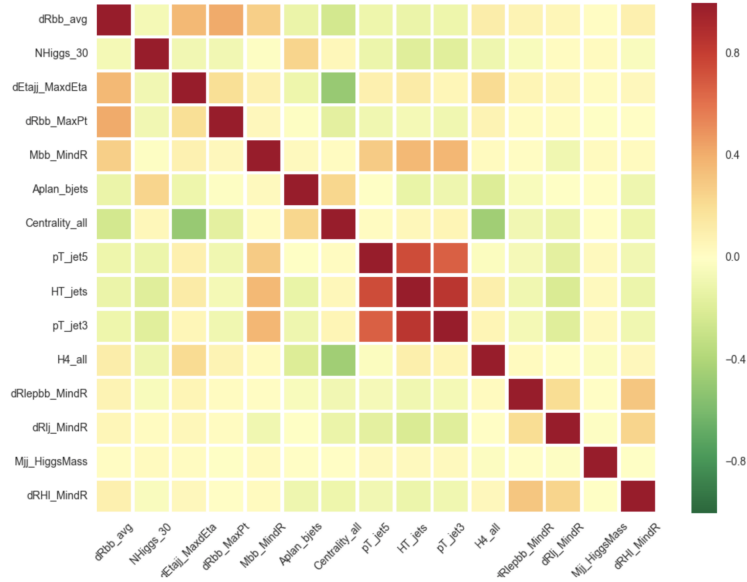
Figure 5.16.: Correlation matrix for the input variables. The scale on the right gives the strength of the correlation, where dark red corresponds to high correlation and dark green to high anti-correlation.
