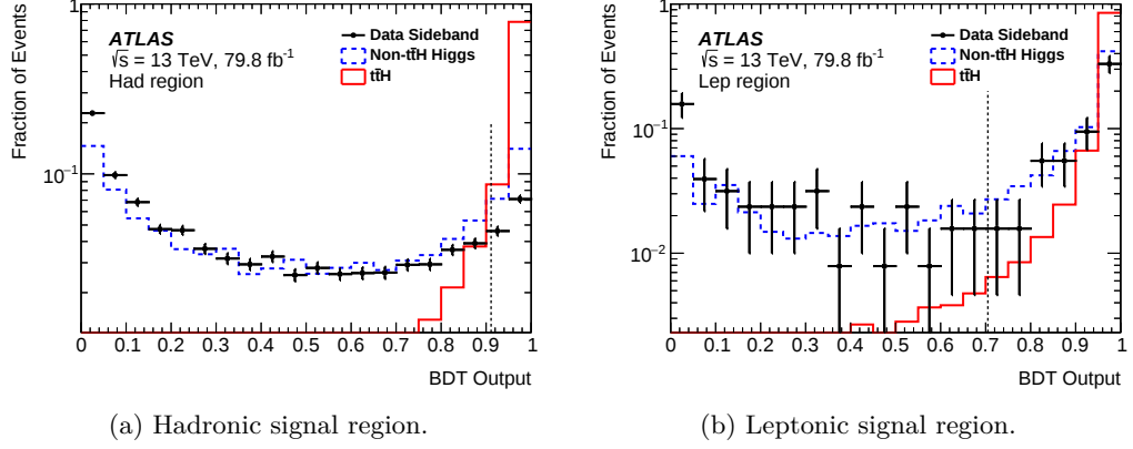
Figure 6.4.: BDT output for the hadronic and leptonic signal regions for the H \rightarrow \gamma\gamma decay channel. Events to the left of the vertical dashed line are rejected. The distributions are normalised to unity.
