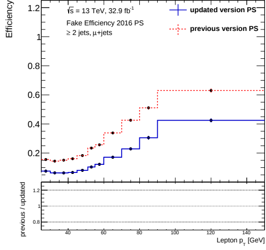
(b) Fake efficiency for the \mu + \text{jets} channel.
