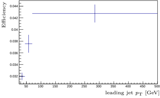
(c) 70 % WP: Efficiency in the case of an electron.
