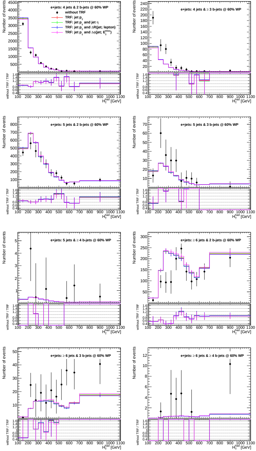
Figure B.2.: Comparison of the event yields of the fake estimation with and without the TRF method. Selection: electron + jets with a b -tagging WP of 60 %.
