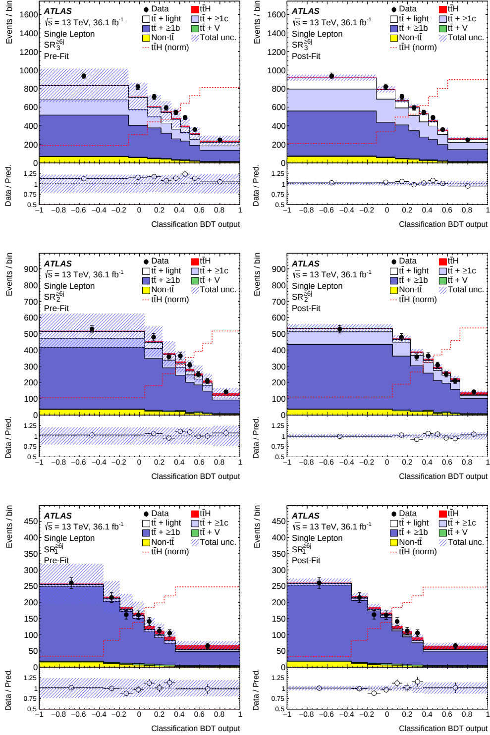
Figure 5.30.: Comparison between data and prediction for the BDT discriminant in the single-lepton channel six-jet SRs before and after the fit.
