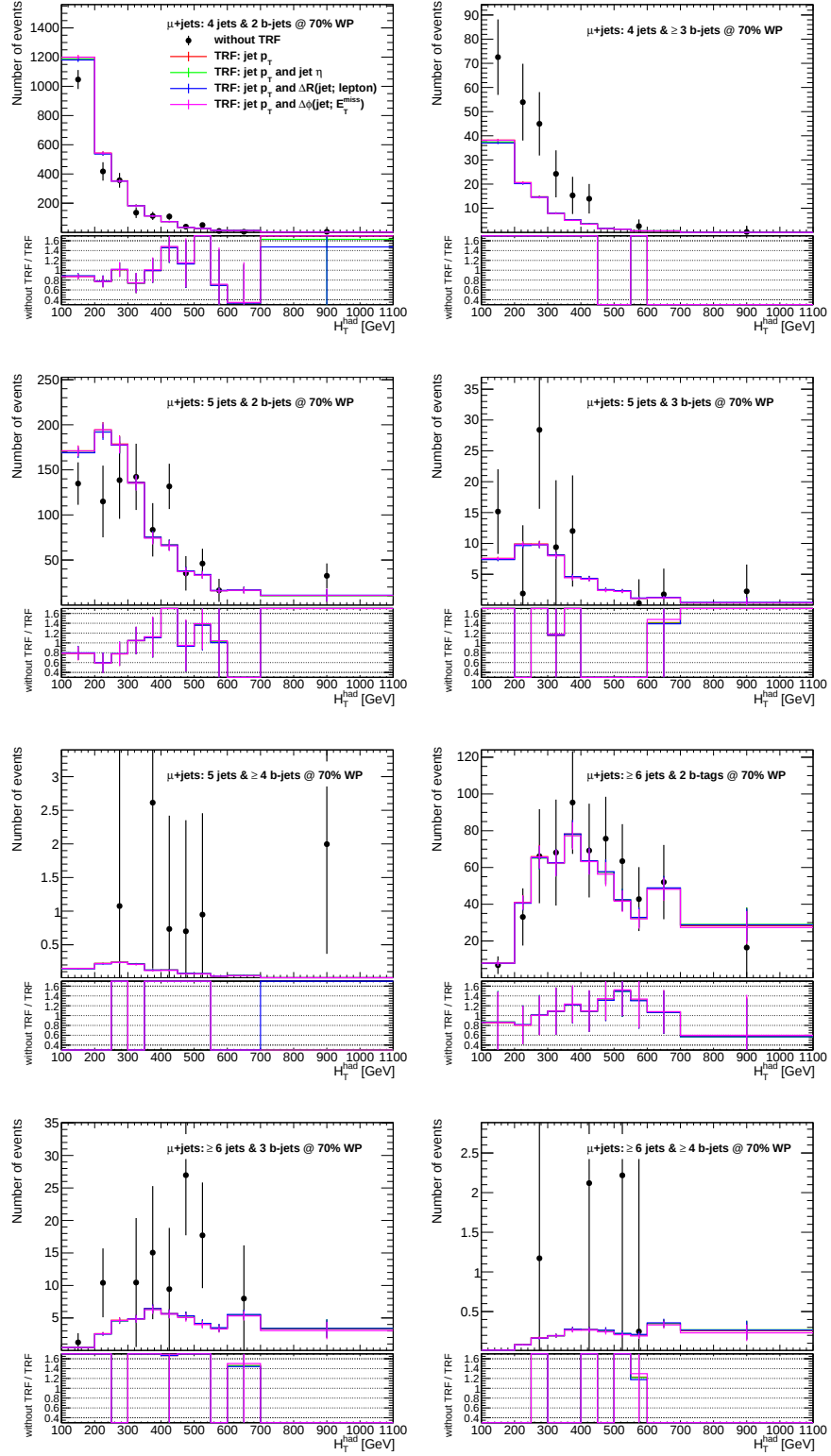
Figure B.5.: Comparison of the event yields of the fake estimation with and without the TRF method. Selection: muon + jets with a b -tagging WP of 70 %.
