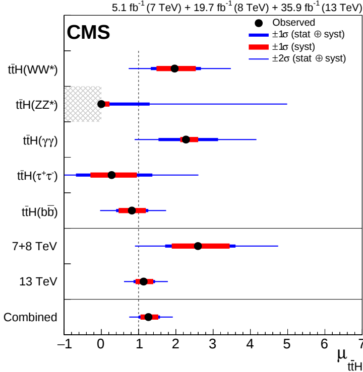
Figure 6.10.: Best fit value of the t\bar{t}H signal strength for the five individual decay channels considered (top), the combined result for 7 and 8 TeV alone and for 13 TeV alone (middle), and the overall combined result (bottom) from CMS.
