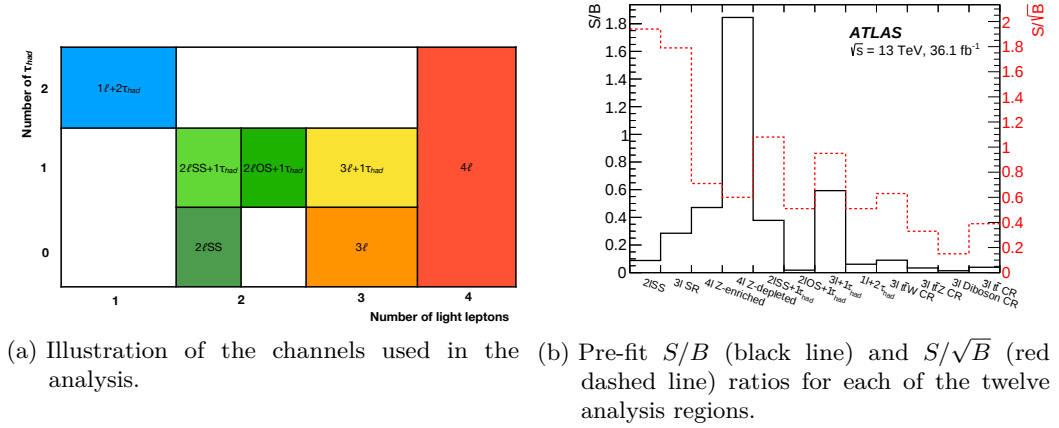
Figure 6.1.: Channels and regions of the H \rightarrow multilepton analysis.
