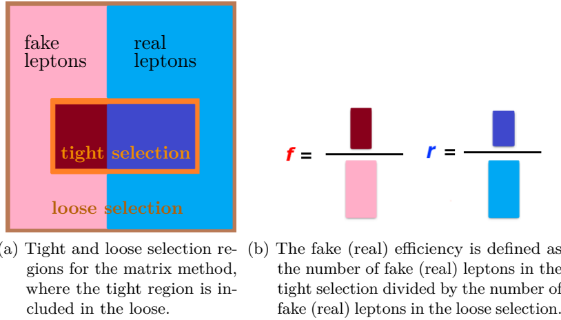
Figure 5.2.: Illustration of the matrix method.
