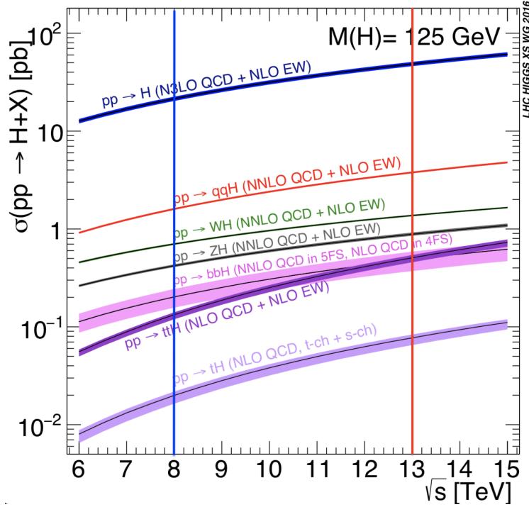
Figure 2.4.: The inclusive cross-section of the Higgs boson production mechanisms as a function of the centre-of-mass energy for proton-proton collisions. The process t\bar{t}H has a cross-section of \sigma_{\sqrt{s}=8 \text{ TeV}}(t\bar{t}H) = 0.13 \text{ pb} and \sigma_{\sqrt{s}=13 \text{ TeV}}(t\bar{t}H) = 0.50 \text{ pb} [65].
