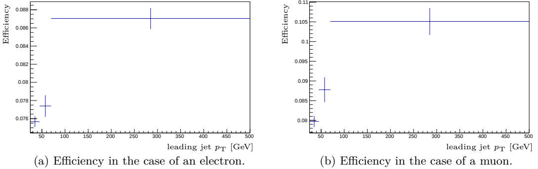
Figure 5.8.: TRF b -tagging efficiency calculated in a 4 jet inclusive region with at least 1 b -jet using a WP of 85 % in dependence of the leading jet p_T ; electrons (a) and muons (b) are considered separately.
