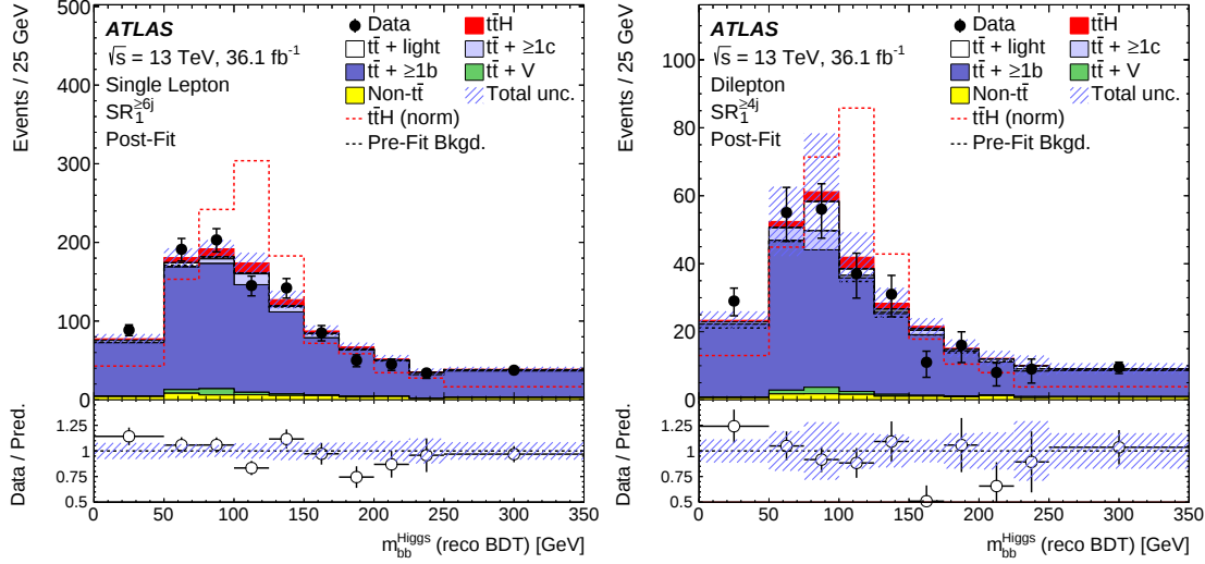
Figure 5.32.: Comparison between data and prediction for the Higgs boson candidate mass from the reconstruction BDT.
