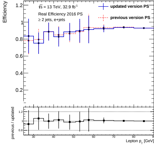
(c) Real efficiency for the e + \text{jets} channel.
