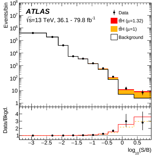
Figure 6.9.: Signal and background yields as a function of \log_{10}(S/B) , compared to data for all analysis categories. The signal is shown normalised to the best-fit value and to the SM prediction, including the background prediction from the fit. In addition, the ratio of the data to the background prediction is compared to the expected distribution including the signal for \mu = 1.32 ( \mu = 1 ) and represented as a solid red line (dashed orange line).
