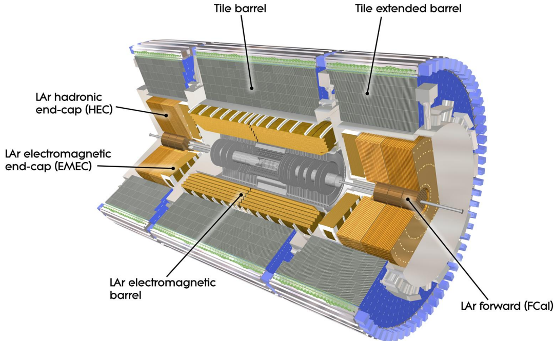
Figure 3.5.: Overview of the calorimeter system. © CERN
