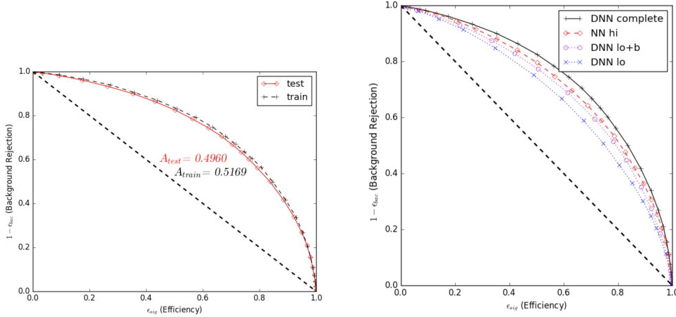
(a) ROC curves for a DNN in the best configuration using the complete variable set. (b) Comparison of performance using a variety of variable sets. A DNN using the complete variable set outperforms all other networks.
