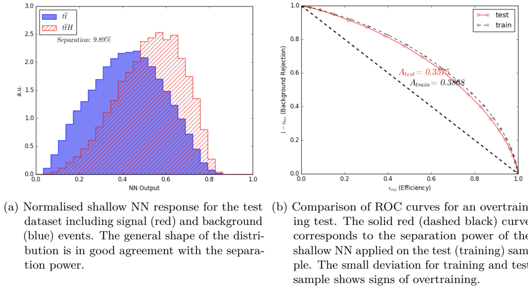
Figure 5.21.: Separation power of a shallow neural network using low-level variables.
