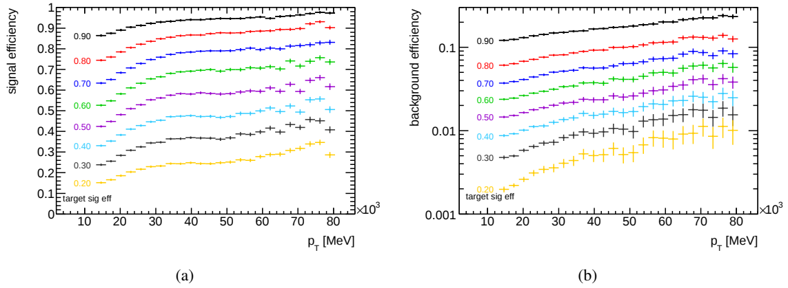
Figure 5.27: Signal (a) and background (b) efficiency \varepsilon_{ID} as a function of \tau_h momentum. The identified candidates pass a flat cut on the BDT score, targeting overall signal efficiencies of 90%, 80%, 70%, 60%, 50%, 40%, 30% and 20%. The tau candidates are 1-prong \tau_h from a simulated Z \rightarrow \tau\tau sample (signal) and multi-jet events from data (background).
