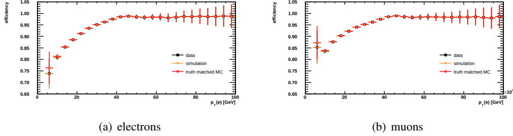
Figure B.2: Efficiency of the track isolation requirement p_T^{\text{iso}(0.4)}/p_T < 0.1 as a function of p_T for (a) electrons and (b) muons. The efficiency is measured on all probe leptons for data and simulation, as well as on truth-matched probe leptons only.
