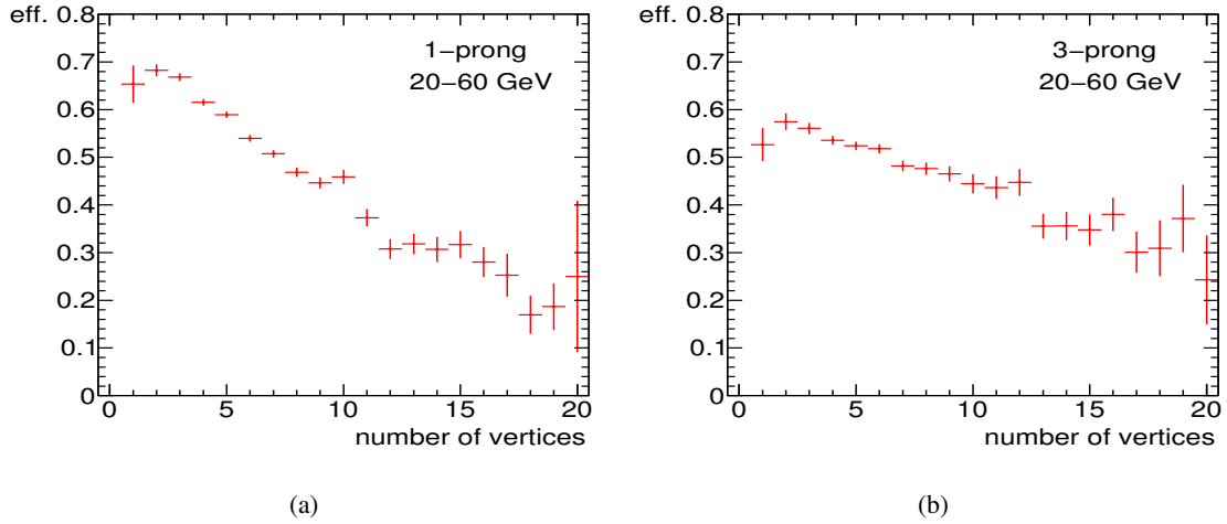
Figure 5.10: Signal efficiency \varepsilon_{ID} as a function of the number of vertices for (a) 1-prong \tau_h and (b) 3-prong \tau_h . The cut on the BDT score is neither tuned in p_T nor N_{vtx} . It targets an overall 50% signal identification efficiency. The BDT is trained inclusive for all pile-up conditions using the same variables and parameters as the 2011 BDT tau ID.
