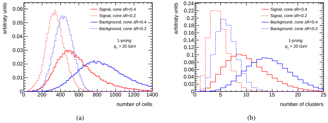
Figure 5.12: Number of (a) cells and (b) clusters for the two cone sizes \Delta R < 0.4 (continuous line) and \Delta R < 0.2 (dashed line) for 1-prong signal and background candidates. Only cells associated to clusters are considered. The signal candidates are from simulated Z \rightarrow \tau\tau decays, and the background candidates are from a simulated dijet sample. The distributions are normalised to unity.
