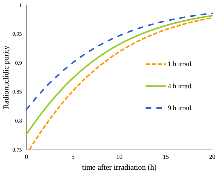
Figure 32: Graph showing the radionuclidic purity as a function of time after EOB and the effect of irradiation times. At longer irradiations the shorter half-life isotopes will approach saturation levels while the ^{135}\text{La} production rate will be almost unchanged. This causes the radionuclidic purity to increase as a function of irradiation time.
