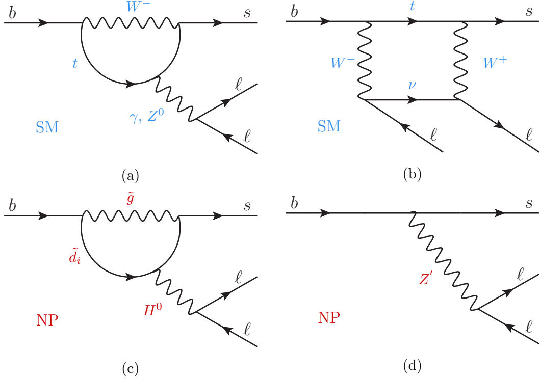
Figure 2: Feynman diagrams for the FCNC transition b \rightarrow s \ell^+ \ell^- : in the SM (a,b) and in possible NP scenarios [15, 16, 17] (c,d).
