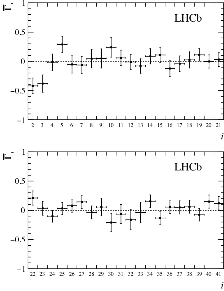
Figure 48: Measurement of the normalised moments, \bar{\Gamma}_i , of the decay B^0 \rightarrow K^+\pi^-\mu^+\mu^- in the range 1.1 < q^2 < 6.0 \text{ GeV}^2/c^4 and 1330 < m(K^+\pi^-) < 1530 \text{ MeV}/c^2 . The uncertainties shown are the quadratic sum of the statistical and systematic uncertainties.
