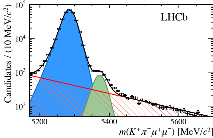
Figure 42: Invariant mass m(K^+\pi^-\mu^+\mu^-) for the control decay B^0 \rightarrow J/\psi K^{*0}(892) . The solid black line represents the total fitted function. The individual components of the B^0 \rightarrow J/\psi K^{*0} (blue shaded area), B_s^0 \rightarrow J/\psi \bar{K}^{*0} (green shaded area) and combinatorial background (red hatched area) are also shown.
