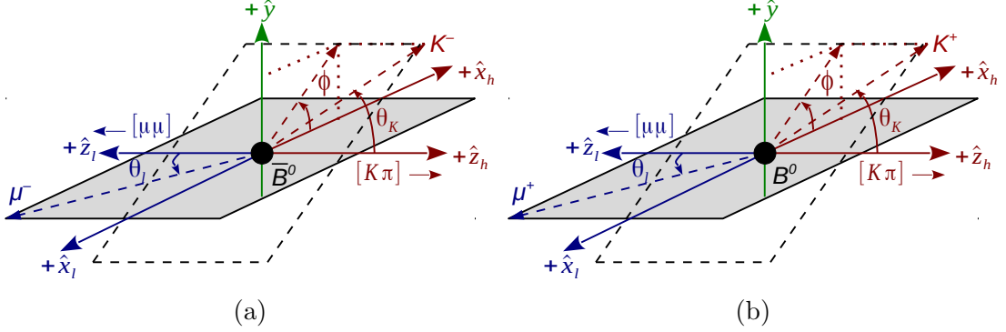
Figure 37: Angle conventions for the (a) \bar{B}^0 \rightarrow K^- \pi^+ \mu^- \mu^+ (b) B^0 \rightarrow K^+ \pi^- \mu^+ \mu^- as described in Ref. [84]. The leptonic and hadronic frames are back-to-back with a common \hat{y} axis. For the dihedral angle \phi between the leptonic and hadronic decay planes, there is an additional sign flip \phi \rightarrow -\phi compared to previous LHCb analyses [66, 67, 68, 69].
