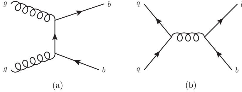
Figure 6: Feynman diagrams of the leading-order production processes for b\bar{b} pairs in proton-proton collisions. These are (a) gluon-gluon fusion and (b) quark-antiquark annihilation [23].
