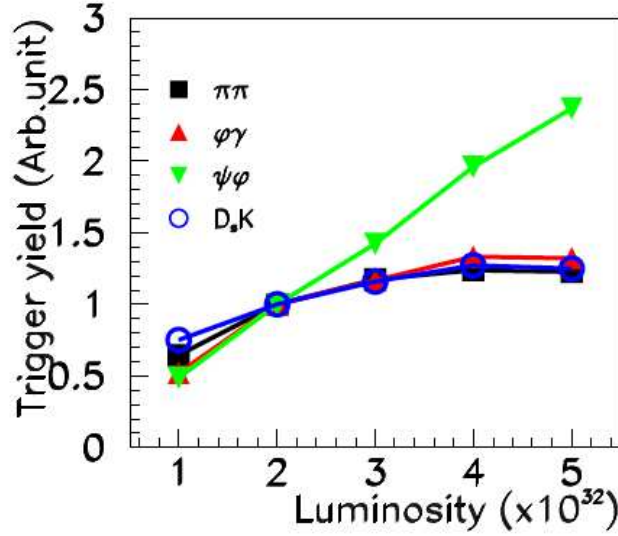
Figure 13: The trigger yield as a function of instantaneous luminosity for different decays of B mesons [48].
