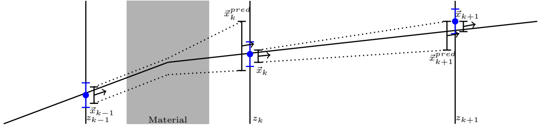
Figure 19: A schematic diagram of the Kalman filter showing the prediction of a state z_k given a state at z_{k-1} . The state at z_k is subsequently updated with information of the measurement at this position. This process is repeated until all measurements have been added.
