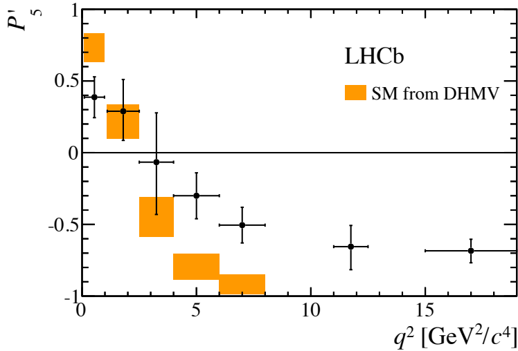
Figure 34: Results of the measurement of the observable P'_5 by the LHCb collaboration. The SM predictions are taken from Ref. [71].
