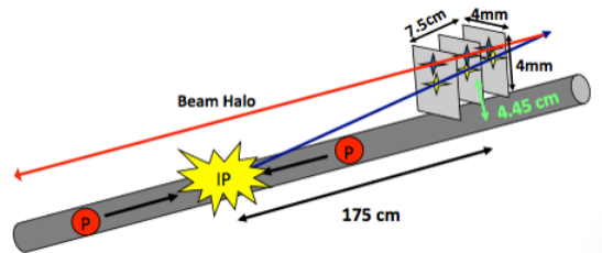
Figure 3.6: An artist's rendition of a single PLT telescope in relation to the interaction point of CMS. Shown are two types of signals which the PLT is able to distinguish due to particle track reconstruction from position measurements with pixelated detectors in three consecutive planes. Events from the IP due to proton collisions, and beam halo events. Beam halo consists of charged particles which are carried around the LHC but do not originate from the interaction point and hence do not measure luminosity. The contribution of halo tracks to the triple-coincidence rate must be subtracted offline based on the track reconstruction.
