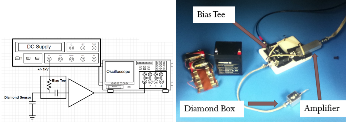
Figure 3.11: A schematic of the TCT setup is shown on the left and a photograph of the setup is on the right.
