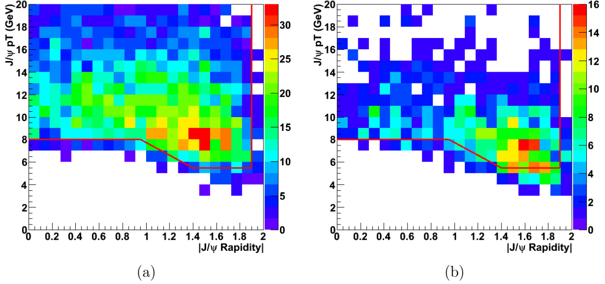
Figure 4.6: Plot (a) shows the J/\psi |y| versus p_T for the SPS-NLO MC sample after the muon acceptance criteria are applied. The J/\psi requirements are indicated by the red line in the figure. Plot (b) shows the same for the DPS MC sample.
