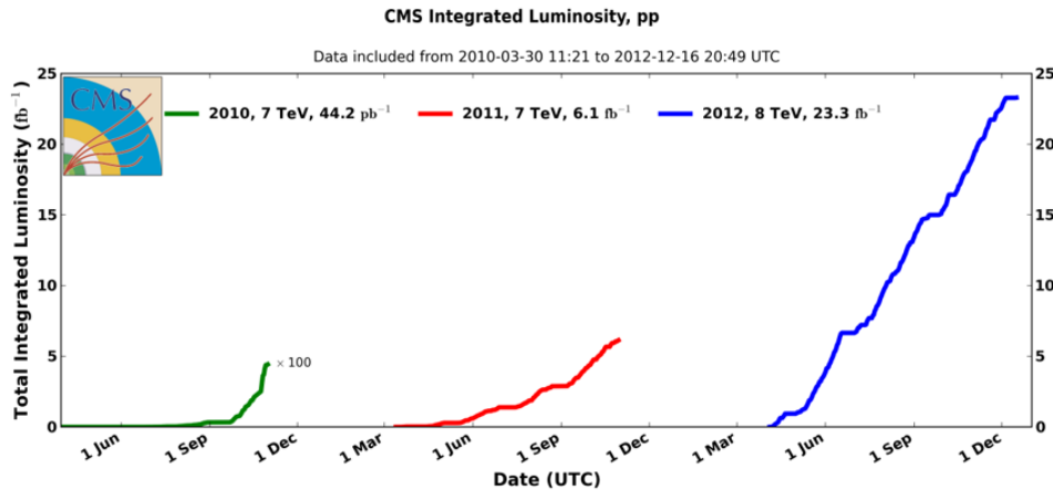
Figure 3.1: This plot shows the integrated luminosity delivered to the CMS detector during the years 2010 (green), 2011 (red), and 2012 (blue).
