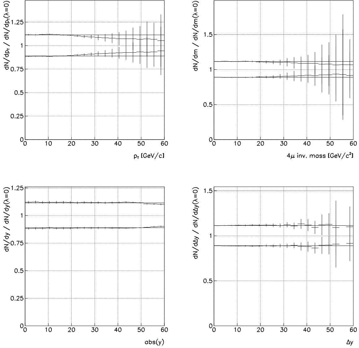
Figure 4.18: Ratios of acceptance corrected simulated SPS-NLO event distributions in 4-muon variables for different assumption of J/\psi polarization. The two ratios in each plot correspond to \lambda \pm 0.2 and have been fit to straight lines that are superimposed to the plot.
