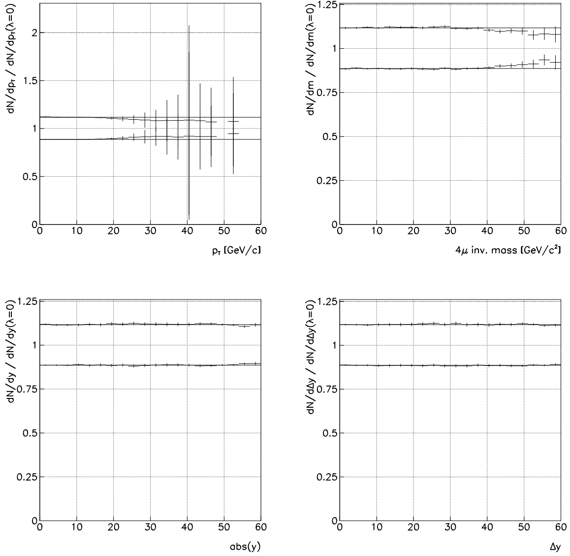
Figure 4.17: Ratios of acceptance corrected simulated DPS event distributions in 4-muon variables for different assumption of J/\psi polarization. The two ratios in each plot correspond to \lambda \pm 0.2 and have been fit to straight lines that are superimposed to the plot.
