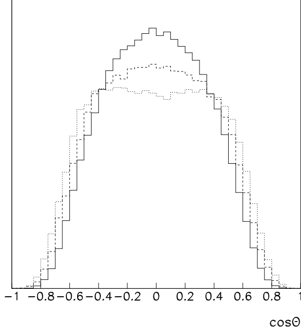
Figure 4.20: Normalized distributions of the angle \theta between the positive decay muon momentum in the rest frame of the J/\psi and the direction of flight of the J/\psi in the laboratory frame for different assumptions for \lambda , within the CMS muon acceptance. The height of the distributions at \cos \theta = 0 increases in the order \lambda = +1, 0, -1 .
