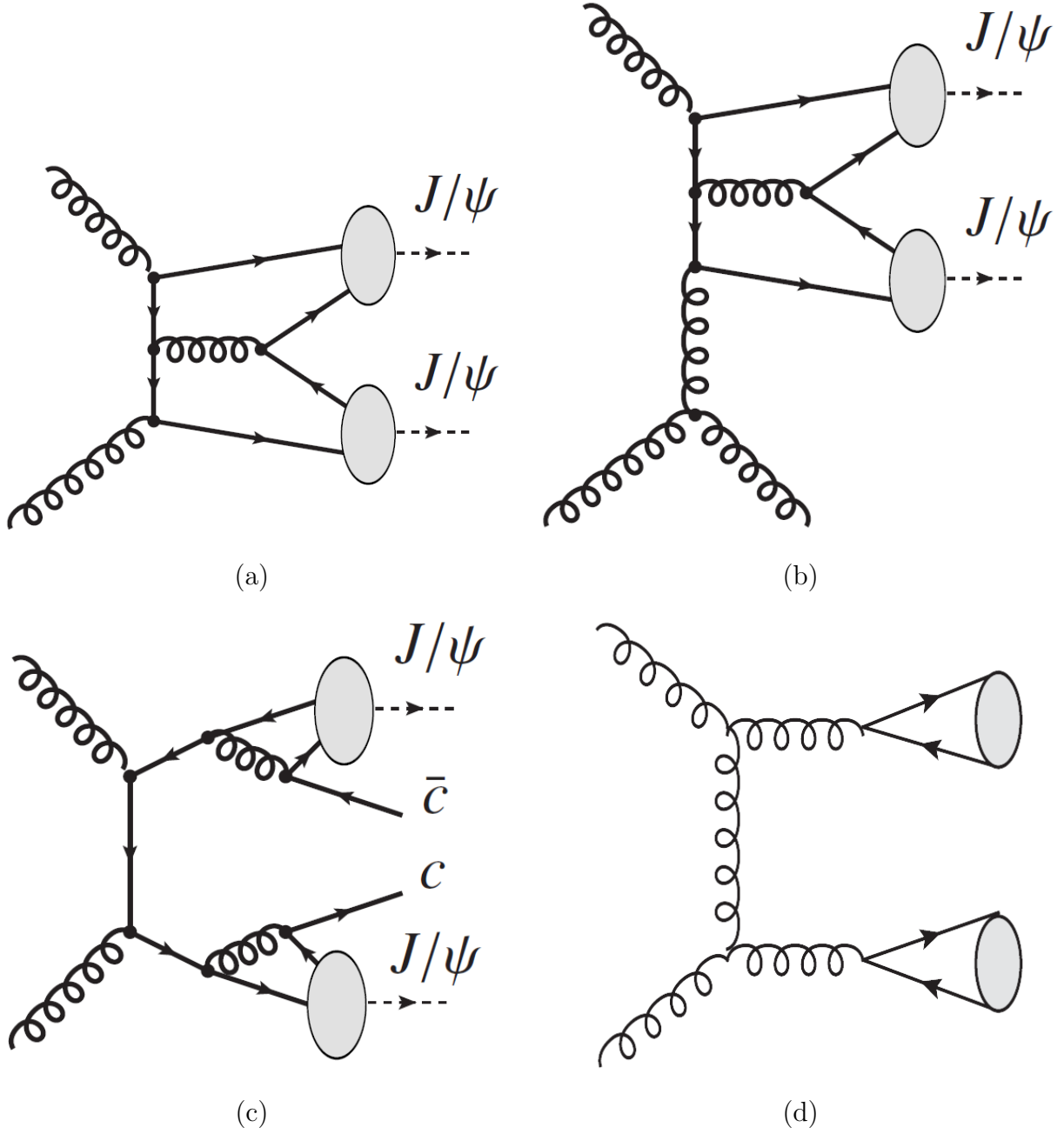
Figure 4.1: Examples of Feynman diagrams of SPS color-singlet prompt J/\psi pair production in pp collisions in (a) leading-order (LO), (b) next-to-leading order (NLO), and (c) next-to-next leading order (NNLO), and (d) SPS color-octet prompt J/\psi - pair production
