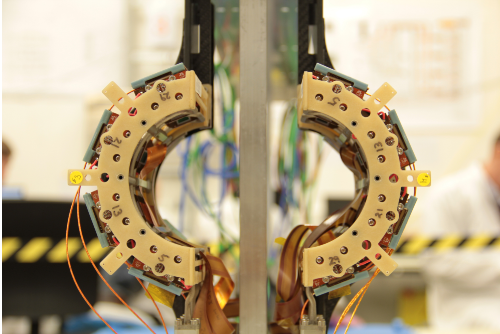
Figure 3.2: A photograph of one half of the PLT detector installed temporarily on metal rails in a clean room.
