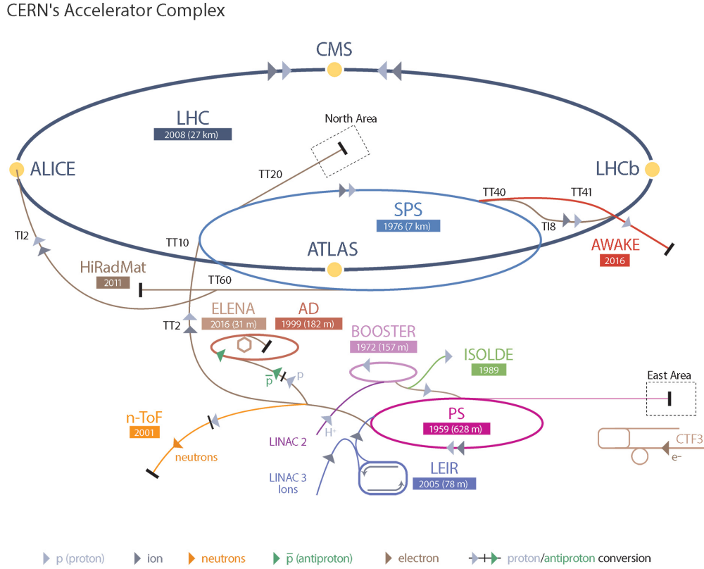
Figure 2.2: A schematic of all the accelerator facilities at CERN. The arrows show the direction of particle beams in each accelerator, the gray arrows representing the proton beams.
