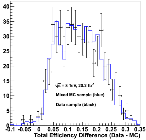
Figure 4.16: The difference of the event efficiency between the T&P tables from data and MC simulation ( \epsilon^{data} - \epsilon^{MC} ), evaluated with the selected data sample (data points) and with the reconstructed MC sample composed of 13% DPS events and 87% SPS-NLO events (blue histogram).
