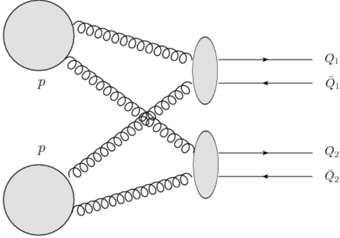
Figure 4.2: Production of two quark anti-quark pairs in the double parton scattering process.
