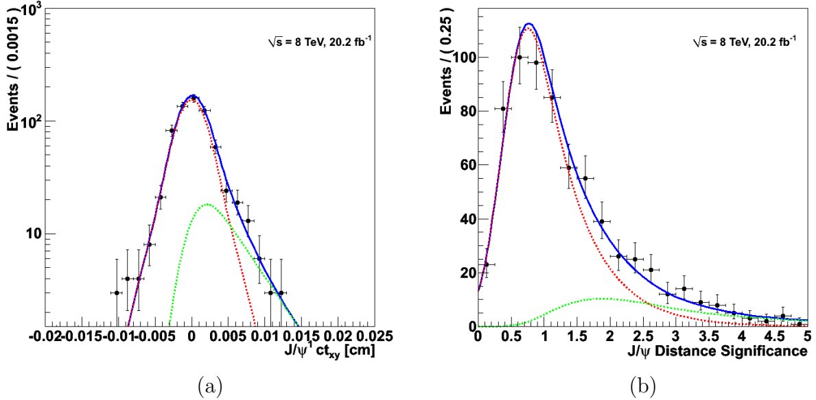
Figure 4.7: Maximum likelihood to the event sample with a greater than 0.5% 4\mu vertex probability requirement. The distribution of the fit variables ct_{xy} (a) and d^{J/\psi} (b) in data with the result of the fit superimposed. The solid blue line indicates the total fit, the dashed red line the signal and the dashed green line the background distribution.
