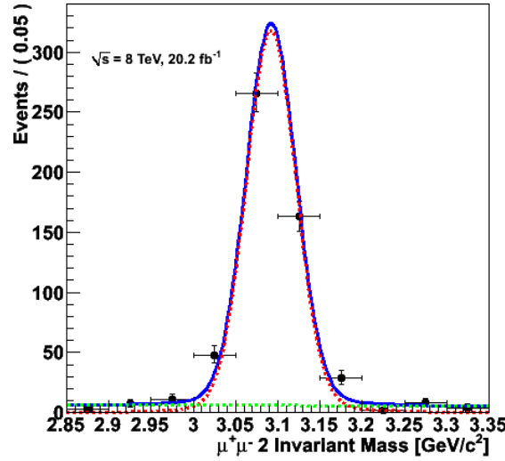
Figure 4.11: Dimuon mass distribution shown with signal and background fit on the full data sample.
