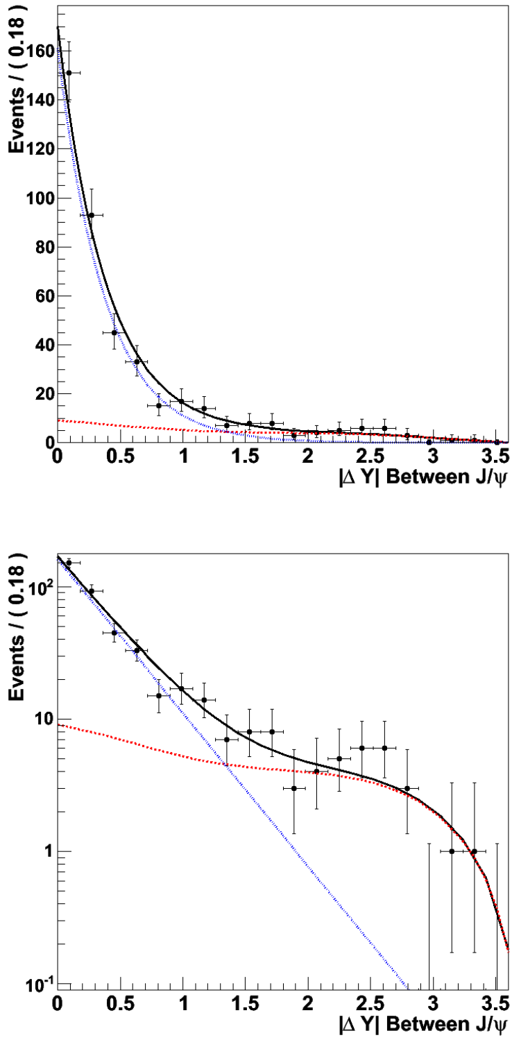
Figure 4.26: The plot on the top shows the data sample fit with the SPS (blue) and DPS (red) shapes. The bottom plot shows the same fit with a log scale.
