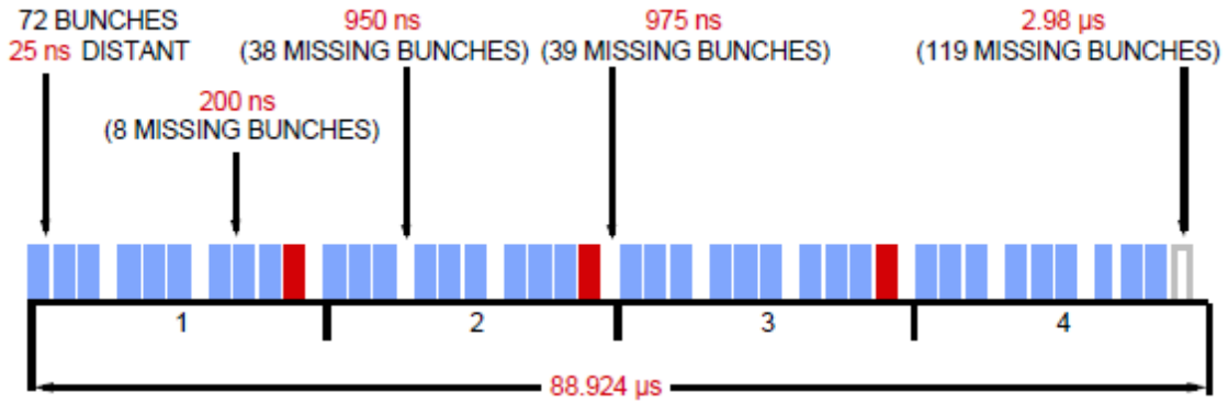
Figure 2.3: A schematic of a full bunch pattern in the LHC, showing the various gaps to accommodate kicker magnets. 72 bunch groups, called batches are accelerated in the PS and delivered to the SPS. The SPS then further accelerates the protons and transfers groups of 3 or 4 batches into the LHC.
