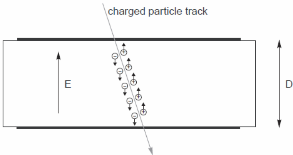
Figure 2.9: The mechanism of charge creation in a material is illustrated. An incident particle deposits energy in the form of electron/hole pairs which are drifted to the edges of the material by means of an applied electric field. The thickness D is about 300\ \mu\text{m} for CMS silicon detectors, and the typical electric field is 0.1\text{V}/\mu\text{m}
