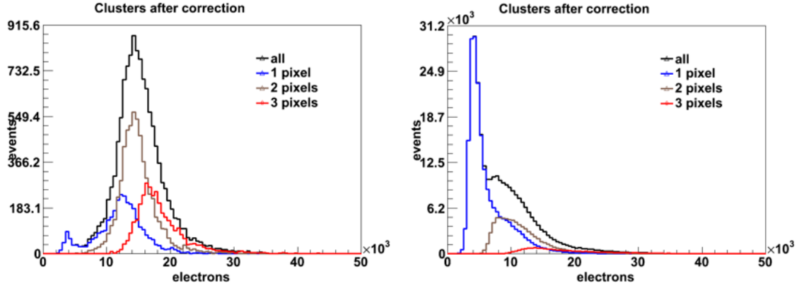
Figure 3.8: The left plot shows charge collection data from the pixel ROC. The ROC groups events such that adjacent pixels over threshold are measured together in a cluster. If charge is spread over 3 or more neighboring pixels, the event is classified as a \geq 3 pixel cluster (red). If only 2 pixels contain charge from the event, it is labeled as a 2 pixel cluster (brown). Single pixel clusters are shown in blue. The black trace is the sum of charge collected from all size clusters. On the right, is a charge signal which is indistinguishable from the noise, to illustrate how charge collection reduction in sensors harms their performance.
