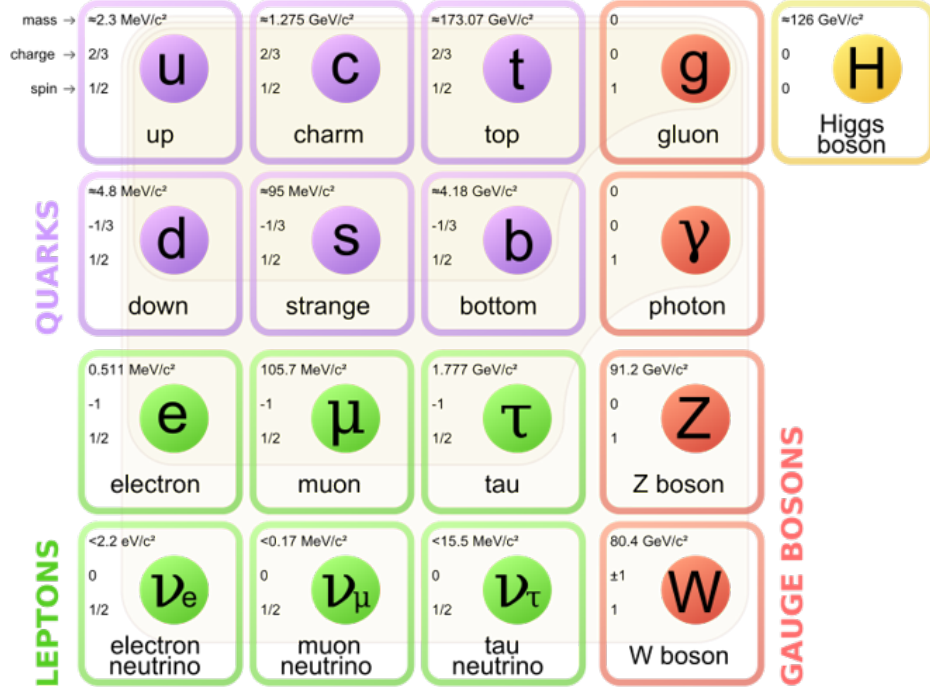
Figure 1.1: The particles of the Standard Model (SM) categorized into quarks, leptons and bosons
