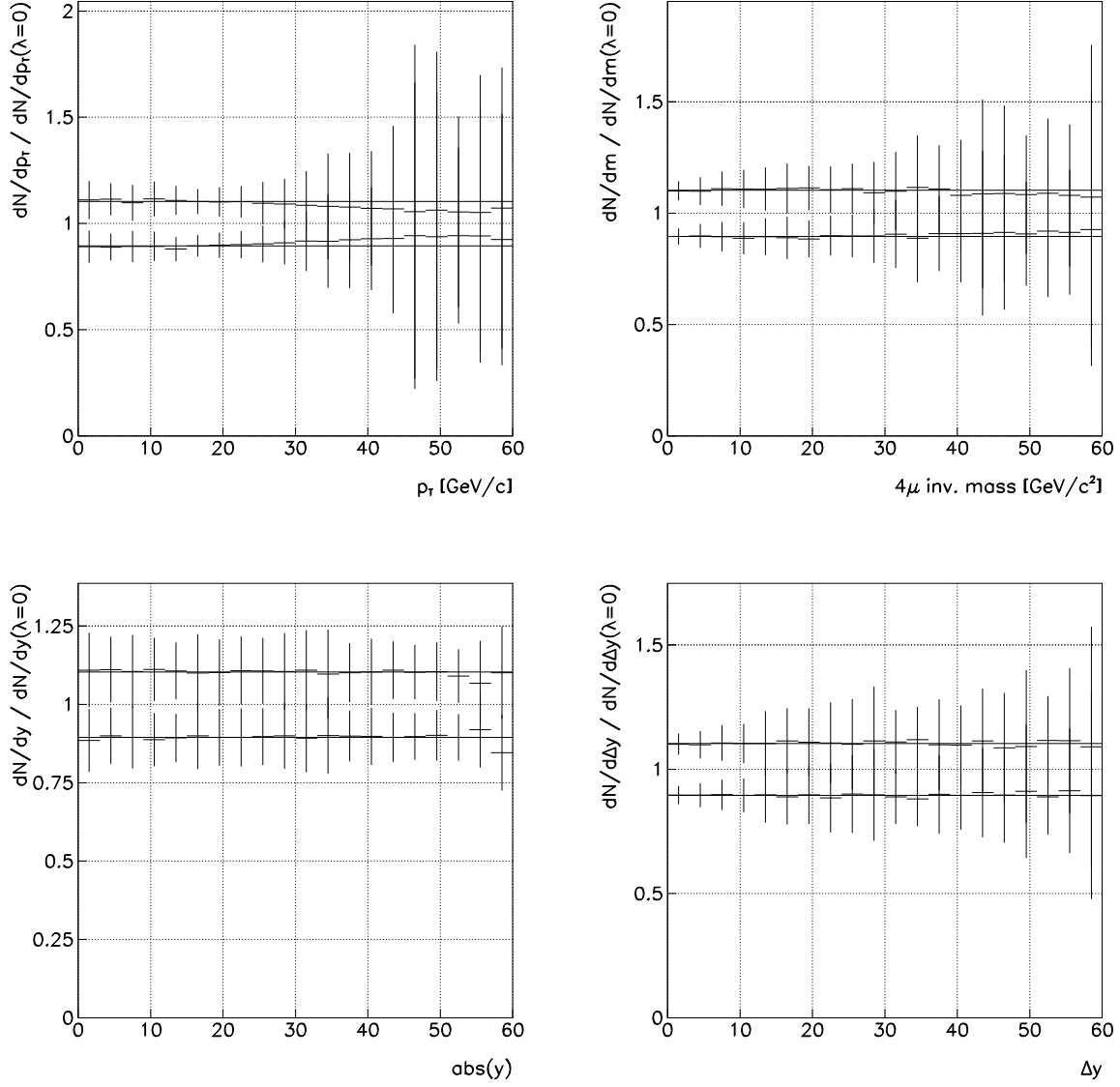
Figure 4.19: Ratios of acceptance corrected simulated data event distributions in 4-muon variables for different assumption of J/\psi polarization. The two ratios in each plot correspond to \lambda \pm 0.2 and have been fit to straight lines that are superimposed to the plot.
