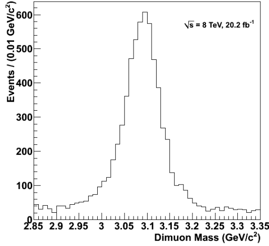
Figure 4.3: The plot shows the \mu\mu invariant mass for passing dimuon candidates in the mass interval allowed by the HLT.
