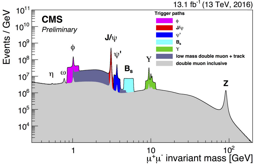
Figure 2.11: Dimuon Invariant mass for events collected with the various quarkonia related triggers. Strong excesses are observed where triggers include requirements on mass ranges, such as around J/\psi (red), \psi' (dark blue), and the set of Y resonances (light green). The signal Z \rightarrow \mu\mu is clearly visible around 90 GeV
