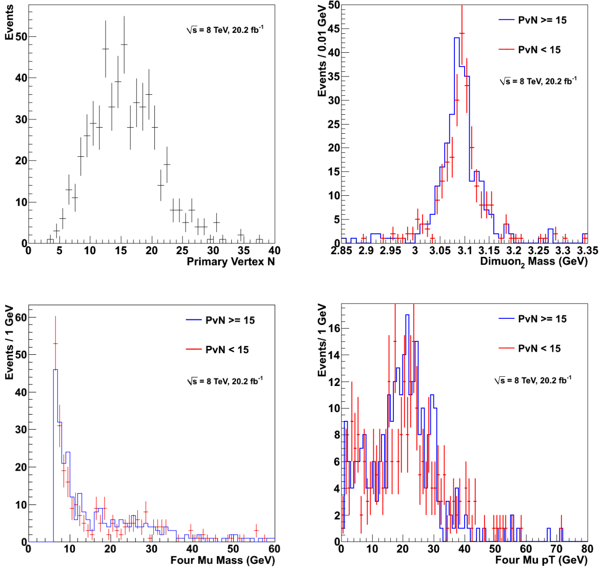
Figure 4.12: The distribution of primary vertices in selected events is shown in the upper left. Variable distributions shown split into low pileup ( PvN < 15 red) and high pileup ( PvN \geq 15 blue) events shown in the low p_T J/\psi \mu\mu invariant mass (upper right) the 4-Muon invariant mass (lower left) and the 4-muon p_T (lower right).
