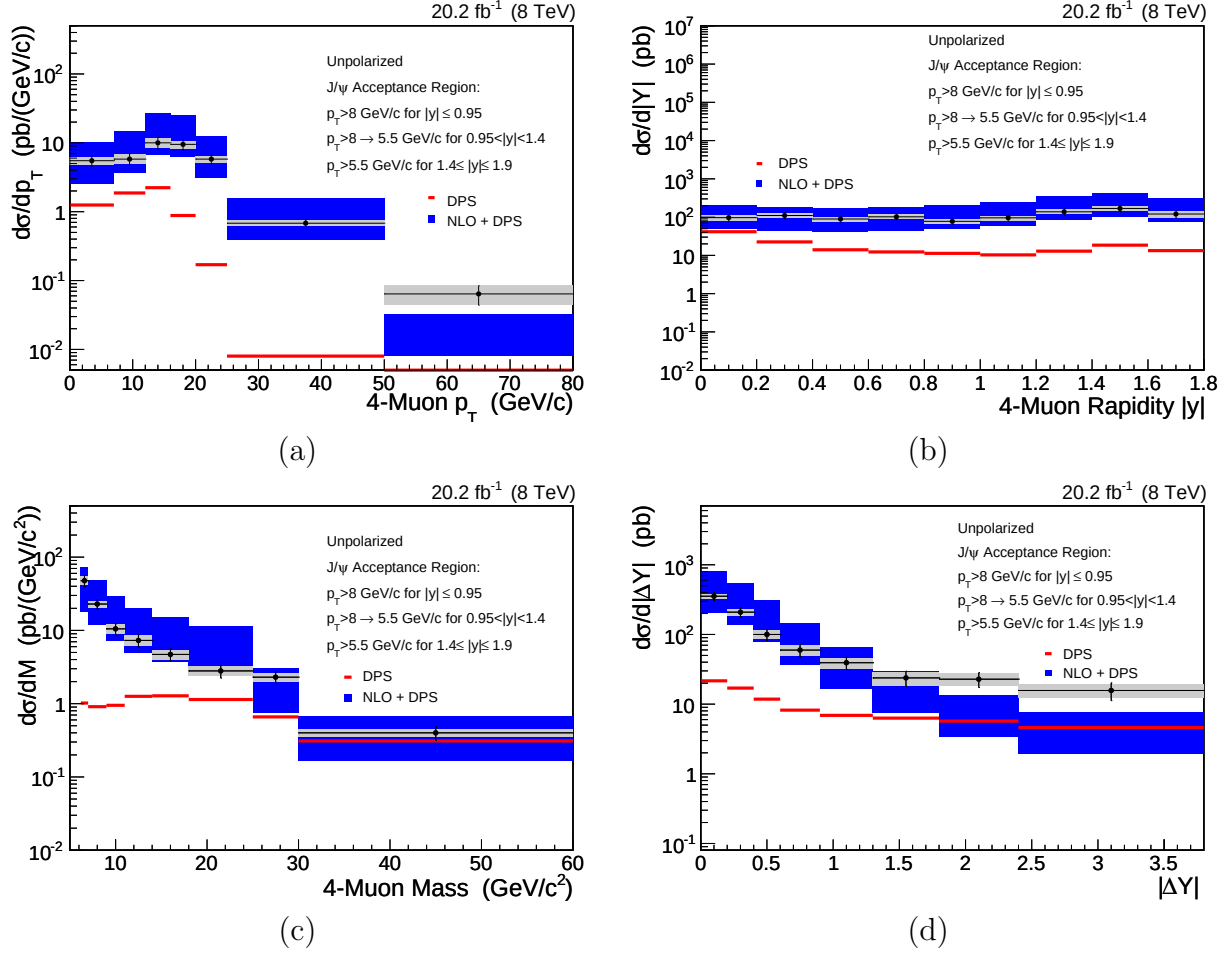
Figure 4.23: Differential cross section distributions for different 4-muon event variables, (a) transverse momentum, (b) the absolute value of the rapidity, (c) invariant mass, and (d) the absolute difference in rapidity between the two J/\psi . The points correspond to data, with statistical error shown as the gray box and the total uncertainty by the error bars. The NLO+DPS model is shown in blue with a model uncertainty of 60% as indicated by the blue boxes. The DPS contribution obtained relative to the cross section in data is shown in red without uncertainty.
