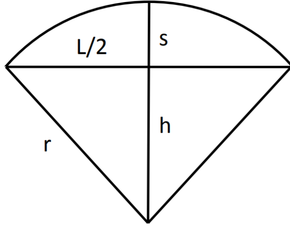
Figure 2.6: A diagram of the sagitta s for a particle passing through a region of length L with a constant magnetic field.
