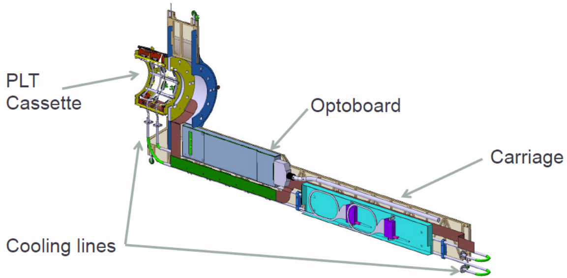
Figure 3.3: A schematic drawing of one quarter of the PLT detector. The sensors are located in the cassette, and the carriage holds front end electronics and cooling infrastructure. The carriage is inserted into the center of CMS such that the telescopes are 1.75 meters from the interaction point. 4 such quarters were installed in 2015.
