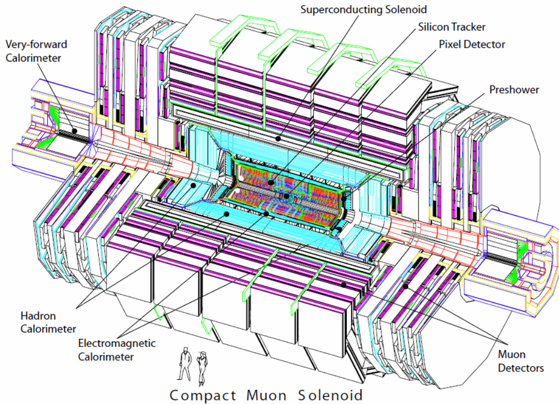
Figure 2.5: A cutaway of the CMS detector, with persons shown for scale comparison. The outermost layers are muon detectors placed between slabs of iron absorbers. The iron layers also function as return yoke for the magnetic field. From outside inwards the muon detectors are followed by the superconducting solenoid, the hadronic calorimeter, the electromagnetic calorimeter, the silicon strip tracker, and the innermost 3 layers are the silicon pixel detector. The beam pipe enters from each end of CMS and collisions take place in the center of the detector.
