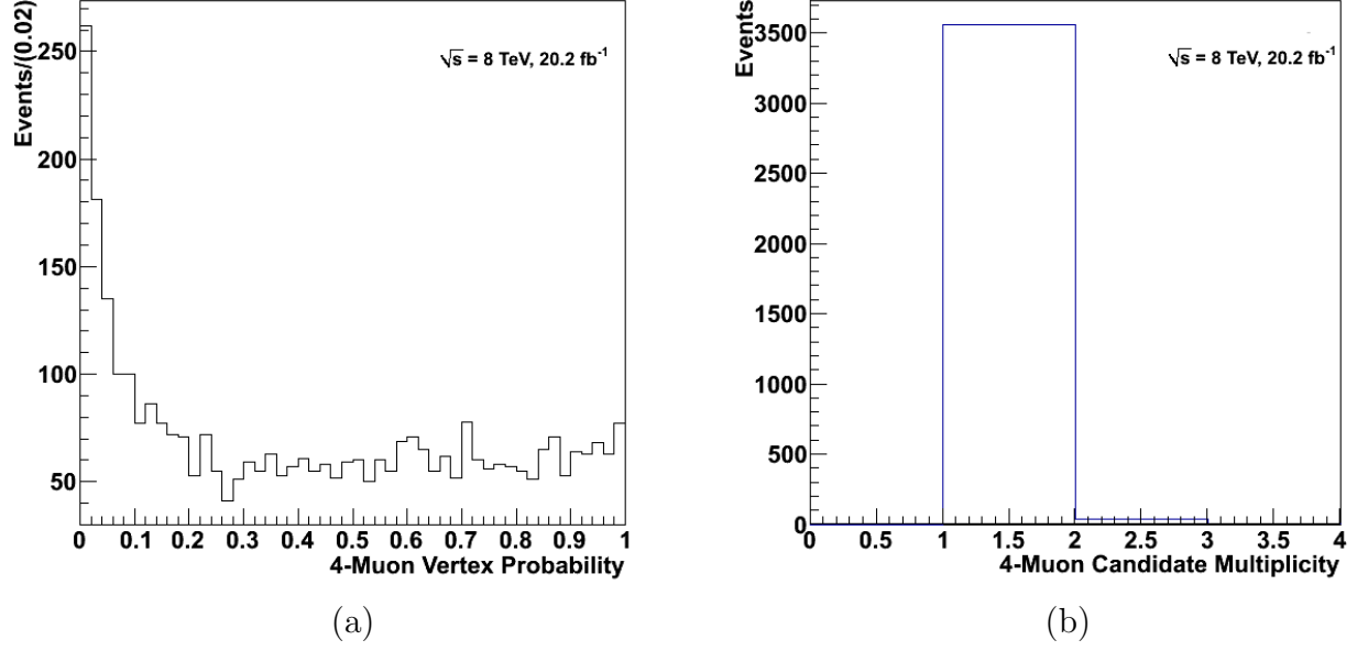
Figure 4.4: The probability distribution from the vertex fit to 4-muon candidates is shown in figure (a). Figure (b) shows the majority of events have only one 4-muon candidates and a small fraction contain 2 passing candidates. Only one candidate per event is chosen.
