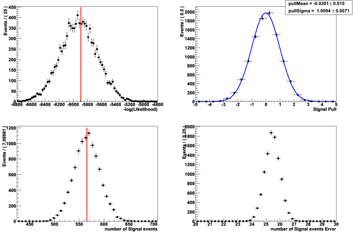
Figure 4.8: 10,000 toy MC of the CTxy and DSig fit were generated and refit. The distribution of NLL is shown in the upper left with a line at the NLL value of the main fit, the pull is shown in the upper right. The lower left plot is the distribution of number of signal in each toy with a line at the main fit value. The distribution of the uncertainty of Nsig is the lower right plot.
