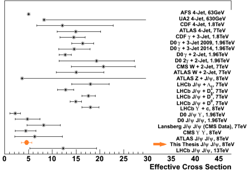
Figure 5.1: Effective cross section values from different experiments at various center of mass energies and for different final states. Values measured by the UA2 experiment [58], AFS experiment [24], ATLAS experiment [1, 4, 6, 2], the LHCb experiment [11, 8, 12], The D0 experiment [15, 16, 18, 13, 14], the CDF experiment [20, 19] and the CMS experiment [82, 51, 56]. The measurement made in this thesis is marked with orange.
