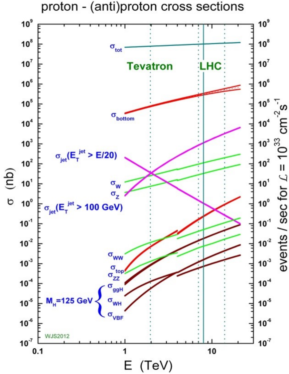
Figure 2.4: Production rates, corresponding to cross sections are shown for various center of mass energies. In the LHC regime, the total production \sigma_{tot} can be seen to be 100 mb, with the highest Higgs production mode \sigma_{ggH} \approx 20 pb, many orders of magnitude lower.
