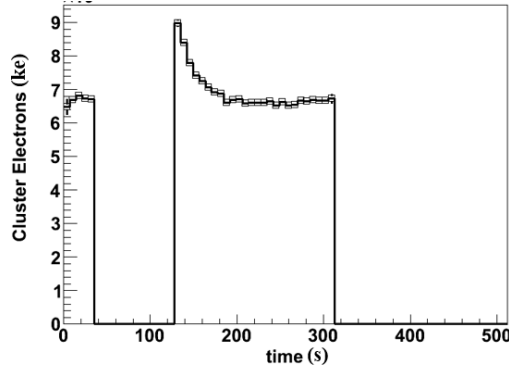
Figure 3.9: The charge collected per cluster integrated over time. The source is opened at the \sim 125 second mark, charge collection begins around 9k electrons per cluster but quickly drops to a plateau of 7k e.
