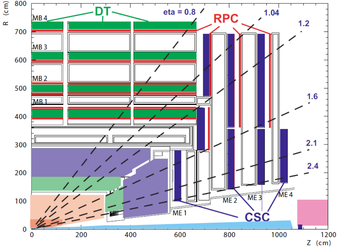
Figure 2.10: A single quarter of the CMS detector, the interaction point is located at the bottom left corner of the diagram. The components of the muon detection chambers are labeled, and the value of \eta for various angles ( \lambda ) with respect to the z axis is shown.
