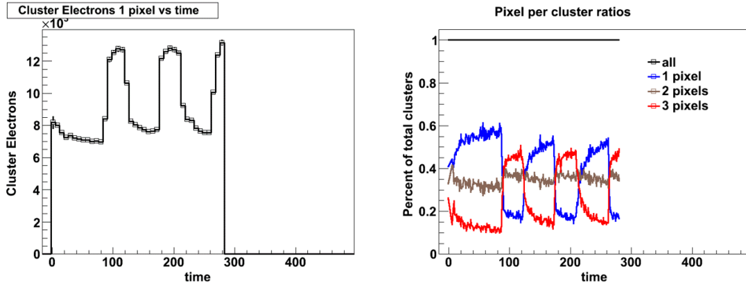
Figure 3.10: Tests done with a 650nm red laser on a diamond sensor. The left plot shows the charge collected from 1 pixel clusters, the peaks and valleys correspond exactly to the laser turning on and off respectively. In the right plot is shown the distribution of single pixel clusters (blue), 2 pixel clusters (brown) and \geq 3 pixel clusters (red) this plot shows a large change in single and large cluster population while the laser is turned on.
