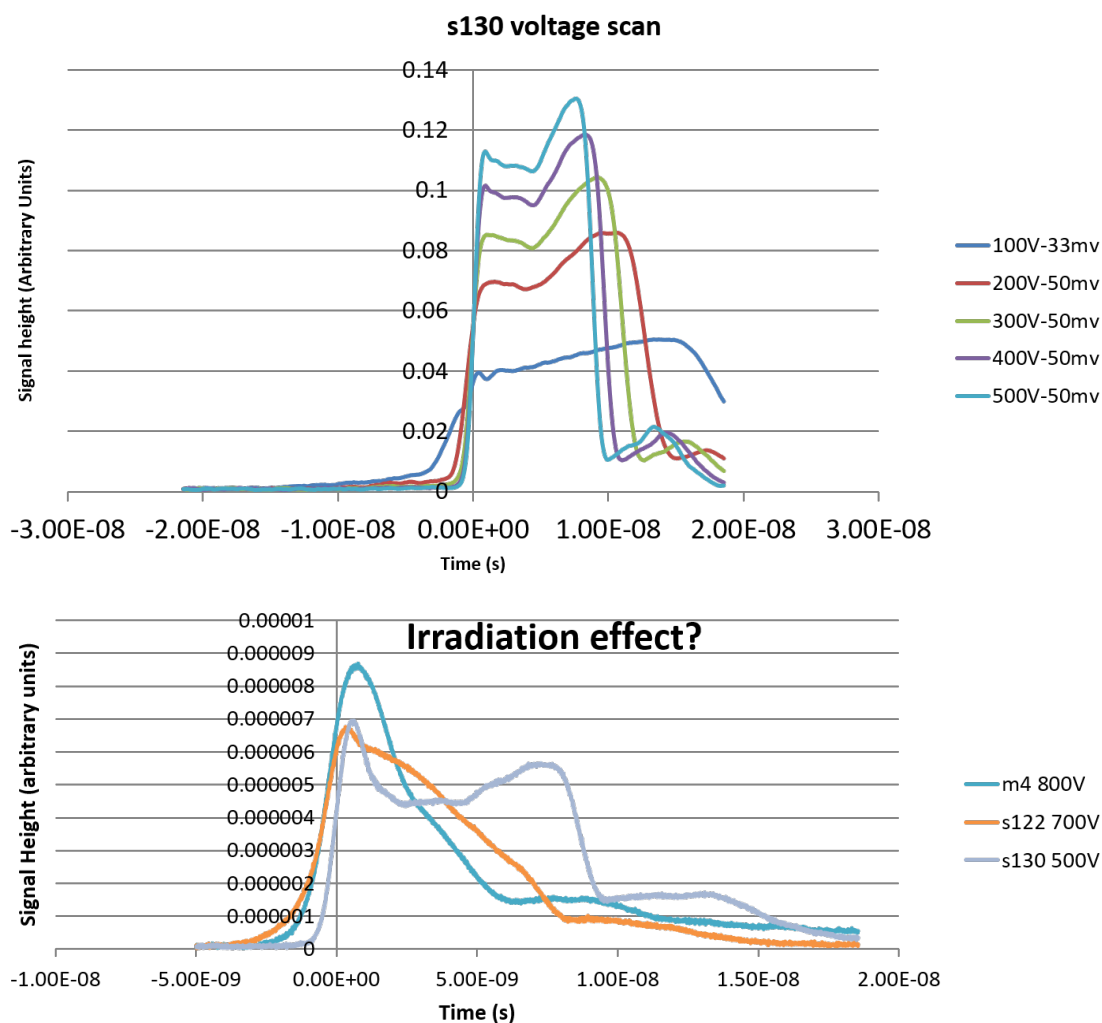
Figure 3.12: The top plot shows an unirradiated diamond's average charge collection pulse at different applied voltages. The bottom plot shows a comparison of an average pulse from 3 diamonds with differing levels of irradiation and applied bias. s130 is unirradiated, s122 has a total dose of 3 \times 10^{14} n/cm^2 and m4 has a total dose of 4 \times 10^{14} n/cm^2 .
