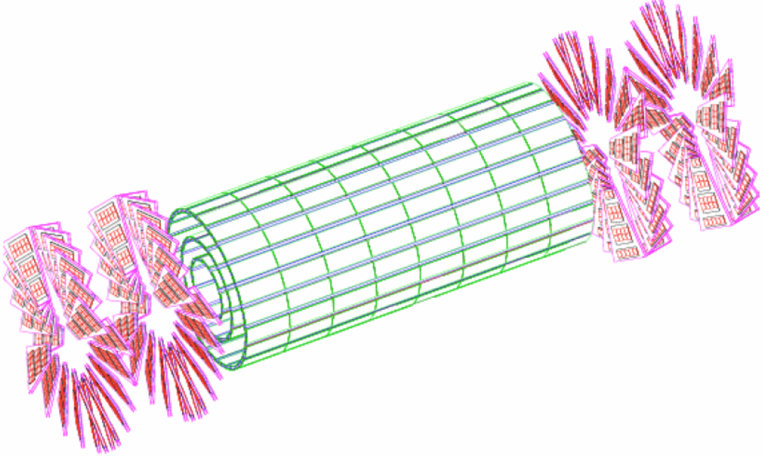
Figure 2.7: A diagram of the silicon pixel detector’s barrel layers (green) and endcap disks (red).
