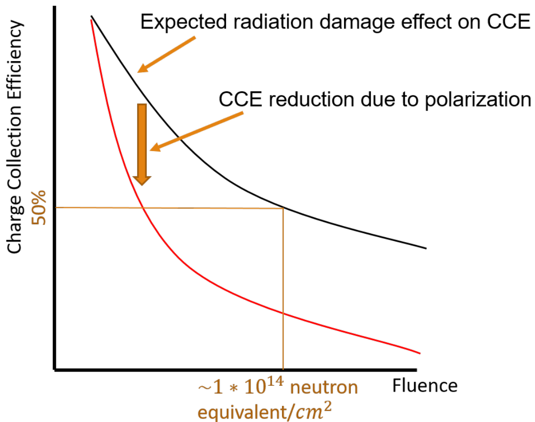
Figure 3.13: A representation of the effect of radiation damage in a scCVD diamond when paired with the observed polarization effect. The black curve represents the expected CCE vs. fluence from a diamond which exhibits no polarization, the red curve represents a fully polarized diamond. In reality the measured CCE will be somewhere between the two curves for a given fluence.
