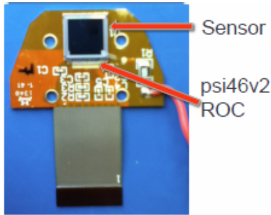
Figure 3.5: A single PLT sensor is shown, the black square is the silicon semiconducting material which creates an electrical signal when a charged particle passes through. The electrical signal is driven into the read out chip (ROC) by means of a bias field applied to the silicon. The information is read out of the ROC through the ribbon cable at the bottom.
