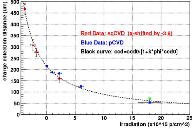
Figure 3.7: The measured charge collection for 2 diamond types after subsequent exposures to 24 GeV protons. The scCVD is shown in red, and the pCVD diamonds are shown in blue and green. The scCVD diamonds are offset in the x direction by the noted amount.
