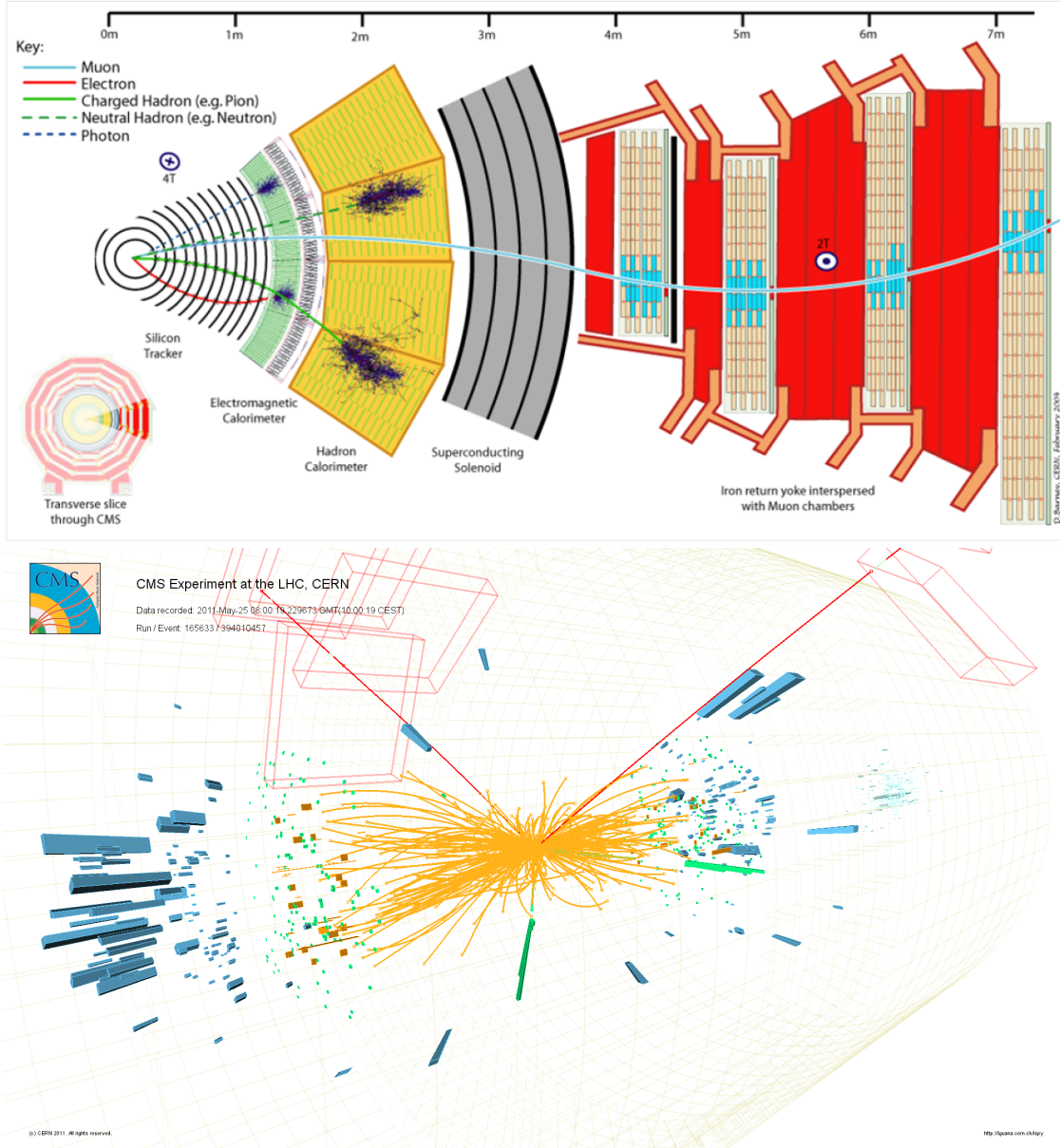
Figure 2.12: Top: A transverse slice of CMS with various types of particle tracks and their measurable signatures. Bottom: A CMS event display [99] which shows pixel and tracker tracks in dark yellow, ECAL deposits as green towers, HCAL deposits as blue towers, and Muon station hits in bright green (the muon station recording the hit is outlined in red). The tracks of 2 possible muon candidates are highlighted with red lines, and 2 large ECAL deposits can be found. This event is a candidate 4-lepton final state which can be produced by J/\psi pair, or Higgs \rightarrow ZZ for example.
