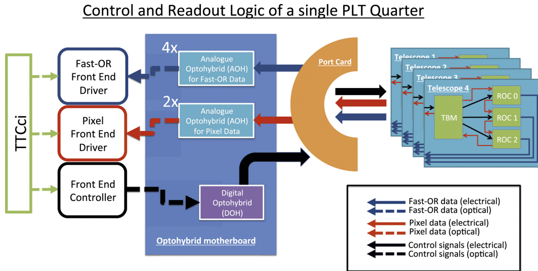
Figure 3.4: A schematic of the read out chain of the PLT. The optomotherboard, port card and telescopes are inside CMS. The optical connections send data to and from the computer center in a nearby cavern.
