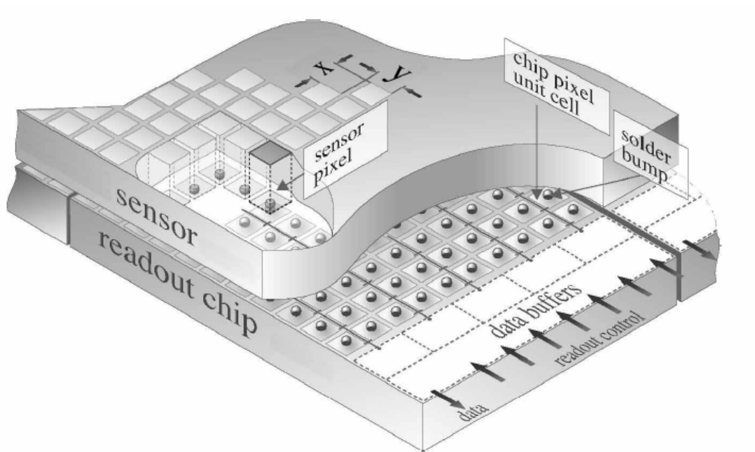
Figure 2.8: Shown is a cutaway diagram of the pixelated ROCs bump bonded to a silicon sensor.
