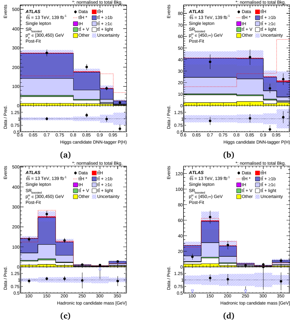
Fig. A.12: Post-fit distributions of (a),(b) the DNN P(H) output for the Higgs-boson candidate as well as (c),(d) the hadronic-top invariant mass in the single-lepton boosted SR_{\text{boosted}} for the 300 \leq p_T^H < 450 \text{ GeV} (left) and p_T^H \geq 450 \text{ GeV} (right) regions, respectively [100]. The t\bar{t}H signal yield (solid red) is normalised to the fitted \mu value from the inclusive fit. The dashed line shows the t\bar{t}H signal distribution normalised to the total background prediction. The uncertainty band includes all uncertainties as well as their correlations. The first (last) bin includes the underflow (overflow).
