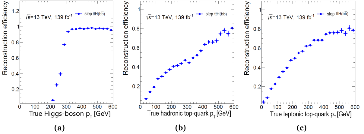
Fig. 6.7: Reconstruction efficiency as a function of the true \hat{p}_T of the candidate in the region characterised by |p_T^{reco}/\hat{p}_T^{true} - 1| < 0.5 and \Delta R(\text{true, reco}) < 0.4 for (a) Higgs-boson (b) hadronic top and (c) leptonic top-quark candidates, in the semi-leptonic t\bar{t}H(H \rightarrow b\bar{b}) sample.
