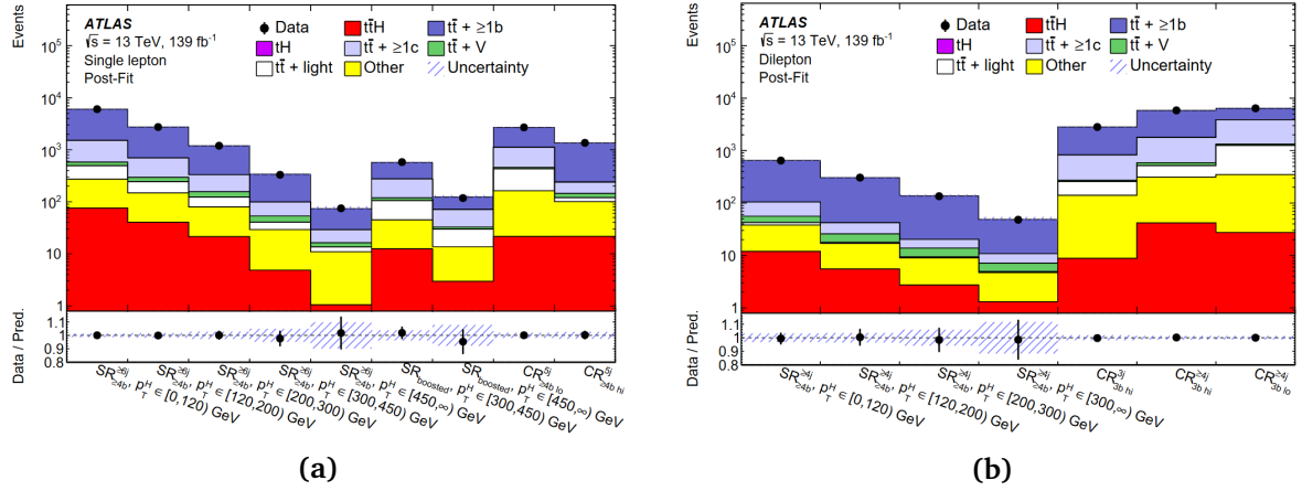
Fig. 8.23: Comparison of the predicted and observed event yields in each of the signal and control regions, in the (a) single-lepton and (b) dilepton channels, after performing the combined fit to data (post-fit) [100]. The uncertainty band includes the statistical and systematic uncertainties as well as their correlations.
