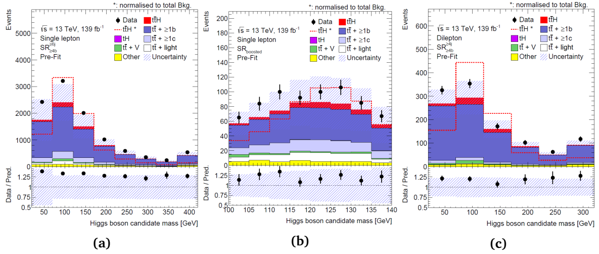
Fig. 8.6: Pre-fit distributions of the reconstructed Higgs boson candidate mass for the (a) single-lepton resolved SR_{\geq 4b}^{\geq 6j} , (b) single-lepton boosted SR_{boosted} , and (c) dilepton SR_{\geq 4b}^{\geq 4j} signal regions. The t\bar{t}H signal yield (solid red) is normalised to the Standard Model expectation. The dashed line shows the t\bar{t}H signal distribution normalised to the total background prediction. The uncertainty band includes the statistical and systematic uncertainties, except for the uncertainty in the k(t\bar{t} + \geq 1b) normalisation factor which is not defined pre-fit. The first (last) bin includes the underflow (overflow).
