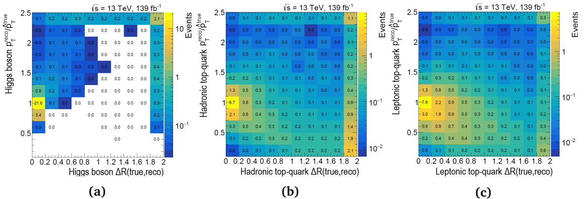
Fig. 6.6: Number of signal events in terms of p_T^{\text{reco}}/\hat{p}_T^{\text{true}} and \Delta R(\text{true}, \text{reco}) for (a) Higgs-boson (b) hadronic top-quark and (c) leptonic top candidates, in the semi-leptonic t\bar{t}H(H \rightarrow b\bar{b}) sample. In both cases, most of the events fall within the |p_T^{\text{reco}}/\hat{p}_T^{\text{true}} - 1| < 0.5 and \Delta R(\text{true}, \text{reco}) < 0.4 region.
