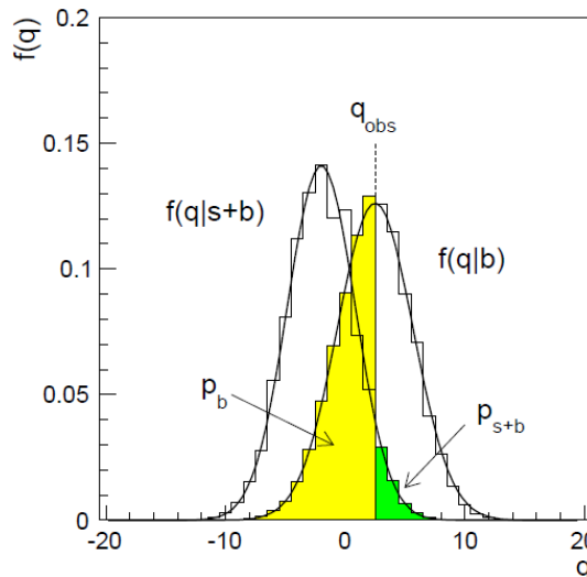
Fig. 8.2: Example of distributions of the test statistics for the background-only ( b ) and signal-plus-background ( s + b ) hypotheses [275].
