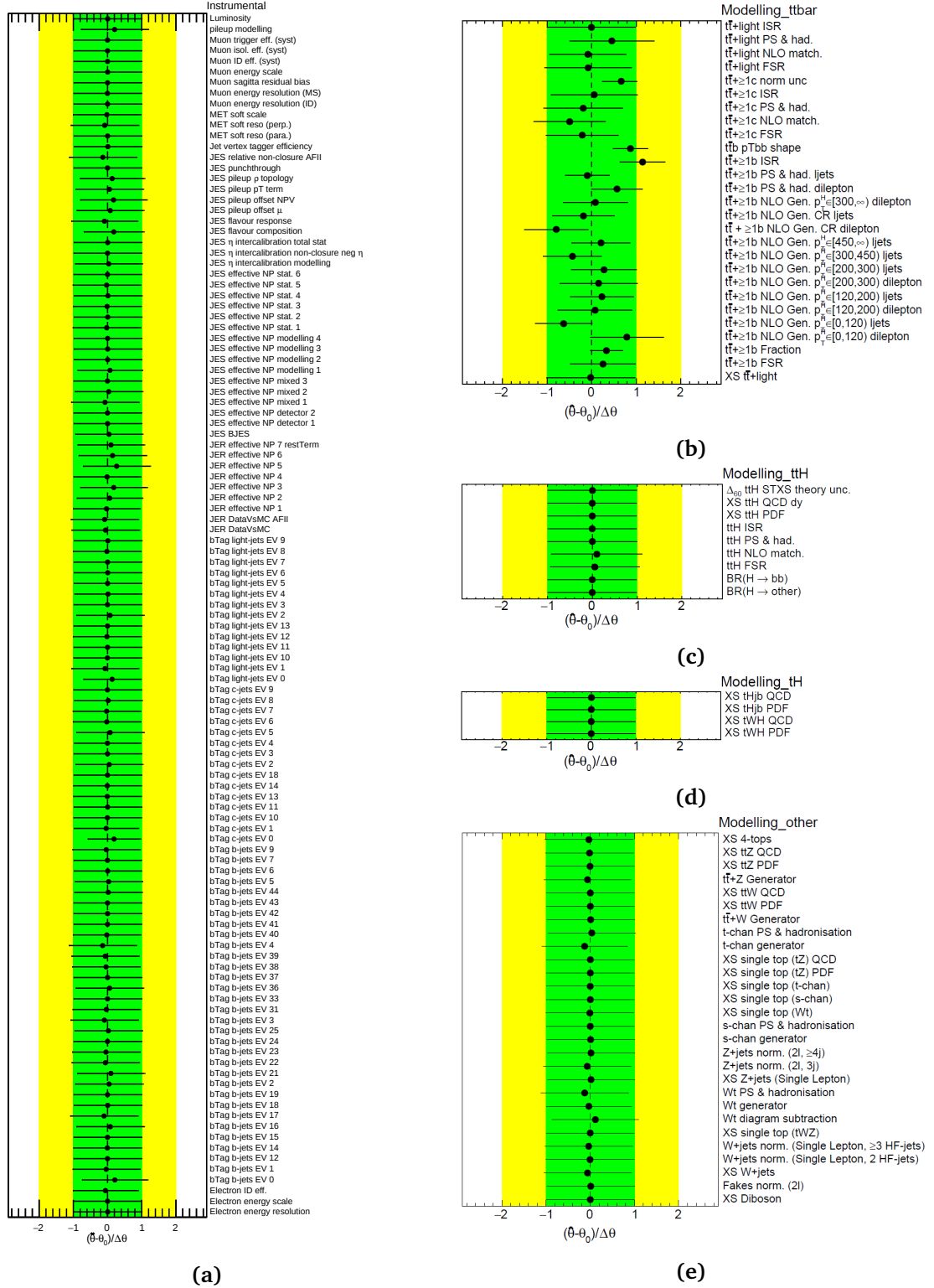
Fig. A.11: Fitted nuisance parameters of the (a) instrumental, (b) t\bar{t} + jets modelling, (c) t\bar{t}H modelling, (d) tH modelling, and (e) other backgrounds modelling systematic uncertainties from the combined STXS fit to data. The green (yellow) area represents the \pm 1(2)\sigma band on the pre-fit systematic uncertainty. The position of the black points shows the pull of the nuisance parameters, i.e. their best-fit value \hat{\theta} relative to their nominal values, \theta_0 . The size of the horizontal bars give the constraint of the nuisance parameters, i.e. their post-fit error relative to the pre-fit one, \Delta\hat{\theta}/\Delta\theta . Both values are given in units of standard deviation ( \sigma ).
