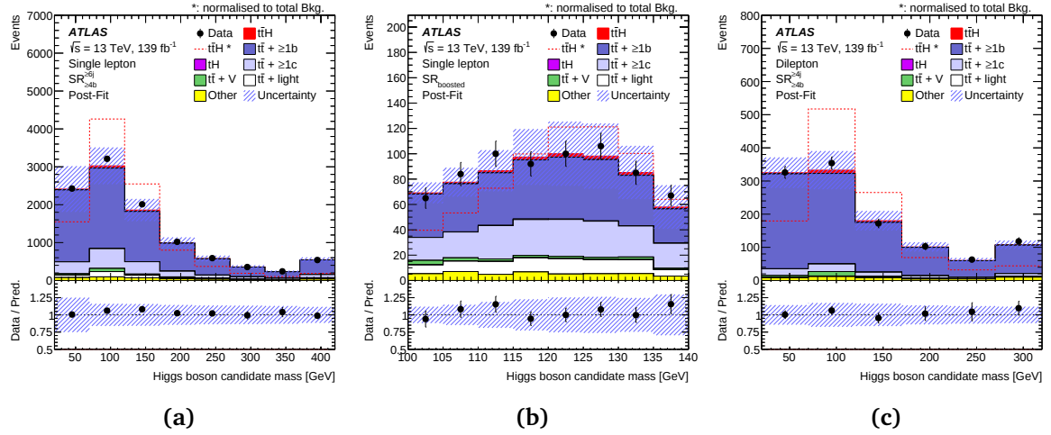
Fig. A.13: Post-fit distributions of the reconstructed Higgs boson candidate mass for the (a) single-lepton resolved SR_{>4b}^{>=6j} , (b) single-lepton boosted SR_{boosted} , and (c) dilepton SR_{>4b}^{>=4j} signal regions [100]. The t\bar{t}H signal yield (solid red) is normalised to the fitted \mu value from the inclusive fit. The dashed line shows the t\bar{t}H signal distribution normalised to the total background prediction. The uncertainty band includes all uncertainties as well as their correlations. The first (last) bin includes the underflow (overflow).
