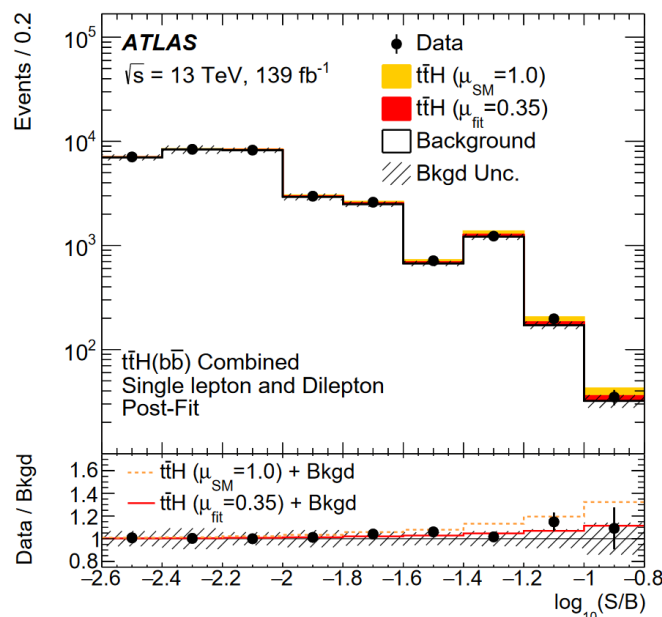
Fig. 8.27: Post-fit yields of signal ( S ) and total background ( B ) as a function of \log(S/B) compared with data [100], from the combined inclusive- \mu fit. Final-discriminant bins in all single-lepton and dilepton analysis regions are combined into bins of \log(S/B) , with the signal normalised to the SM prediction used for the computation of \log(S/B) . The signal is then shown normalised to the best-fit value and the SM prediction. The lower frame reports the ratio of data to background, and this is compared with the expected t\bar{t}H -signal-plus-background yield divided by the background-only yield for the best-fit signal strength (solid red line) and the SM prediction (dashed orange line).
