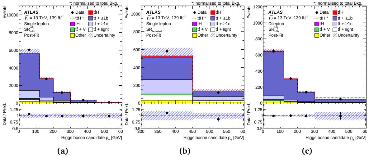
Fig. 8.21: Post-fit distributions of the reconstructed Higgs boson candidate for the (a) single-lepton resolved SR_{4b}^{>6j} , (b) single-lepton boosted SR_{boosted} , and (c) dilepton SR_{4b}^{>4j} signal regions [100]. The t\bar{t}H signal yield (solid red) is normalised to the fitted \mu value from the inclusive fit. The dashed line shows the t\bar{t}H signal distribution normalised to the total background prediction. The uncertainty band includes all uncertainties as well as their correlations. The last bin includes the overflow.
