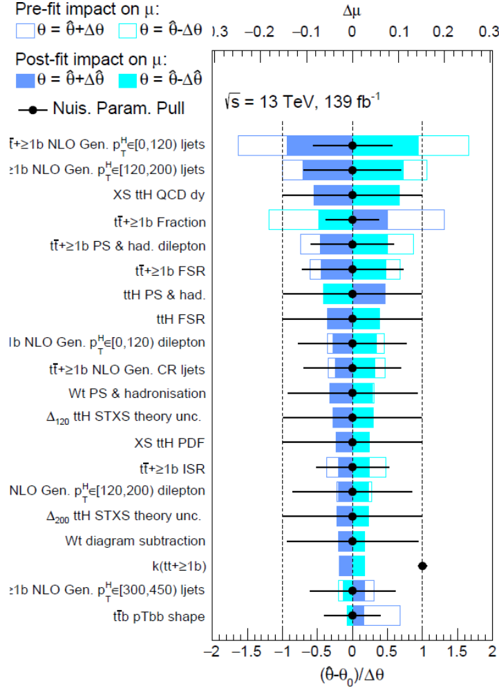
Fig. 8.11: Ranking of the 20 nuisance parameters with the largest post-fit impact on \mu in the combined inclusive cross-section fit to the Asimov dataset. Nuisance parameters corresponding to statistical uncertainties in the MC simulated event samples are not included. The empty blue rectangles correspond to the pre-fit impact on \mu , while the filled blue ones to the post-fit impact on \mu , both referring to the upper scale. The impact of each nuisance parameter, \Delta\mu , is computed by comparing the nominal best-fit value of \mu with the result of the fit when fixing the considered nuisance parameter to its best-fit value, \hat{\theta} , shifted by its pre-fit (post-fit) uncertainties \pm\Delta\hat{\theta} ( \pm\Delta\theta ). The black points show the pulls of the nuisance parameters relative to their nominal values, \theta_0 = 0 . These pulls and their relative post-fit errors, \Delta\hat{\theta}/\Delta\theta , refer to the lower scale. The parameter k(t\bar{t} + \geq 1b) refers to the free-floating normalisation of the t\bar{t} + \geq 1b background, for which the pre-fit impact on \mu is not defined, while its nominal value is \theta_0 = 1 . The "ljets" ("dilep") label refers to the single-lepton (dilepton) channel.
