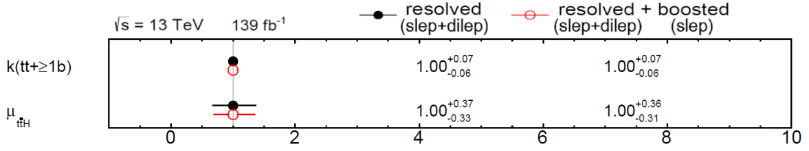
Fig. 8.10: Fitted normalisation factor for the t\bar{t} + \geq 1b background and signal strength from the S+B fit to the Asimov dataset in the inclusive cross-section measurement, combining only the resolved (single-lepton and dilepton) regions (in black) compared to the full combination (including also the single-lepton boosted region) (in red).
