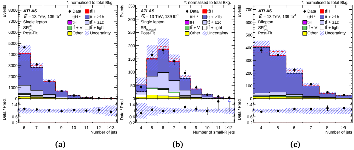
Fig. 8.20: Post-fit distributions of the number of jets for the (a) single-lepton resolved SR_{>4b}^{>6j} , (b) single-lepton boosted SR_{boosted} , and (c) dilepton SR_{>4b}^{>4j} signal regions [100]. The t\bar{t}H signal yield (solid red) is normalised to the fitted \mu value from the inclusive fit. The dashed line shows the t\bar{t}H signal distribution normalised to the total background prediction. The uncertainty band includes all uncertainties as well as their correlations. The last bin includes the overflow.
