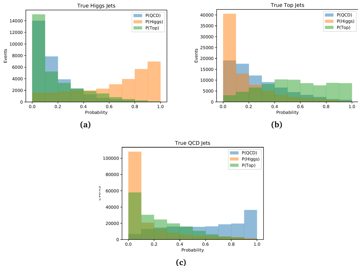
Fig. 6.13: DNN output distributions: the probabilities P(H) , P(t) and P(QCD) , for the true-reco matched (a) Higgs-boson jets, (b) top-quark jets, and (c) QCD jets. In each case, a high discrimination power is shown [253].
