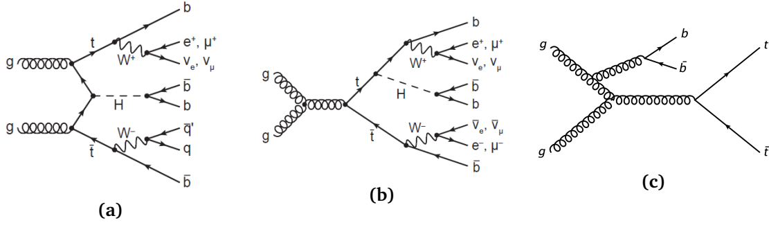
Fig. 2.15: Exemplary tree-level Feynman diagrams for the production of a Higgs boson in association with a top-quark pair (here produced via gluon fusion), t\bar{t}H , including the subsequent decays of the top quark-antiquark pair in a) the single-lepton channel (t-channel) and b) the dilepton channel (s-channel), as well as the subsequent decay of the Higgs boson into a bottom quark-antiquark pair ( H \rightarrow b\bar{b} ), and for (c) the main t\bar{t} + b\bar{b} background process.
