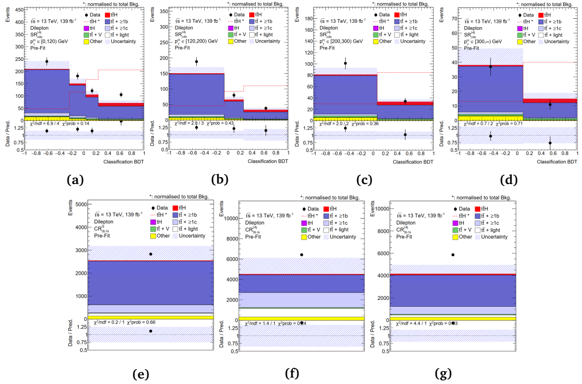
Fig. 8.5: Comparison between data and MC prediction for the BDT discriminant and the event yield in the SRs and CRs of the dilepton channel, respectively, before performing the fit to data (pre-fit). The signal region, SR_{\geq 4b}^{4j} , split into (a) 0 \leq p_T^H < 120 GeV, (b) 120 \leq p_T^H < 200 GeV, (c) 200 \leq p_T^H < 300 GeV, (d) p_T^H \geq 300 GeV regions, as well as the control regions (e) CR_{\geq 3b hi}^{3j} , (f) CR_{\geq 3b lo}^{4j} , and (g) CR_{\geq 3b hi}^{4j} are shown. The t\bar{t}H signal yield (solid red) is normalised to the Standard Model expectation. The dashed line shows the t\bar{t}H signal distribution normalised to the total background prediction. The uncertainty band includes the statistical and systematic uncertainties. The uncertainty on the t\bar{t} + \geq 1b background normalisation is not included as it is a free-floating parameter of the fit.
