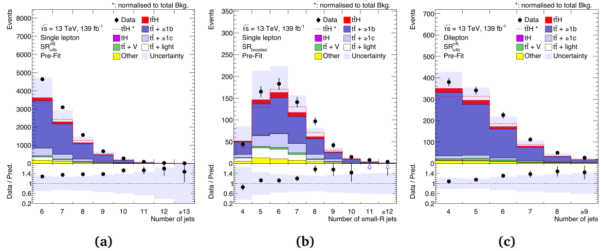
Fig. 8.7: Pre-fit distributions of the number of jets for the (a) single-lepton resolved SR_{\geq 4b}^{\geq 6j} , (b) single-lepton boosted SR_{boosted} , and (c) dilepton SR_{\geq 4b}^{\geq 4j} signal regions [100]. The t\bar{t}H signal yield (solid red) is normalised to the Standard Model expectation. The dashed line shows the t\bar{t}H signal distribution normalised to the total background prediction. The uncertainty band includes the statistical and systematic uncertainties, except for the uncertainty in the k(t\bar{t} + \geq 1b) normalisation factor which is not defined pre-fit. The last bin includes the overflow.
