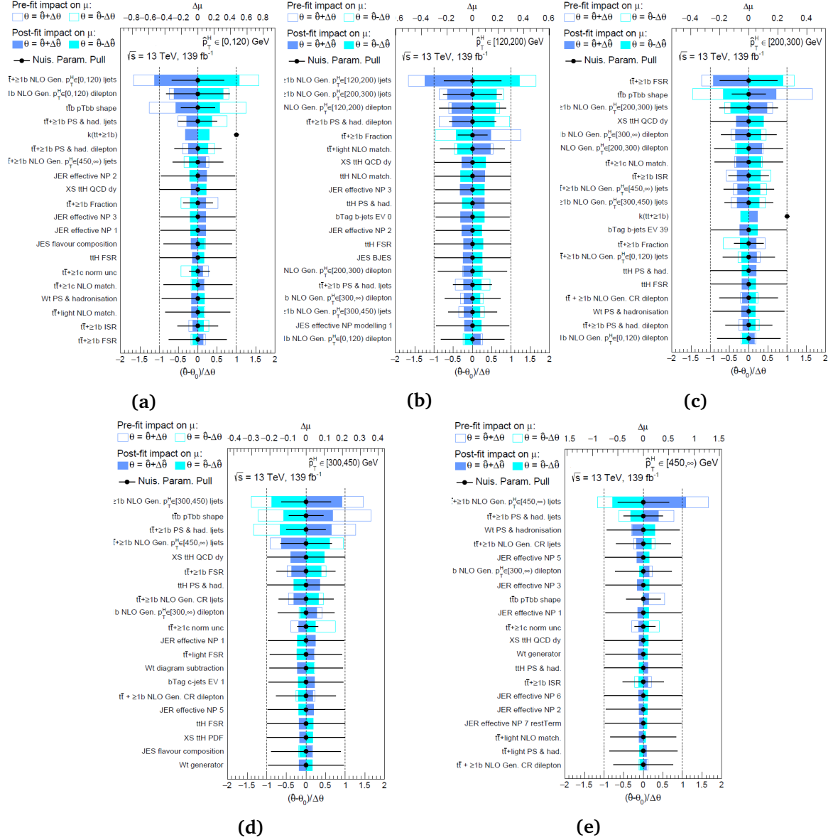
Fig. 8.15: Ranking of the 20 nuisance parameters with the largest post-fit impact on \mu in the combined STXS fit to the Asimov dataset, for (a) 0 \leq \hat{p}_T^H < 120 GeV, (b) 120 \leq \hat{p}_T^H < 200 GeV, (c) 200 \leq \hat{p}_T^H < 300 GeV, (d) 300 \leq \hat{p}_T^H < 450 GeV, and (e) \hat{p}_T^H \geq 450 GeV. Nuisance parameters corresponding to statistical uncertainties in the MC simulated event samples are not included. The empty blue rectangles correspond to the pre-fit impact on \mu , while the filled blue ones to the post-fit impact on \mu , both referring to the upper scale. The impact of each nuisance parameter, \Delta\mu , is computed by comparing the nominal best-fit value of \mu with the result of the fit when fixing the considered nuisance parameter to its best-fit value, \hat{\theta} , shifted by its pre-fit (post-fit) uncertainties \pm\Delta\hat{\theta} ( \pm\Delta\theta ). The black points show the pulls of the nuisance parameters relative to their nominal values, \theta_0 = 0 . These pulls and their relative post-fit errors, \Delta\hat{\theta}/\Delta\theta , refer to the lower scale. The parameter k(t\bar{t} + \geq 1b) refers to the free-floating normalisation of the t\bar{t} + \geq 1b background, for which the pre-fit impact on \mu is not defined, while its nominal value is \theta_0 = 1 . For the experimental uncertainties, that are decomposed into several independent sources, NP X corresponds to the X^{th} nuisance parameter, ordered by their impact on \mu . The "ljets" ("dilep") label refers to the single-lepton (dilepton) channel.
