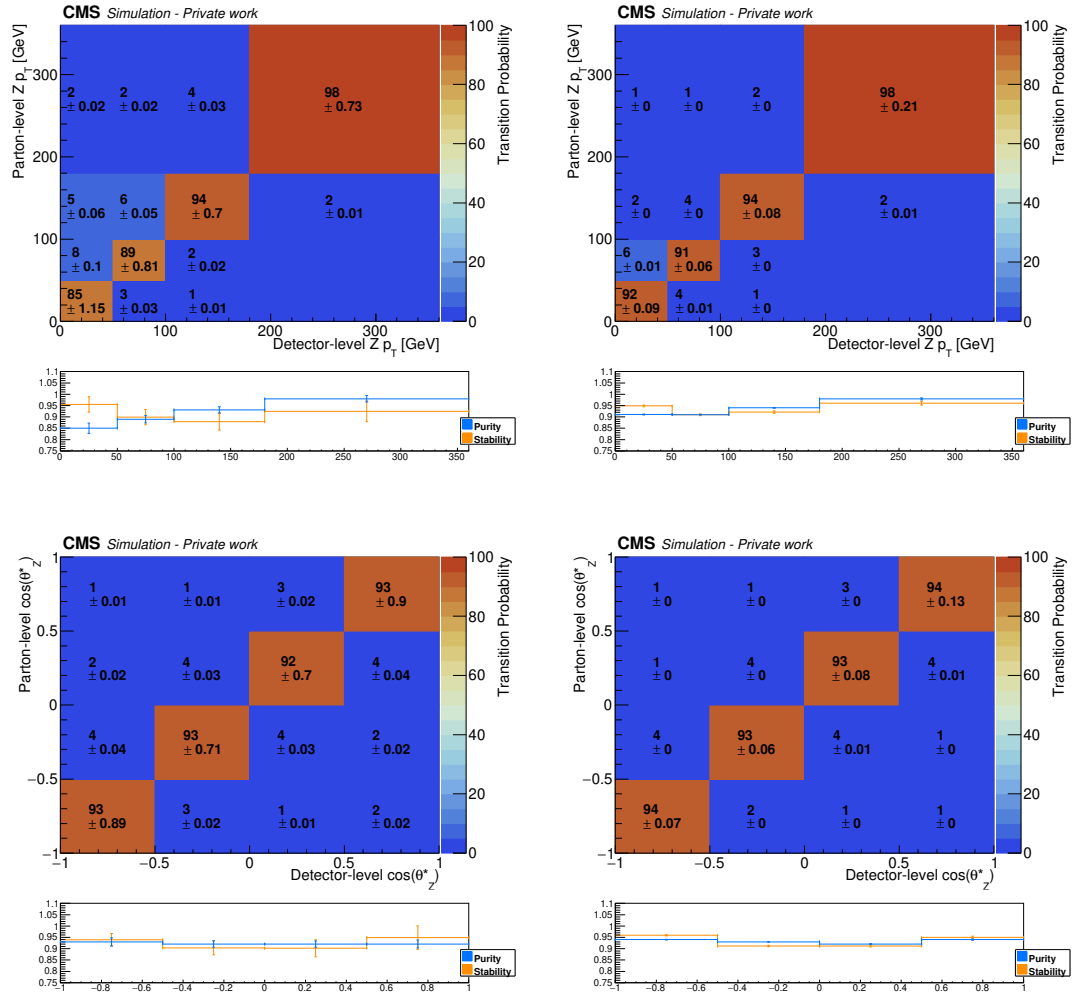
Figure 5.6: Response matrices for the sum of the t\bar{t}Z and tWZ (left) and tZq (right) samples. Plots refer to p_T(Z) (top) and \cos(\theta_Z^*) (bottom).
