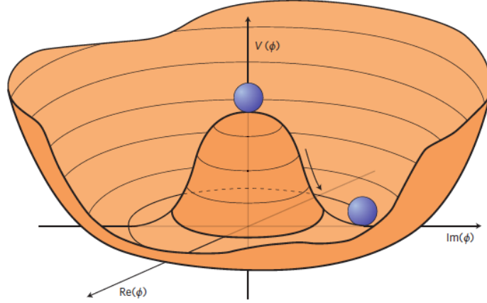
Figure 1.3: Shape of the potential V(\phi) in the case of a complex scalar field. The minima are an infinite set of states corresponding to a circle in the complex \phi plane and the choice of one of these points spontaneously breaks the symmetry of the model. Plot taken from [14].
