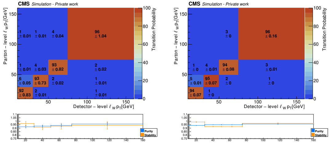
Figure A.1: Response matrices for the sum of the t\bar{t}Z and tWZ (left) and tZq (right) samples. Plots refer to p_T(\ell_W) .
