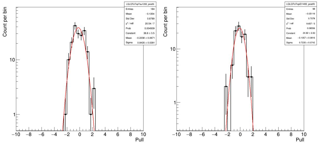
Figure 7.46: Histogram of pulls for the LQ\text{-}H BDT regions from the B_\tau = 1 (left) and B_e + B_\mu = 1 (right) trainings, for the combined 2016–2018 data set in the background-only hypothesis. These plots include all the bins from both 3-object and 4-object channels.
