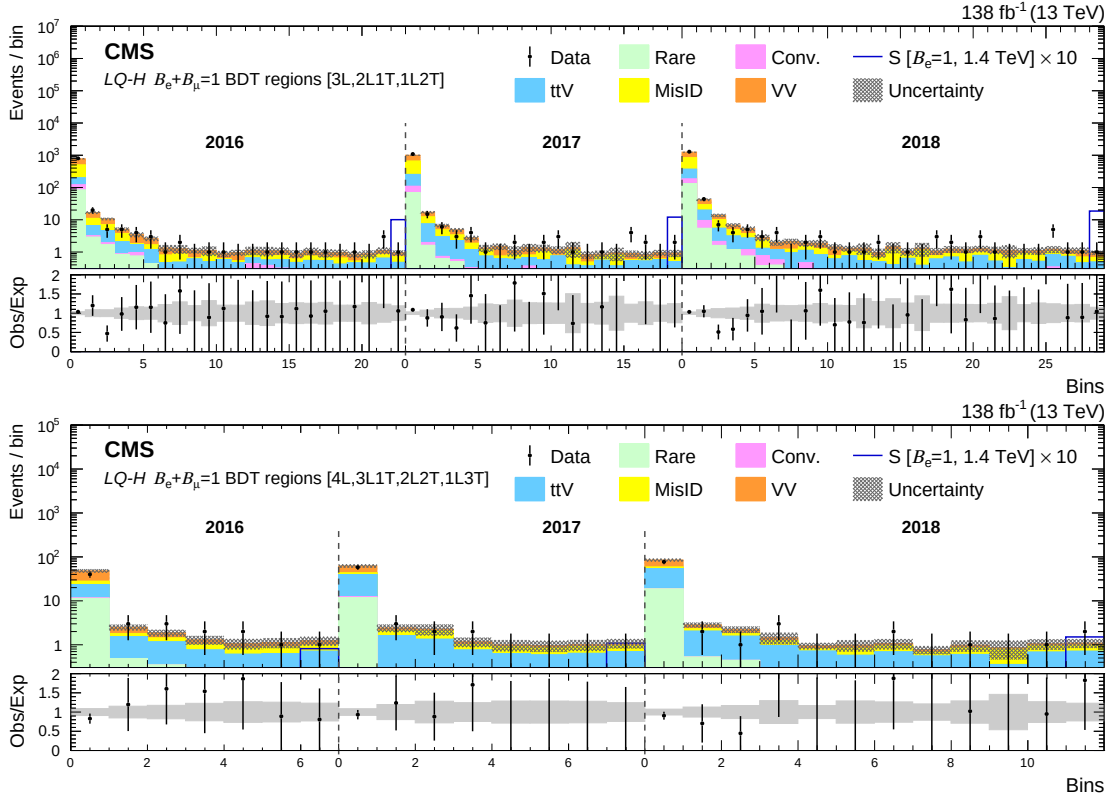
Figure 7.45: LQ-H BDT regions for the B_e + B_\mu = 1 training, in the 3-object channels (upper) and 4-object channels (lower) for the combined 2016–2018 data set. The lower panel shows the ratio of observed events to the total expected background prediction. The gray band on the ratio represents the sum of statistical and systematic uncertainties in the SM background prediction. The expected SM background distributions and the uncertainties are shown after fitting the data under the background-only hypothesis. For illustration, an example signal hypothesis for the production of the scalar leptoquark coupled to a top quark and an electron or a muon, before the fit, is also overlaid.
