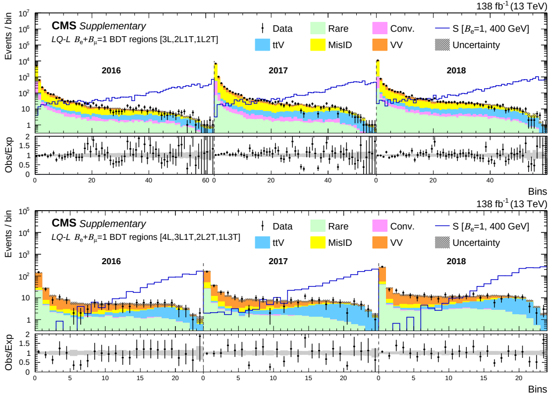
Figure 7.43: LQ-L BDT regions for the B_e + B_\mu = 1 training, in the 3-object channels (upper) and 4-object channels (lower) for the combined 2016–2018 data set. The lower panel shows the ratio of observed events to the total expected background prediction. The gray band on the ratio represents the sum of statistical and systematic uncertainties in the SM background prediction. The expected SM background distributions and the uncertainties are shown after fitting the data under the background-only hypothesis. For illustration, an example signal hypothesis for the production of the scalar leptoquark coupled to a top quark and an electron or a muon, before the fit, is also overlaid.
