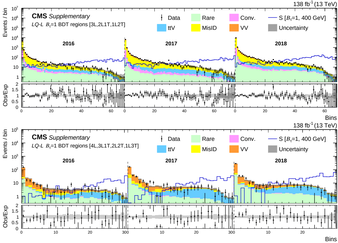
Figure 7.39: LQ-L BDT regions for the B_\tau = 1 training, in the 3-object channels (upper) and 4-object channels (lower) for the combined 2016–2018 data set. The lower panel shows the ratio of observed events to the total expected background prediction. The gray band on the ratio represents the sum of statistical and systematic uncertainties in the SM background prediction. The expected SM background distributions and the uncertainties are shown after fitting the data under the background-only hypothesis. For illustration, an example signal hypothesis for the production of the scalar leptoquark coupled to a top quark and a \tau lepton, before the fit, is also overlaid.
