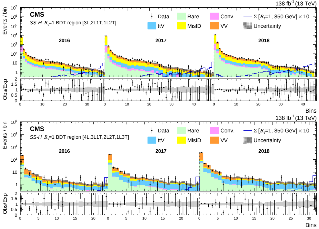
Figure 7.33: SS-H BDT regions for the B_\tau = 1 training, in the 3-object channels (upper) and 4-object channels (lower) for the combined 2016–2018 data set. The lower panel shows the ratio of observed events to the total expected background prediction. The gray band on the ratio represents the sum of statistical and systematic uncertainties in the SM background prediction. The expected SM background distributions and the uncertainties are shown after fitting the data under the background-only hypothesis. For illustration, an example signal hypothesis for the production of the type-III seesaw heavy fermions in the scenario with mixing exclusively to \tau lepton, before the fit, is also overlaid.
