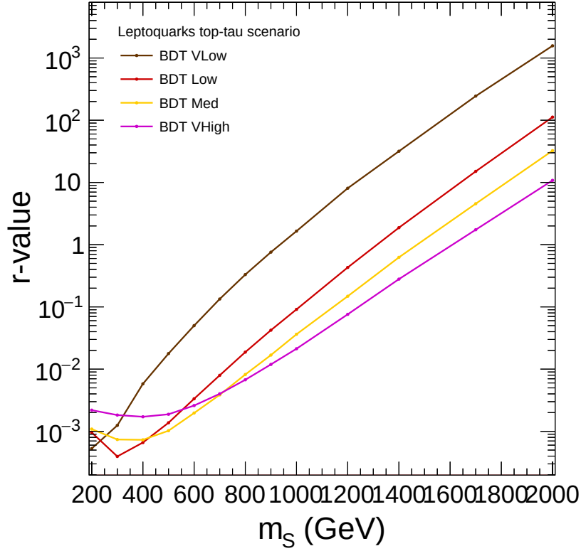
Figure 7.37: The expected limits including the complete set of uncertainties for the leptiquark model in the \mathcal{B}_\tau = 1 scenario using a single BDT used for the whole mass range (left). This test informs the choice of BDT for a particular mass point.
