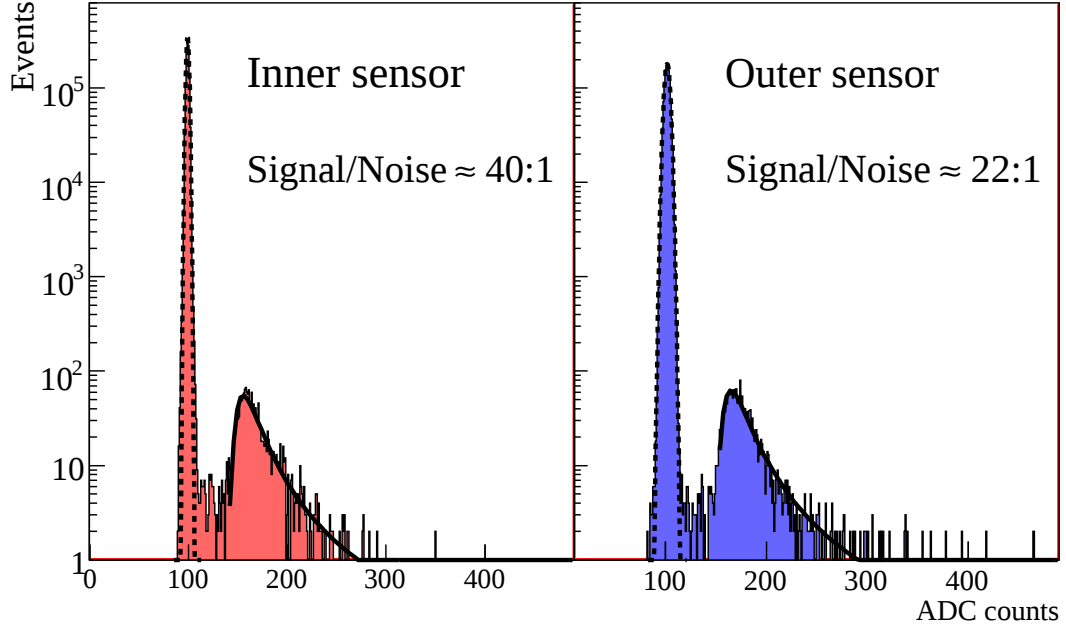
Figure 7.6: Measured signal-to-noise ratio of inner (left) and outer (right) silicon sensors using 630 MeV e^- from ASTRID
