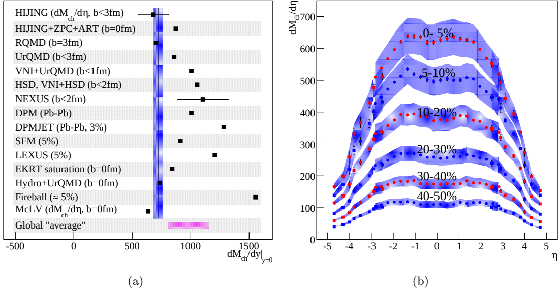
Figure 2.2: (a) Comparison of various model predictions of the charged particle density in Au–Au at \sqrt{s_{NN}} = 200\text{ GeV} compared to the PHOBOS observation, indicated by the vertical line. The vertical band represents the systematic errors on the PHOBOS data, while the horizontal band is the average of all the predictions. Adapted from [49]. (b) Charged particle density in Au–Au at \sqrt{s_{NN}} = 200\text{ GeV} at different centralities, as measured by BRAHMS. Adapted from [50].
