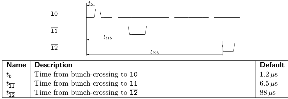
Figure 5.27: Timing of triggers
