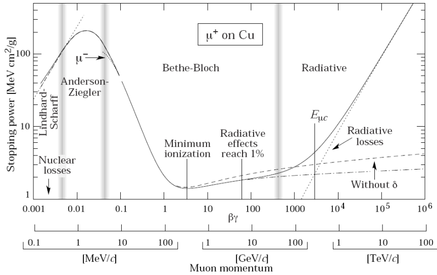
Figure 5.9: Bethe–Bloch equation evaluated for \mu on copper
