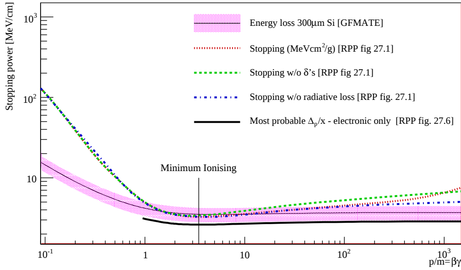
Figure 5.11: Mean and most probable energy loss in 300\ \mu\text{m} Si. GFMATE is the routine used in the GEANT simulation program and RPP refers to the Review of Particle Physics [81].
