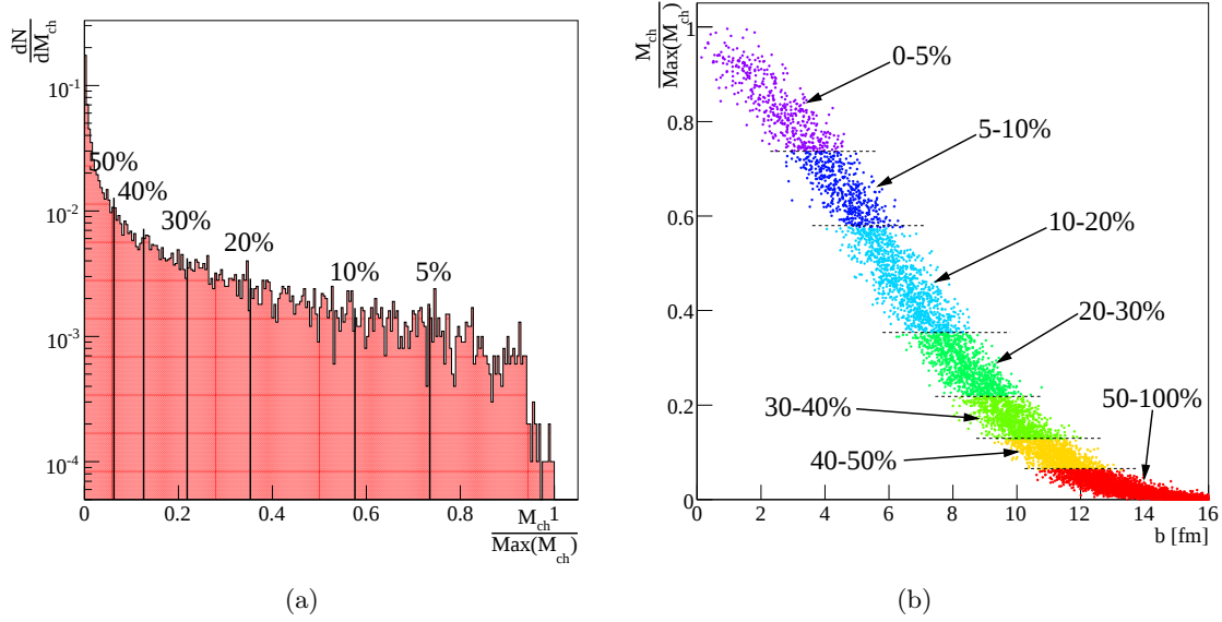
Figure 2.1: (a) Definition of centrality cuts from observed total charged particle multiplicity. The data in the figure is from a 10,000 HIJING Pb–Pb at \sqrt{s_{NN}} = 5500 GeV. The x axis has been scaled to the maximum observable total charged particle multiplicity. (b) Comparison of centrality classes to impact parameter. Clearly, the mapping from impact parameter b to centrality class is not one-to-one, and the mapping is therefore not invertible.
