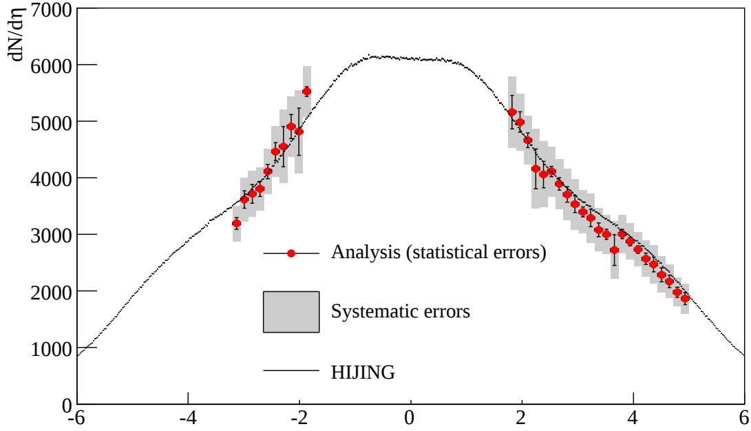
Figure 8.12: The primary charged particle density as reconstructed by the FMD, and compared to the input of 1000 events of HIJING model data with b \in [0, 5]\text{fm} . The error bars indicate the statistical error, while the grey boxes indicate the systematic error estimated by comparing to the Poisson method [102].
