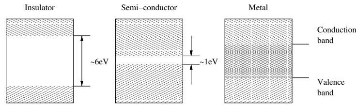
Figure 5.4: Valence and Conduction band gap in insulators, semi-conductors, and metals. Adapted from [77].
