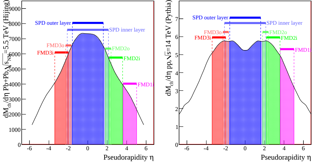
Figure 4.2: Total charged particle multiplicity coverage of ALICE, broken up by detector system. The data is from a HIJING simulation of central Pb–Pb at \sqrt{s_{NN}} = 5500 \text{ GeV} and PYTHIA simulation of pp at \sqrt{s} = 14000 \text{ GeV} .
