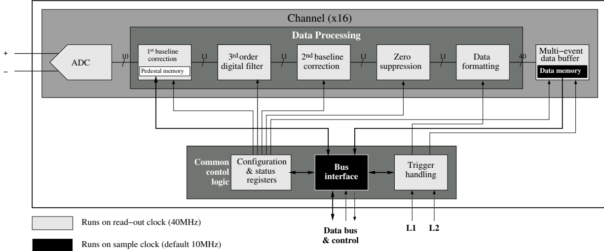
Figure 5.21: Schematic architecture of the ALTRO chip. The processing chain for all 16 channels is the same — First, the analogue signal is converted to 10 bits. Then a series of digital processing units are invoked in turn, if so enabled in the configuration registers. Finally, the processed data is formatted into 40bit words and stored in the multi-event buffer. All this is done at the speed of the sample clock (default is 10 MHz). On request, the data is strobed out over the bus. The bus interface and the data memory is working at the speed of the read-out bus (40 MHz).
