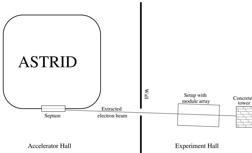
Figure 7.1: Extraction of parasitic beam from ASTRID.
