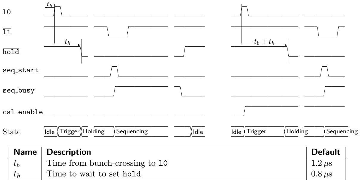
Figure 5.28: State changes in the trigger handling module. The left side illustrates normal trigger conditions, where the trigger is received 1.2 \mu\text{s} after the collision. The right hand side illustrates the case of pulser calibrations, where an additional delay of t_b is introduced before asserting \overline{\text{hold}} .
