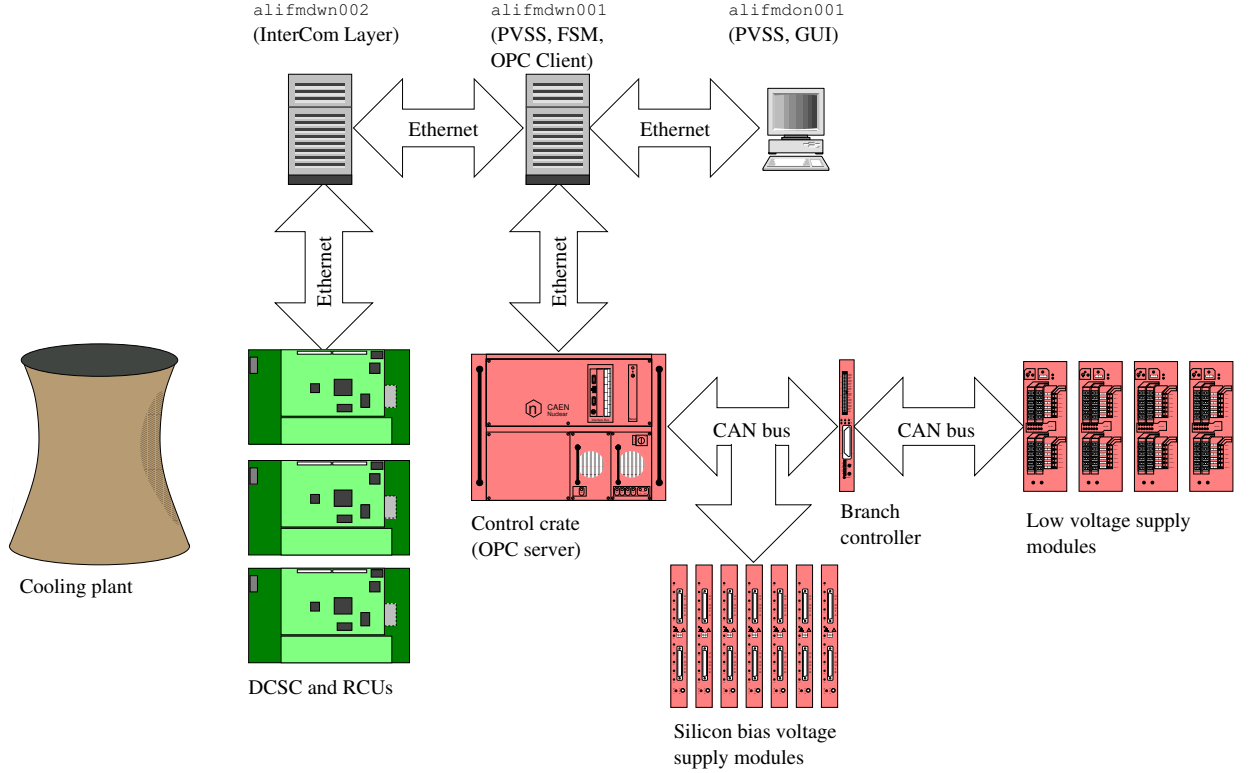
Figure 6.3: The FMD DCS architecture.
