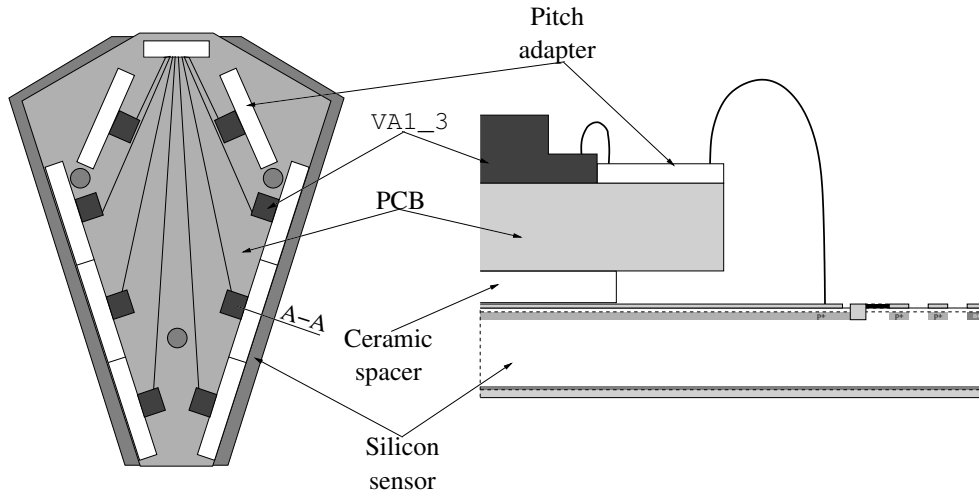
Figure 5.12: Schematic drawing of an inner-type hybrid. The right-hand side shows a schematic section through the stack at A-A. Note, that the detail is not to scale.
