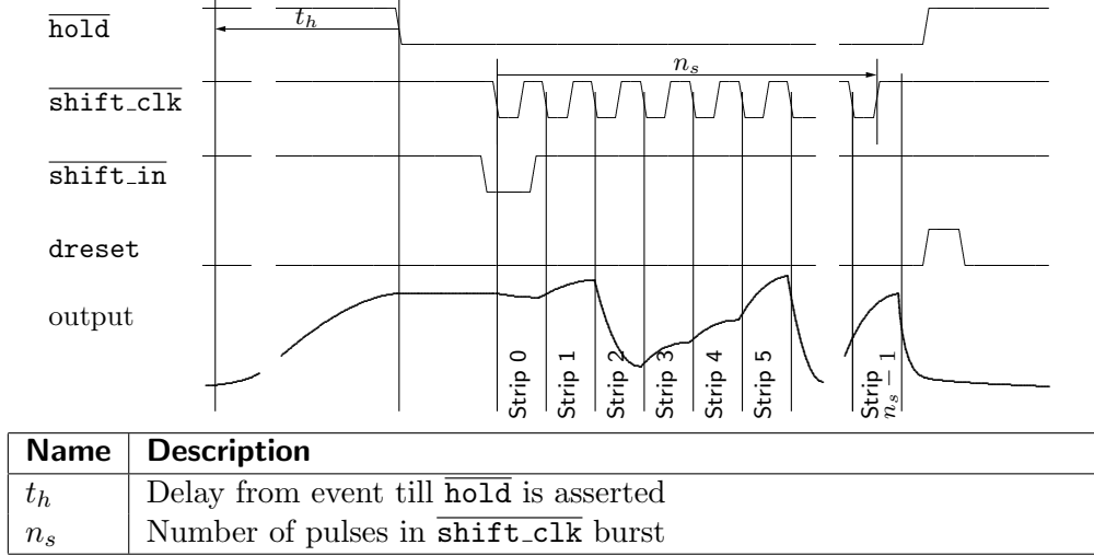
Figure 5.15: Read-out of all 128 channel in a VA1 3 chip. shift_in together with shift_clk resets the shift register to point at the first channel, while each subsequent falling edge of shift_clk makes the shift register point at the next channel. At the end of the read-out, a single pulse on dreset can be sent to clear the digital parts of the chip, though it is generally not needed.
