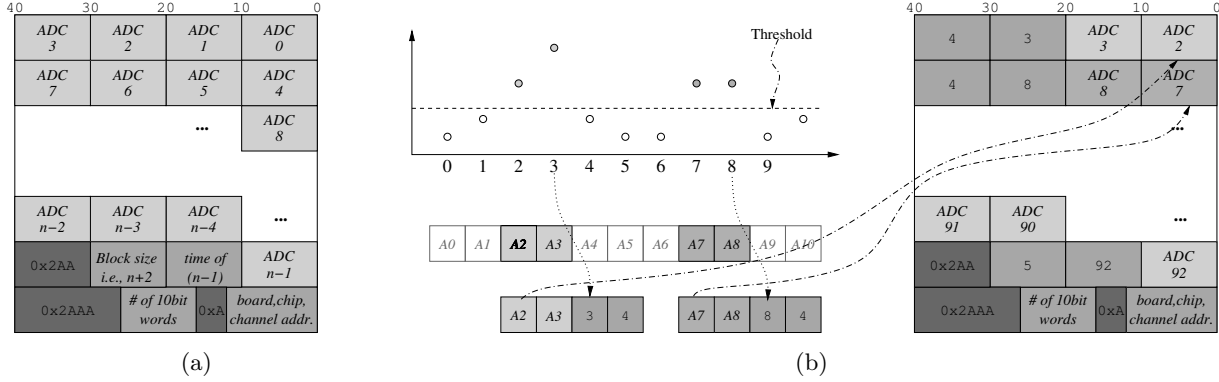
Figure 5.23: ALTRO channel data format. The trailer consist of the channel address, given as 12bits of ( board,chip,channel ). (a) In case of no zero suppression. All n ADC counts are put into one block (here starting at ADC\ 0 and ending at ADC\ n-1 ) followed by the time of the last 10bit word, and the total length of the block ( n + 2 ). (b) In case of zero suppression, only the values over threshold are stored. If there appears holes due to ignored counts (such as counts A3 , A4 , and A5 ), then a block trailer is appended, consisting of the time of the last ADC count, and the total size of the block. The blocks are then concatenated, and filler words are appended to pad to the 40bit word size.
