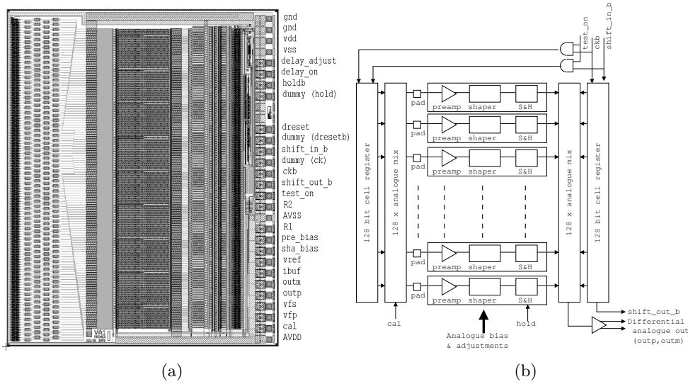
Figure 5.13: Architecture of the VA1 3 chip.
