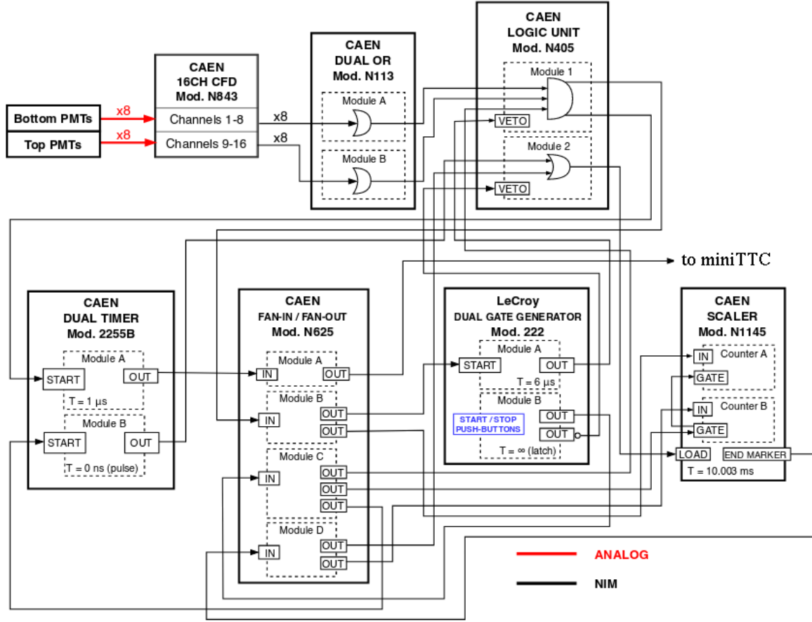
Figure 4.3: The NIM logic crate uses a series of discriminators, logical OR and logical AND modules to generate 1 \mu s wide NIM trigger. A gate generator produces a 6 \mu s veto in between consecutive trigger pulses [55].
