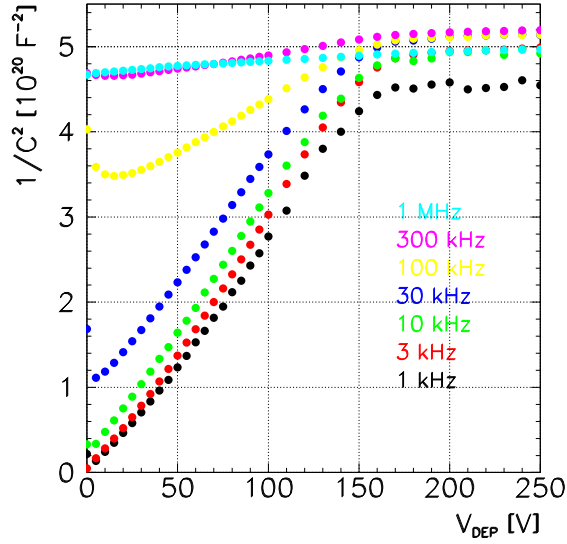
Figure 2.4: C/V measurement of a diode, irradiated to 5 \cdot 10^{13} \text{ n/cm}^2 and annealed for five months at 20^\circ\text{C} . The difference in signals obtained by different measurement frequencies is shown. The measurement was performed at 5^\circ\text{C} .
