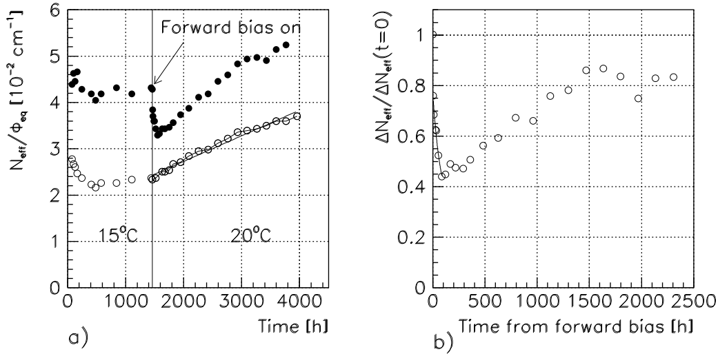
Figure 6.10: a) Time development of N_{eff} for the biased and unbiased diode from the pair D2. They were kept at 15°C until the end of beneficial annealing. Then they were moved to 20°C and 350V of reverse bias of the diode D2A was replaced by approximately 10V of forward bias. b) Time development of the difference. Difference in N_{eff} normalised to the initial value is shown versus time from switching off the bias.
