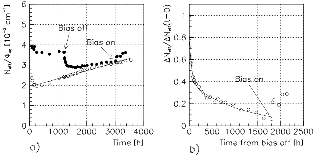
Figure 6.9: a) Time development of N_{eff} for the biased and unbiased diode from the pair UO6. They were kept at 20°C before and after the bias of the diode UO6B was switched off. b) Time development of the difference. Difference in N_{eff} normalised to the initial value is shown versus time from switching off the bias. Agreement of a two exponentials fit (eq. 6.2) with the measured data is also shown.
