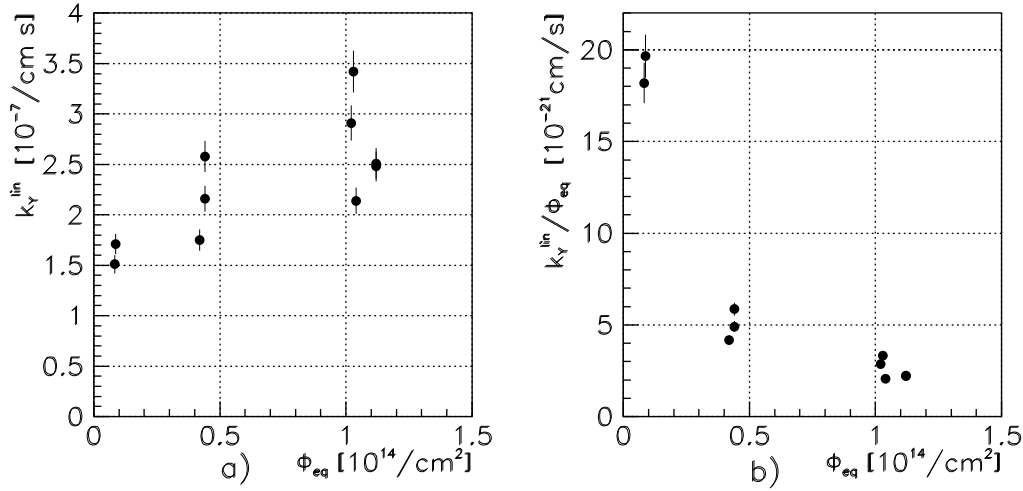
Figure 4.6: a) k_Y^{lin} and b) k_Y^{lin}/\Phi_{eq} for the group annealed at 60°C. In case of a first order dynamics, the distribution in figure a) should be flat, while for second order, the distribution b) should be flat.
