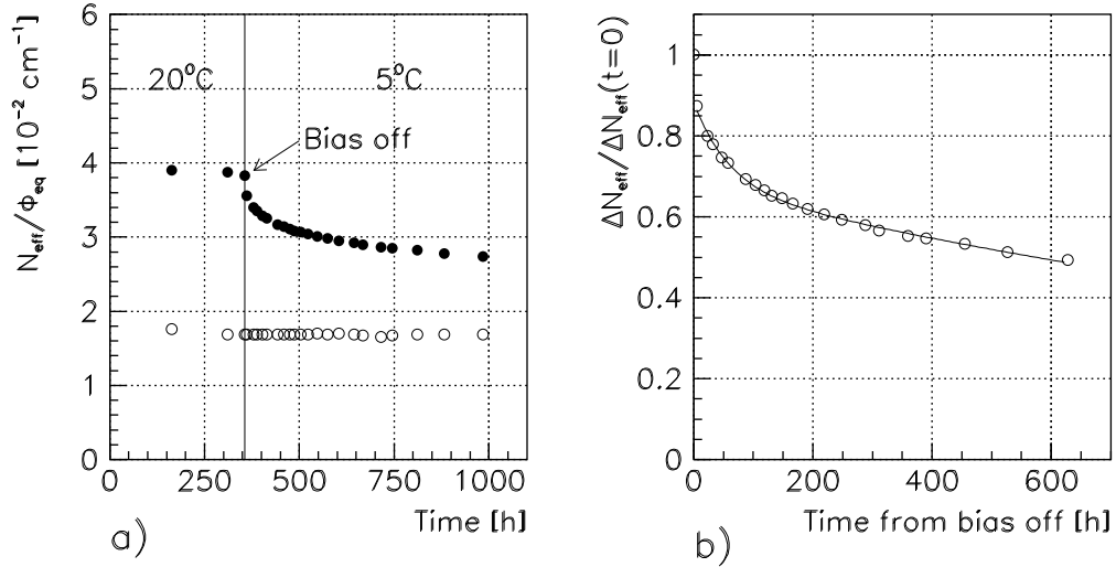
Figure 6.8: a) Time development of N_{eff} for the biased and unbiased diode from the pair BA4. They were kept at 20°C until the end of beneficial annealing. Then they were moved to 5°C and bias of the diode BA4B was switched off. b) Time development of the difference. Difference in N_{eff} normalised to the initial value is shown versus time from switching off the bias. Agreement of a two exponentials fit (eq. 6.2) with the measured data is also shown.
