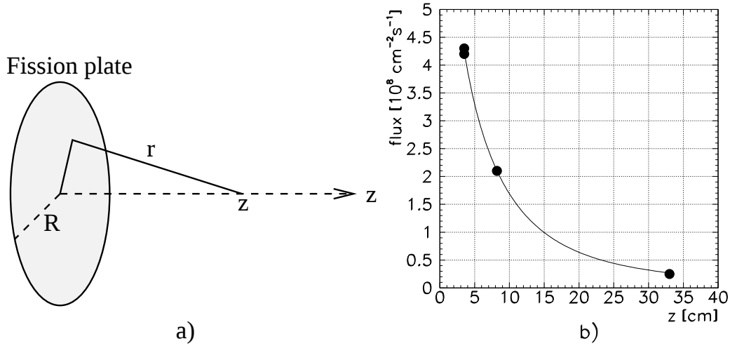
Figure 3.4: Dependence of the fast neutron flux on the distance from the fission plate. a) Schematical presentation of the setup. b) Comparison of measurements [36] and calculations.
