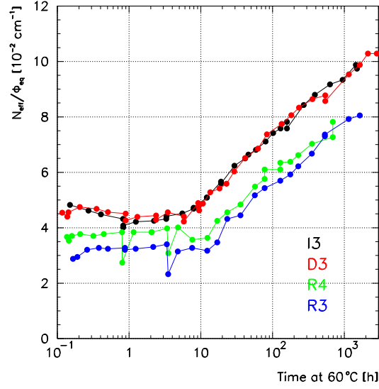
Figure 4.13: Comparison of N_{eff} development of planar (I3,D3) and MESA (R4,R3) samples after heating to 60°C.
