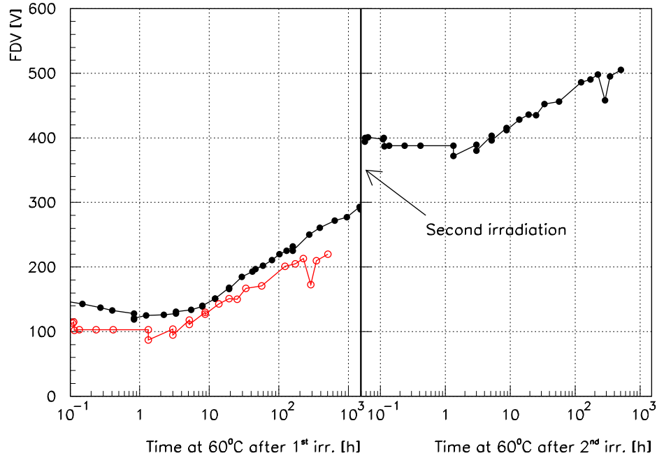
Figure 4.11: Time development of FDV for the diode I3 after the first and the second neutron irradiation ( 4.4 \cdot 10^{13} \text{ n/cm}^2 and 4.1 \cdot 10^{13} \text{ n/cm}^2 1 MeV neutron equivalent, respectively). Open circles are used to compare the effect of the first and the second irradiation. They represent the change in full depletion voltage induced by the second irradiation (i.e. FDV after second irradiation reduced for the value of the FDV before the second irradiation).
