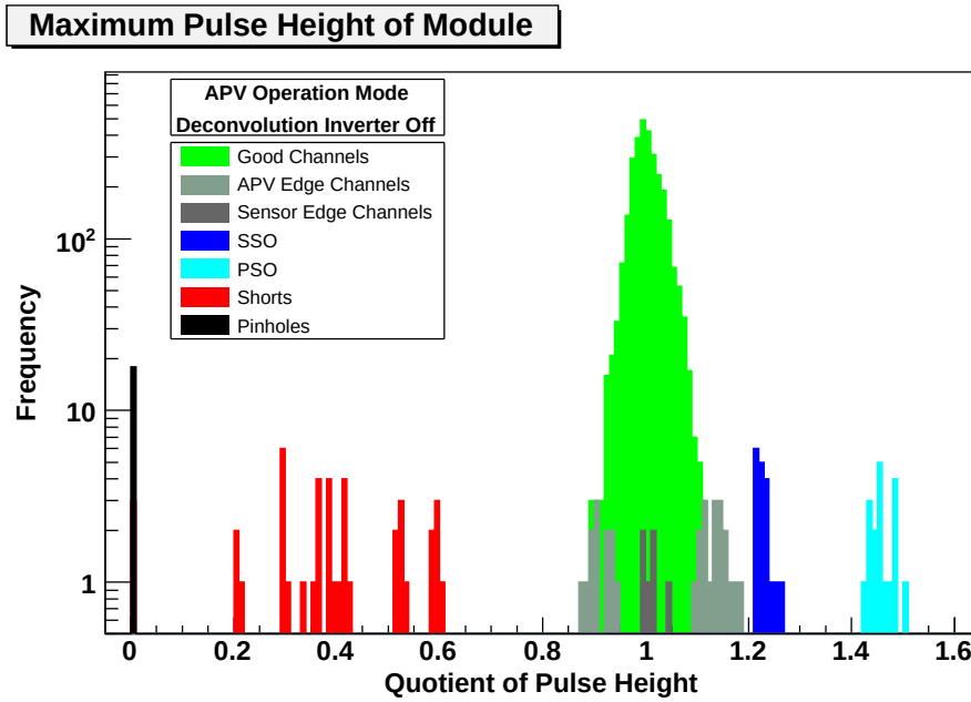
Figure 5.25: The maximum pulse height in deconvolution inverter off mode. The input capacitance of disconnected channels is lower compared to good channels. Thus the maximum pulse height is increased for these channels. The short circuited channels share part of the injected charge. Thus the pulse height of these channels is lower while the pulse height for pinholes is zero as the absolute pulse height is such small that no fit is applied to the data.
