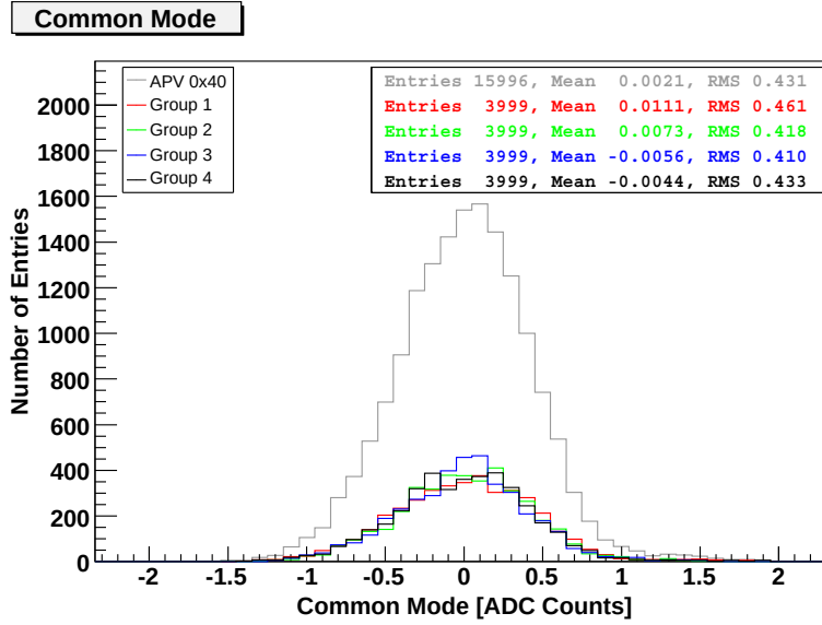
Figure 3.9: Common mode histogram for the four groups of channels of an APV and the sum of the the four distributions. The RMS of the histogram for the APV mainly depends on the radio frequency shielding and the grounding scheme of the test stand.
