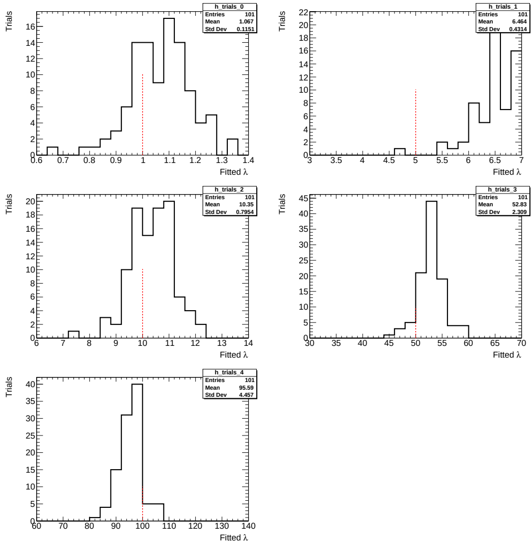
Figure 6.25: Distribution of the \lambda values fitted for each of the 5 width points using a bootstrap with 101 trials. The dotted red line represents the reference value.
