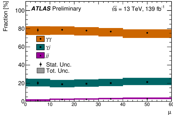
Figure 5.3: The purity of selected diphoton events, measured in bins of \mu (the mean number of interactions per bunch crossing). The fraction of \gamma\gamma , \gamma j and j j events in each \mu region is measured using the procedure described in Section 5.7.
