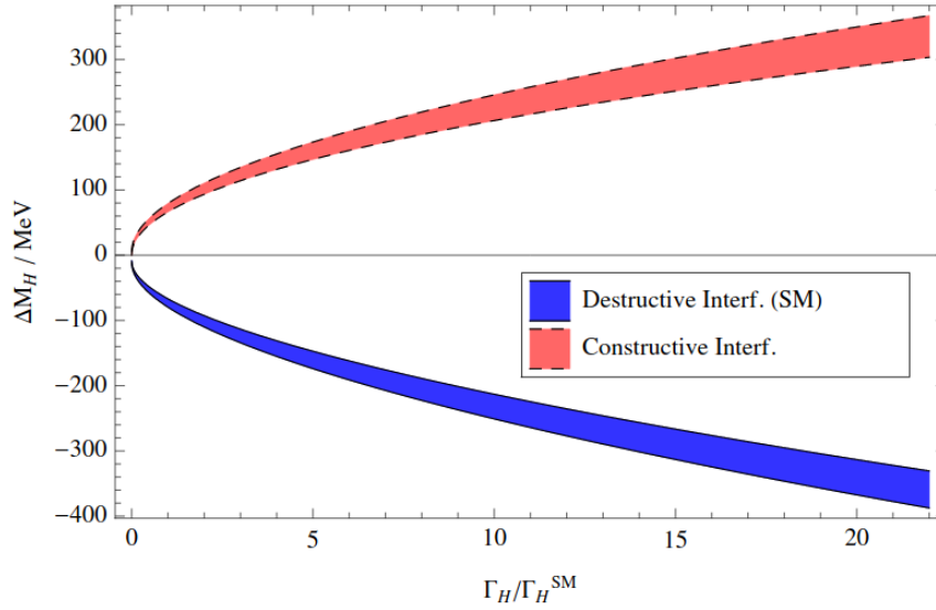
Figure 1.10: Higgs mass shift as a function of the Higgs width (From Ref.[58]).
