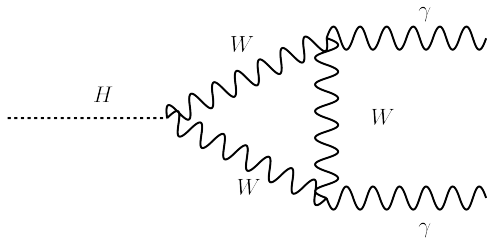
(a) Diphoton decay mediated by a loop of heavy gauge bosons.
