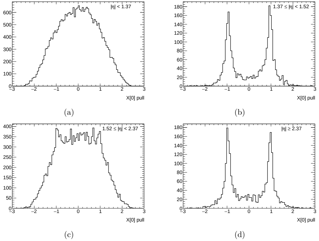
Figure 4.21: Distributions in various regions of the calorimeter of the pull values of the ramp intercept parameter X[0] .
