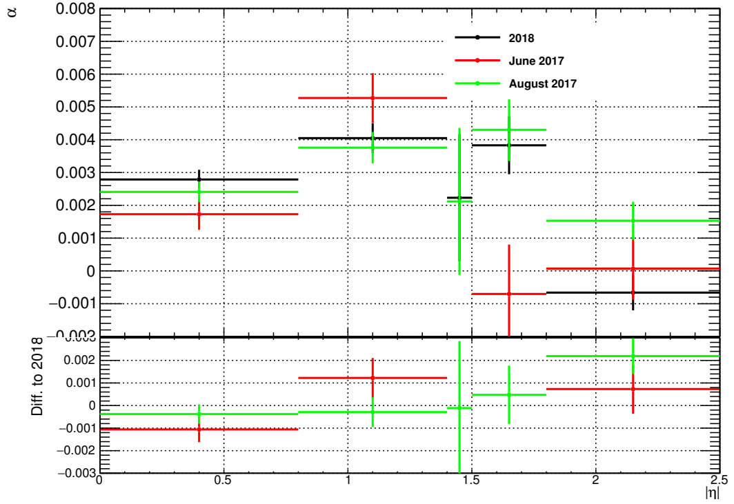
Figure 4.45: Values of the scale factors in the 5 |\eta| bins using 2018 data and 2017 data. The bottom panel shows the difference with respect to 2018 data.
