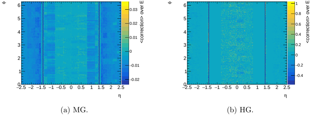
Figure 4.50: Map of the correction in the \eta - \phi space of the second layer of the LAr calorimeter.
