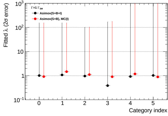
Figure 6.23: Results of the injection test and comparison with the nominal Asimov fit results per category.
