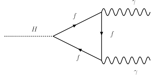
(b) Diphoton decay mediated by a heavy fermion loop.
