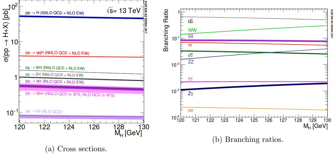
Figure 1.6: Cross sections as a function of m_H for different production modes and corresponding order in perturbation theory at which they have been calculated (left). Branching ratios of the Higgs boson decaying into different final states as a function of m_H (right) [42].
