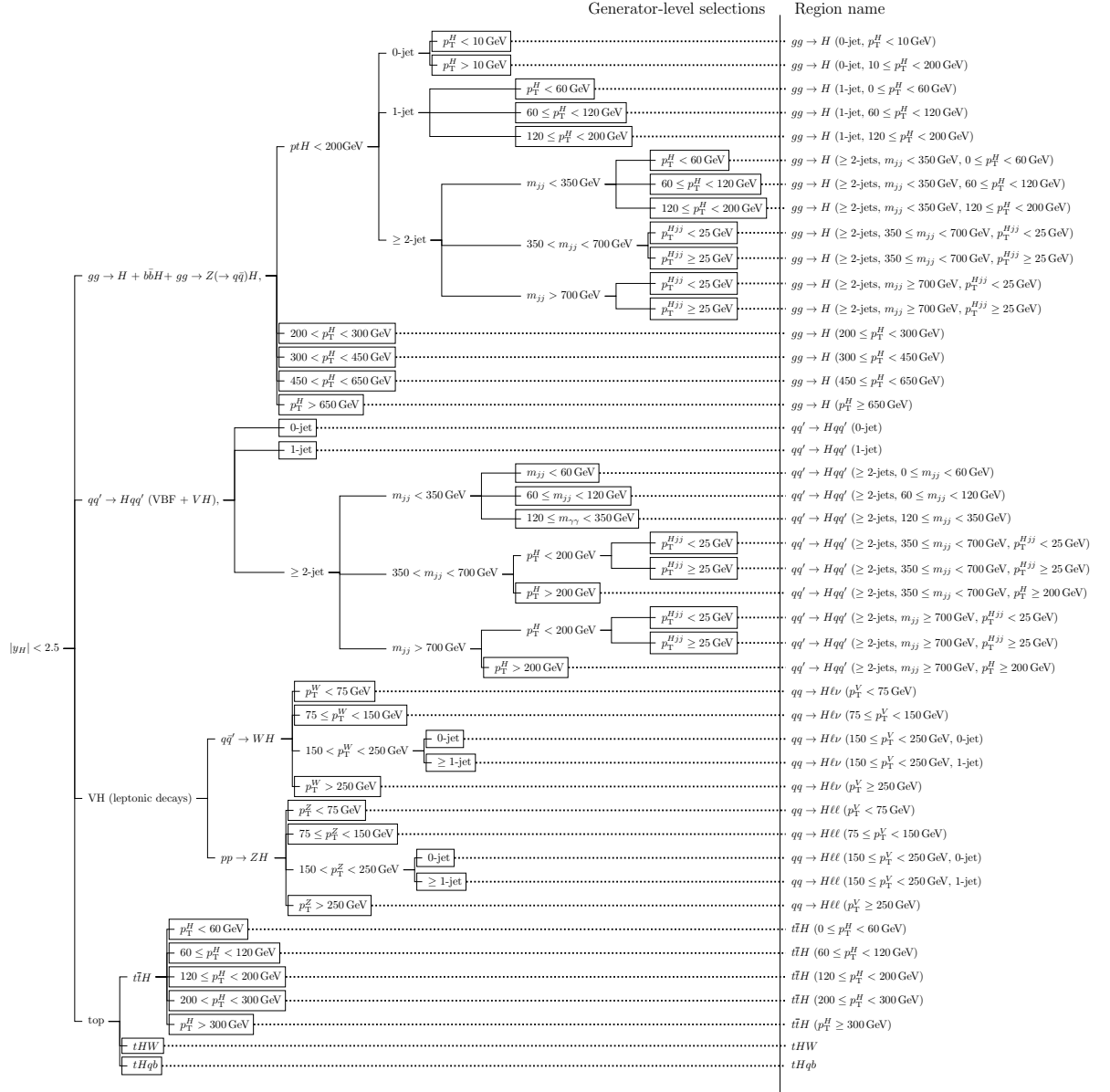
Figure 5.1: Summary of the STXS measurement regions considered in the analysis. The left part of the plot shows the selections applied on the generator-level quantities of simulated signal events, with the selections applied sequentially along the branches of the graph. The final selection for each region is indicated by a box, and the name of each region, used in the rest of this chapter, is shown on the right.
