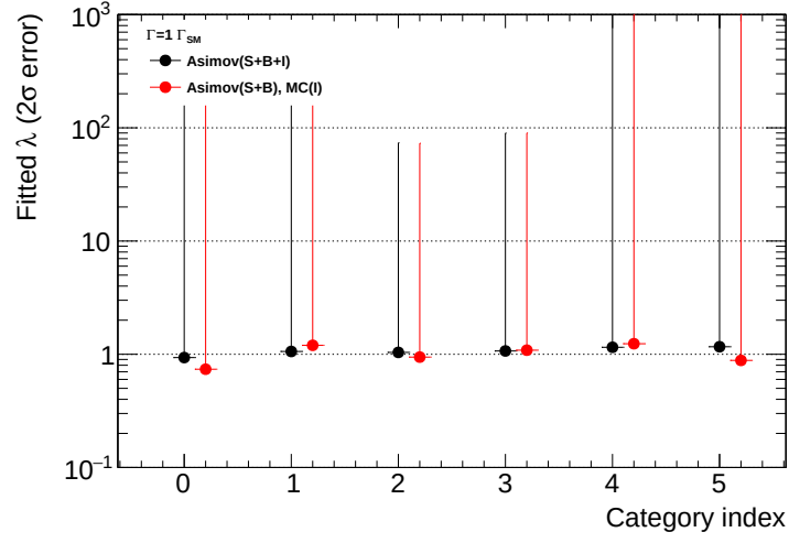
Figure A.6: Results of the injection test and comparison with the nominal Asimov fit results per category, using the alternative parametrization.
