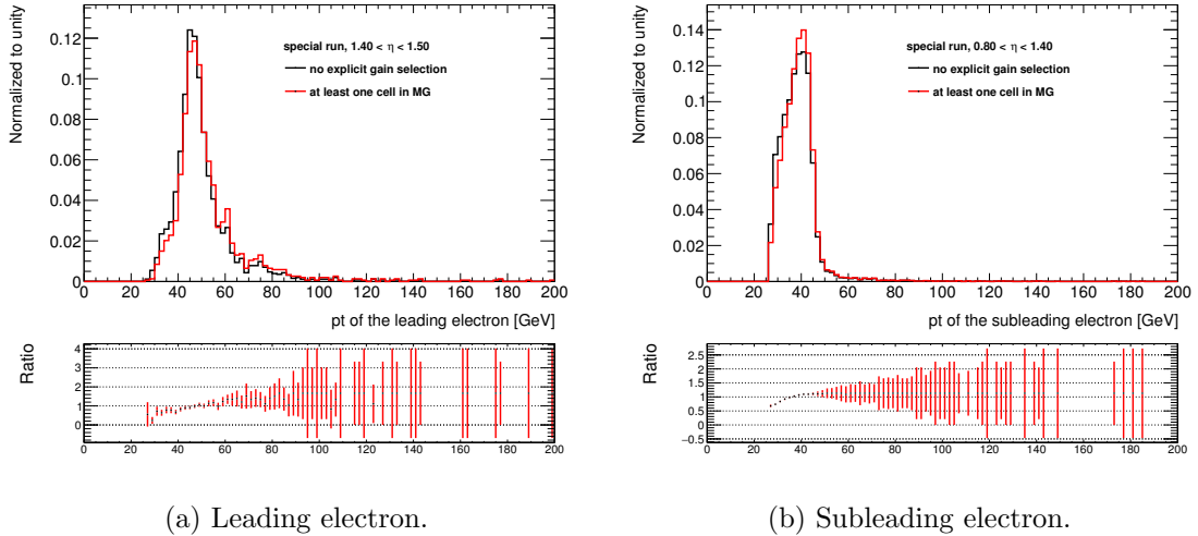
Figure 4.42: p_T distributions of the electrons in the special run for the two |\eta| regions with the highest fraction of contaminated electrons. The nominal case (black line) is compared to the configuration where the special run is composed only by events reconstructed in MG (red line). Bottom panels show the ratio between the two distributions.
