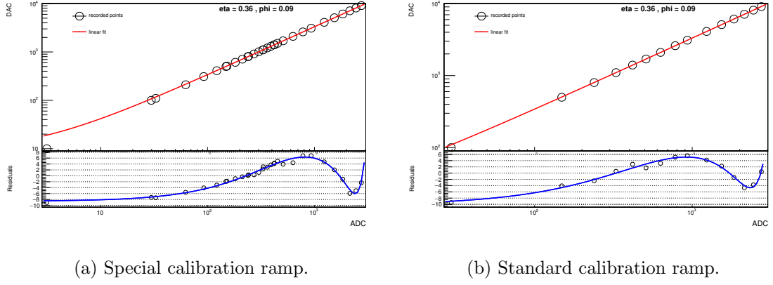
Figure 4.53: Special ramps are recorded on average with twice as many points as the standard ramps in the low DAC region.
