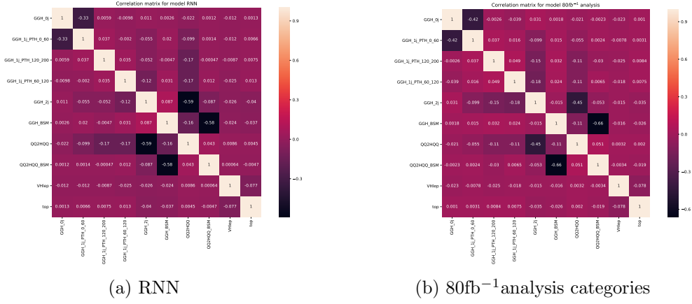
Figure 5.15: Correlations among the 10 fitted POIs obtained using the categorization proposed in this section (a) and the categorization used for the 80fb^{-1} analysis (b).
