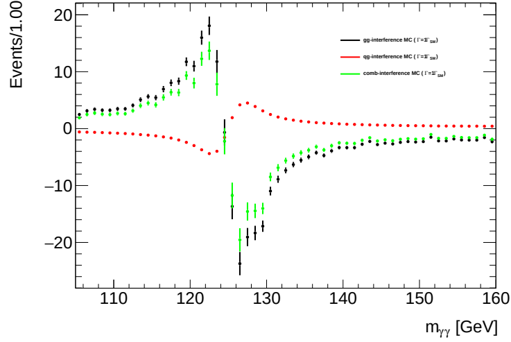
Figure 6.26: Distribution of m_{\gamma\gamma} for the gg -interference (black), qq -interference (red) and their combination (green). Diphoton selection is applied.
