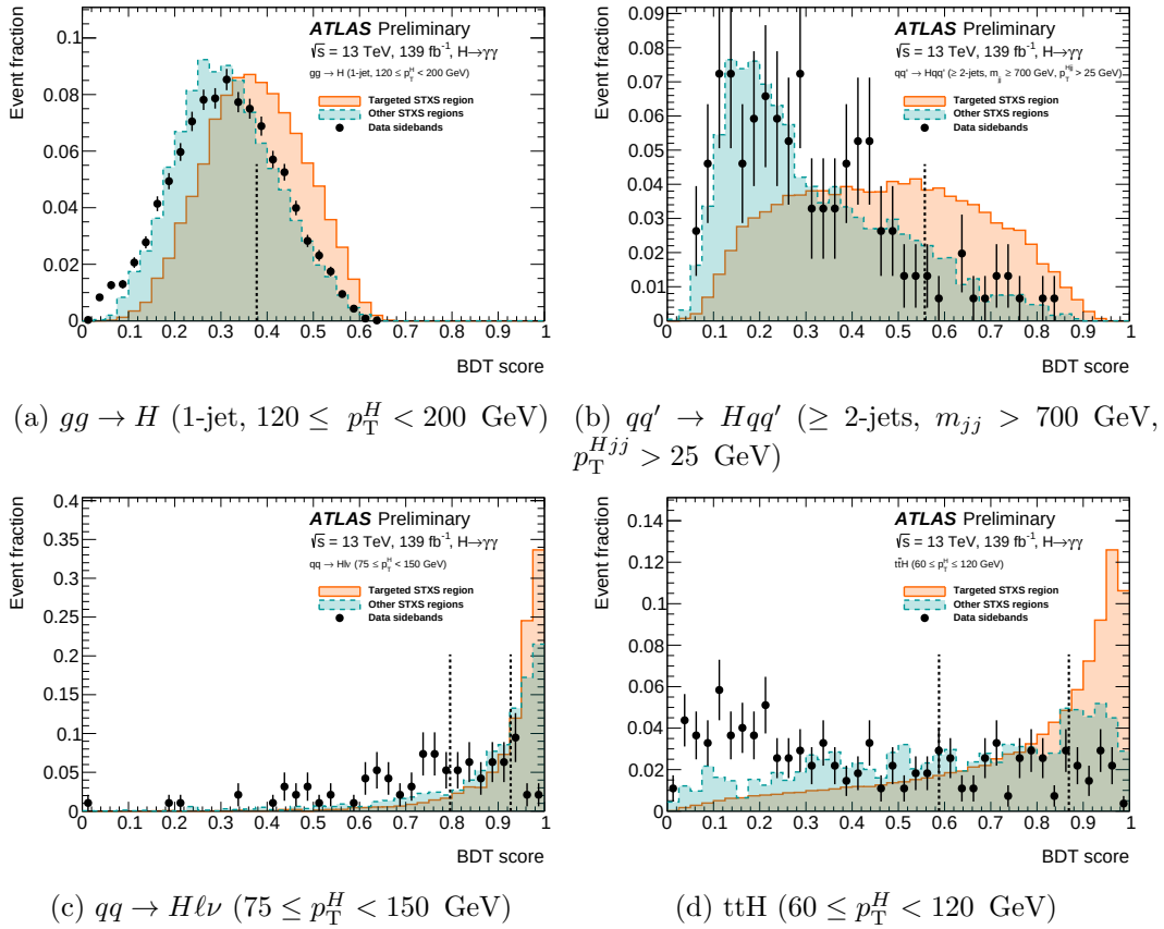
Figure 5.5: Binary BDT discriminant distributions in four representative STXS classes. For each class, the binary BDT discriminant distribution is shown for the target STXS region (solid), other STXS regions (dashed), and background (dots) represented by the events in the diphoton mass sidebands ( 105 < m_{\gamma\gamma} < 120 GeV or 130 < m_{\gamma\gamma} < 160 GeV). The vertical lines delimit categories used in the analysis for each class.
